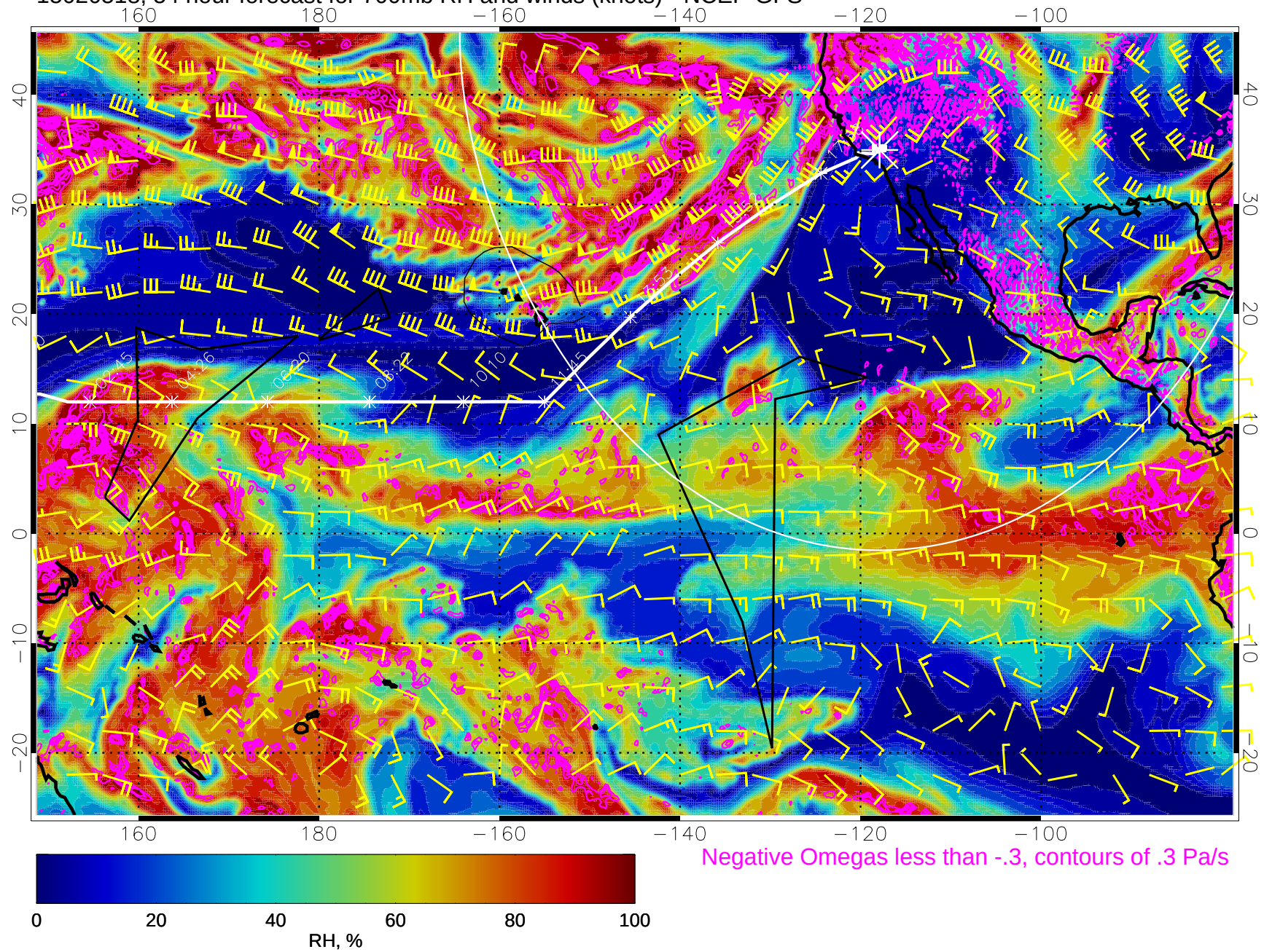
15020518, 54 hour forecast for 700mb RH and winds (knots) - NCEP GFS
