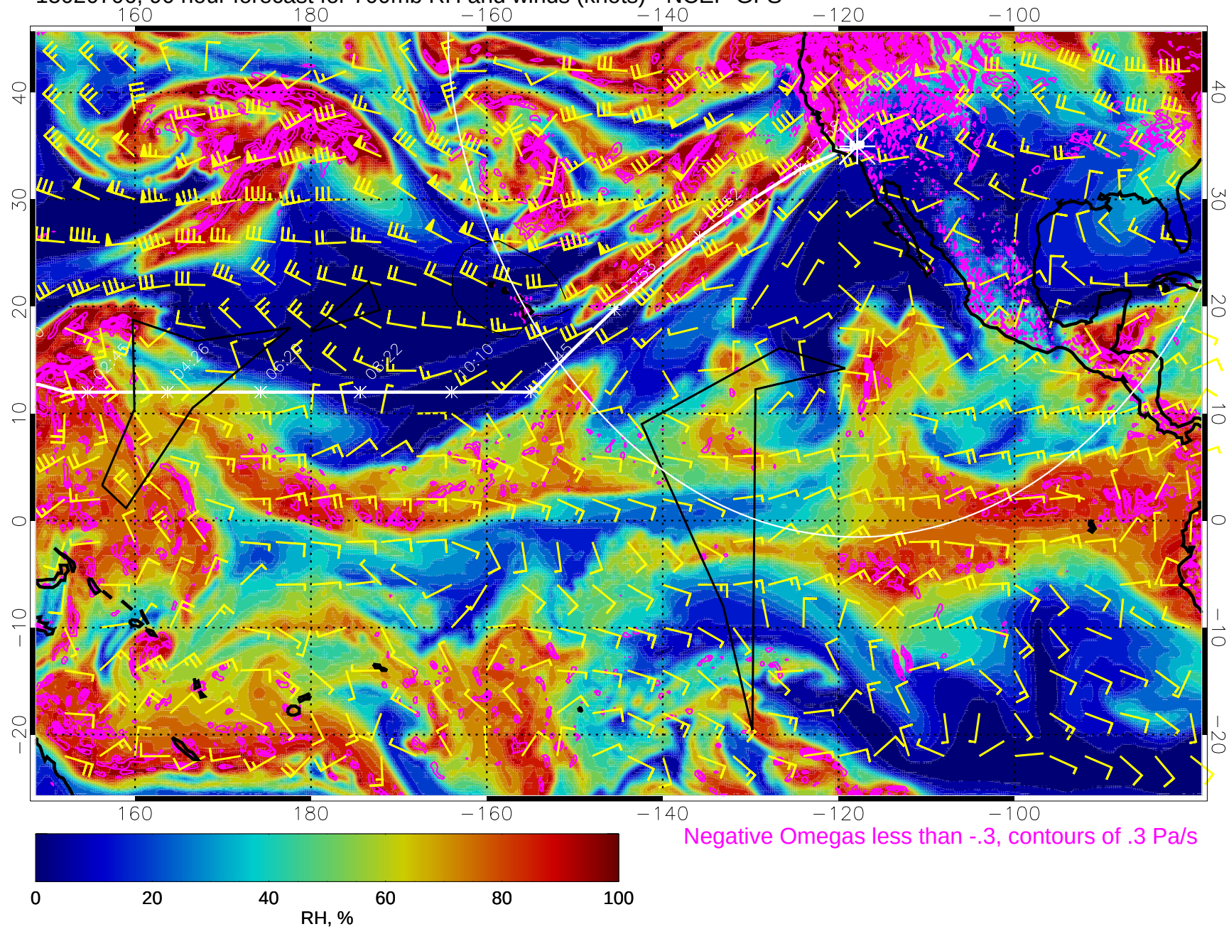
15020706, 90 hour forecast for 700mb RH and winds (knots) - NCEP GFS
