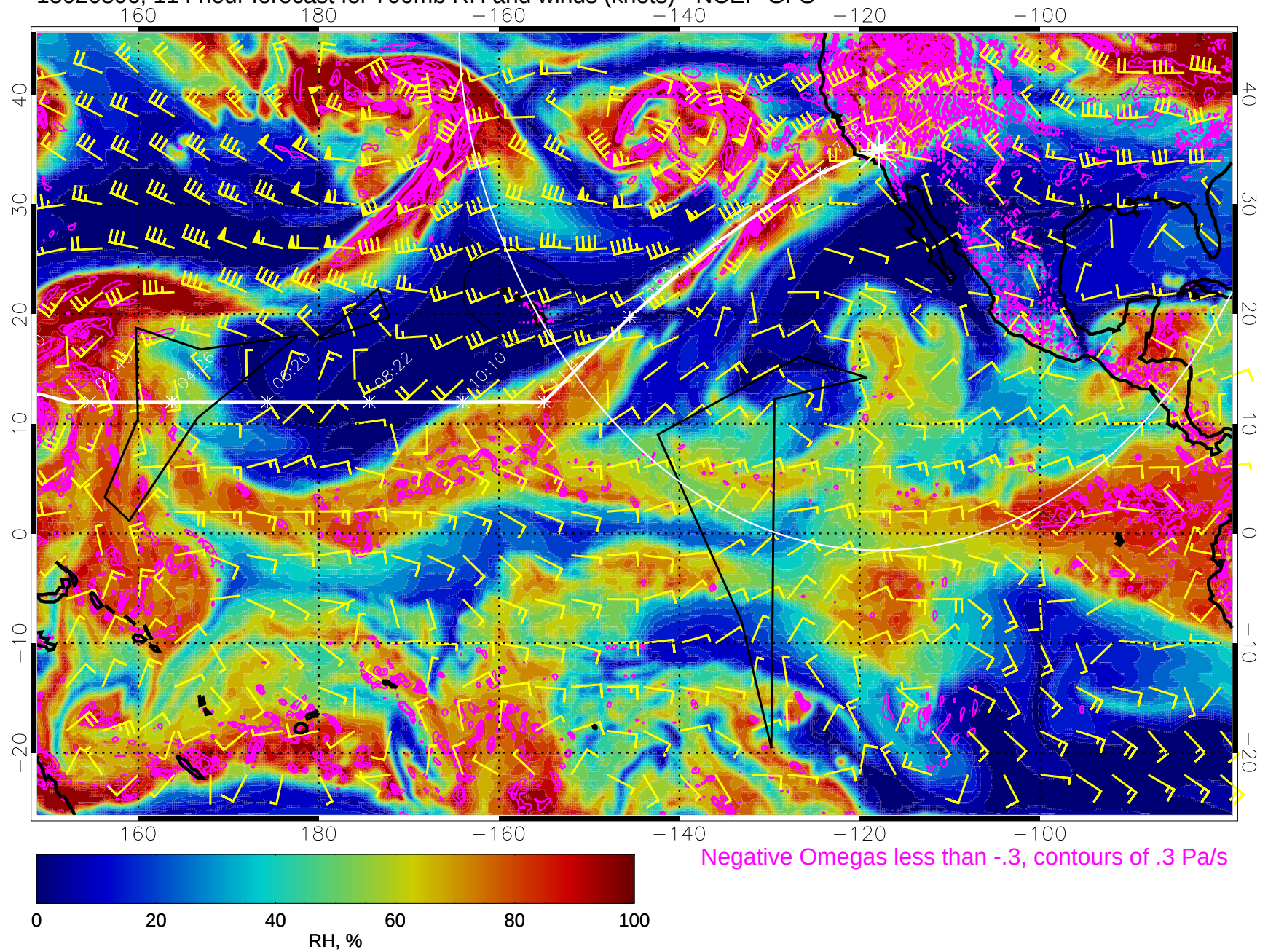
15020806, 114 hour forecast for 700mb RH and winds (knots) - NCEP GFS
