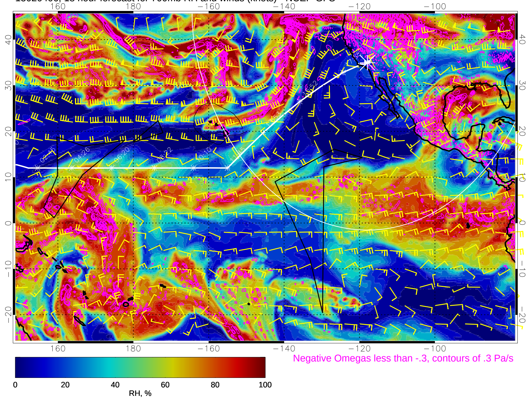
15020406, 18 hour forecast for 700mb RH and winds (knots) - NCEP GFS
