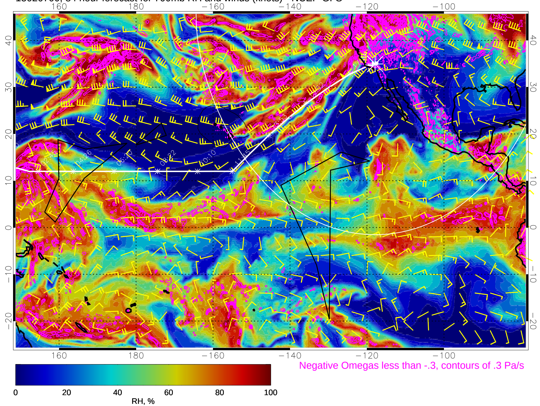
15020700, 84 hour forecast for 700mb RH and winds (knots) - NCEP GFS
