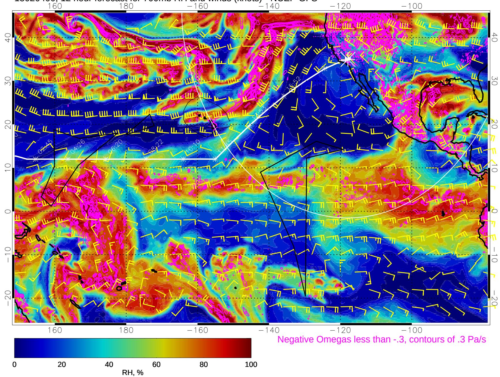
15020400, 12 hour forecast for 700mb RH and winds (knots) - NCEP GFS
