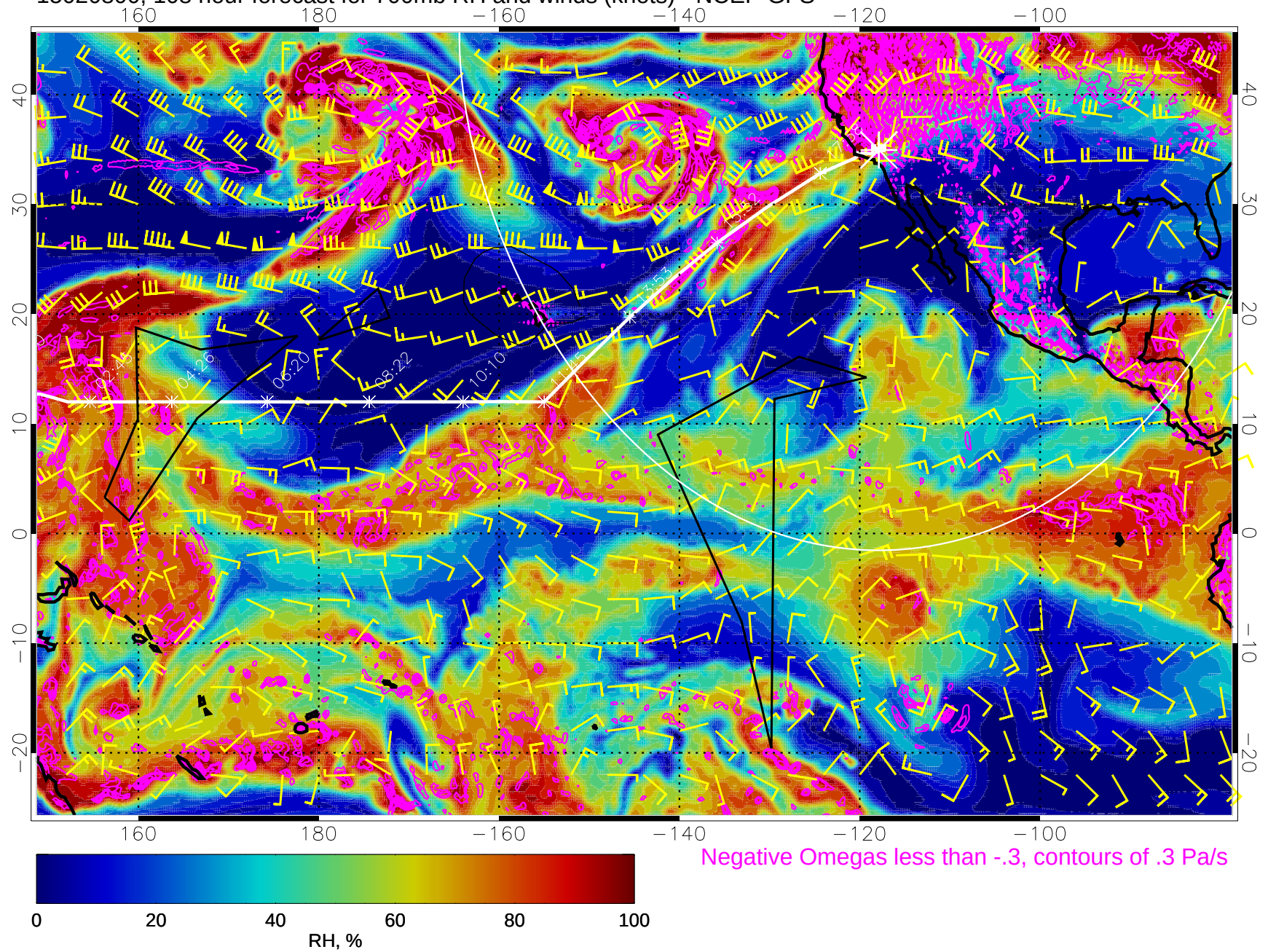
15020800, 108 hour forecast for 700mb RH and winds (knots) - NCEP GFS
