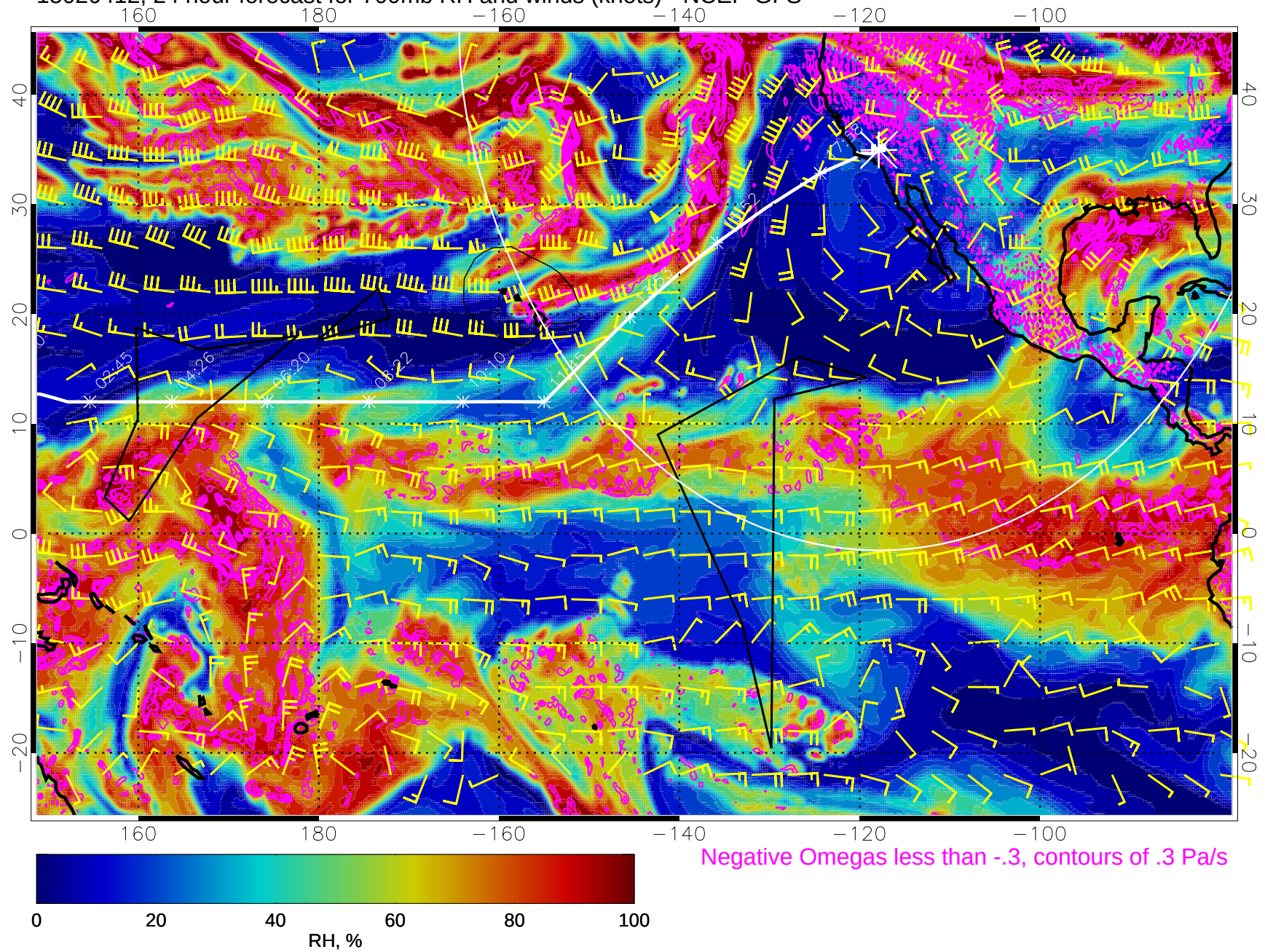
15020412, 24 hour forecast for 700mb RH and winds (knots) - NCEP GFS
