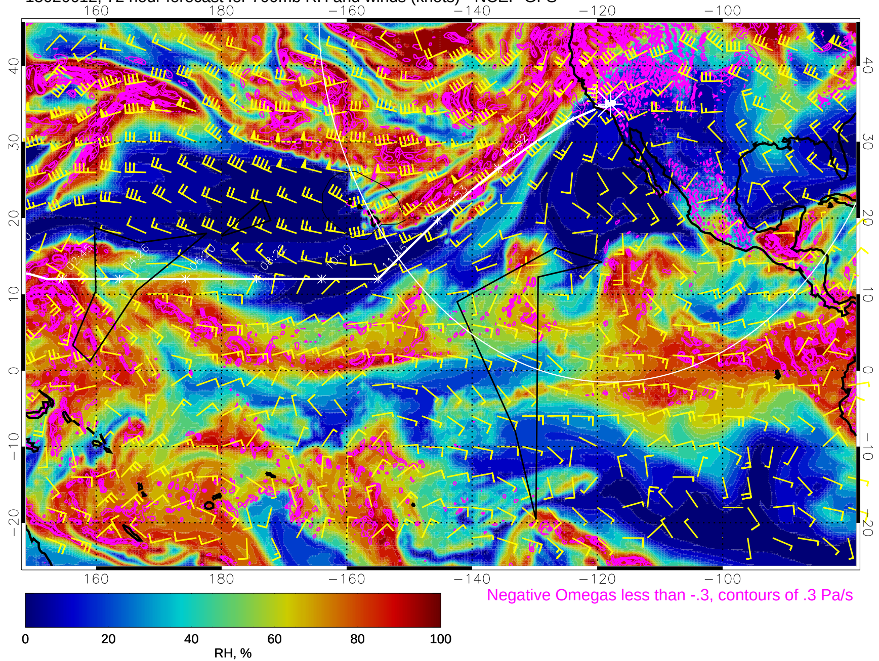
15020612, 72 hour forecast for 700mb RH and winds (knots) - NCEP GFS
