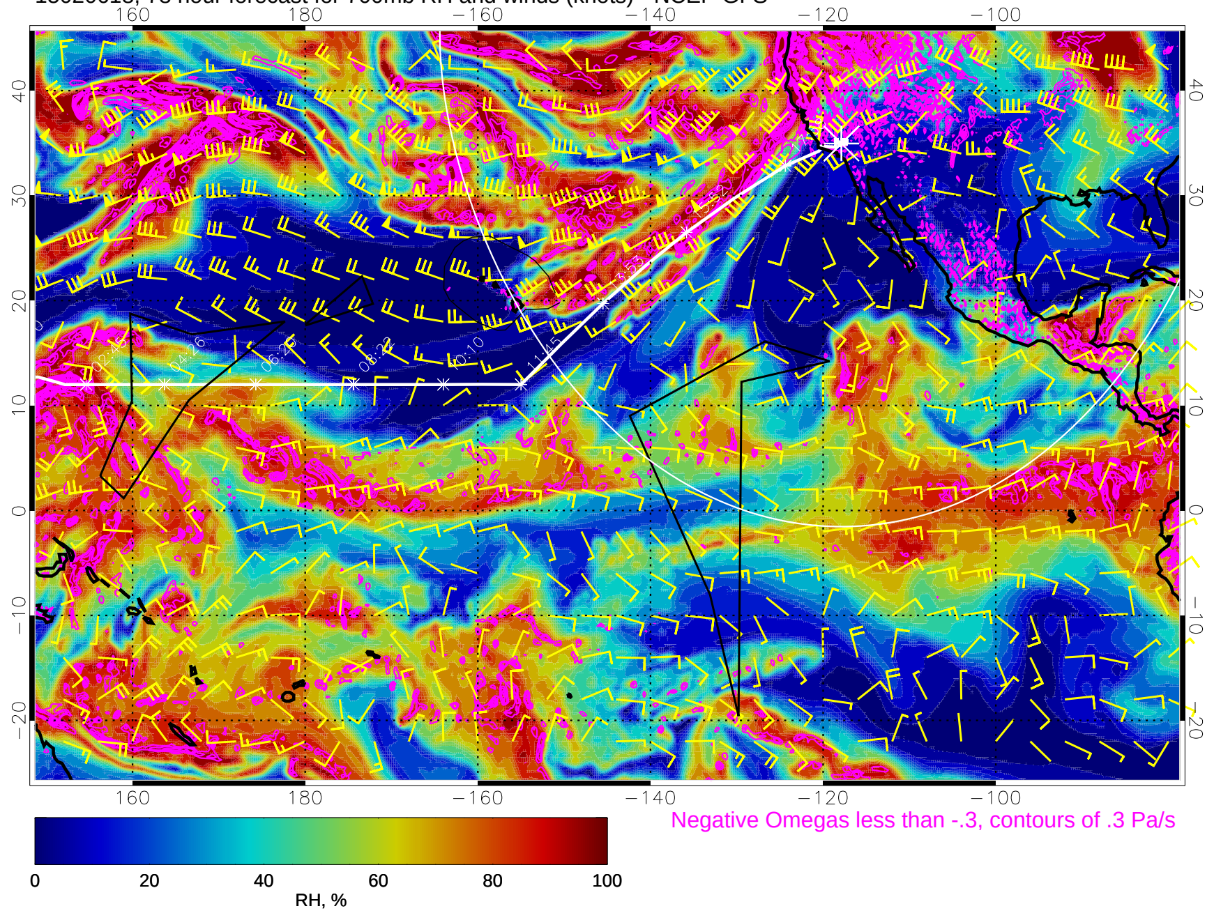
15020618, 78 hour forecast for 700mb RH and winds (knots) - NCEP GFS
