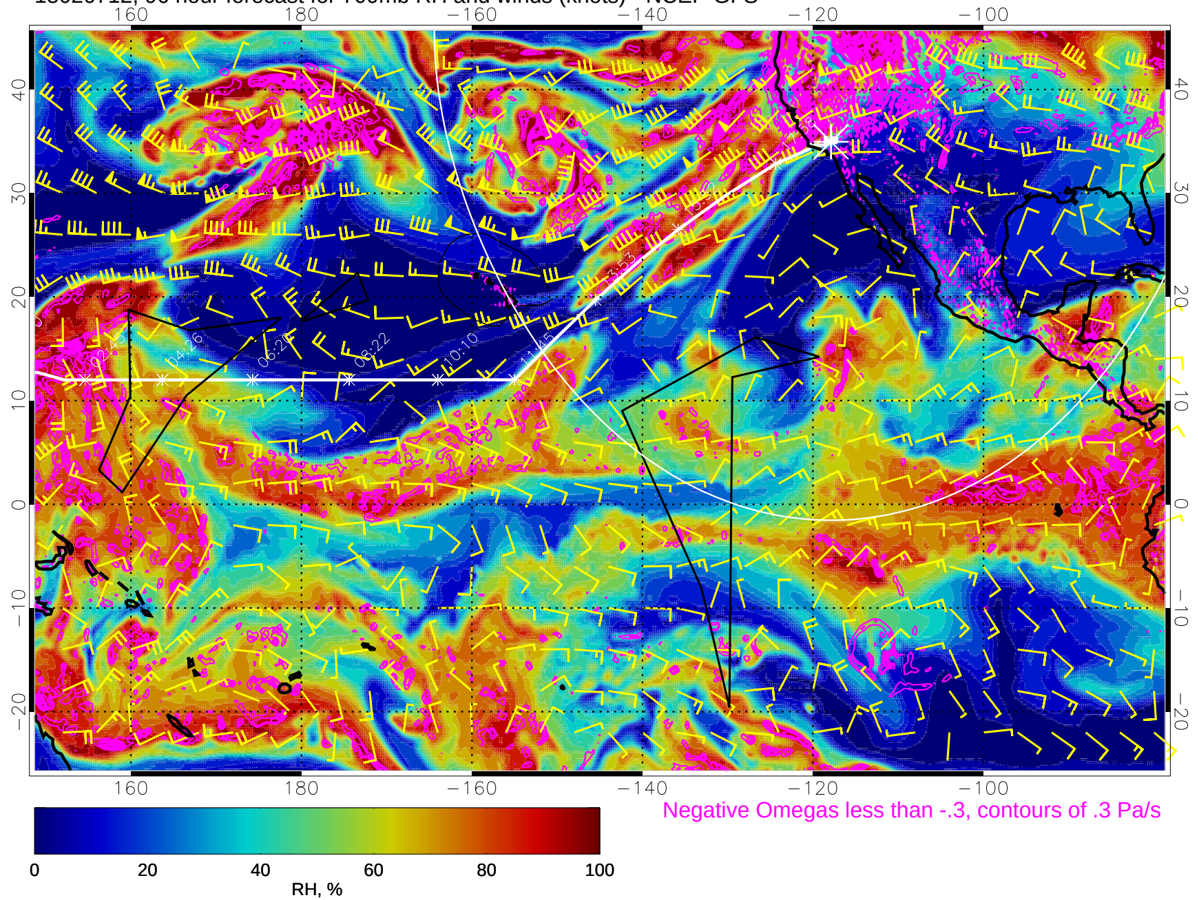
15020712, 96 hour forecast for 700mb RH and winds (knots) - NCEP GFS
