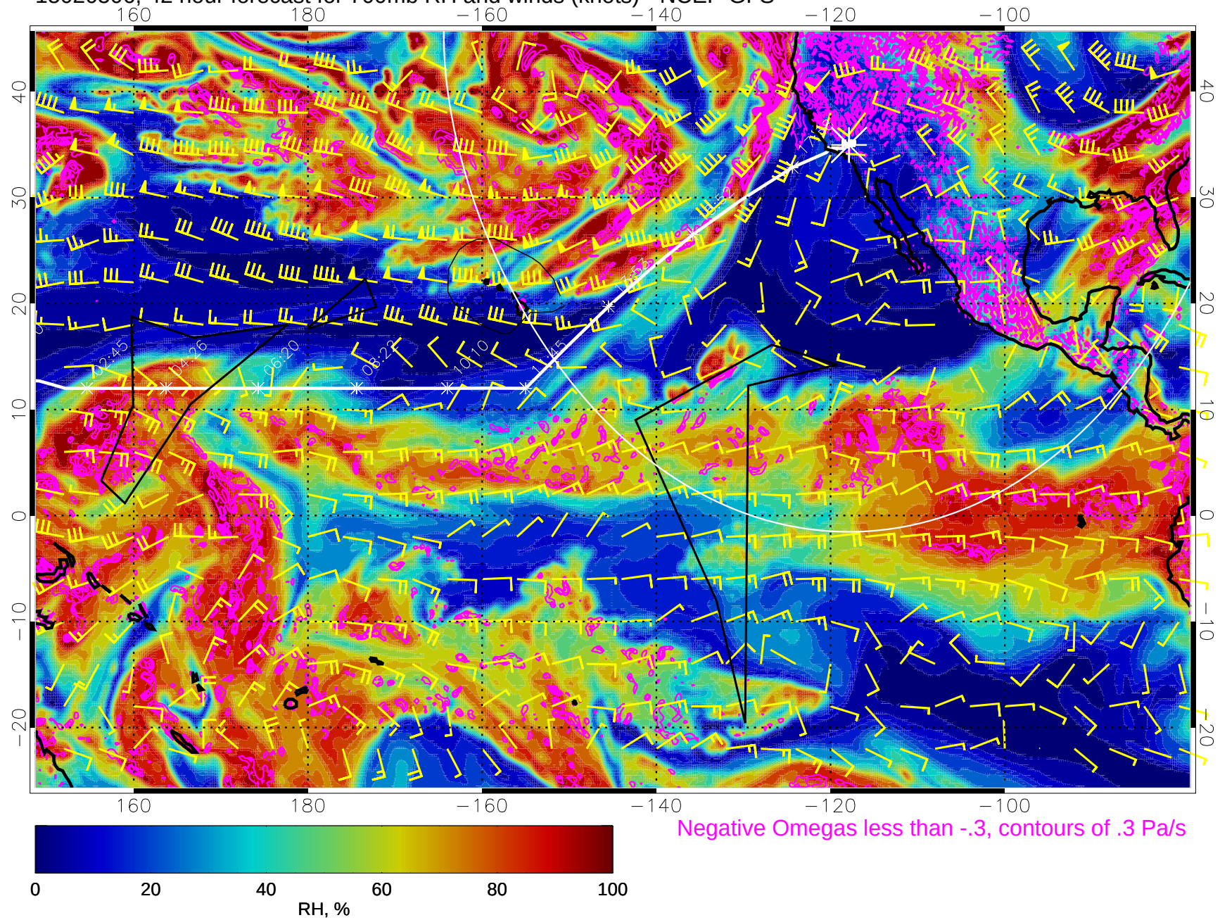
15020506, 42 hour forecast for 700mb RH and winds (knots) - NCEP GFS
