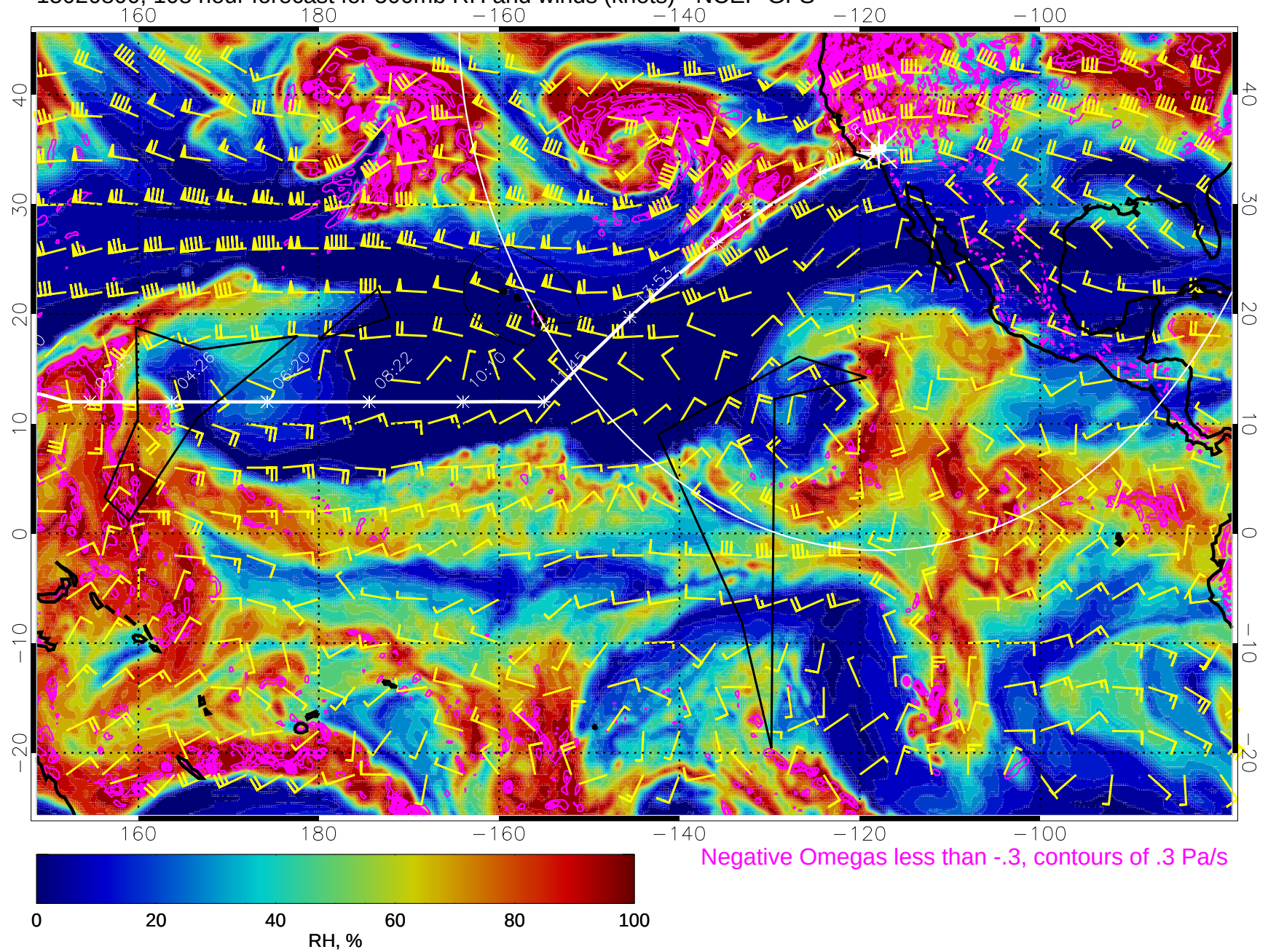
15020800, 108 hour forecast for 500mb RH and winds (knots) - NCEP GFS
