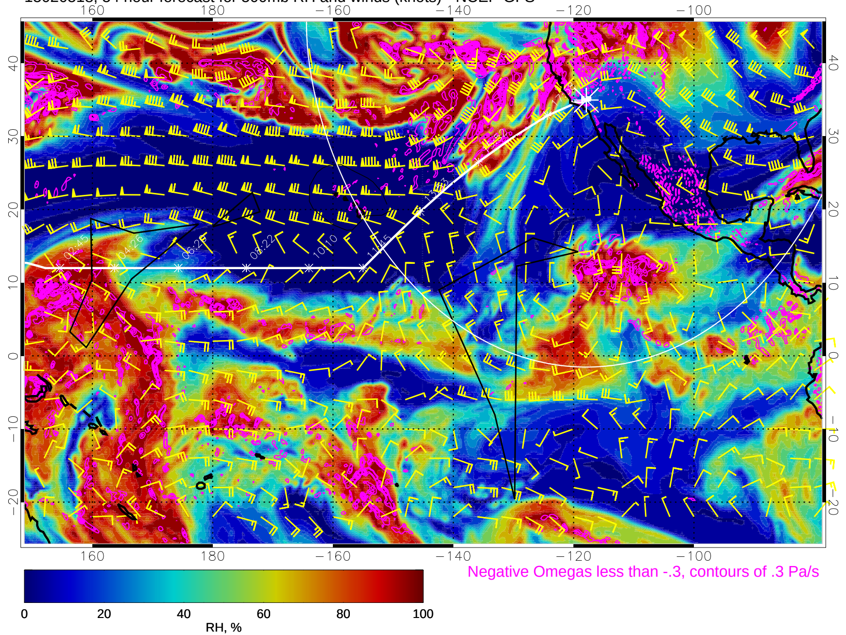
15020518, 54 hour forecast for 500mb RH and winds (knots) - NCEP GFS
