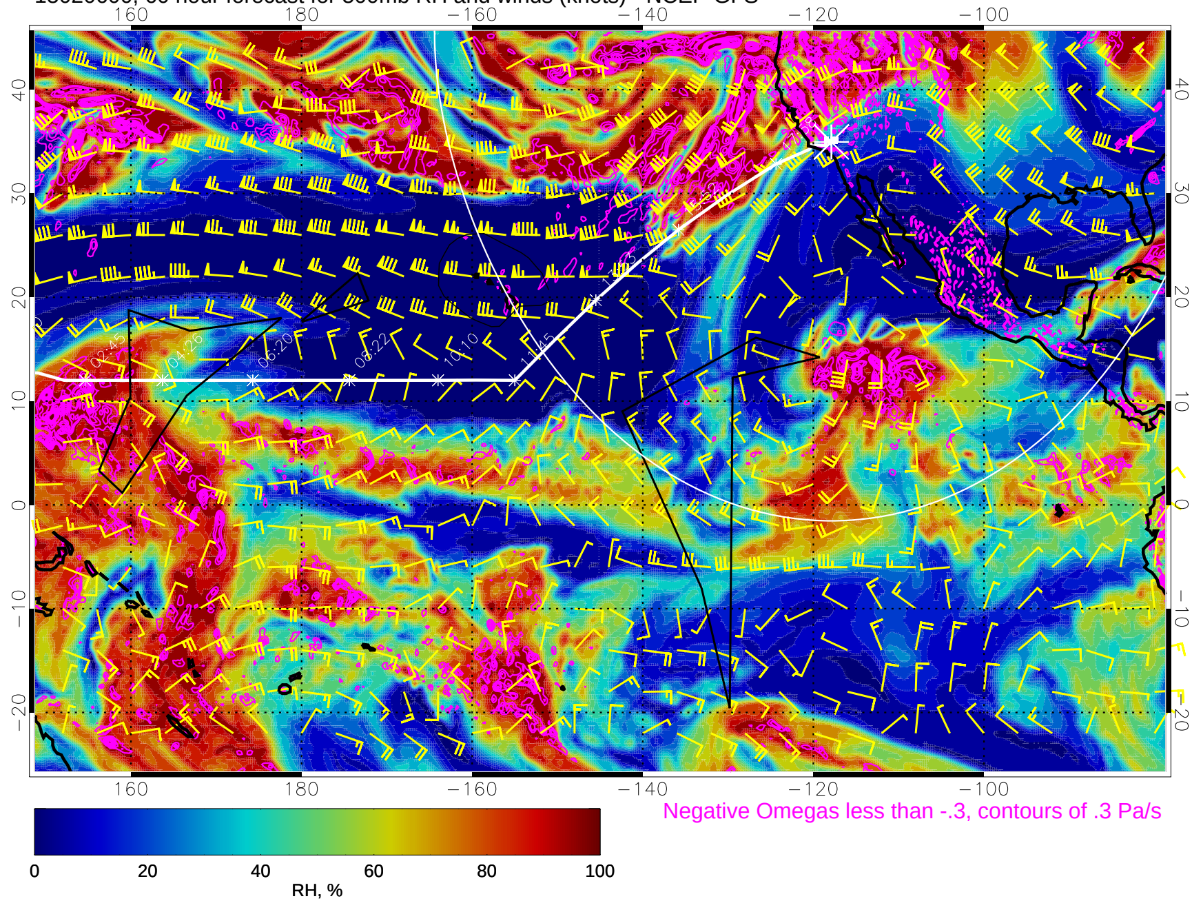
15020600, 60 hour forecast for 500mb RH and winds (knots) - NCEP GFS
