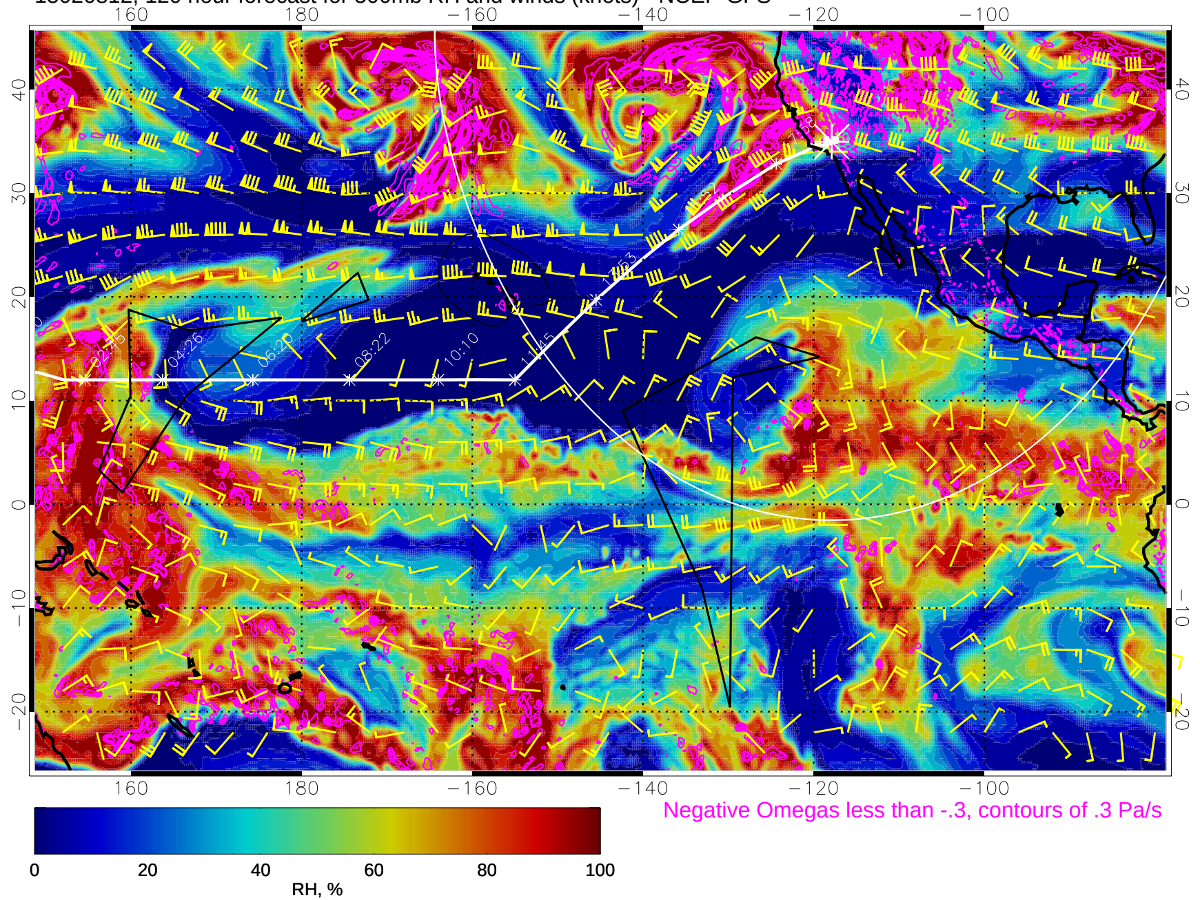
15020812, 120 hour forecast for 500mb RH and winds (knots) - NCEP GFS
