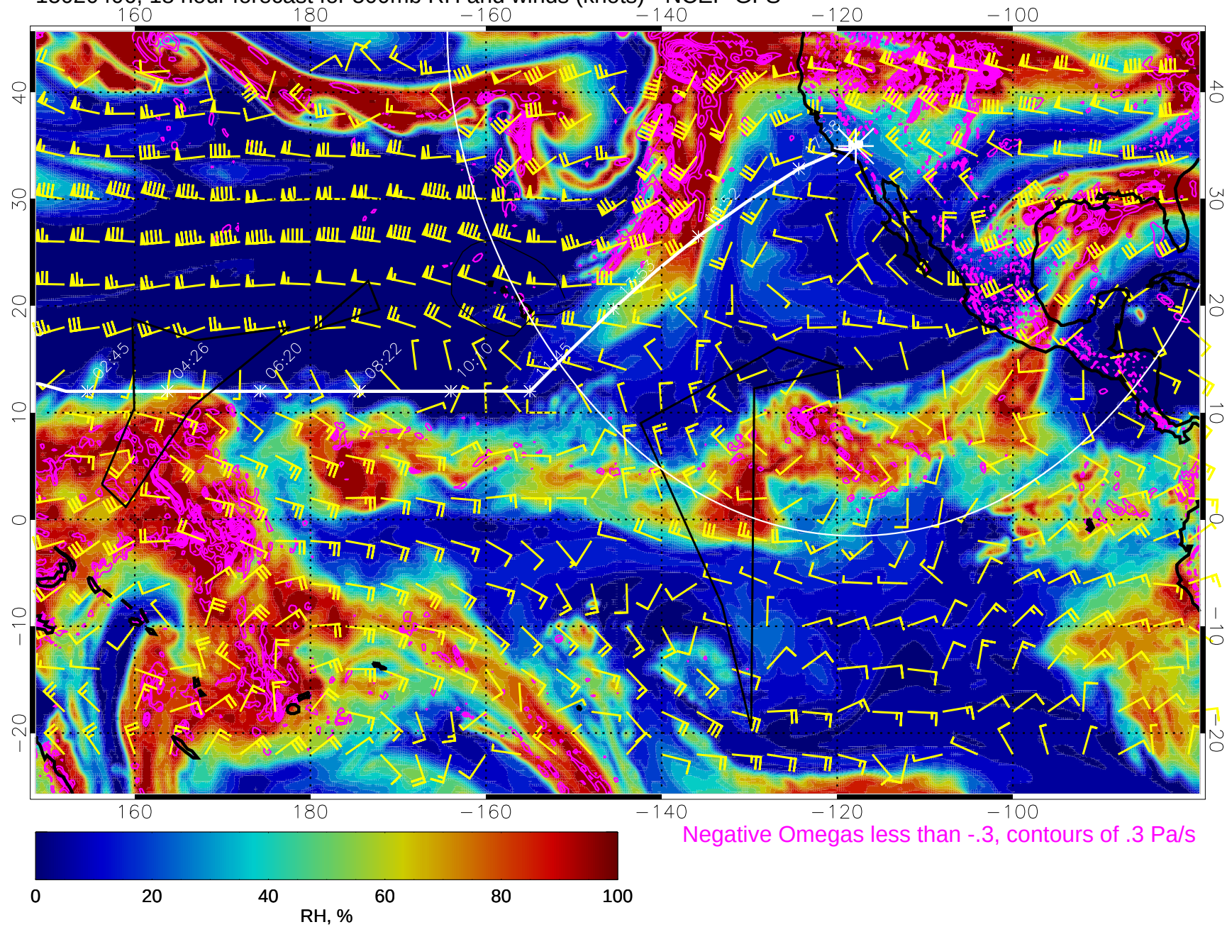
15020406, 18 hour forecast for 500mb RH and winds (knots) - NCEP GFS
