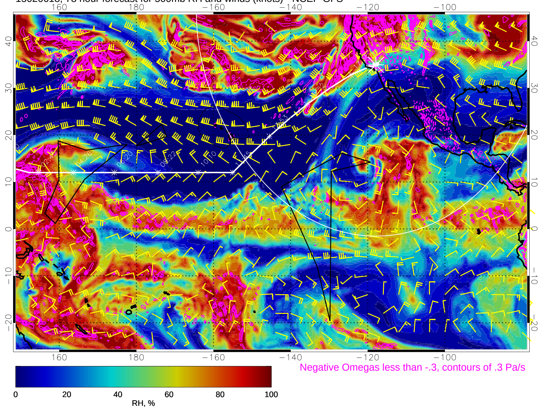
15020618, 78 hour forecast for 500mb RH and winds (knots) - NCEP GFS
