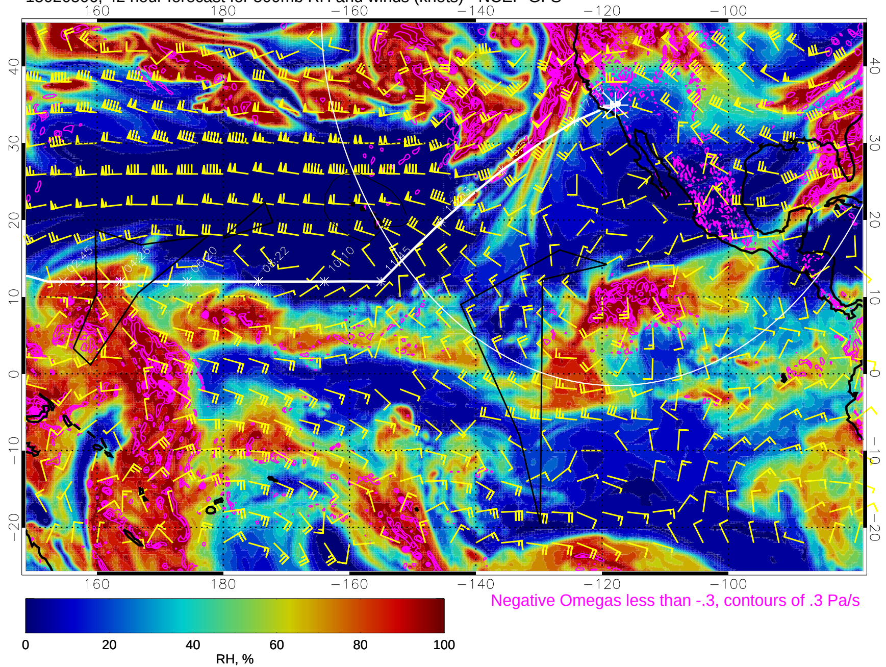
15020506, 42 hour forecast for 500mb RH and winds (knots) - NCEP GFS
