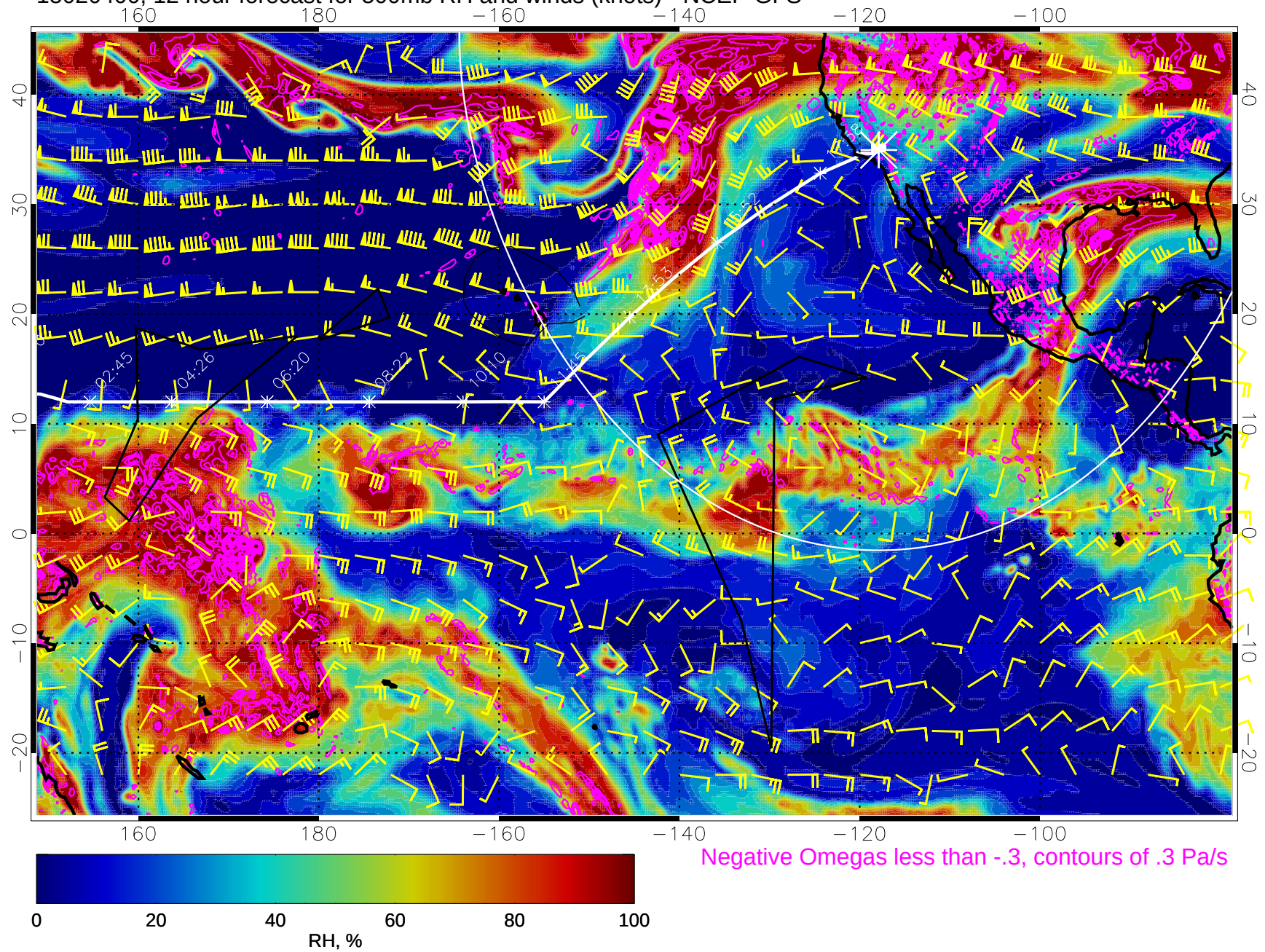
15020400, 12 hour forecast for 500mb RH and winds (knots) - NCEP GFS
