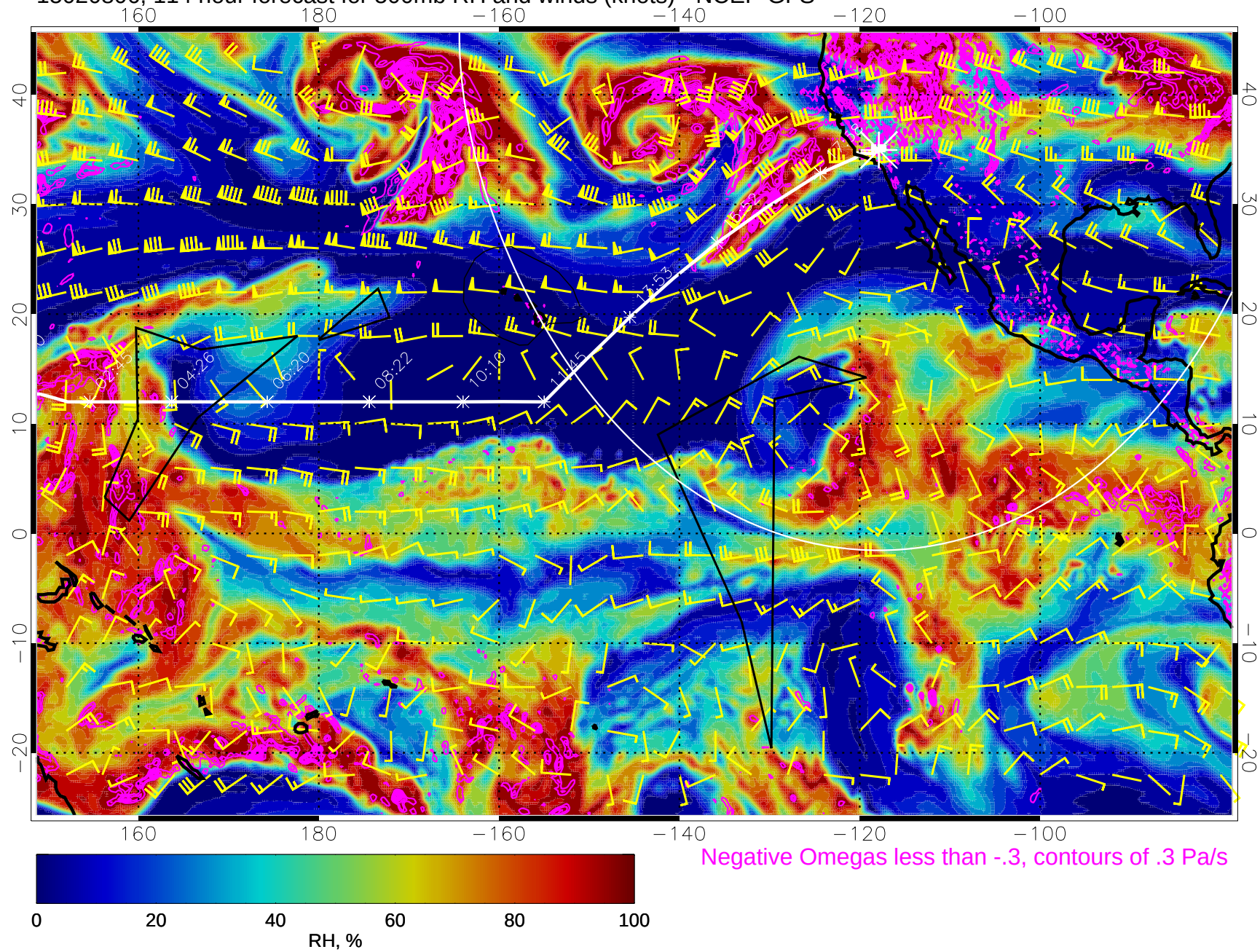
15020806, 114 hour forecast for 500mb RH and winds (knots) - NCEP GFS
