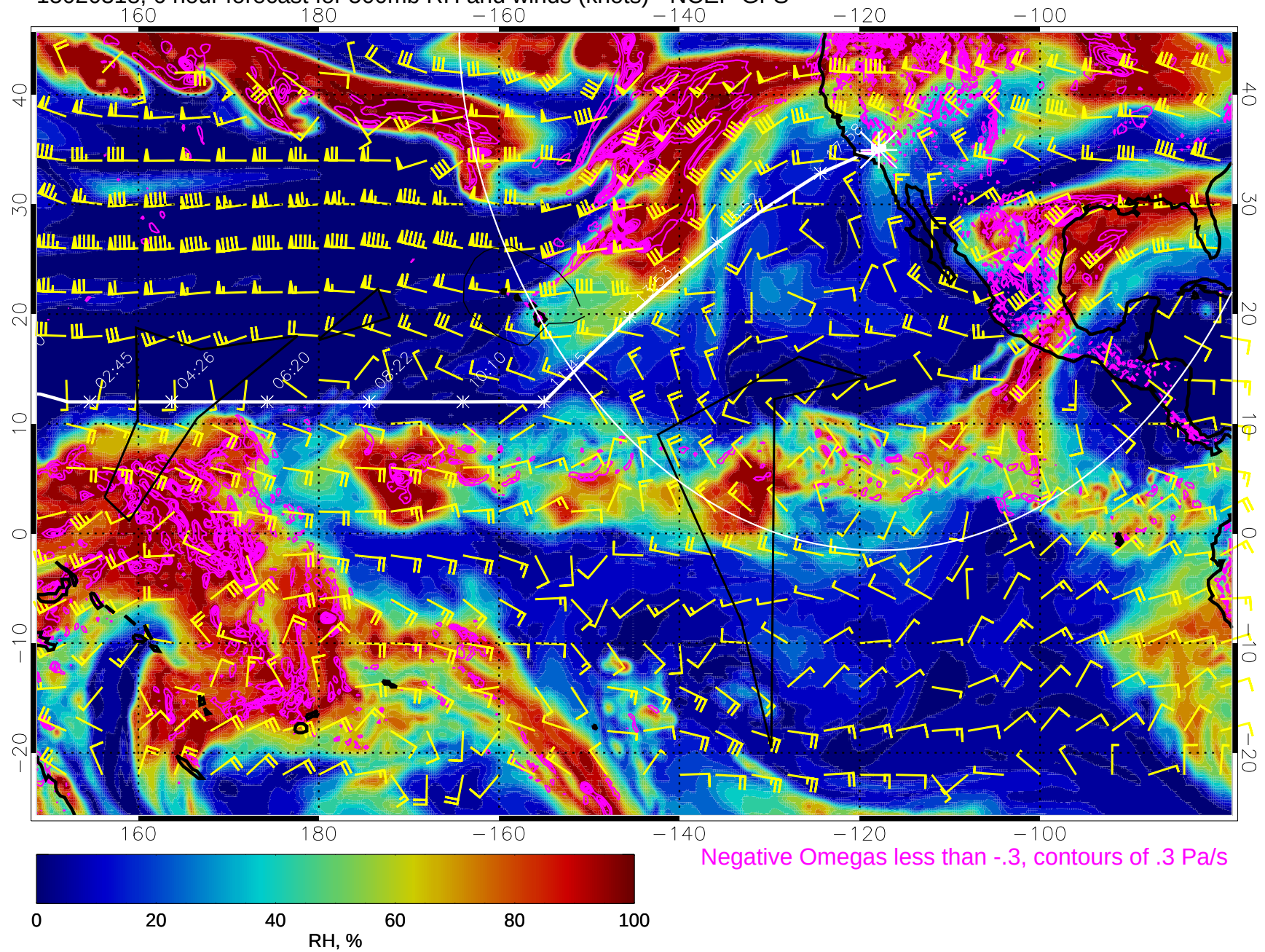
15020318, 6 hour forecast for 500mb RH and winds (knots) - NCEP GFS
