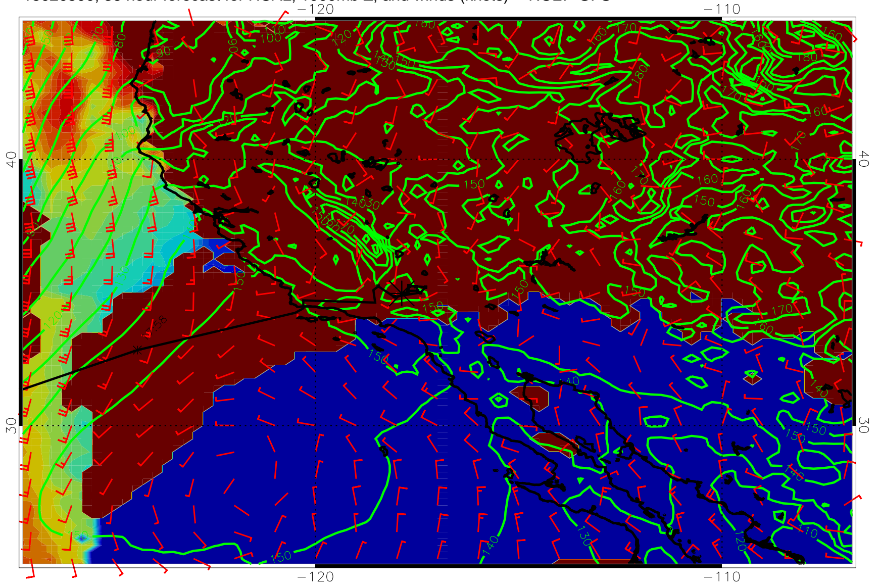
15020500, 36 hour forecast for HCAL, 1000mb Z, and winds (knots) -- NCEP GFS
