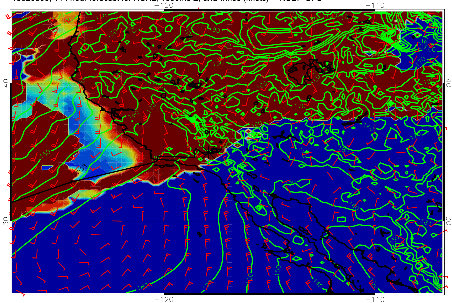
15020806, 114 hour forecast for HCAL, 1000mb Z, and winds (knots) -- NCEP GFS
