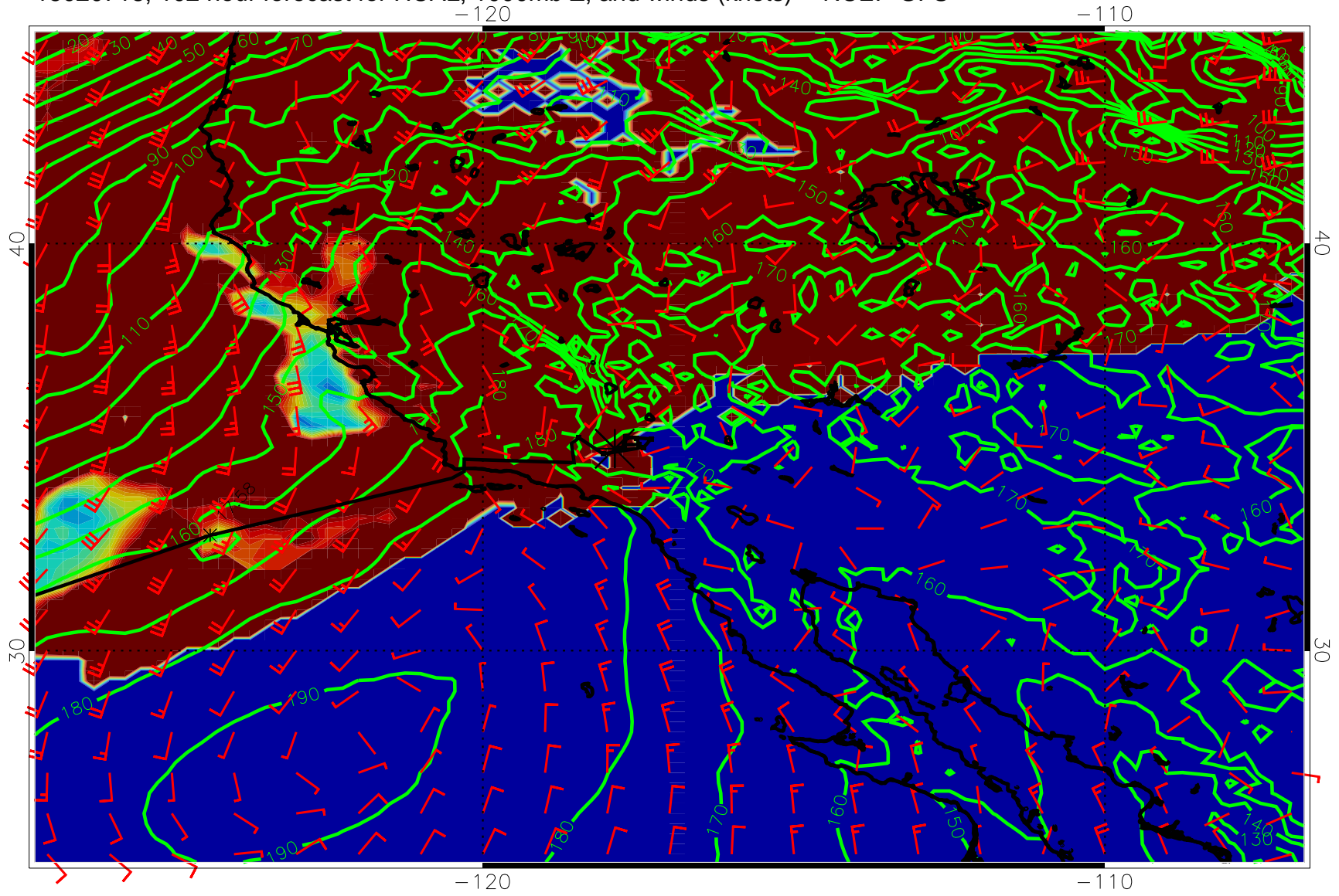
15020718, 102 hour forecast for HCAL, 1000mb Z, and winds (knots) -- NCEP GFS
