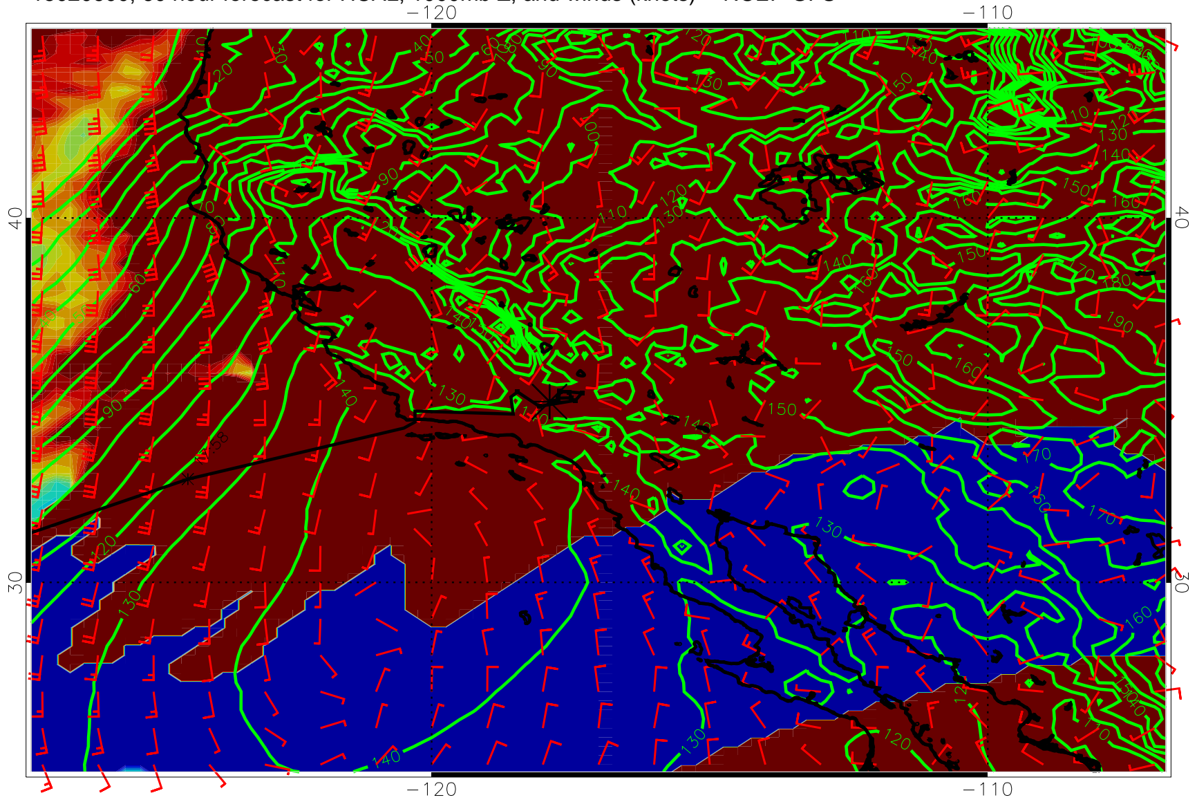
15020600, 60 hour forecast for HCAL, 1000mb Z, and winds (knots) -- NCEP GFS
