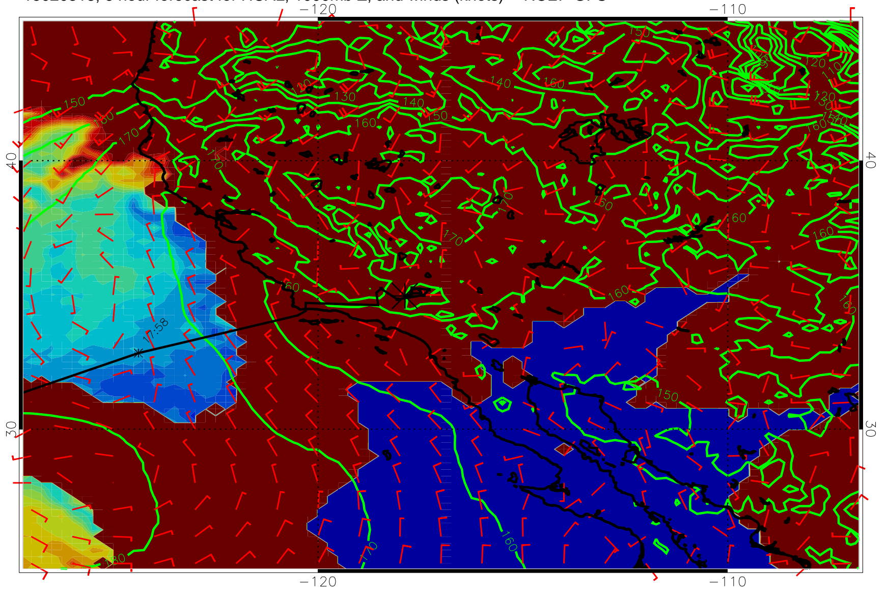
15020318, 6 hour forecast for HCAL, 1000mb Z, and winds (knots) -- NCEP GFS
