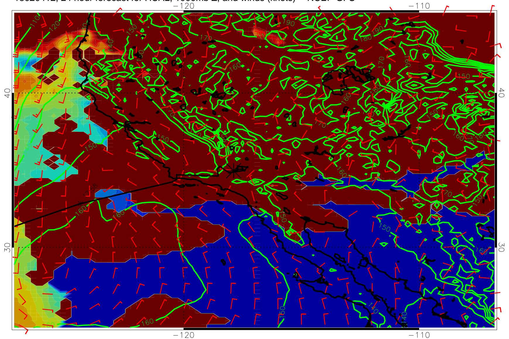
15020412, 24 hour forecast for HCAL, 1000mb Z, and winds (knots) -- NCEP GFS
