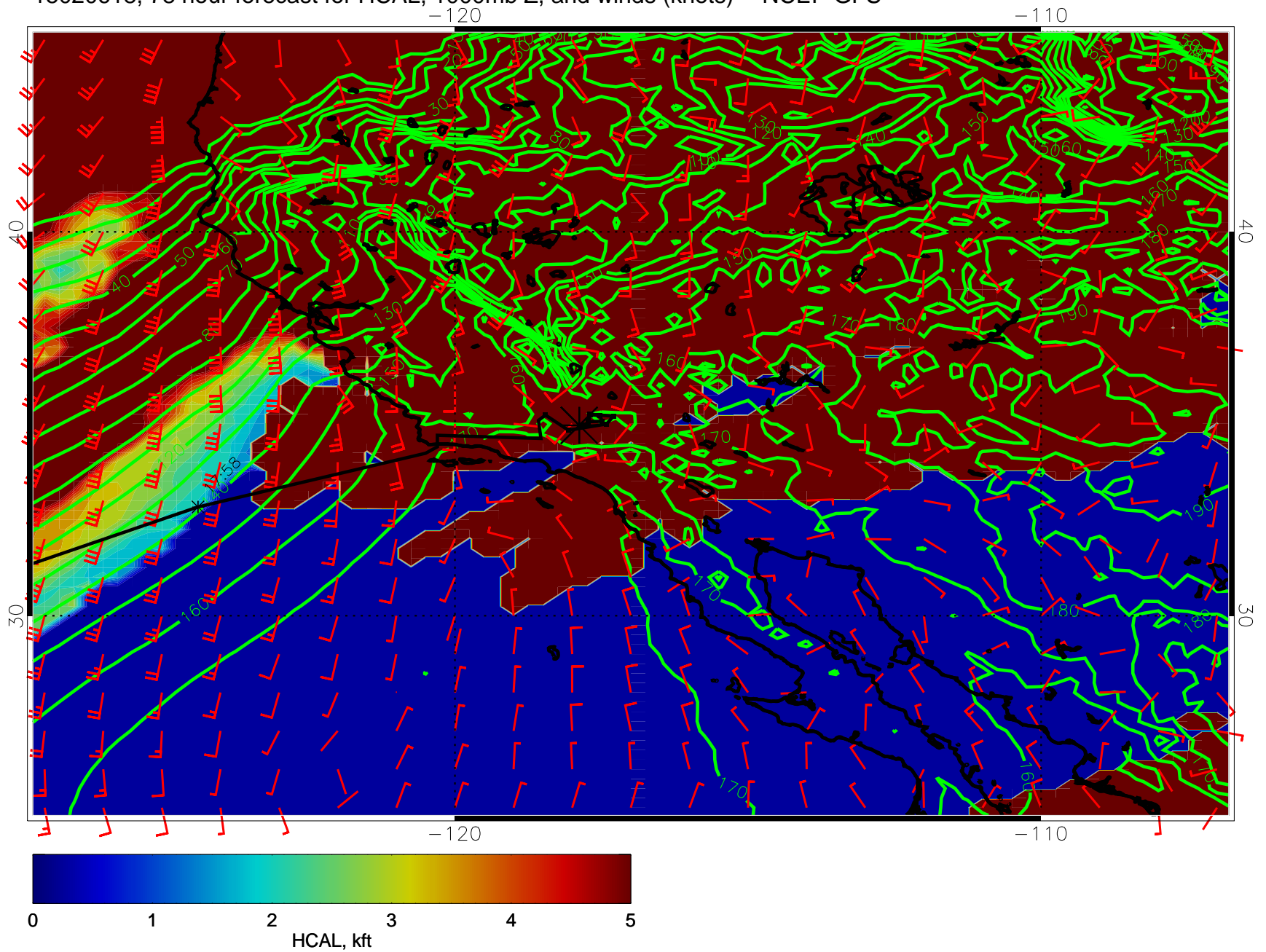
15020618, 78 hour forecast for HCAL, 1000mb Z, and winds (knots) -- NCEP GFS
