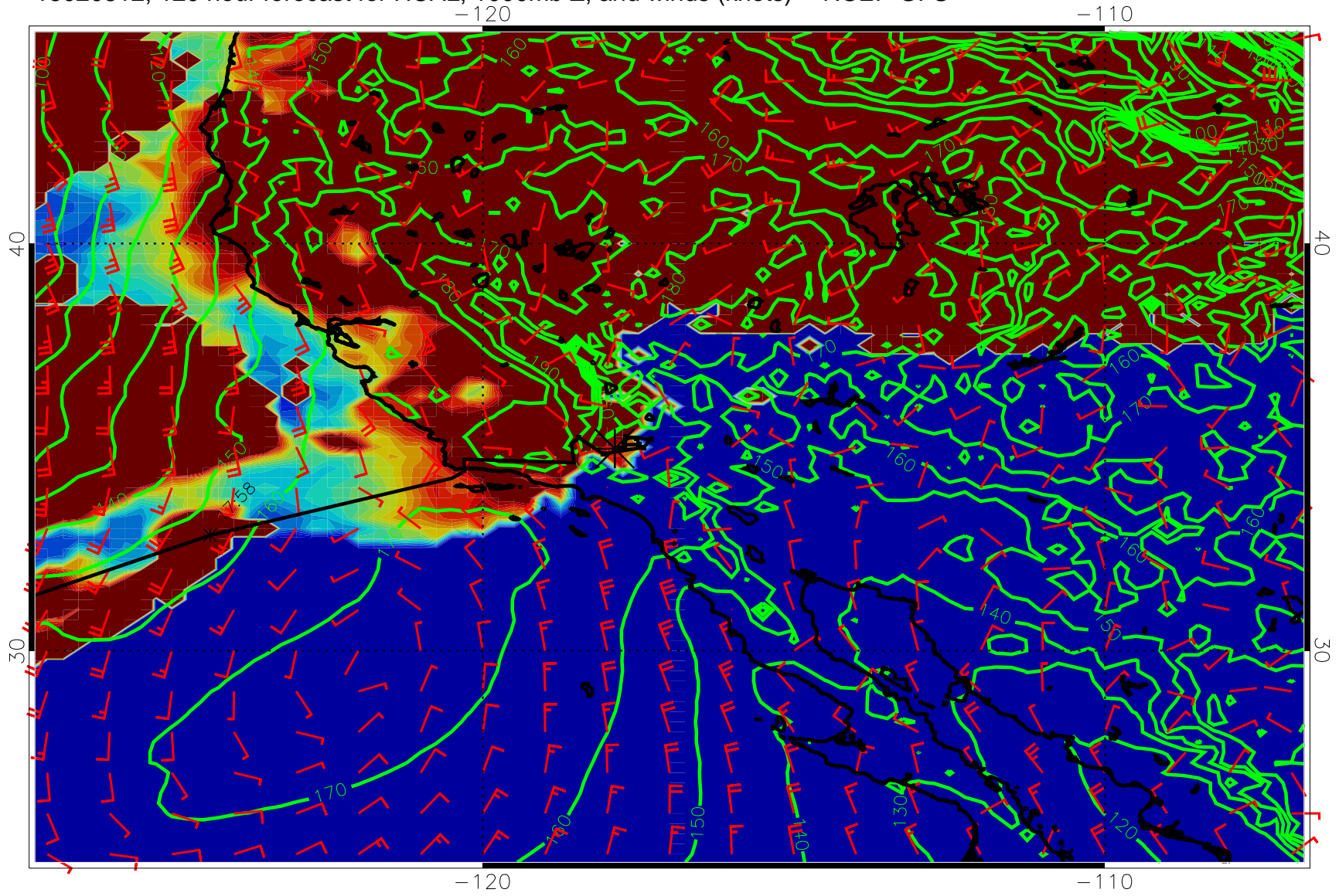
15020812, 120 hour forecast for HCAL, 1000mb Z, and winds (knots) -- NCEP GFS
