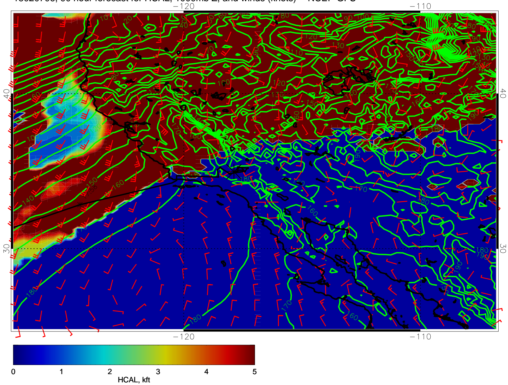
15020706, 90 hour forecast for HCAL, 1000mb Z, and winds (knots) -- NCEP GFS
