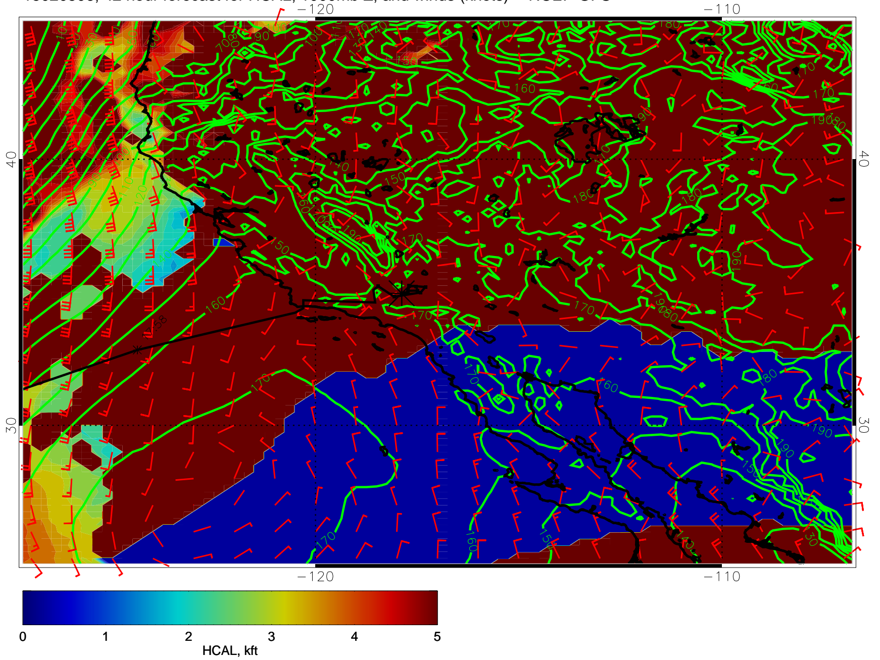
15020506, 42 hour forecast for HCAL, 1000mb Z, and winds (knots) -- NCEP GFS
