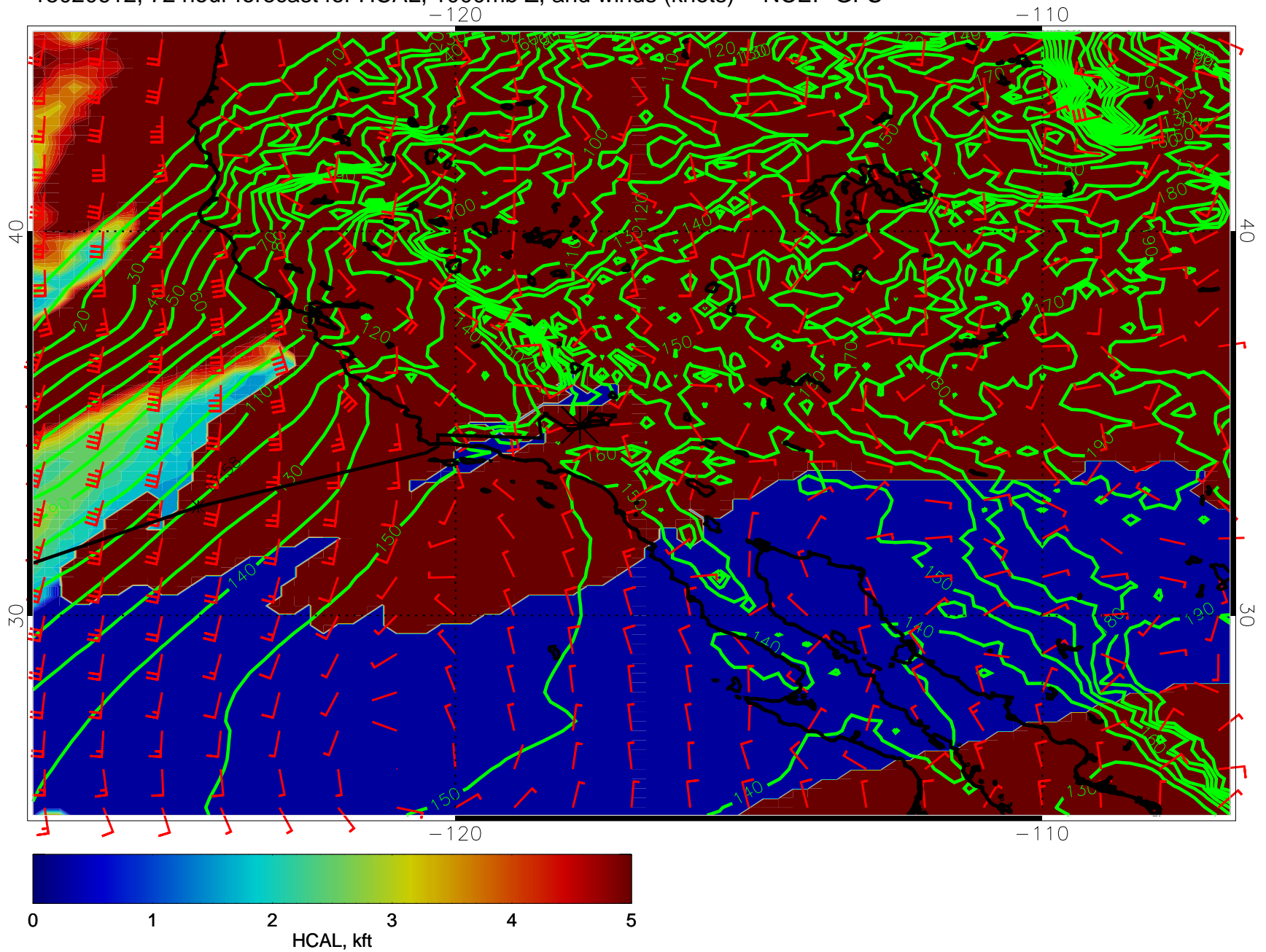
15020612, 72 hour forecast for HCAL, 1000mb Z, and winds (knots) -- NCEP GFS
