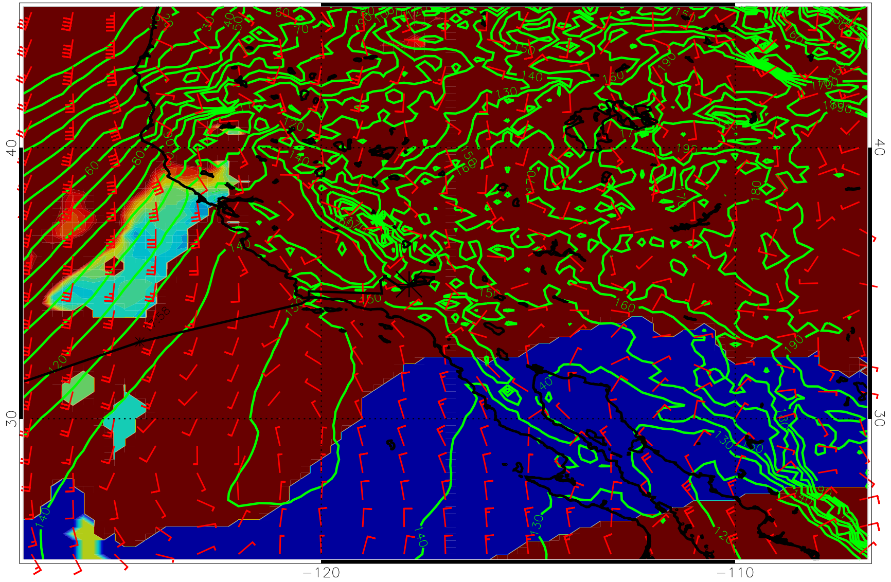
15020512, 48 hour forecast for HCAL, 1000mb Z, and winds (knots) -- NCEP GFS -120 -110
