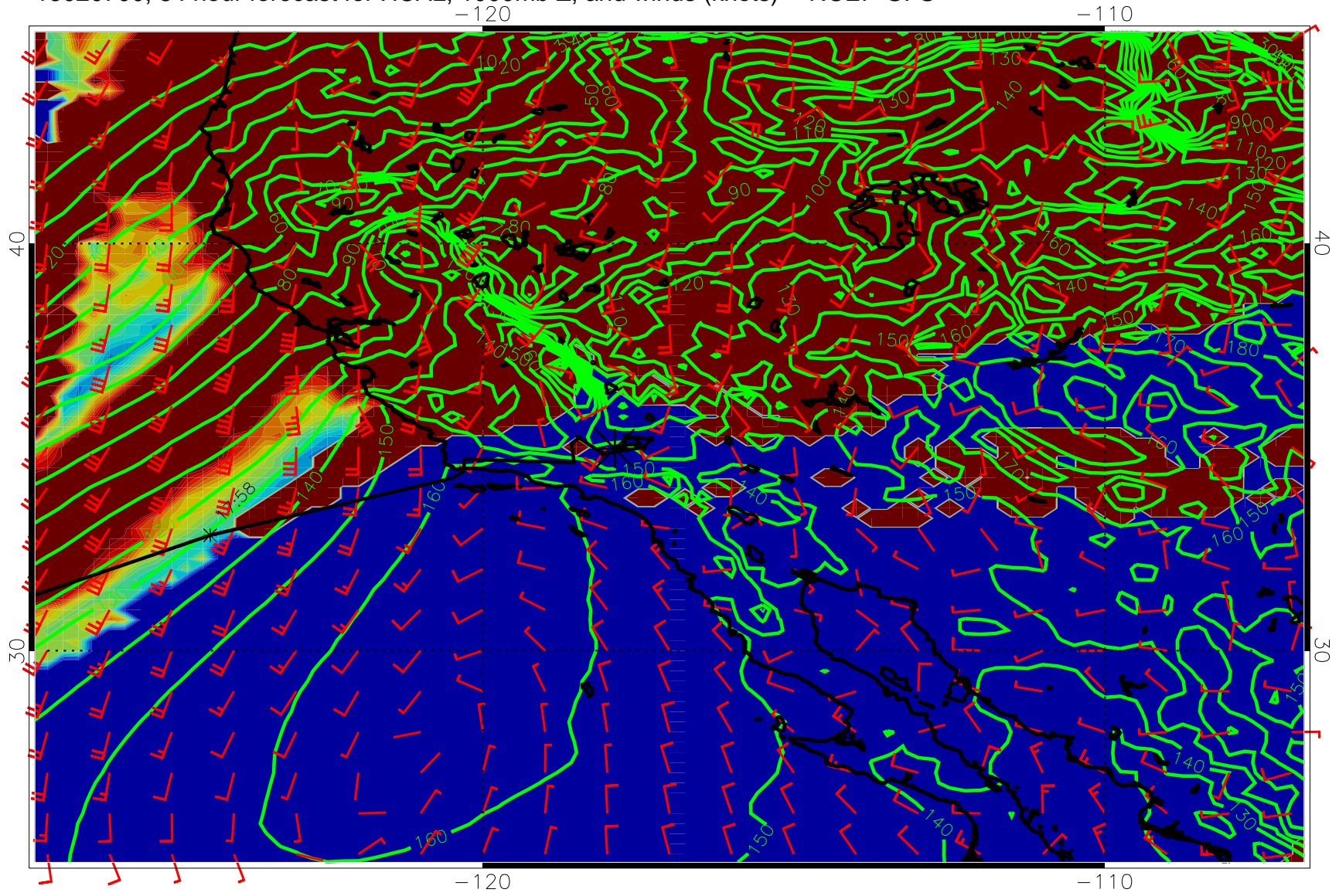
15020700, 84 hour forecast for HCAL, 1000mb Z, and winds (knots) -- NCEP GFS
