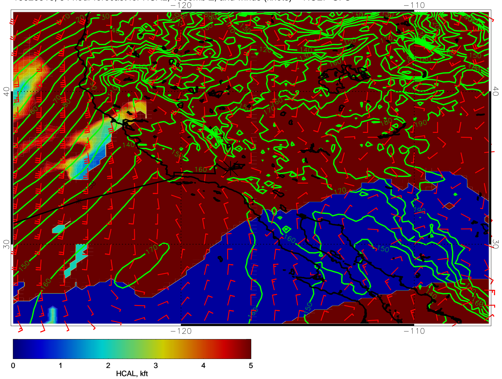
15020518, 54 hour forecast for HCAL, 1000mb Z, and winds (knots) -- NCEP GFS
