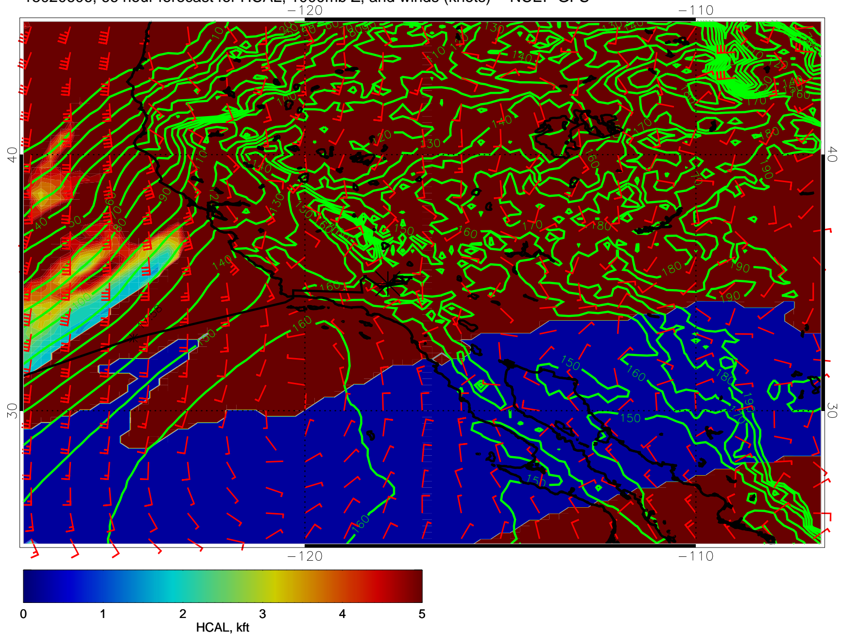
15020606, 66 hour forecast for HCAL, 1000mb Z, and winds (knots) -- NCEP GFS
