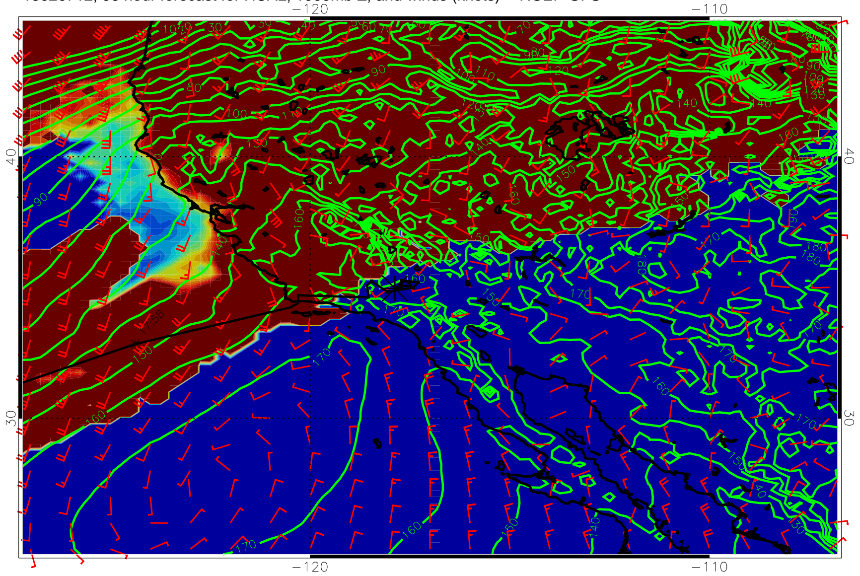
15020712, 96 hour forecast for HCAL, 1000mb Z, and winds (knots) -- NCEP GFS
