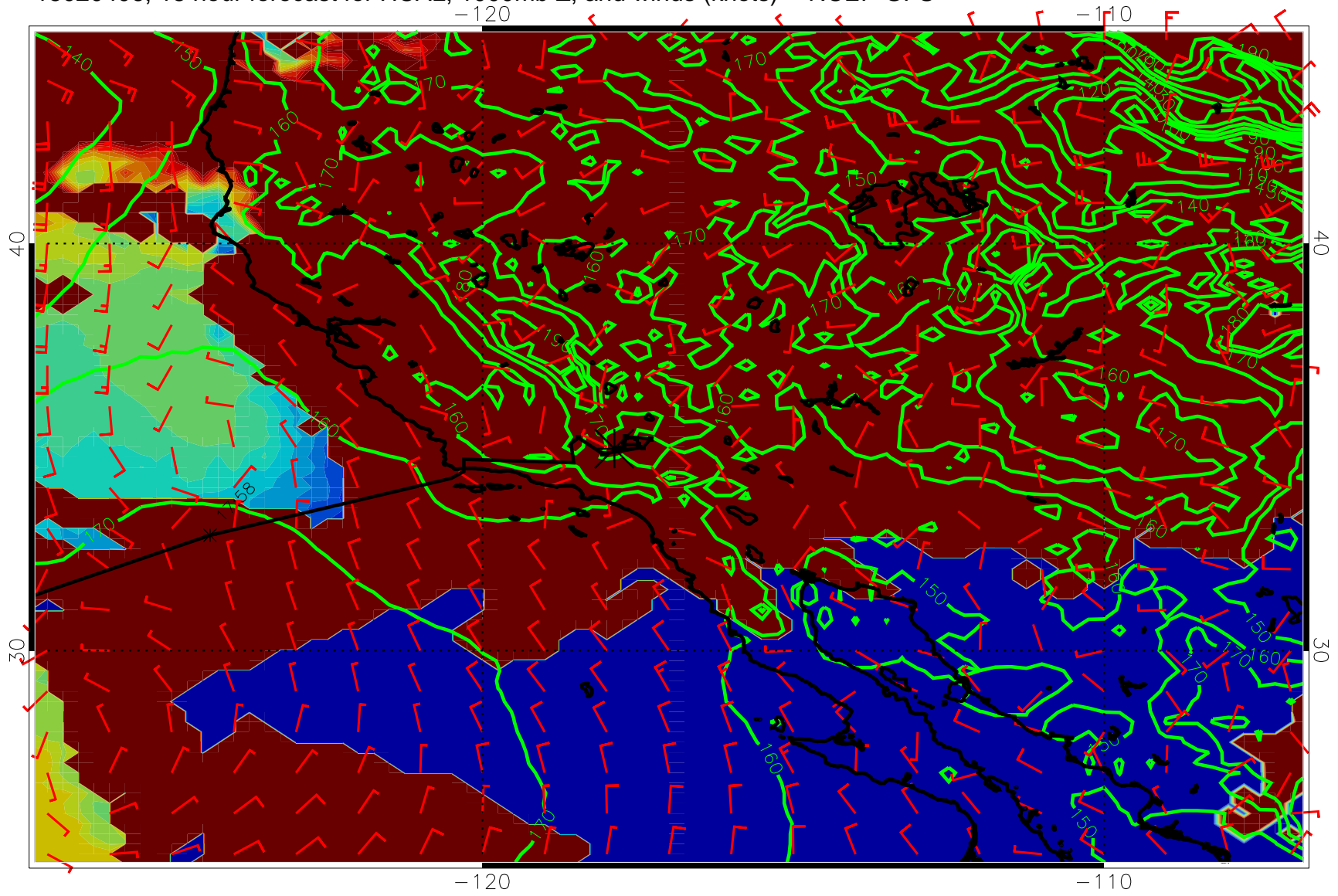
15020406, 18 hour forecast for HCAL, 1000mb Z, and winds (knots) -- NCEP GFS
