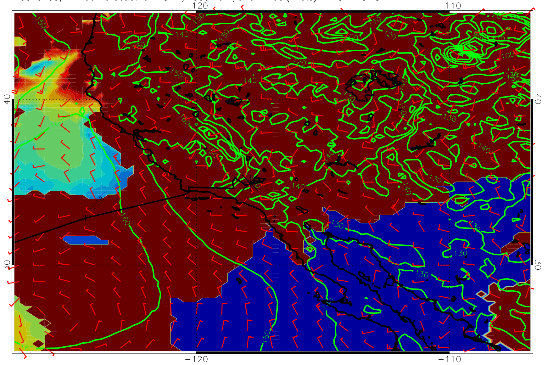
15020400, 12 hour forecast for HCAL, 1000mb Z, and winds (knots) -- NCEP GFS
