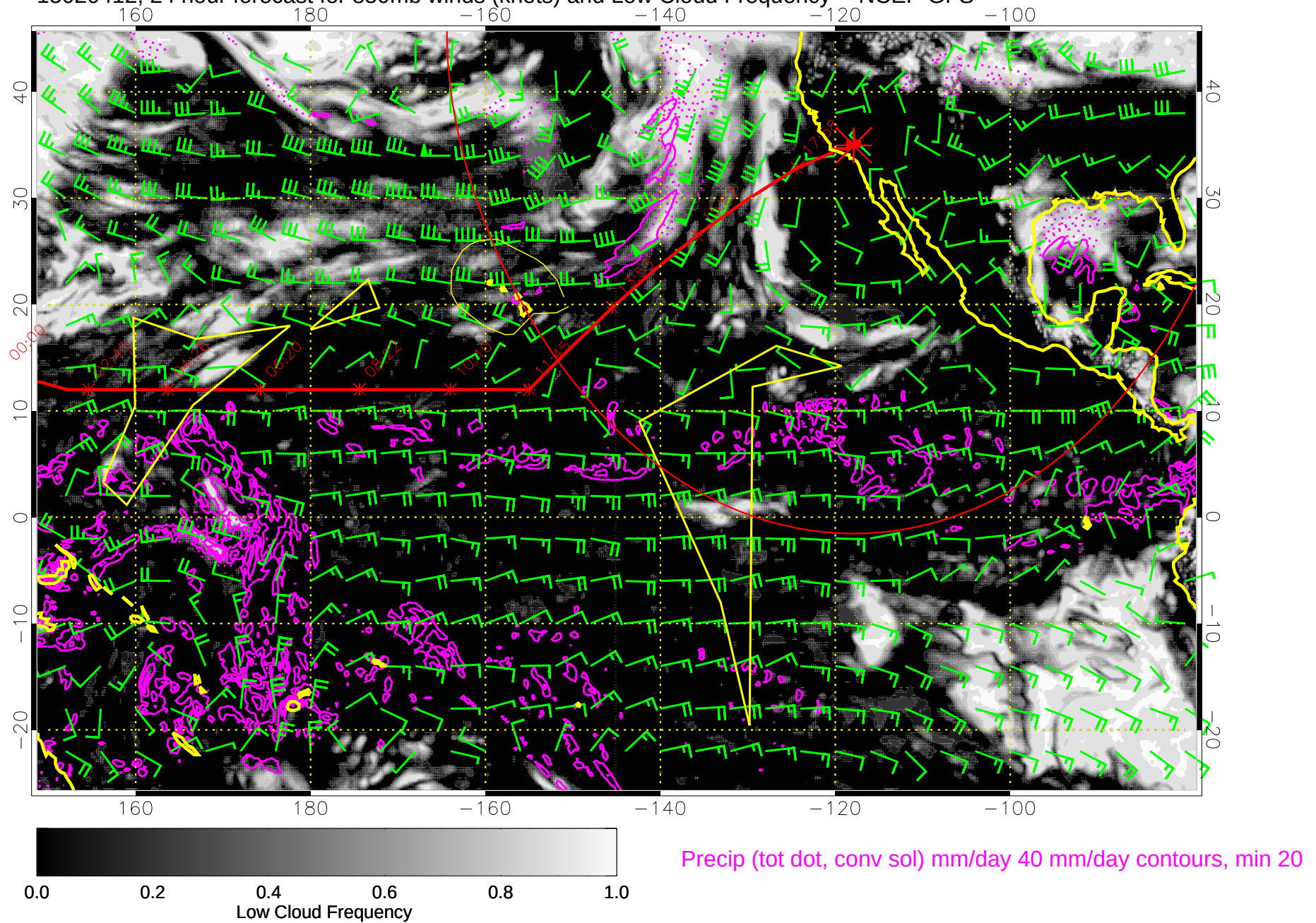
15020412, 24 hour forecast for 850mb winds (knots) and Low Cloud Frequency -- NCEP GFS
