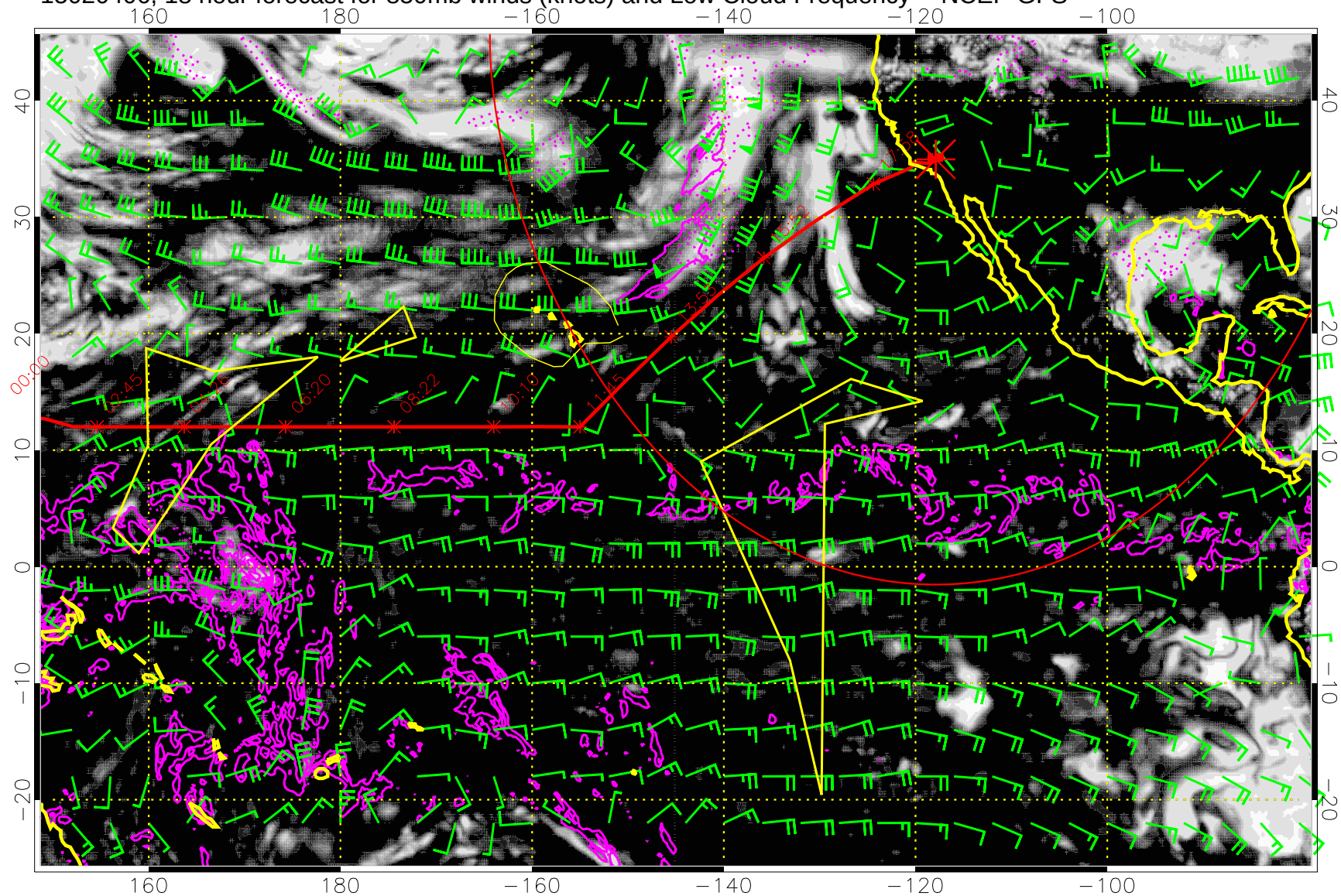
15020406, 18 hour forecast for 850mb winds (knots) and Low Cloud Frequency -- NCEP GFS
