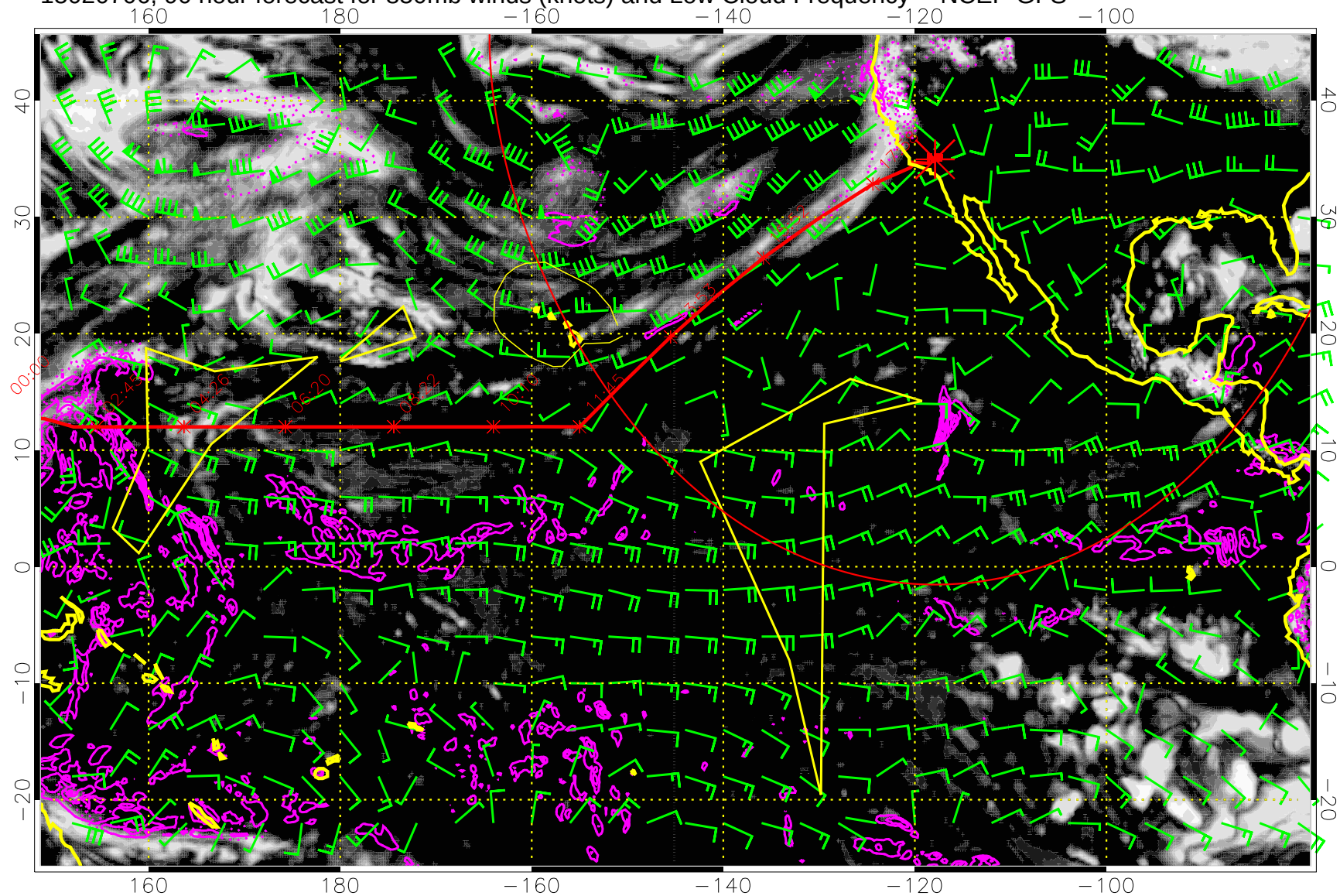
15020706, 90 hour forecast for 850mb winds (knots) and Low Cloud Frequency -- NCEP GFS
