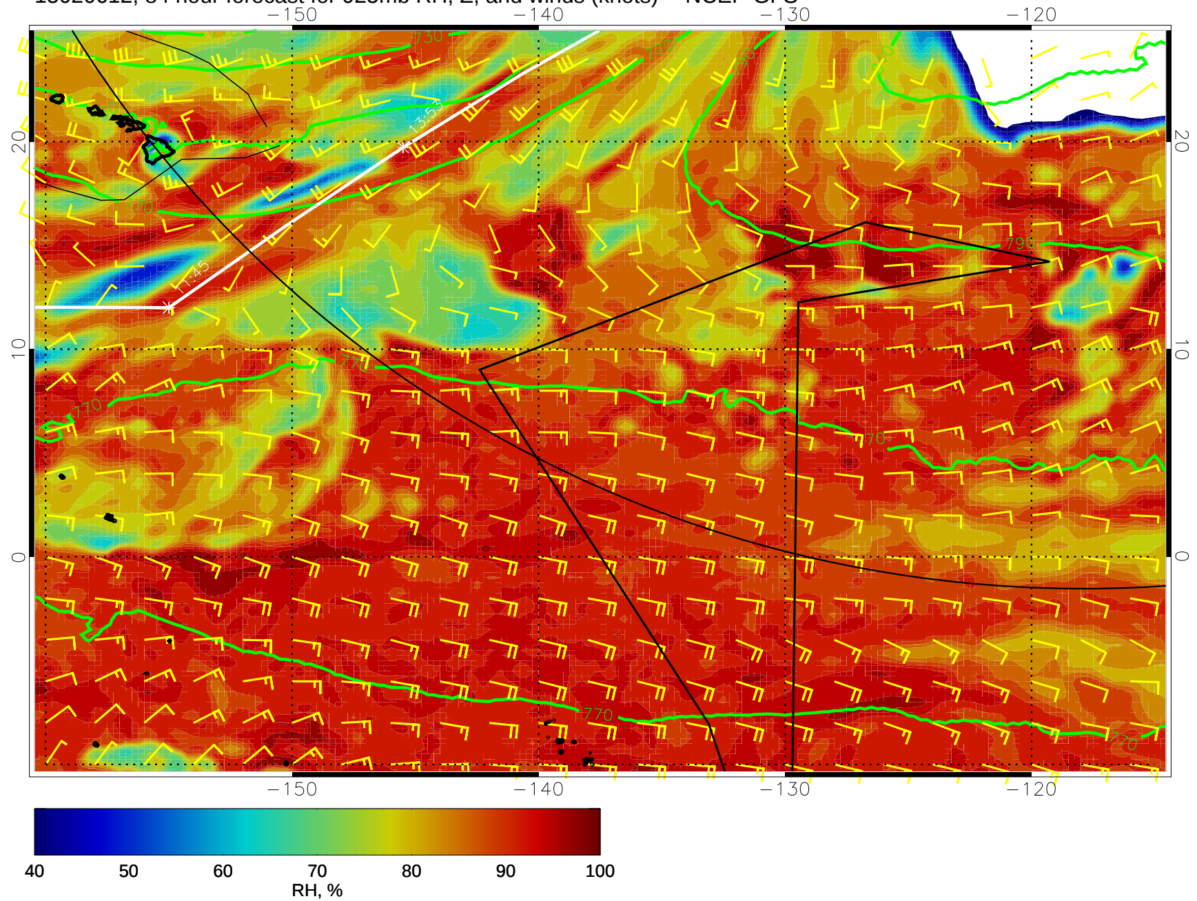
15020612, 84 hour forecast for 925mb RH, Z, and winds (knots) -- NCEP GFS
