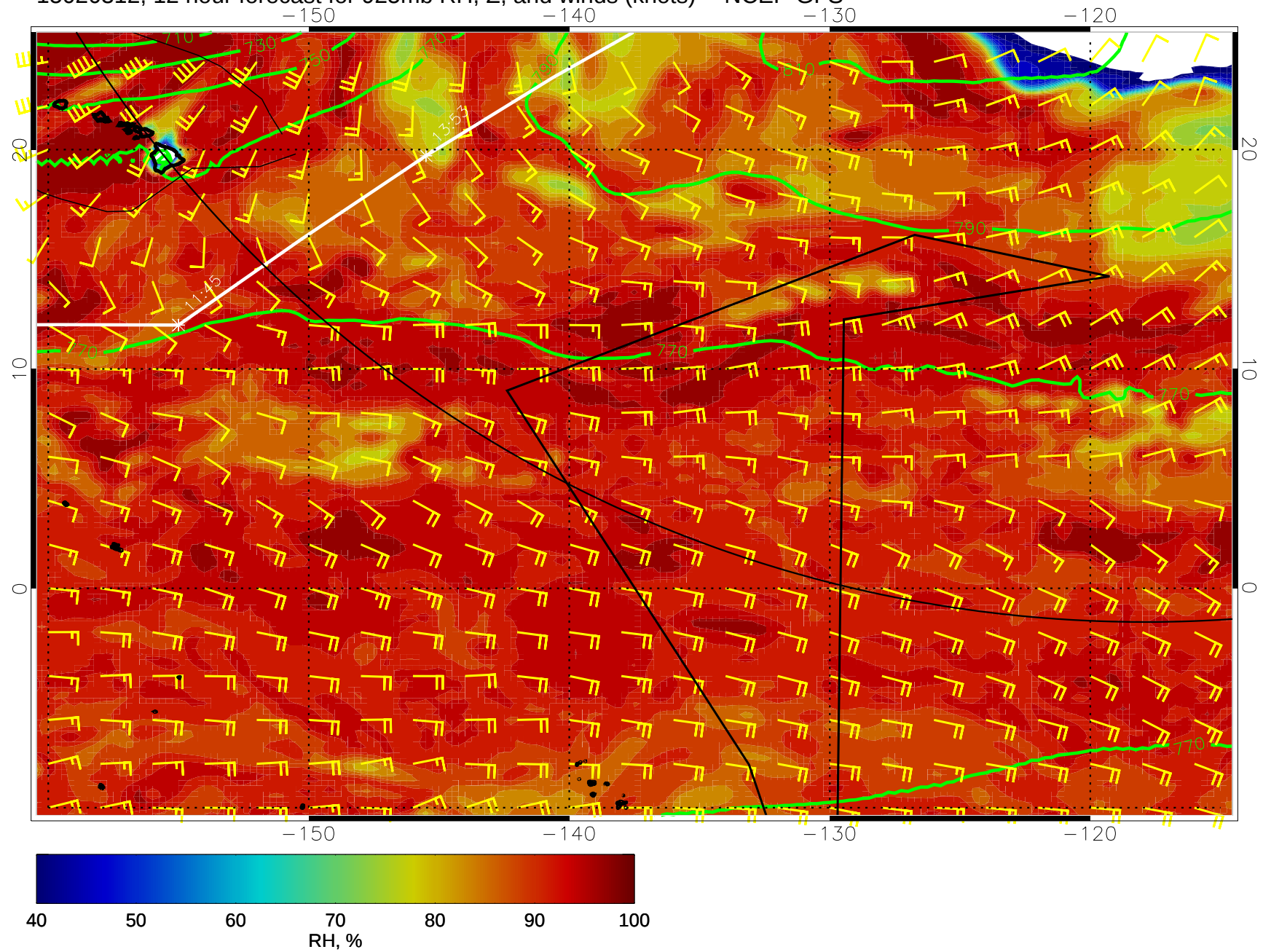
15020312, 12 hour forecast for 925mb RH, Z, and winds (knots) -- NCEP GFS
