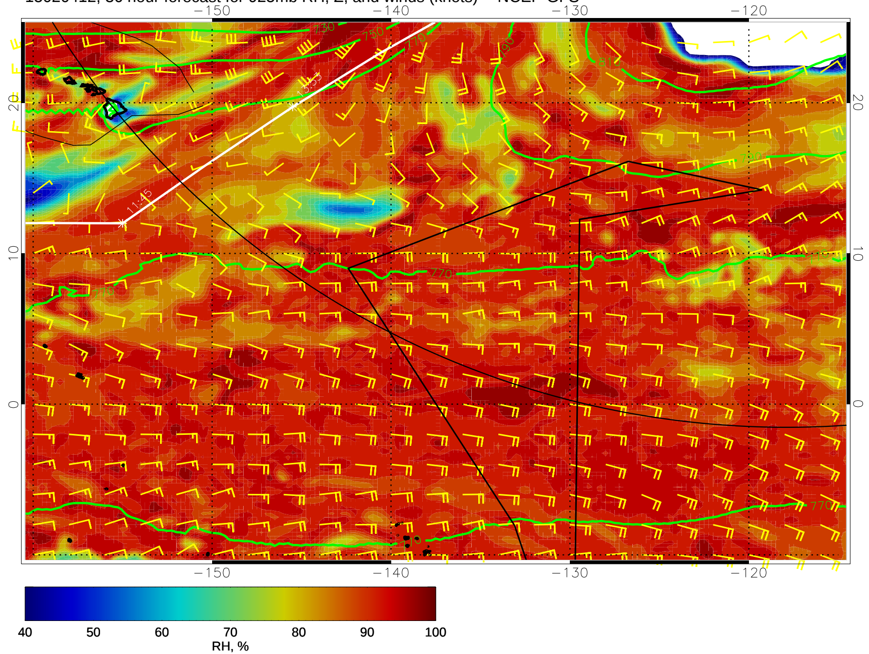
15020412, 36 hour forecast for 925mb RH, Z, and winds (knots) -- NCEP GFS
