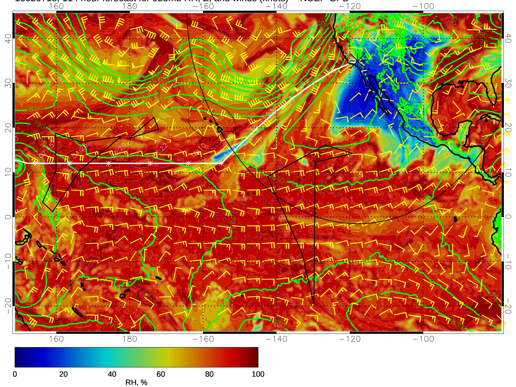
15020718, 114 hour forecast for 925mb RH, Z, and winds (knots) -- NCEP GFS
