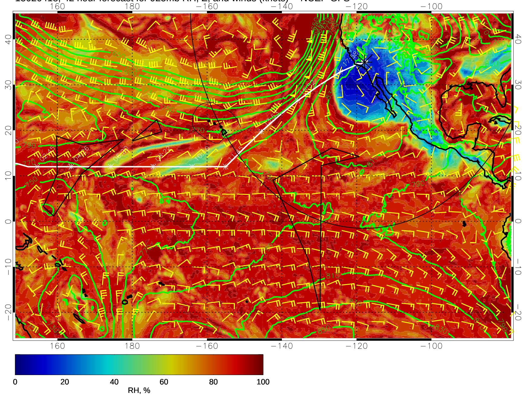
15020418, 42 hour forecast for 925mb RH, Z, and winds (knots) -- NCEP GFS
