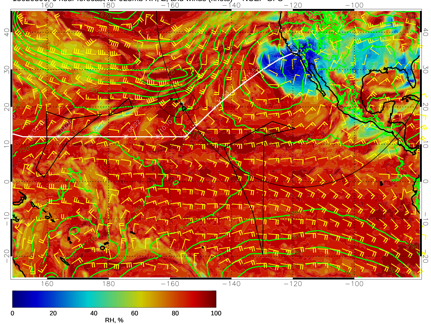
15020306, 6 hour forecast for 925mb RH, Z, and winds (knots) -- NCEP GFS
