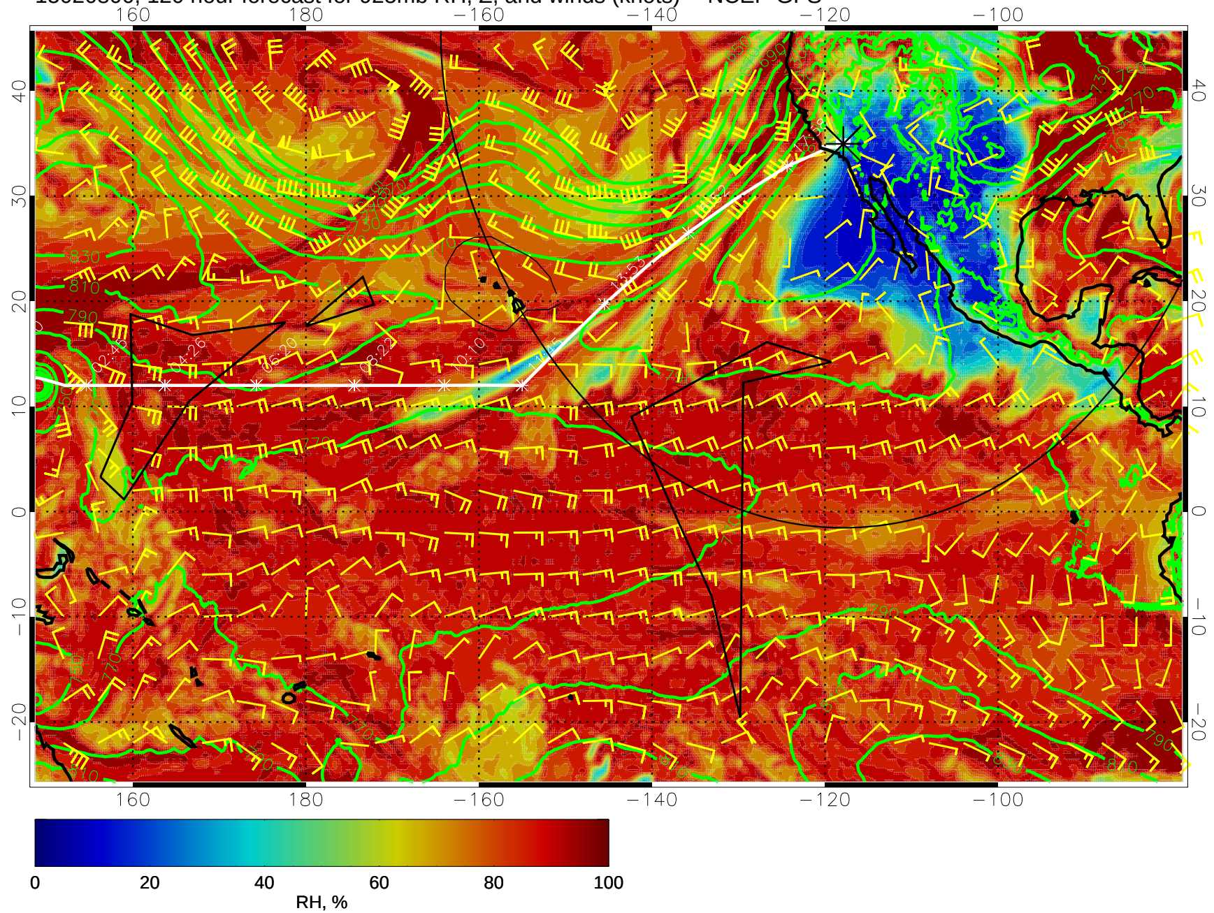
15020800, 120 hour forecast for 925mb RH, Z, and winds (knots) -- NCEP GFS
