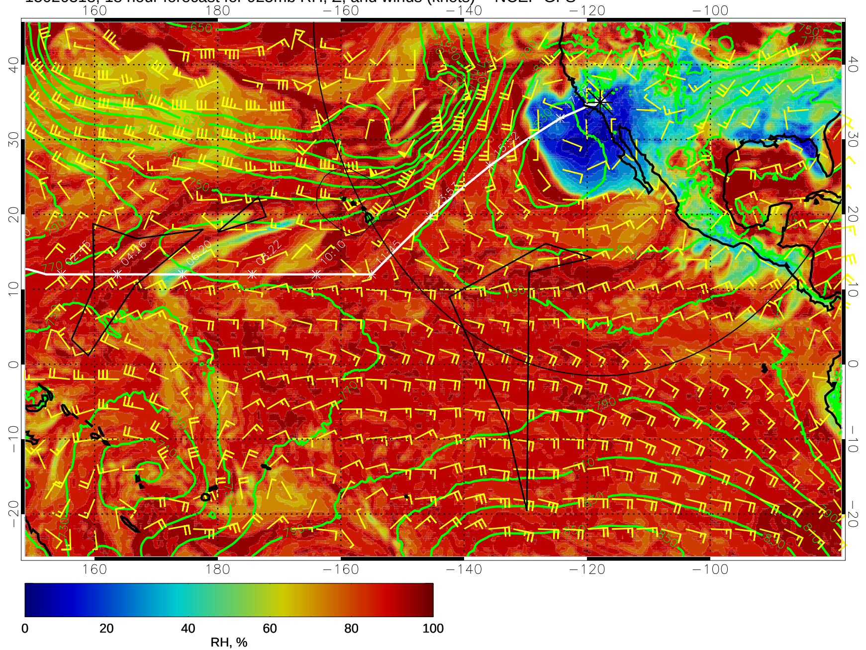
15020318, 18 hour forecast for 925mb RH, Z, and winds (knots) -- NCEP GFS
