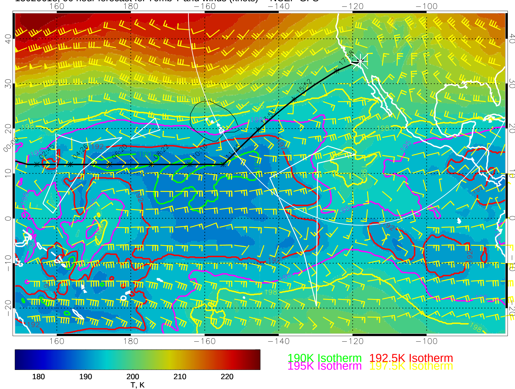
15020618, 90 hour forecast for 70mb T and winds (knots) -- NCEP GFS
