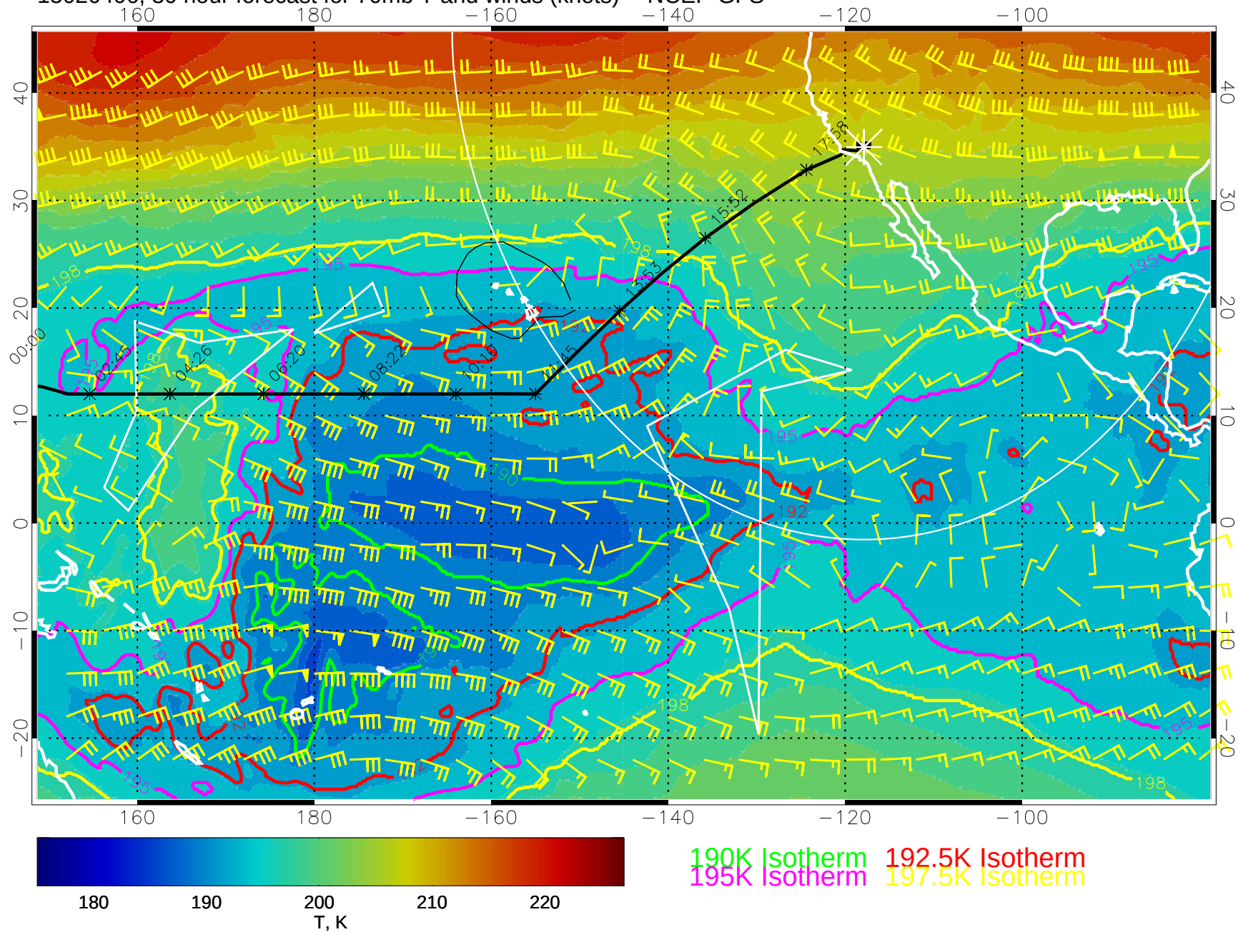
15020406, 30 hour forecast for 70mb T and winds (knots) -- NCEP GFS
