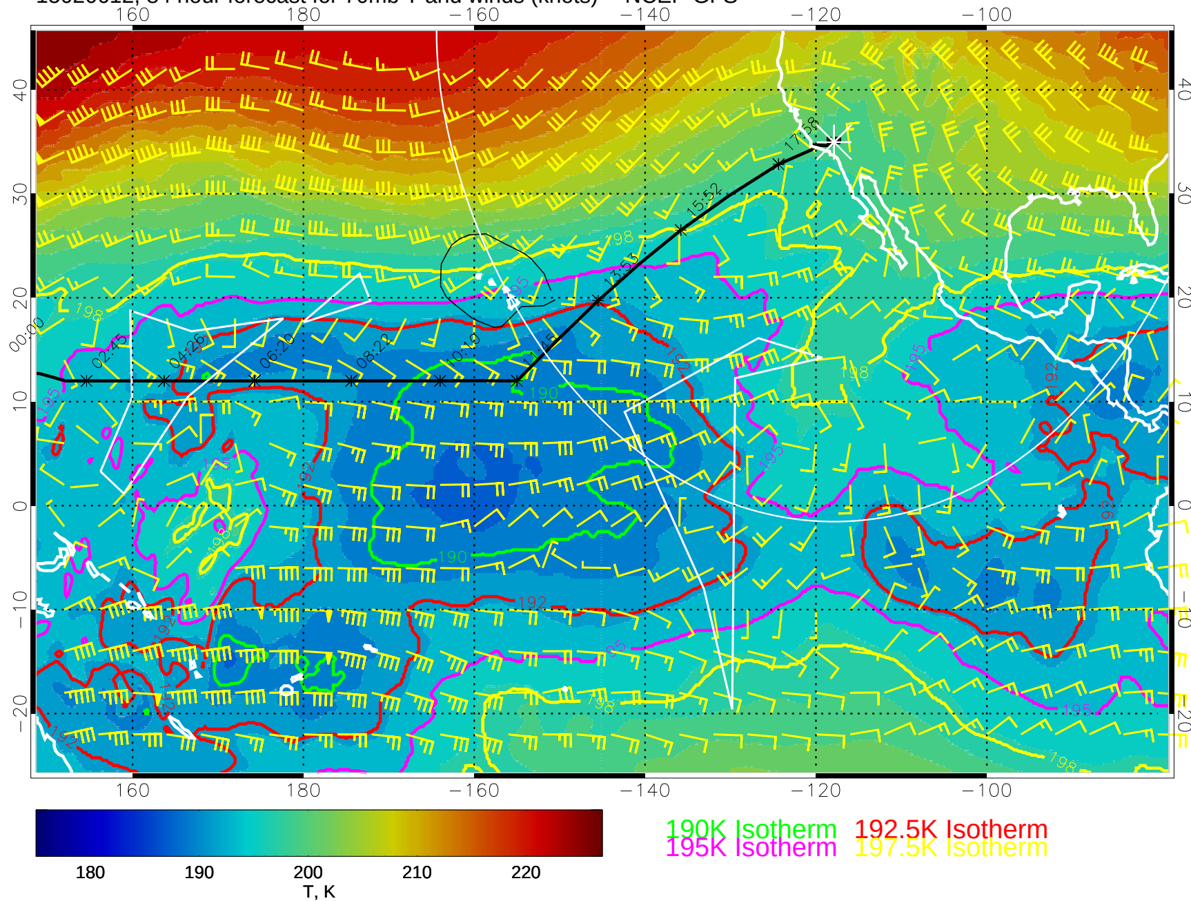
15020612, 84 hour forecast for 70mb T and winds (knots) -- NCEP GFS
