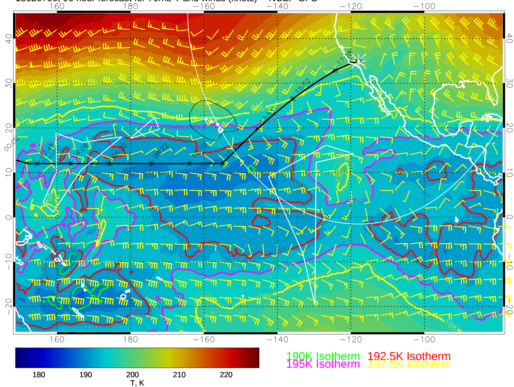
15020700, 96 hour forecast for 70mb T and winds (knots) -- NCEP GFS
