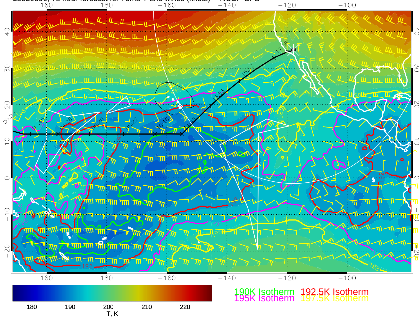
15020606, 78 hour forecast for 70mb T and winds (knots) -- NCEP GFS
