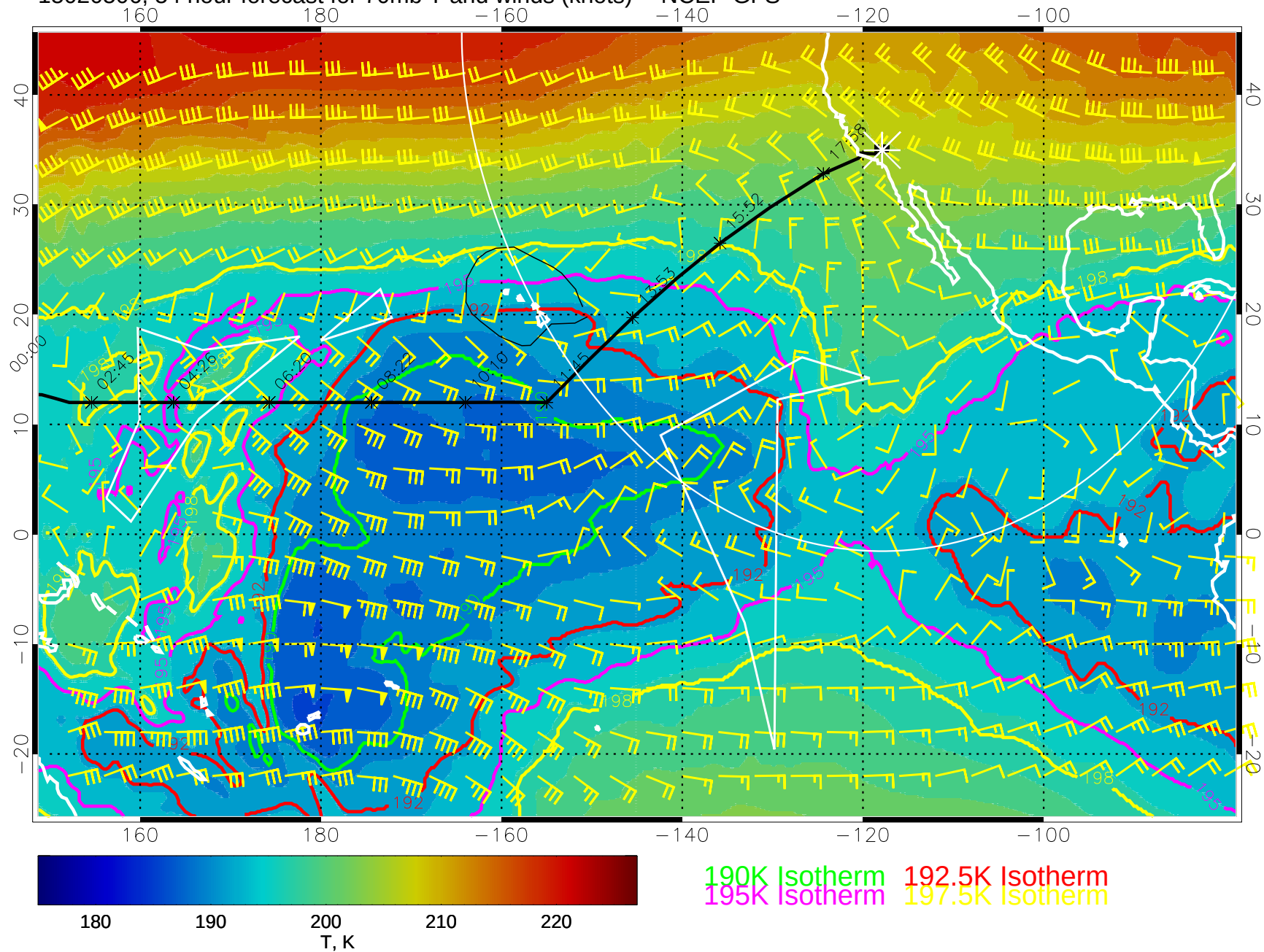
15020506, 54 hour forecast for 70mb T and winds (knots) -- NCEP GFS
