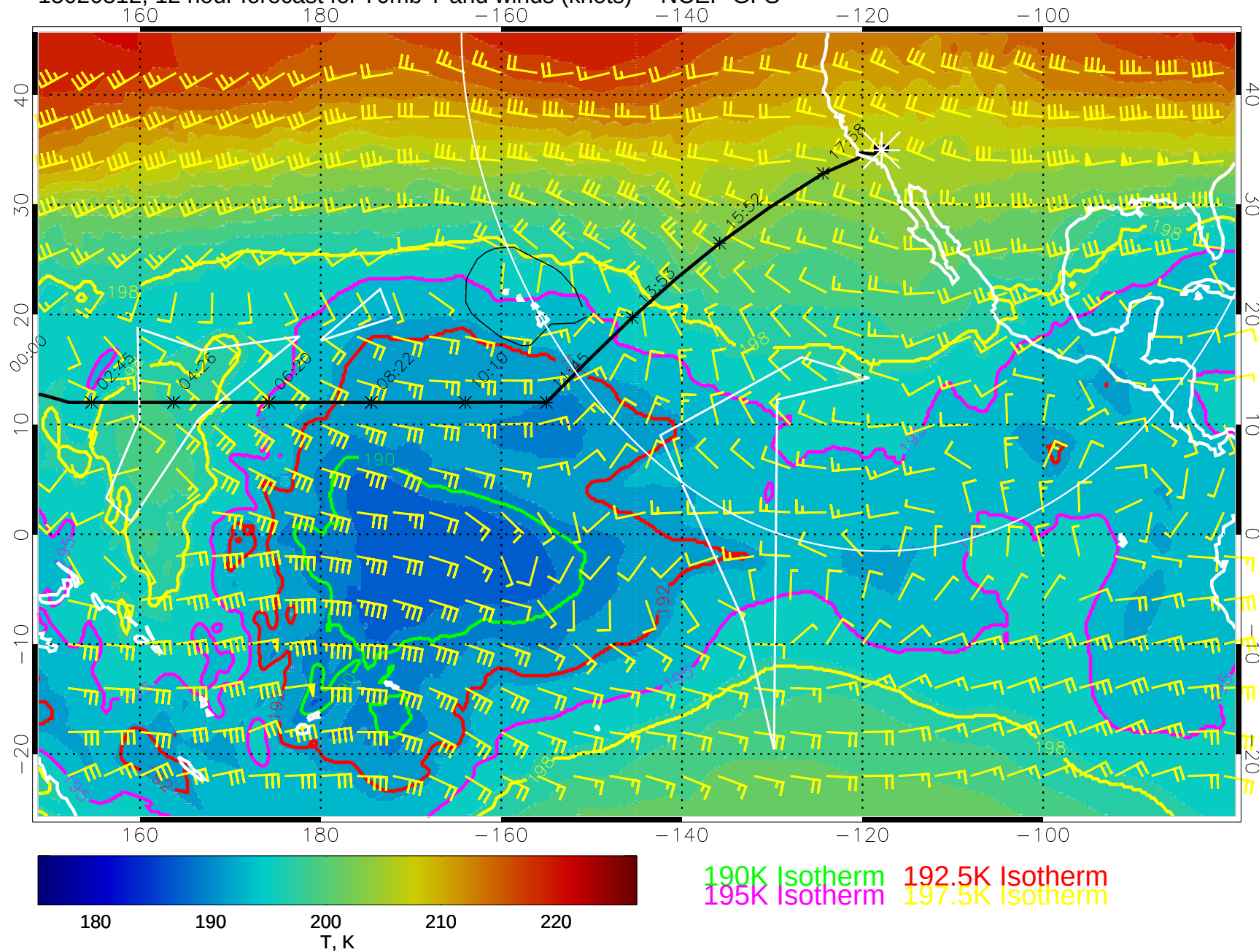
15020312, 12 hour forecast for 70mb T and winds (knots) -- NCEP GFS
