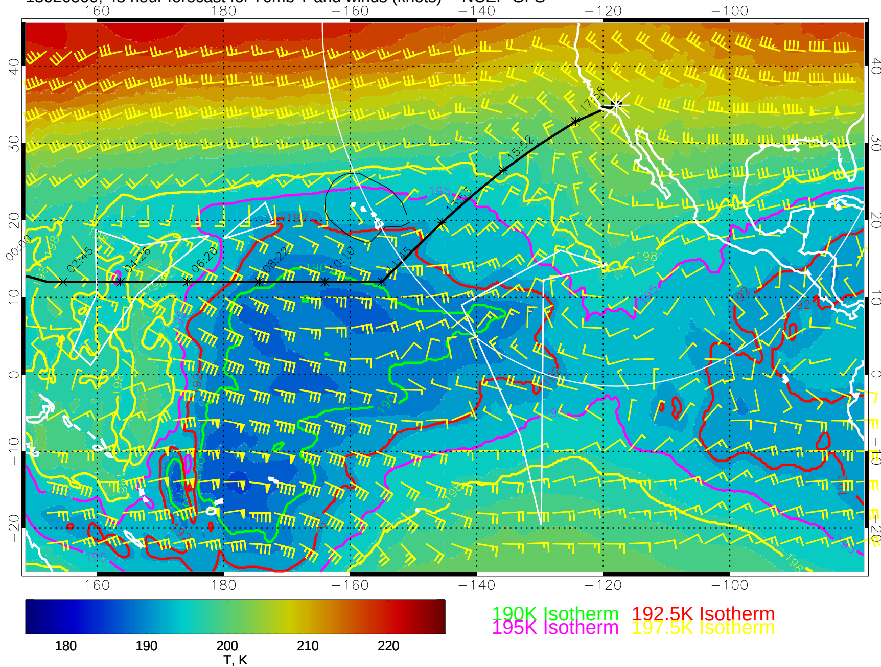
15020500, 48 hour forecast for 70mb T and winds (knots) -- NCEP GFS
