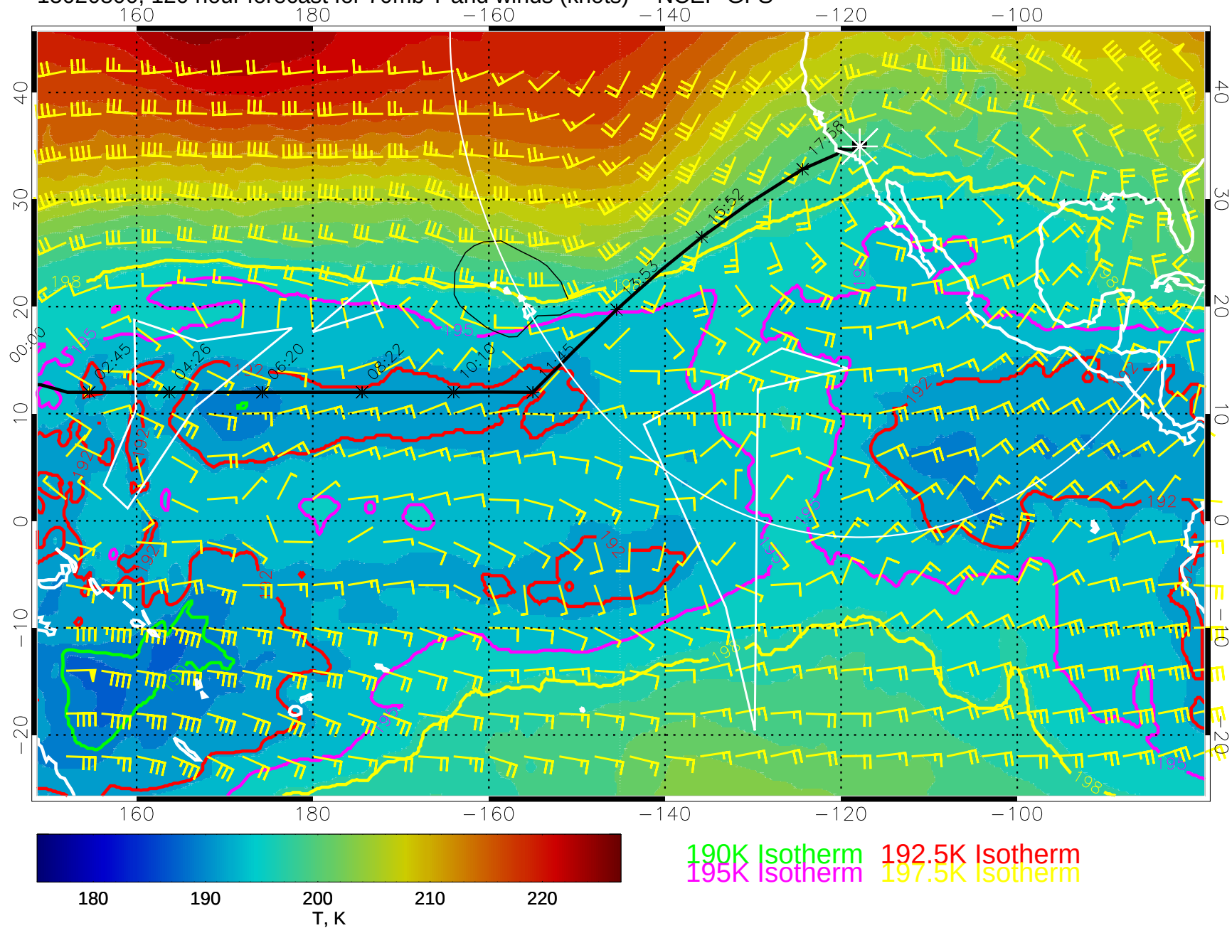
15020800, 120 hour forecast for 70mb T and winds (knots) -- NCEP GFS
