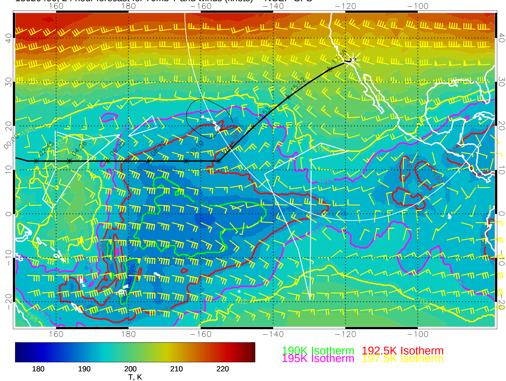
15020400, 24 hour forecast for 70mb T and winds (knots) -- NCEP GFS
