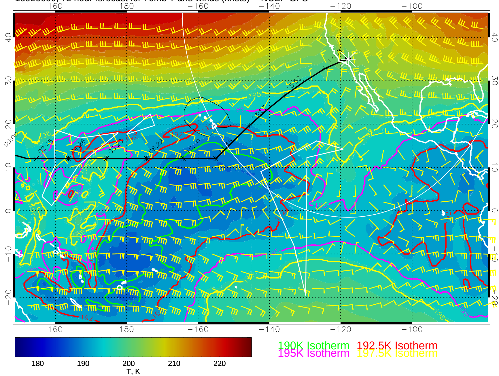
15020600, 72 hour forecast for 70mb T and winds (knots) -- NCEP GFS
