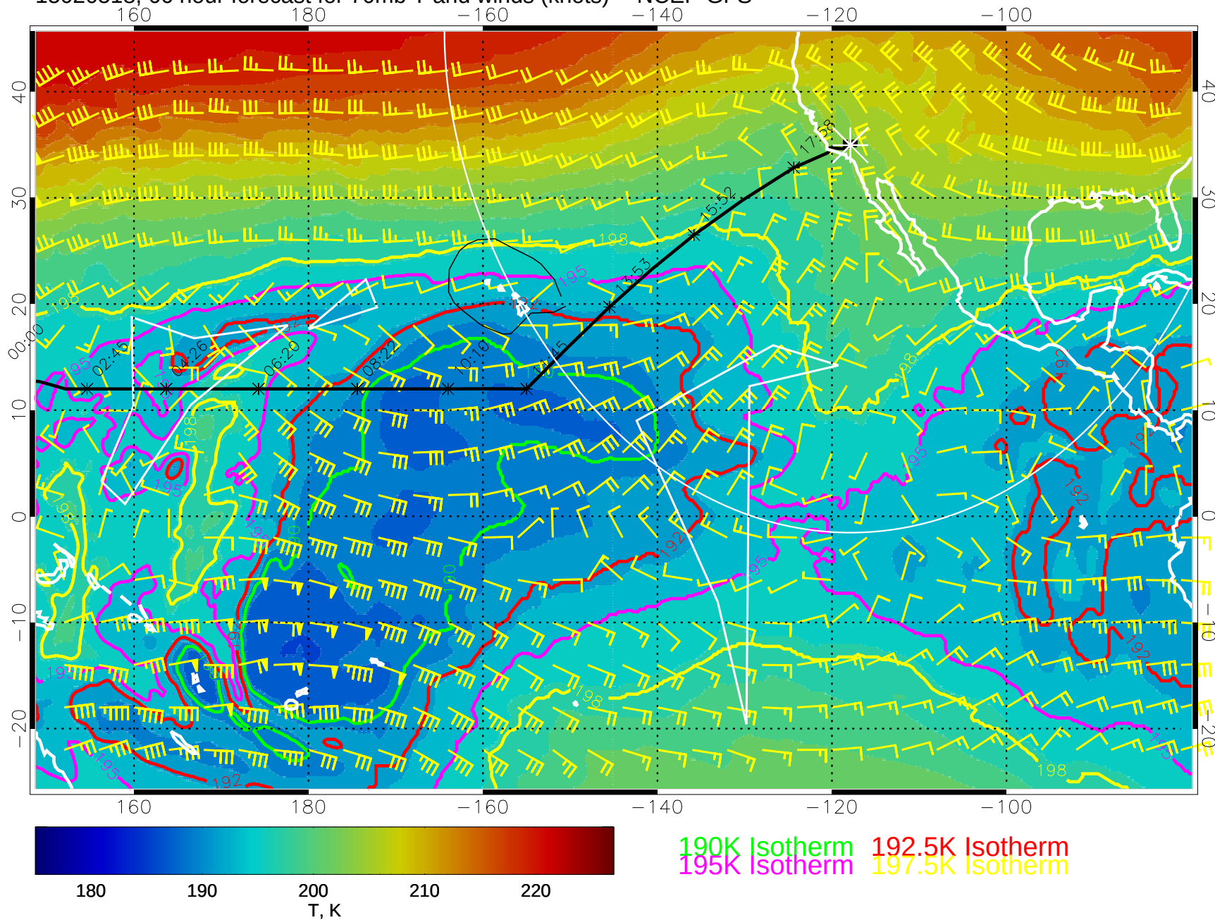
15020518, 66 hour forecast for 70mb T and winds (knots) -- NCEP GFS
