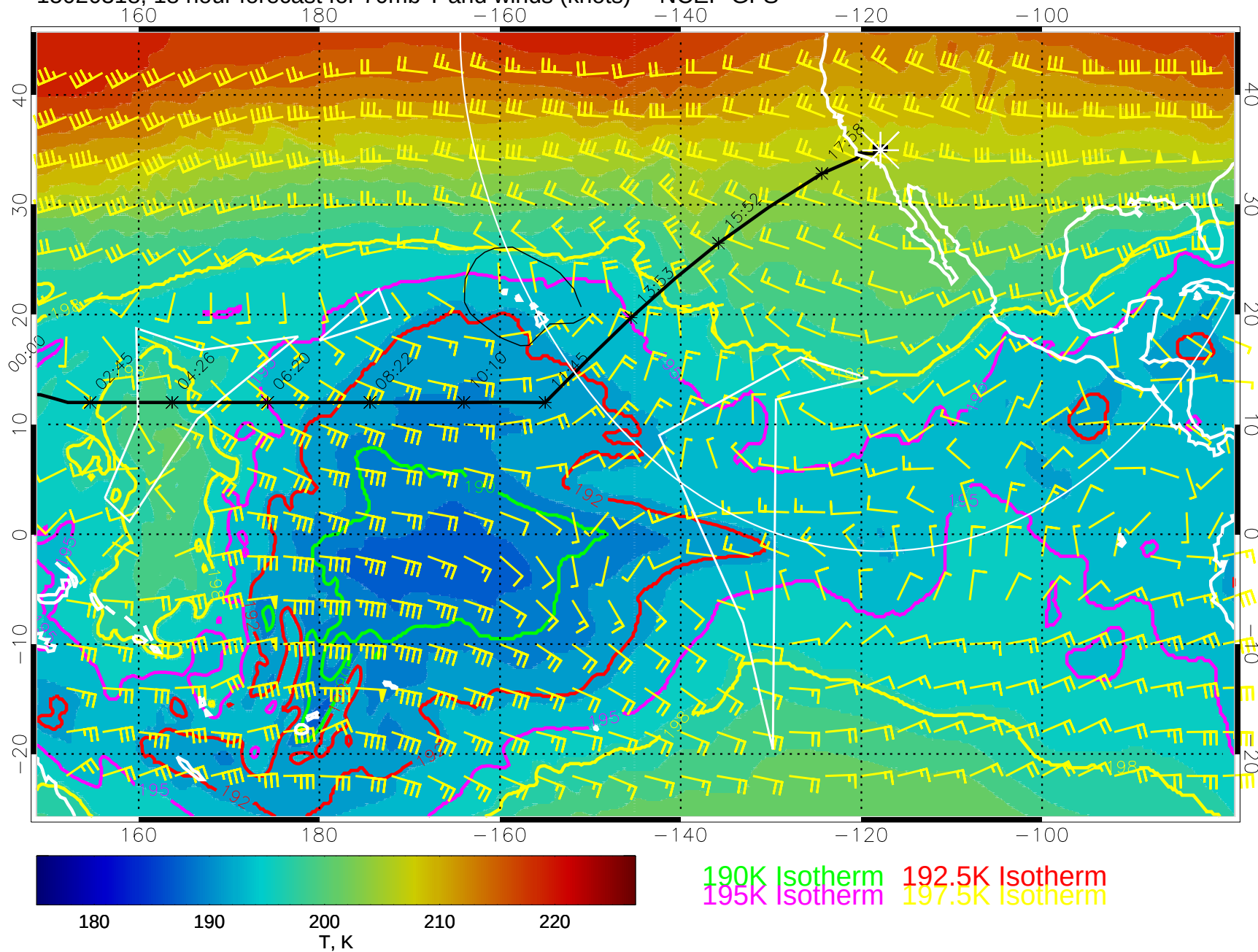
15020318, 18 hour forecast for 70mb T and winds (knots) -- NCEP GFS
