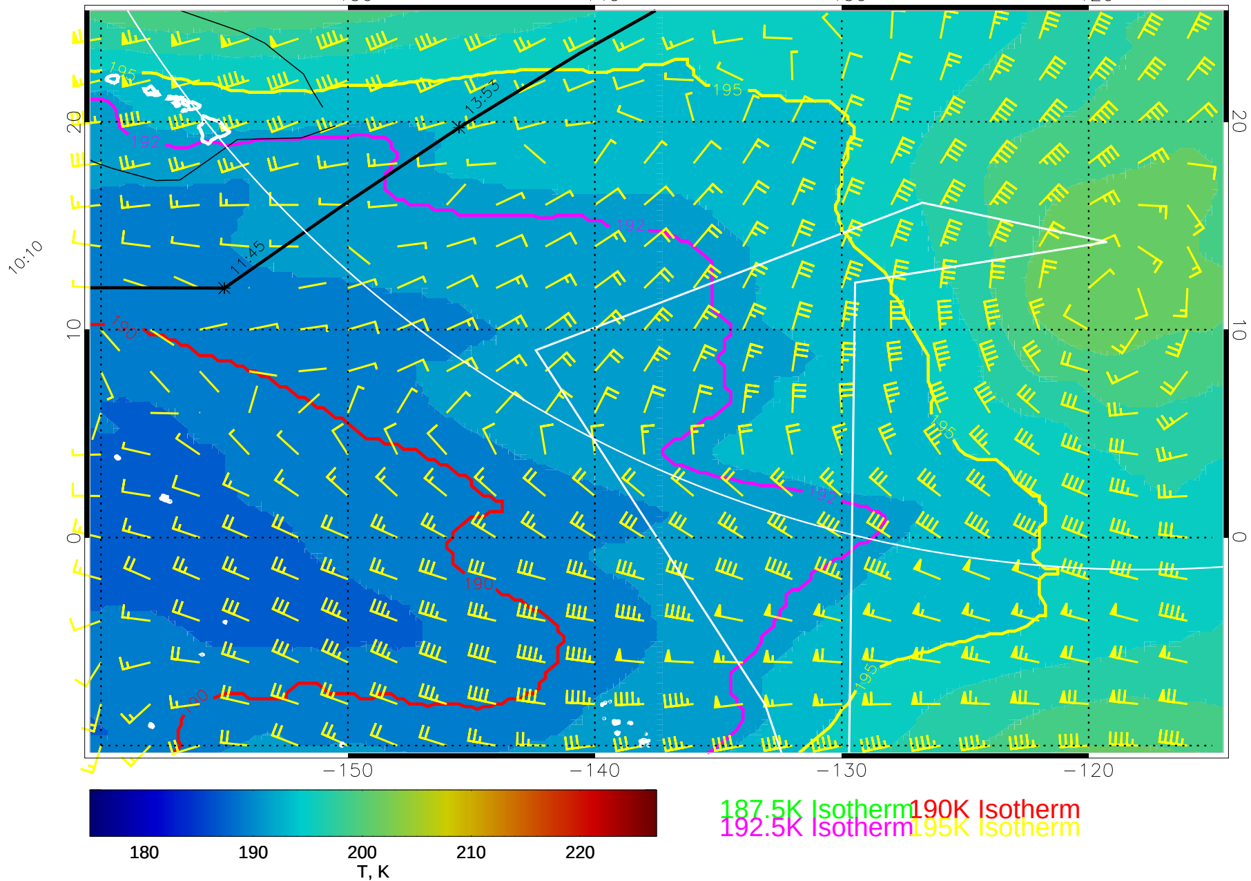
15020612, 84 hour forecast for 100mb T and winds (knots) -- NCEP GFS
