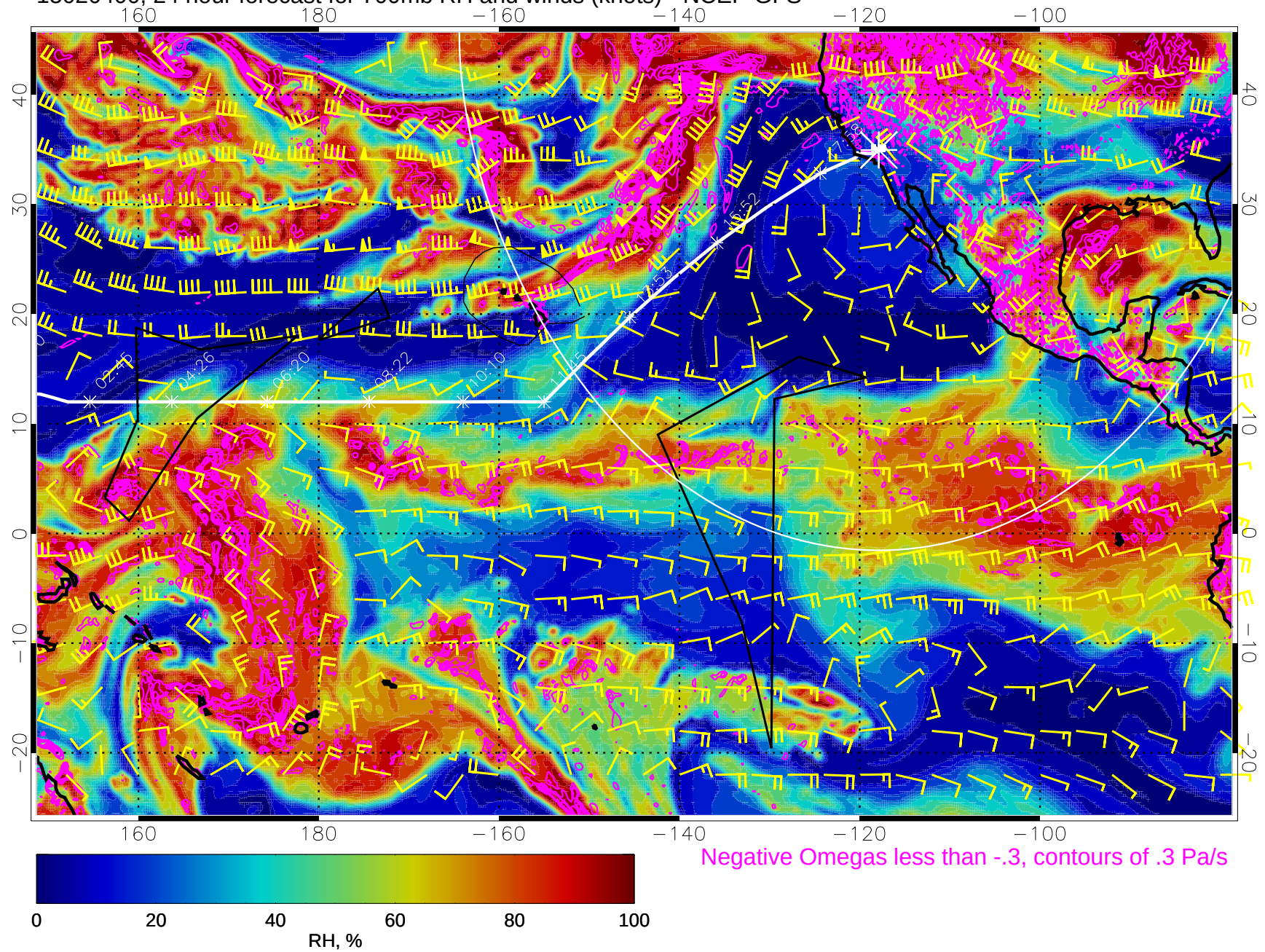
15020400, 24 hour forecast for 700mb RH and winds (knots) - NCEP GFS
