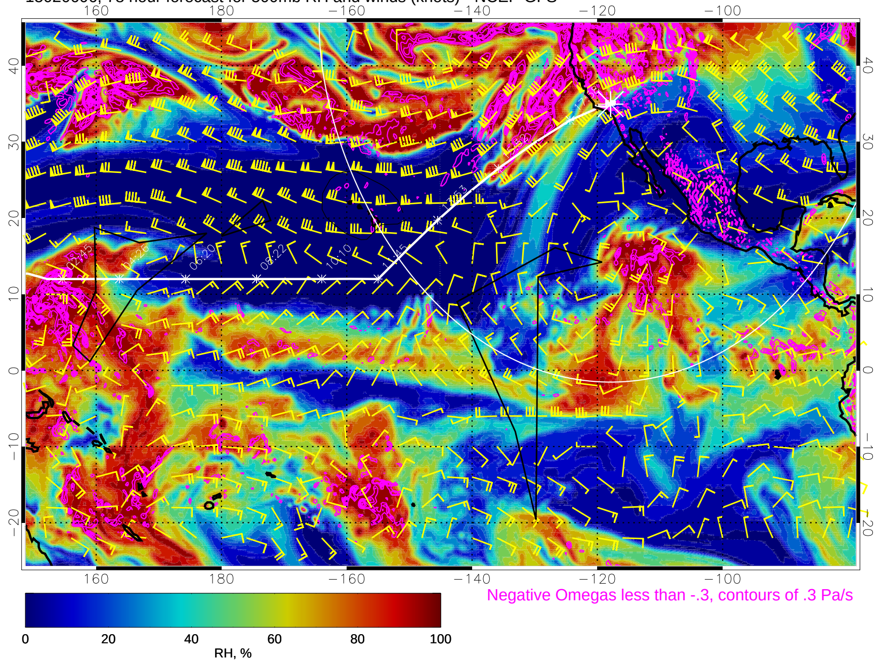
15020606, 78 hour forecast for 500mb RH and winds (knots) - NCEP GFS
