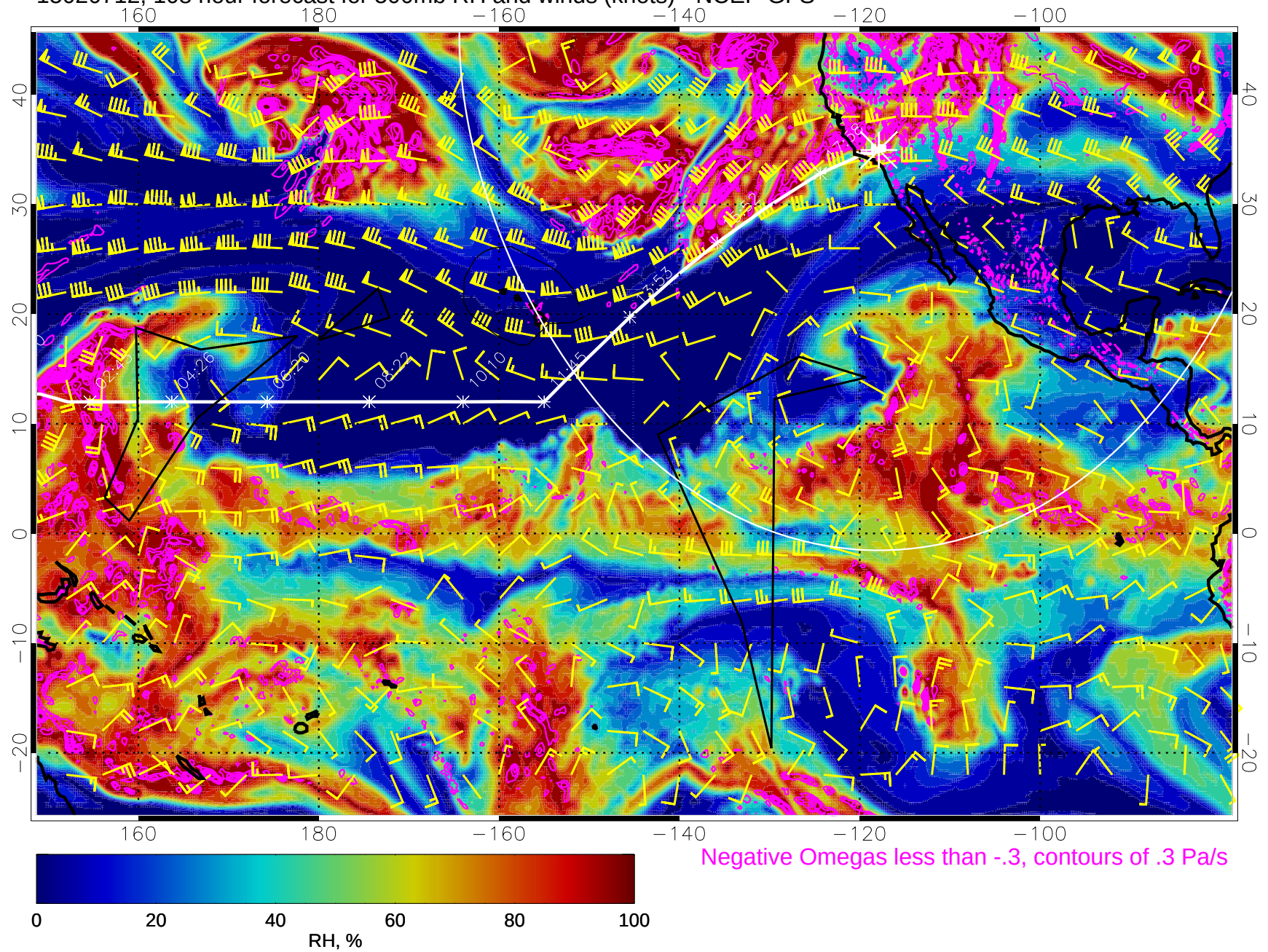
15020712, 108 hour forecast for 500mb RH and winds (knots) - NCEP GFS
