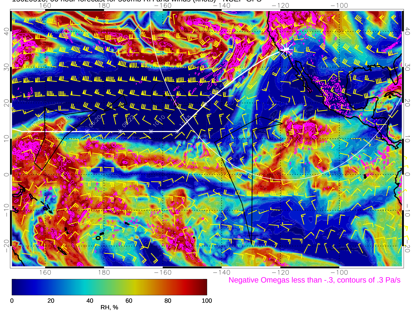
15020518, 66 hour forecast for 500mb RH and winds (knots) - NCEP GFS
