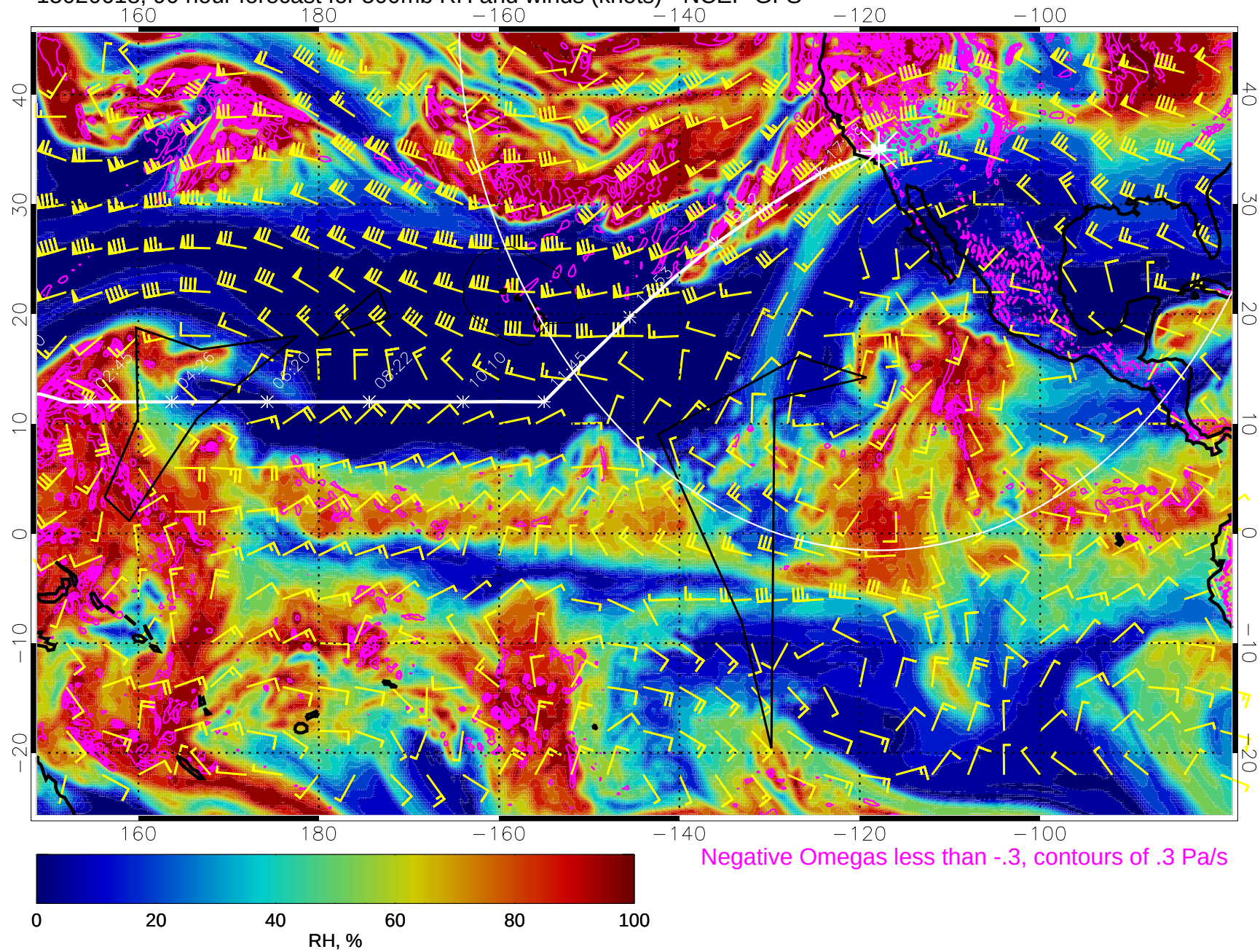
15020618, 90 hour forecast for 500mb RH and winds (knots) - NCEP GFS
