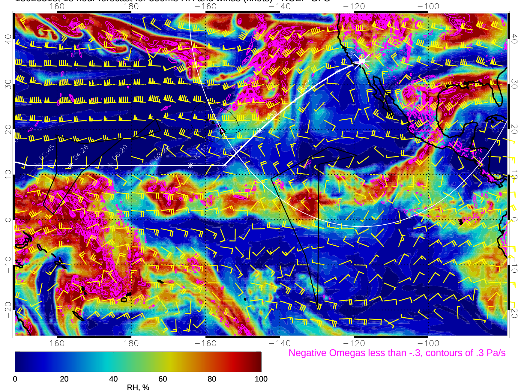
15020318, 18 hour forecast for 500mb RH and winds (knots) - NCEP GFS
