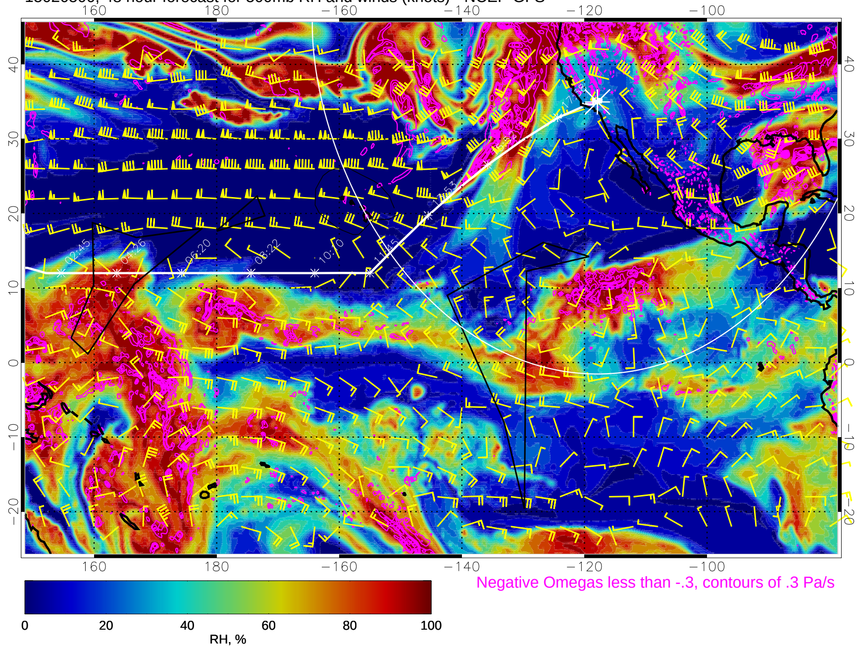
15020500, 48 hour forecast for 500mb RH and winds (knots) - NCEP GFS
