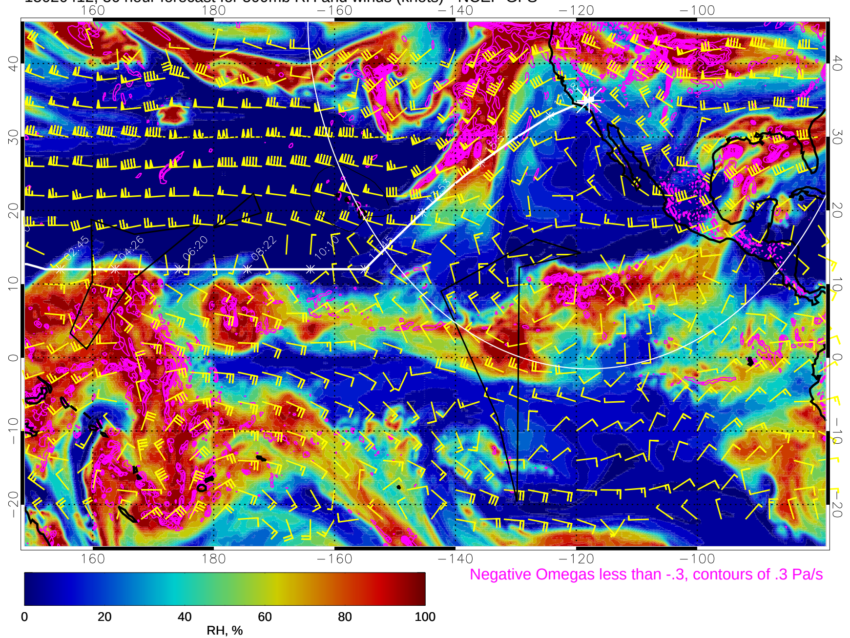
15020412, 36 hour forecast for 500mb RH and winds (knots) - NCEP GFS
