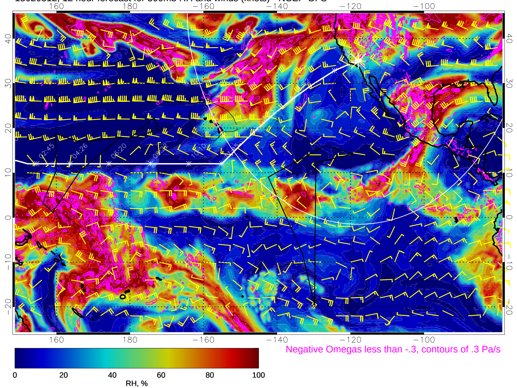
15020312, 12 hour forecast for 500mb RH and winds (knots) - NCEP GFS
