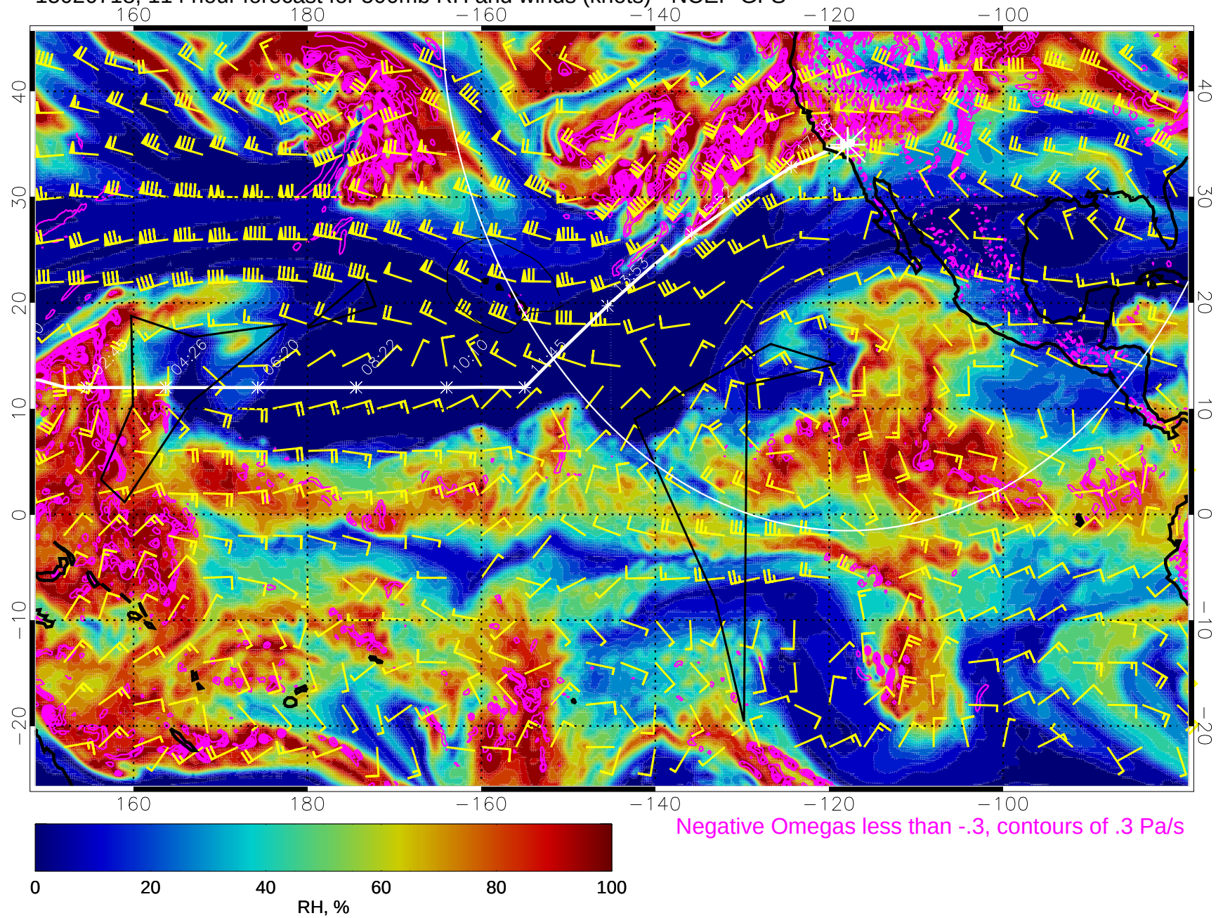
15020718, 114 hour forecast for 500mb RH and winds (knots) - NCEP GFS
