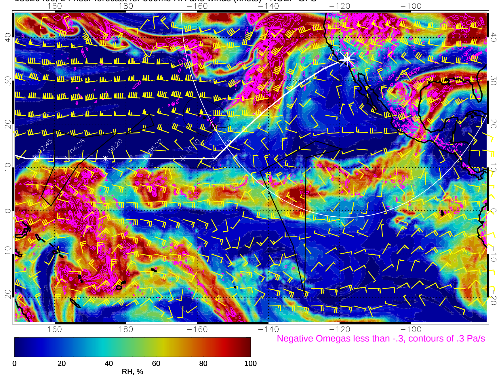
15020400, 24 hour forecast for 500mb RH and winds (knots) - NCEP GFS
