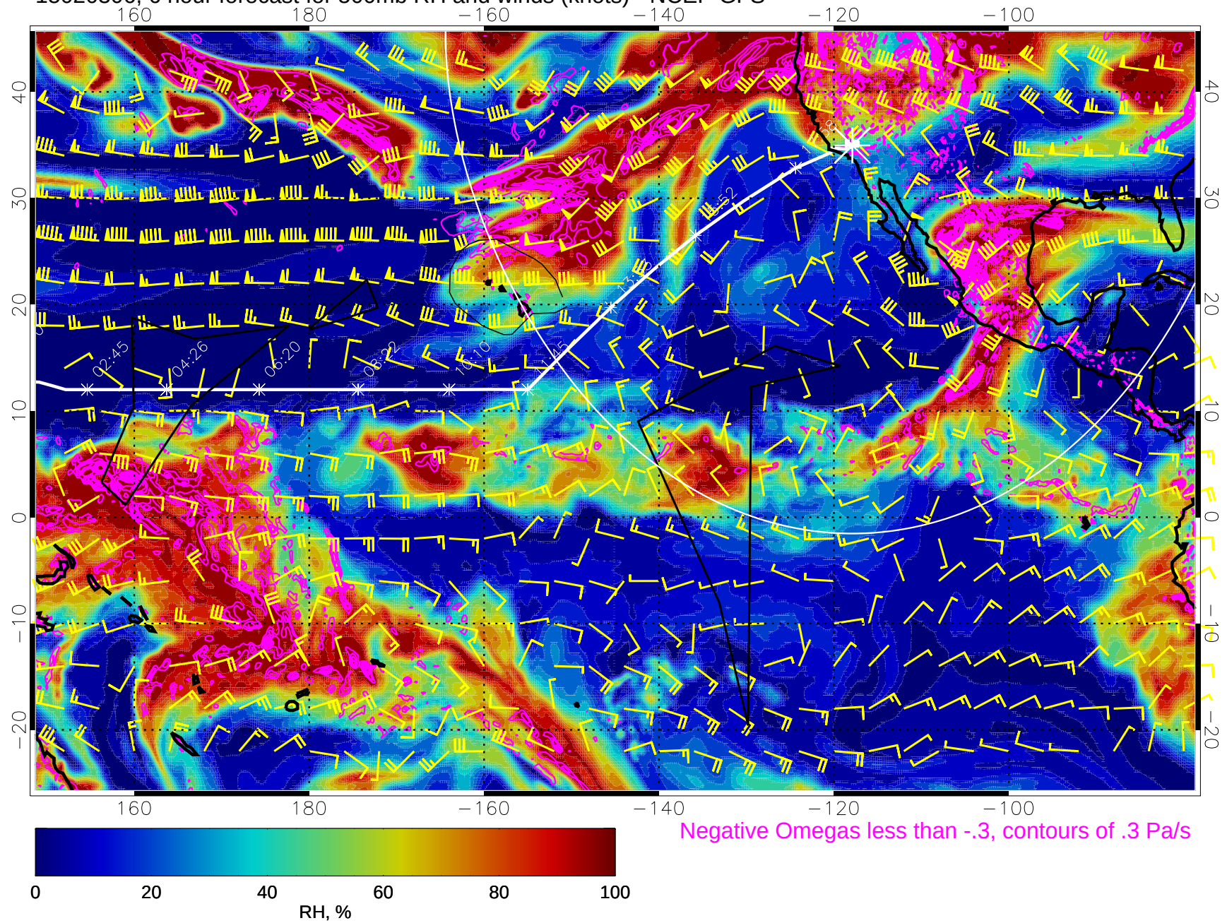
15020306, 6 hour forecast for 500mb RH and winds (knots) - NCEP GFS
