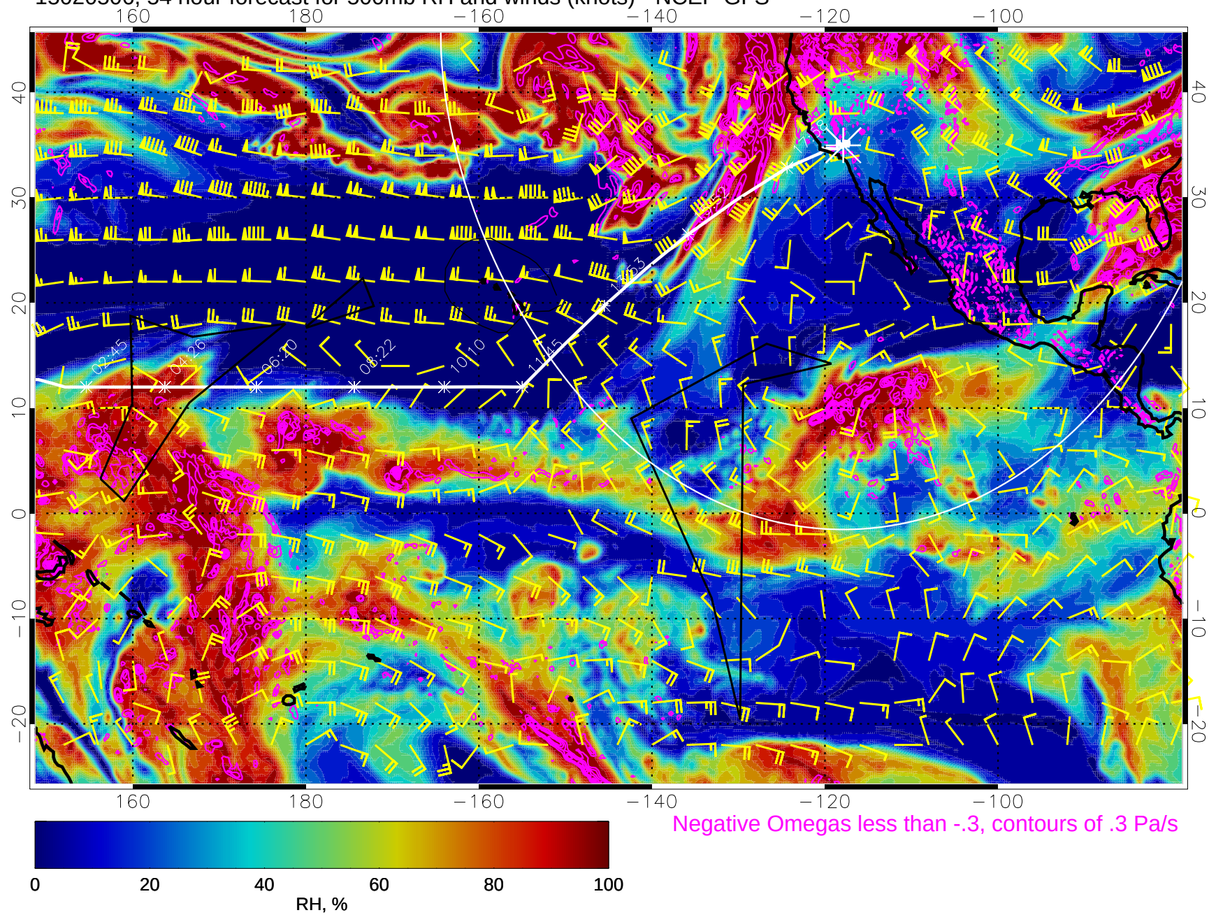
15020506, 54 hour forecast for 500mb RH and winds (knots) - NCEP GFS
