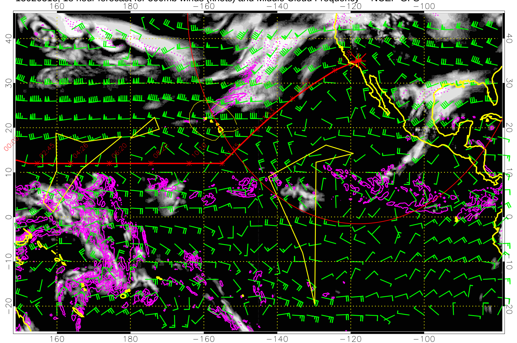
15020318, 18 hour forecast for 500mb winds (knots) and Middle Cloud Frequency -- NCEP GFS
