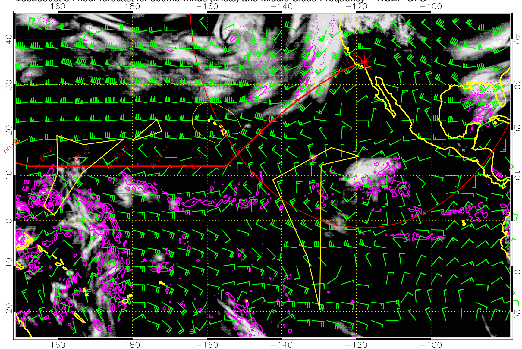
15020506, 54 hour forecast for 500mb winds (knots) and Middle Cloud Frequency -- NCEP GFS
