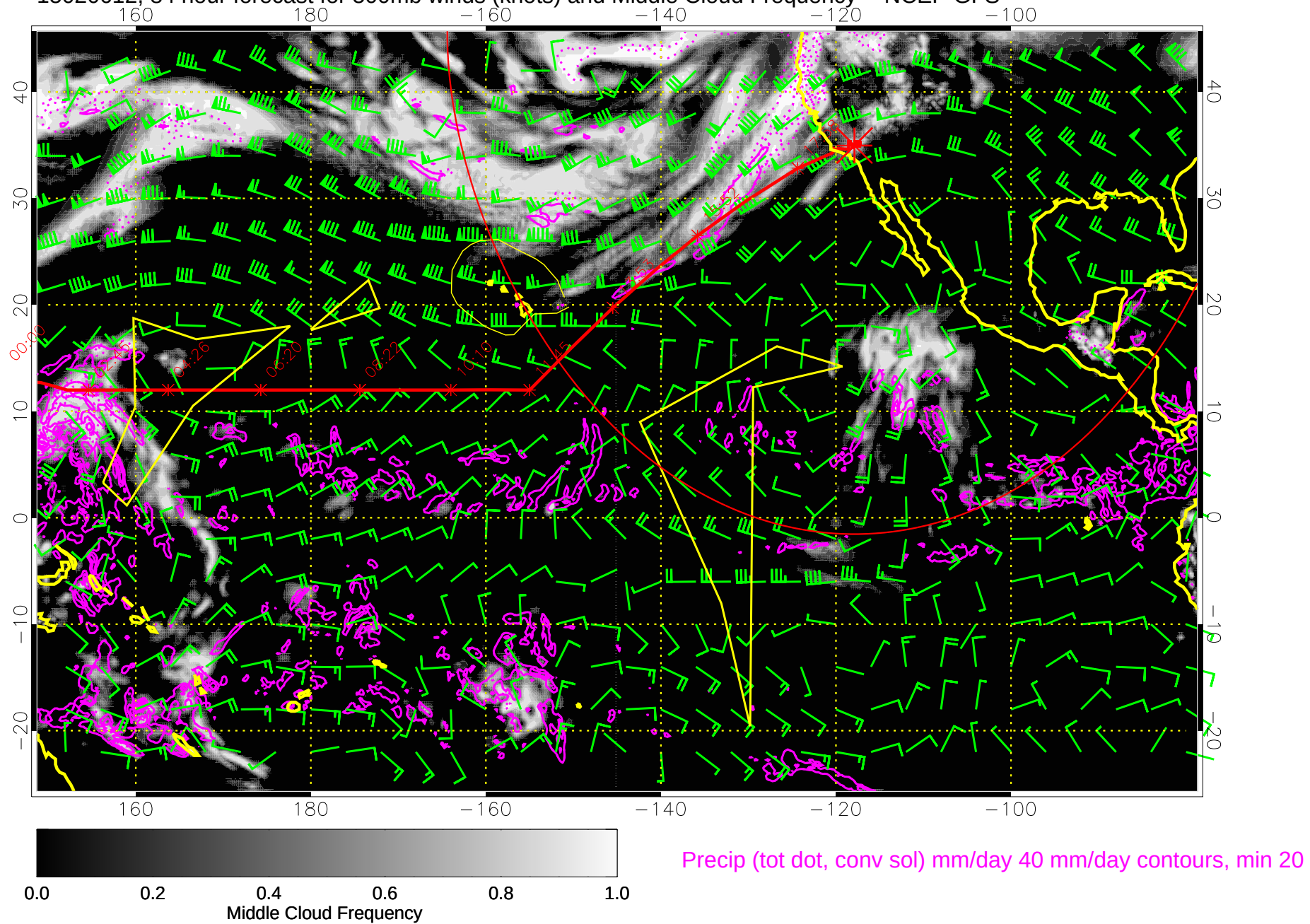
15020612, 84 hour forecast for 500mb winds (knots) and Middle Cloud Frequency -- NCEP GFS
