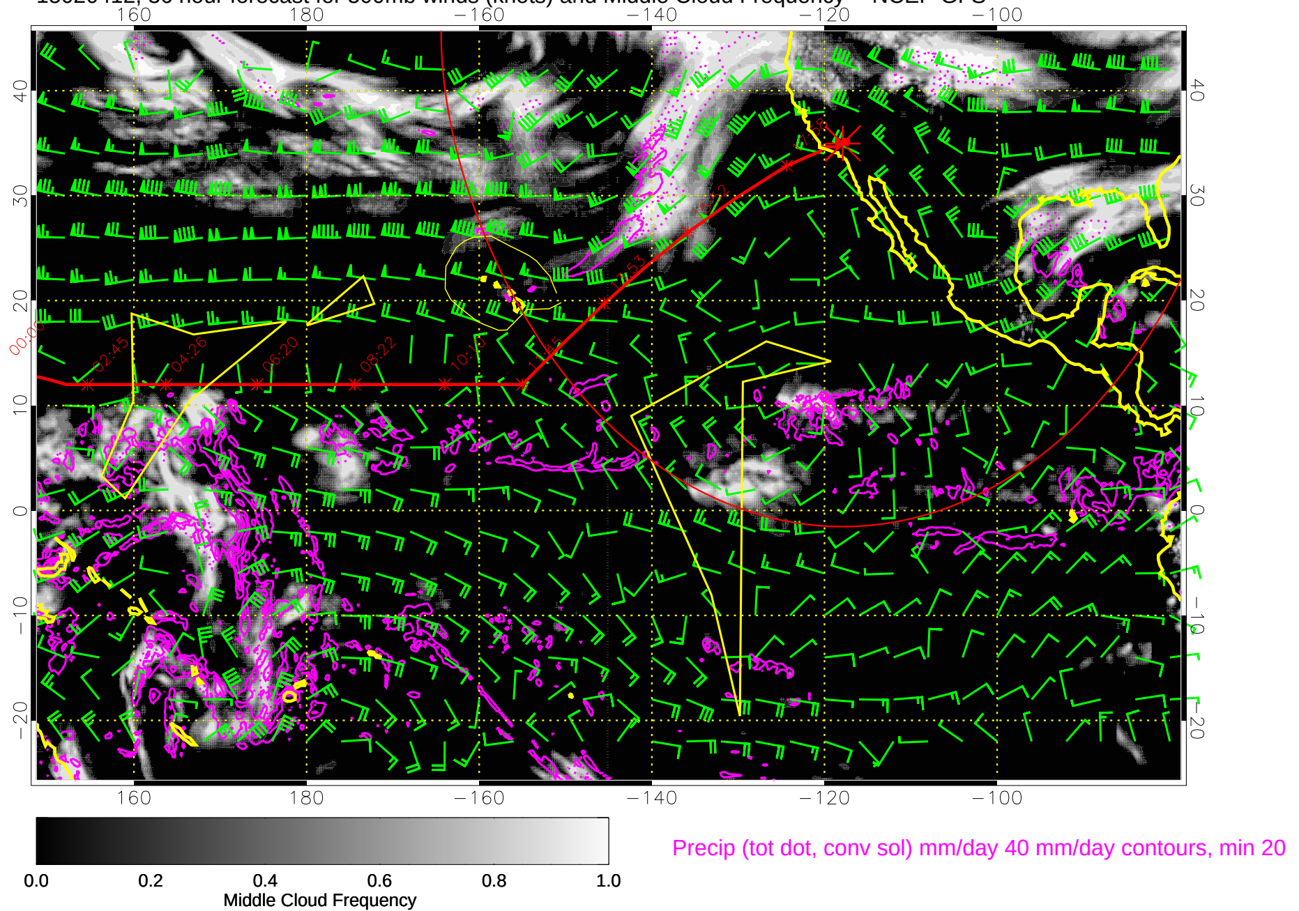
15020412, 36 hour forecast for 500mb winds (knots) and Middle Cloud Frequency -- NCEP GFS
