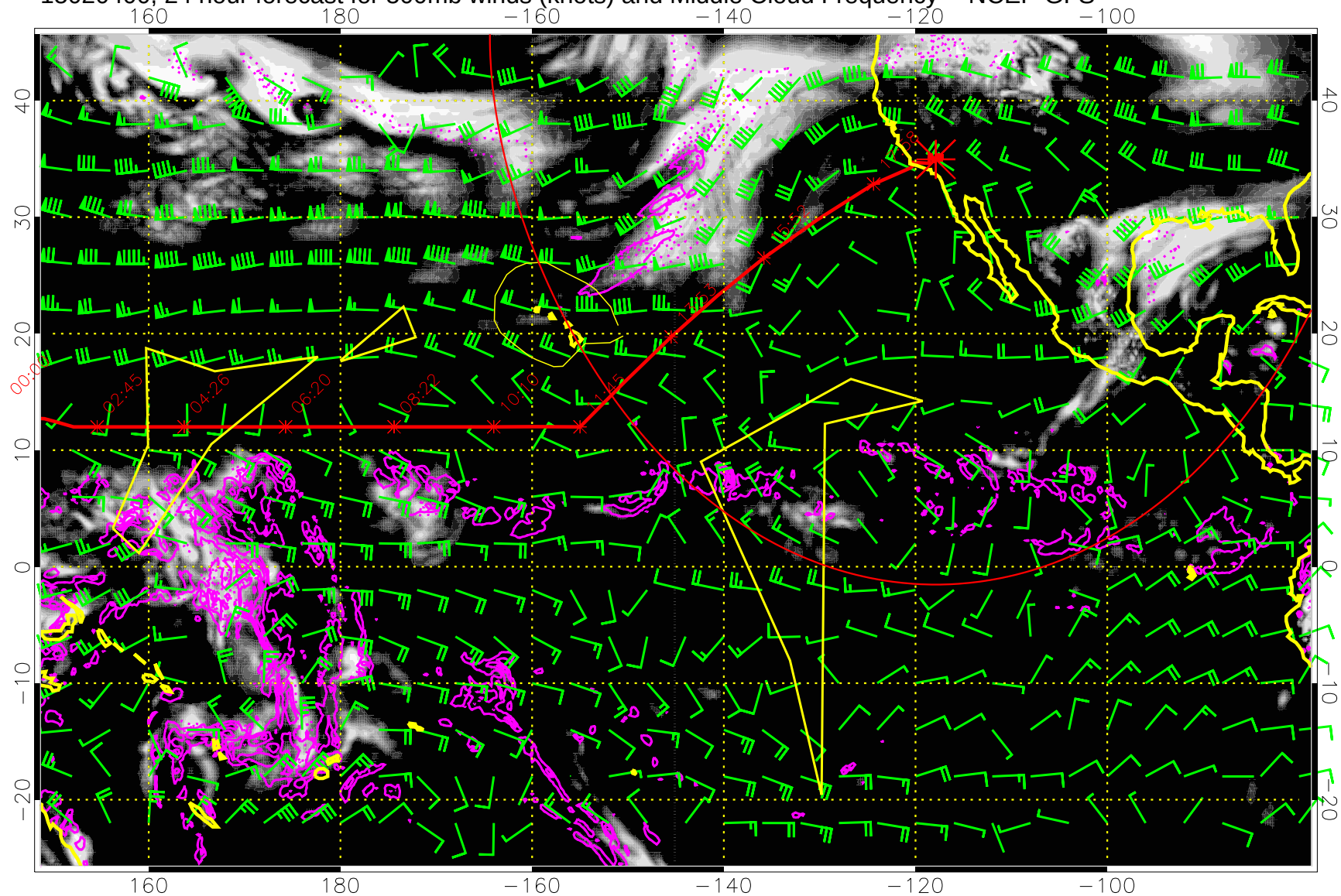
15020400, 24 hour forecast for 500mb winds (knots) and Middle Cloud Frequency -- NCEP GFS
