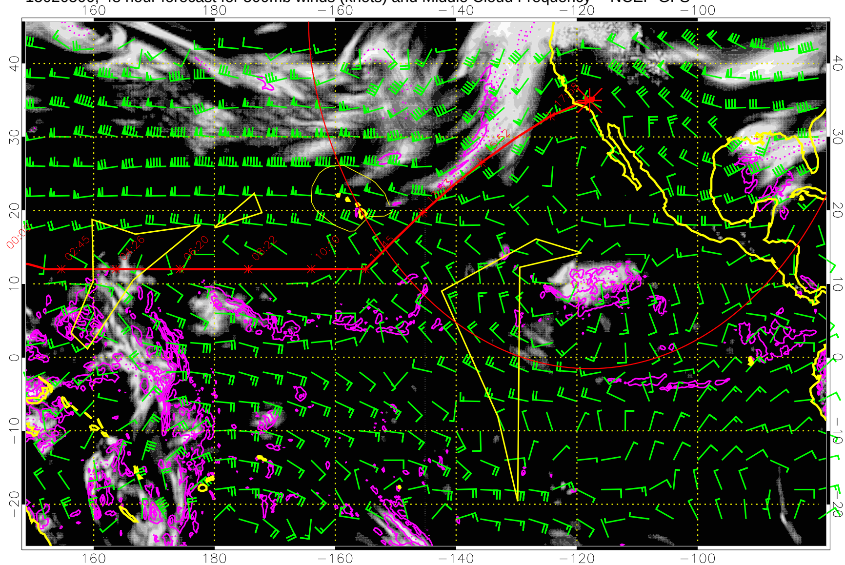
15020500, 48 hour forecast for 500mb winds (knots) and Middle Cloud Frequency -- NCEP GFS
