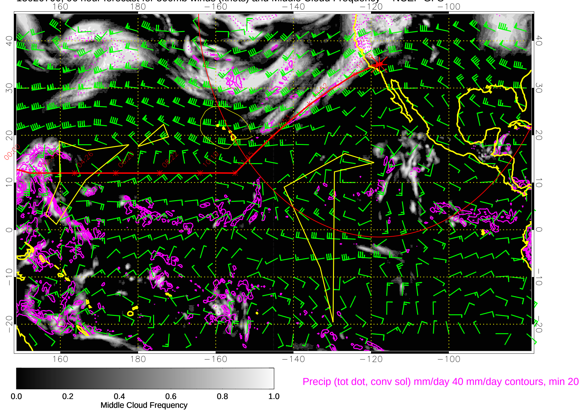
15020700, 96 hour forecast for 500mb winds (knots) and Middle Cloud Frequency -- NCEP GFS
