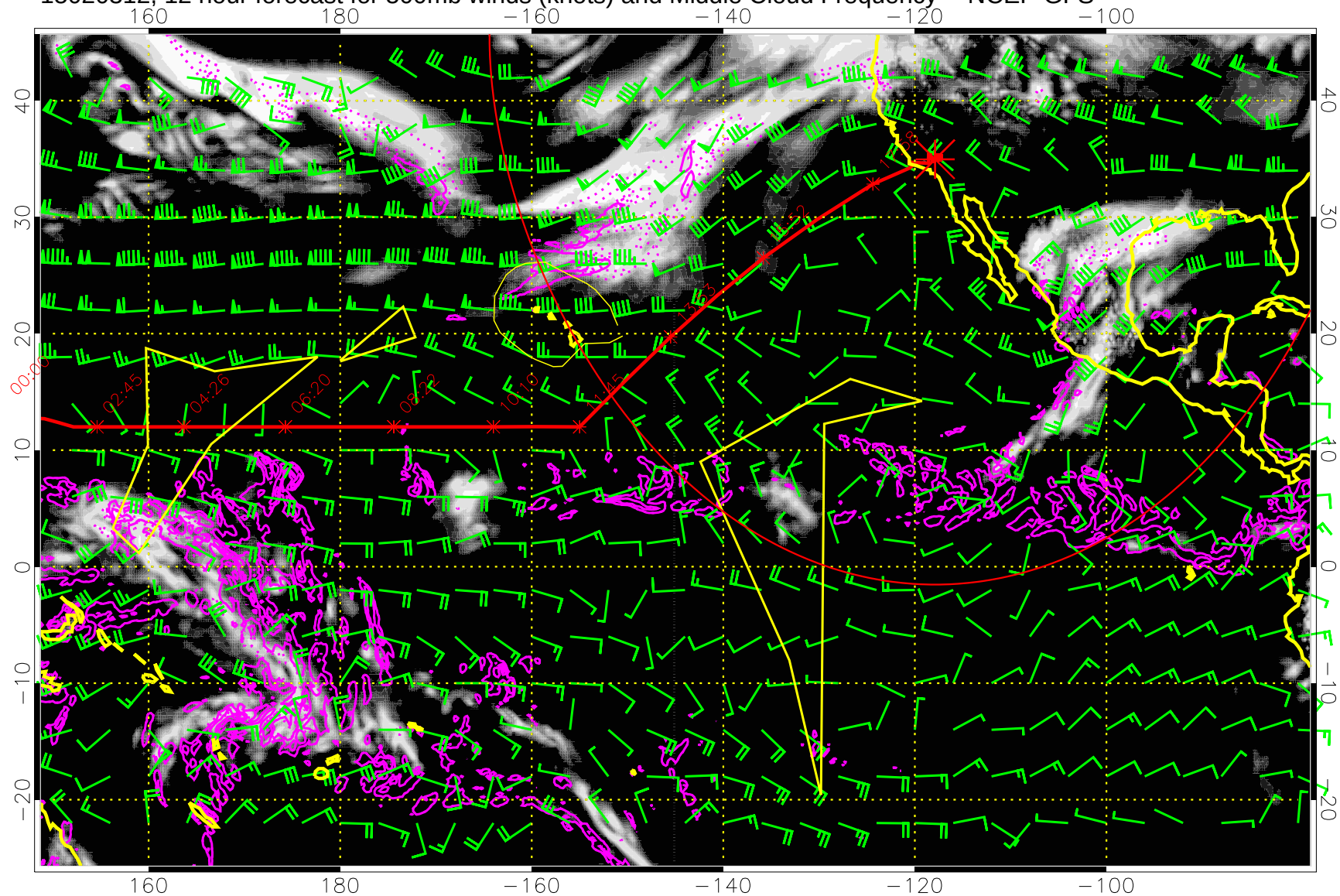
15020312, 12 hour forecast for 500mb winds (knots) and Middle Cloud Frequency -- NCEP GFS
