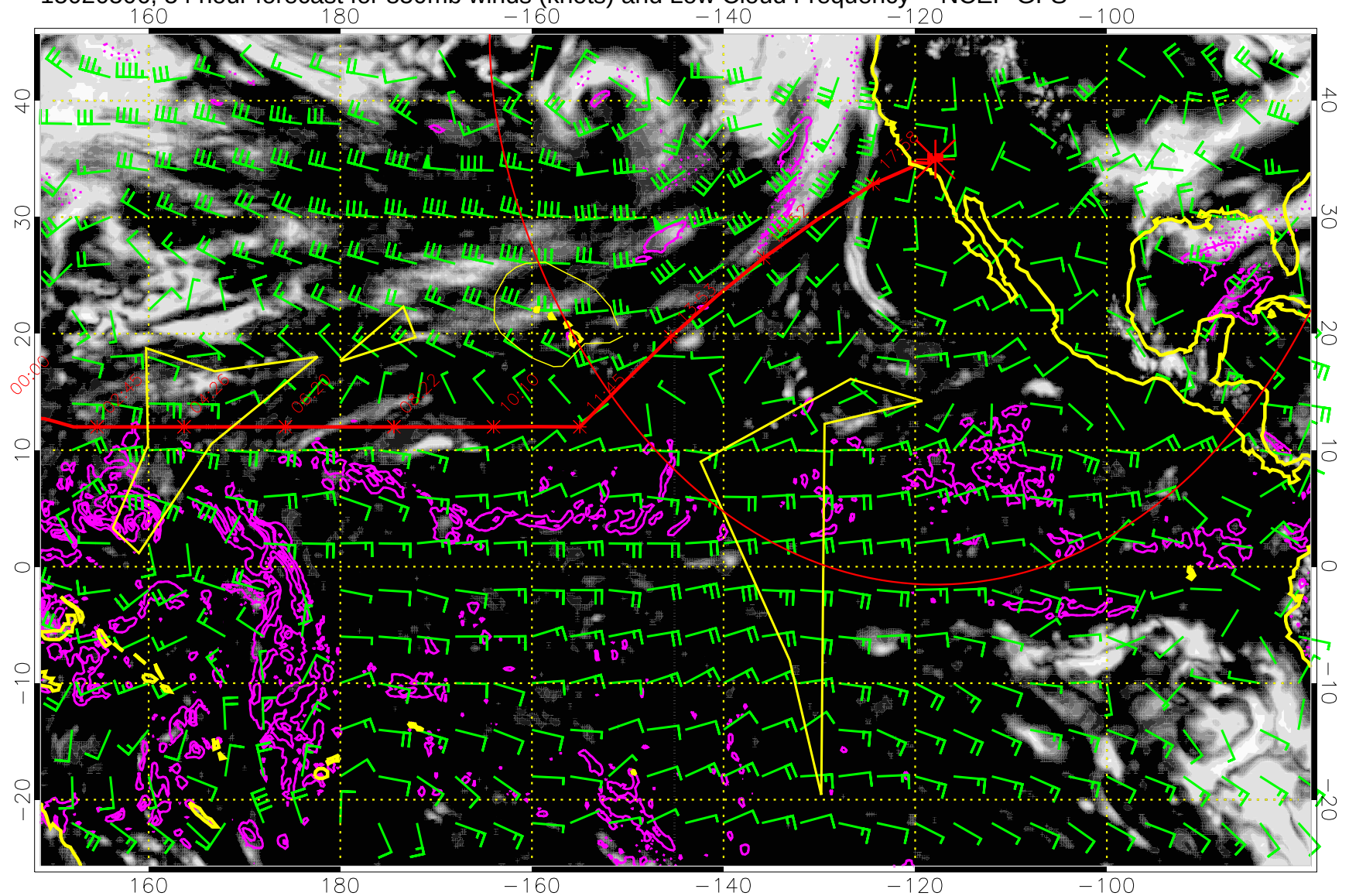
15020506, 54 hour forecast for 850mb winds (knots) and Low Cloud Frequency -- NCEP GFS
