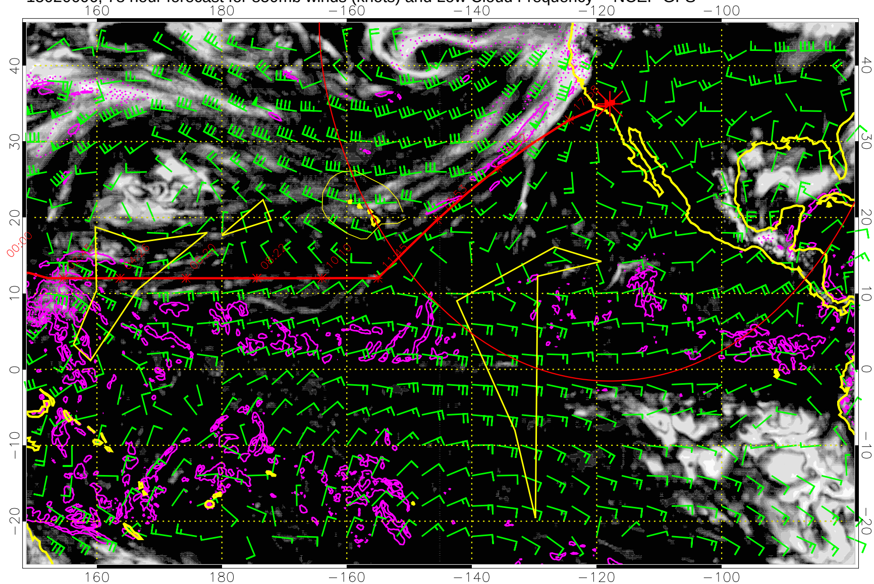
15020606, 78 hour forecast for 850mb winds (knots) and Low Cloud Frequency -- NCEP GFS
