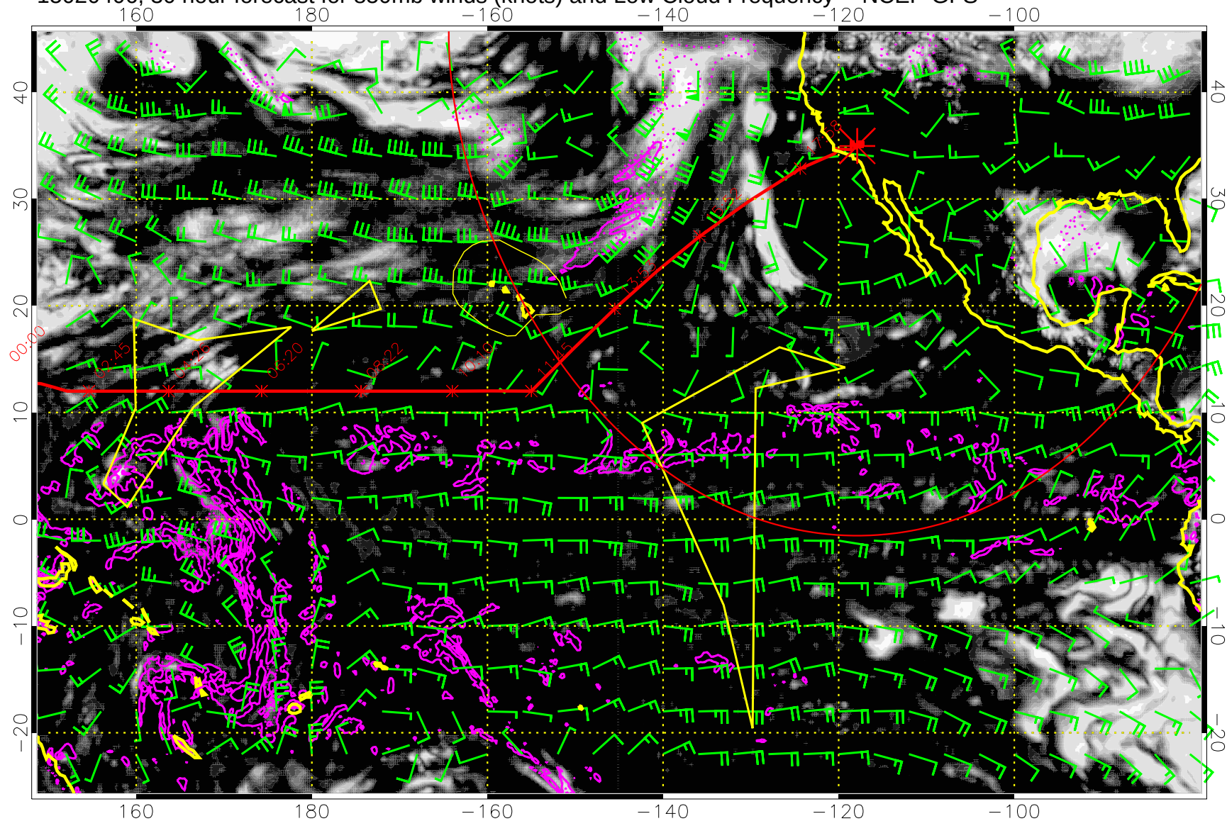
15020406, 30 hour forecast for 850mb winds (knots) and Low Cloud Frequency -- NCEP GFS
