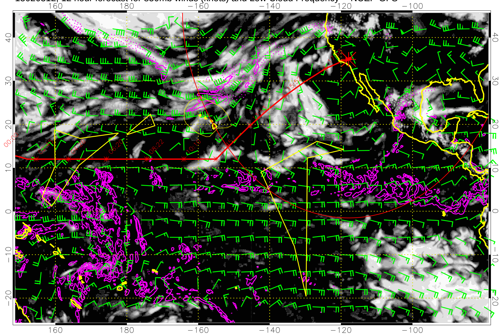
15020312, 12 hour forecast for 850mb winds (knots) and Low Cloud Frequency -- NCEP GFS
