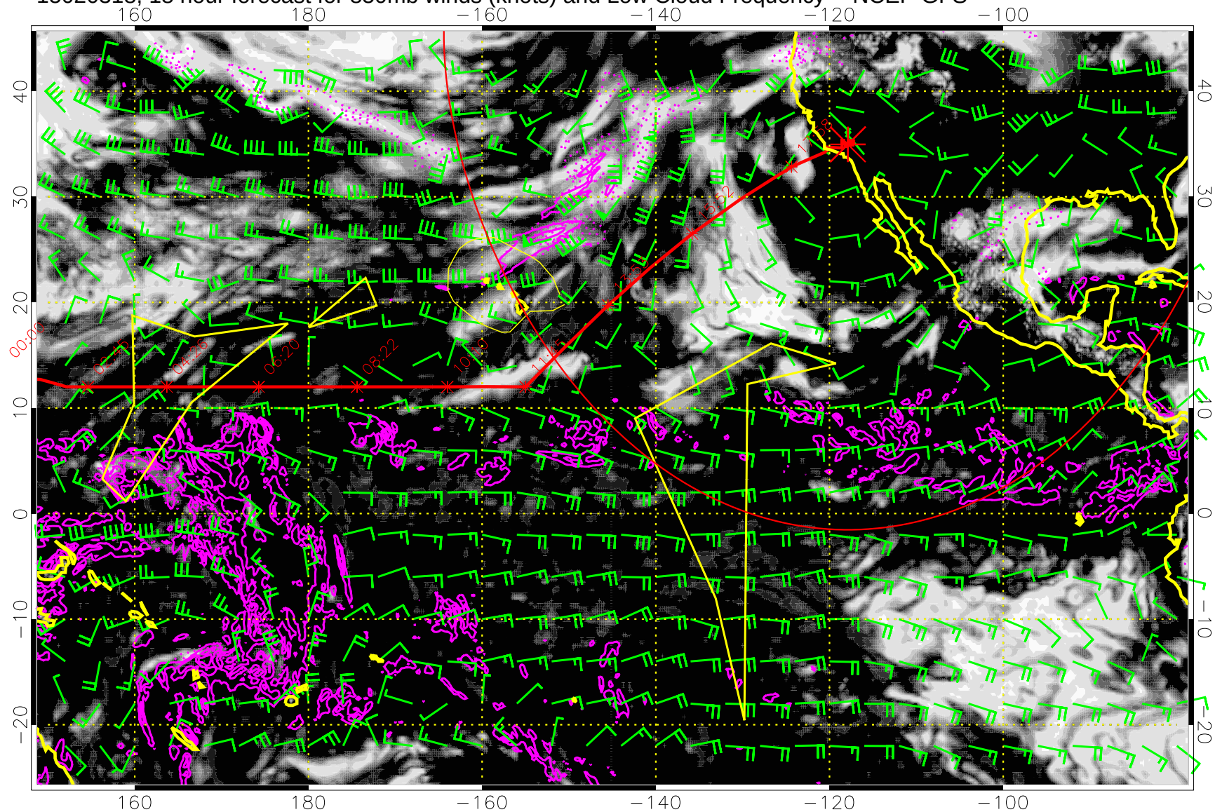
15020318, 18 hour forecast for 850mb winds (knots) and Low Cloud Frequency -- NCEP GFS
