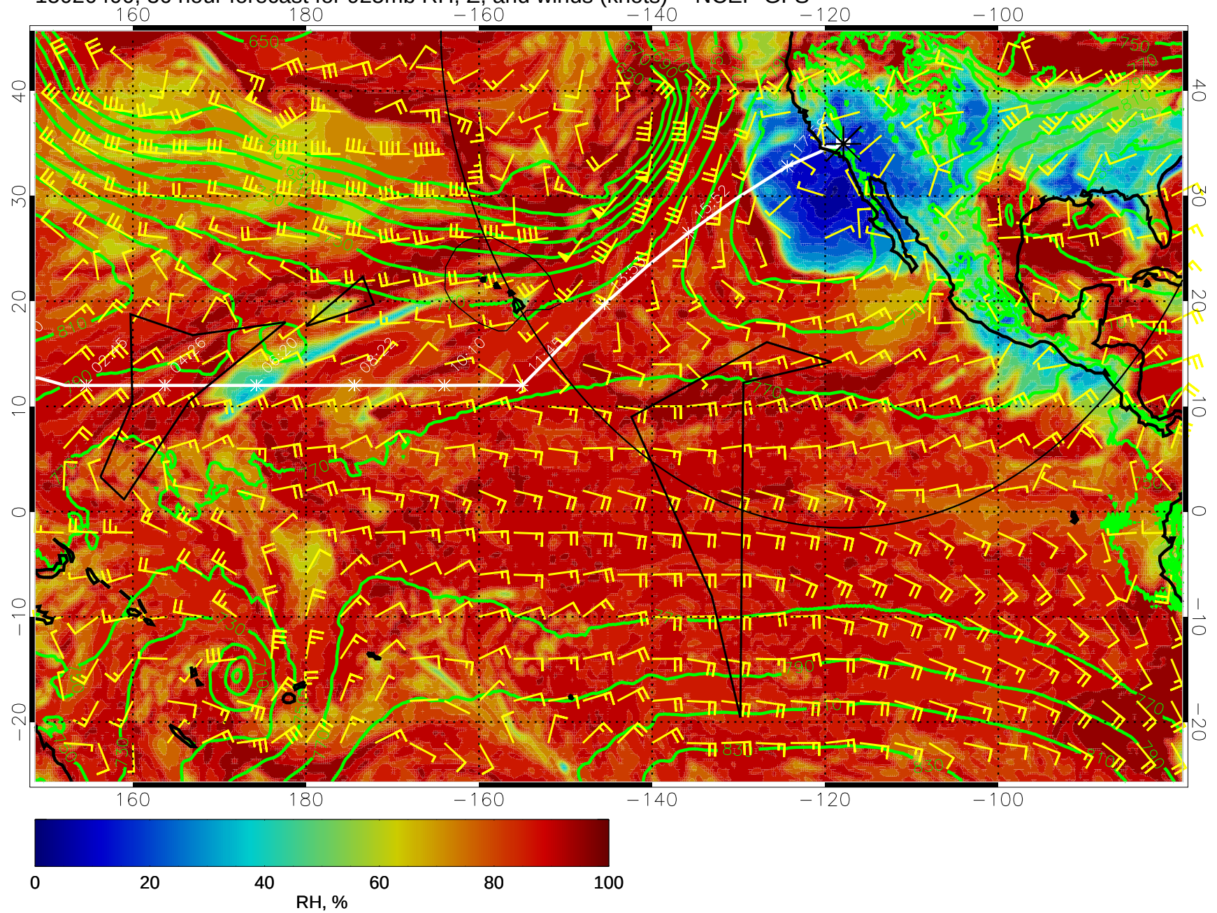
15020400, 36 hour forecast for 925mb RH, Z, and winds (knots) -- NCEP GFS
