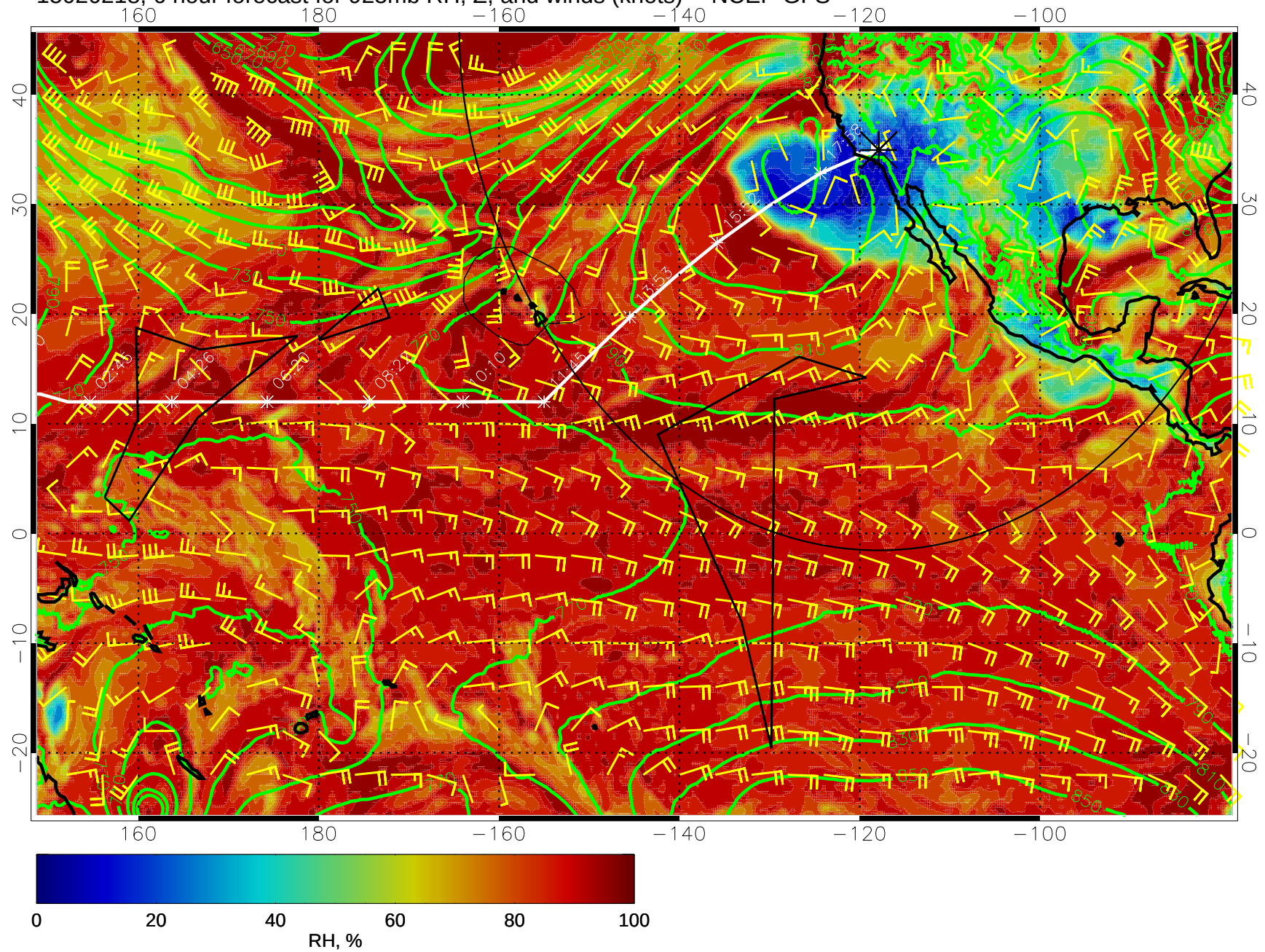
15020218, 6 hour forecast for 925mb RH, Z, and winds (knots) -- NCEP GFS
