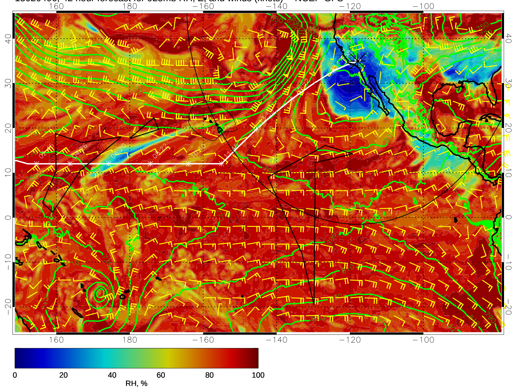
15020406, 42 hour forecast for 925mb RH, Z, and winds (knots) -- NCEP GFS
