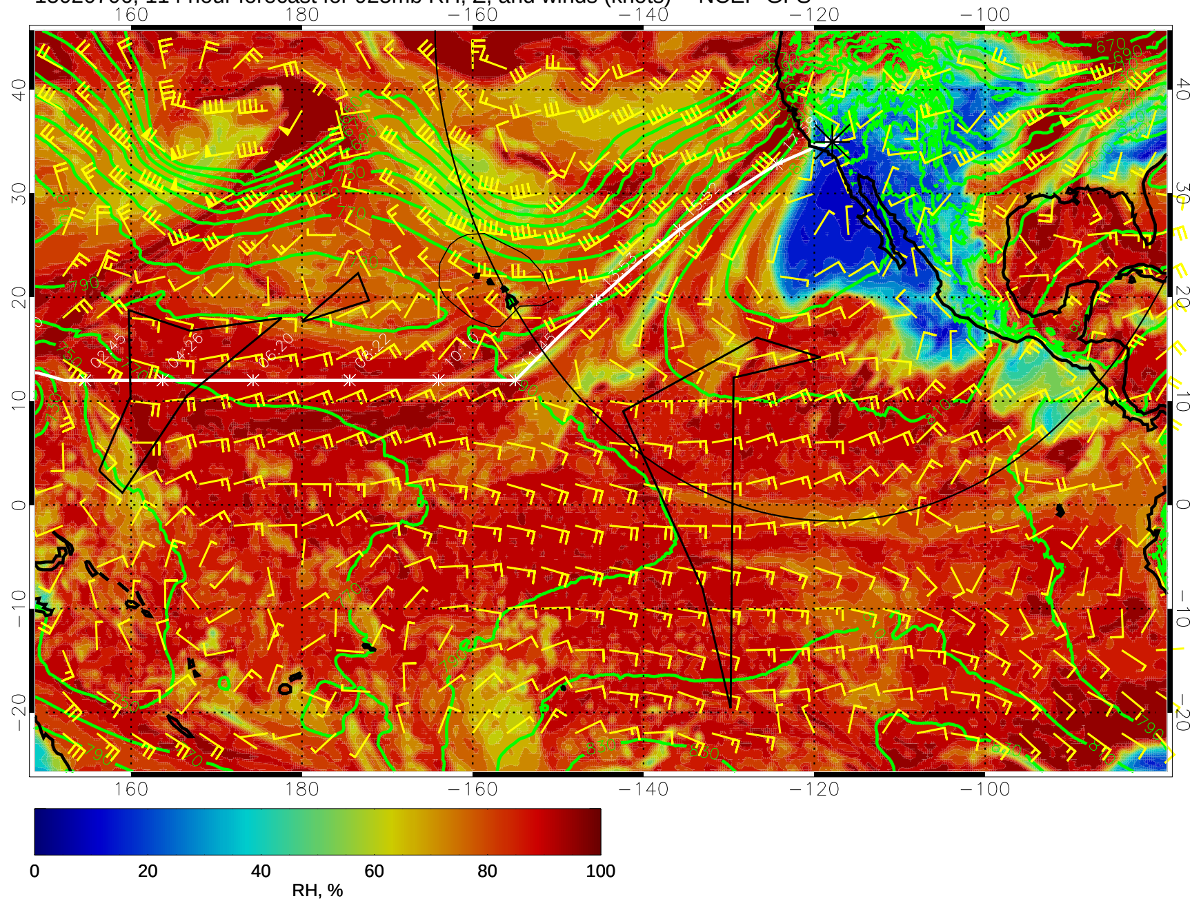
15020706, 114 hour forecast for 925mb RH, Z, and winds (knots) -- NCEP GFS
