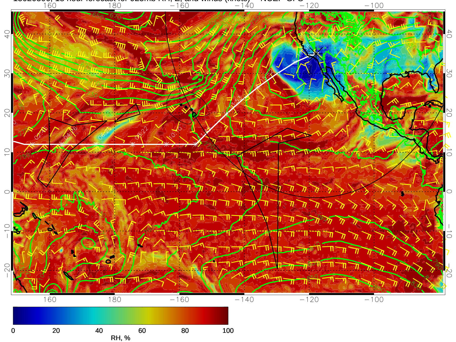
15020306, 18 hour forecast for 925mb RH, Z, and winds (knots) -- NCEP GFS
