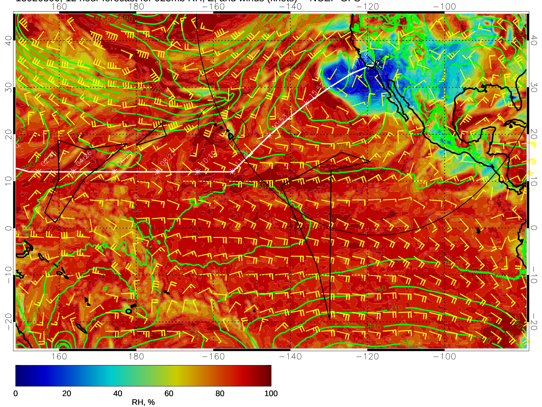
15020300, 12 hour forecast for 925mb RH, Z, and winds (knots) -- NCEP GFS
