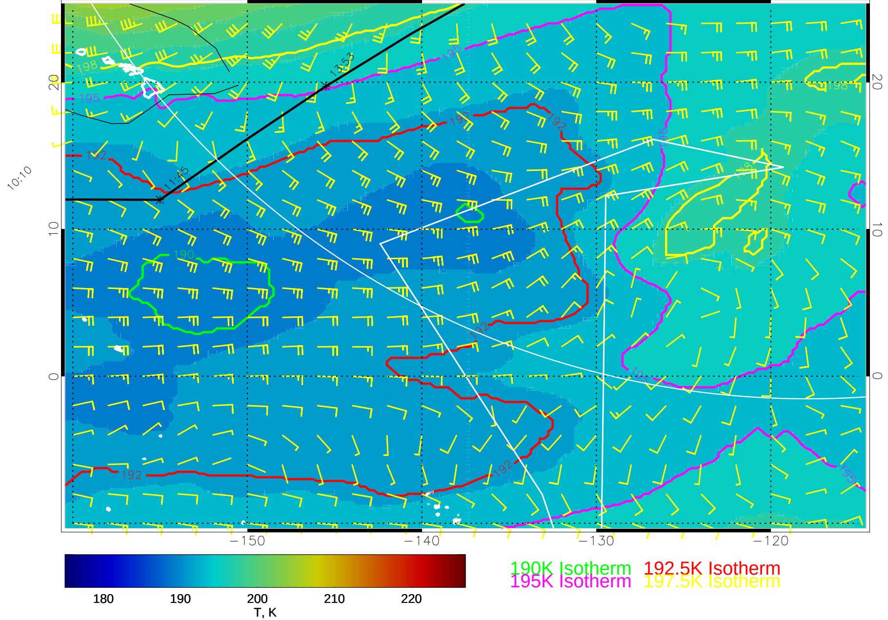
15020706, 114 hour forecast for 70mb T and winds (knots) -- NCEP GFS
