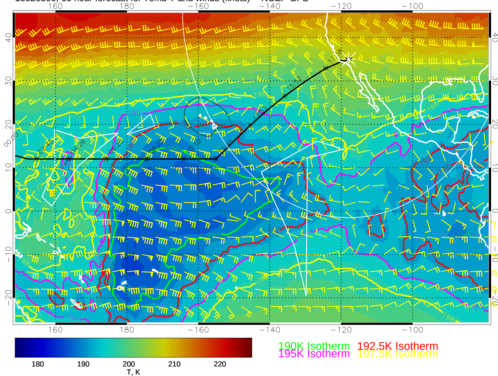
15020500, 60 hour forecast for 70mb T and winds (knots) -- NCEP GFS
