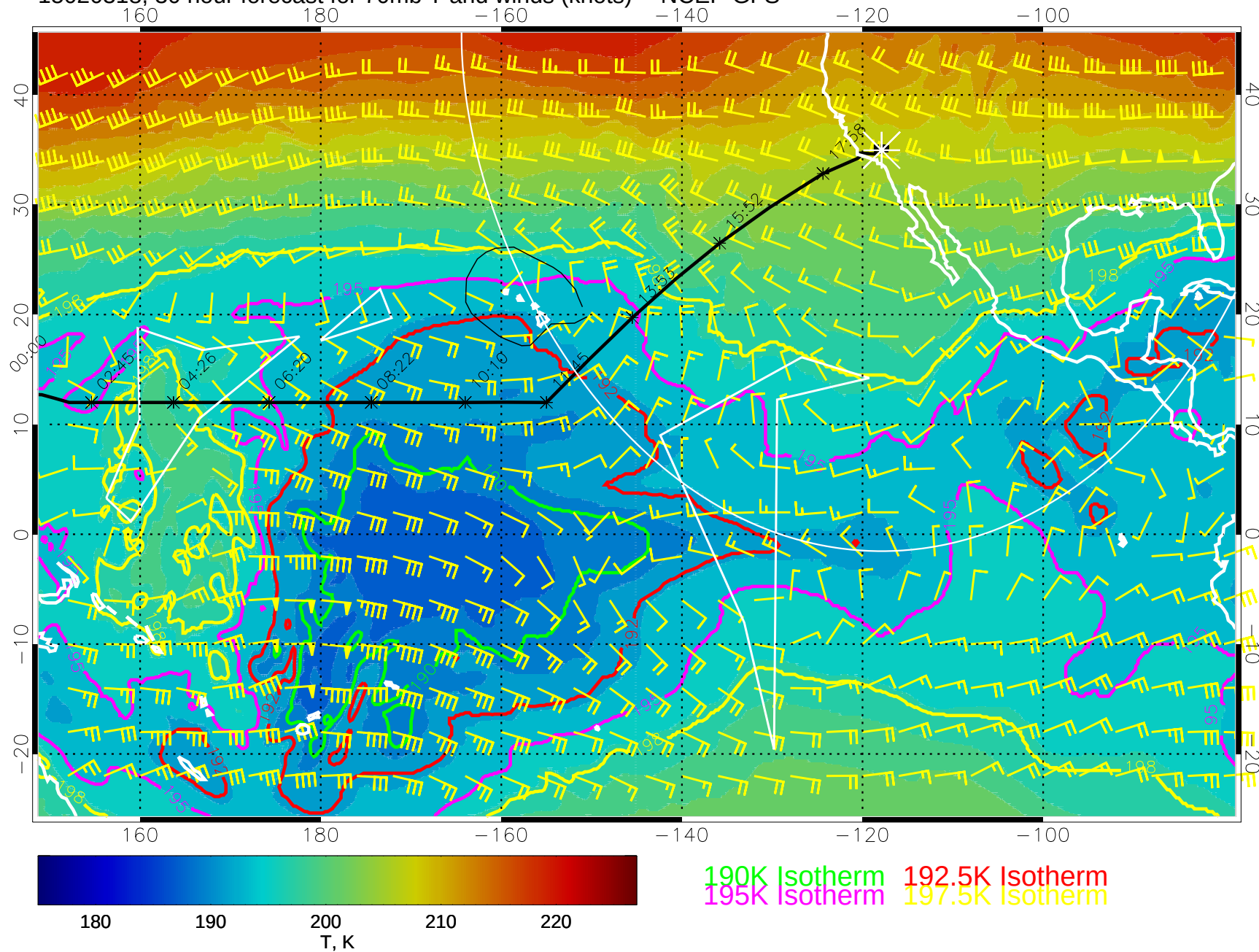
15020318, 30 hour forecast for 70mb T and winds (knots) -- NCEP GFS
