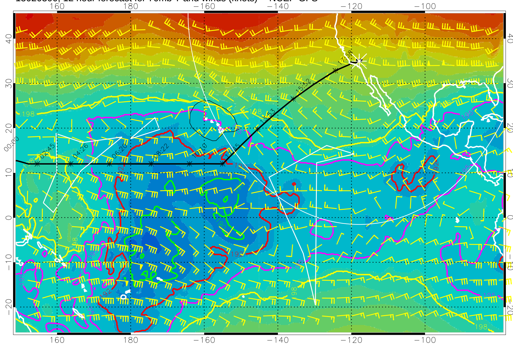
15020300, 12 hour forecast for 70mb T and winds (knots) -- NCEP GFS
