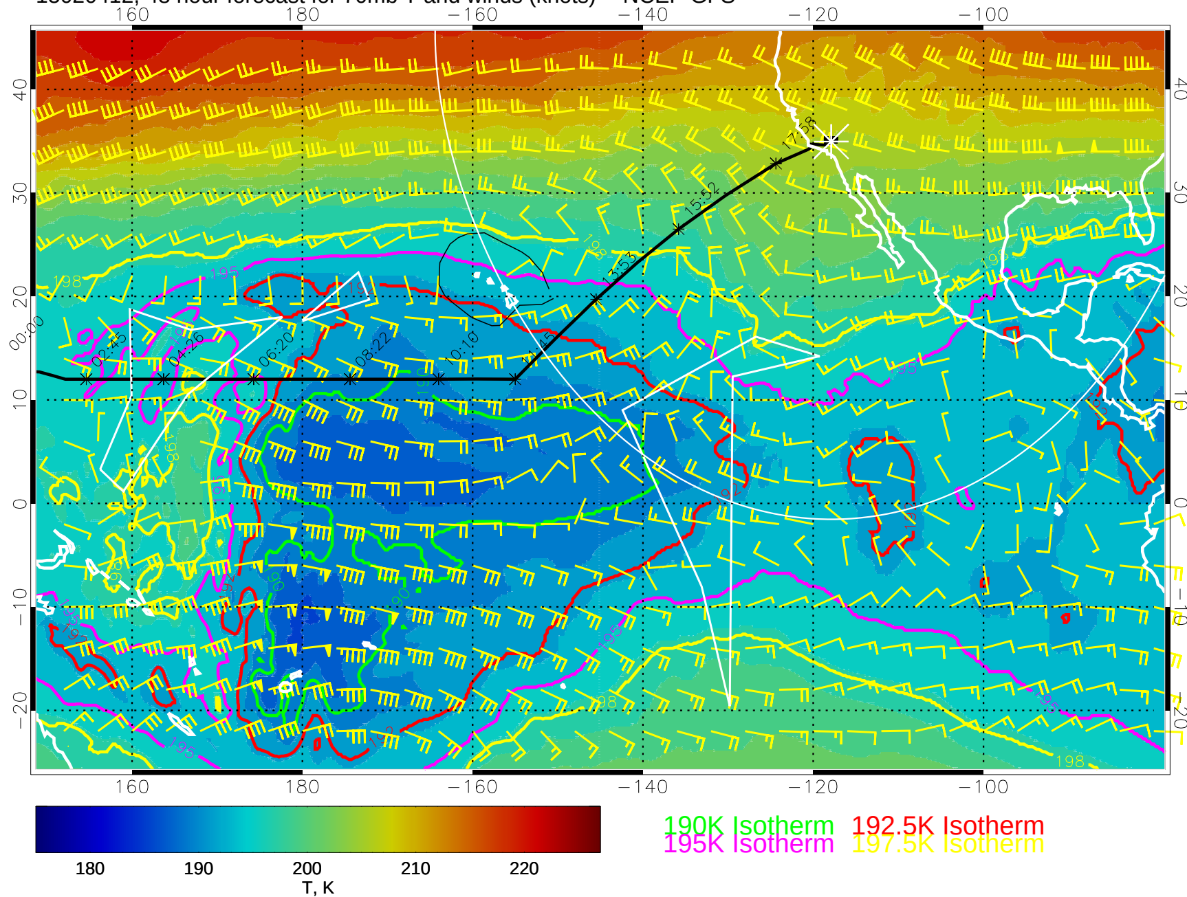
15020412, 48 hour forecast for 70mb T and winds (knots) -- NCEP GFS
