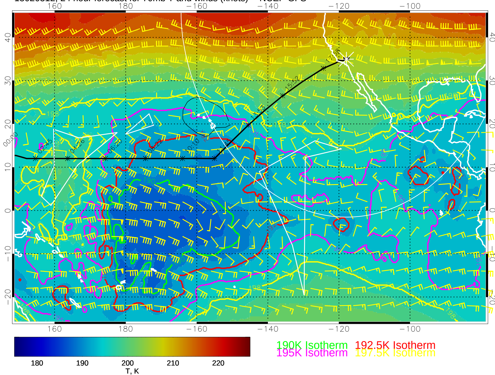
15020312, 24 hour forecast for 70mb T and winds (knots) -- NCEP GFS
