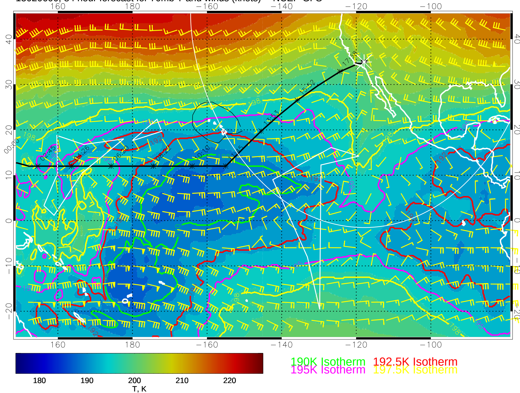
15020600, 84 hour forecast for 70mb T and winds (knots) -- NCEP GFS
