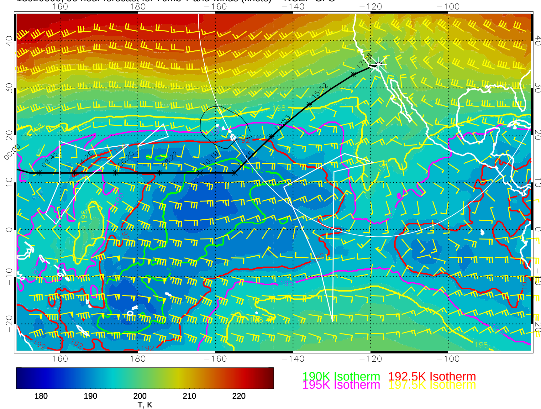
15020606, 90 hour forecast for 70mb T and winds (knots) -- NCEP GFS
