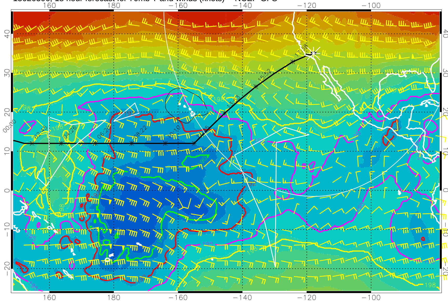
15020306, 18 hour forecast for 70mb T and winds (knots) -- NCEP GFS
