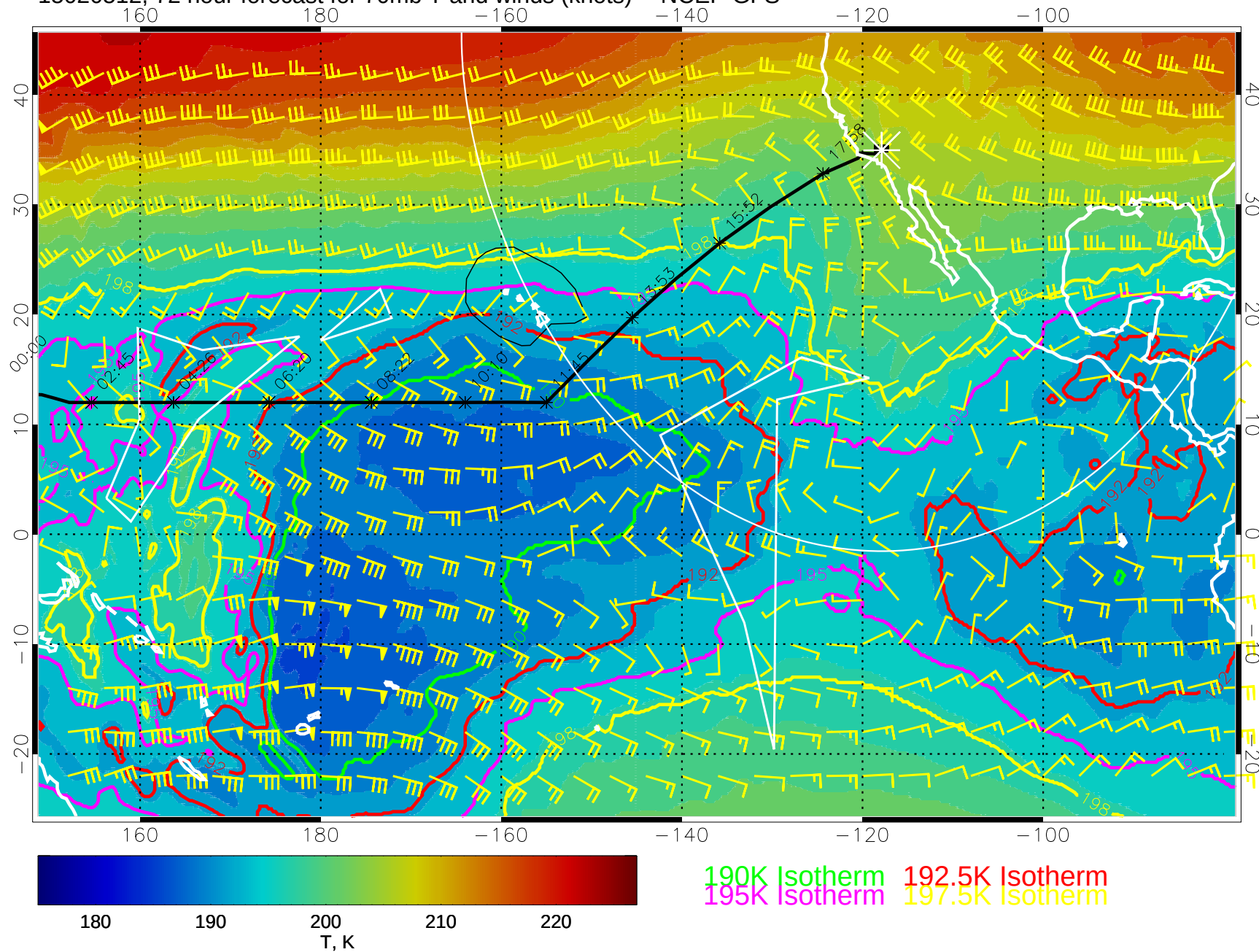
15020512, 72 hour forecast for 70mb T and winds (knots) -- NCEP GFS
