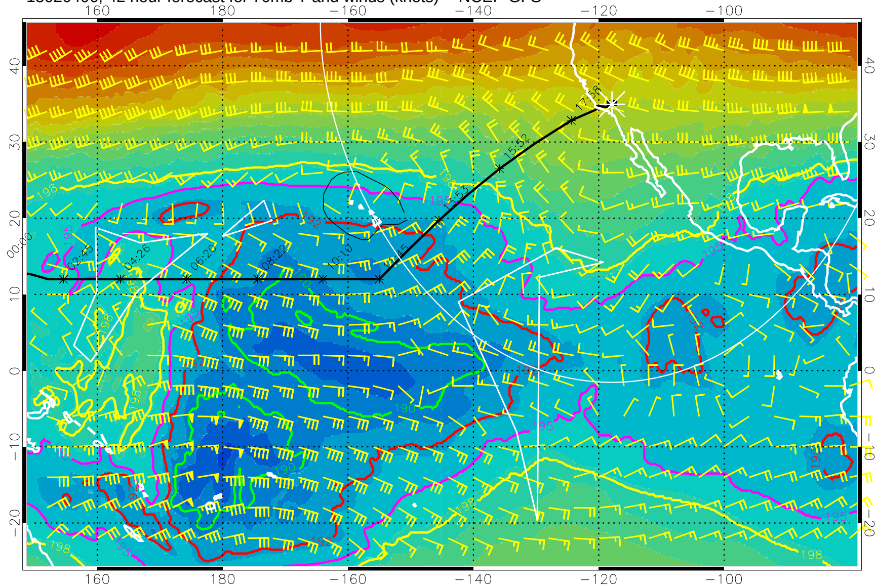
15020406, 42 hour forecast for 70mb T and winds (knots) -- NCEP GFS
