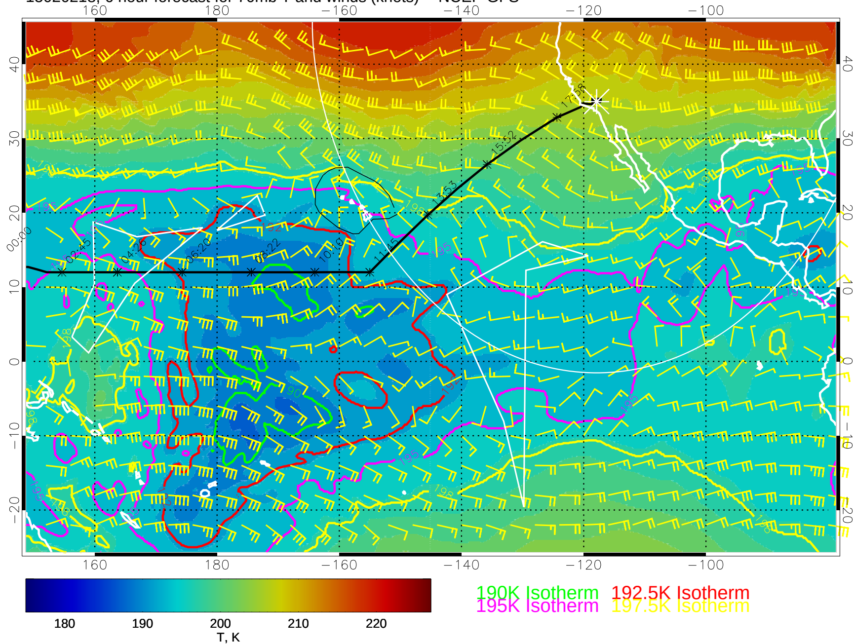
15020218, 6 hour forecast for 70mb T and winds (knots) -- NCEP GFS
