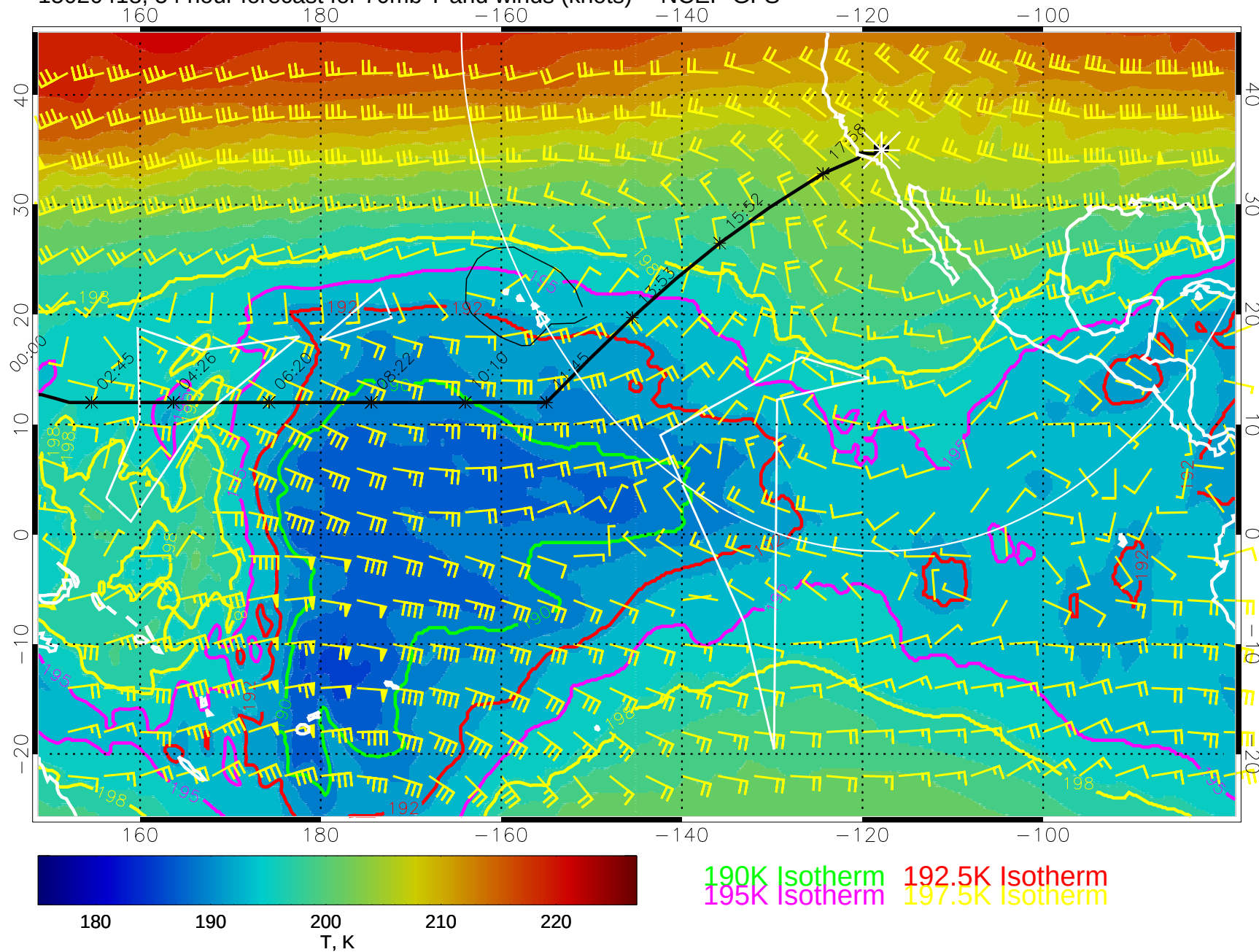
15020418, 54 hour forecast for 70mb T and winds (knots) -- NCEP GFS
