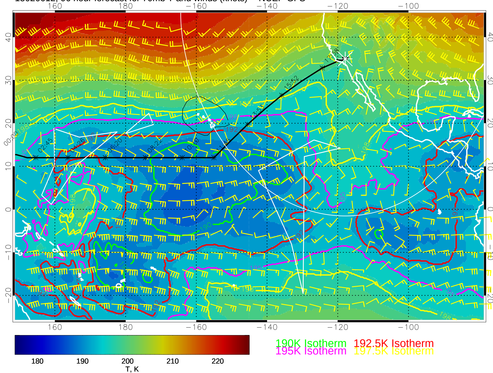
15020612, 96 hour forecast for 70mb T and winds (knots) -- NCEP GFS
