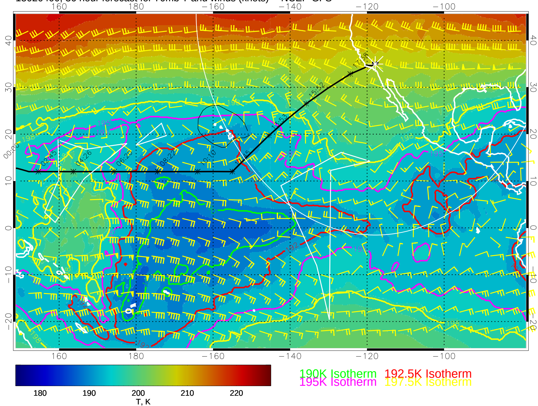
15020400, 36 hour forecast for 70mb T and winds (knots) -- NCEP GFS
