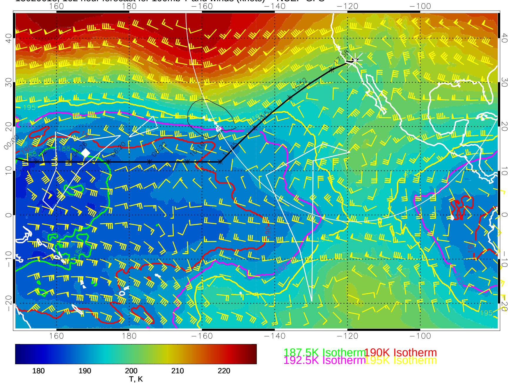
15020618, 102 hour forecast for 100mb T and winds (knots) -- NCEP GFS
