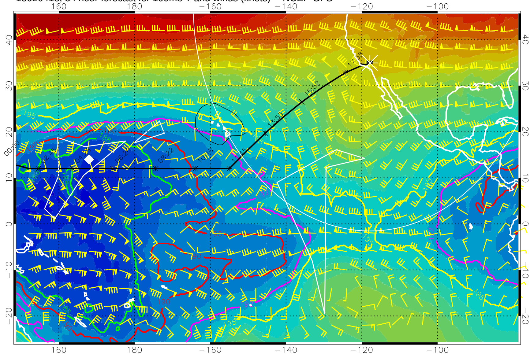
15020418, 54 hour forecast for 100mb T and winds (knots) -- NCEP GFS
