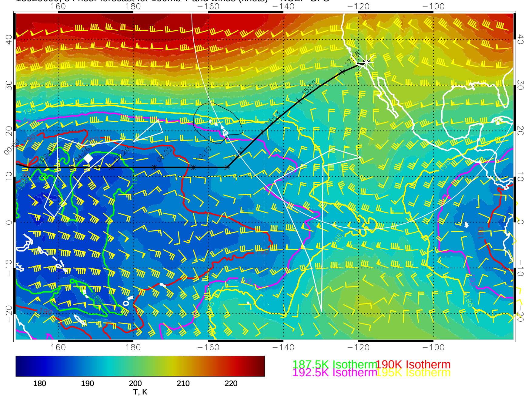
15020600, 84 hour forecast for 100mb T and winds (knots) -- NCEP GFS
