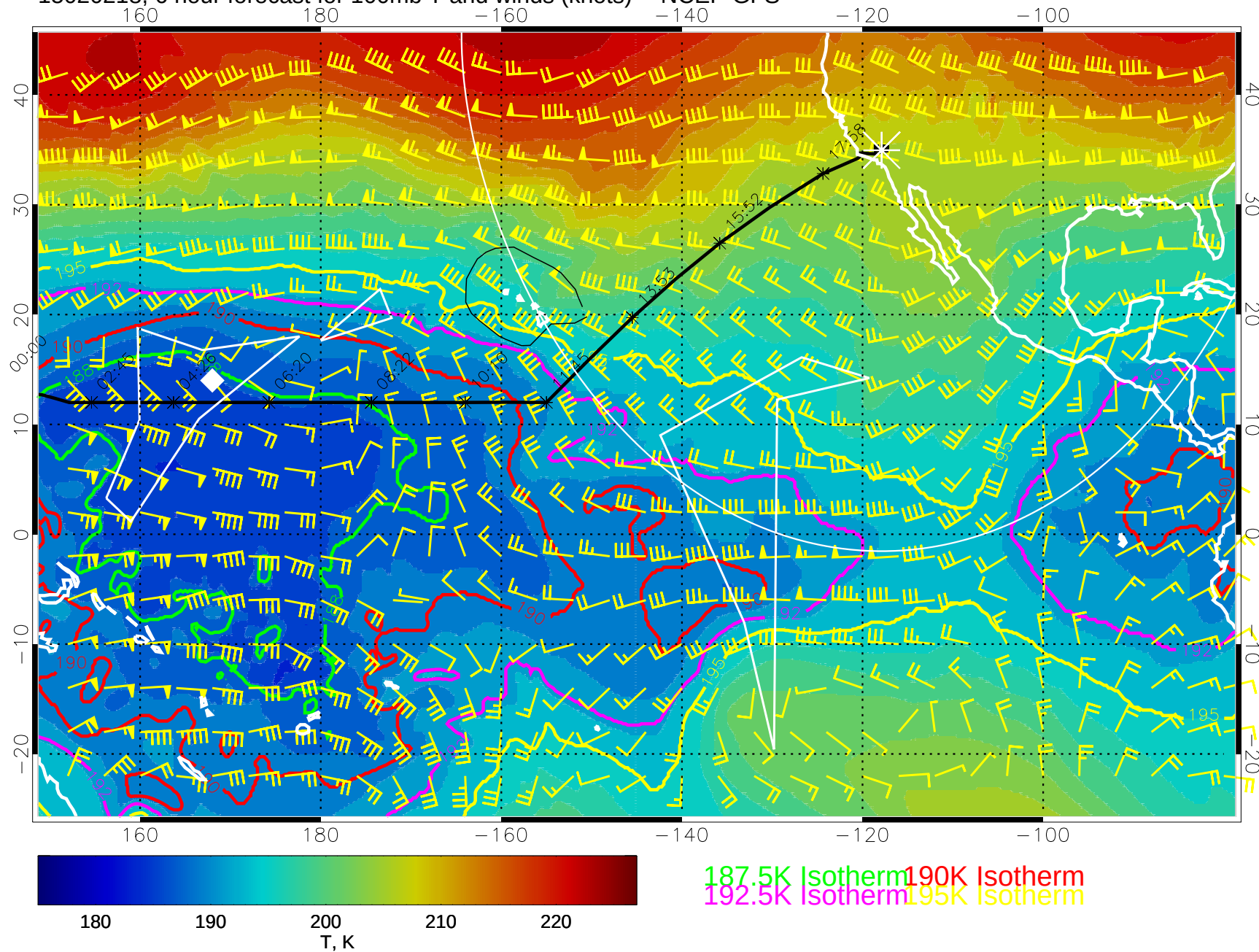
15020218, 6 hour forecast for 100mb T and winds (knots) -- NCEP GFS
