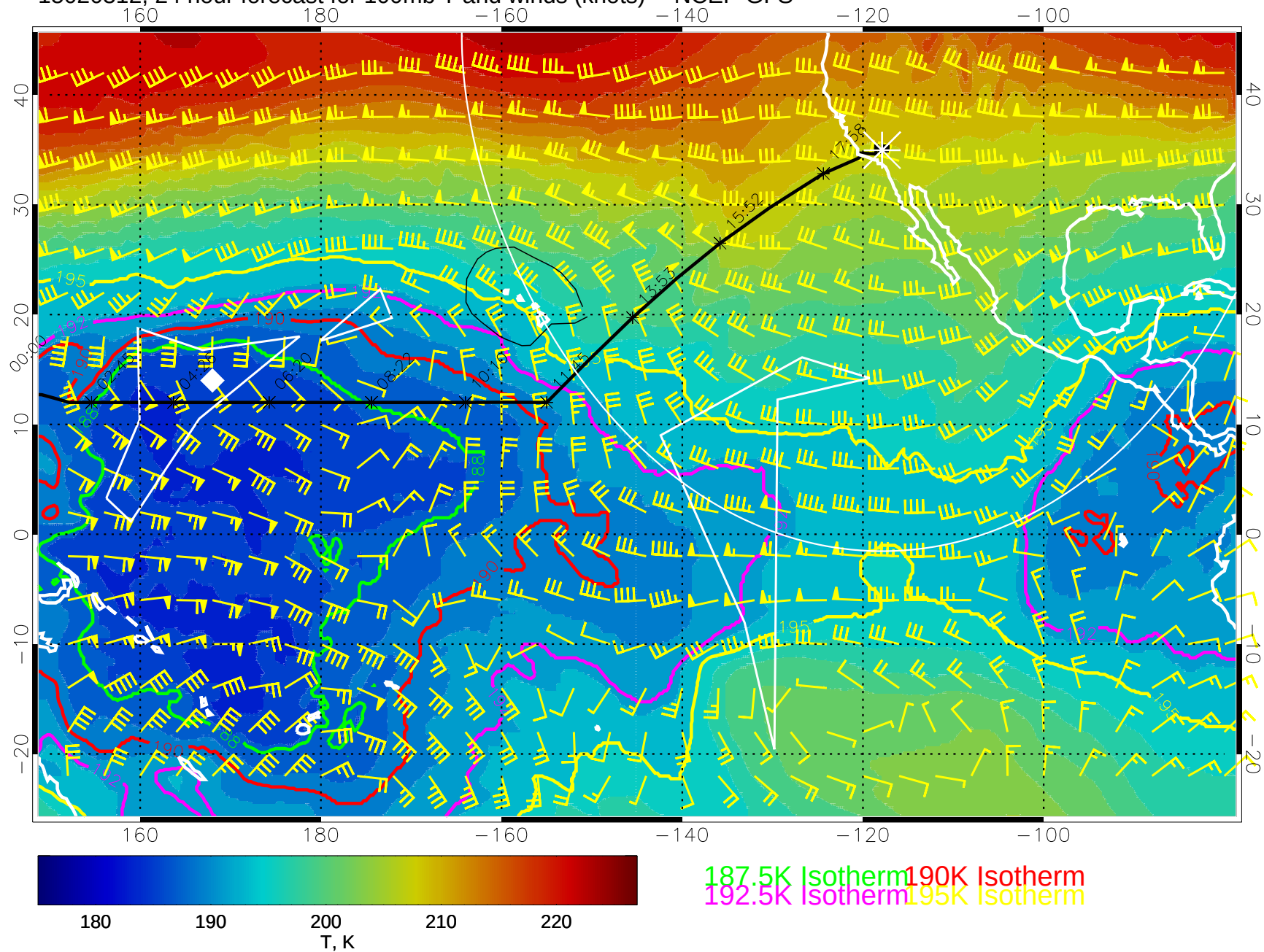
15020312, 24 hour forecast for 100mb T and winds (knots) -- NCEP GFS
