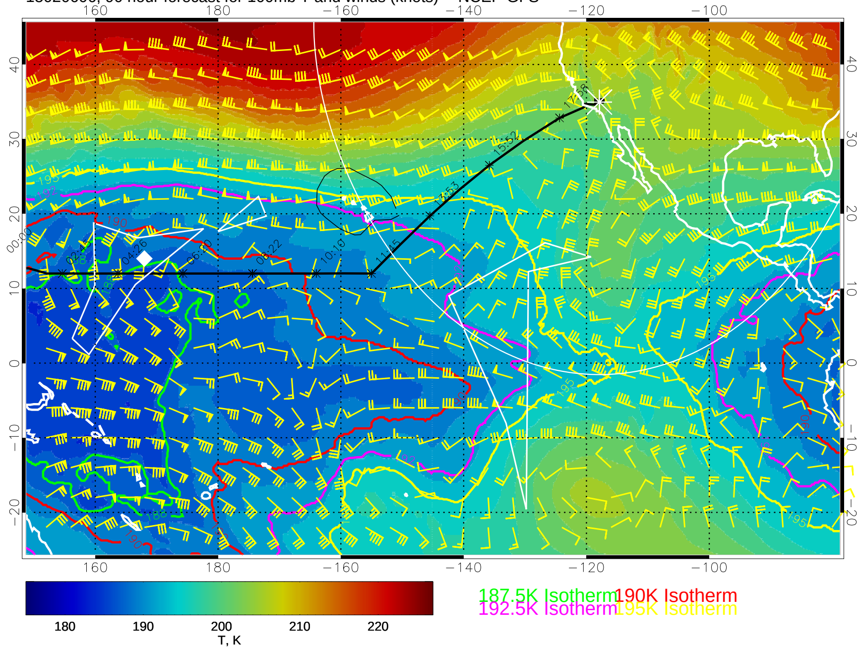
15020606, 90 hour forecast for 100mb T and winds (knots) -- NCEP GFS
