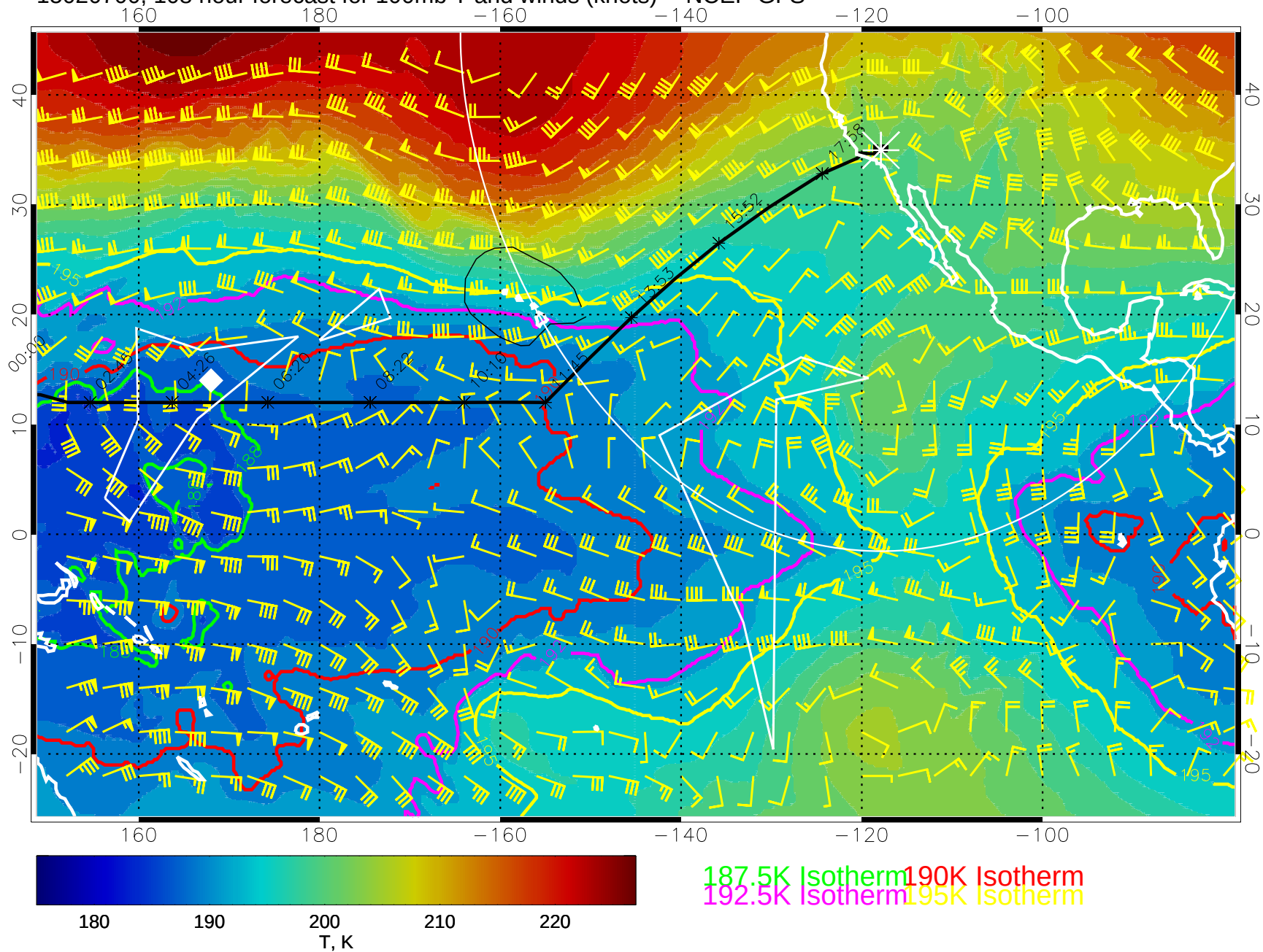
15020700, 108 hour forecast for 100mb T and winds (knots) -- NCEP GFS
