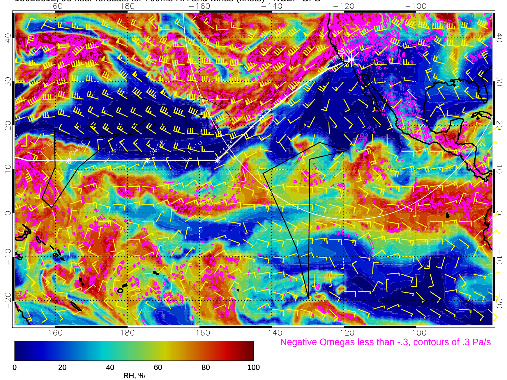
15020612, 96 hour forecast for 700mb RH and winds (knots) - NCEP GFS
