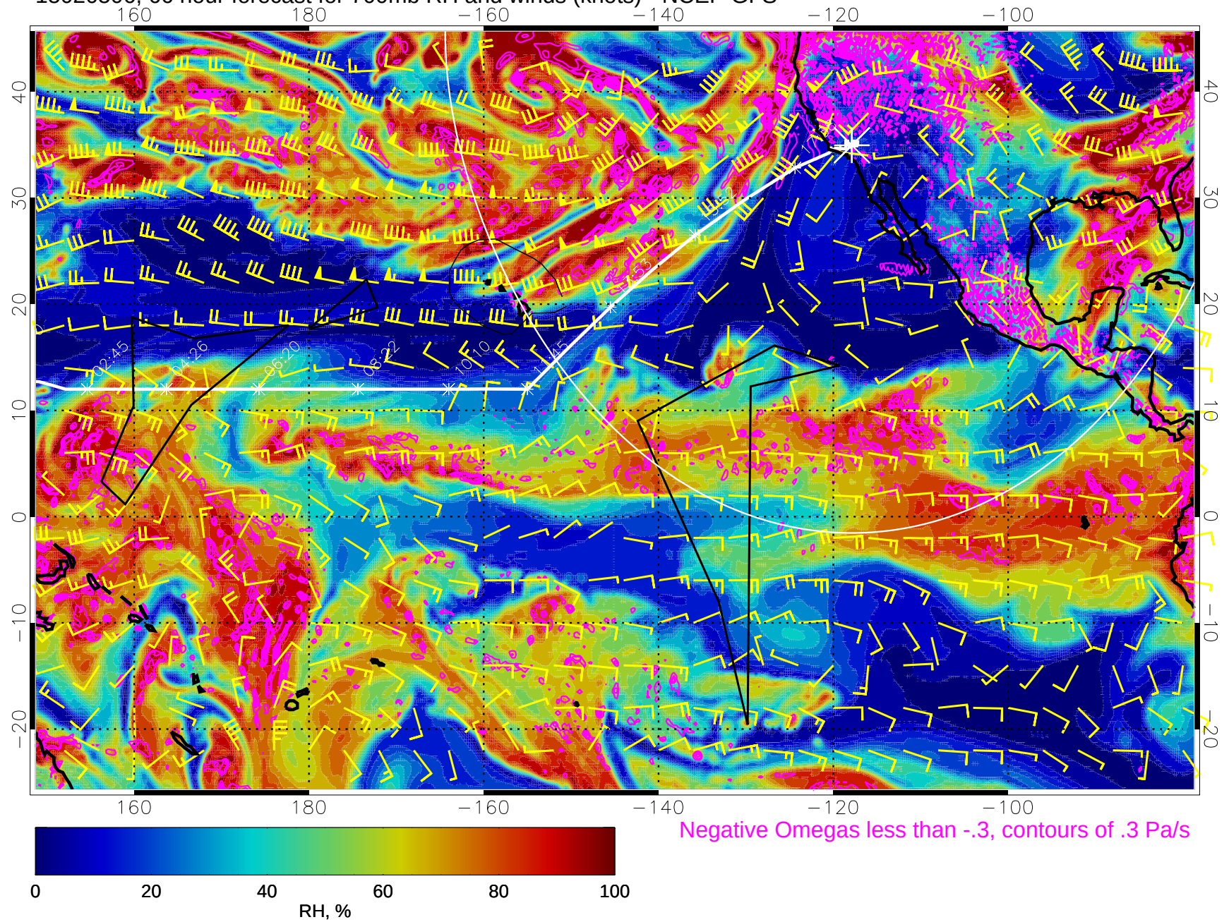
15020506, 66 hour forecast for 700mb RH and winds (knots) - NCEP GFS
