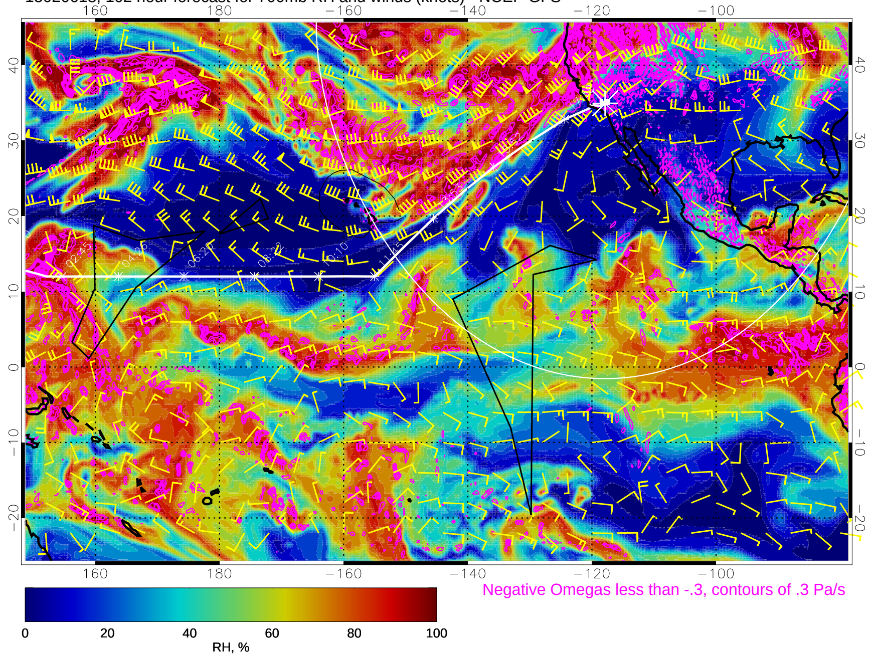
15020618, 102 hour forecast for 700mb RH and winds (knots) - NCEP GFS
