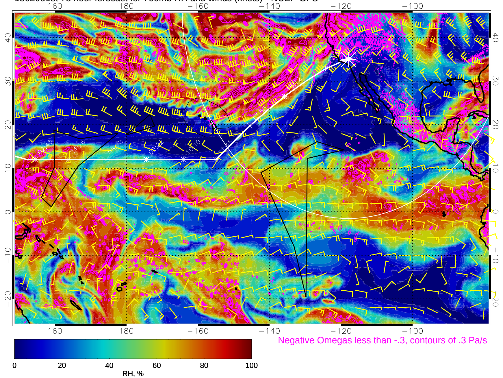
15020518, 78 hour forecast for 700mb RH and winds (knots) - NCEP GFS
