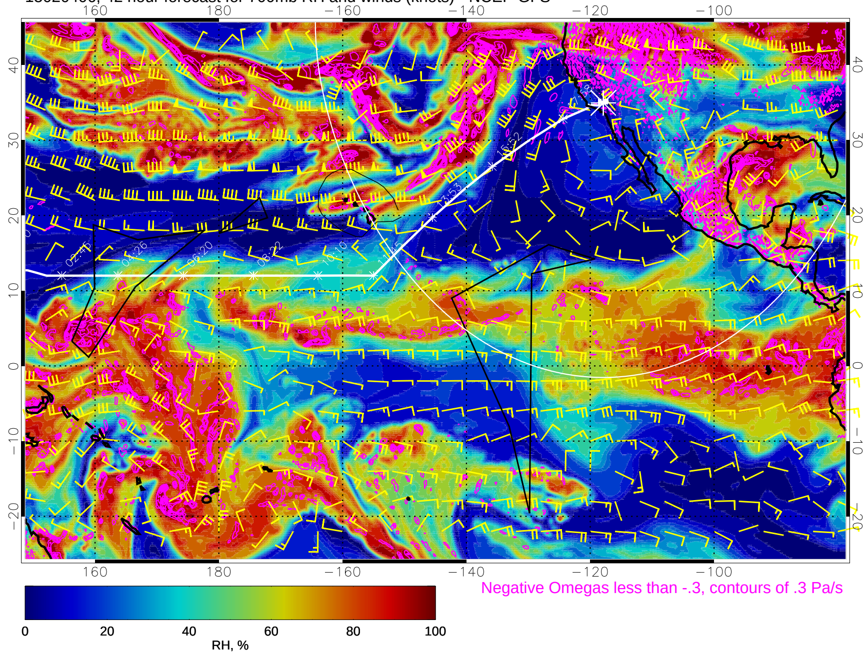
15020406, 42 hour forecast for 700mb RH and winds (knots) - NCEP GFS
