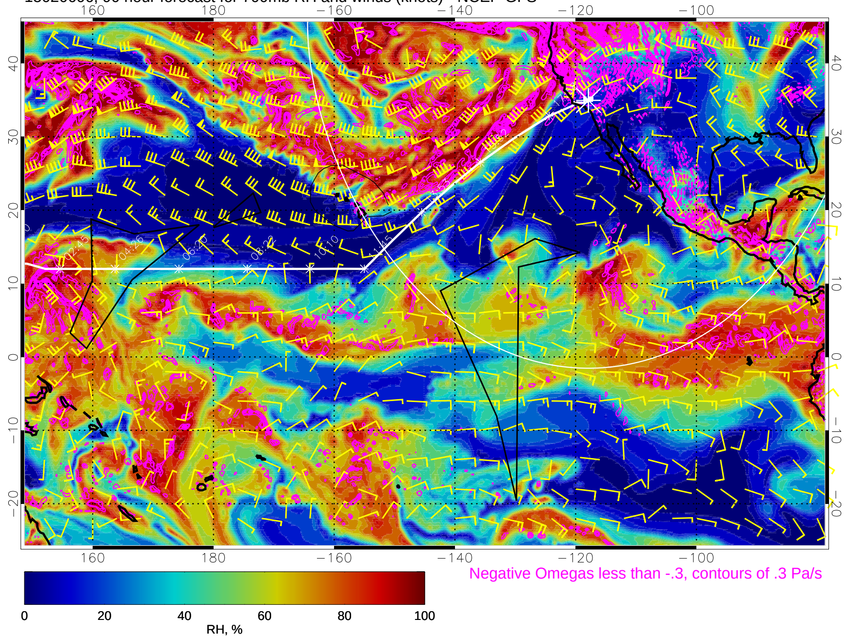
15020606, 90 hour forecast for 700mb RH and winds (knots) - NCEP GFS
