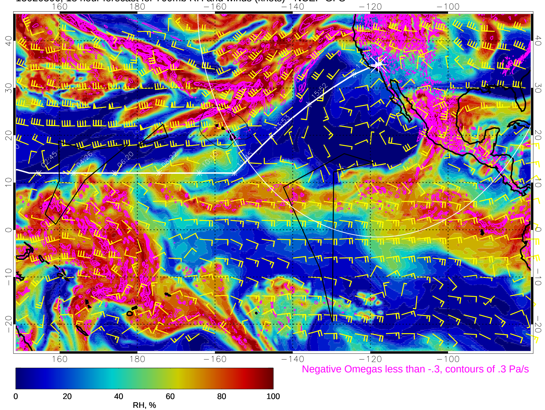
15020306, 18 hour forecast for 700mb RH and winds (knots) - NCEP GFS
