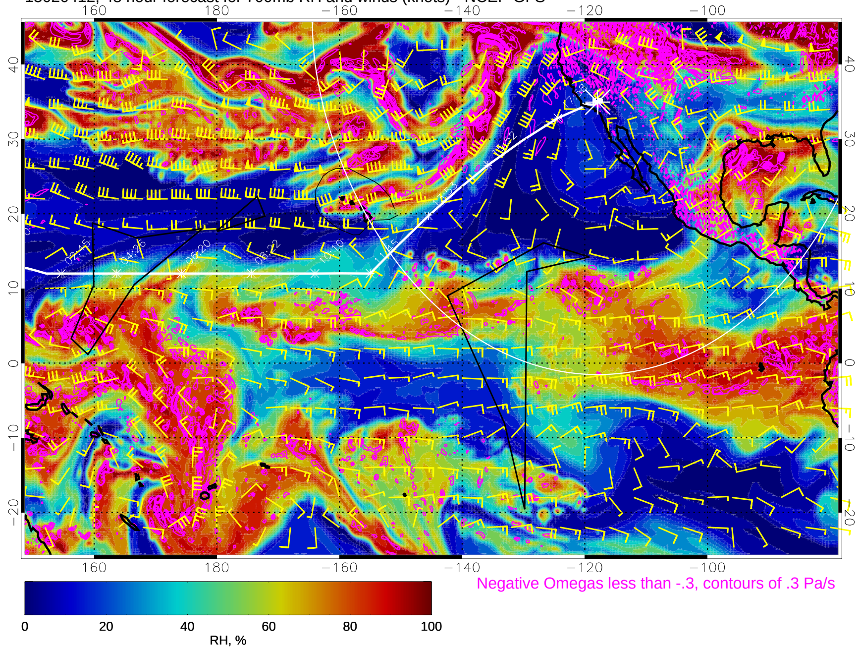
15020412, 48 hour forecast for 700mb RH and winds (knots) - NCEP GFS
