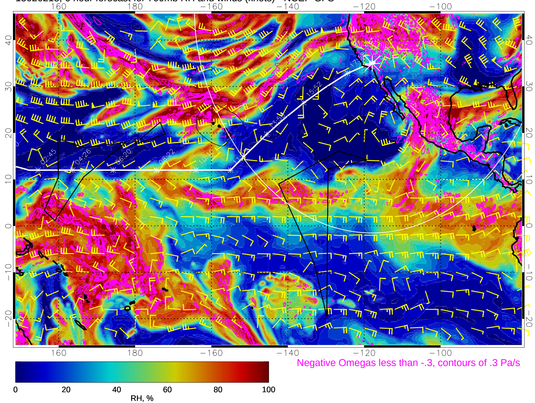
15020218, 6 hour forecast for 700mb RH and winds (knots) - NCEP GFS
