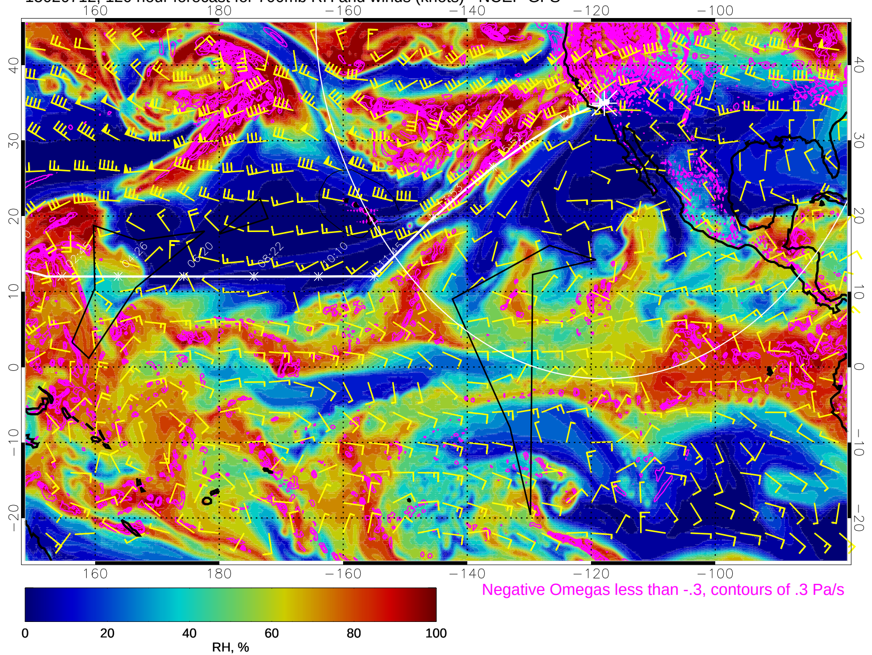
15020712, 120 hour forecast for 700mb RH and winds (knots) - NCEP GFS
