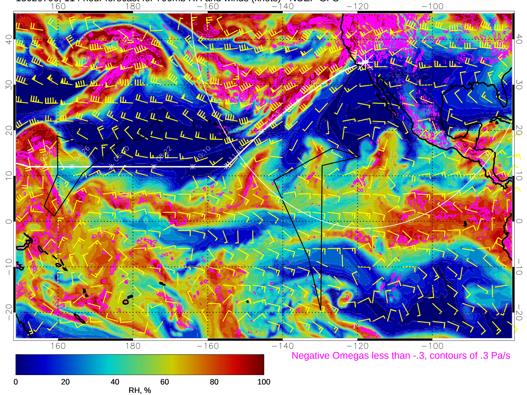
15020706, 114 hour forecast for 700mb RH and winds (knots) - NCEP GFS
