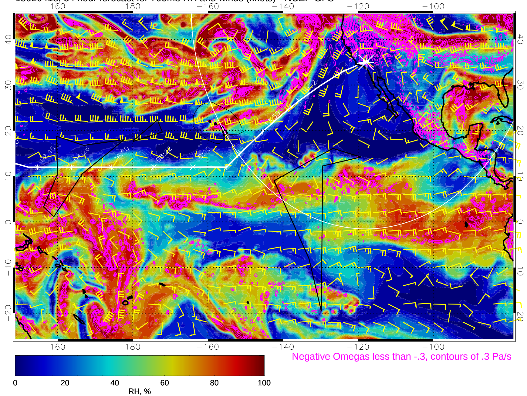
15020418, 54 hour forecast for 700mb RH and winds (knots) - NCEP GFS
