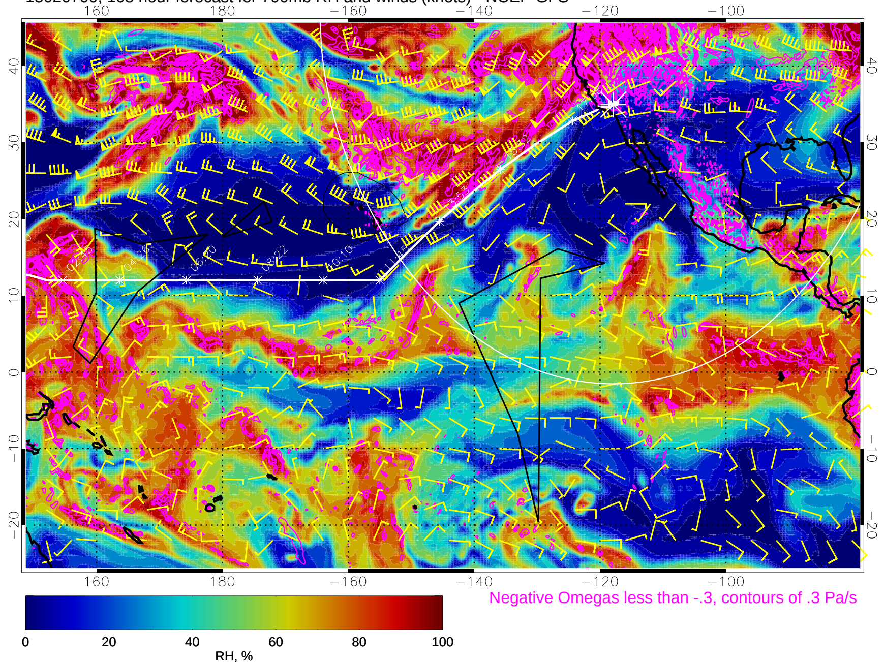
15020700, 108 hour forecast for 700mb RH and winds (knots) - NCEP GFS
