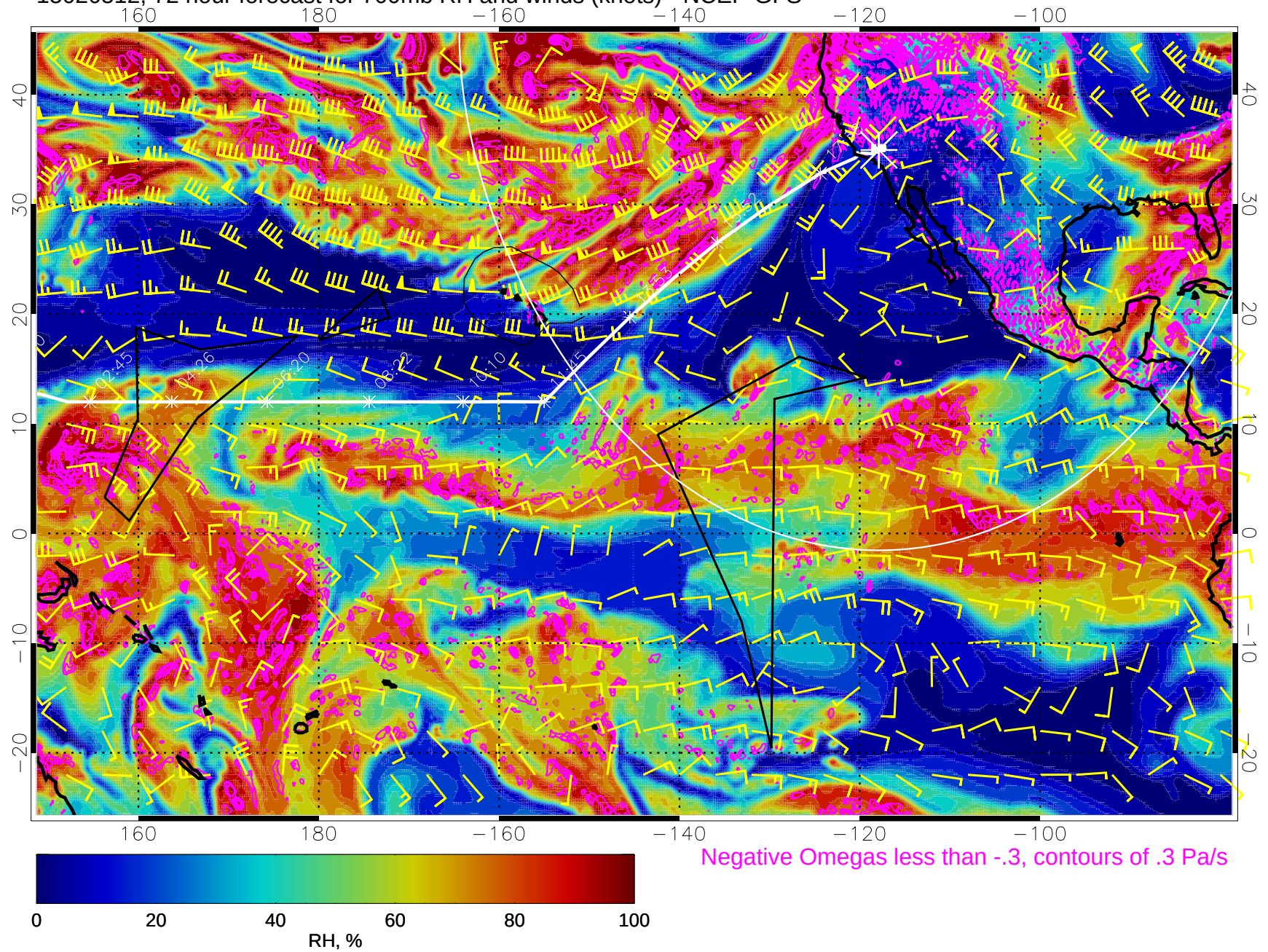
15020512, 72 hour forecast for 700mb RH and winds (knots) - NCEP GFS
