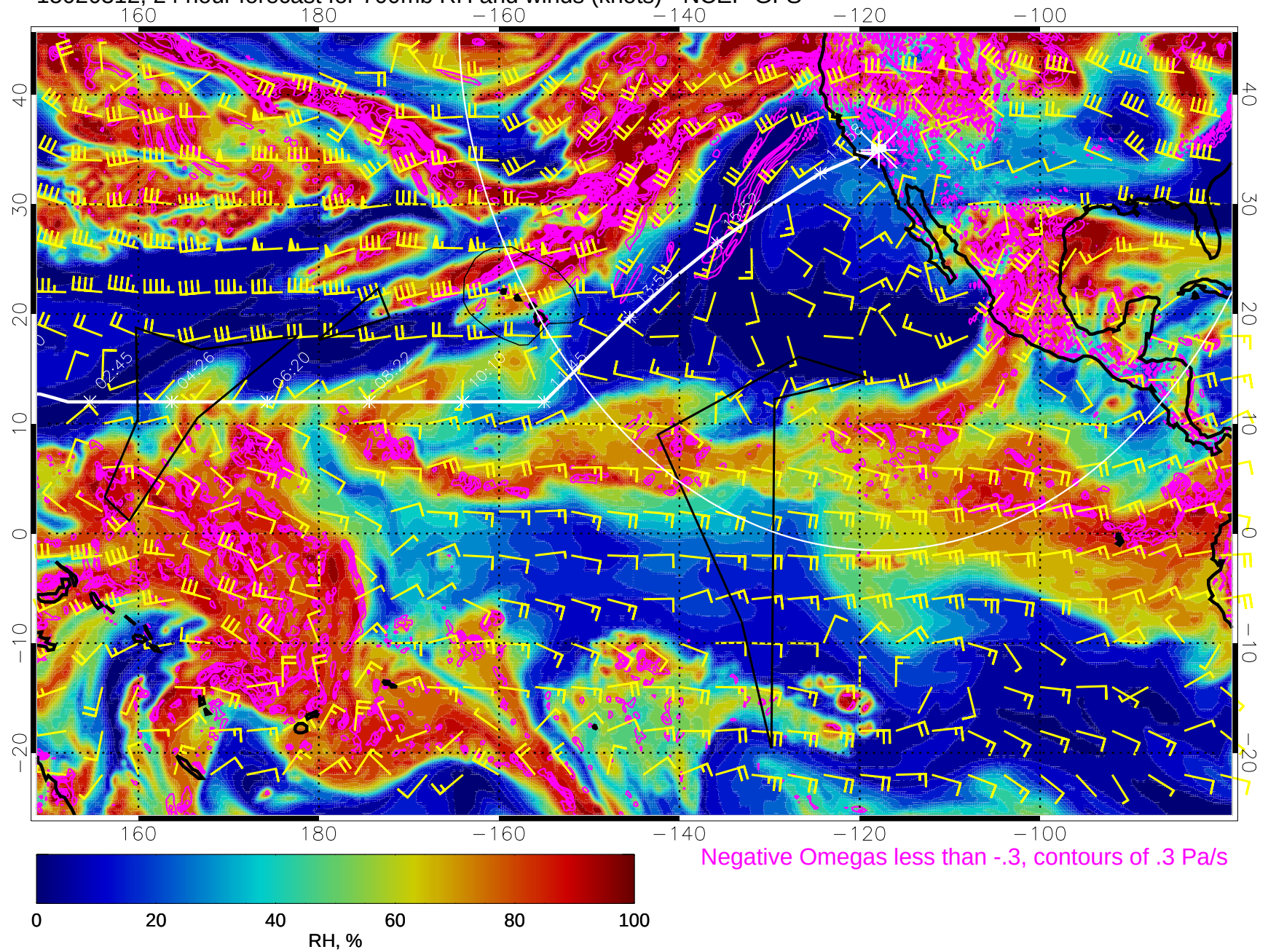
15020312, 24 hour forecast for 700mb RH and winds (knots) - NCEP GFS
