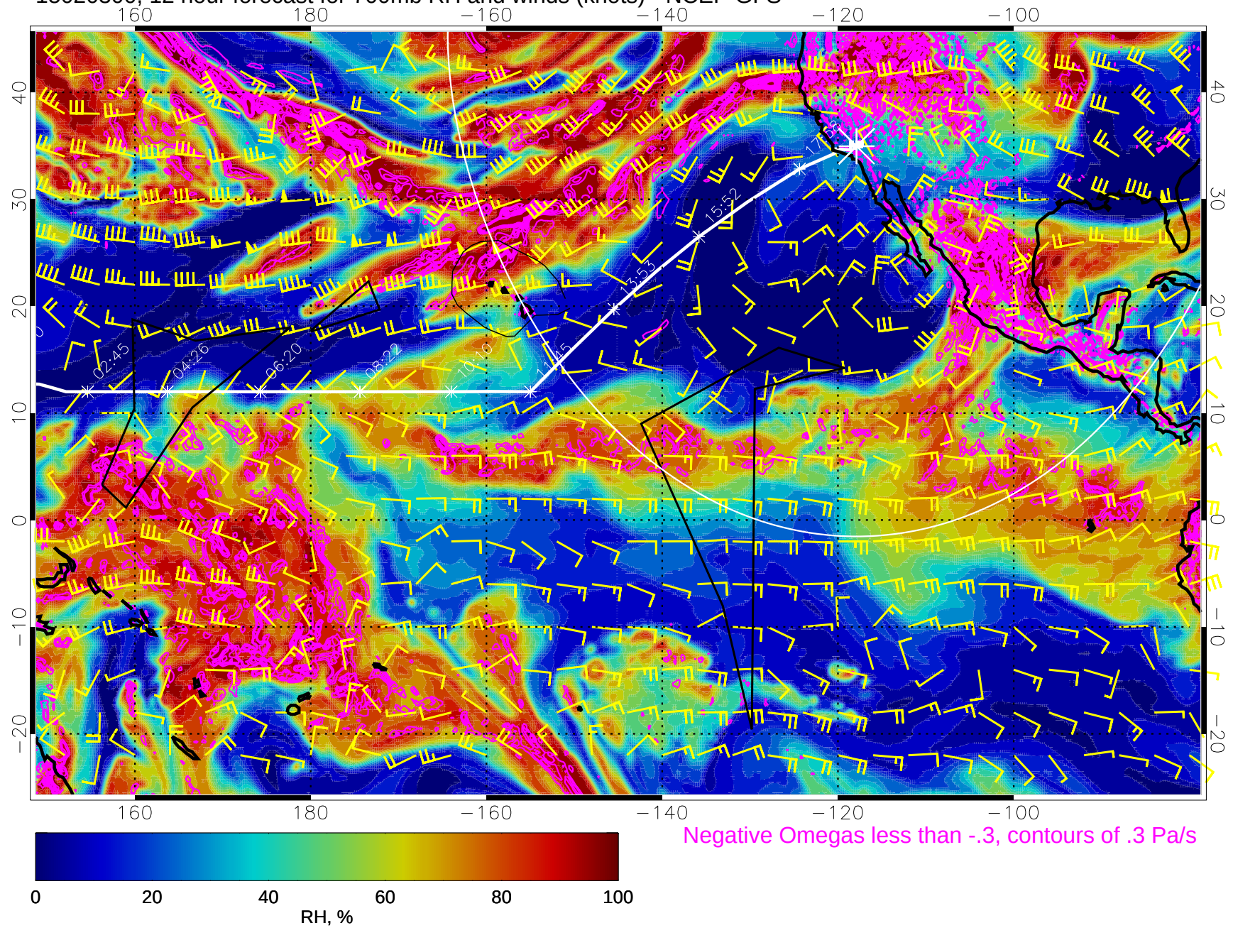
15020300, 12 hour forecast for 700mb RH and winds (knots) - NCEP GFS
