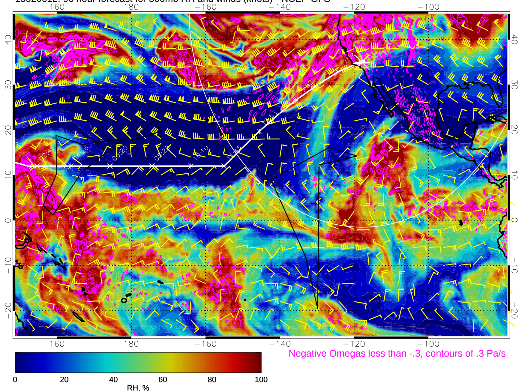
15020612, 96 hour forecast for 500mb RH and winds (knots) - NCEP GFS
