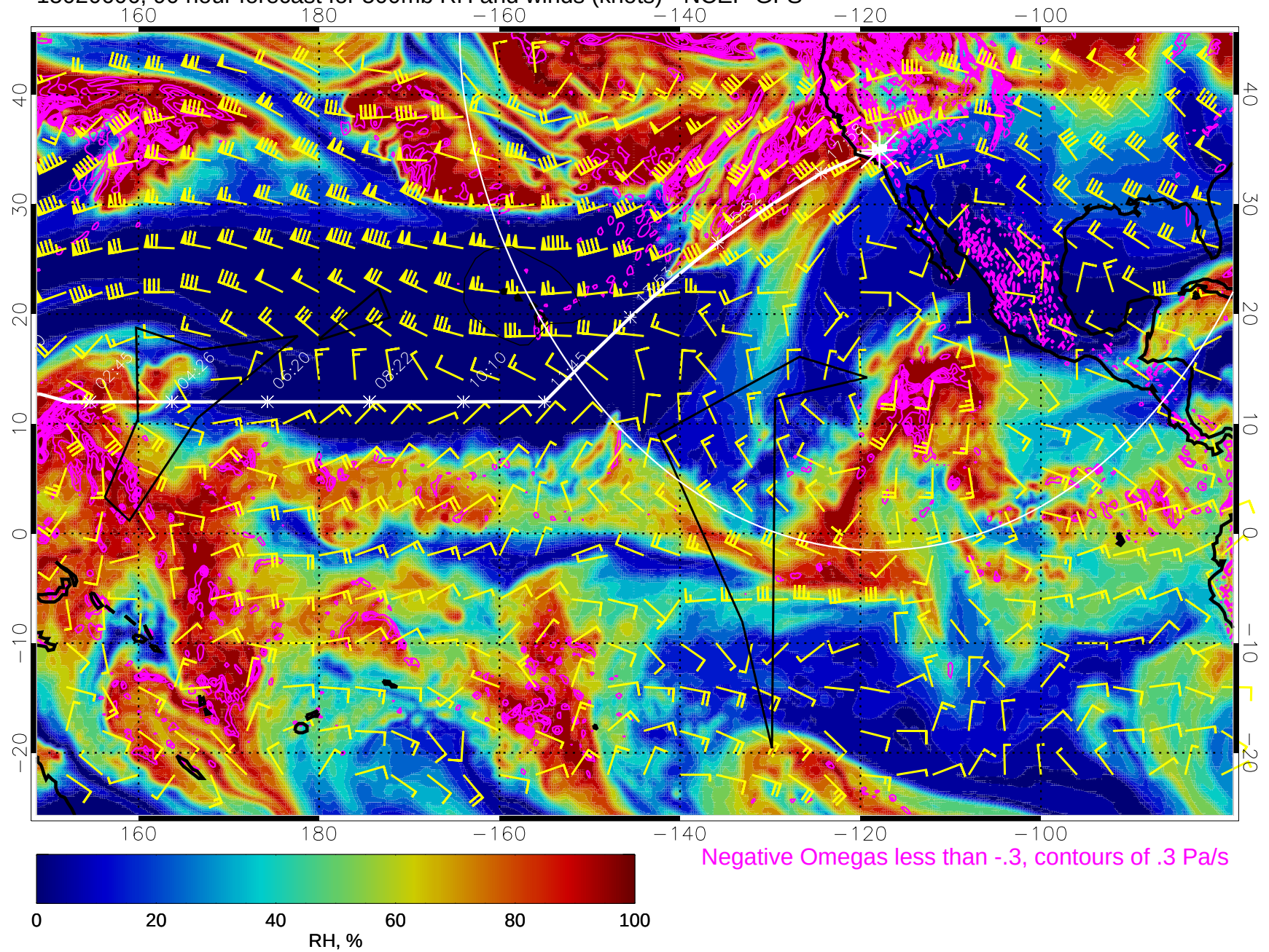
15020606, 90 hour forecast for 500mb RH and winds (knots) - NCEP GFS
