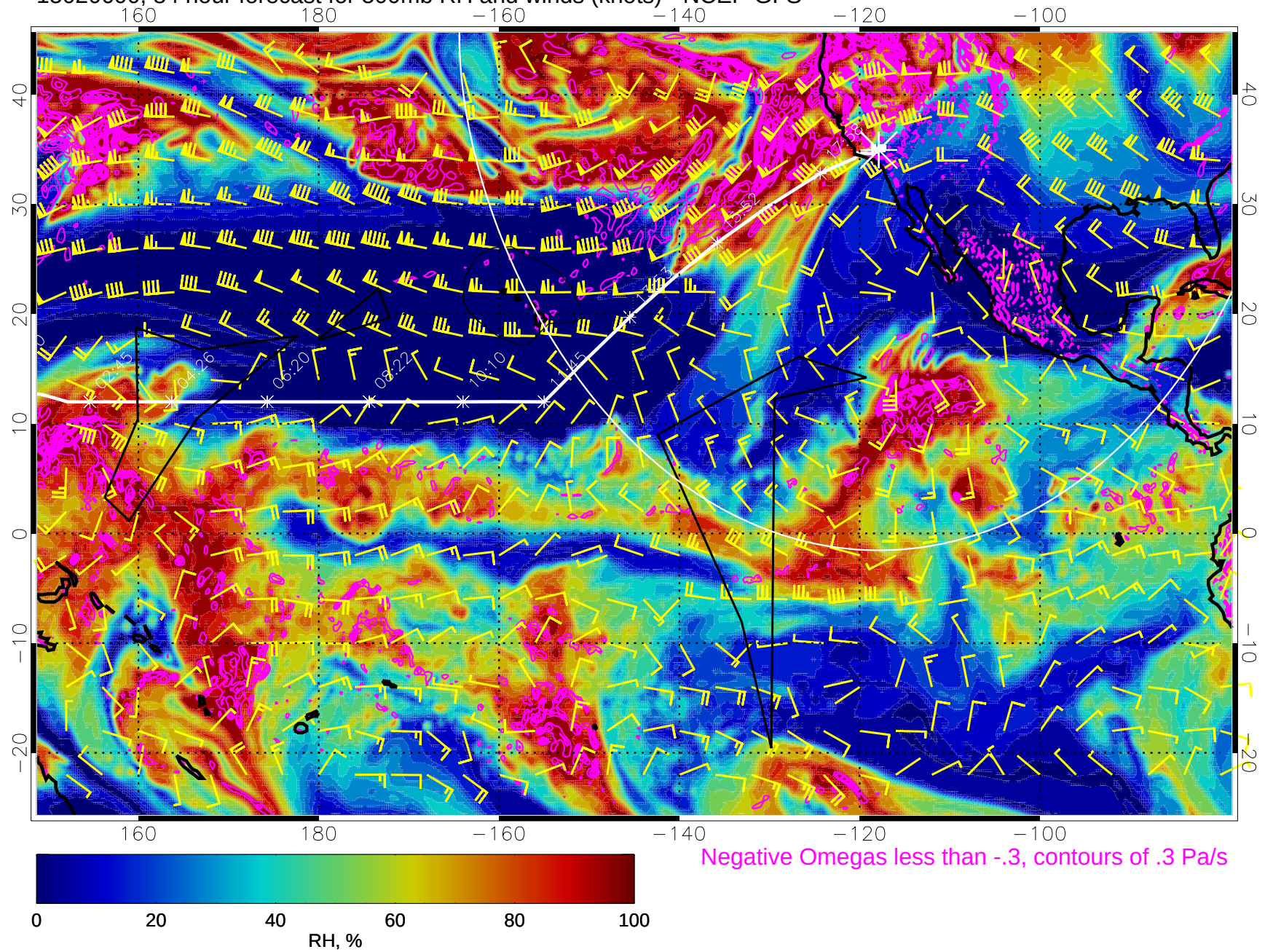
15020600, 84 hour forecast for 500mb RH and winds (knots) - NCEP GFS
