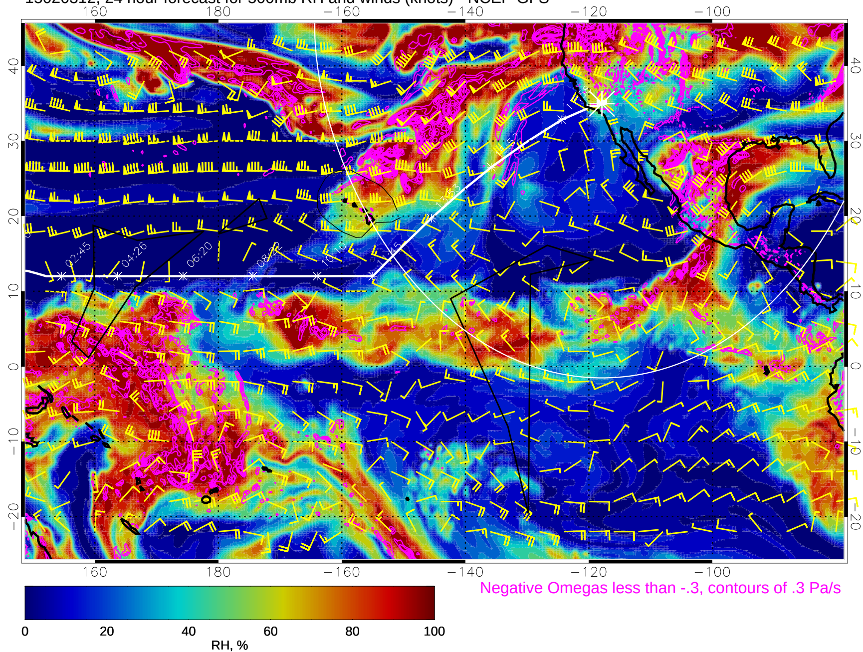
15020312, 24 hour forecast for 500mb RH and winds (knots) - NCEP GFS
