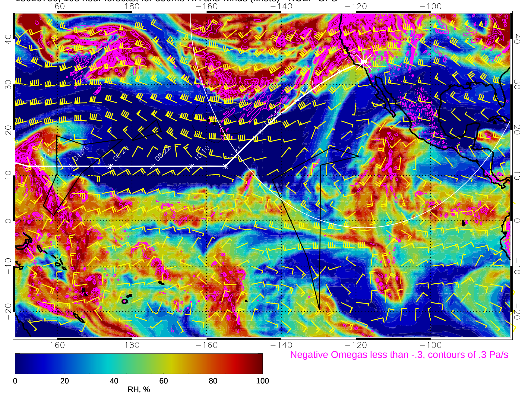
15020700, 108 hour forecast for 500mb RH and winds (knots) - NCEP GFS
