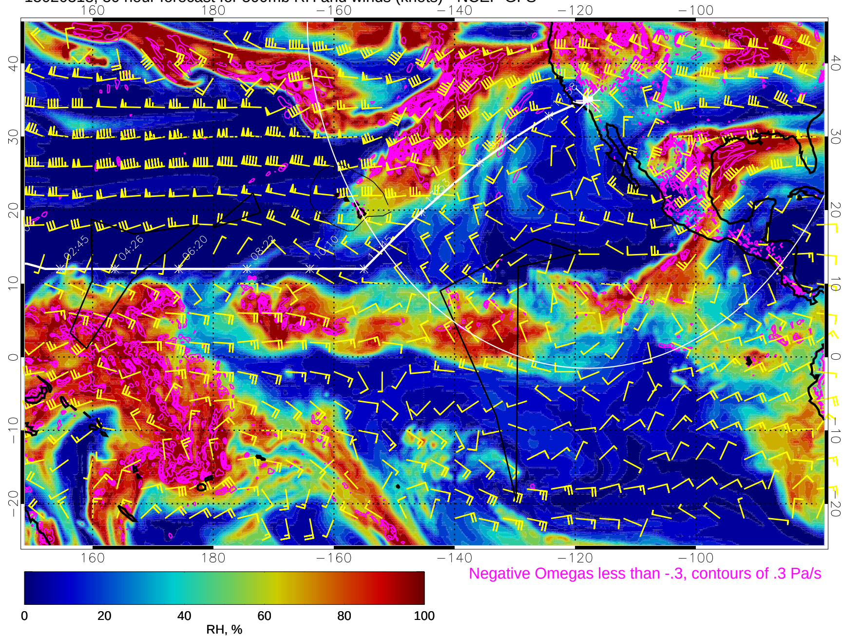
15020318, 30 hour forecast for 500mb RH and winds (knots) - NCEP GFS
