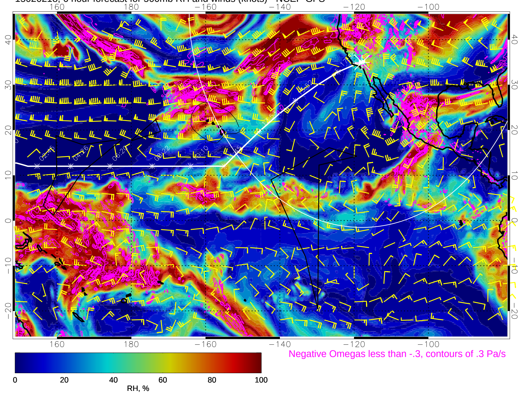
15020218, 6 hour forecast for 500mb RH and winds (knots) - NCEP GFS
