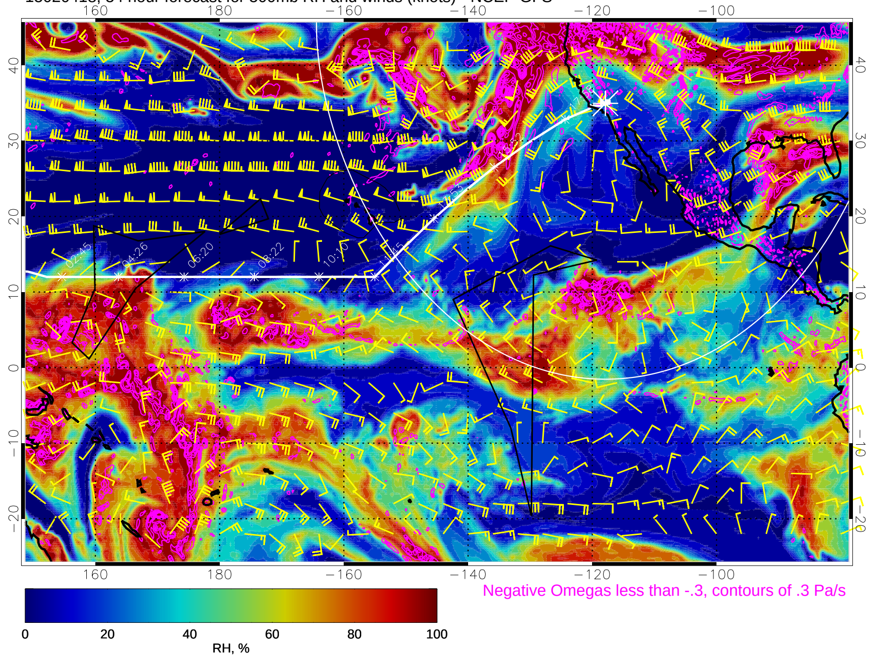
15020418, 54 hour forecast for 500mb RH and winds (knots) - NCEP GFS
