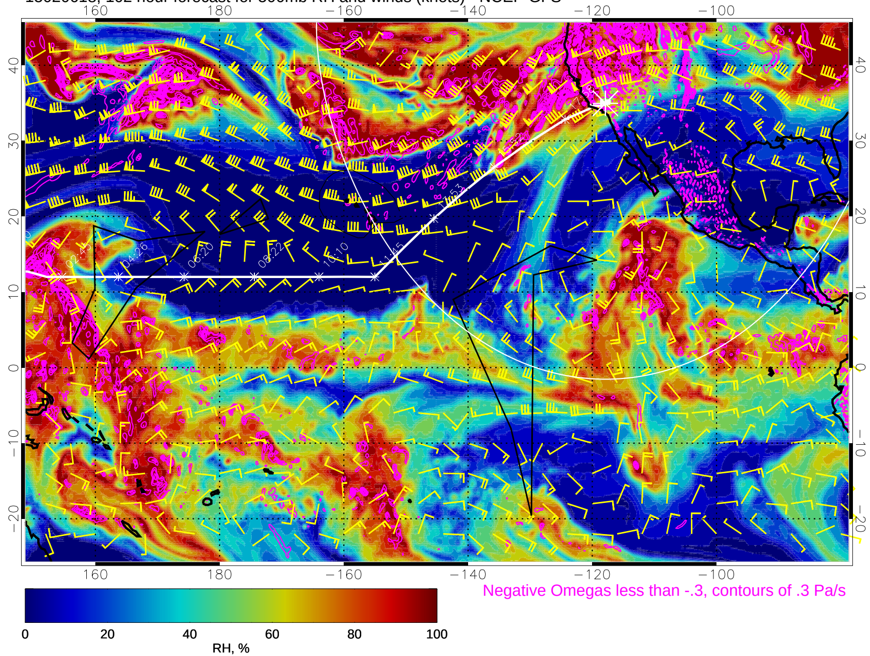
15020618, 102 hour forecast for 500mb RH and winds (knots) - NCEP GFS
