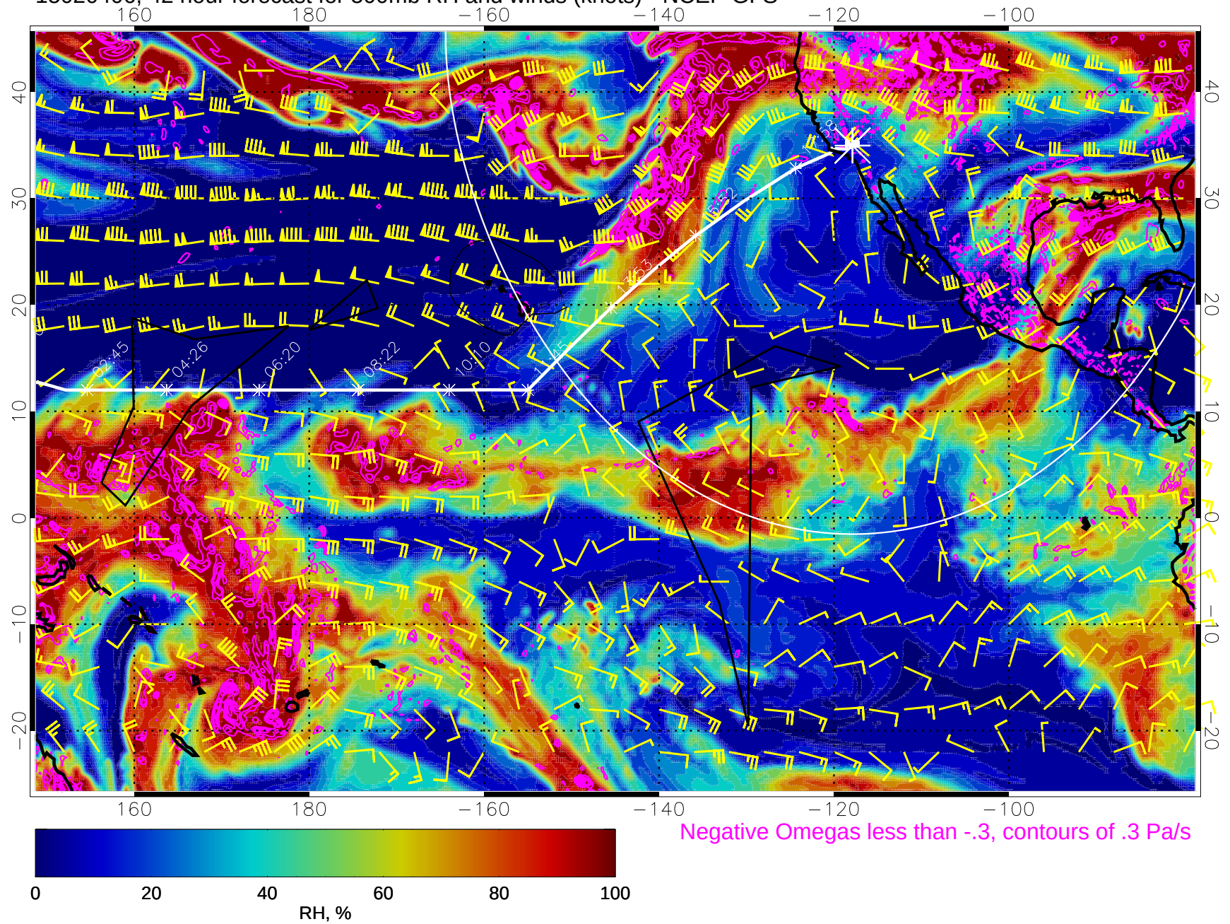
15020406, 42 hour forecast for 500mb RH and winds (knots) - NCEP GFS
