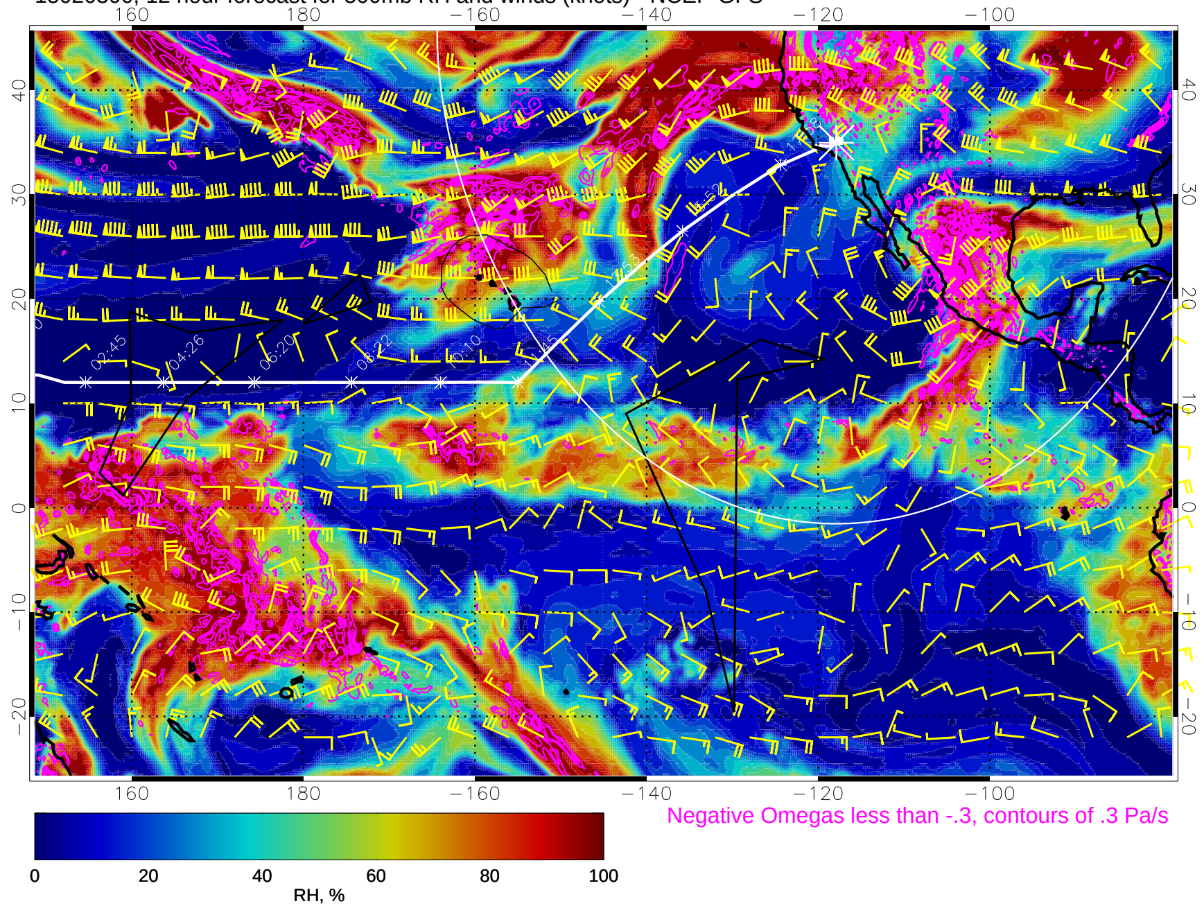
15020300, 12 hour forecast for 500mb RH and winds (knots) - NCEP GFS
