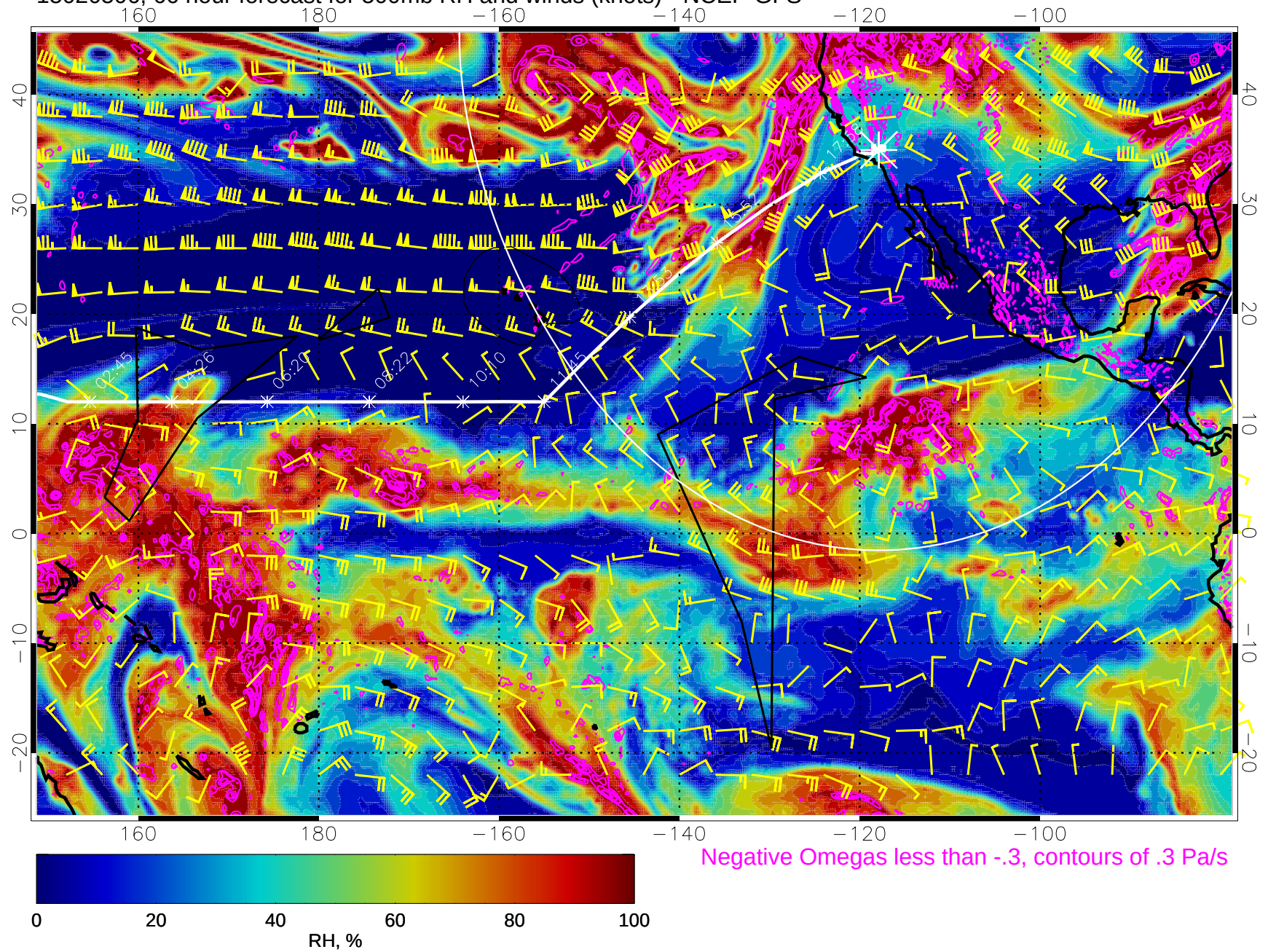
15020506, 66 hour forecast for 500mb RH and winds (knots) - NCEP GFS
