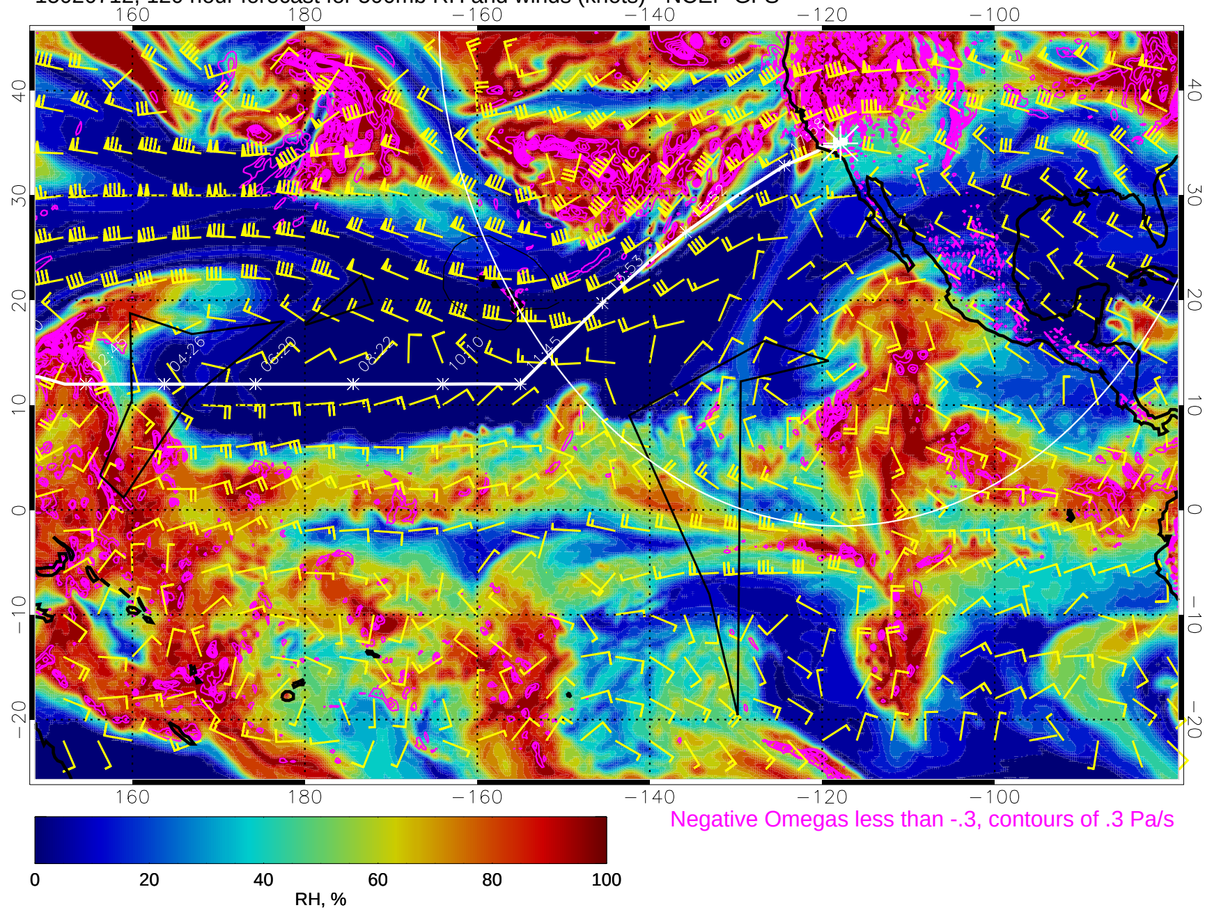
15020712, 120 hour forecast for 500mb RH and winds (knots) - NCEP GFS
