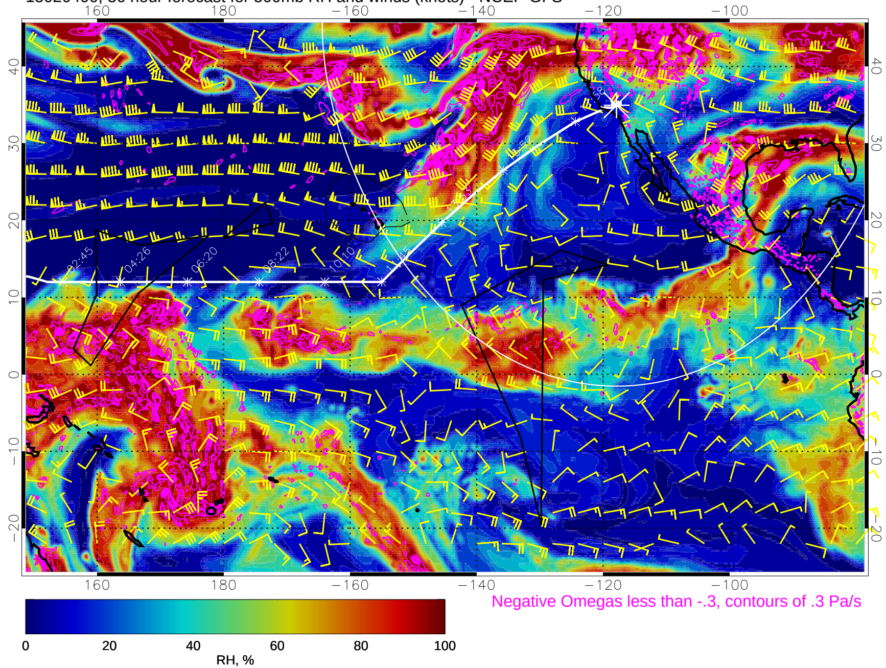
15020400, 36 hour forecast for 500mb RH and winds (knots) - NCEP GFS
