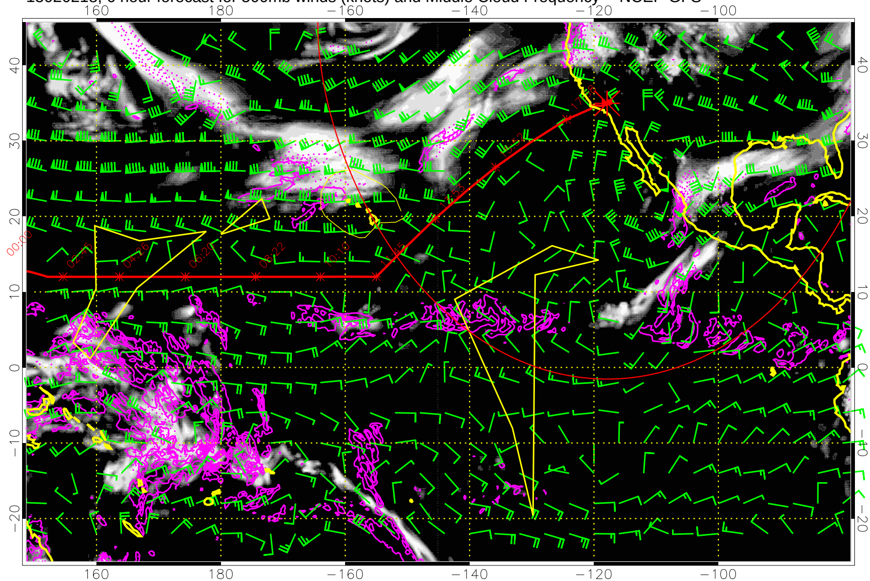
15020218, 6 hour forecast for 500mb winds (knots) and Middle Cloud Frequency -- NCEP GFS
