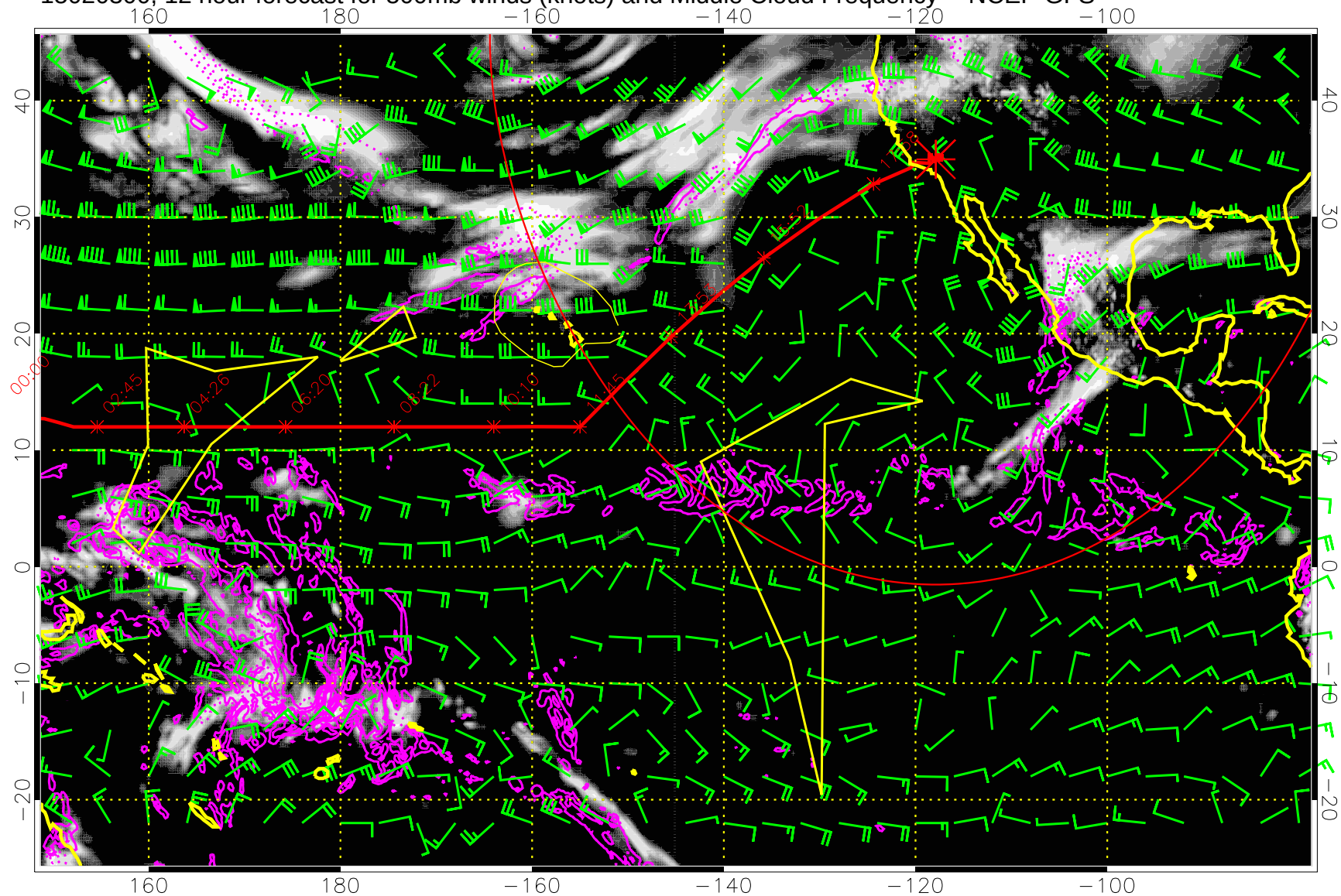
15020300, 12 hour forecast for 500mb winds (knots) and Middle Cloud Frequency -- NCEP GFS
