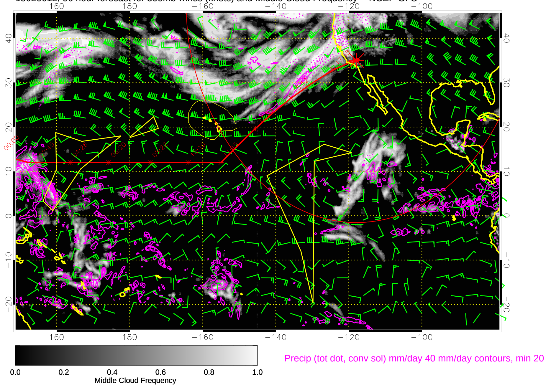
15020612, 96 hour forecast for 500mb winds (knots) and Middle Cloud Frequency -- NCEP GFS
