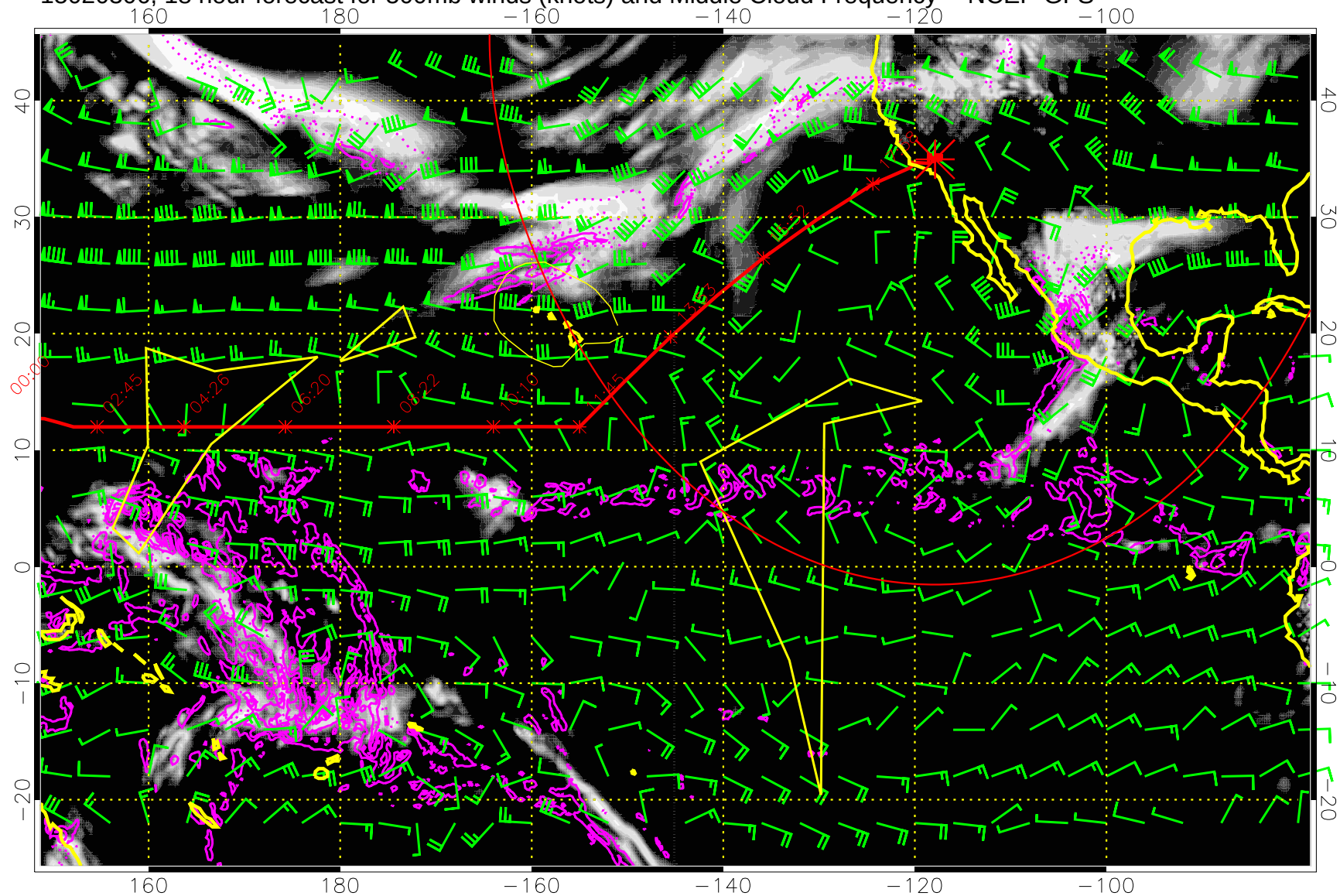
15020306, 18 hour forecast for 500mb winds (knots) and Middle Cloud Frequency -- NCEP GFS
