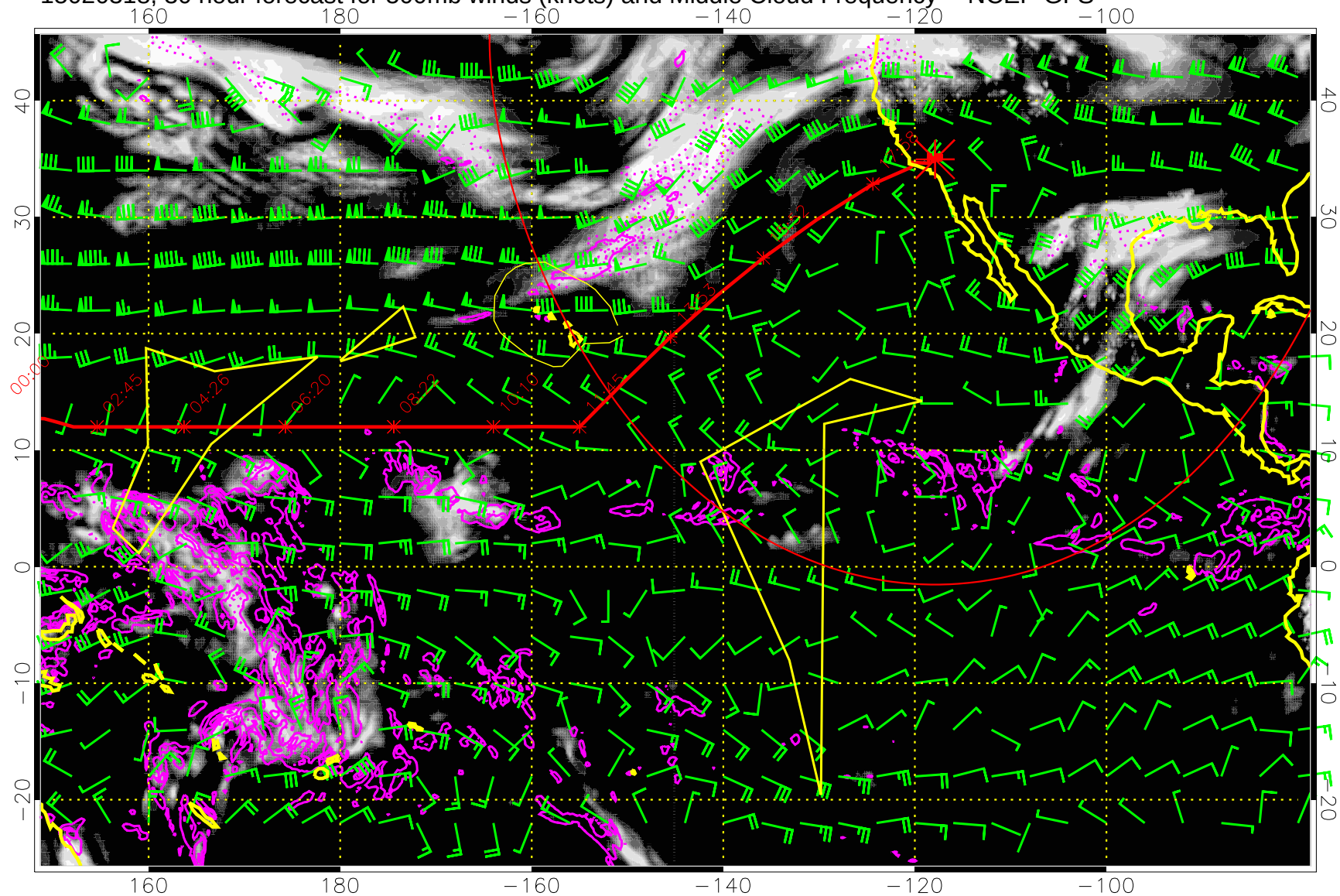
15020318, 30 hour forecast for 500mb winds (knots) and Middle Cloud Frequency -- NCEP GFS
