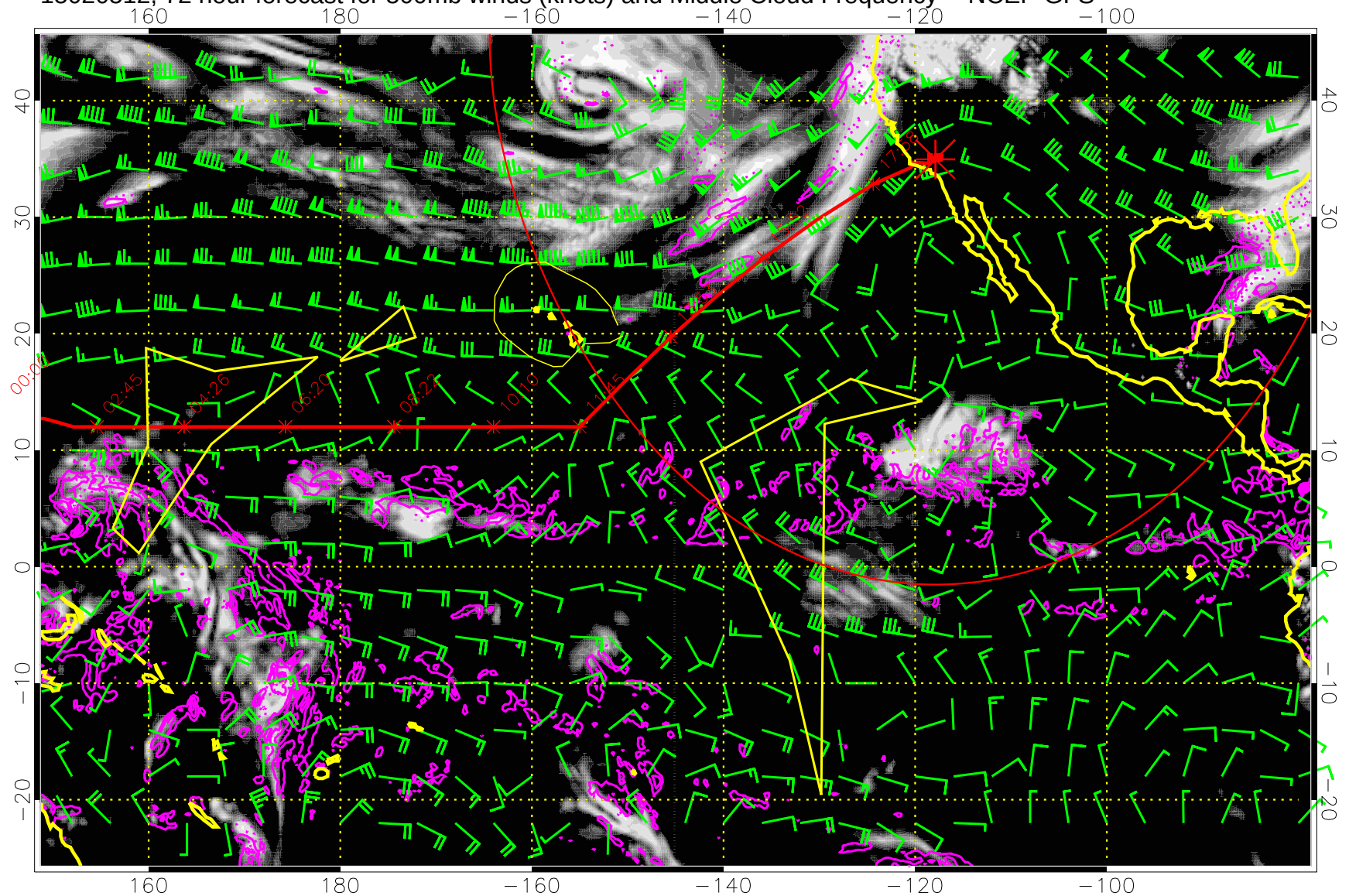
15020512, 72 hour forecast for 500mb winds (knots) and Middle Cloud Frequency -- NCEP GFS
