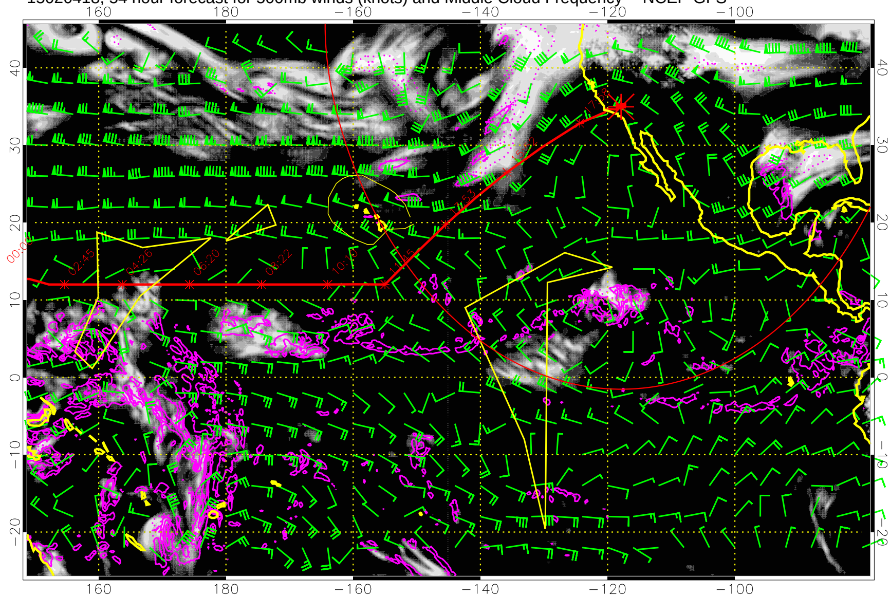
15020418, 54 hour forecast for 500mb winds (knots) and Middle Cloud Frequency -- NCEP GFS
