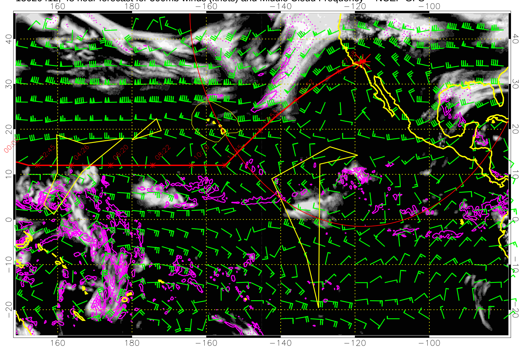
15020412, 48 hour forecast for 500mb winds (knots) and Middle Cloud Frequency -- NCEP GFS
