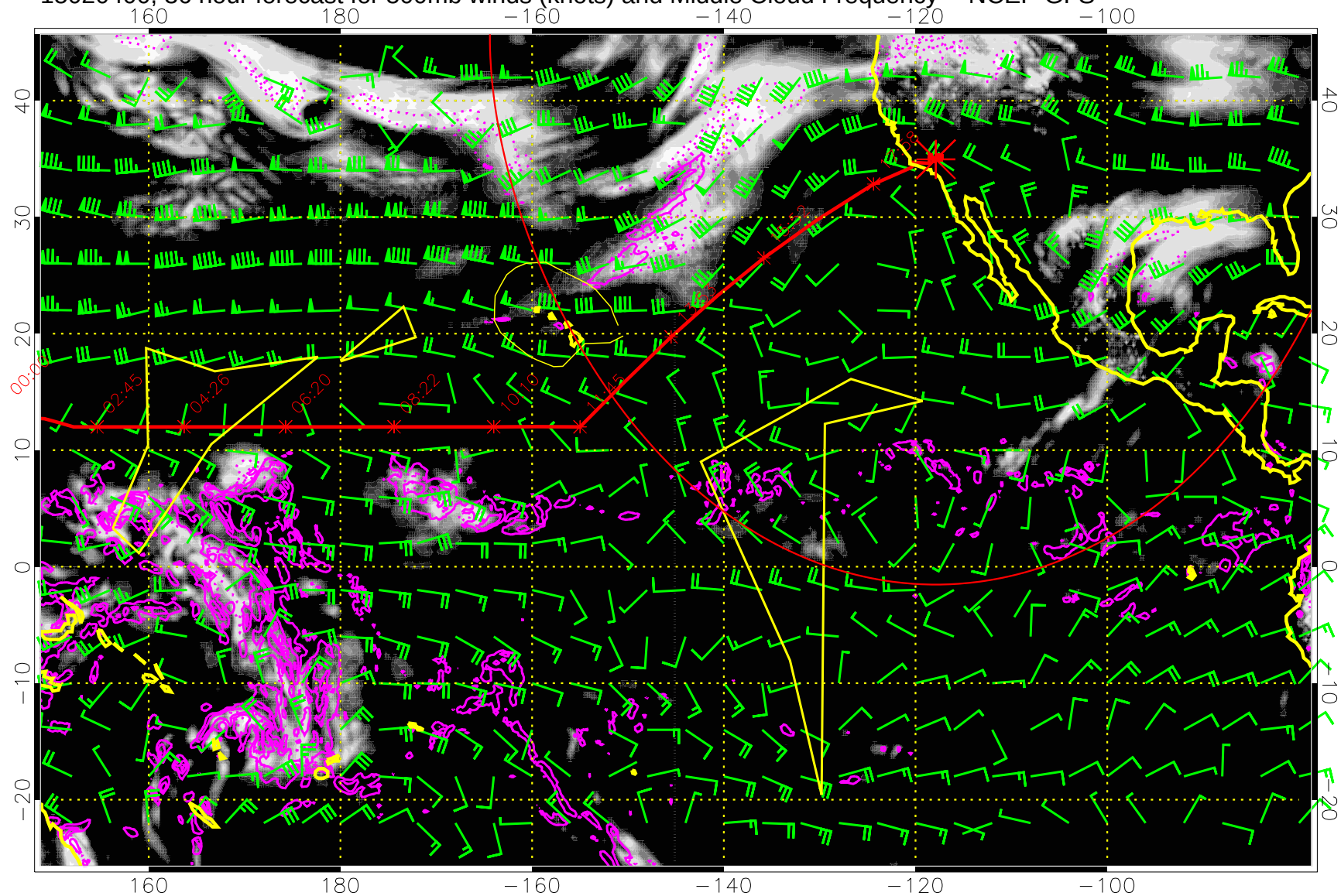
15020400, 36 hour forecast for 500mb winds (knots) and Middle Cloud Frequency -- NCEP GFS
