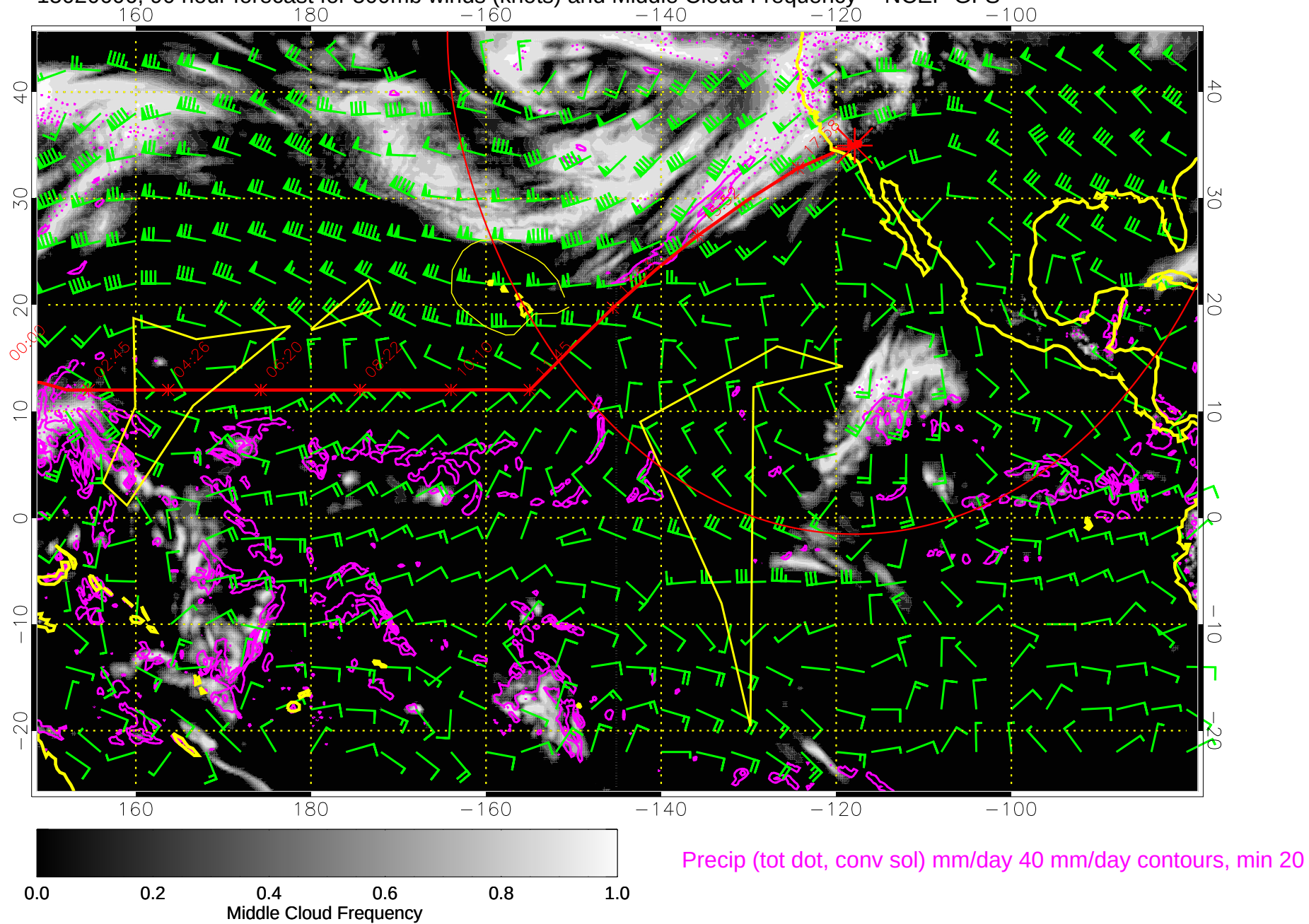
15020606, 90 hour forecast for 500mb winds (knots) and Middle Cloud Frequency -- NCEP GFS
