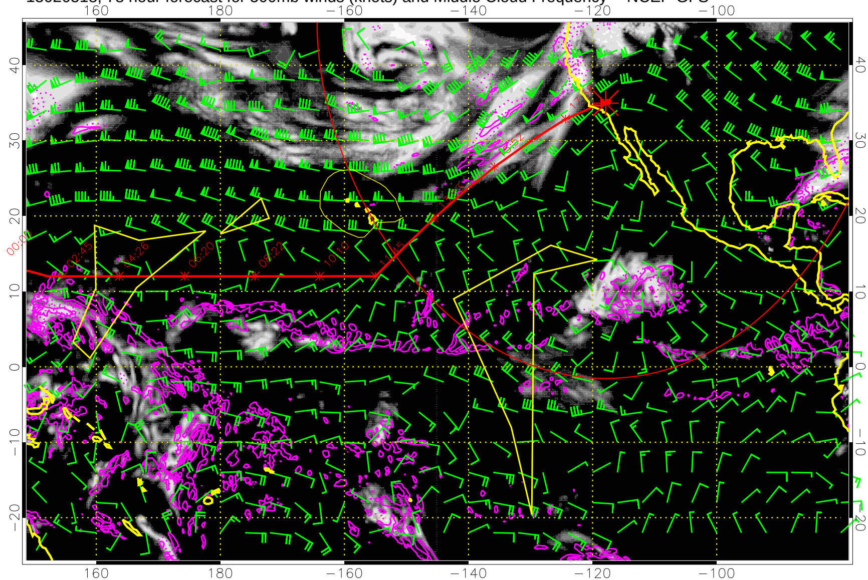
15020518, 78 hour forecast for 500mb winds (knots) and Middle Cloud Frequency -- NCEP GFS
