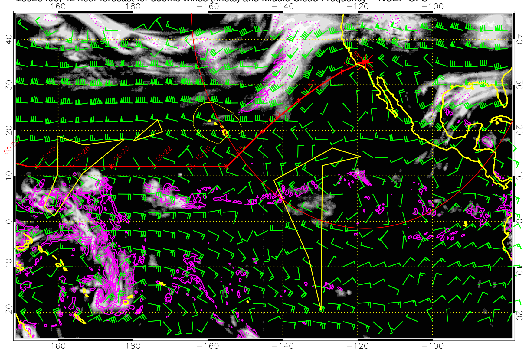
15020406, 42 hour forecast for 500mb winds (knots) and Middle Cloud Frequency -- NCEP GFS
