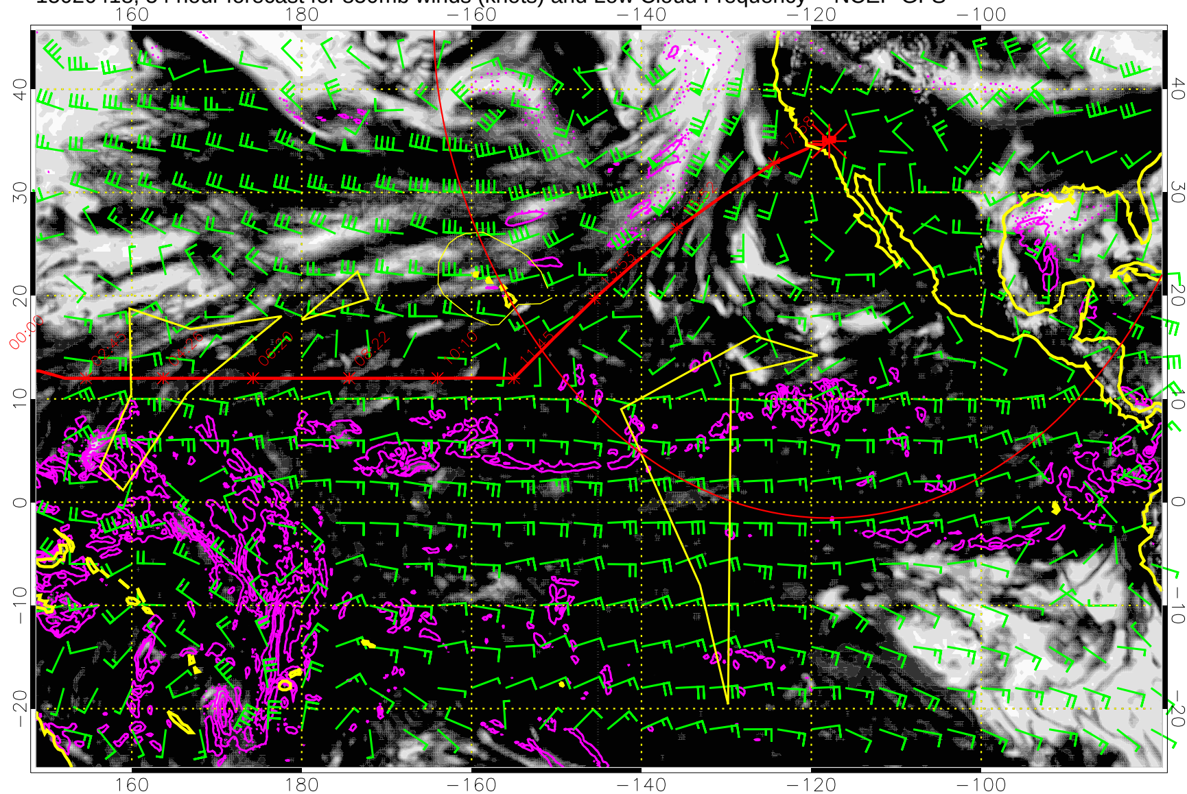
15020418, 54 hour forecast for 850mb winds (knots) and Low Cloud Frequency -- NCEP GFS
