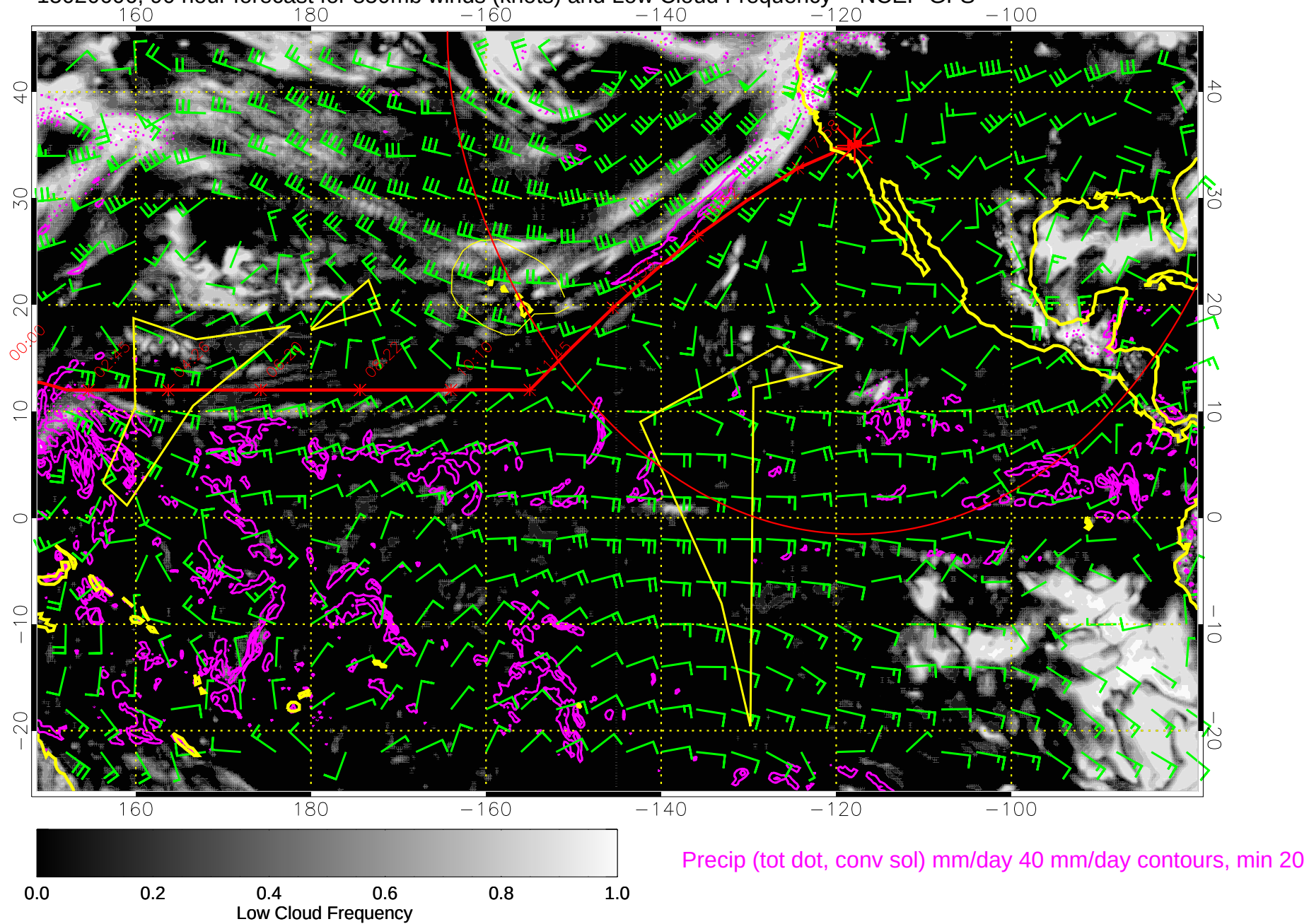
15020606, 90 hour forecast for 850mb winds (knots) and Low Cloud Frequency -- NCEP GFS
