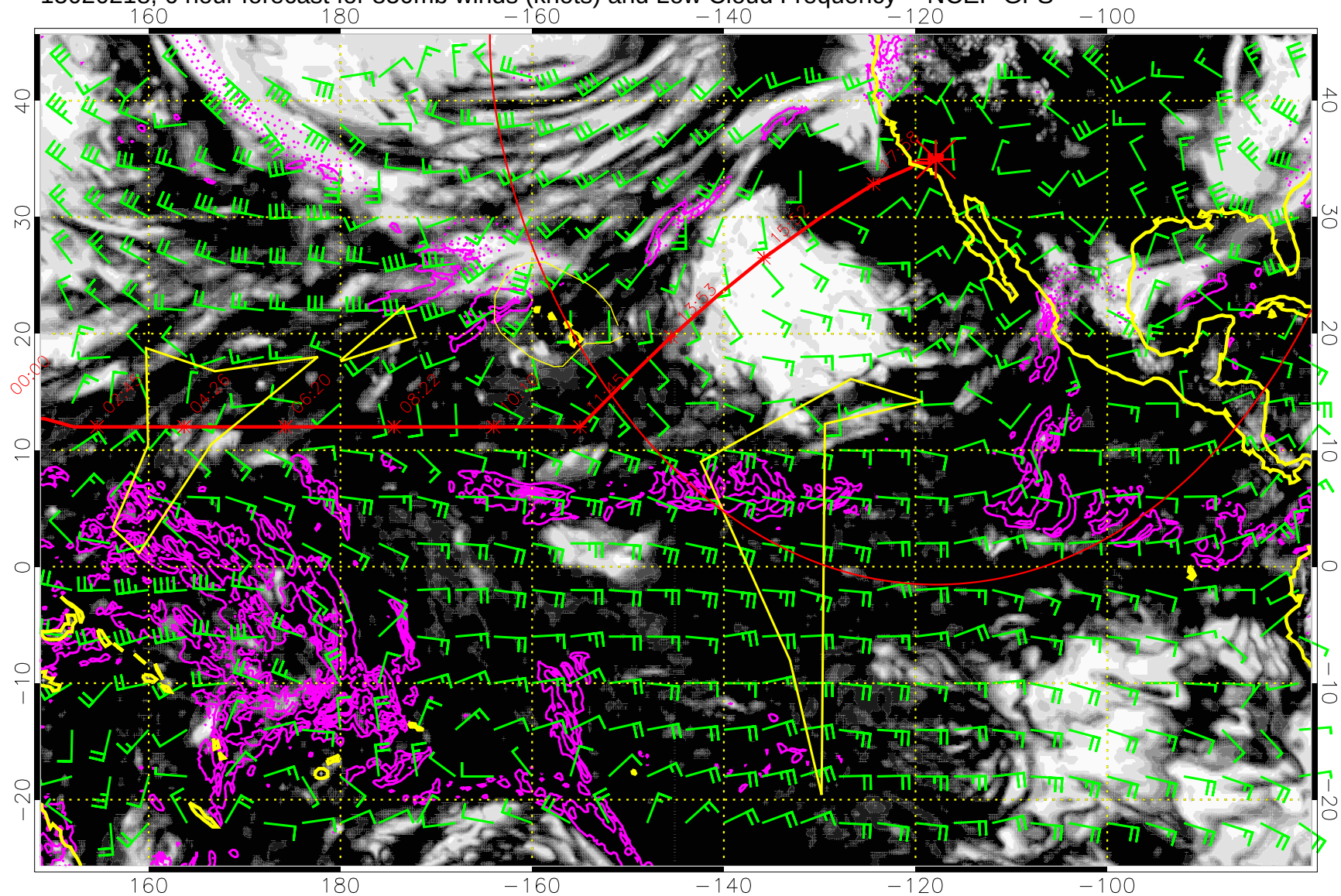
15020218, 6 hour forecast for 850mb winds (knots) and Low Cloud Frequency -- NCEP GFS
