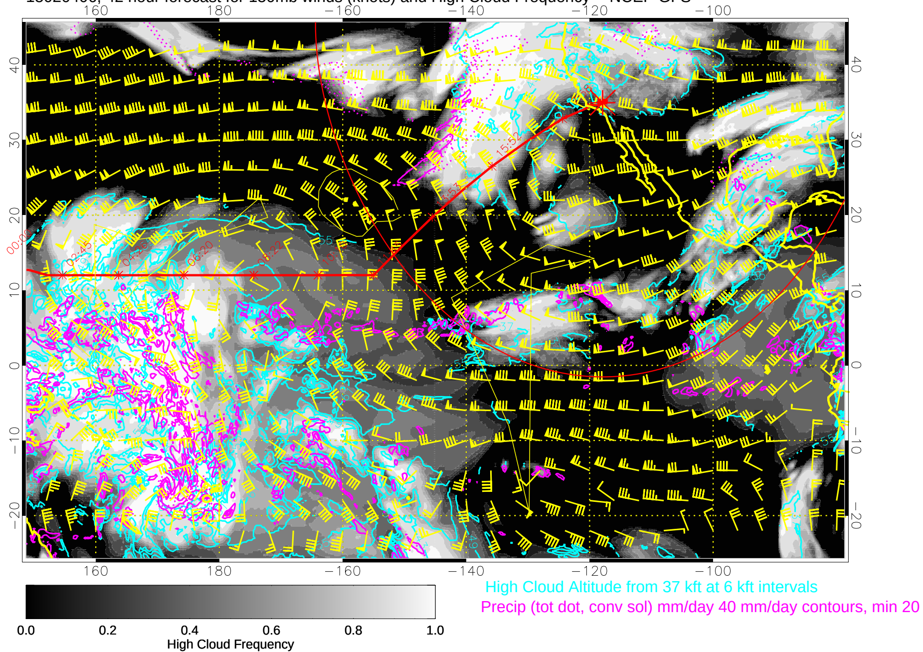
15020406, 42 hour forecast for 150mb winds (knots) and High Cloud Frequency -- NCEP GFS
