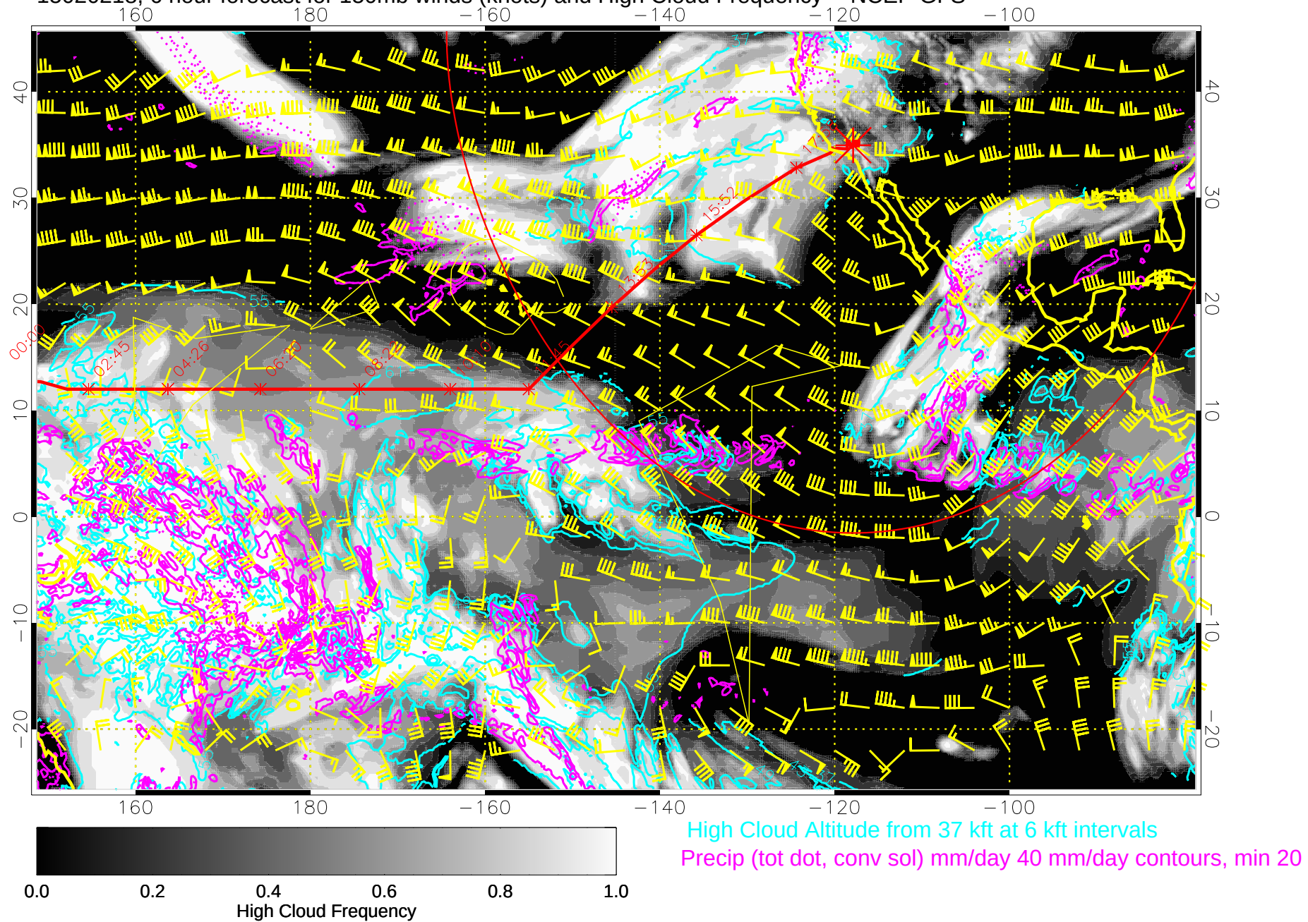
15020218, 6 hour forecast for 150mb winds (knots) and High Cloud Frequency -- NCEP GFS
