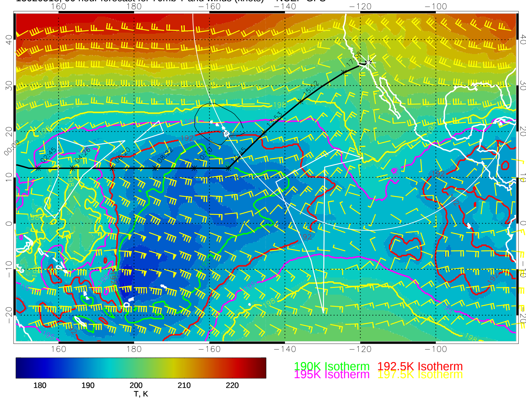
15020518, 90 hour forecast for 70mb T and winds (knots) -- NCEP GFS
