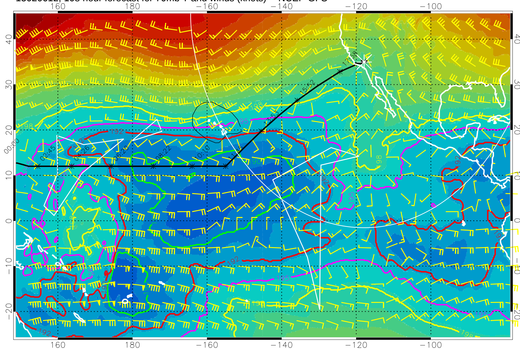
15020612, 108 hour forecast for 70mb T and winds (knots) -- NCEP GFS
