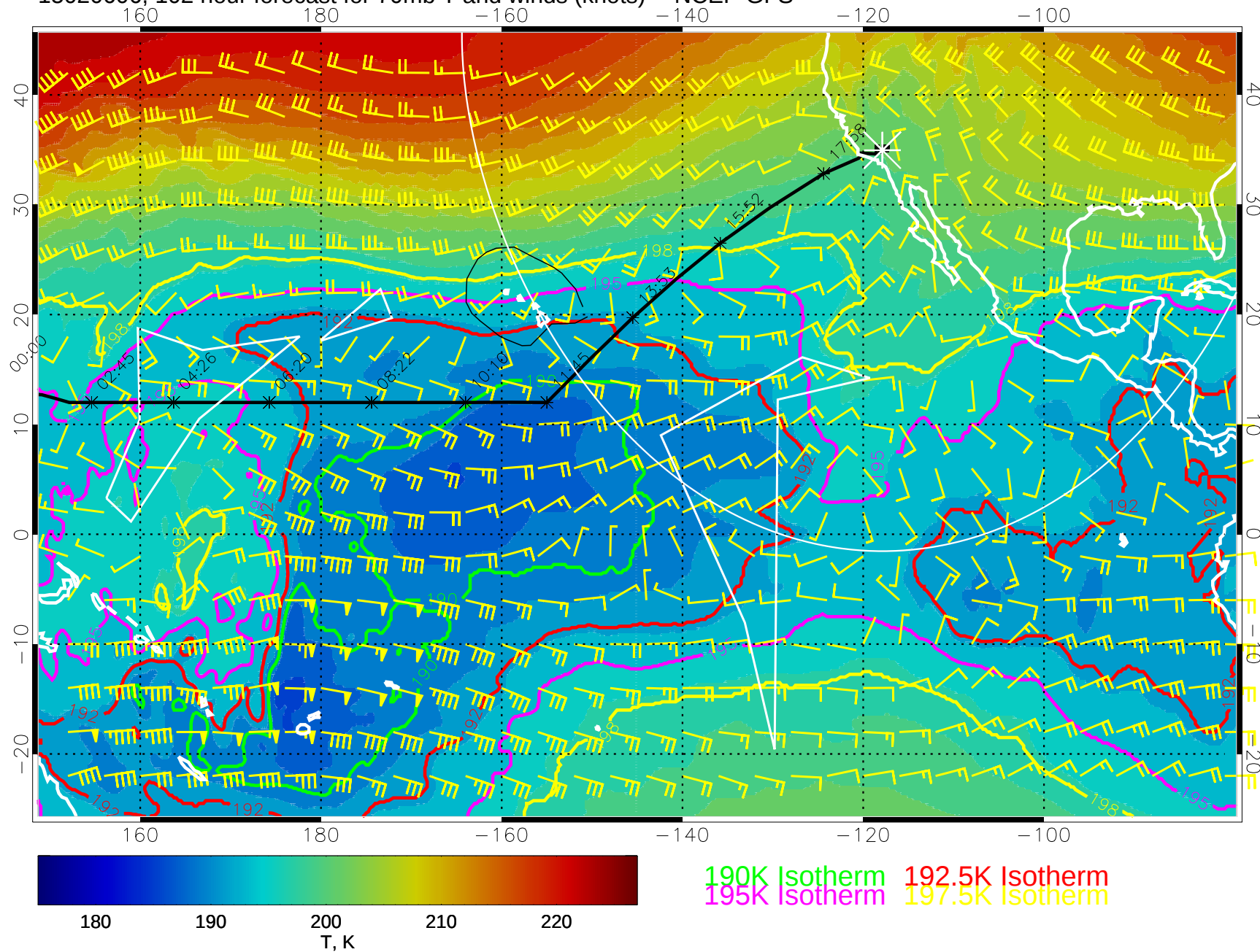
15020606, 102 hour forecast for 70mb T and winds (knots) -- NCEP GFS
