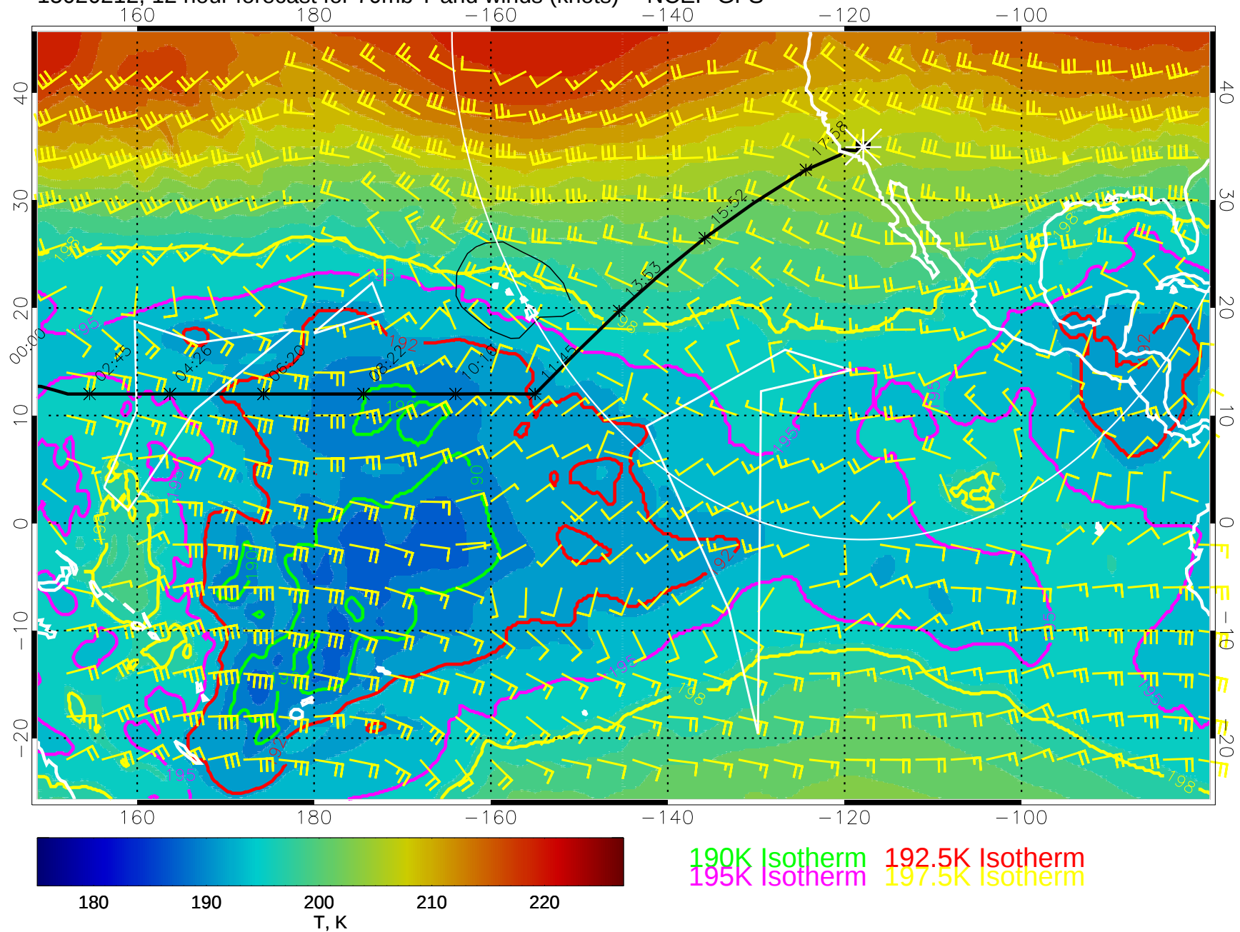
15020212, 12 hour forecast for 70mb T and winds (knots) -- NCEP GFS
