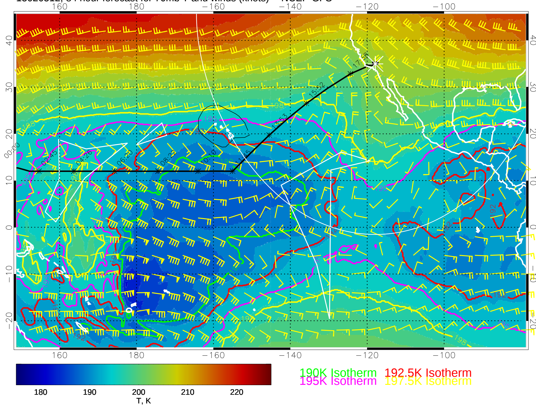
15020512, 84 hour forecast for 70mb T and winds (knots) -- NCEP GFS
