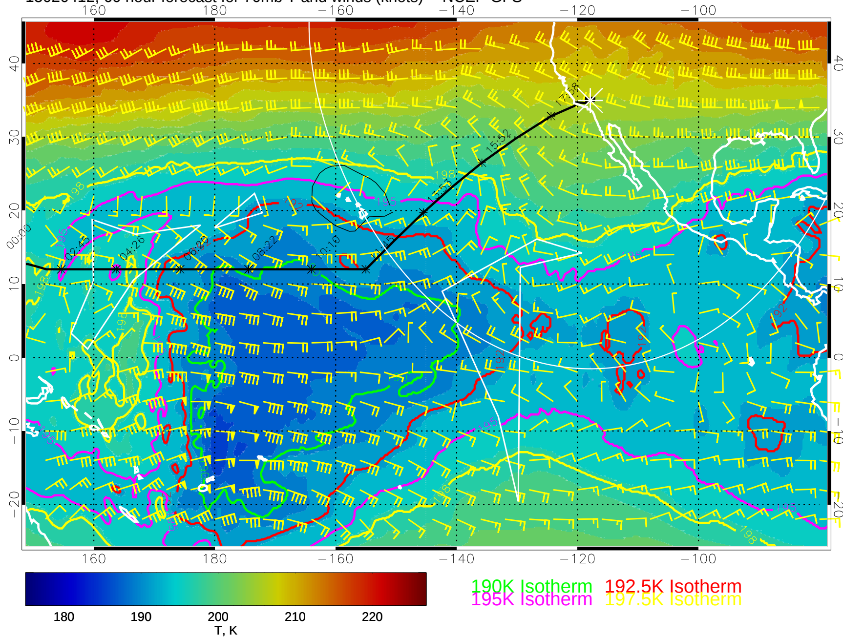
15020412, 60 hour forecast for 70mb T and winds (knots) -- NCEP GFS
