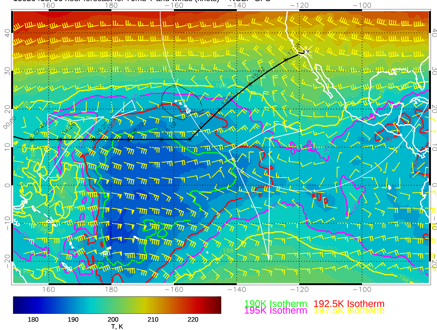
15020418, 66 hour forecast for 70mb T and winds (knots) -- NCEP GFS
