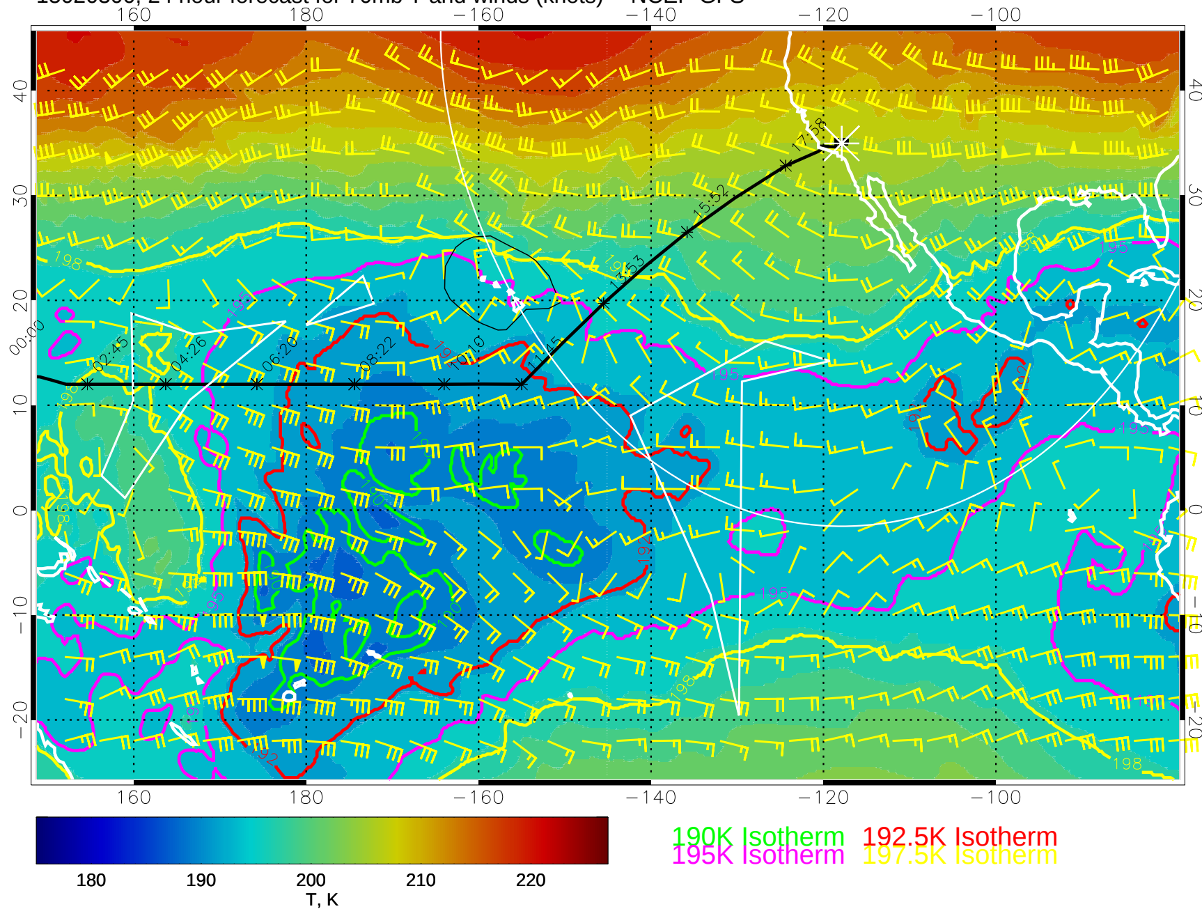
15020300, 24 hour forecast for 70mb T and winds (knots) -- NCEP GFS
