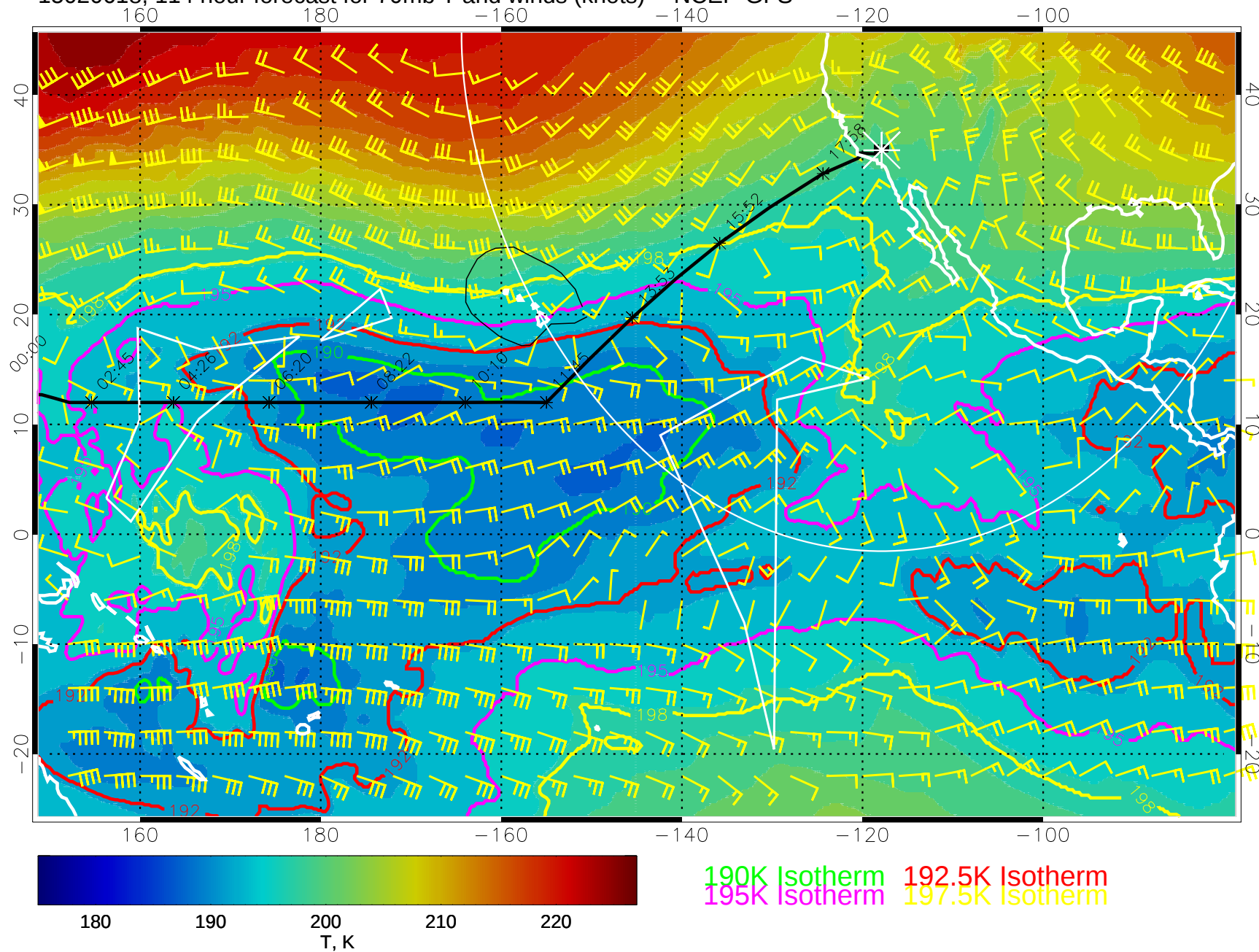
15020618, 114 hour forecast for 70mb T and winds (knots) -- NCEP GFS
