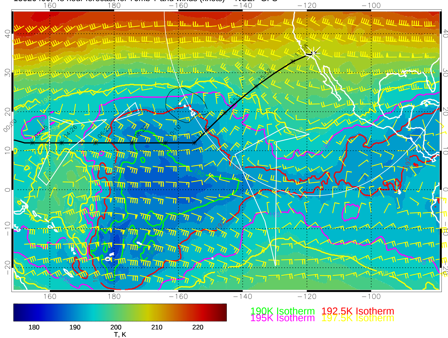
15020400, 48 hour forecast for 70mb T and winds (knots) -- NCEP GFS
