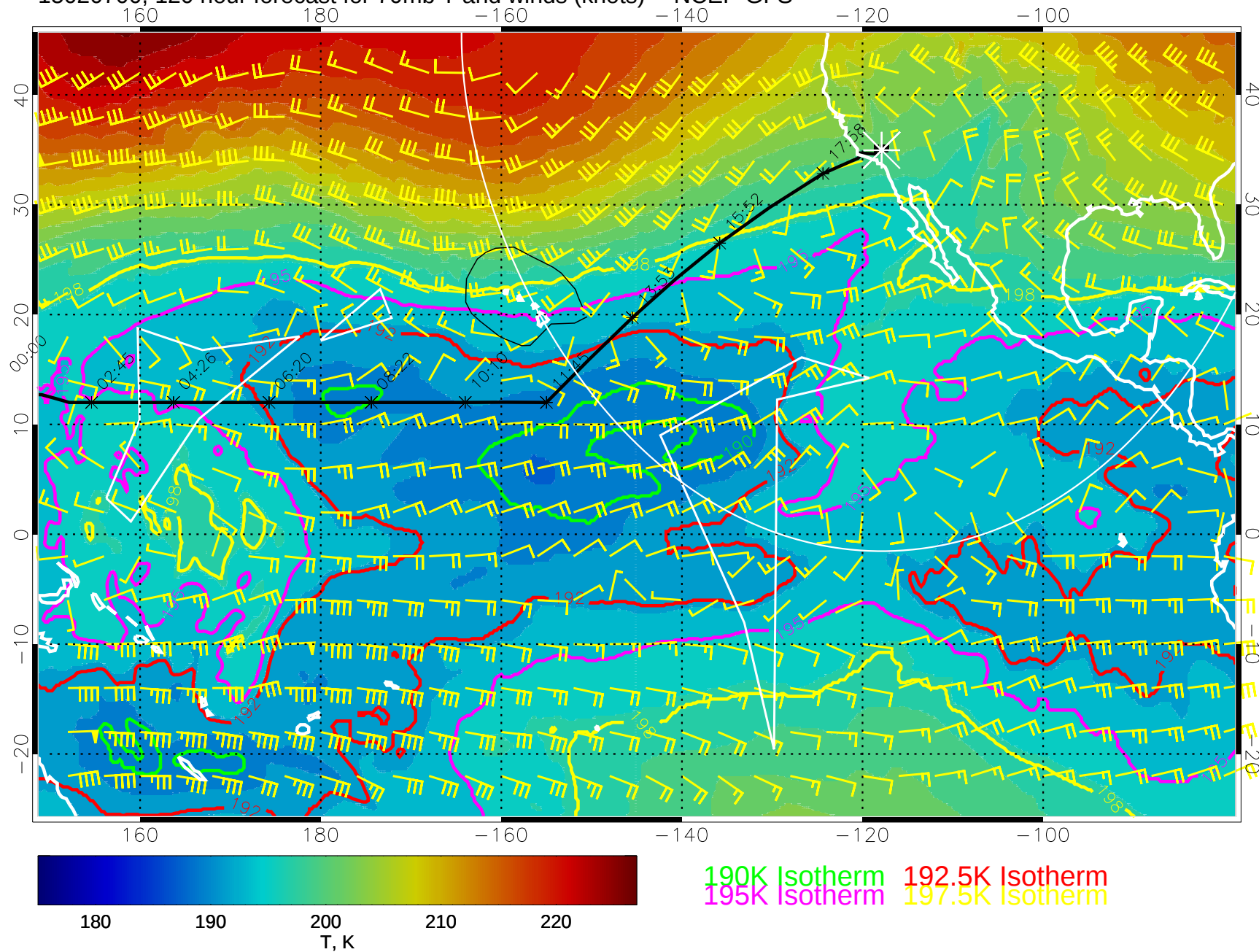
15020700, 120 hour forecast for 70mb T and winds (knots) -- NCEP GFS
