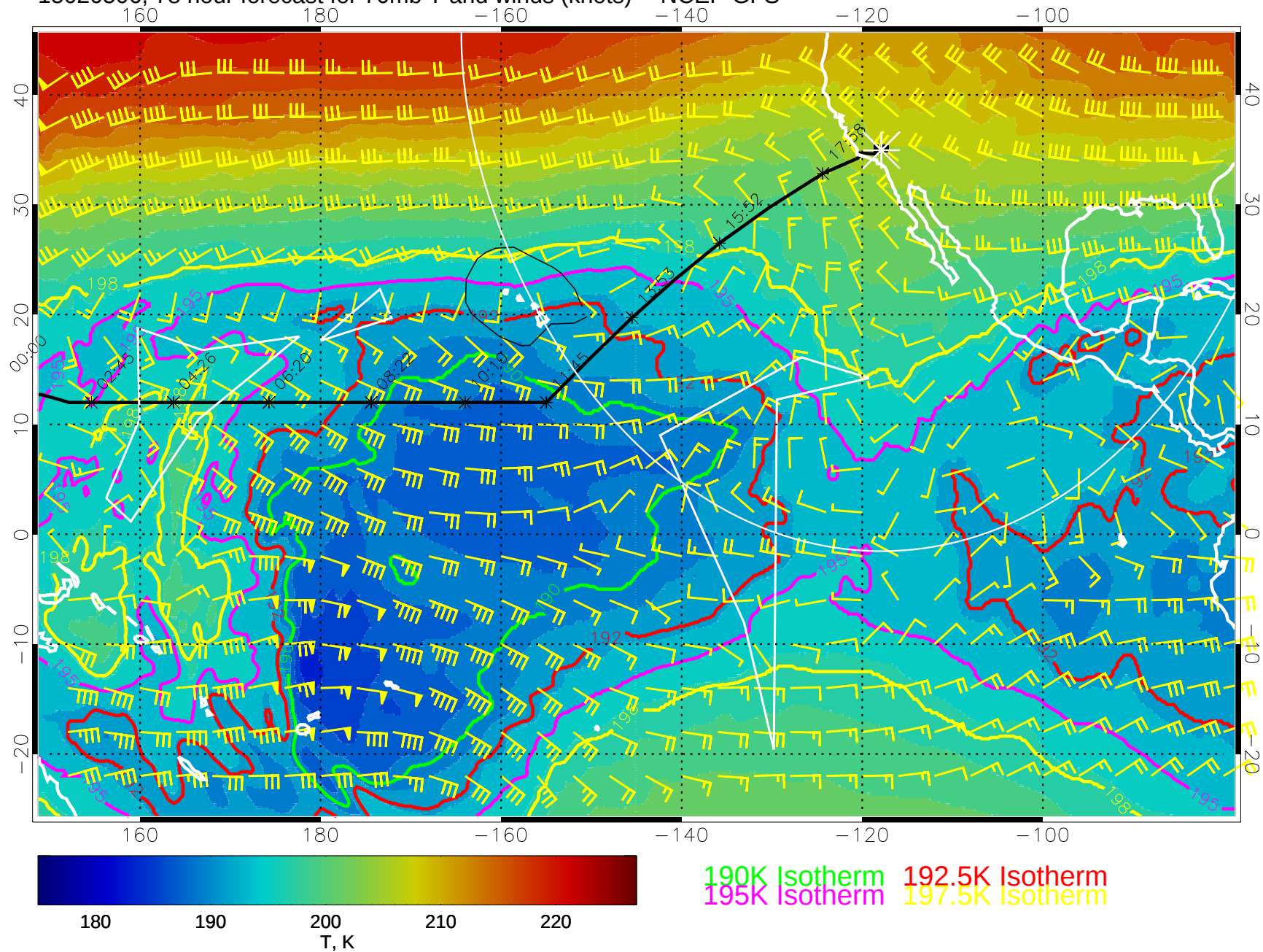
15020506, 78 hour forecast for 70mb T and winds (knots) -- NCEP GFS
