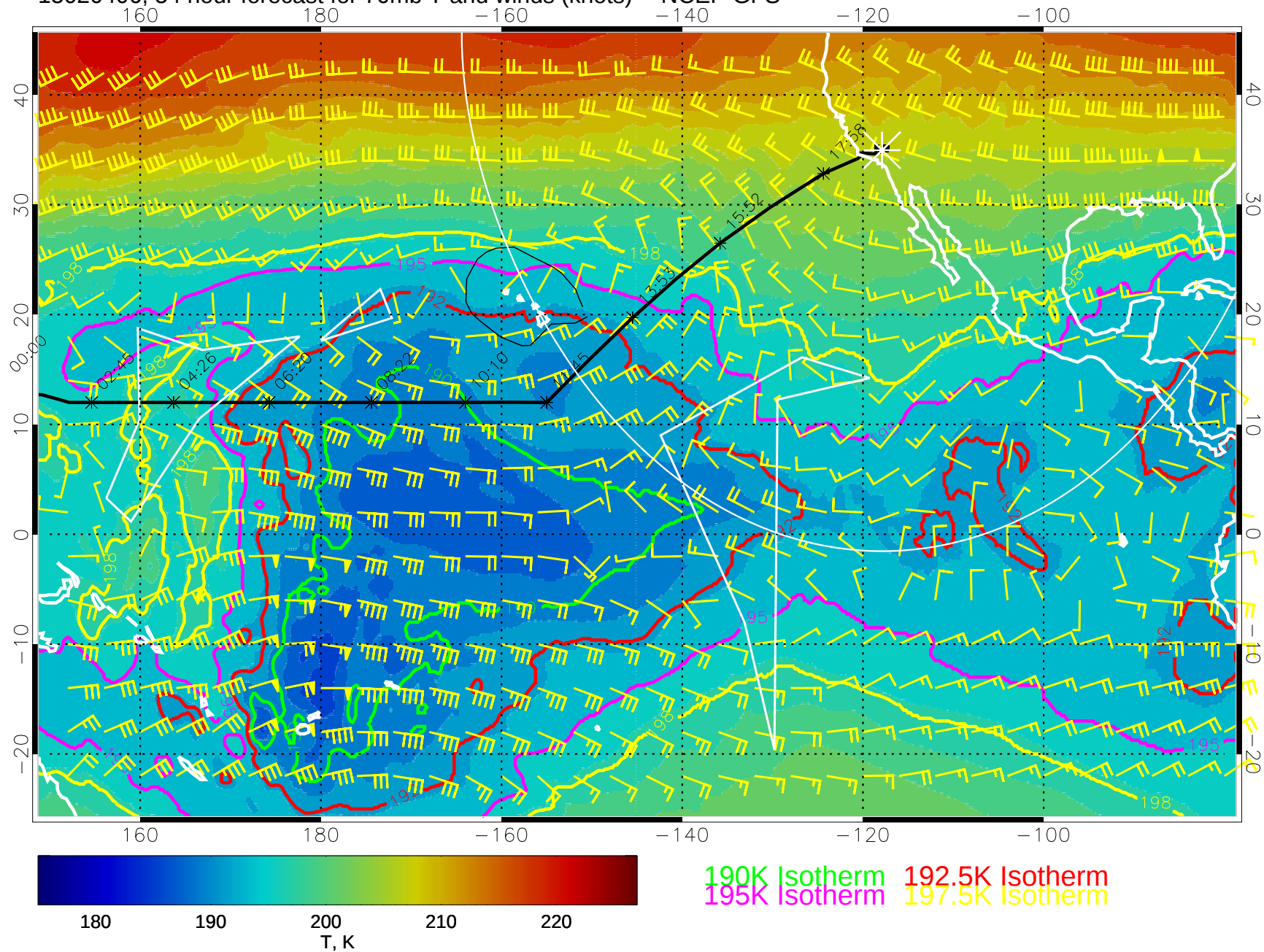
15020406, 54 hour forecast for 70mb T and winds (knots) -- NCEP GFS
