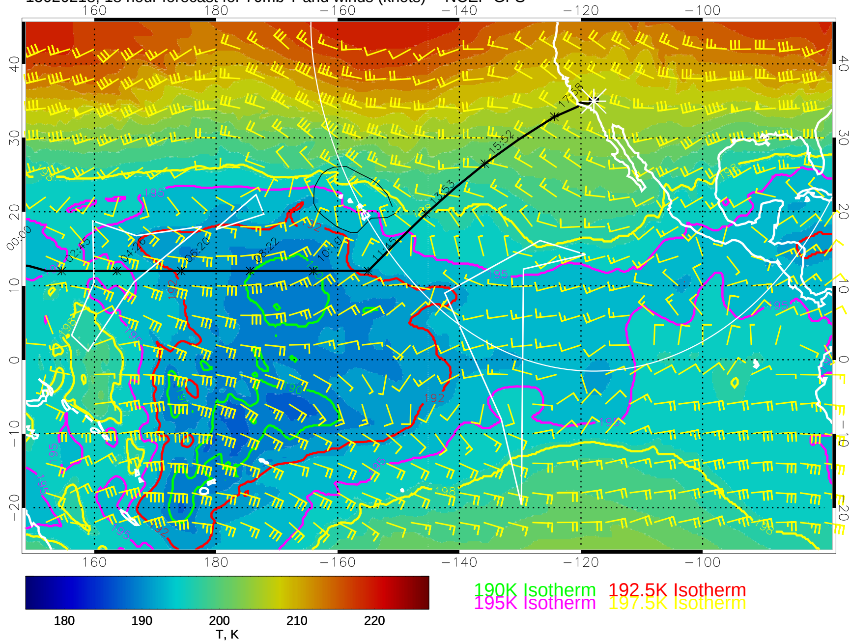
15020218, 18 hour forecast for 70mb T and winds (knots) -- NCEP GFS
