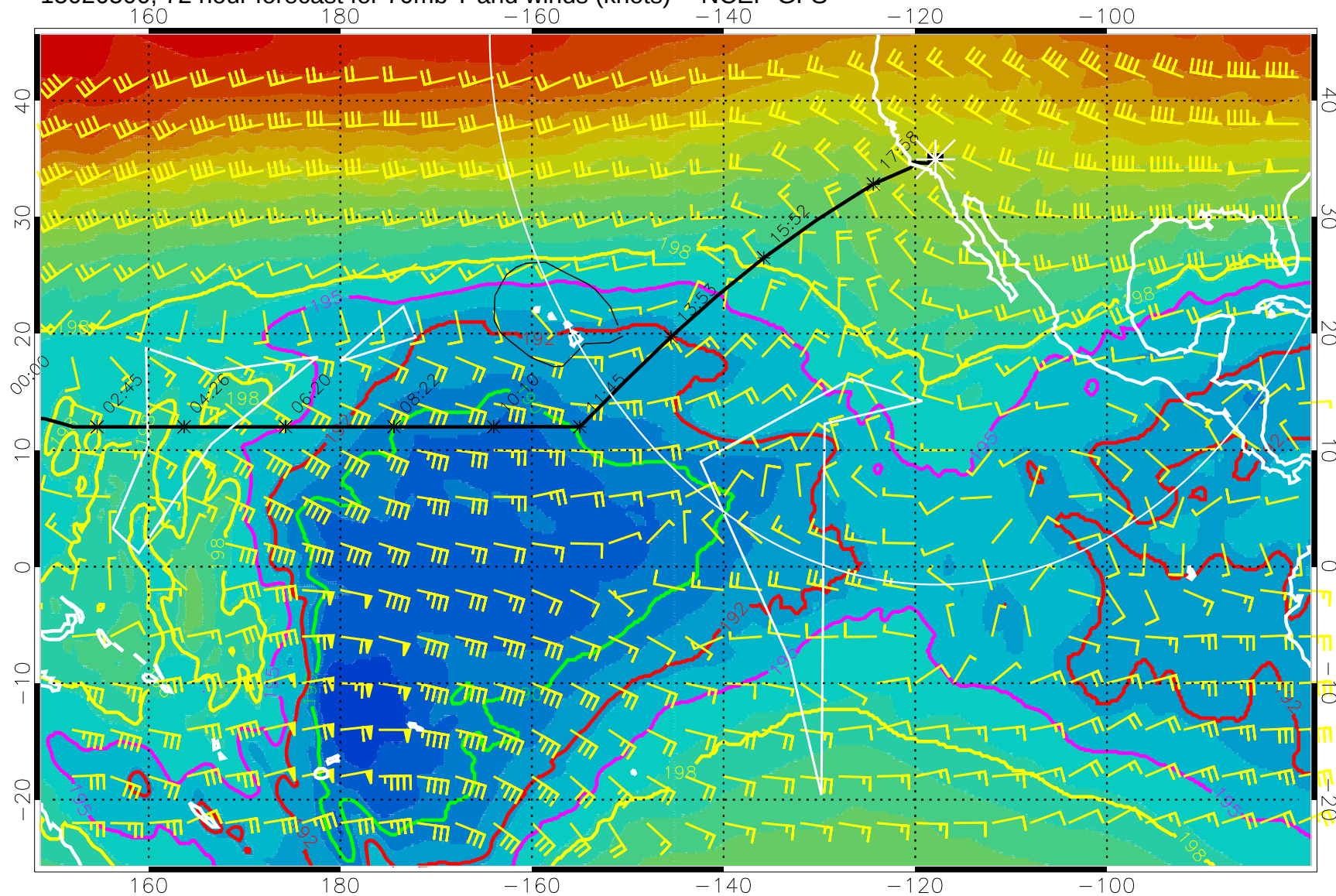
15020500, 72 hour forecast for 70mb T and winds (knots) -- NCEP GFS
