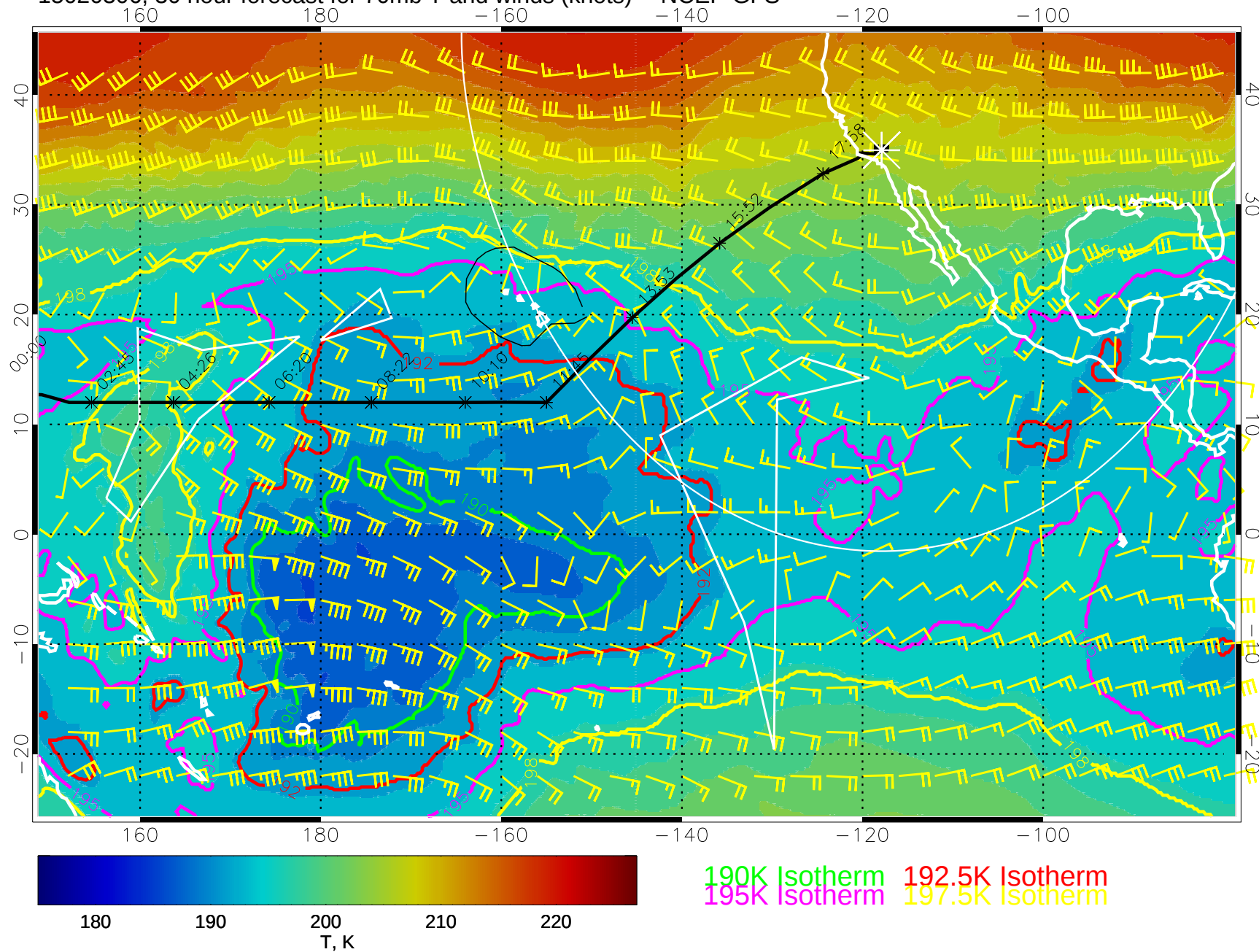
15020306, 30 hour forecast for 70mb T and winds (knots) -- NCEP GFS
