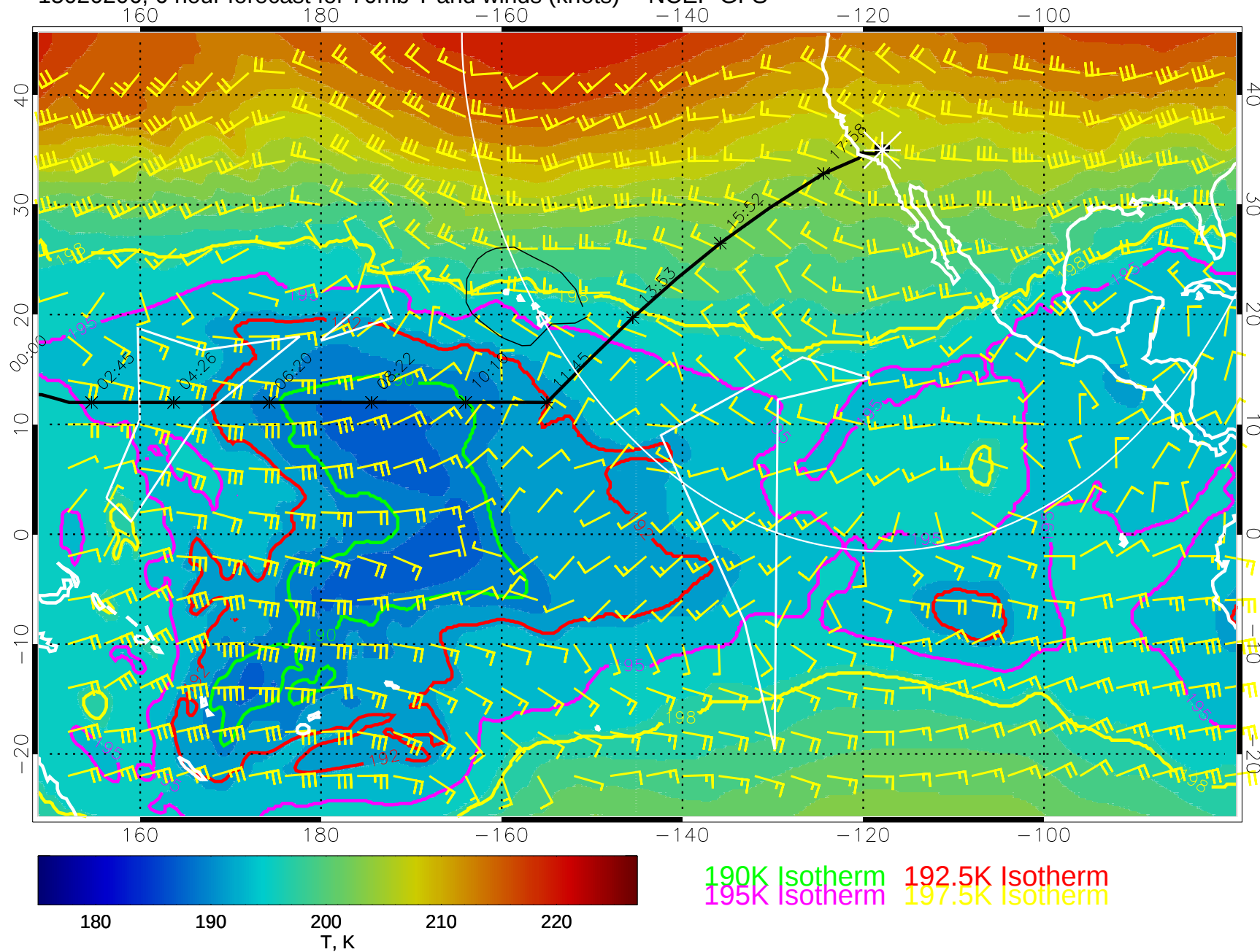
15020206, 6 hour forecast for 70mb T and winds (knots) -- NCEP GFS
