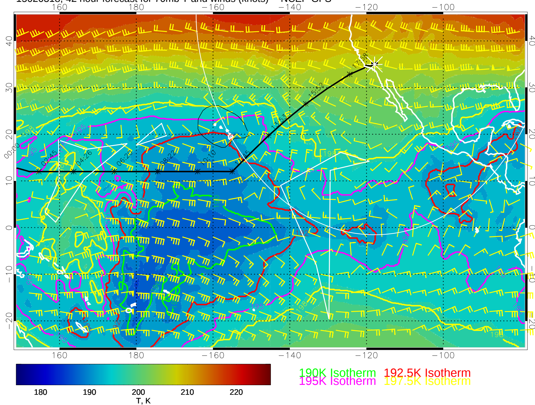
15020318, 42 hour forecast for 70mb T and winds (knots) -- NCEP GFS
