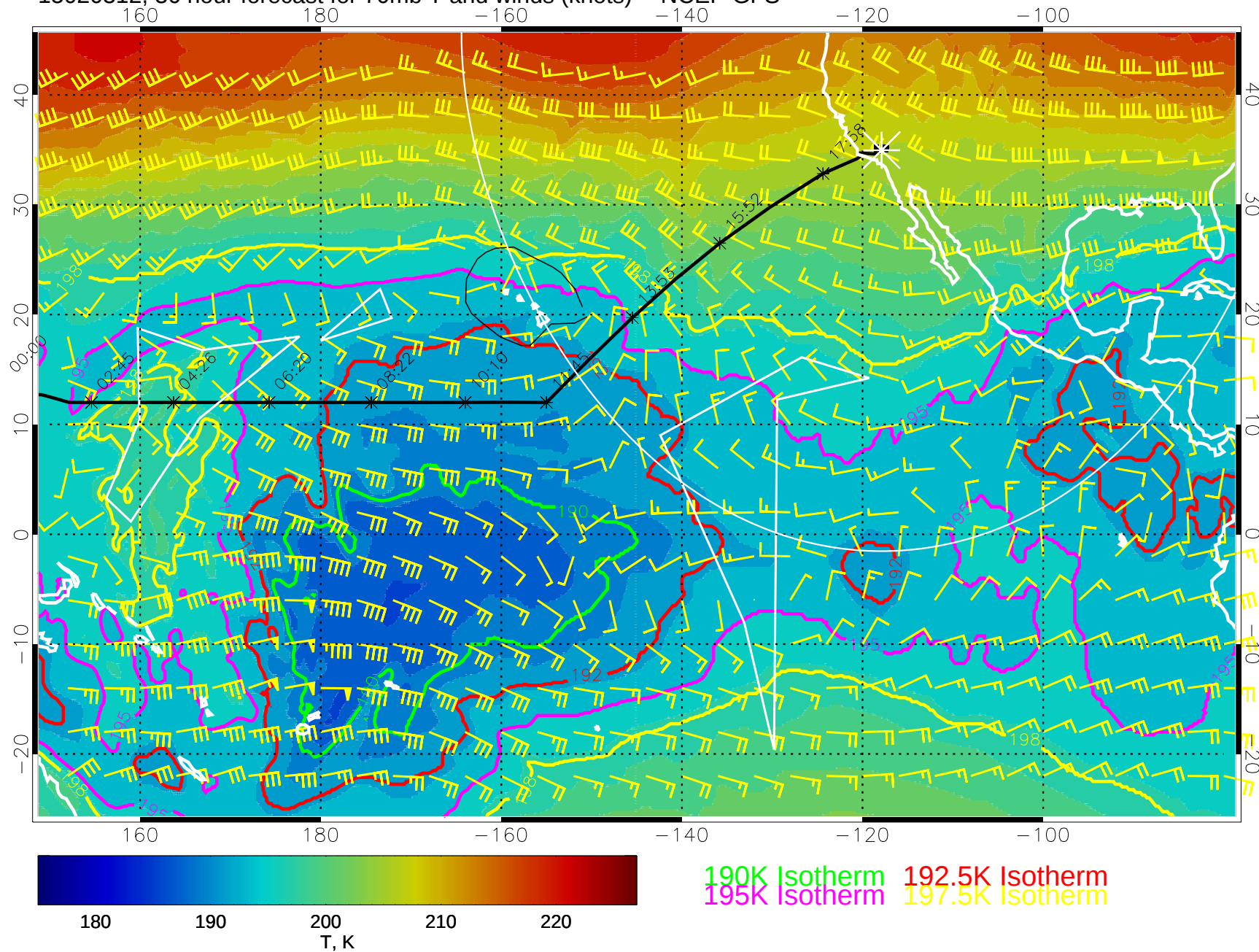
15020312, 36 hour forecast for 70mb T and winds (knots) -- NCEP GFS
