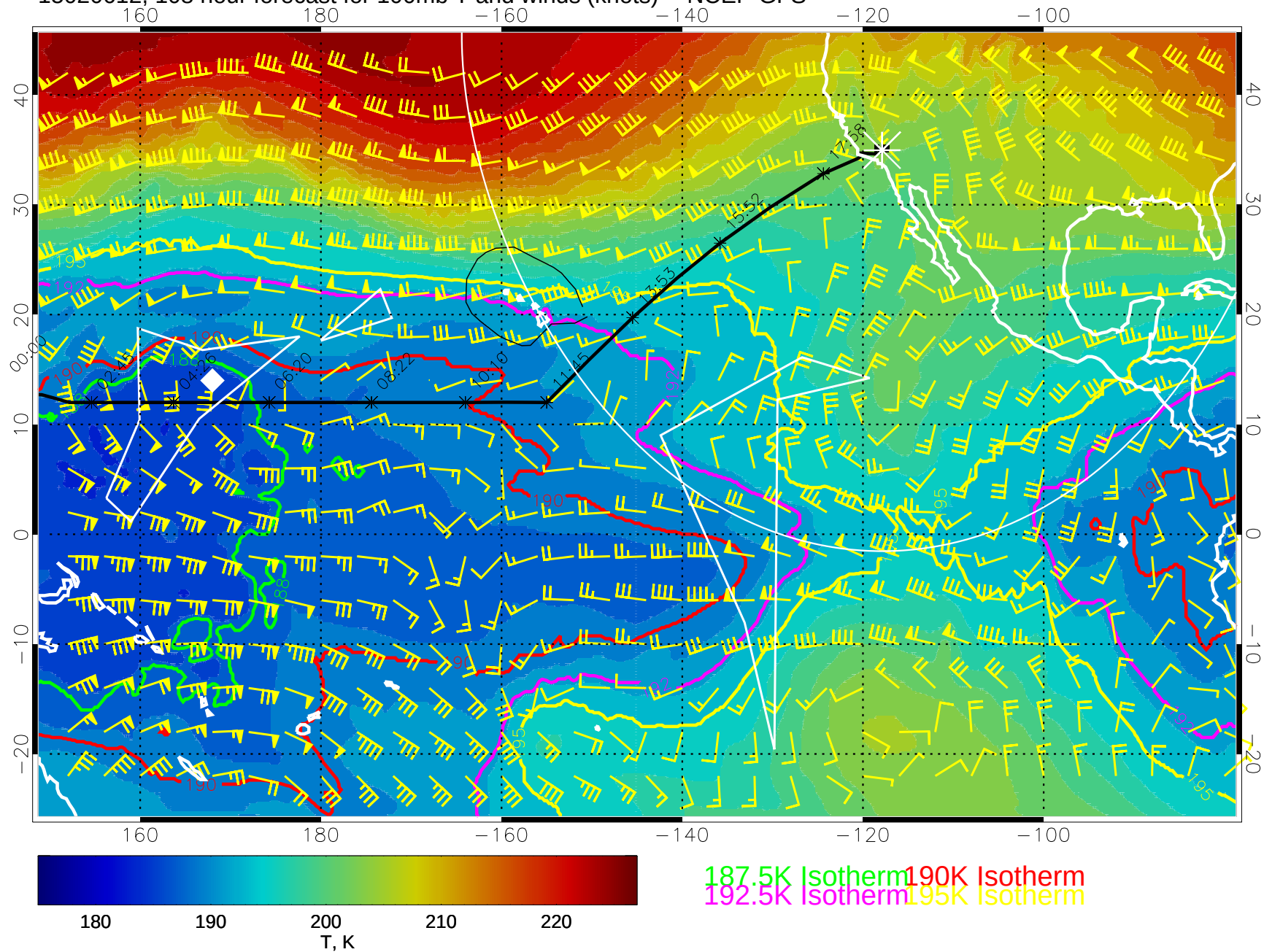
15020612, 108 hour forecast for 100mb T and winds (knots) -- NCEP GFS
