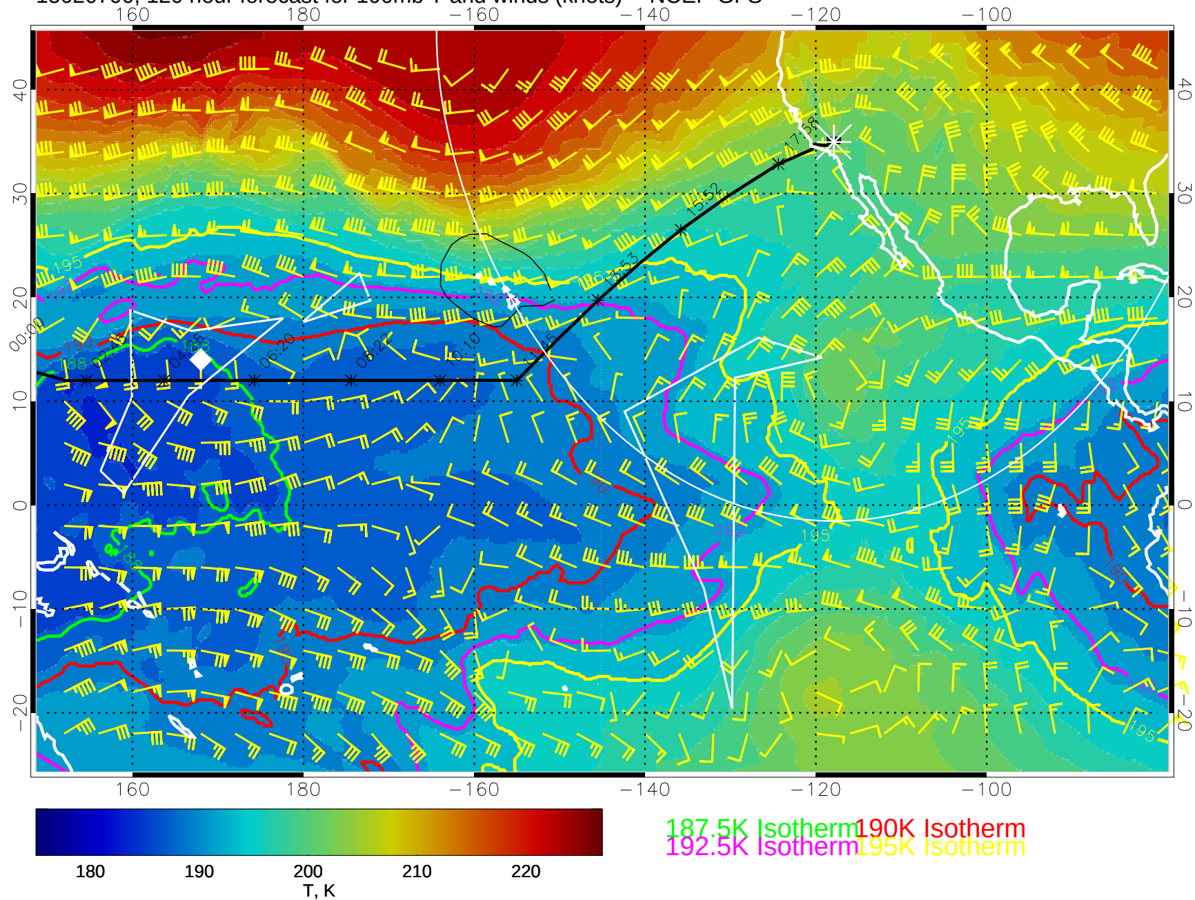
15020700, 120 hour forecast for 100mb T and winds (knots) -- NCEP GFS
