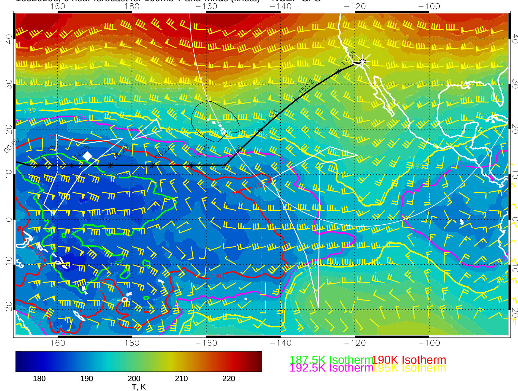
15020206, 6 hour forecast for 100mb T and winds (knots) -- NCEP GFS
