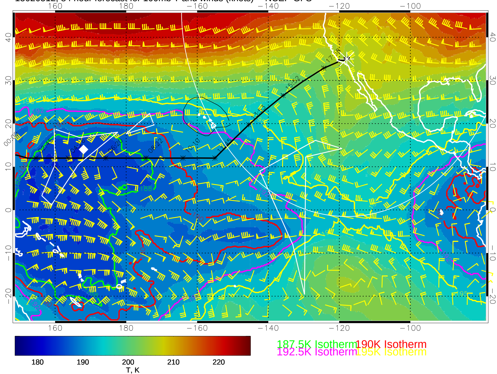
15020512, 84 hour forecast for 100mb T and winds (knots) -- NCEP GFS
