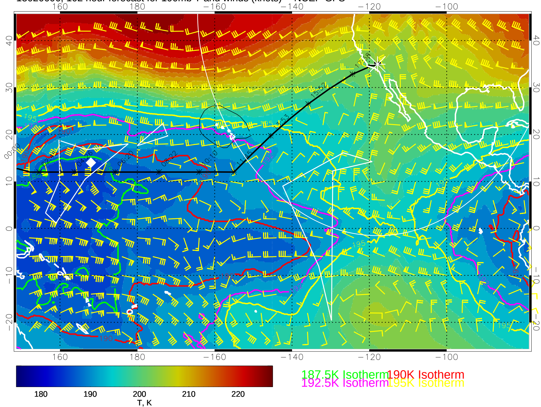
15020606, 102 hour forecast for 100mb T and winds (knots) -- NCEP GFS
