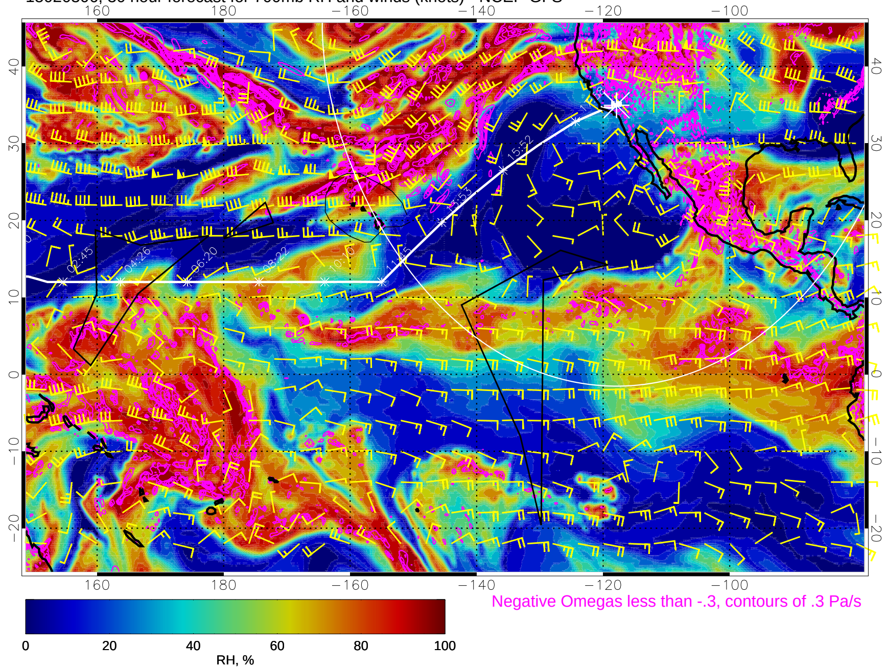
15020306, 30 hour forecast for 700mb RH and winds (knots) - NCEP GFS
