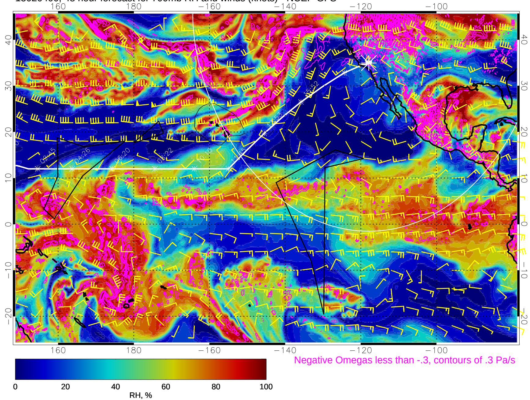
15020400, 48 hour forecast for 700mb RH and winds (knots) - NCEP GFS
