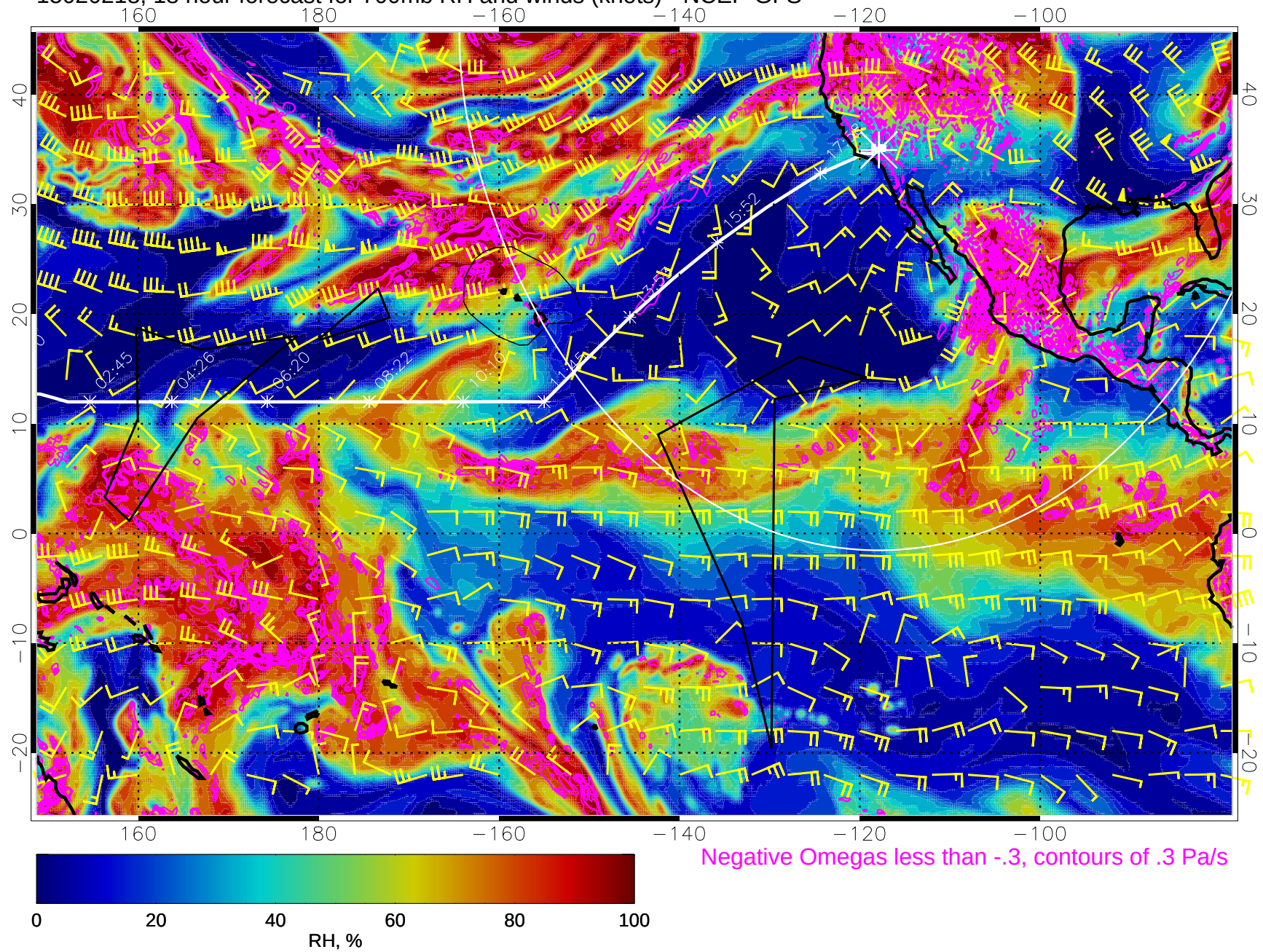
15020218, 18 hour forecast for 700mb RH and winds (knots) - NCEP GFS
