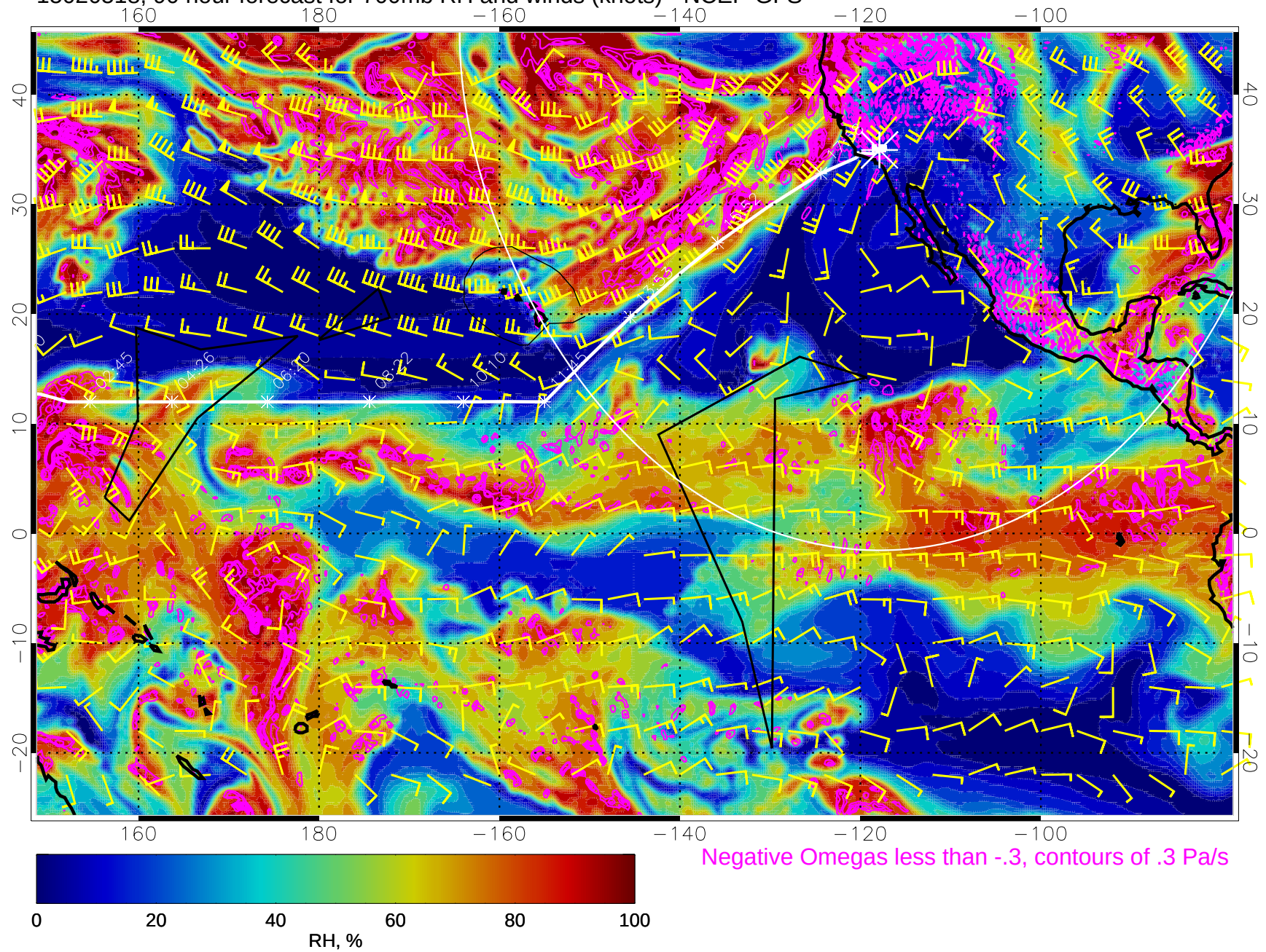
15020518, 90 hour forecast for 700mb RH and winds (knots) - NCEP GFS
