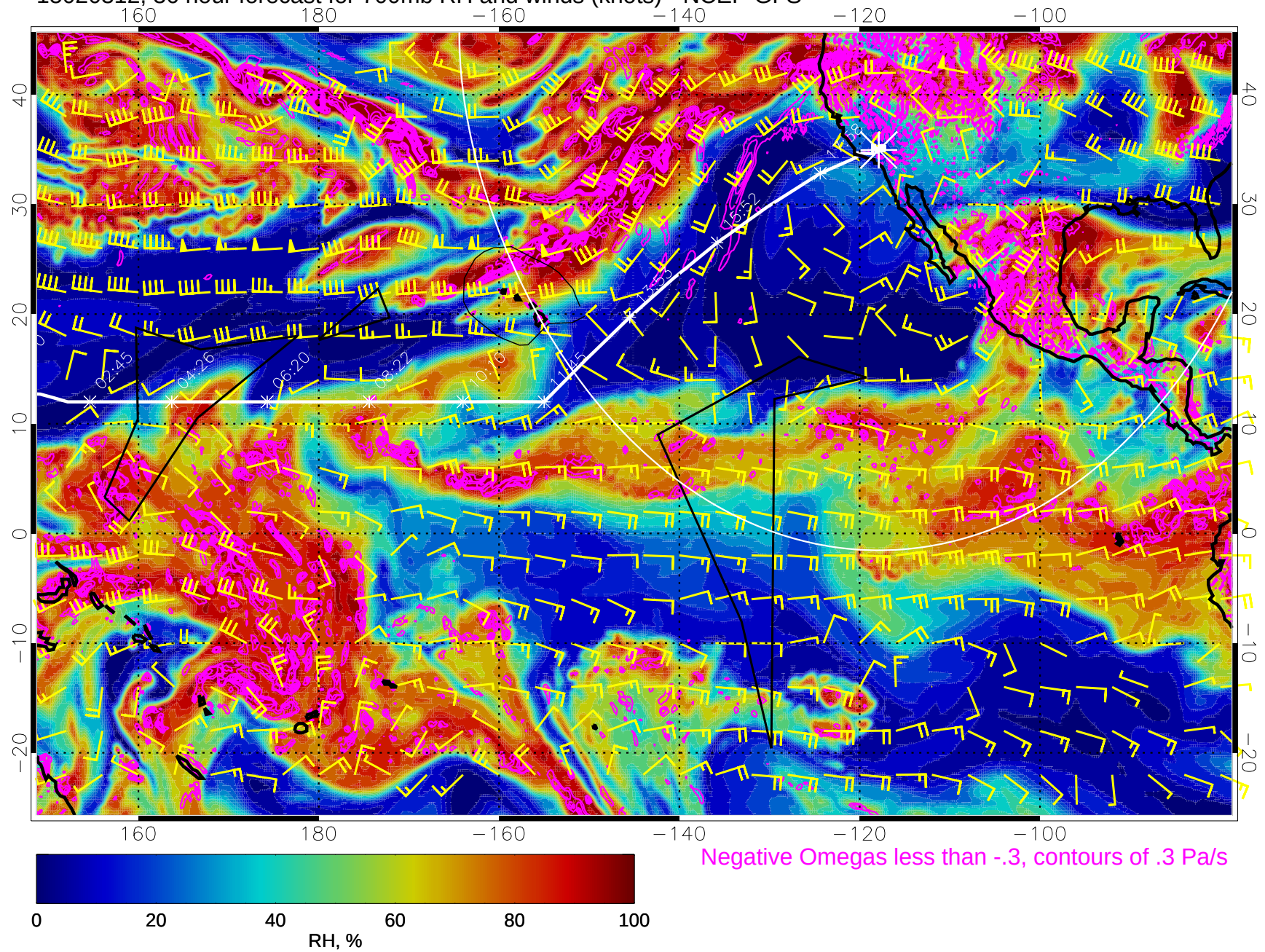
15020312, 36 hour forecast for 700mb RH and winds (knots) - NCEP GFS
