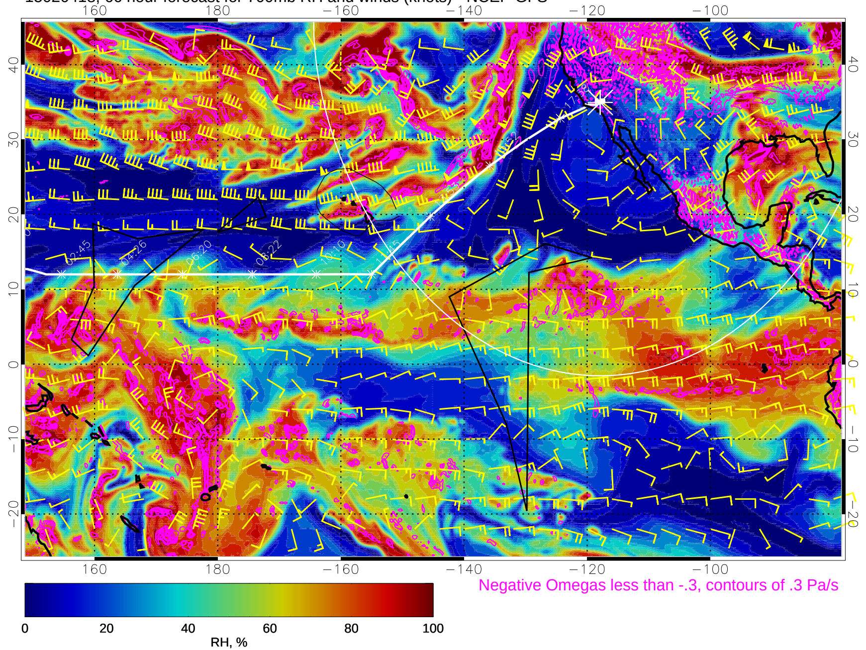
15020418, 66 hour forecast for 700mb RH and winds (knots) - NCEP GFS
