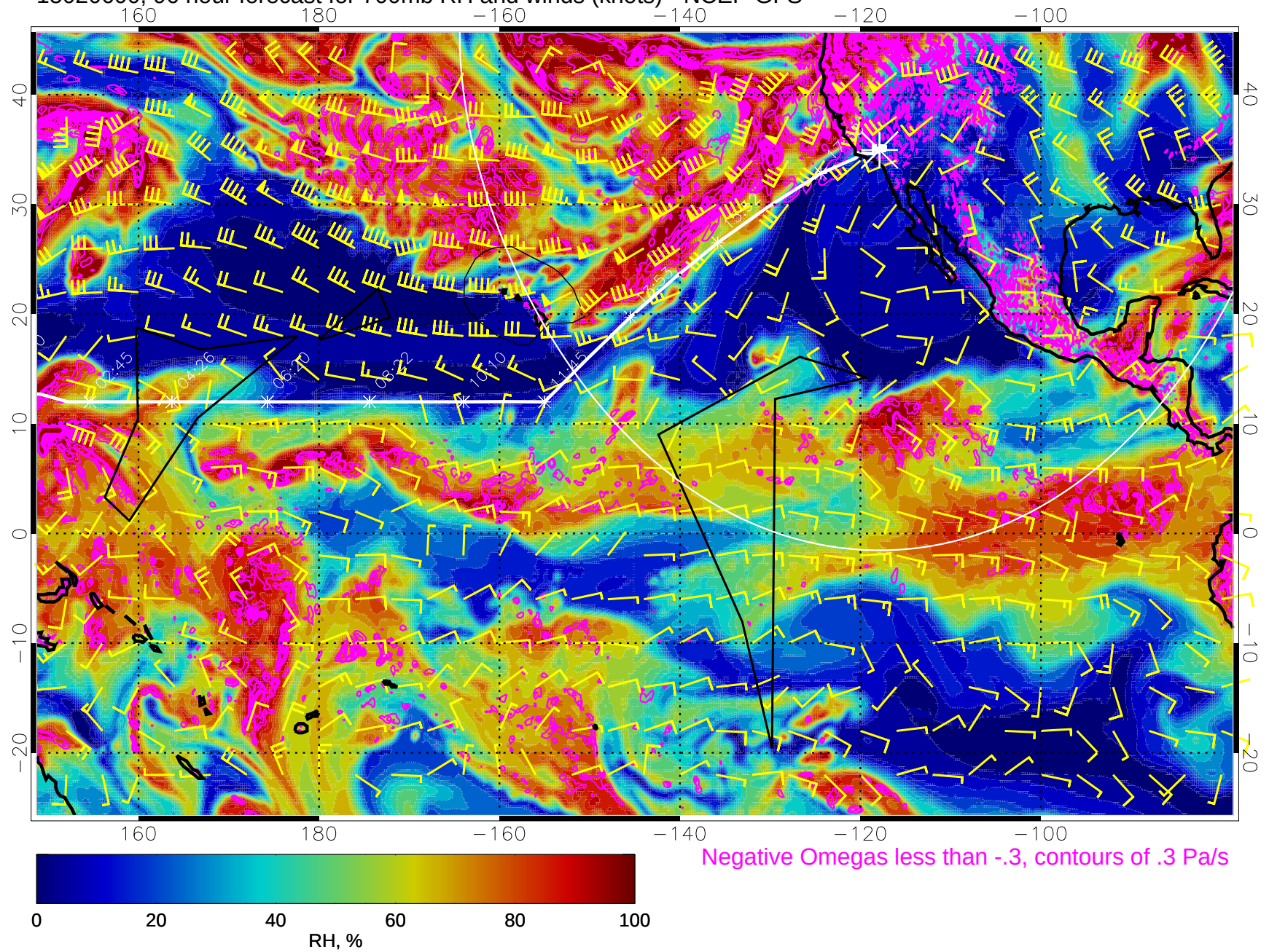
15020600, 96 hour forecast for 700mb RH and winds (knots) - NCEP GFS
