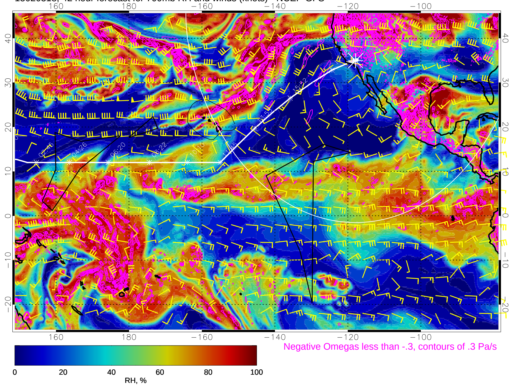
15020318, 42 hour forecast for 700mb RH and winds (knots) - NCEP GFS
