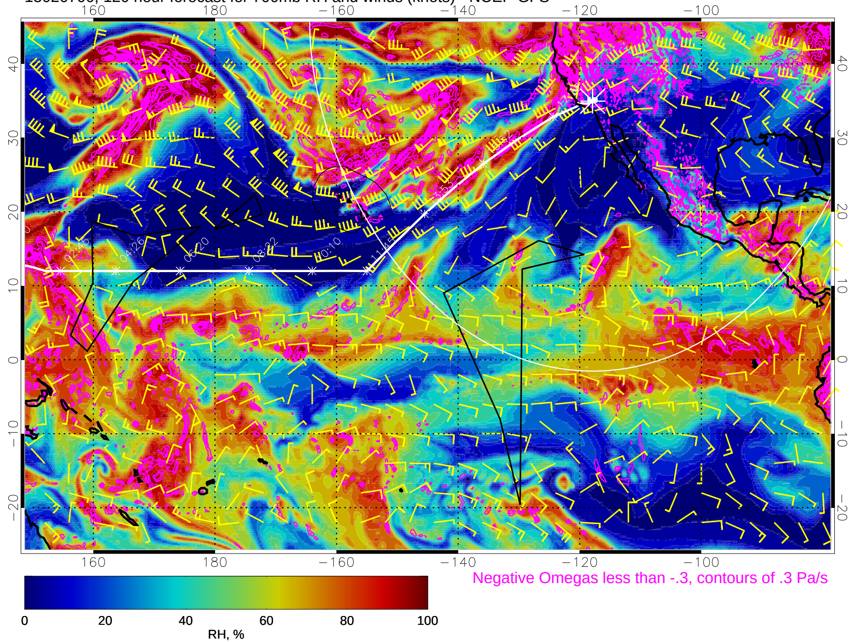
15020700, 120 hour forecast for 700mb RH and winds (knots) - NCEP GFS
