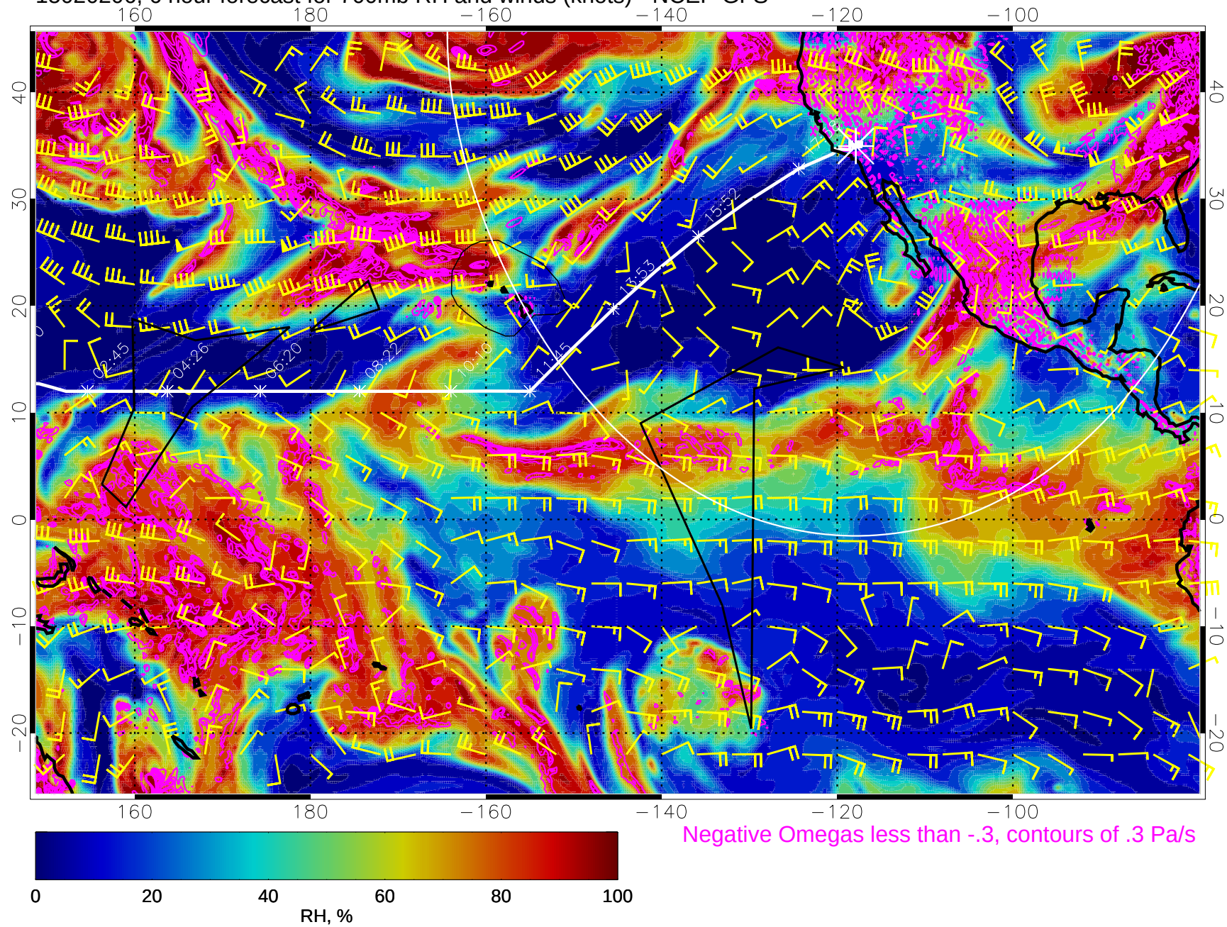
15020206, 6 hour forecast for 700mb RH and winds (knots) - NCEP GFS
