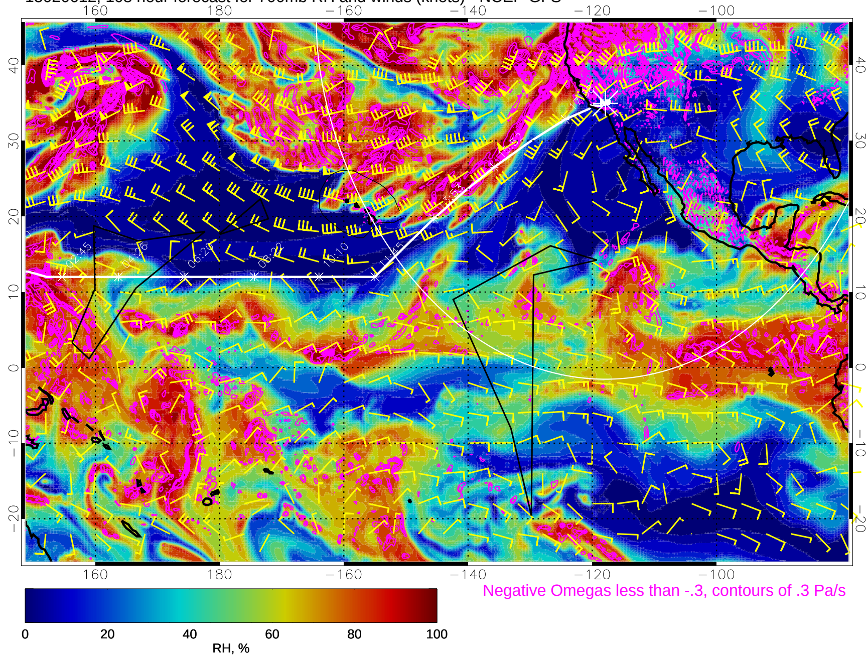
15020612, 108 hour forecast for 700mb RH and winds (knots) - NCEP GFS
