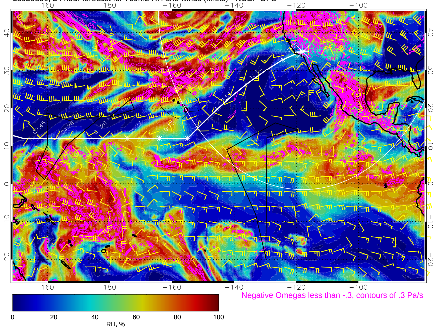
15020300, 24 hour forecast for 700mb RH and winds (knots) - NCEP GFS
