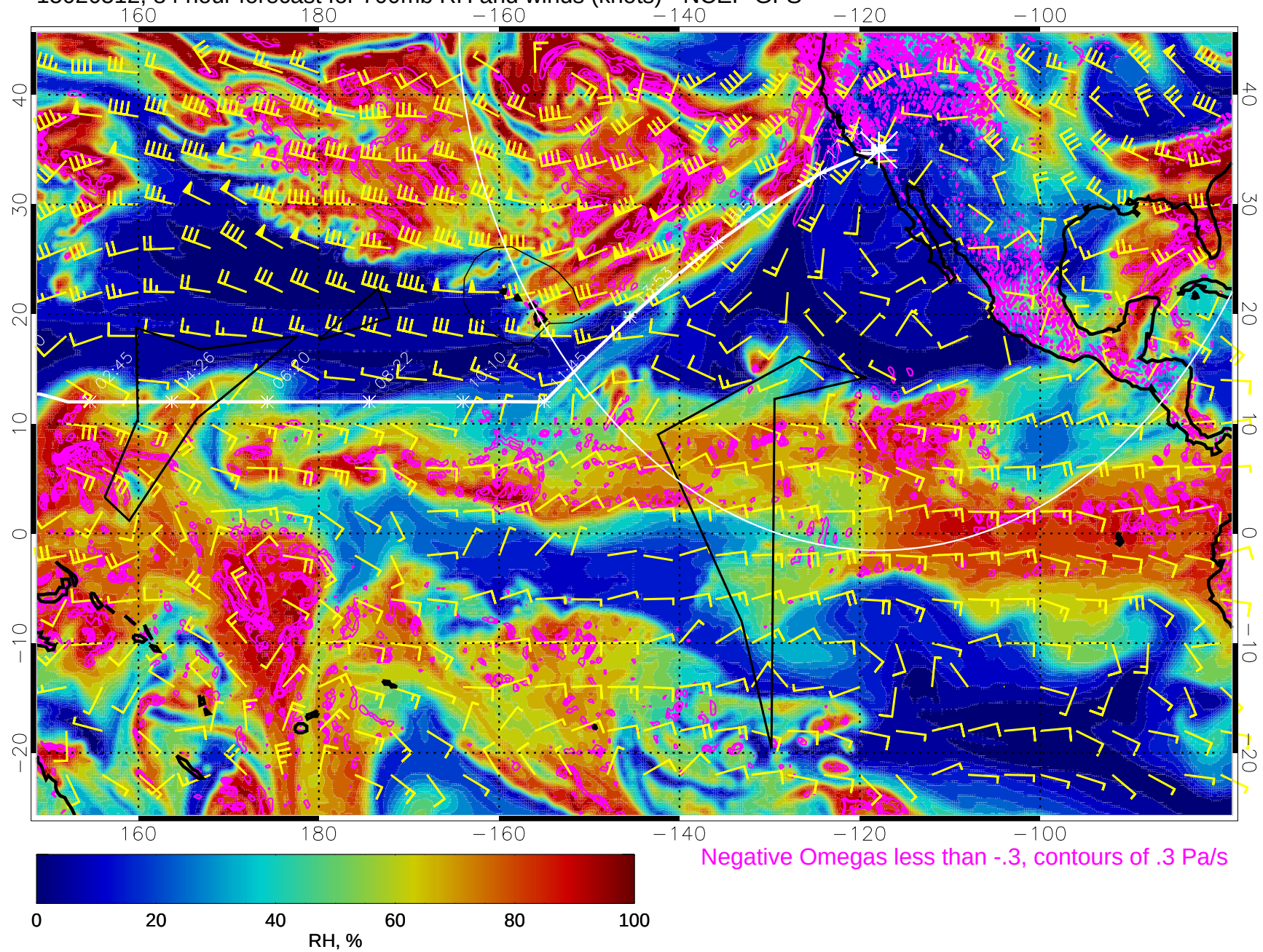
15020512, 84 hour forecast for 700mb RH and winds (knots) - NCEP GFS
