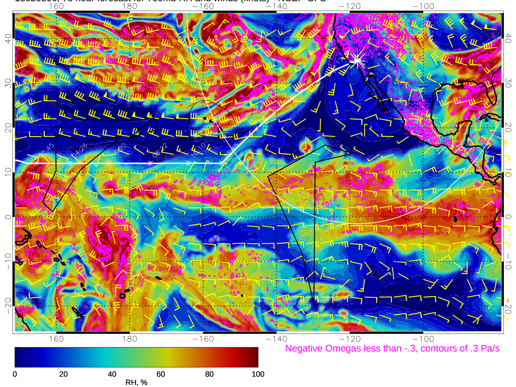
15020506, 78 hour forecast for 700mb RH and winds (knots) - NCEP GFS
