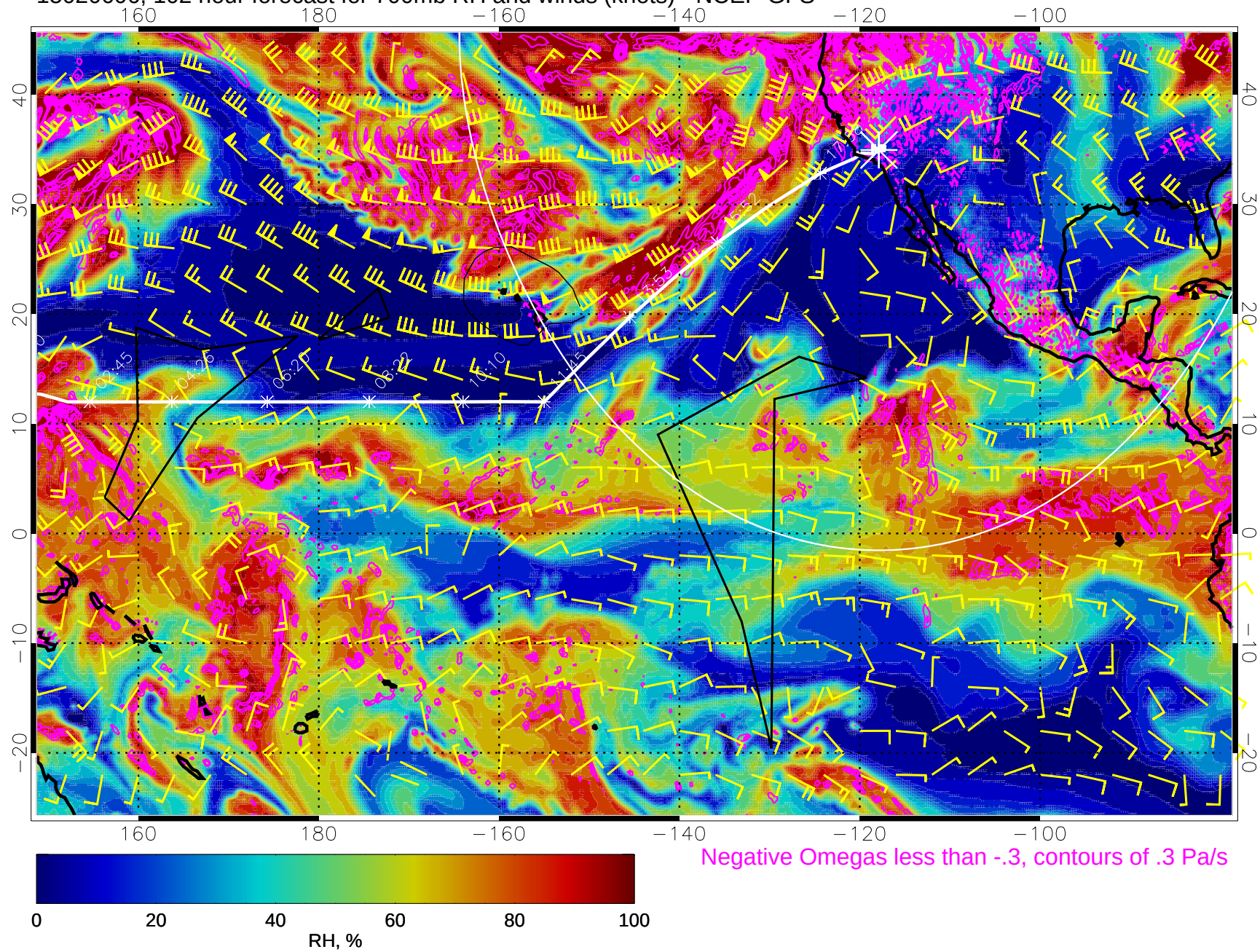
15020606, 102 hour forecast for 700mb RH and winds (knots) - NCEP GFS
