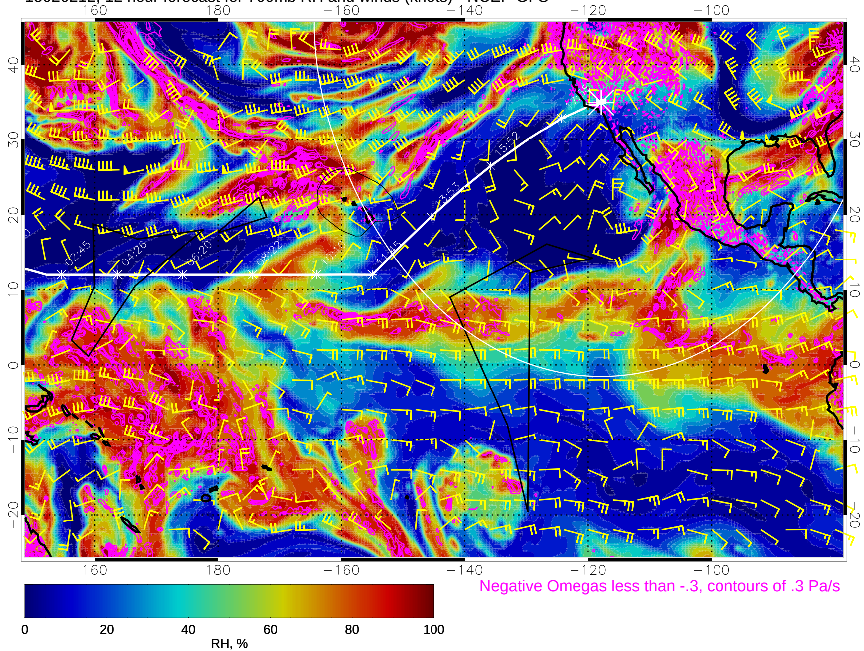
15020212, 12 hour forecast for 700mb RH and winds (knots) - NCEP GFS
