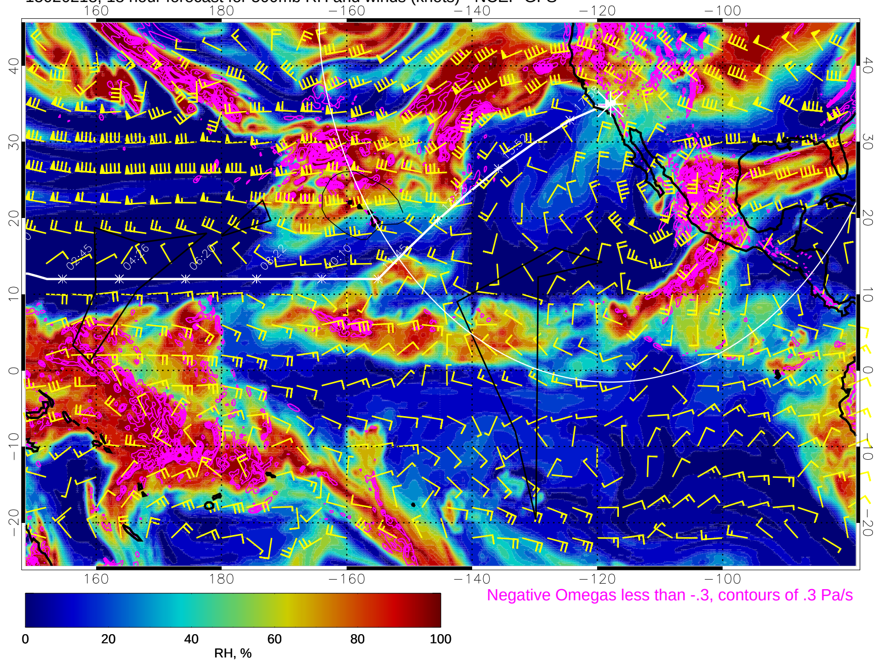
15020218, 18 hour forecast for 500mb RH and winds (knots) - NCEP GFS
