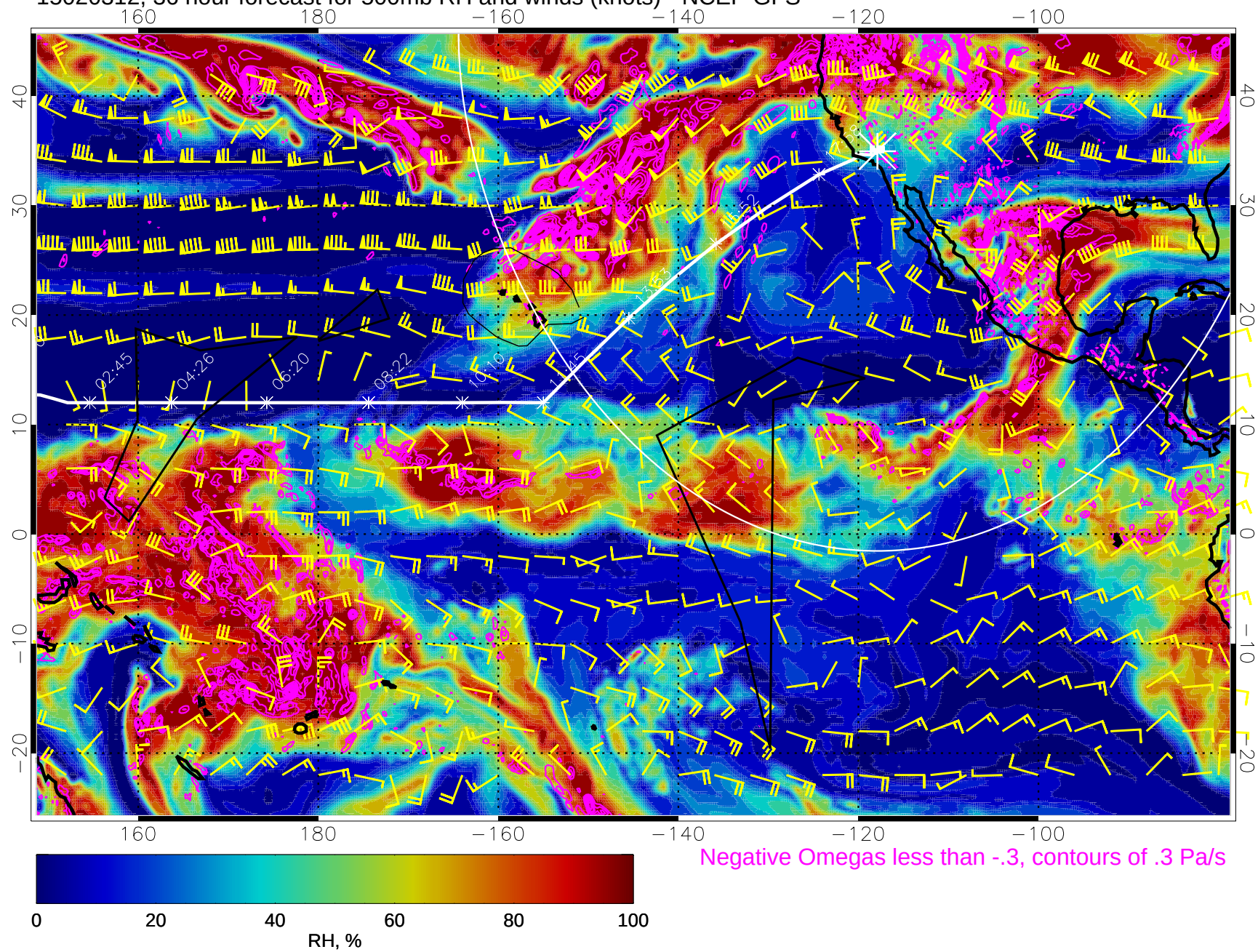
15020312, 36 hour forecast for 500mb RH and winds (knots) - NCEP GFS
