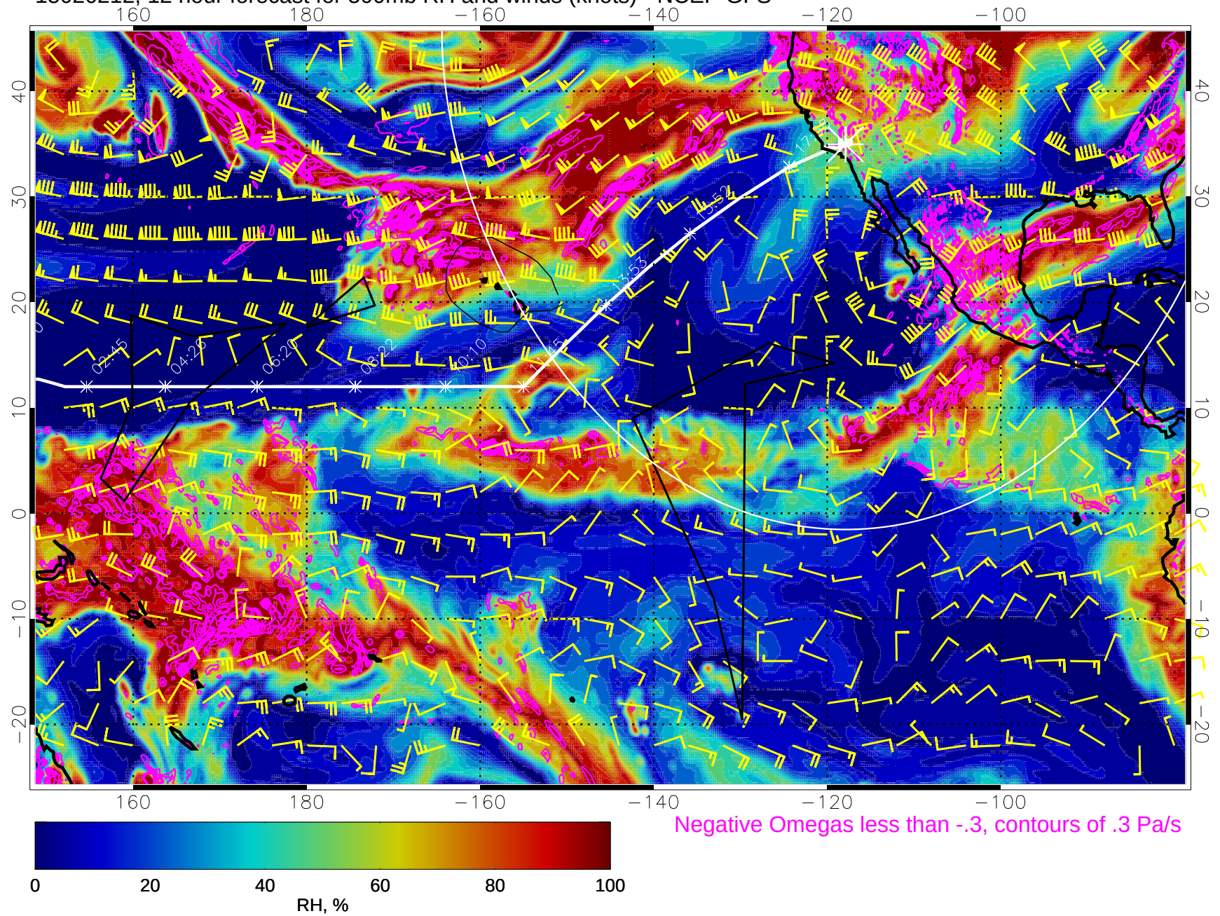
15020212, 12 hour forecast for 500mb RH and winds (knots) - NCEP GFS
