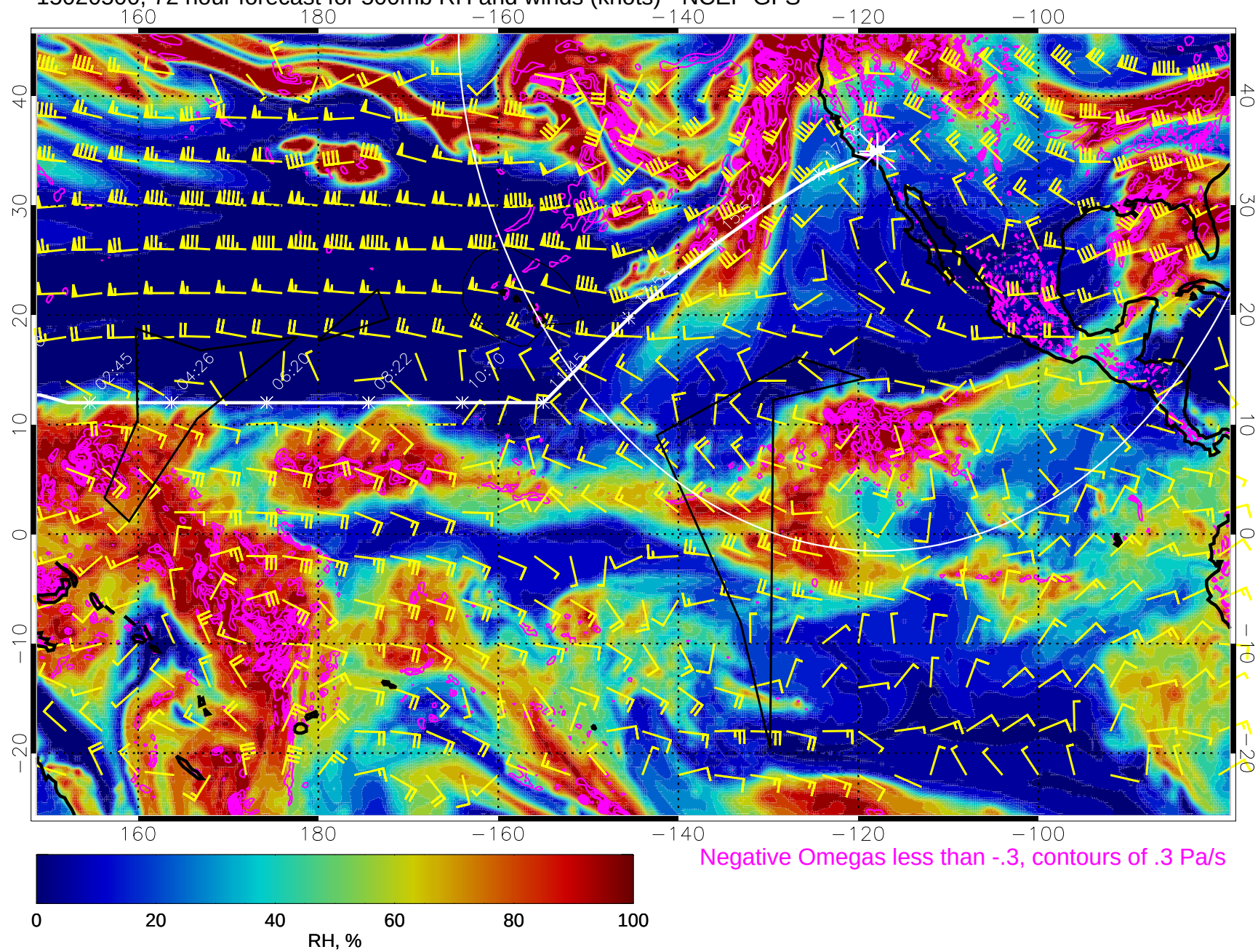
15020500, 72 hour forecast for 500mb RH and winds (knots) - NCEP GFS
