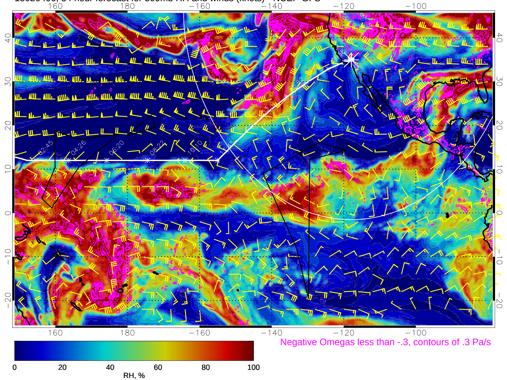
15020406, 54 hour forecast for 500mb RH and winds (knots) - NCEP GFS
