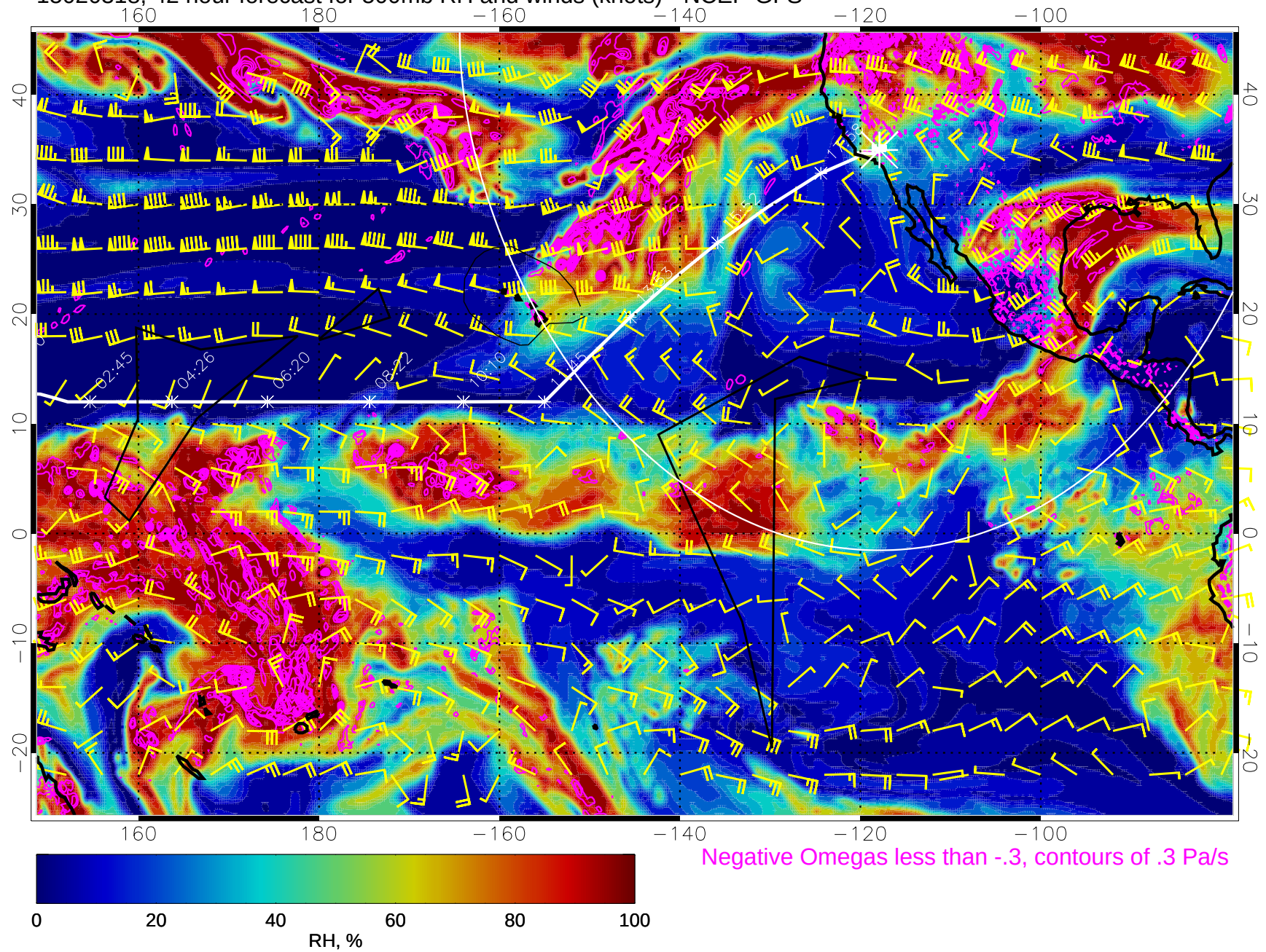
15020318, 42 hour forecast for 500mb RH and winds (knots) - NCEP GFS
