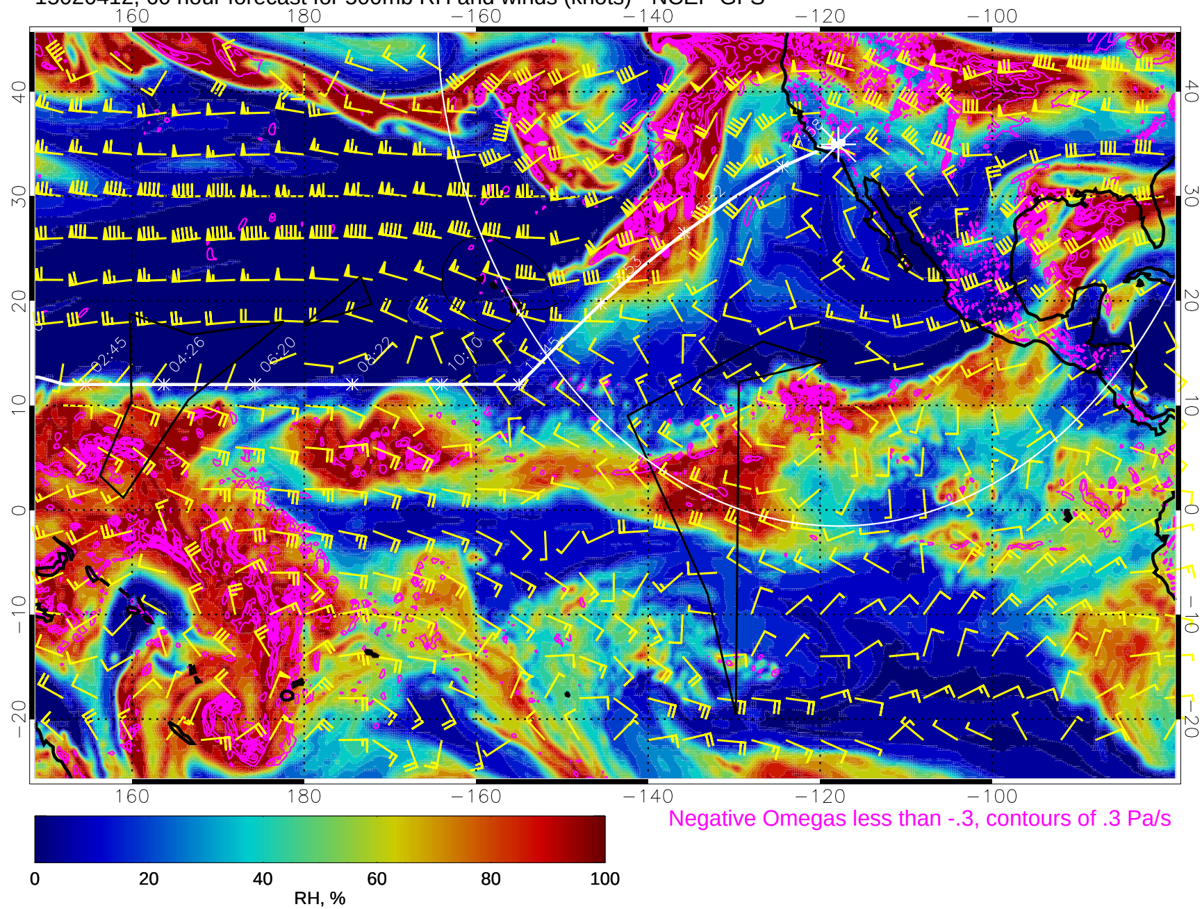
15020412, 60 hour forecast for 500mb RH and winds (knots) - NCEP GFS
