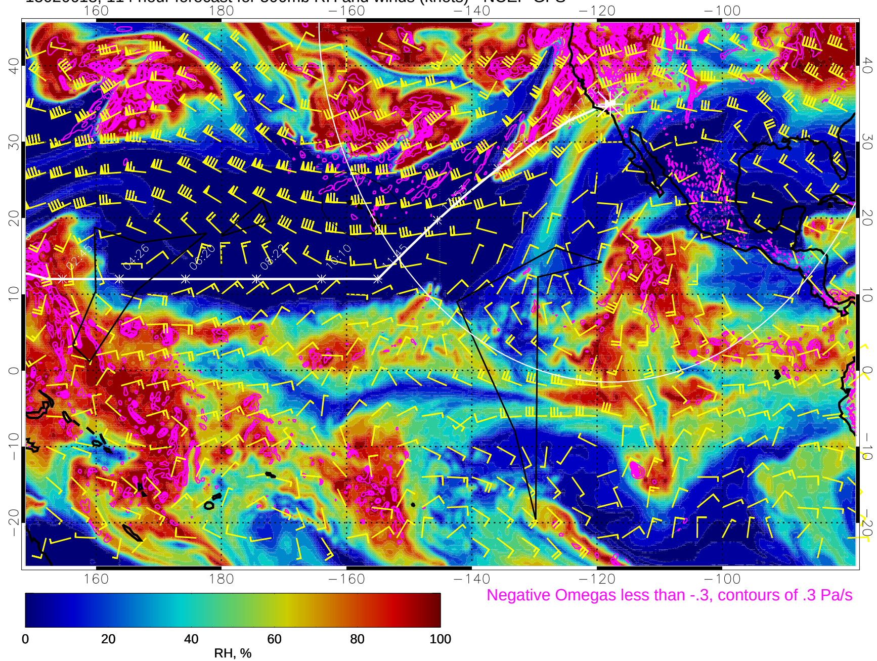
15020618, 114 hour forecast for 500mb RH and winds (knots) - NCEP GFS
