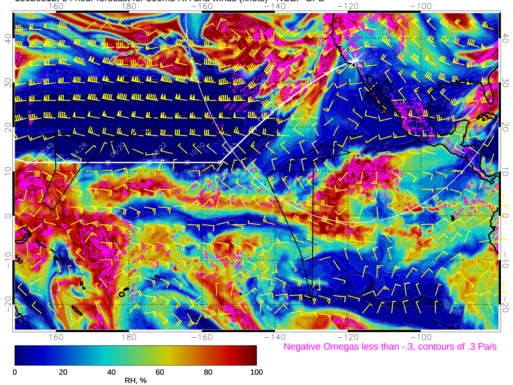
15020512, 84 hour forecast for 500mb RH and winds (knots) - NCEP GFS
