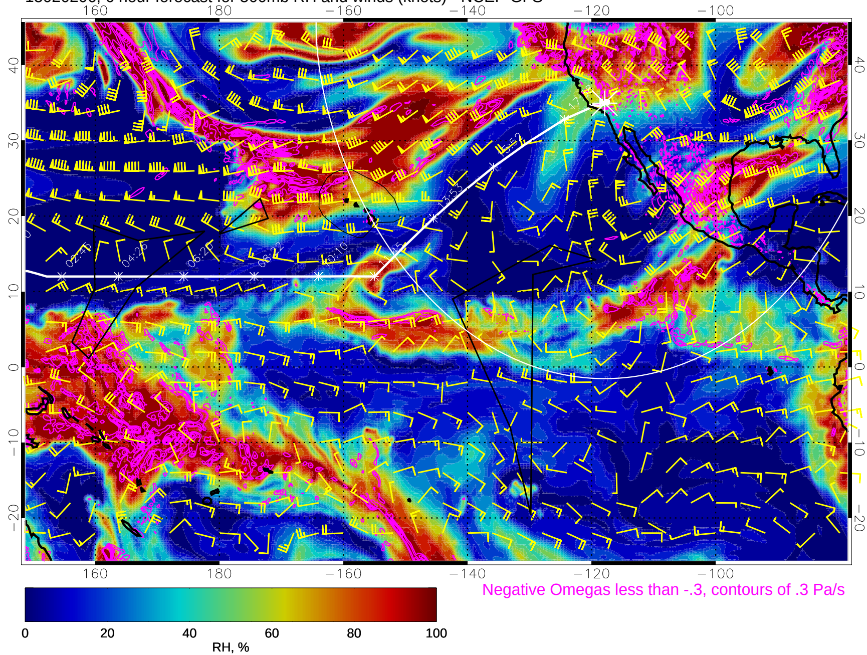
15020206, 6 hour forecast for 500mb RH and winds (knots) - NCEP GFS
