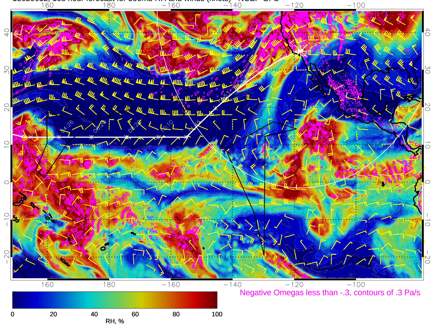
15020612, 108 hour forecast for 500mb RH and winds (knots) - NCEP GFS
