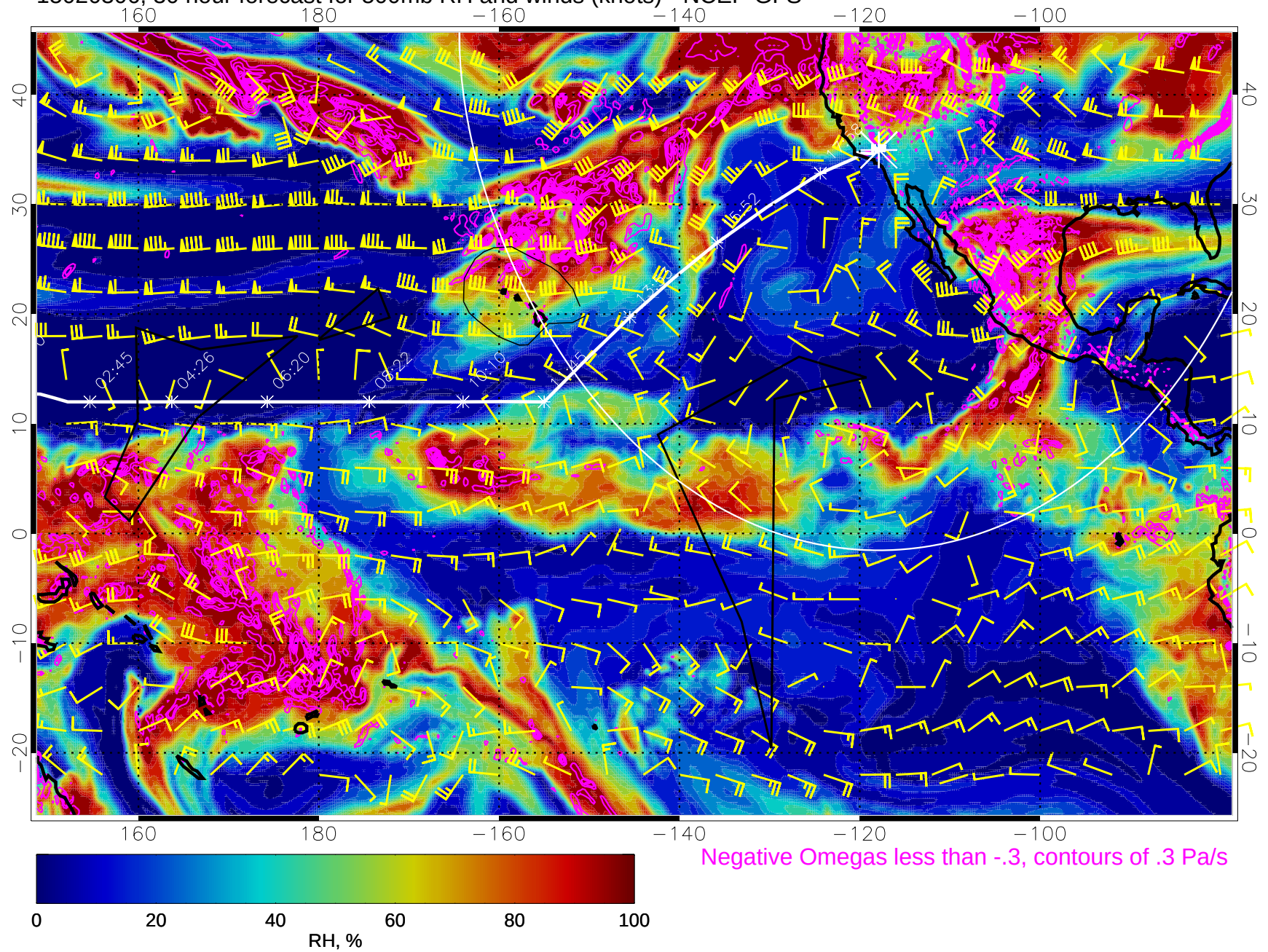
15020306, 30 hour forecast for 500mb RH and winds (knots) - NCEP GFS
