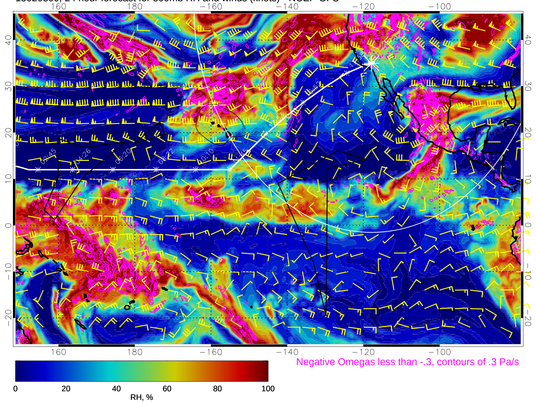
15020300, 24 hour forecast for 500mb RH and winds (knots) - NCEP GFS
