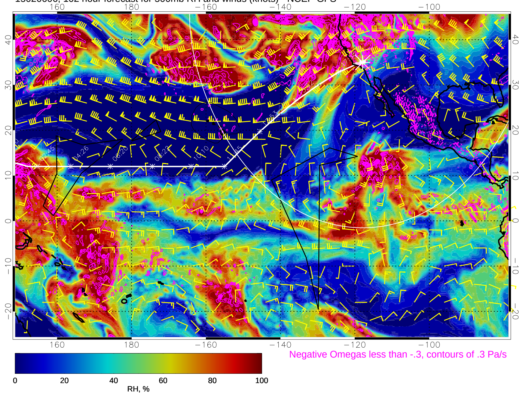
15020606, 102 hour forecast for 500mb RH and winds (knots) - NCEP GFS
