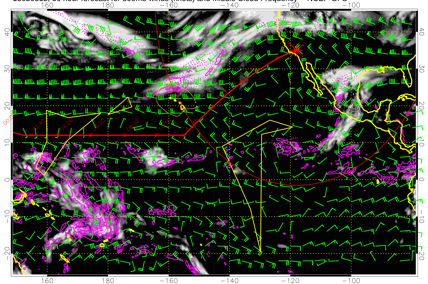
15020312, 36 hour forecast for 500mb winds (knots) and Middle Cloud Frequency -- NCEP GFS
