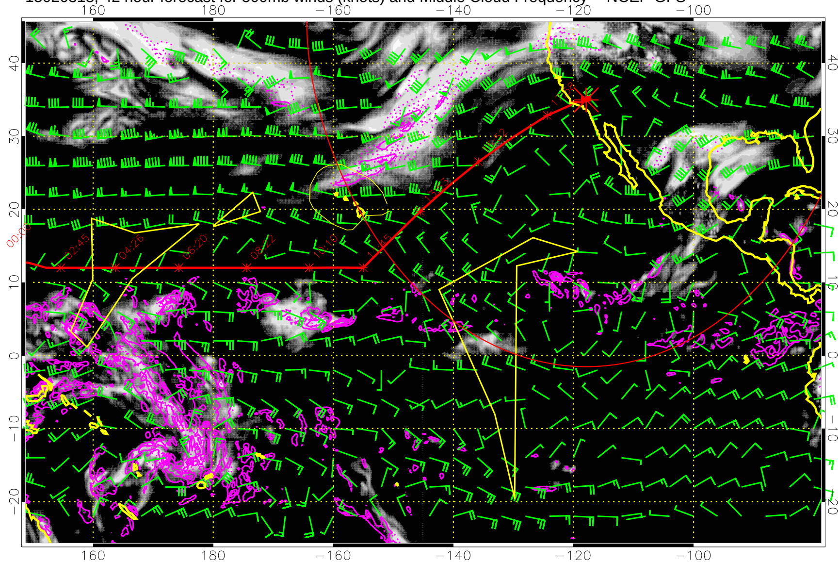
15020318, 42 hour forecast for 500mb winds (knots) and Middle Cloud Frequency -- NCEP GFS
