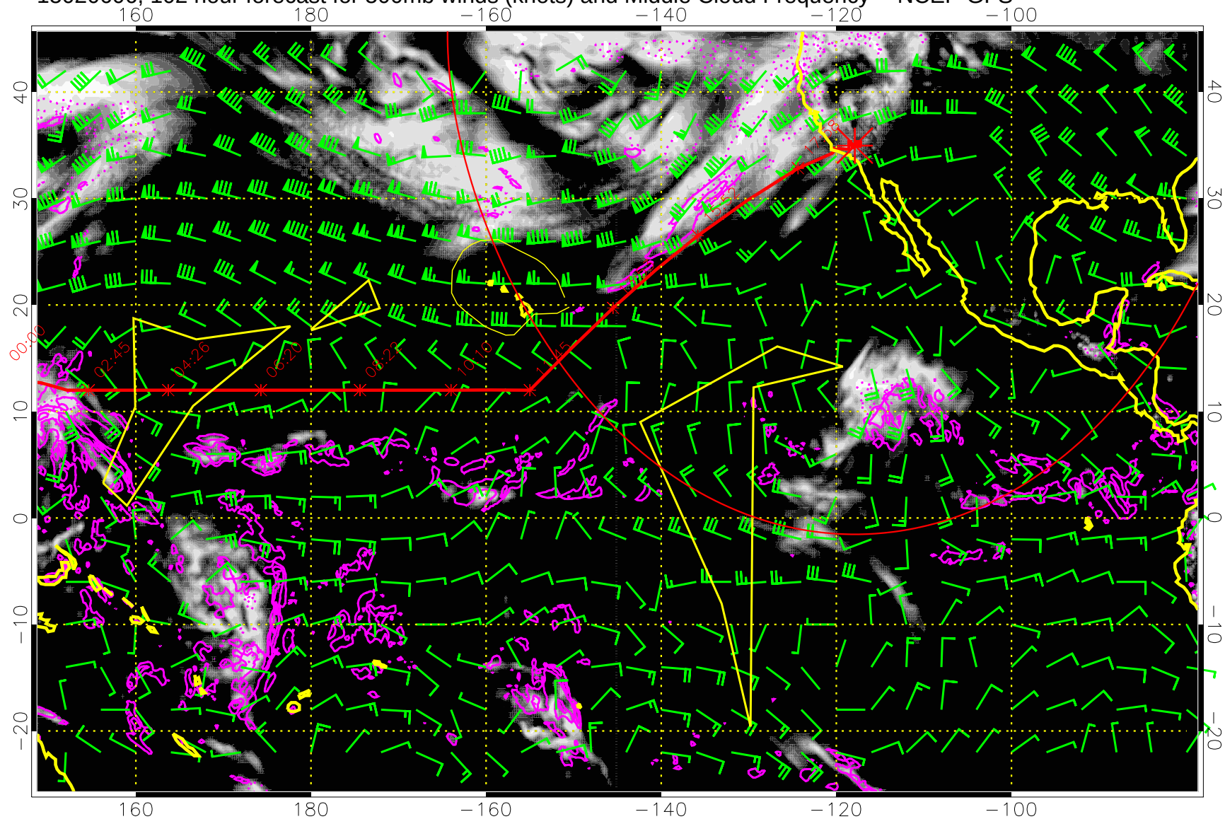
15020606, 102 hour forecast for 500mb winds (knots) and Middle Cloud Frequency -- NCEP GFS
