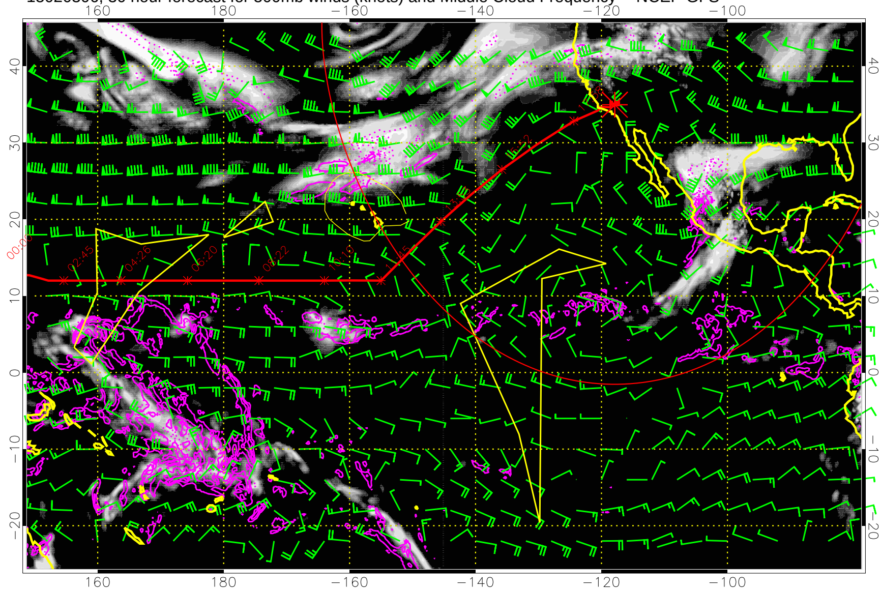
15020306, 30 hour forecast for 500mb winds (knots) and Middle Cloud Frequency -- NCEP GFS
