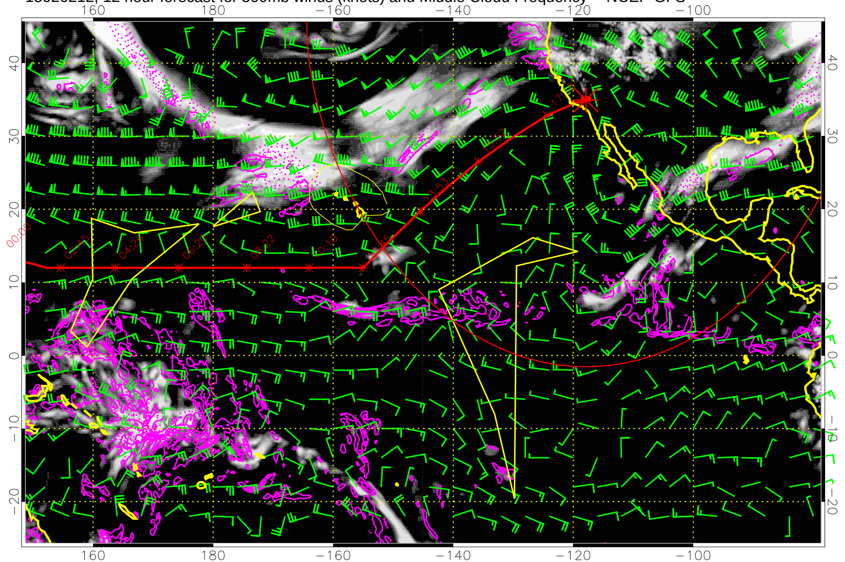
15020212, 12 hour forecast for 500mb winds (knots) and Middle Cloud Frequency -- NCEP GFS
