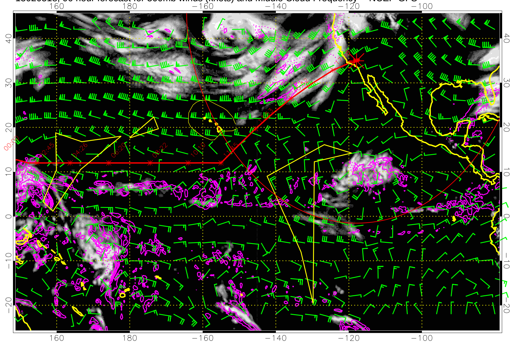
15020518, 90 hour forecast for 500mb winds (knots) and Middle Cloud Frequency -- NCEP GFS
