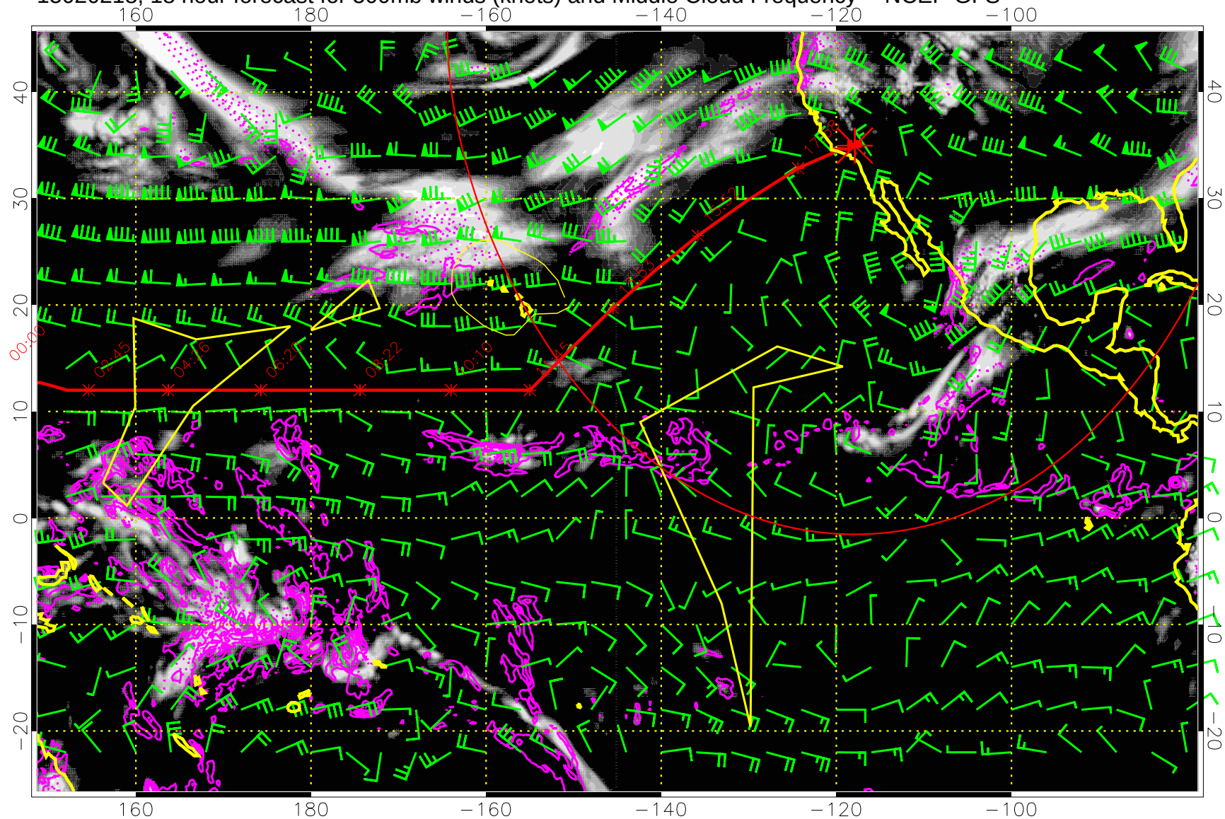
15020218, 18 hour forecast for 500mb winds (knots) and Middle Cloud Frequency -- NCEP GFS
