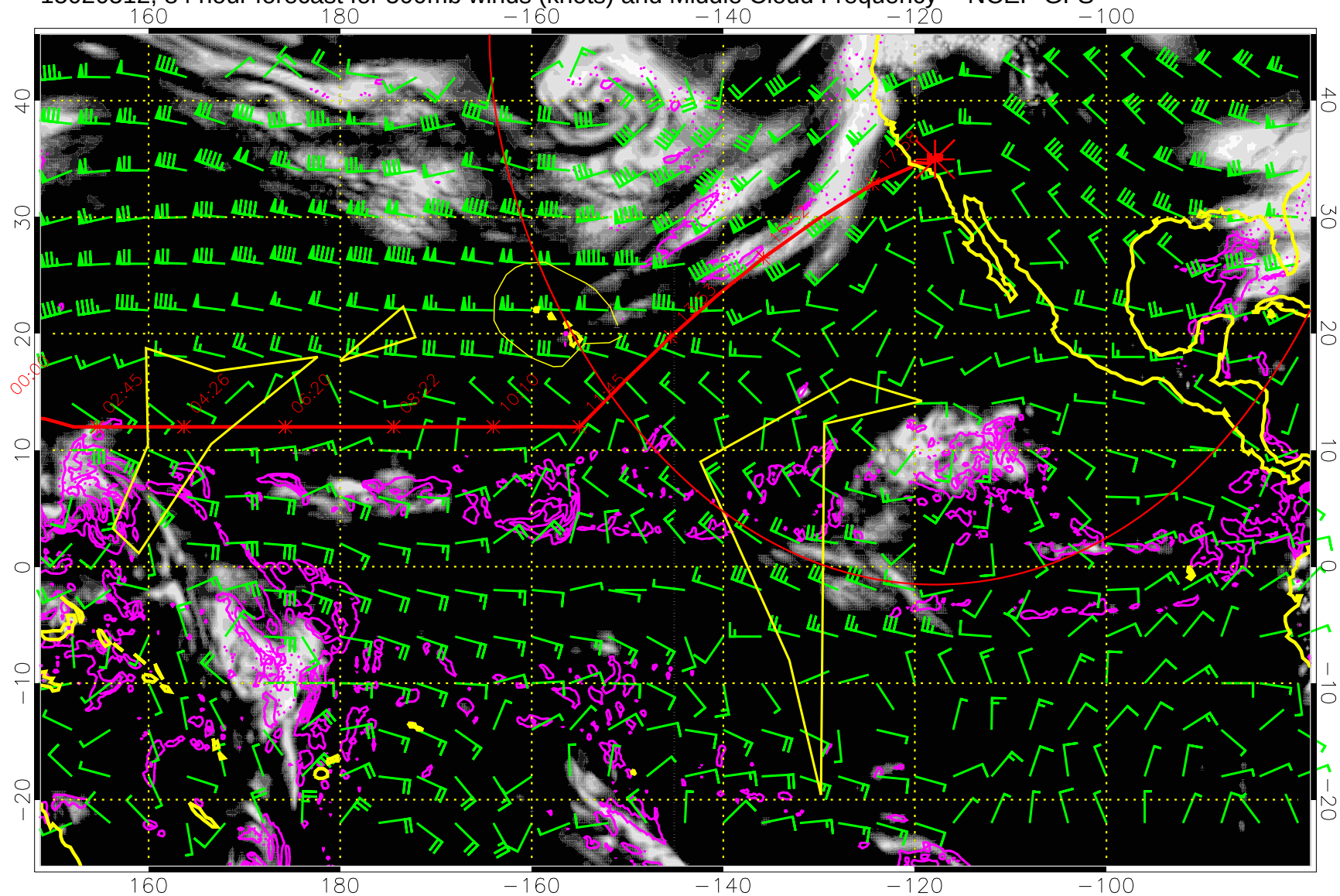
15020512, 84 hour forecast for 500mb winds (knots) and Middle Cloud Frequency -- NCEP GFS
