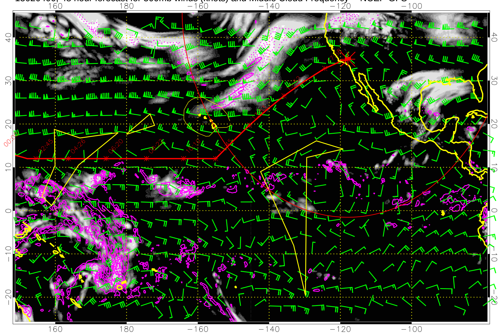
15020400, 48 hour forecast for 500mb winds (knots) and Middle Cloud Frequency -- NCEP GFS
