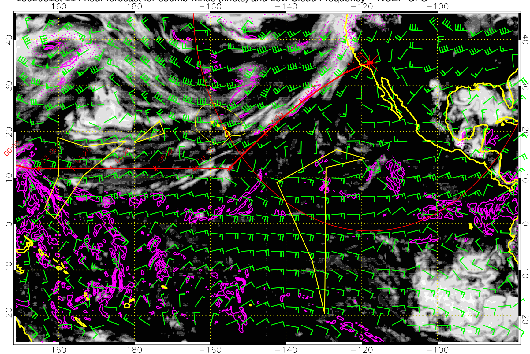
15020618, 114 hour forecast for 850mb winds (knots) and Low Cloud Frequency -- NCEP GFS
