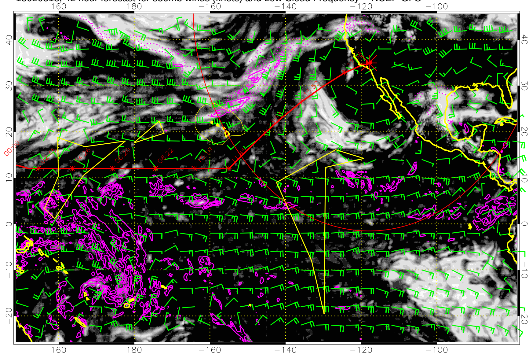
15020318, 42 hour forecast for 850mb winds (knots) and Low Cloud Frequency -- NCEP GFS
