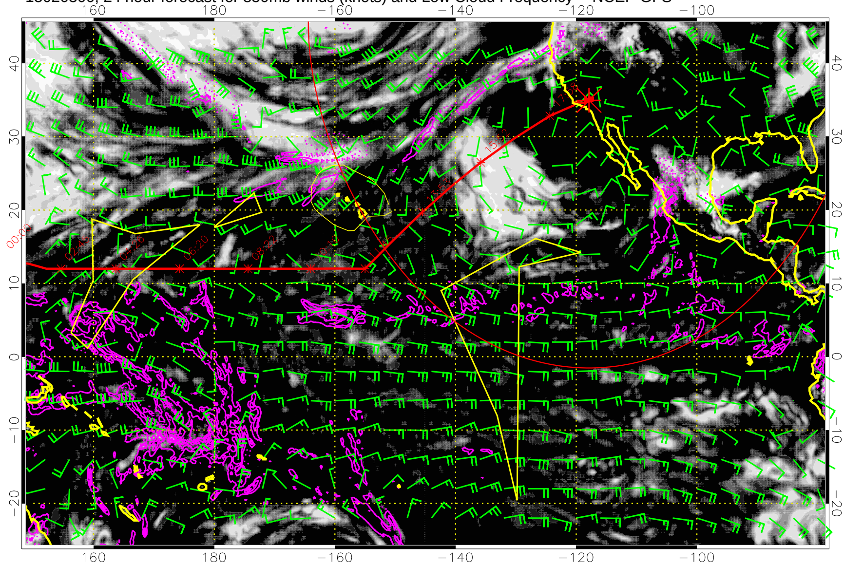
15020300, 24 hour forecast for 850mb winds (knots) and Low Cloud Frequency -- NCEP GFS
