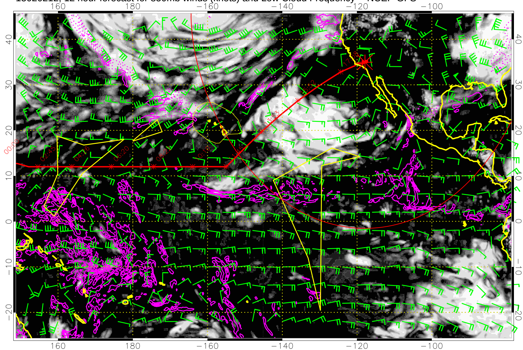
15020212, 12 hour forecast for 850mb winds (knots) and Low Cloud Frequency -- NCEP GFS
