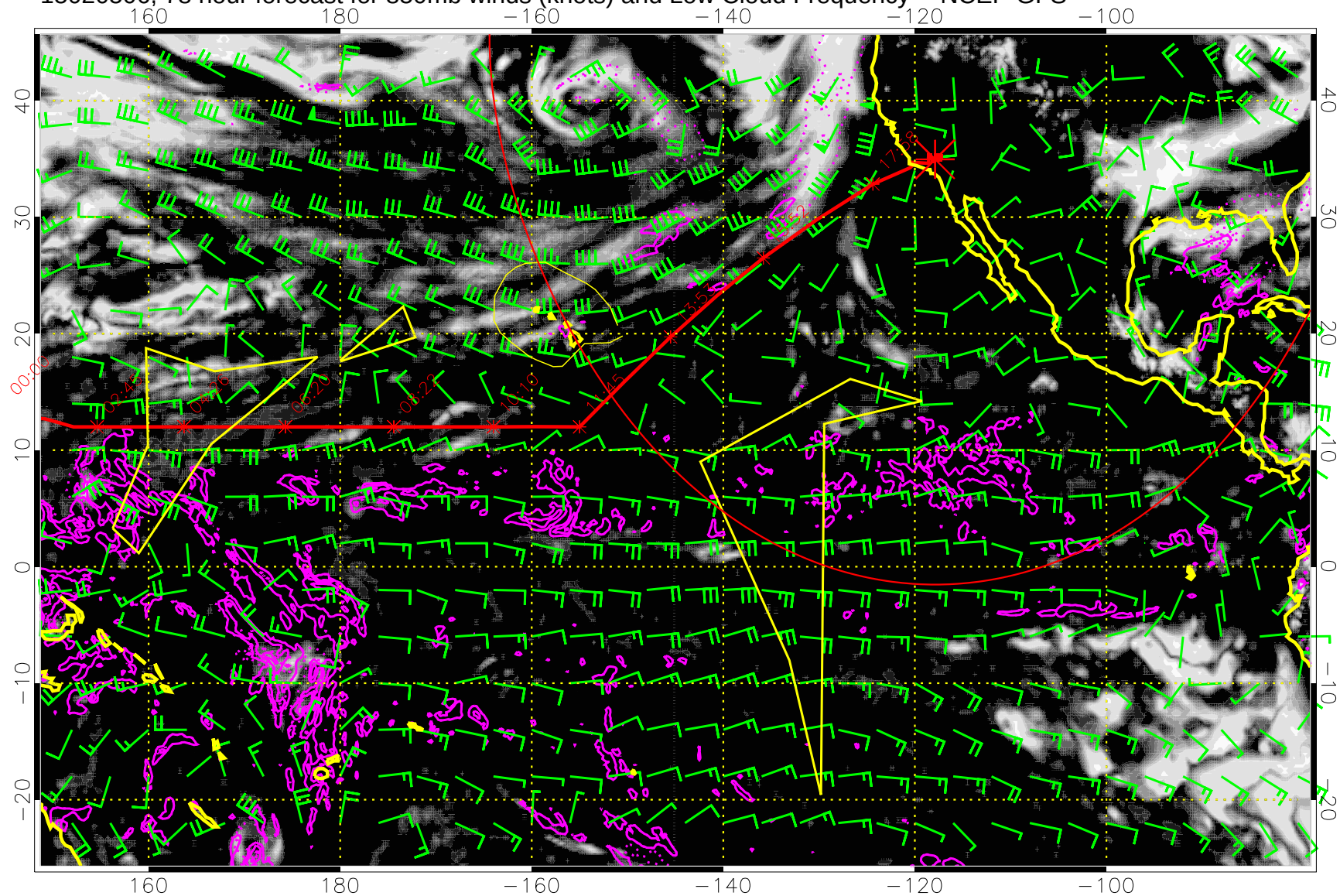
15020506, 78 hour forecast for 850mb winds (knots) and Low Cloud Frequency -- NCEP GFS
