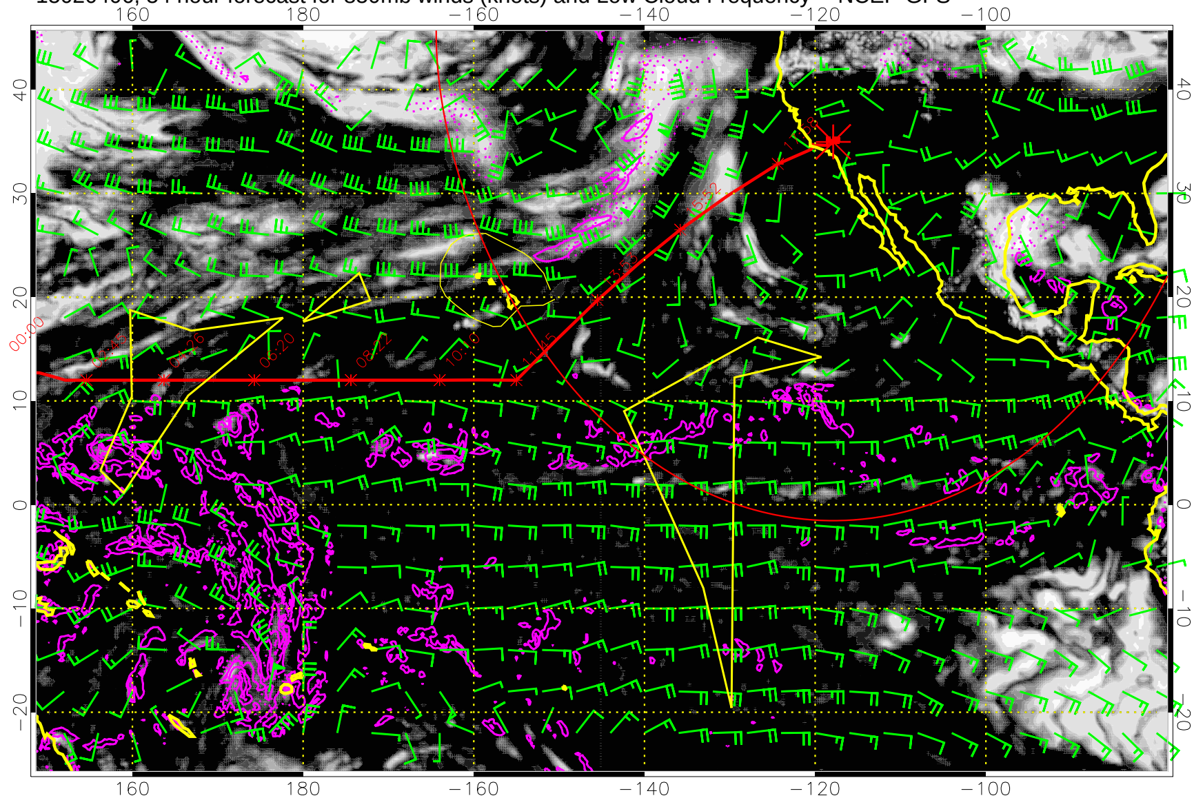
15020406, 54 hour forecast for 850mb winds (knots) and Low Cloud Frequency -- NCEP GFS
