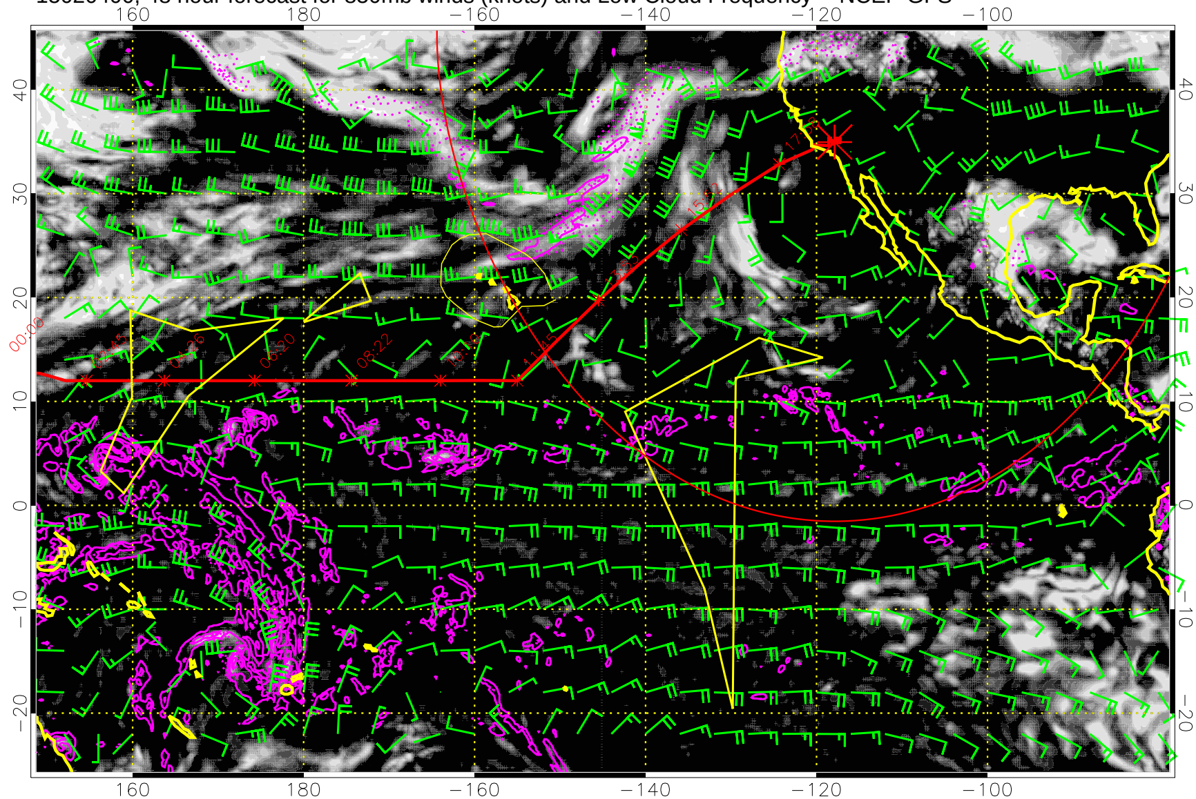
15020400, 48 hour forecast for 850mb winds (knots) and Low Cloud Frequency -- NCEP GFS
