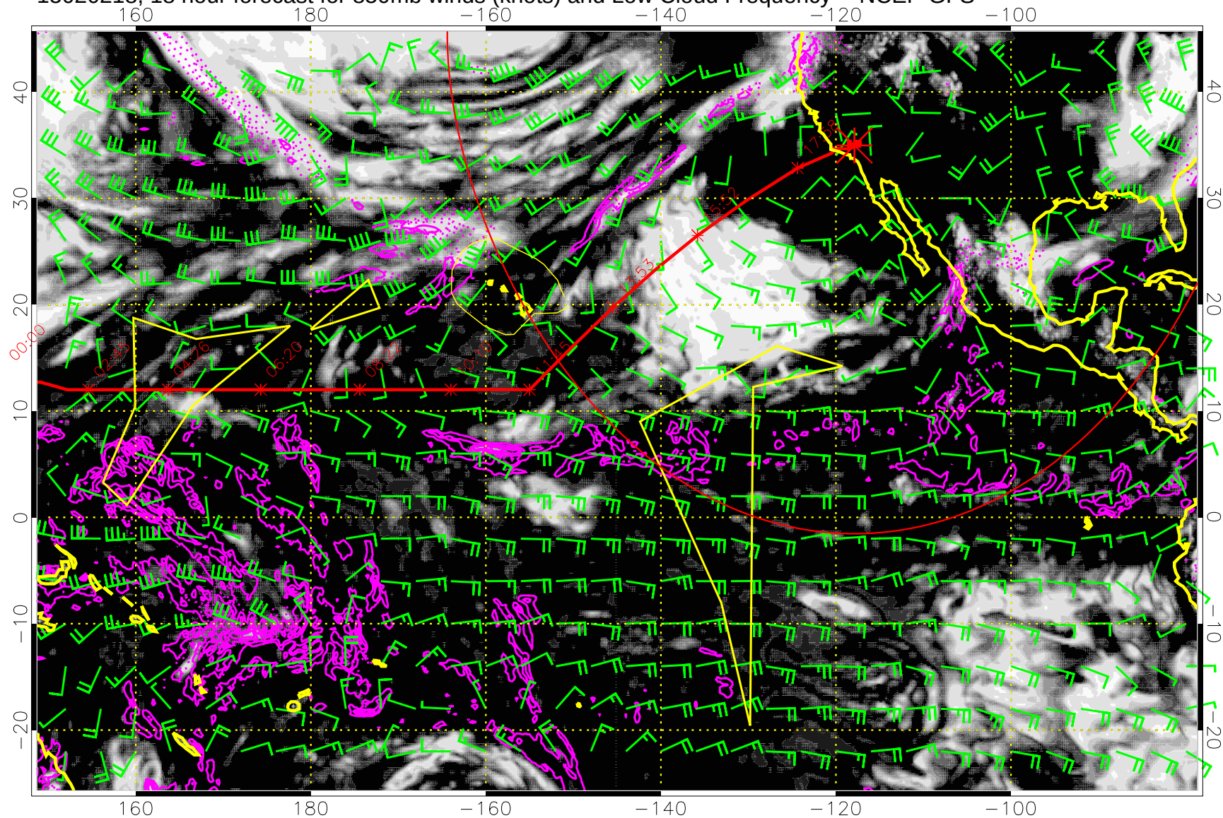
15020218, 18 hour forecast for 850mb winds (knots) and Low Cloud Frequency -- NCEP GFS
