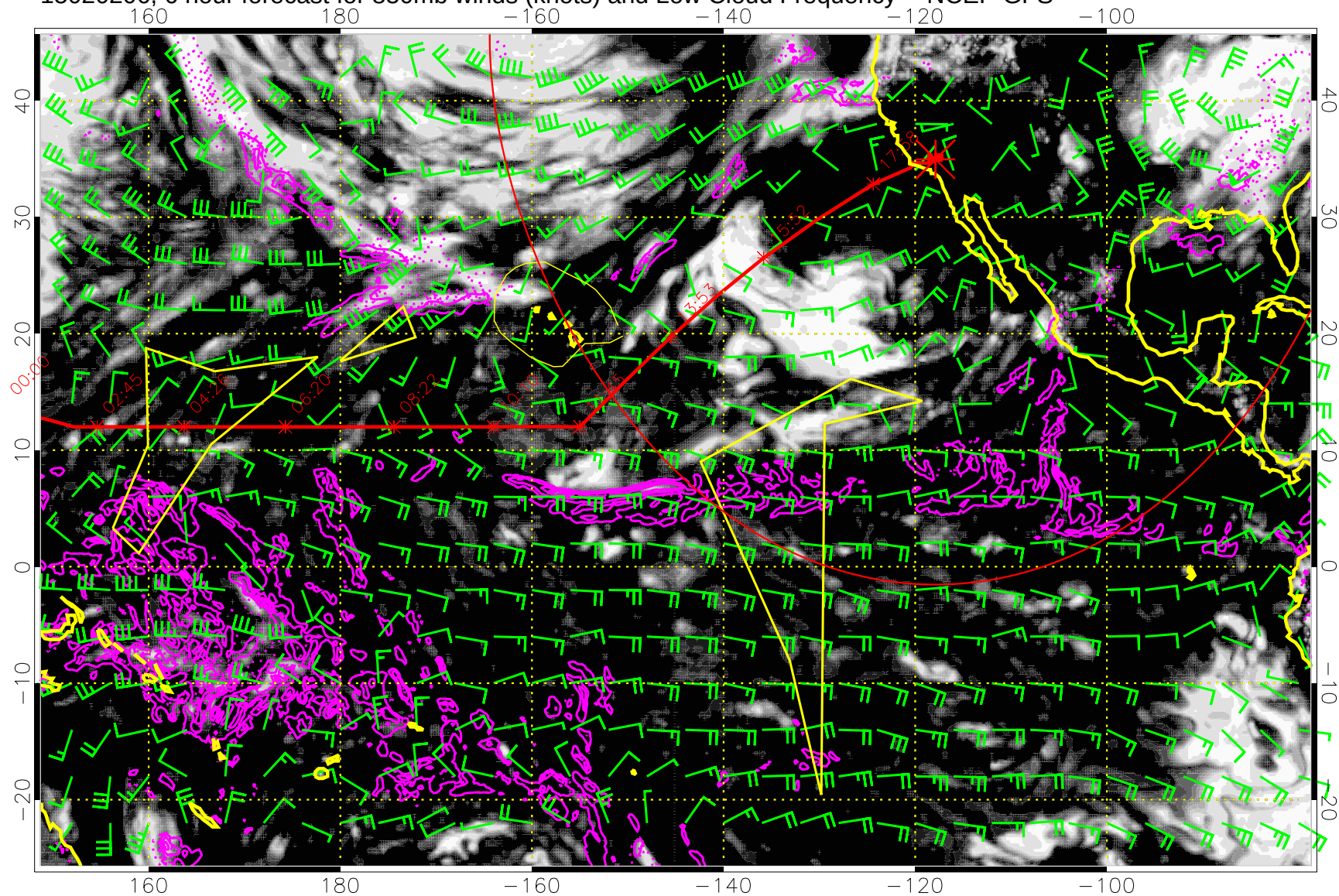
15020206, 6 hour forecast for 850mb winds (knots) and Low Cloud Frequency -- NCEP GFS
