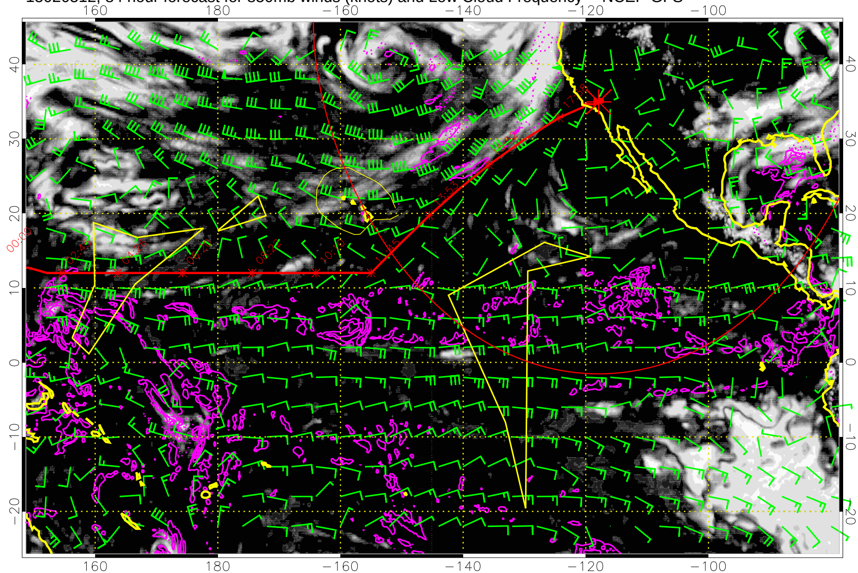
15020512, 84 hour forecast for 850mb winds (knots) and Low Cloud Frequency -- NCEP GFS
