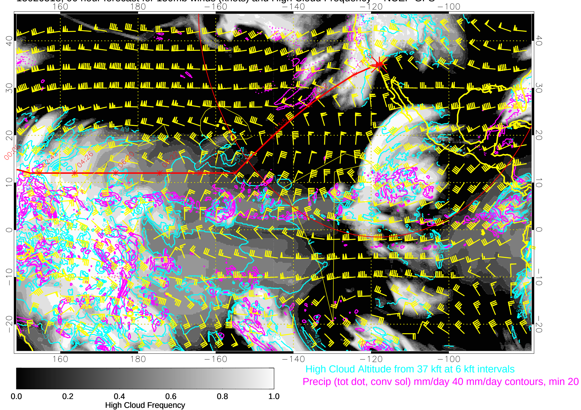
15020518, 90 hour forecast for 150mb winds (knots) and High Cloud Frequency -- NCEP GFS
