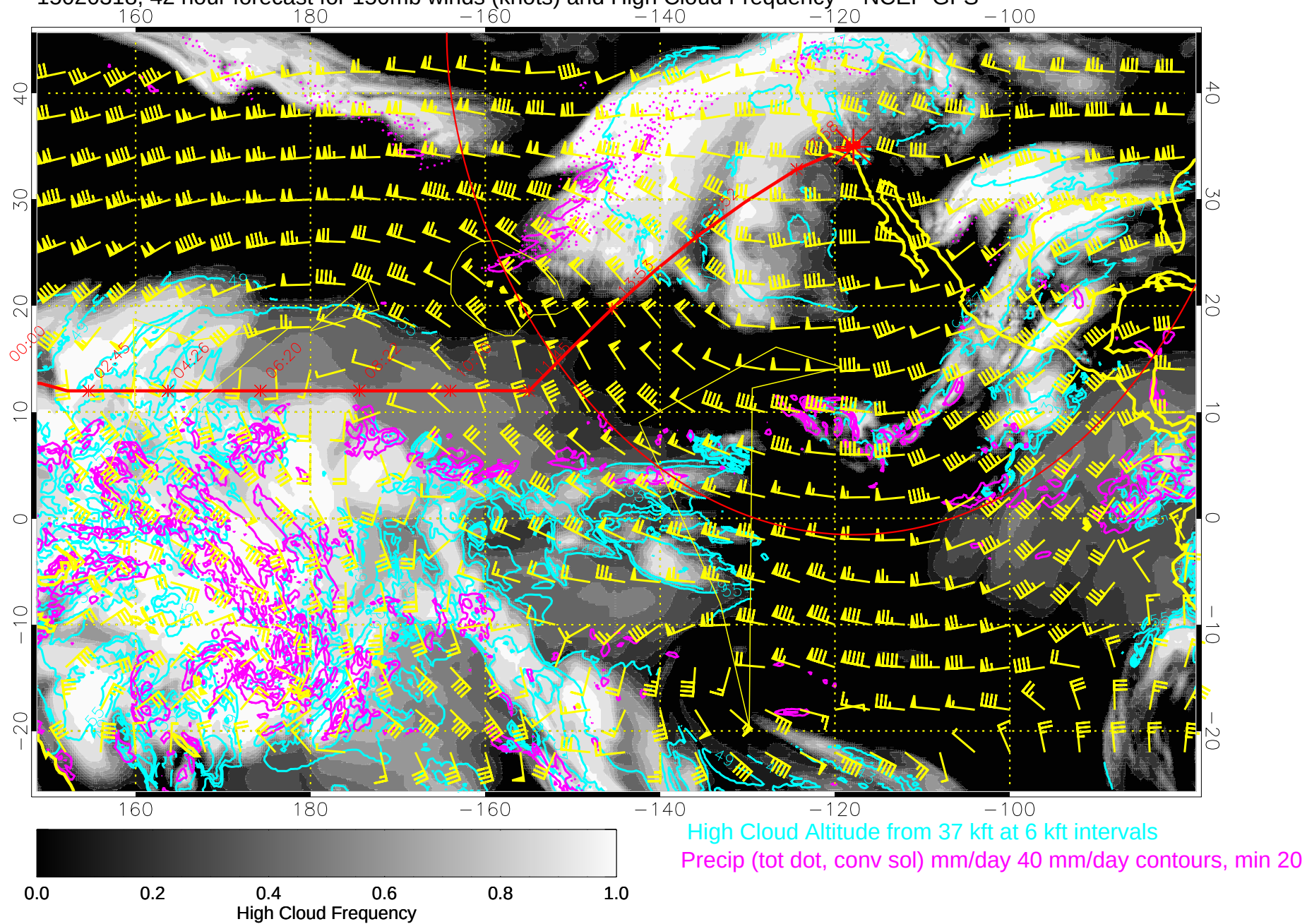
15020318, 42 hour forecast for 150mb winds (knots) and High Cloud Frequency -- NCEP GFS
