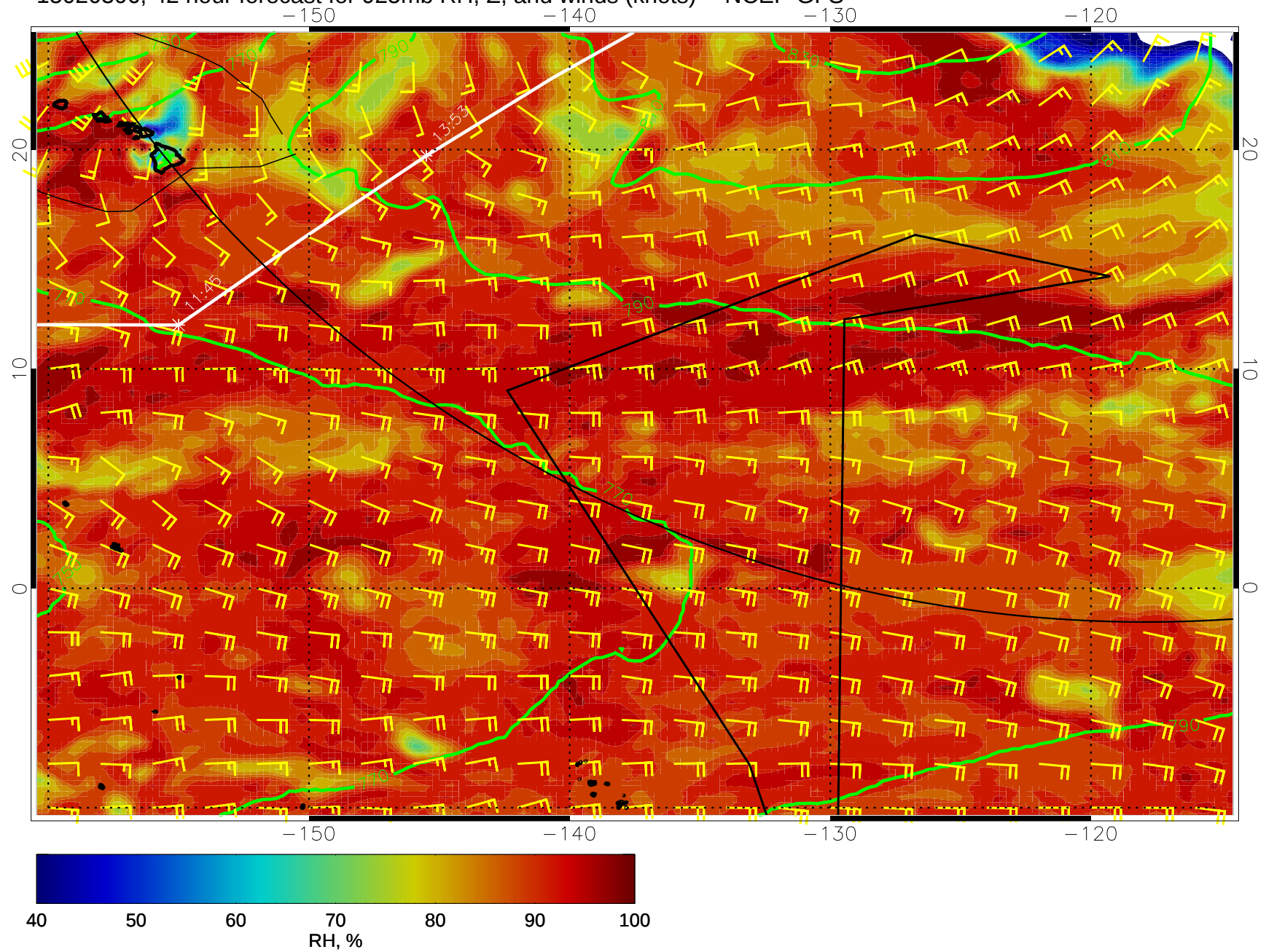
15020306, 42 hour forecast for 925mb RH, Z, and winds (knots) -- NCEP GFS
