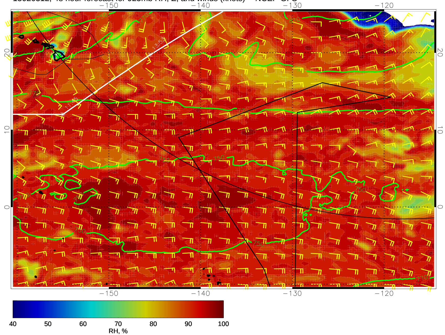
15020312, 48 hour forecast for 925mb RH, Z, and winds (knots) -- NCEP GFS
