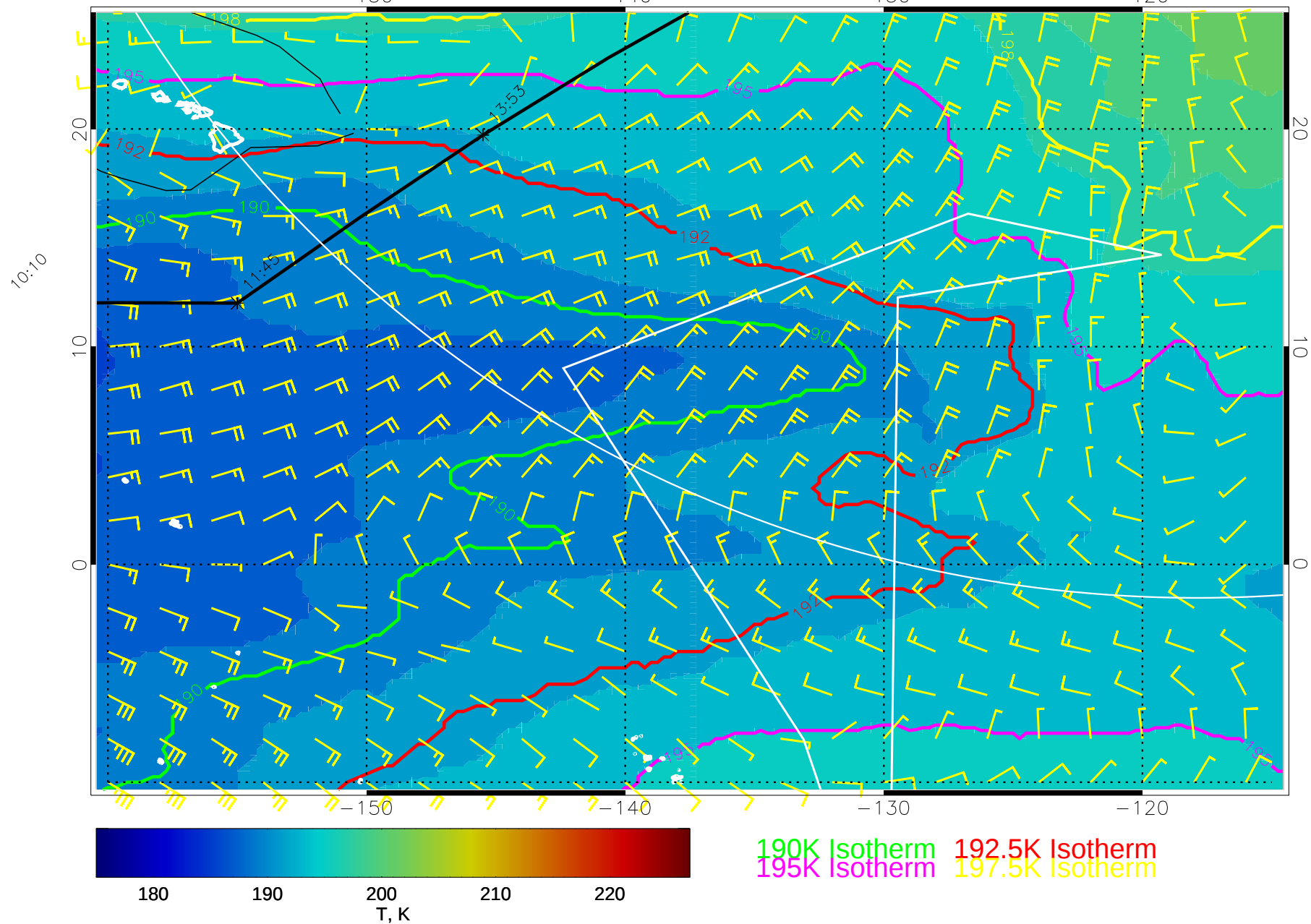
15020518, 102 hour forecast for 70mb T and winds (knots) -- NCEP GFS
