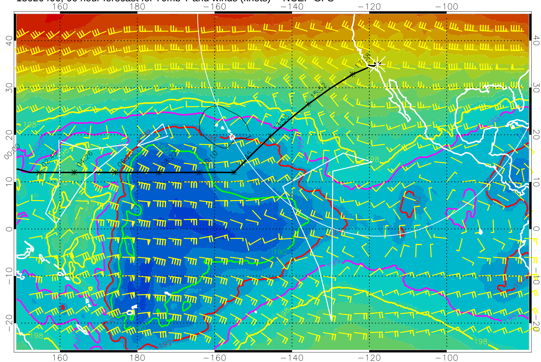
15020406, 66 hour forecast for 70mb T and winds (knots) -- NCEP GFS
