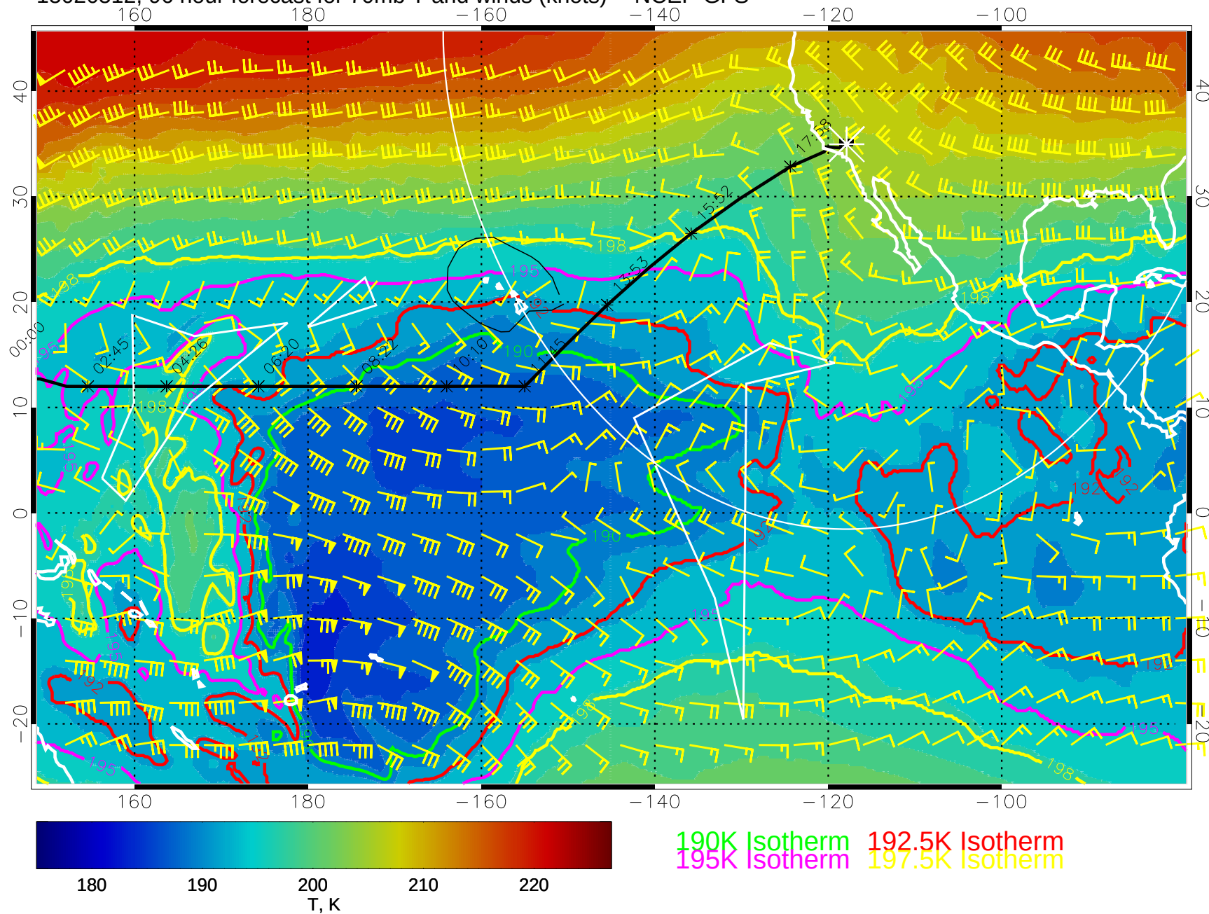
15020512, 96 hour forecast for 70mb T and winds (knots) -- NCEP GFS
