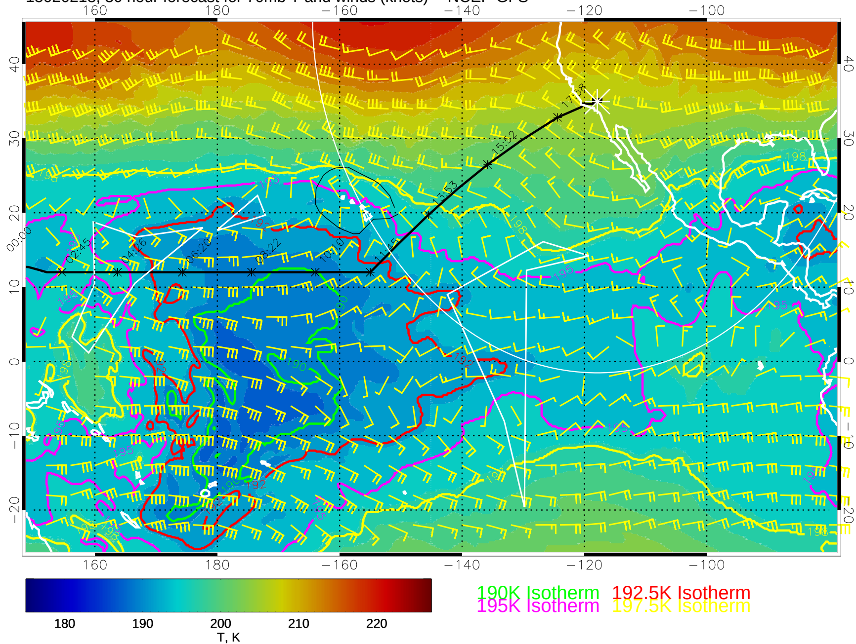
15020218, 30 hour forecast for 70mb T and winds (knots) -- NCEP GFS
