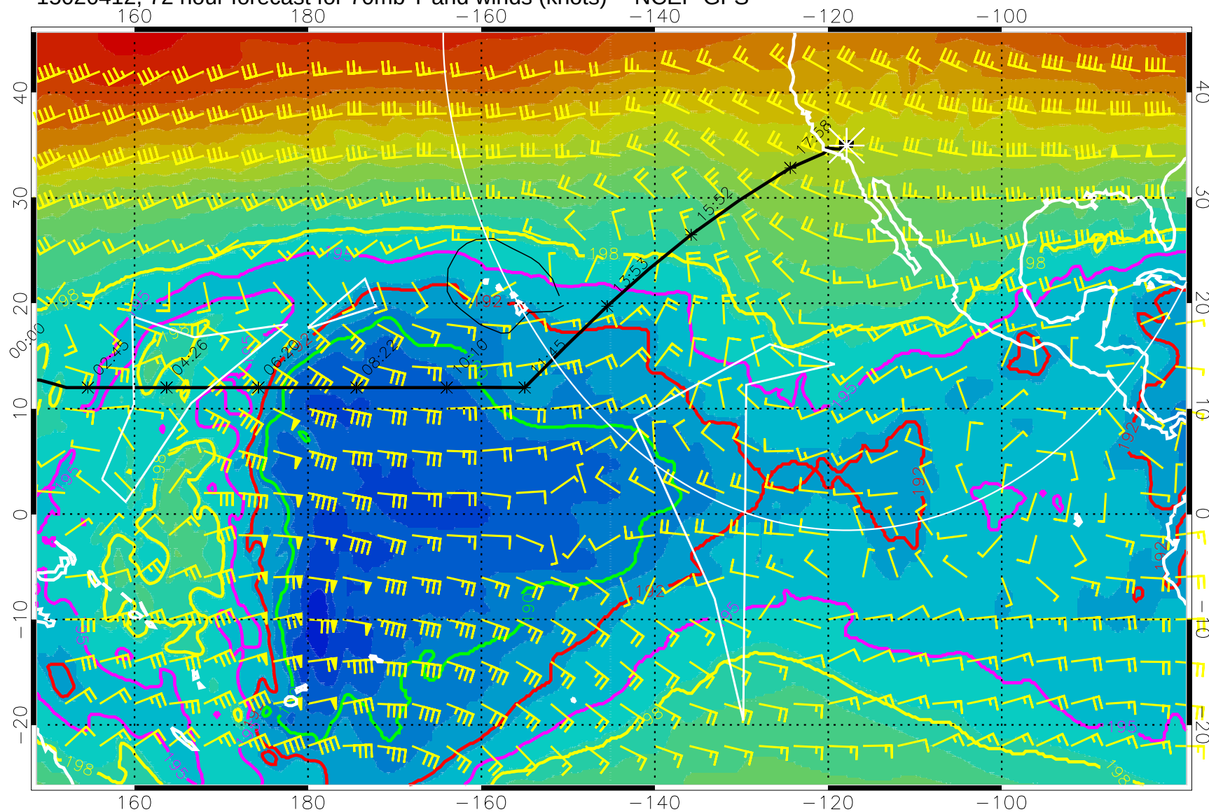
15020412, 72 hour forecast for 70mb T and winds (knots) -- NCEP GFS
