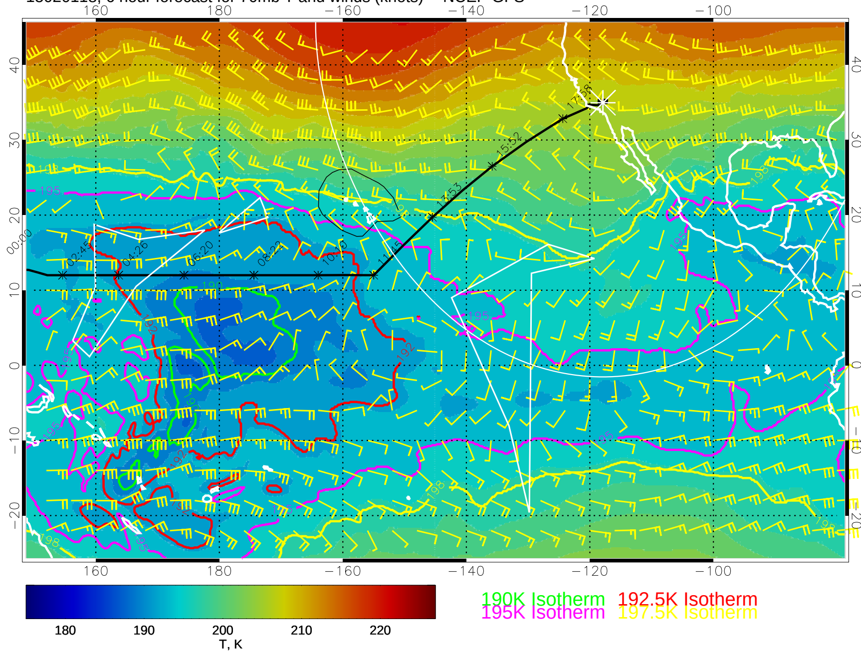
15020118, 6 hour forecast for 70mb T and winds (knots) -- NCEP GFS
