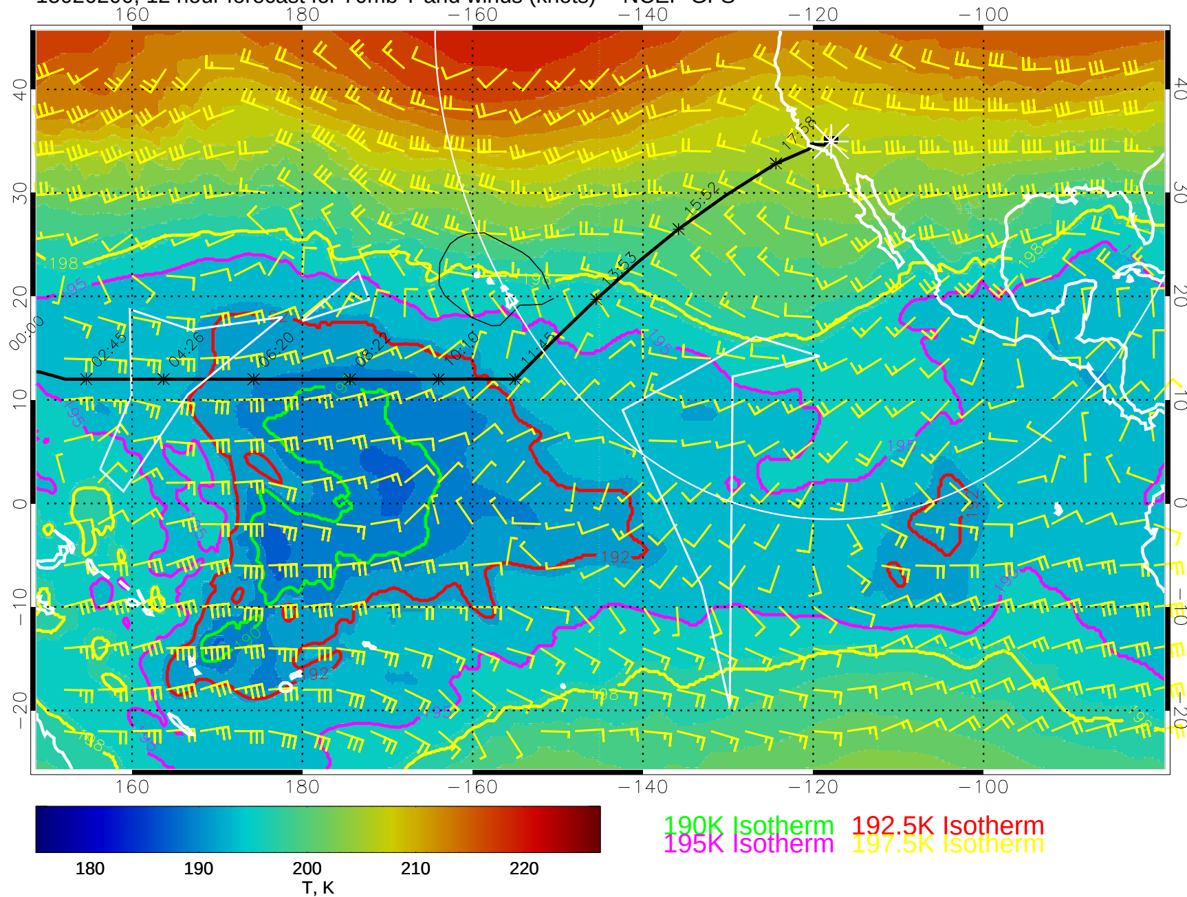
15020200, 12 hour forecast for 70mb T and winds (knots) -- NCEP GFS
