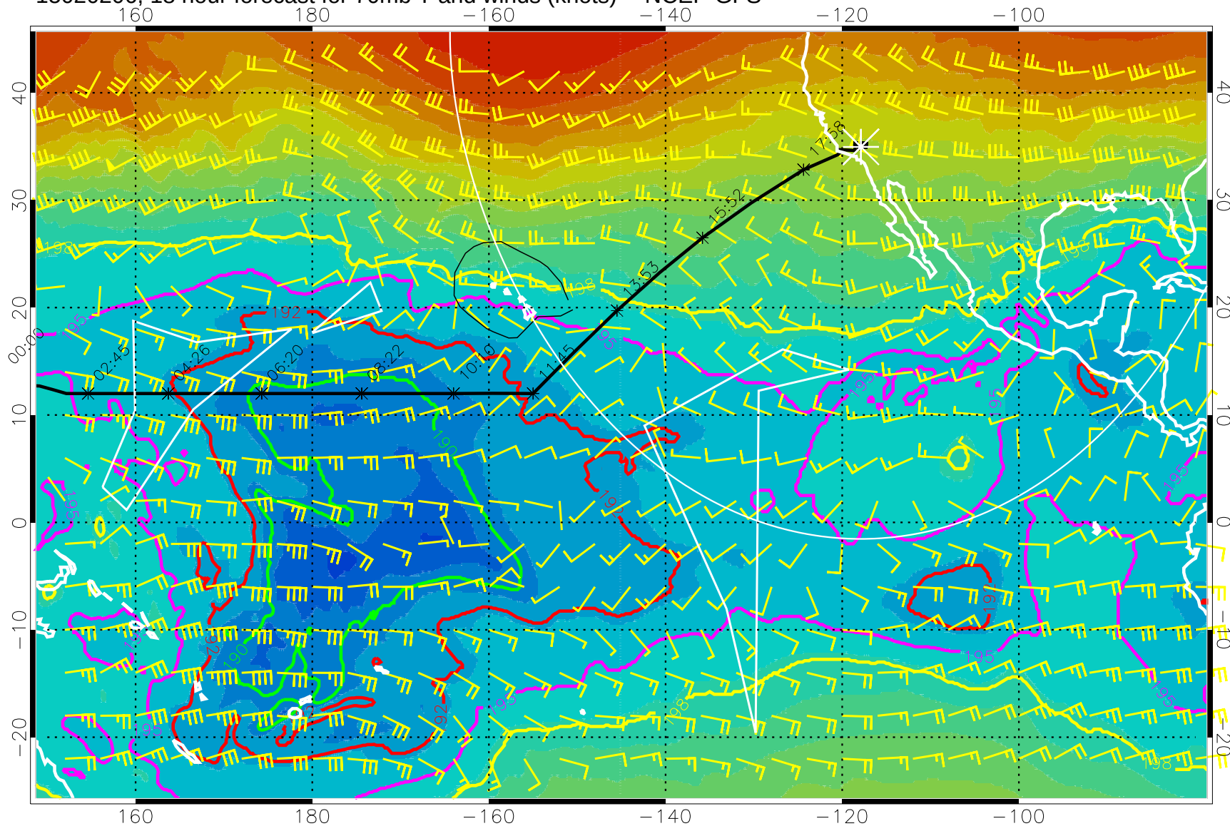
15020206, 18 hour forecast for 70mb T and winds (knots) -- NCEP GFS
