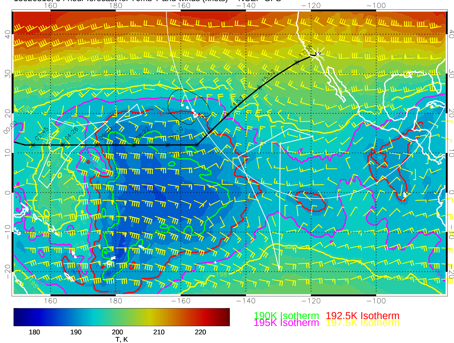
15020318, 54 hour forecast for 70mb T and winds (knots) -- NCEP GFS
