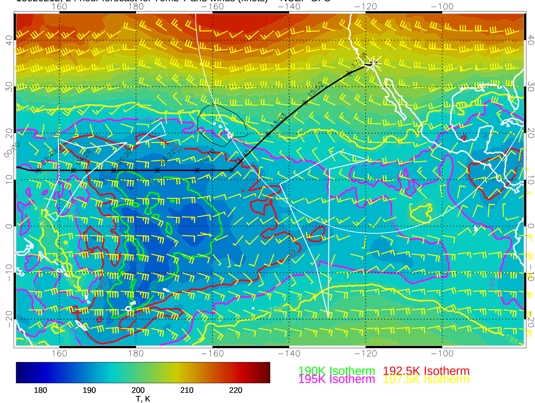
15020212, 24 hour forecast for 70mb T and winds (knots) -- NCEP GFS
