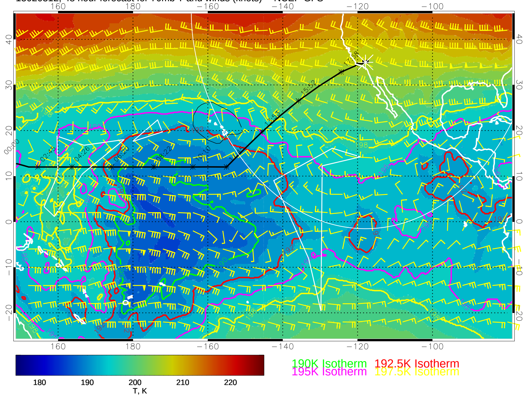
15020312, 48 hour forecast for 70mb T and winds (knots) -- NCEP GFS
