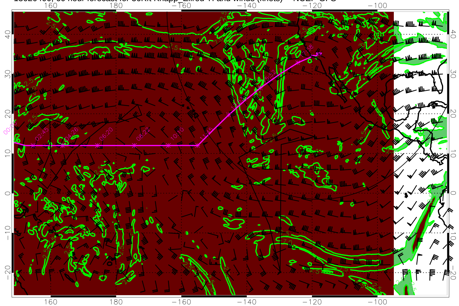
15020400, 60 hour forecast for 36Kft Knapp_Ellrod TI and winds (knots) -- NCEP GFS
