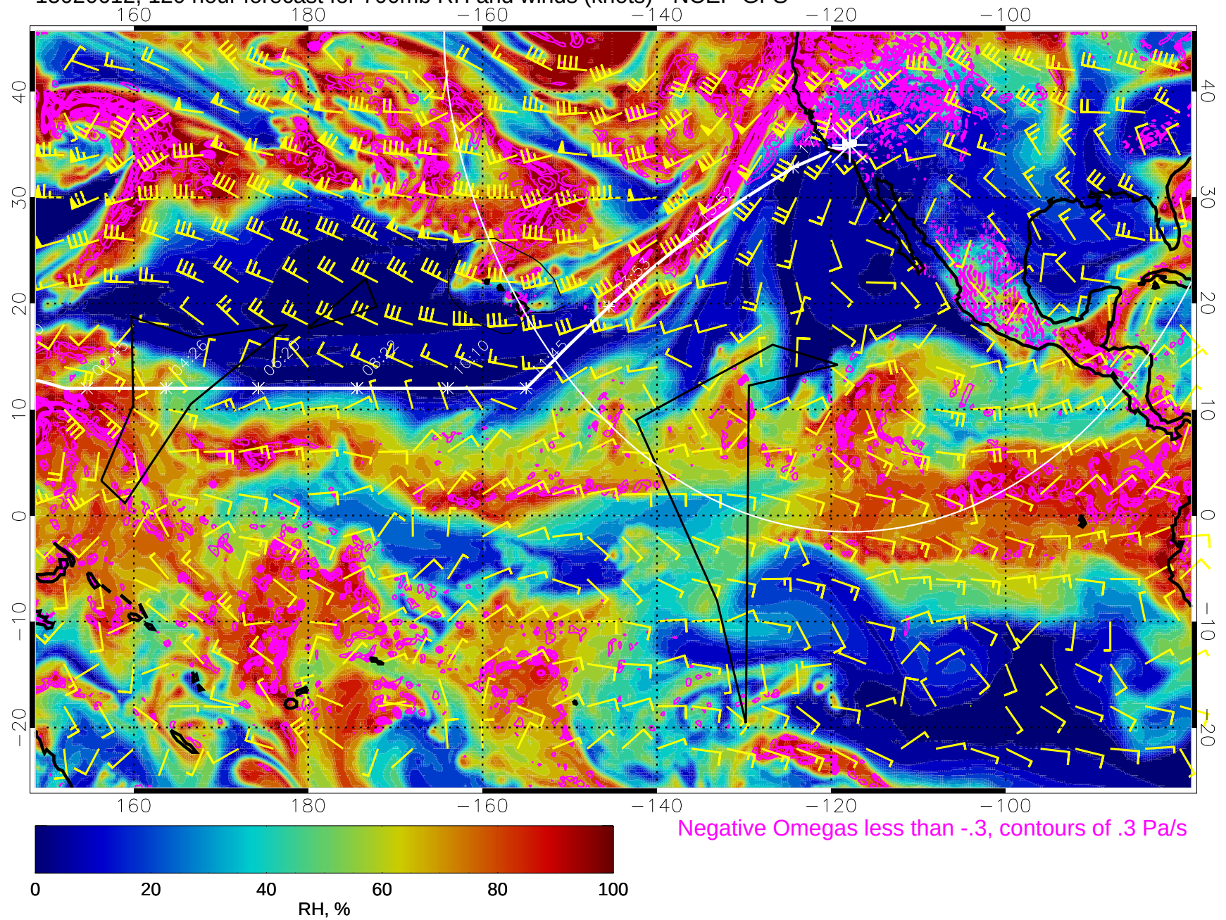
15020612, 120 hour forecast for 700mb RH and winds (knots) - NCEP GFS
