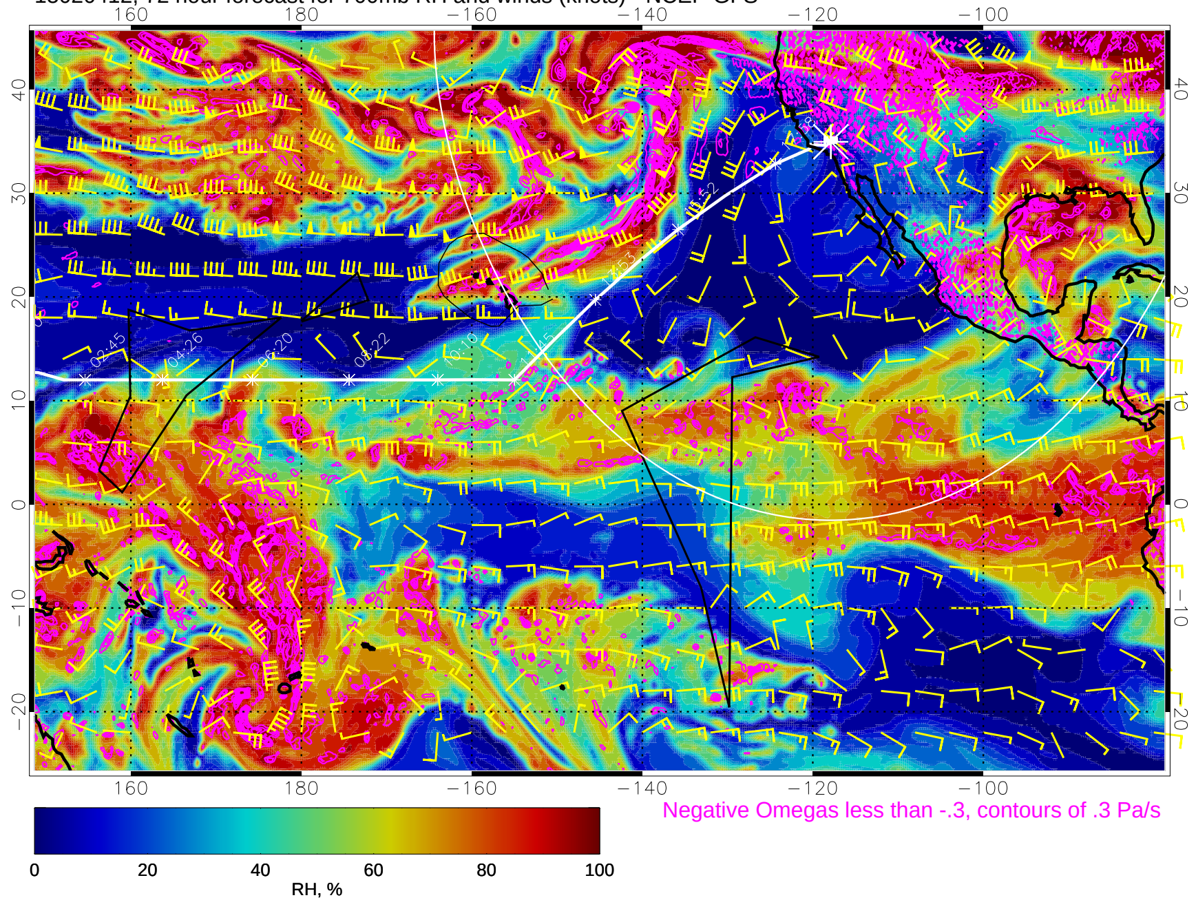
15020412, 72 hour forecast for 700mb RH and winds (knots) - NCEP GFS
