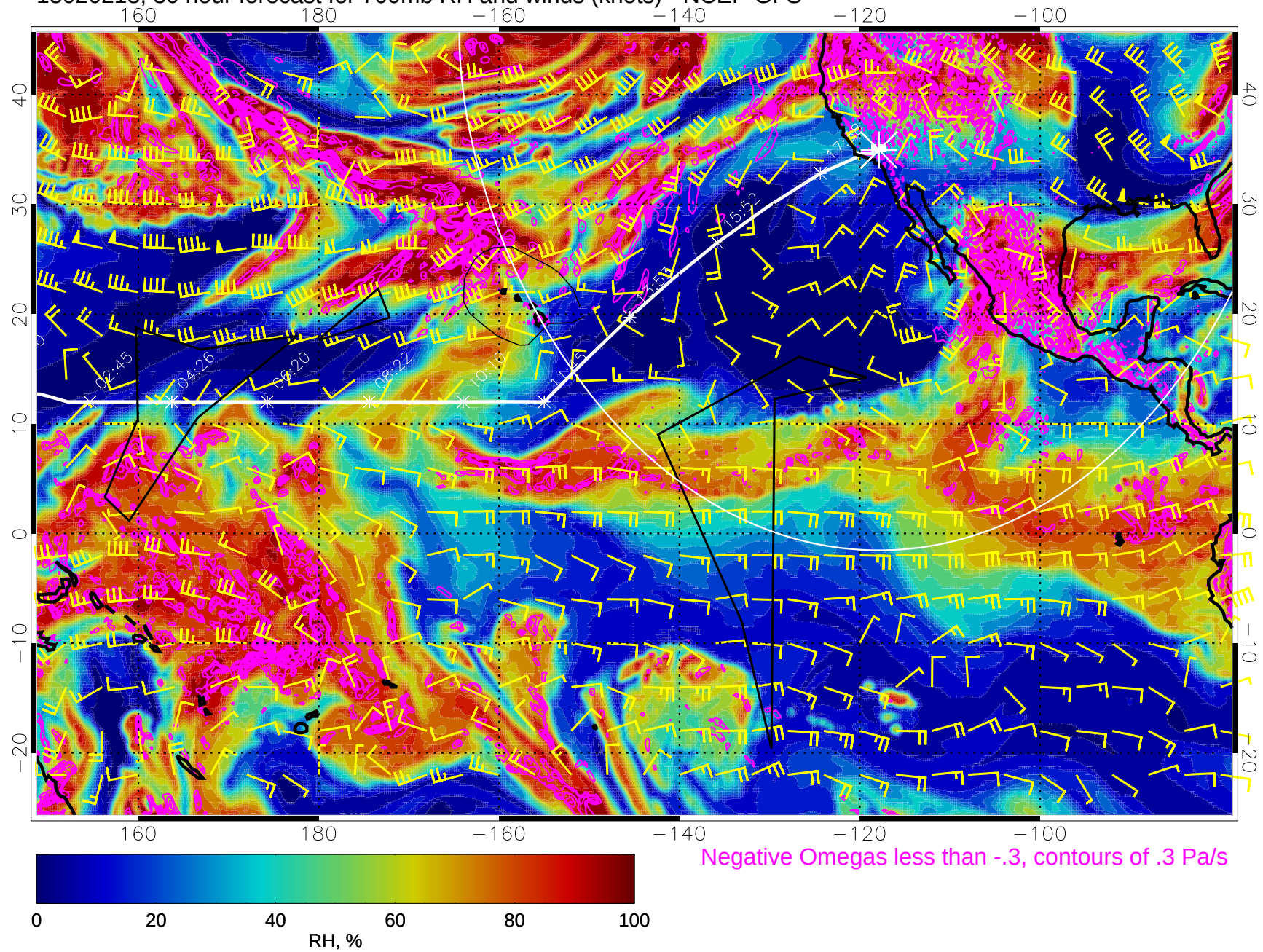
15020218, 30 hour forecast for 700mb RH and winds (knots) - NCEP GFS
