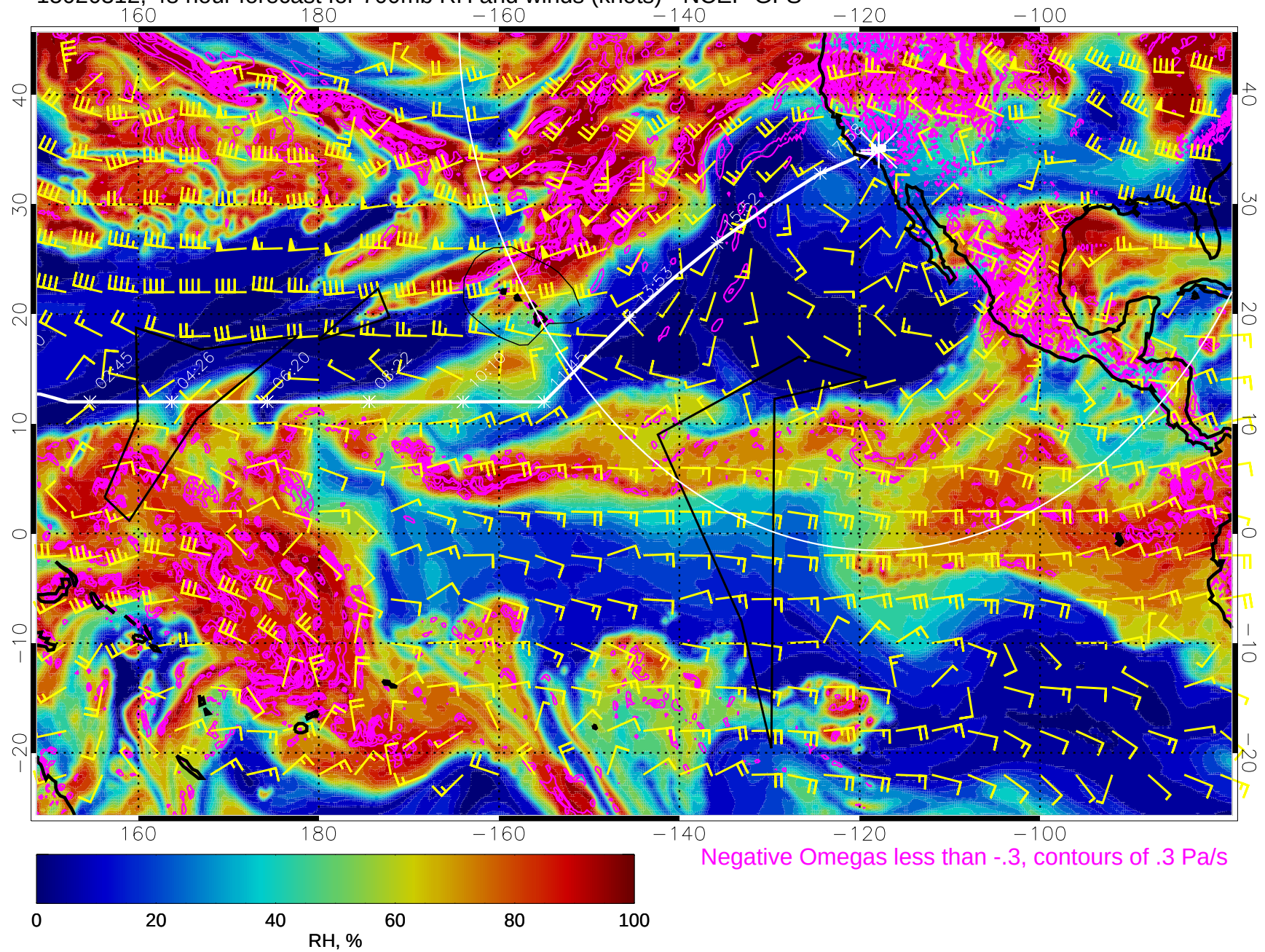
15020312, 48 hour forecast for 700mb RH and winds (knots) - NCEP GFS
