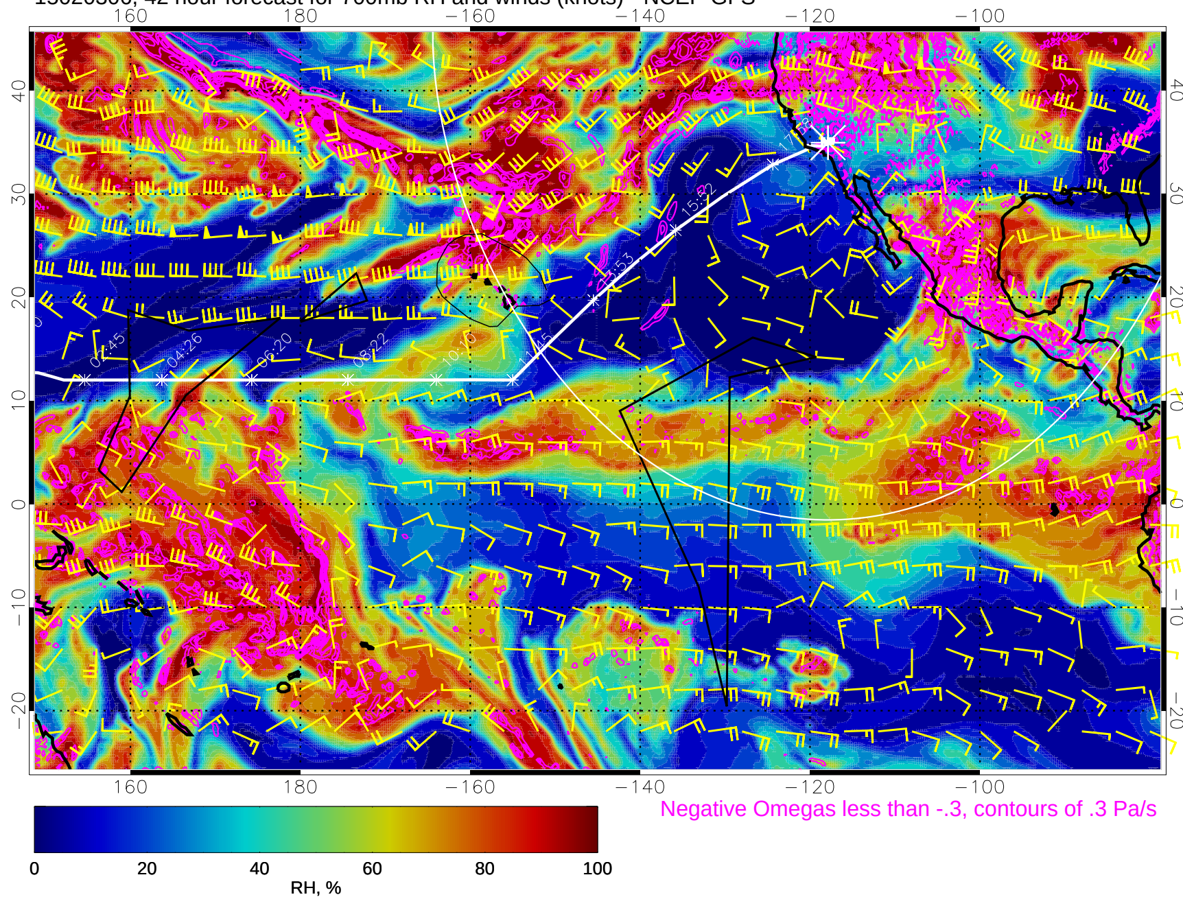
15020306, 42 hour forecast for 700mb RH and winds (knots) - NCEP GFS
