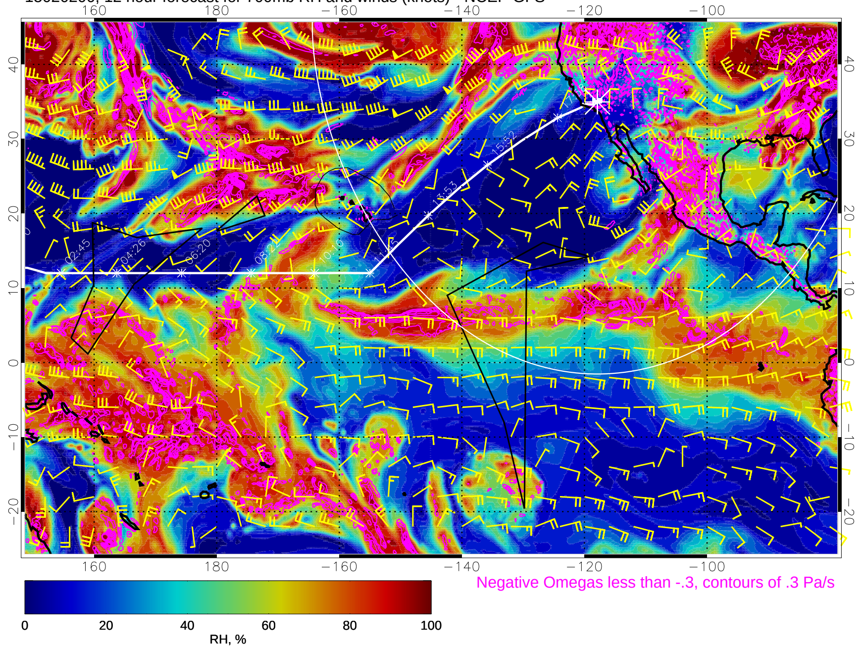
15020200, 12 hour forecast for 700mb RH and winds (knots) - NCEP GFS
