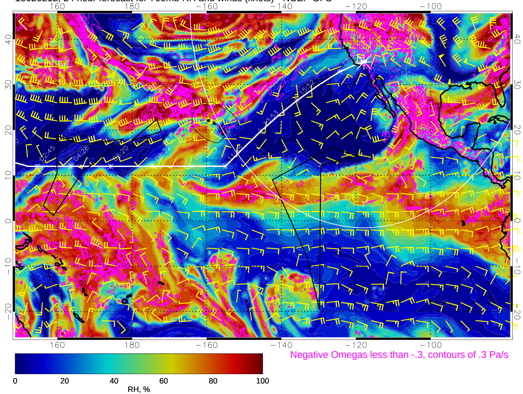
15020212, 24 hour forecast for 700mb RH and winds (knots) - NCEP GFS
