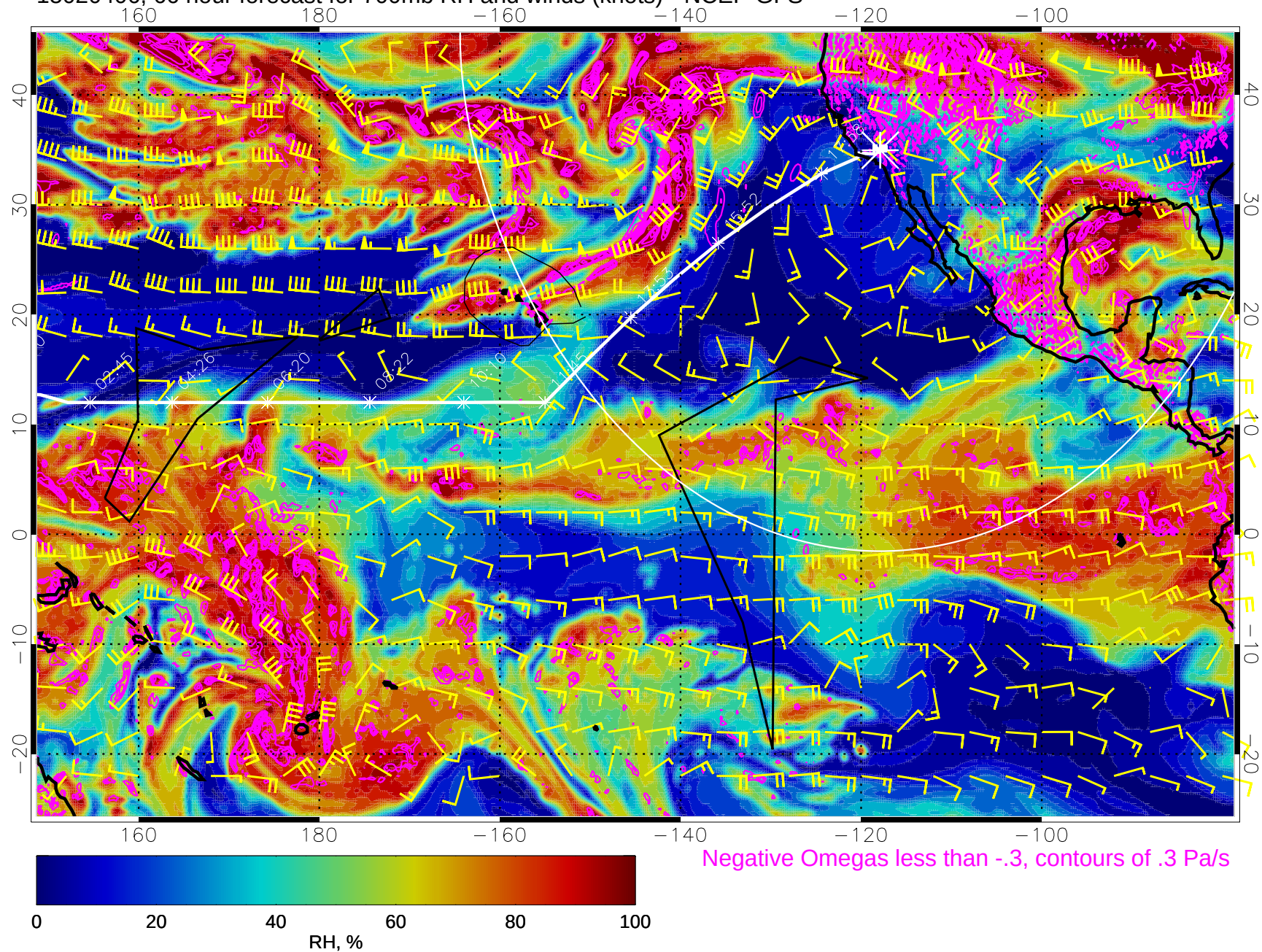
15020406, 66 hour forecast for 700mb RH and winds (knots) - NCEP GFS
