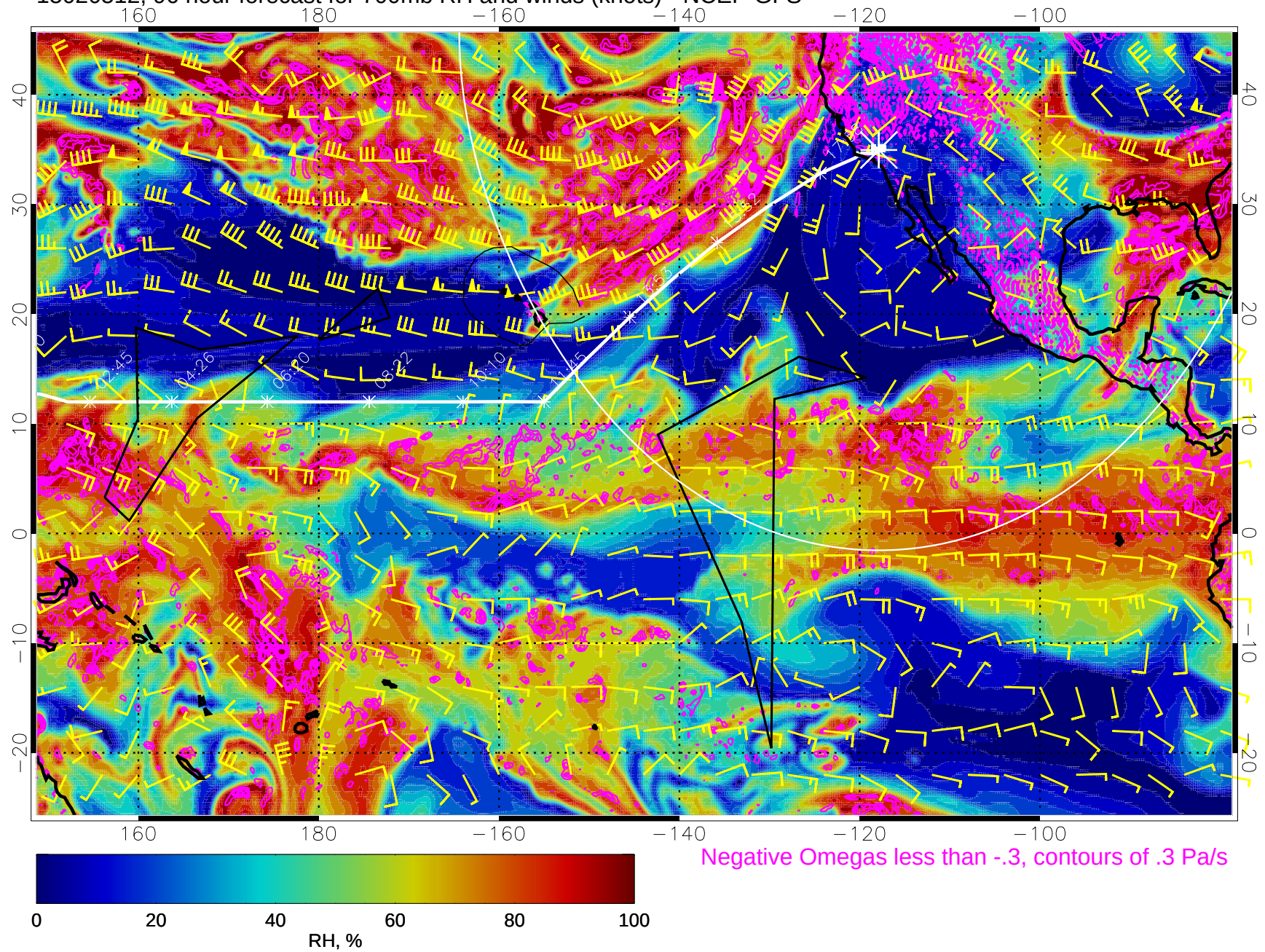
15020512, 96 hour forecast for 700mb RH and winds (knots) - NCEP GFS
