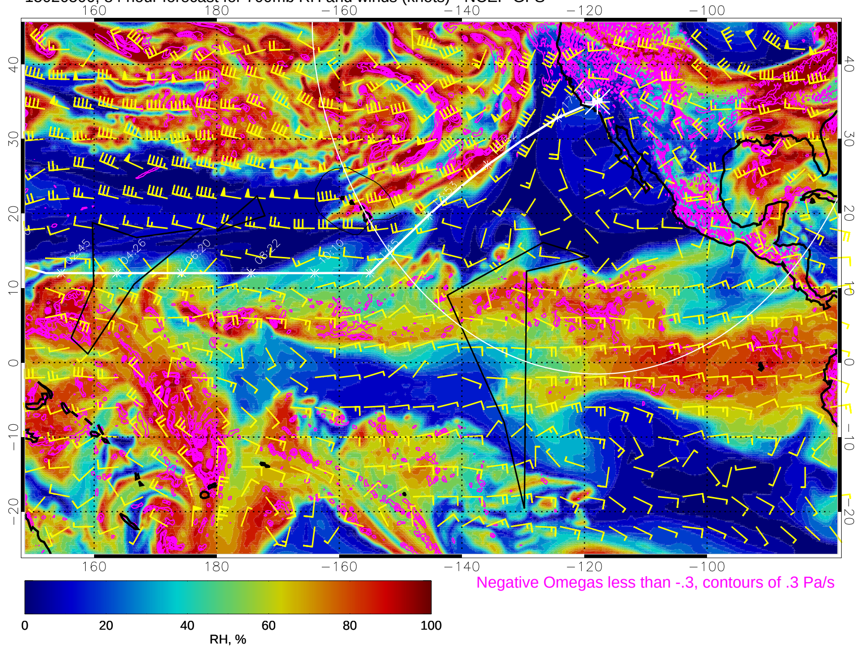
15020500, 84 hour forecast for 700mb RH and winds (knots) - NCEP GFS
