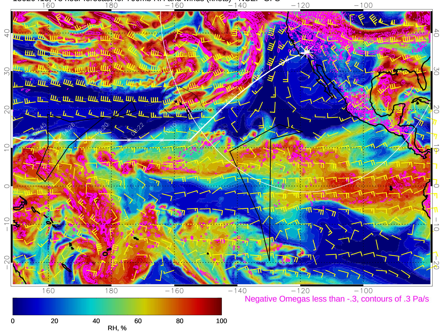
15020418, 78 hour forecast for 700mb RH and winds (knots) - NCEP GFS
