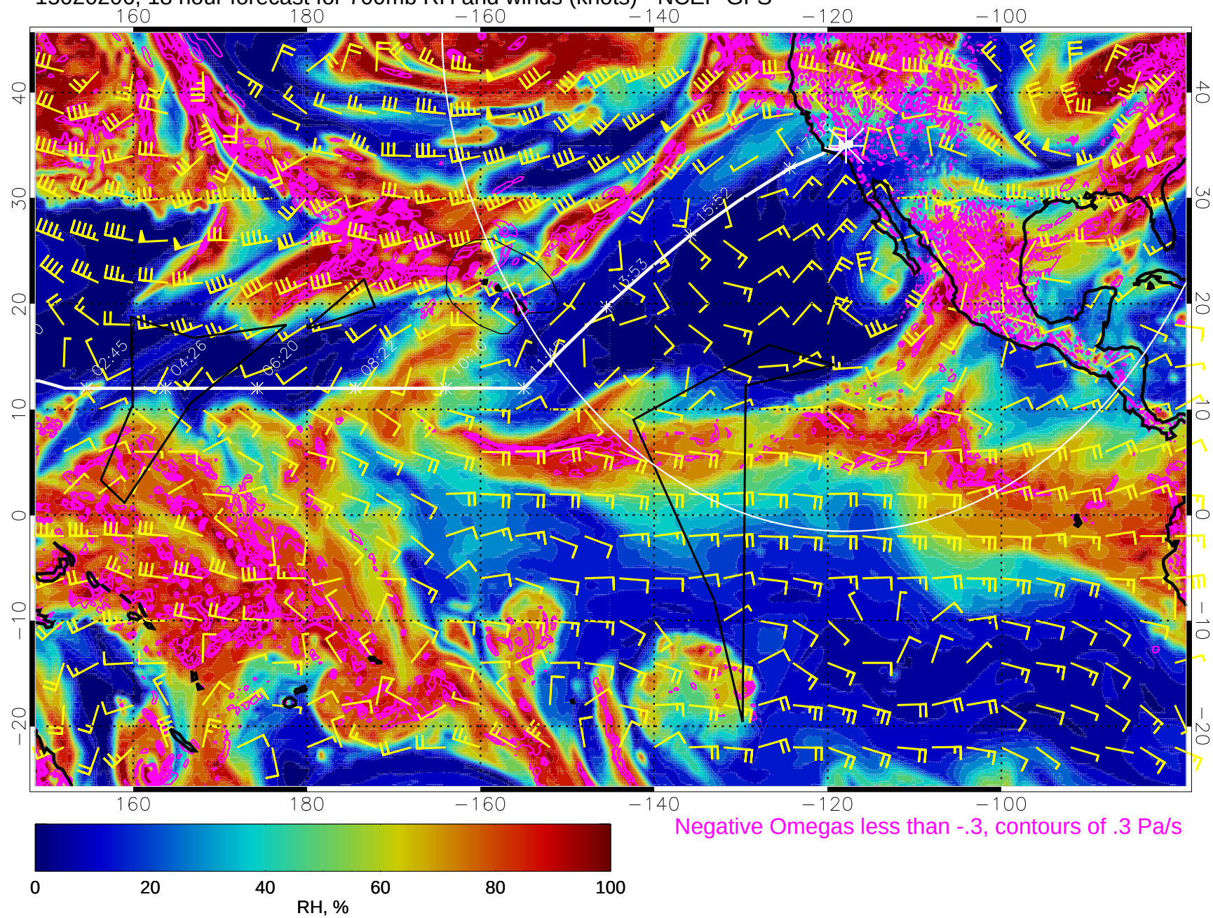
15020206, 18 hour forecast for 700mb RH and winds (knots) - NCEP GFS
