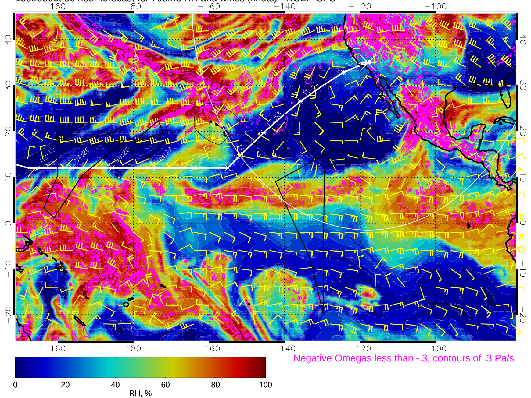
15020300, 36 hour forecast for 700mb RH and winds (knots) - NCEP GFS
