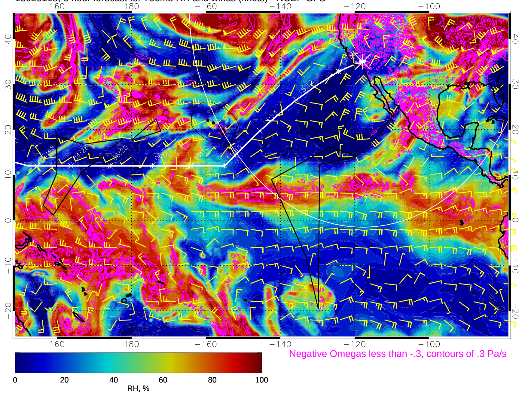
15020118, 6 hour forecast for 700mb RH and winds (knots) - NCEP GFS
