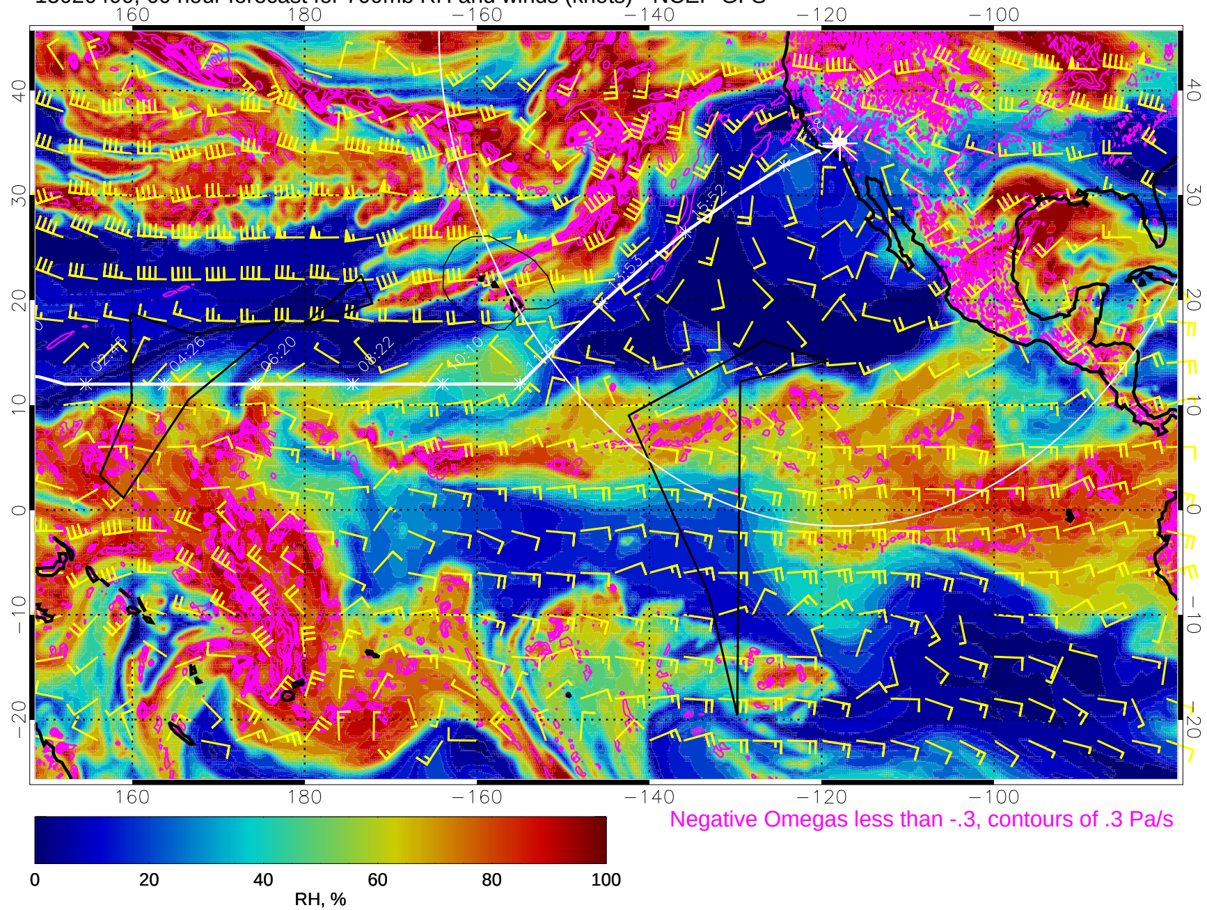
15020400, 60 hour forecast for 700mb RH and winds (knots) - NCEP GFS
