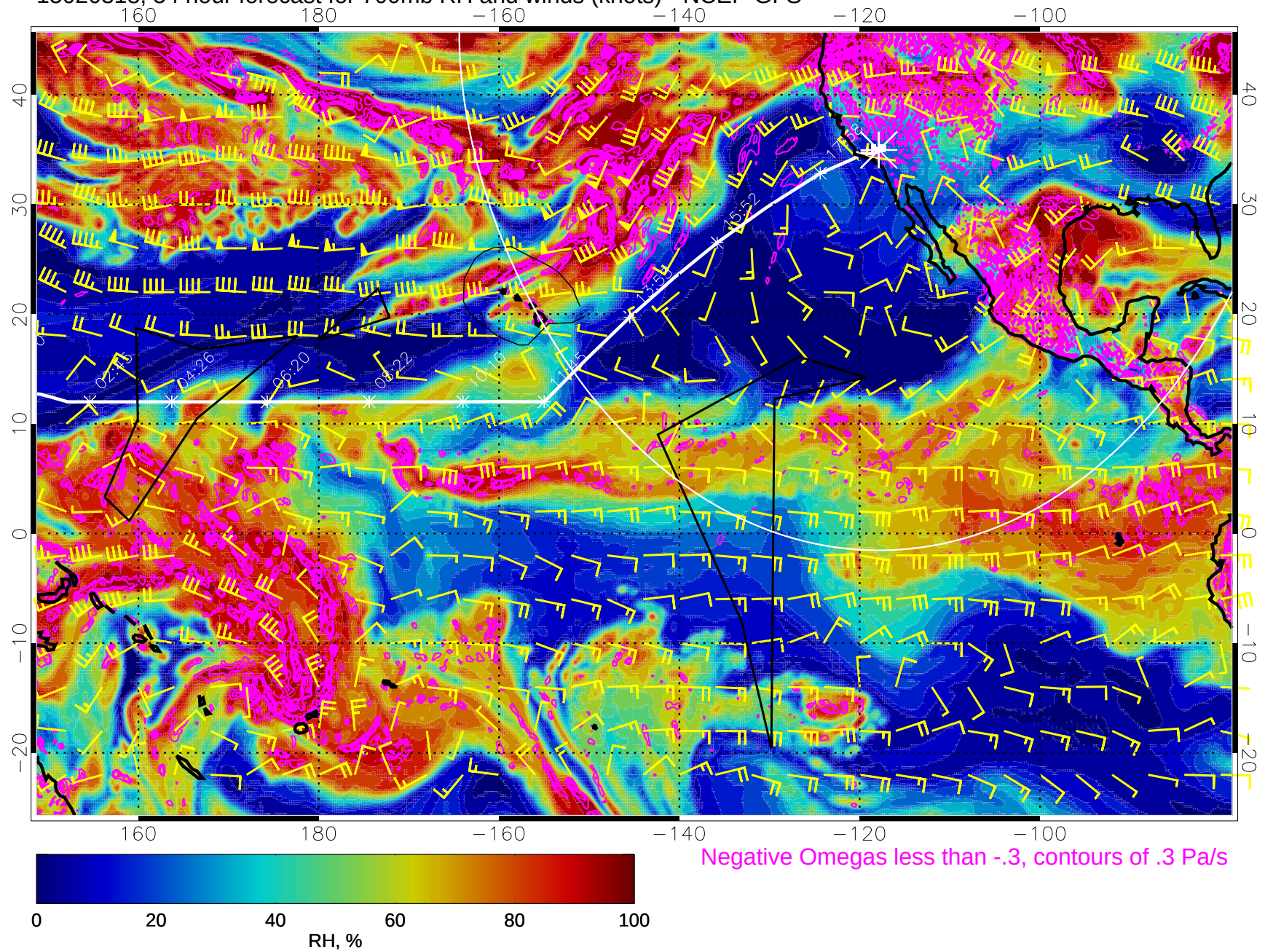
15020318, 54 hour forecast for 700mb RH and winds (knots) - NCEP GFS
