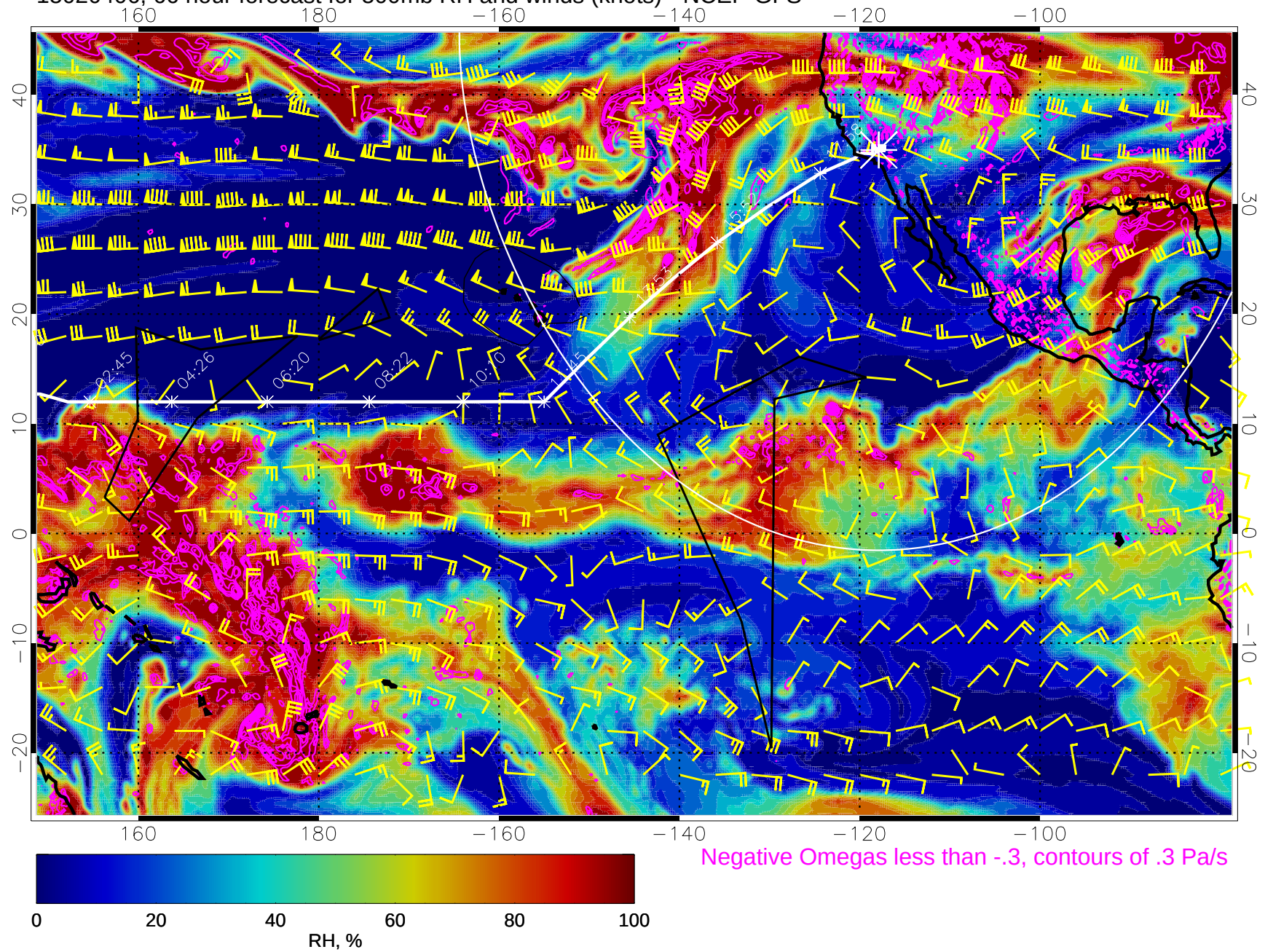
15020406, 66 hour forecast for 500mb RH and winds (knots) - NCEP GFS
