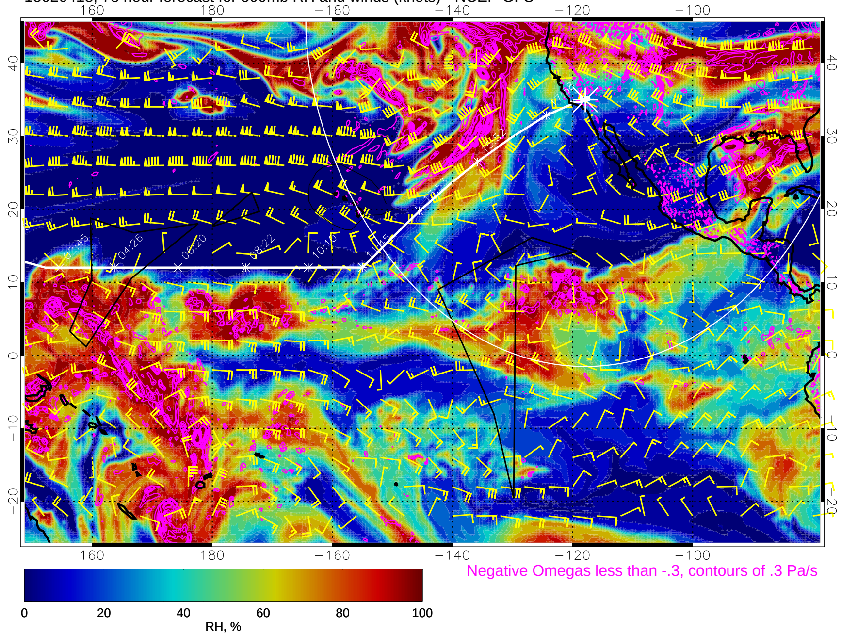
15020418, 78 hour forecast for 500mb RH and winds (knots) - NCEP GFS
