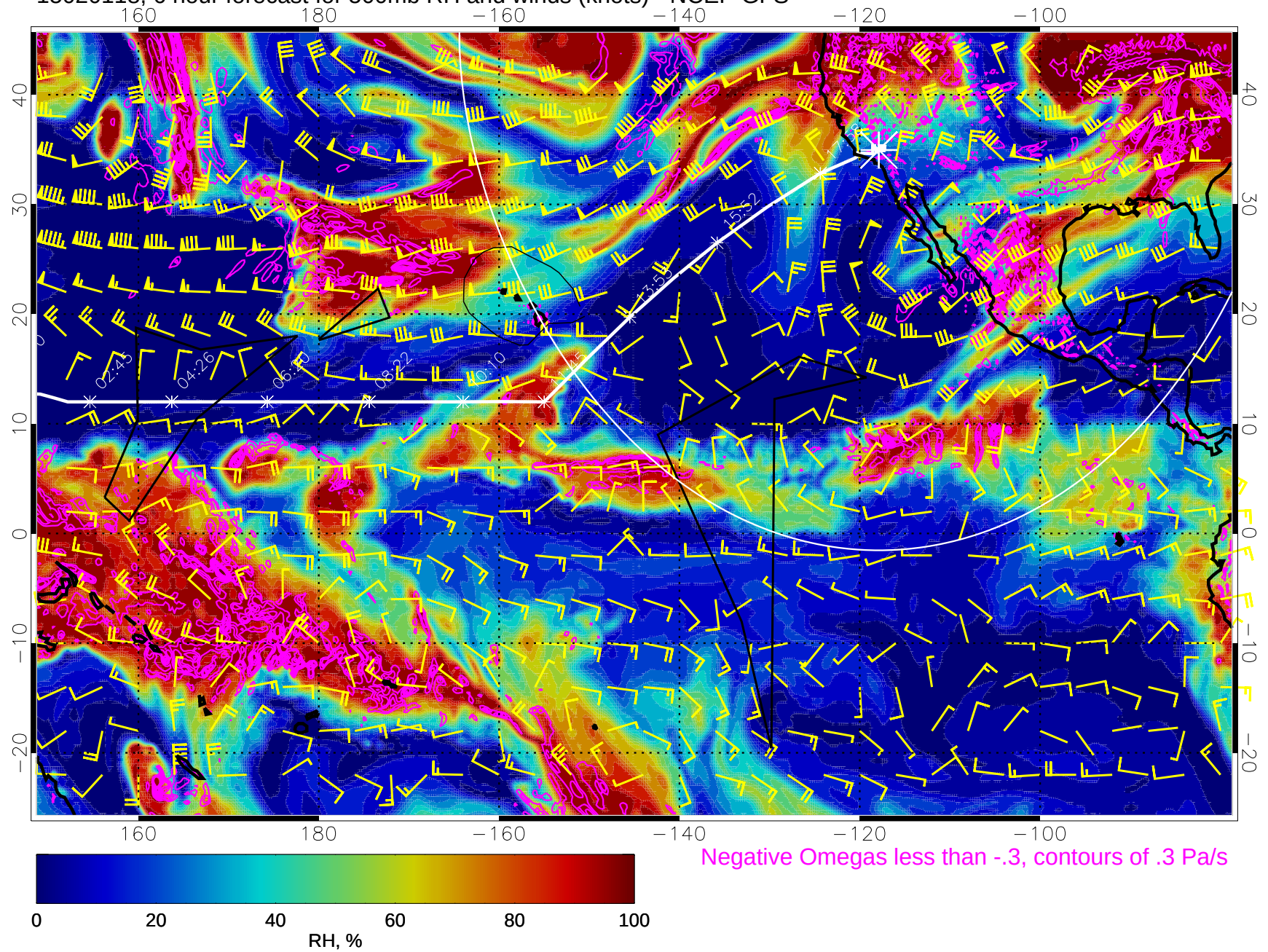
15020118, 6 hour forecast for 500mb RH and winds (knots) - NCEP GFS
