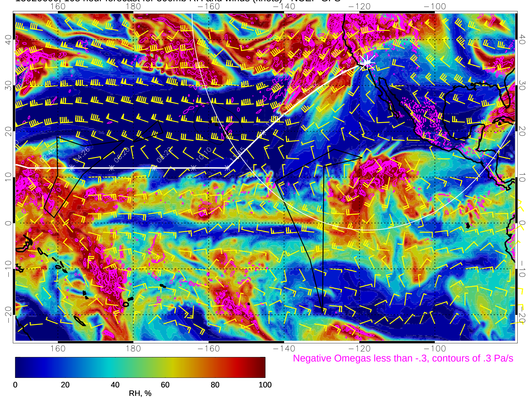
15020600, 108 hour forecast for 500mb RH and winds (knots) - NCEP GFS
