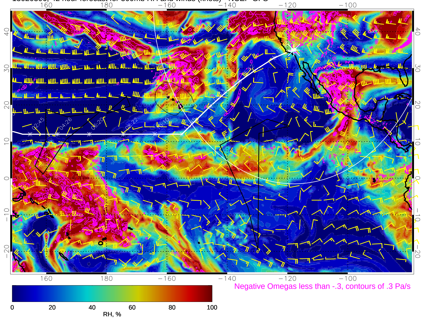
15020306, 42 hour forecast for 500mb RH and winds (knots) - NCEP GFS
