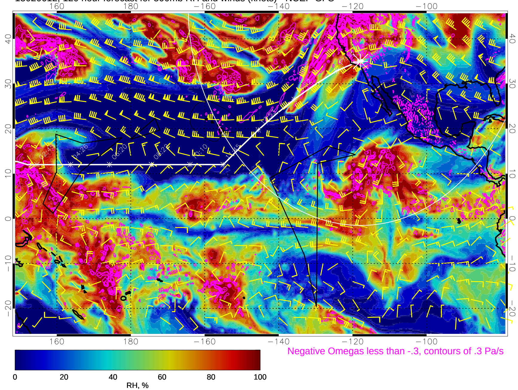
15020612, 120 hour forecast for 500mb RH and winds (knots) - NCEP GFS
