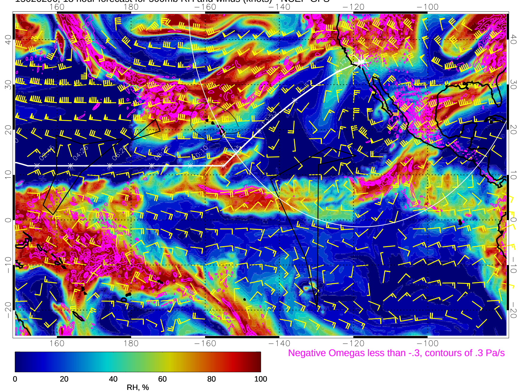
15020206, 18 hour forecast for 500mb RH and winds (knots) - NCEP GFS
