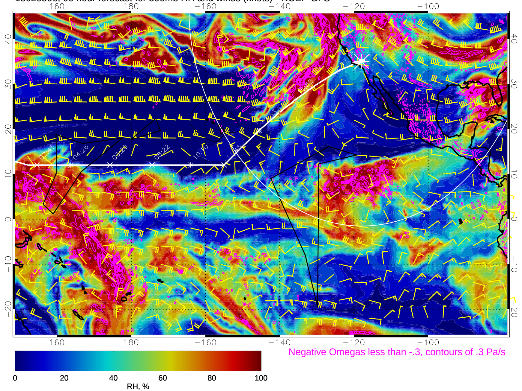
15020506, 90 hour forecast for 500mb RH and winds (knots) - NCEP GFS
