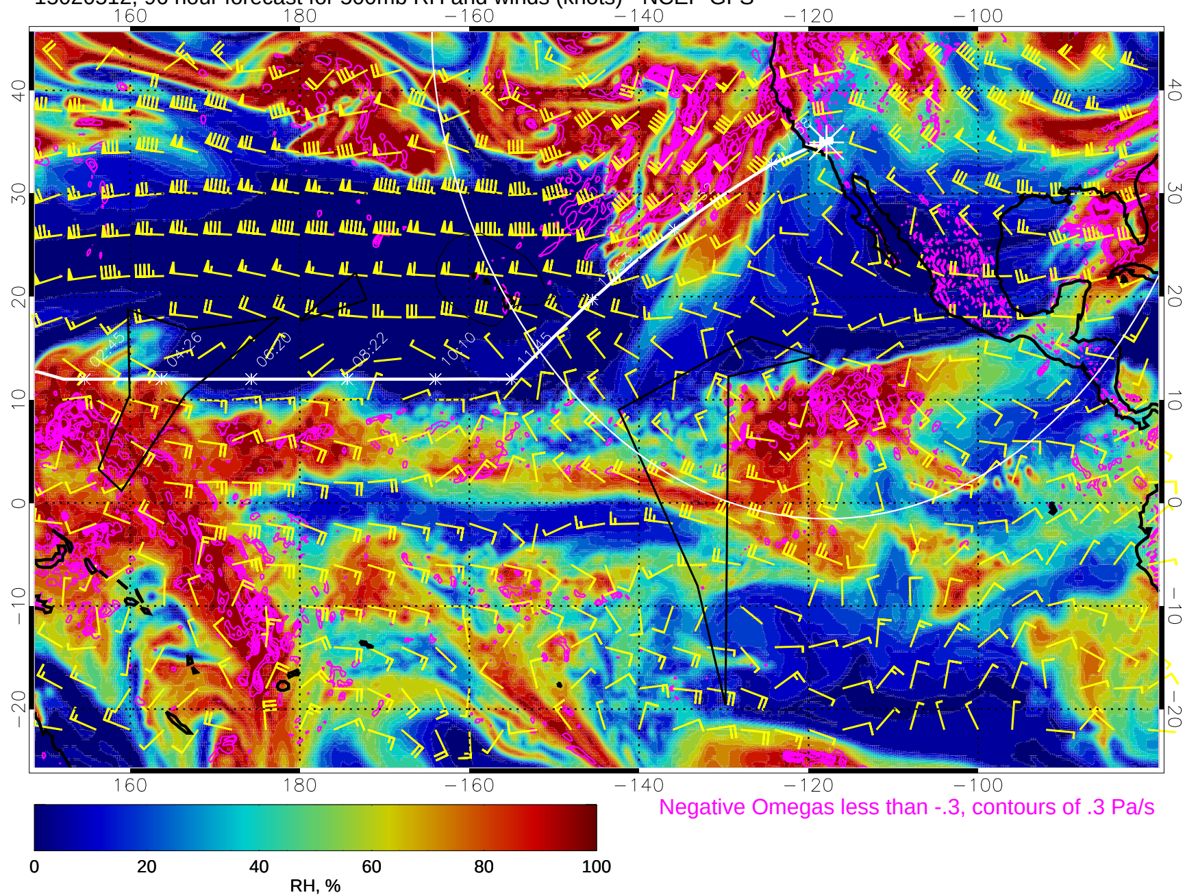
15020512, 96 hour forecast for 500mb RH and winds (knots) - NCEP GFS
