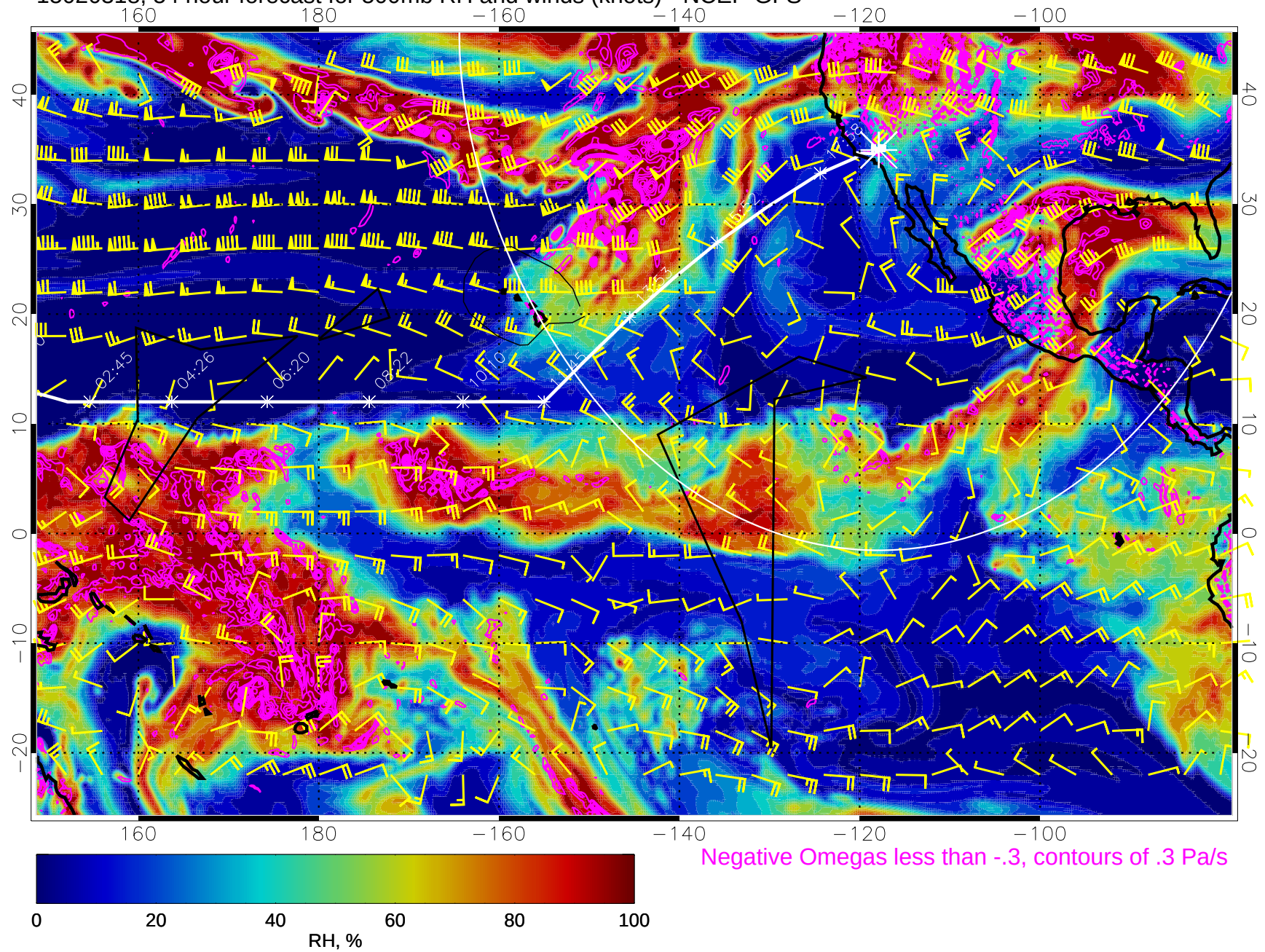
15020318, 54 hour forecast for 500mb RH and winds (knots) - NCEP GFS
