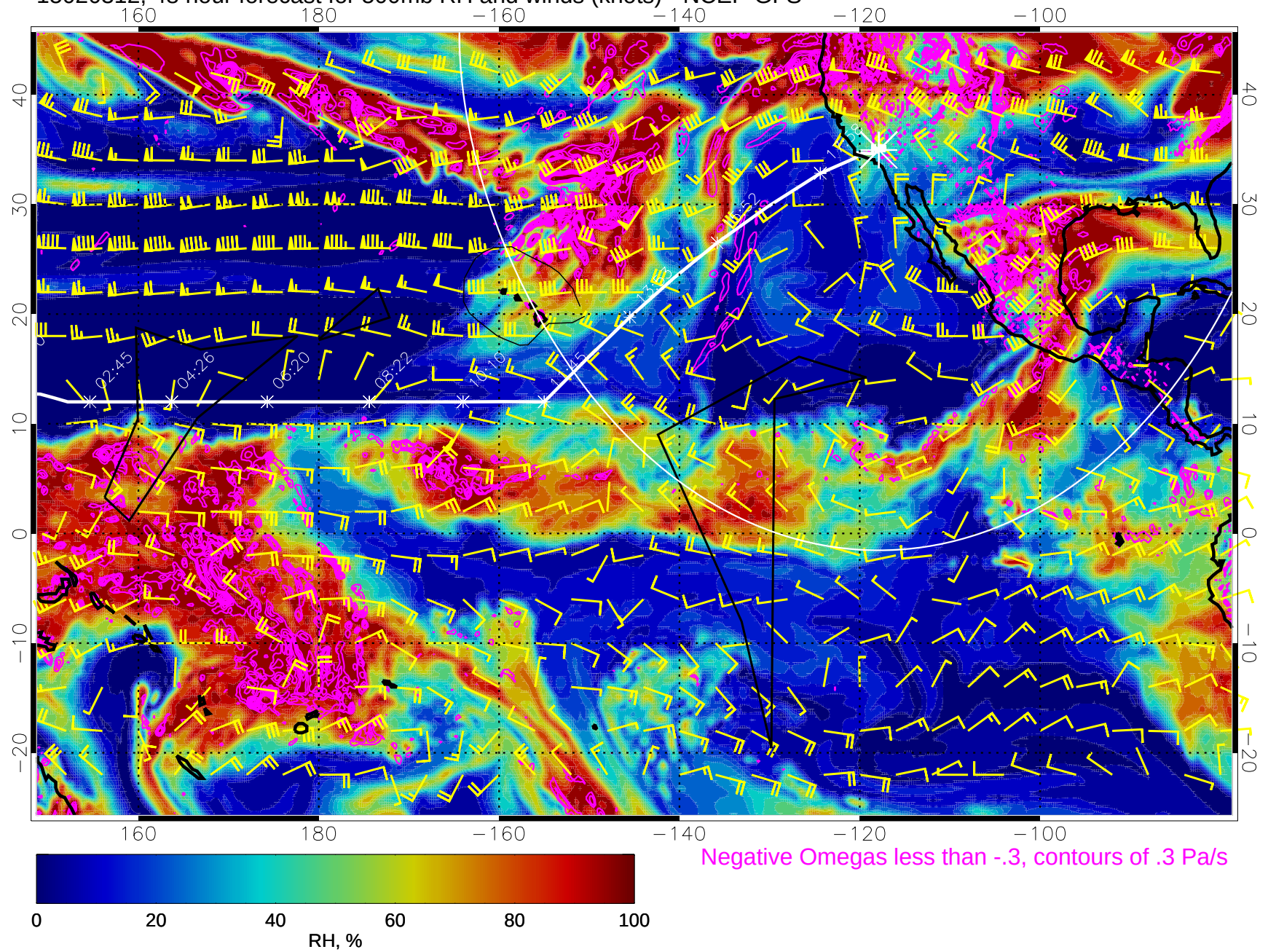
15020312, 48 hour forecast for 500mb RH and winds (knots) - NCEP GFS
