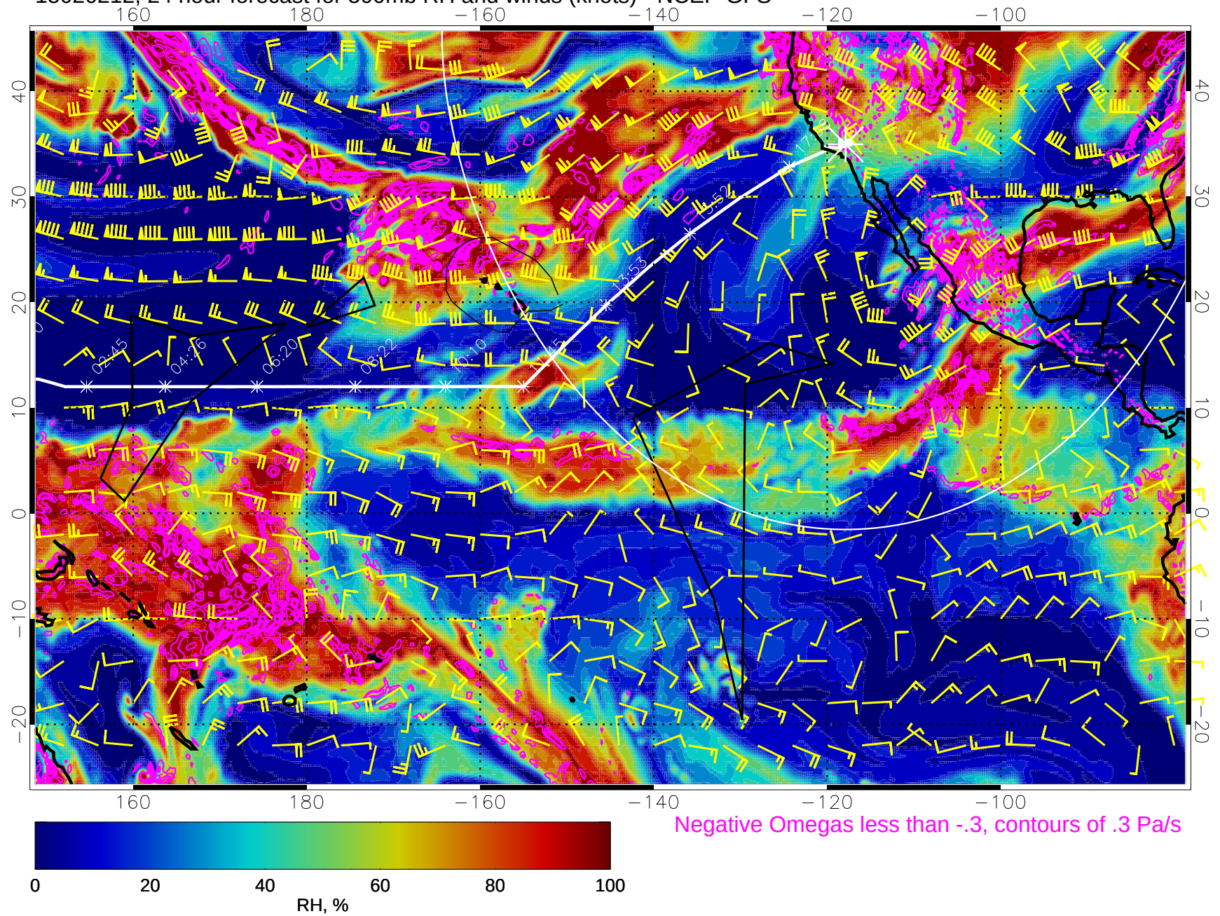
15020212, 24 hour forecast for 500mb RH and winds (knots) - NCEP GFS
