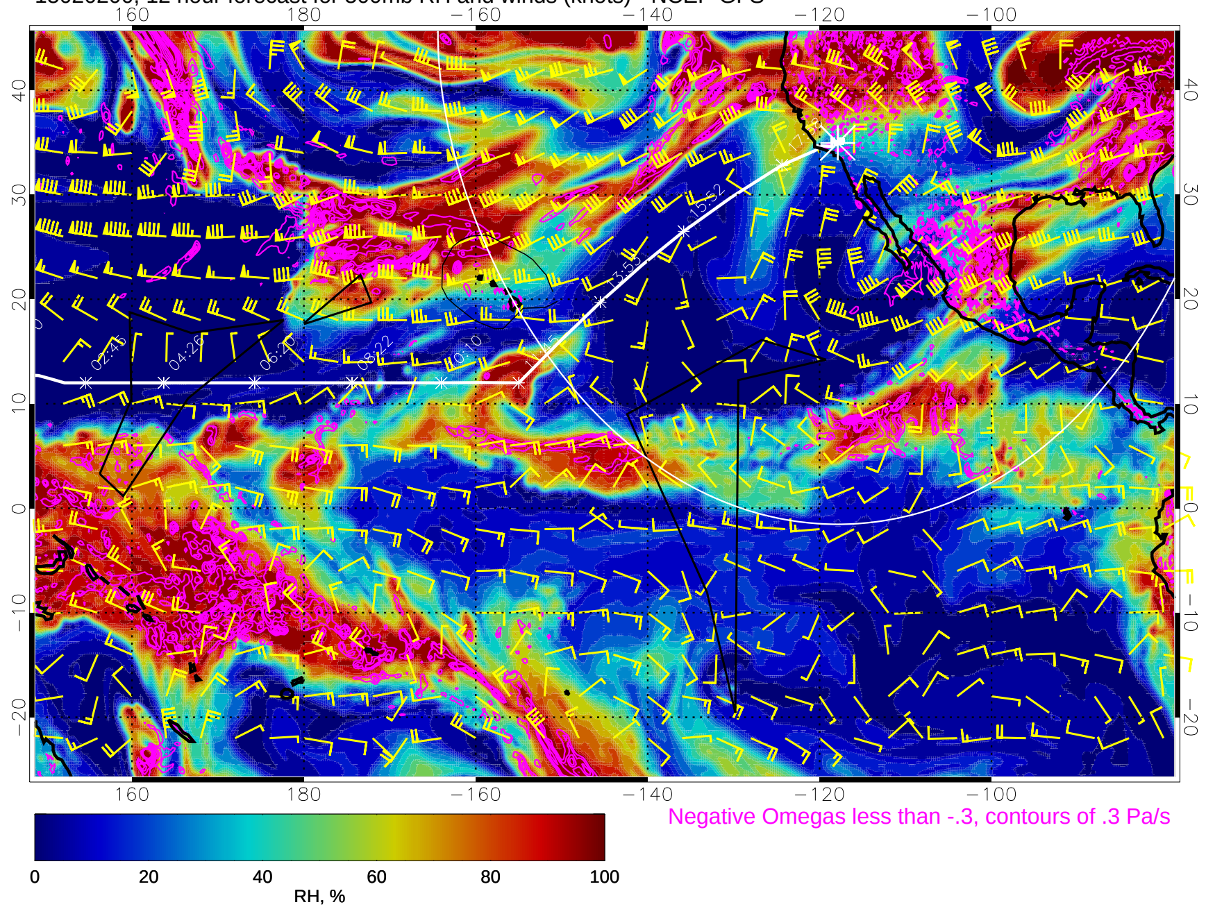
15020200, 12 hour forecast for 500mb RH and winds (knots) - NCEP GFS
