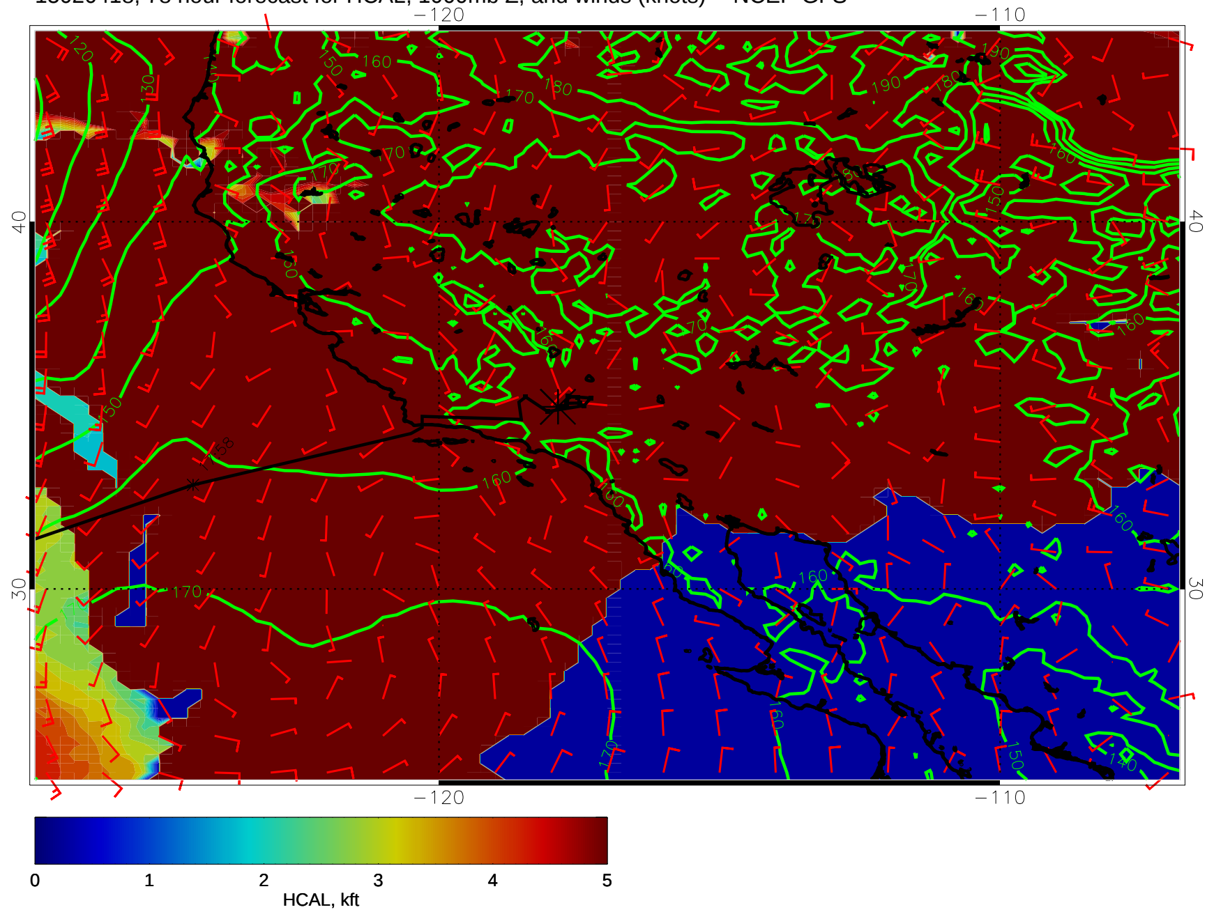
15020418, 78 hour forecast for HCAL, 1000mb Z, and winds (knots) -- NCEP GFS
