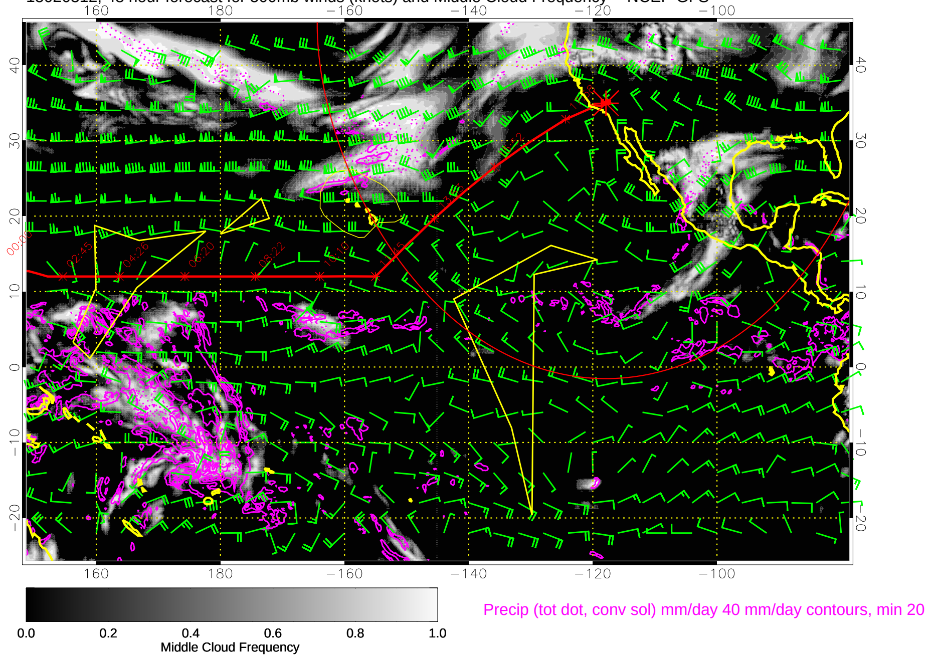
15020312, 48 hour forecast for 500mb winds (knots) and Middle Cloud Frequency -- NCEP GFS
