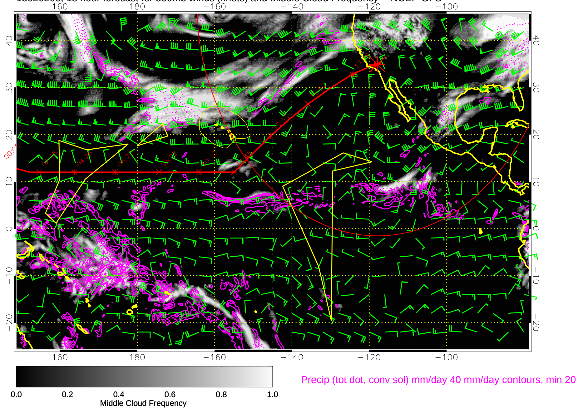
15020206, 18 hour forecast for 500mb winds (knots) and Middle Cloud Frequency -- NCEP GFS
