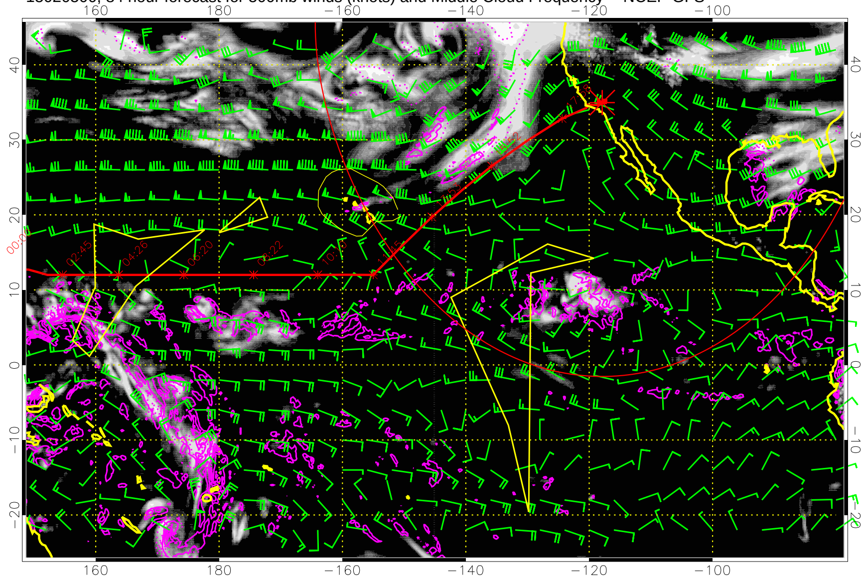
15020500, 84 hour forecast for 500mb winds (knots) and Middle Cloud Frequency -- NCEP GFS
