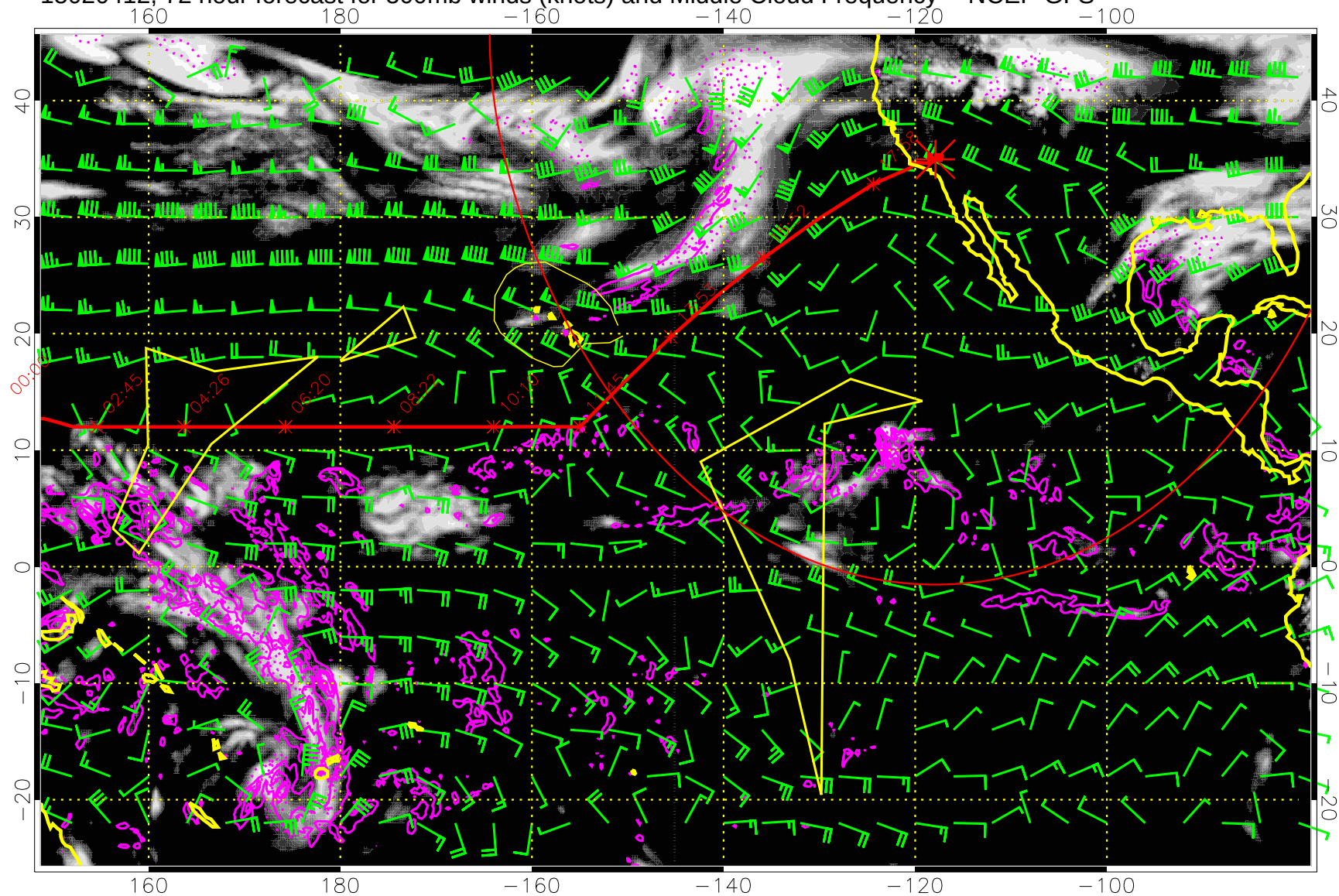
15020412, 72 hour forecast for 500mb winds (knots) and Middle Cloud Frequency -- NCEP GFS
