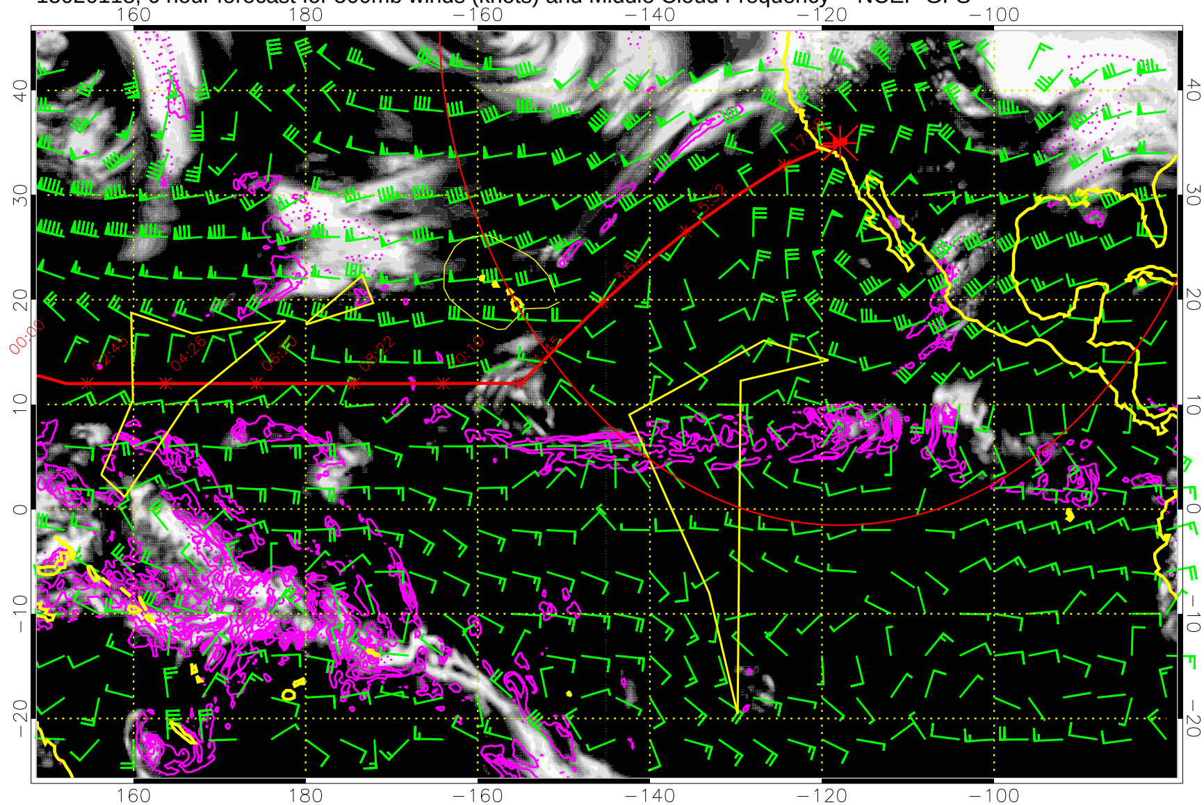
15020118, 6 hour forecast for 500mb winds (knots) and Middle Cloud Frequency -- NCEP GFS
