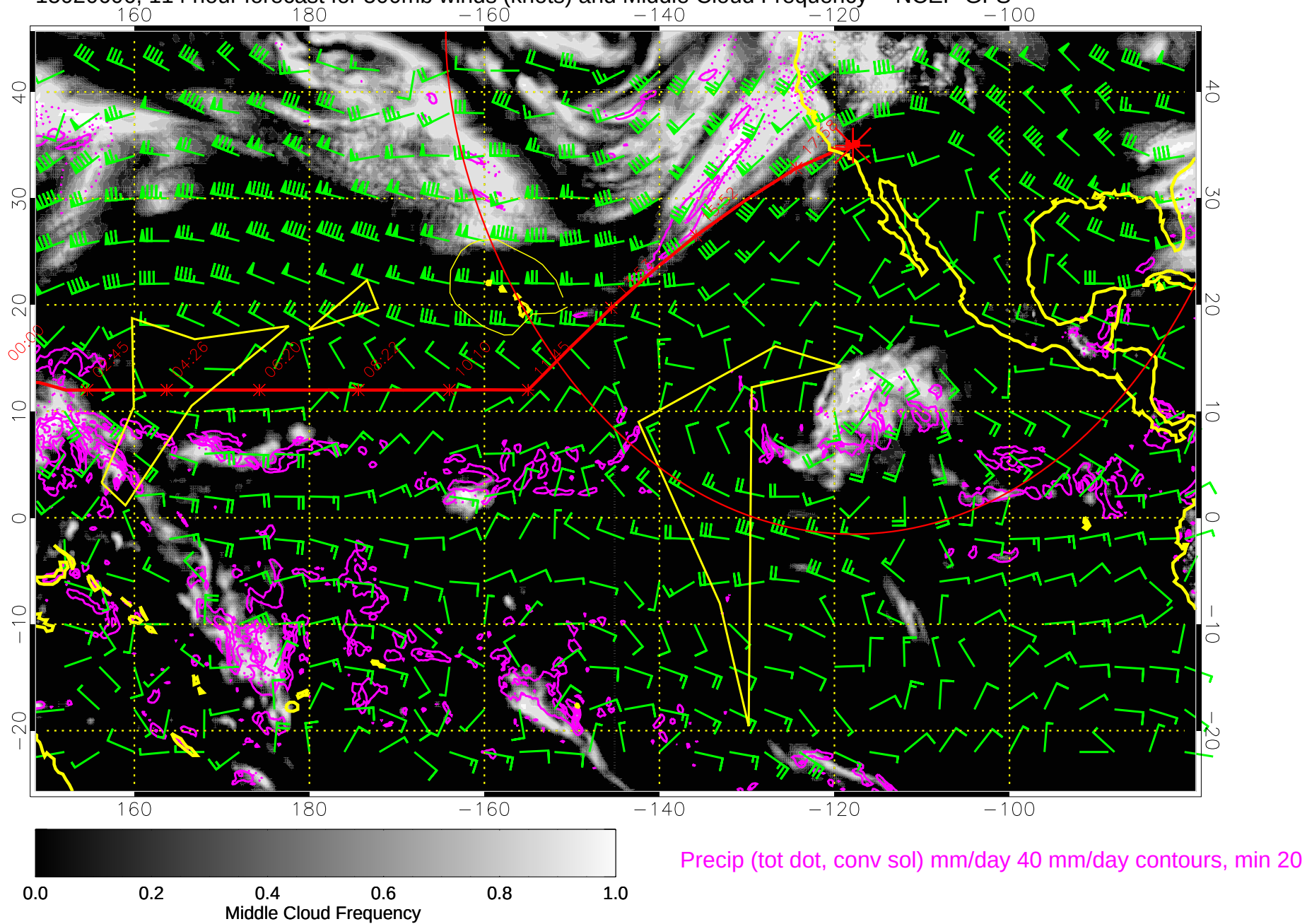
15020606, 114 hour forecast for 500mb winds (knots) and Middle Cloud Frequency -- NCEP GFS
