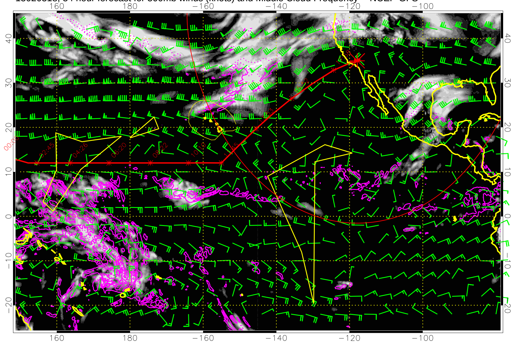
15020318, 54 hour forecast for 500mb winds (knots) and Middle Cloud Frequency -- NCEP GFS
