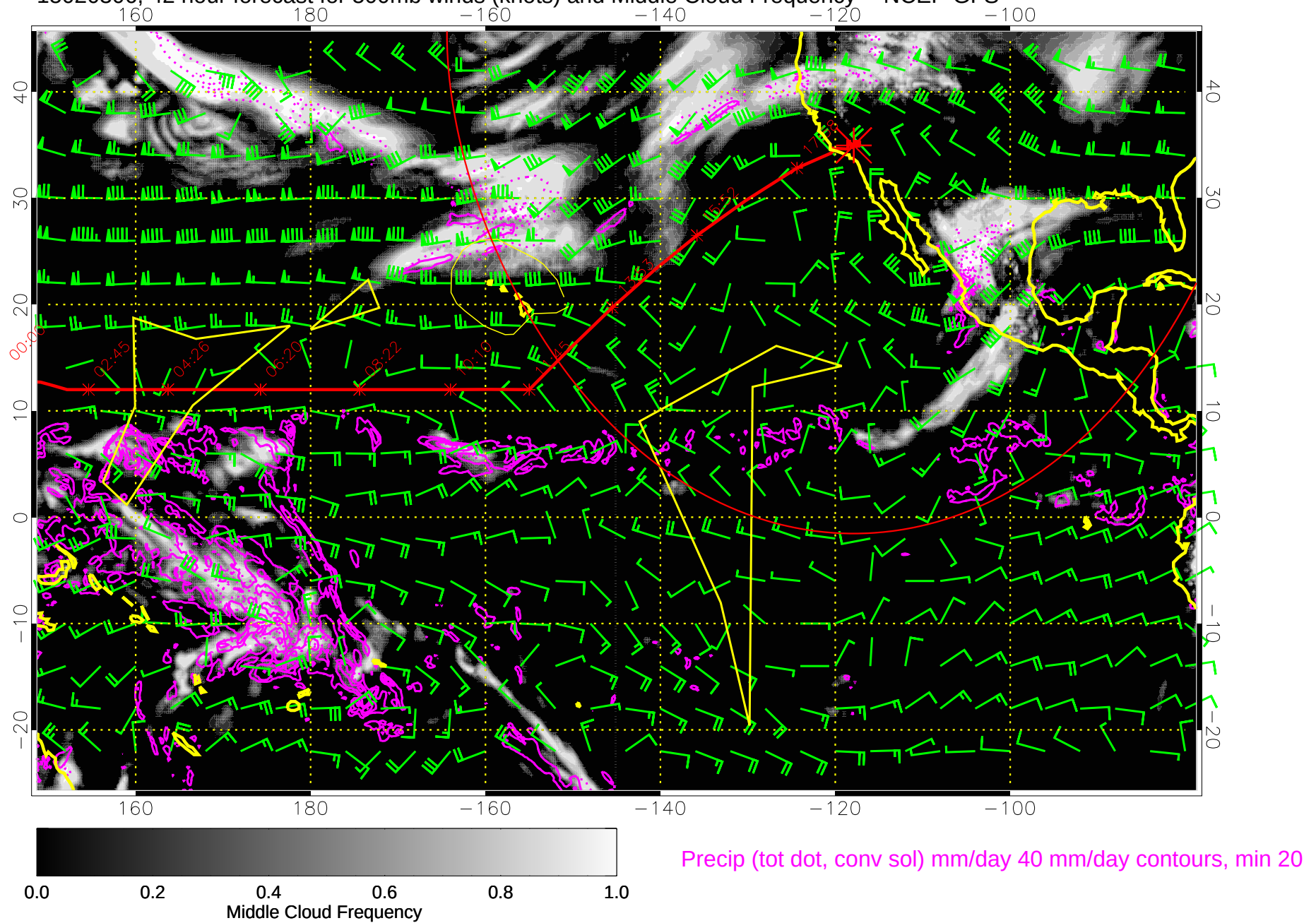
15020306, 42 hour forecast for 500mb winds (knots) and Middle Cloud Frequency -- NCEP GFS
