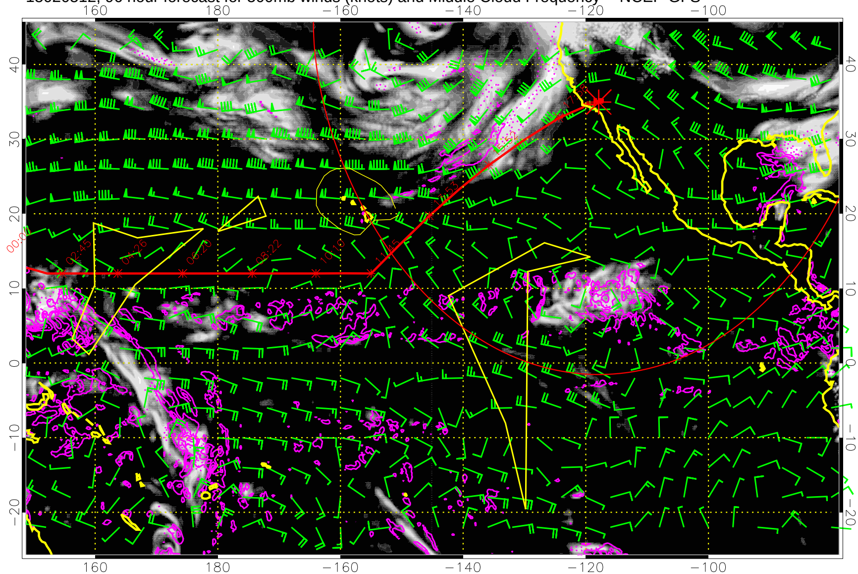
15020512, 96 hour forecast for 500mb winds (knots) and Middle Cloud Frequency -- NCEP GFS
