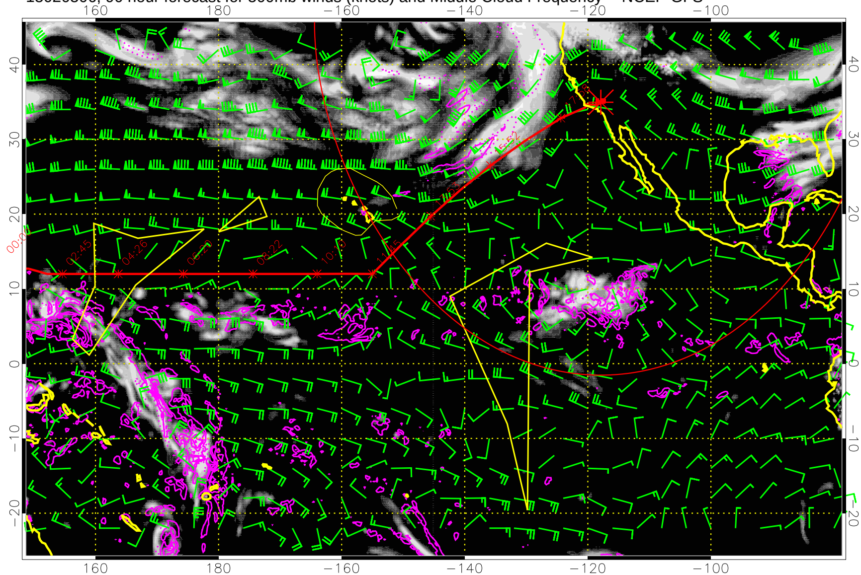
15020506, 90 hour forecast for 500mb winds (knots) and Middle Cloud Frequency -- NCEP GFS
