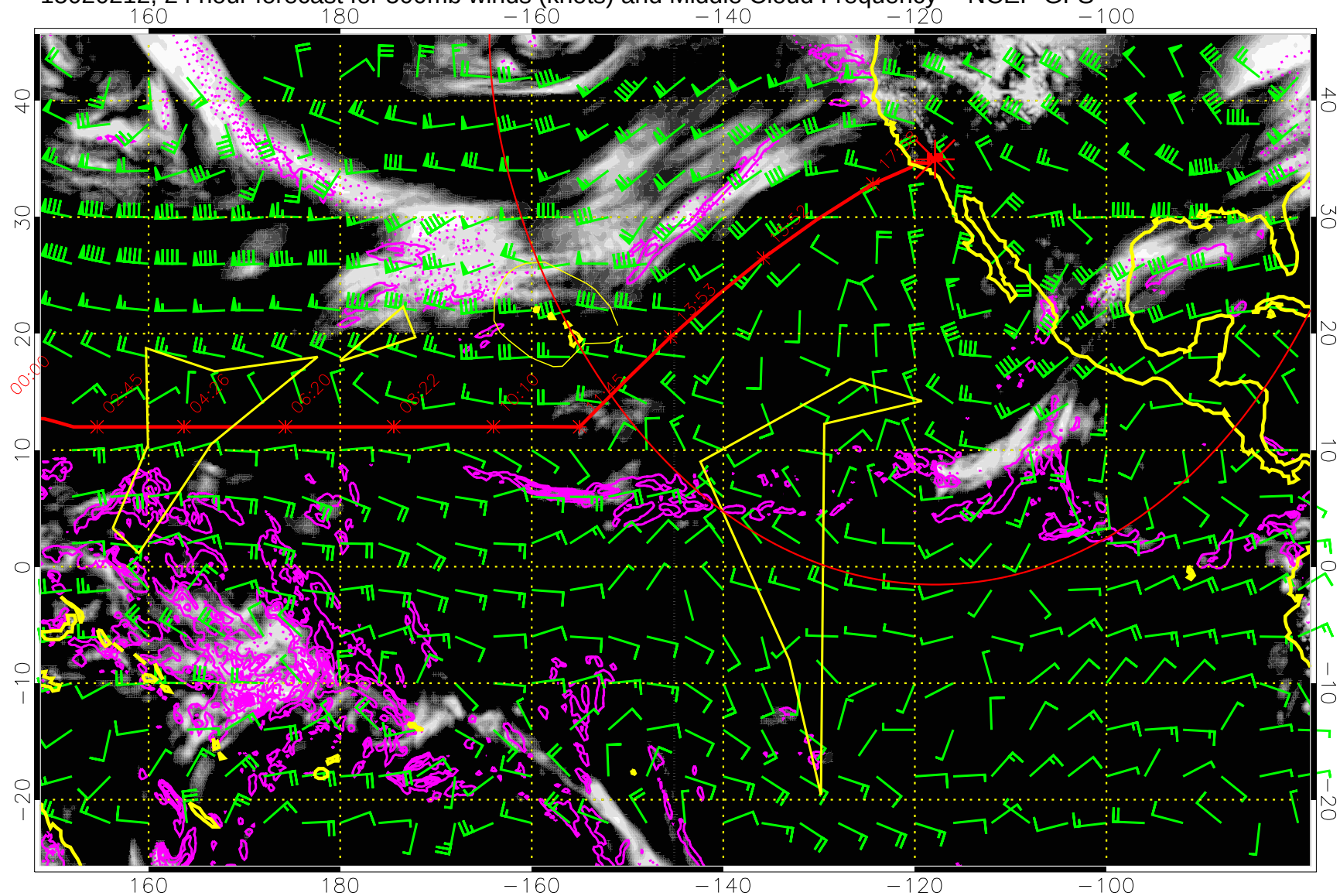
15020212, 24 hour forecast for 500mb winds (knots) and Middle Cloud Frequency -- NCEP GFS
