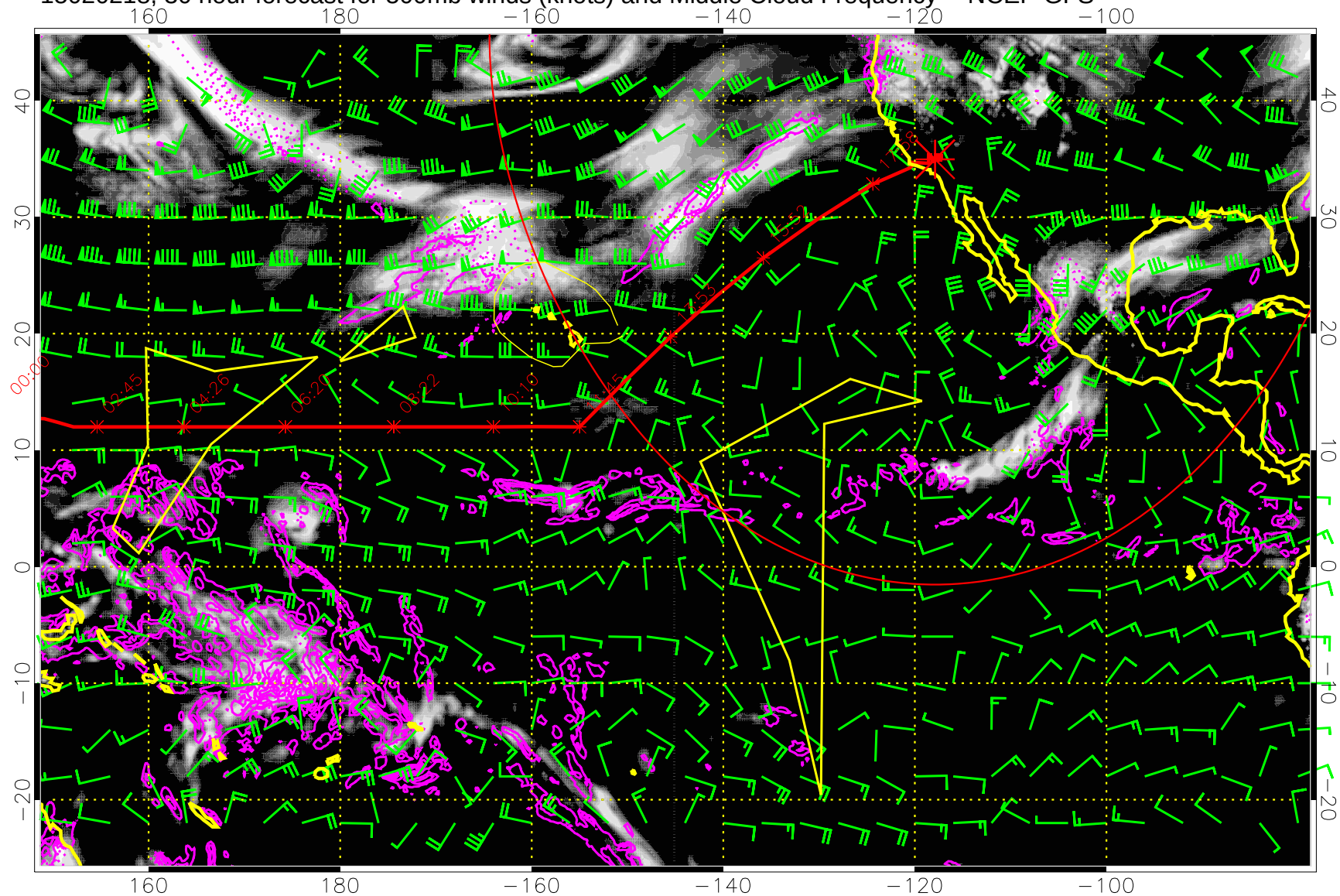
15020218, 30 hour forecast for 500mb winds (knots) and Middle Cloud Frequency -- NCEP GFS
