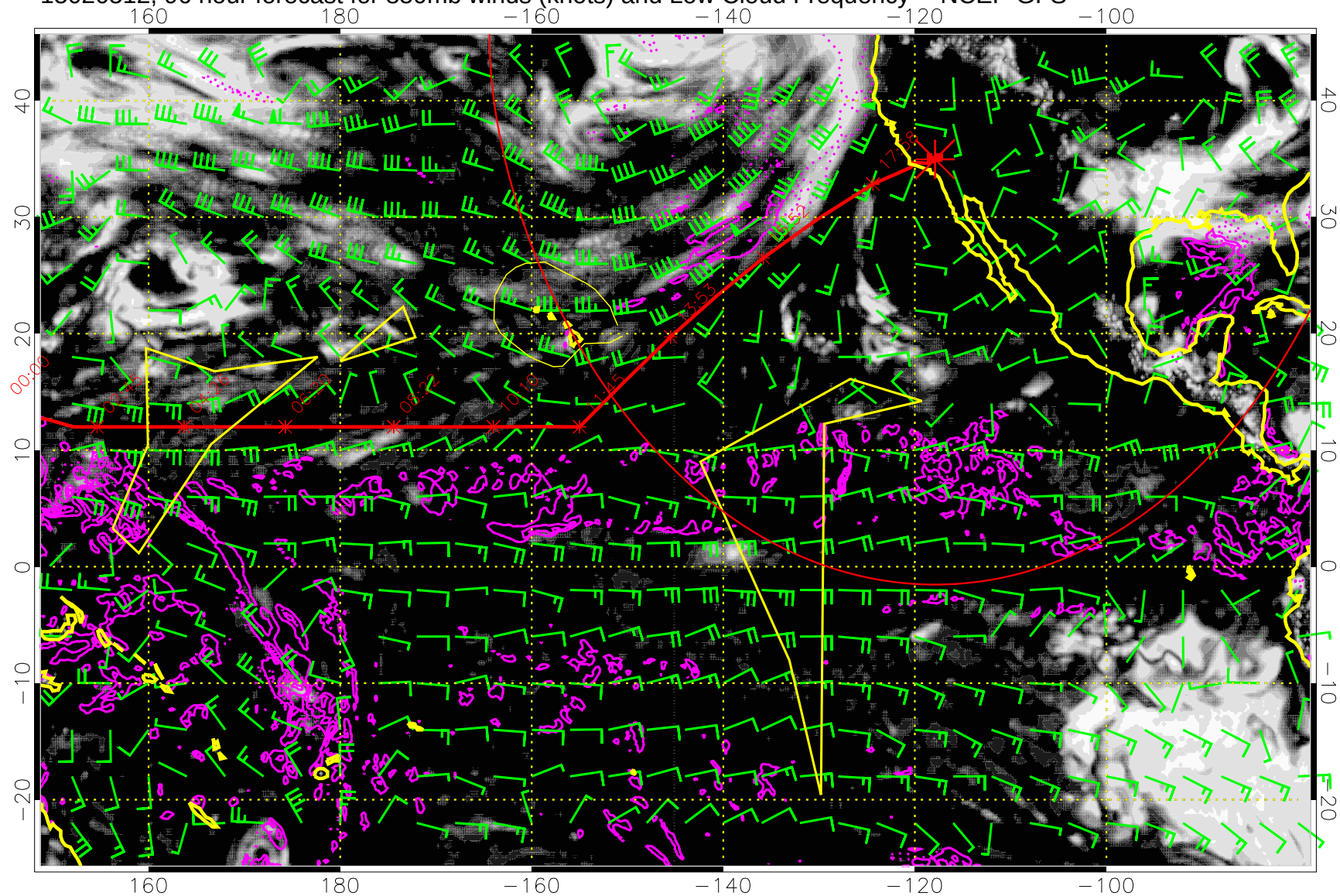
15020512, 96 hour forecast for 850mb winds (knots) and Low Cloud Frequency -- NCEP GFS
