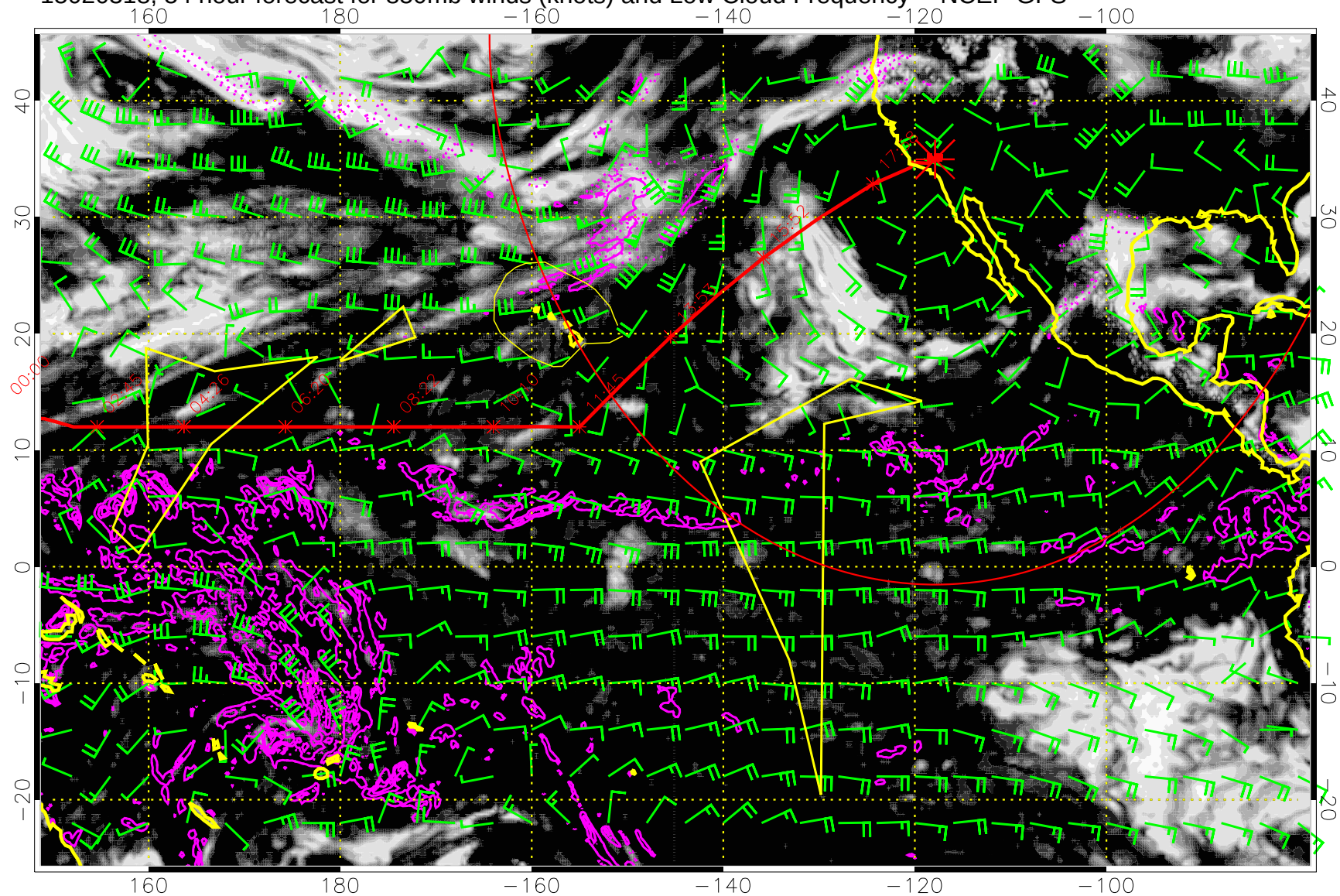
15020318, 54 hour forecast for 850mb winds (knots) and Low Cloud Frequency -- NCEP GFS
