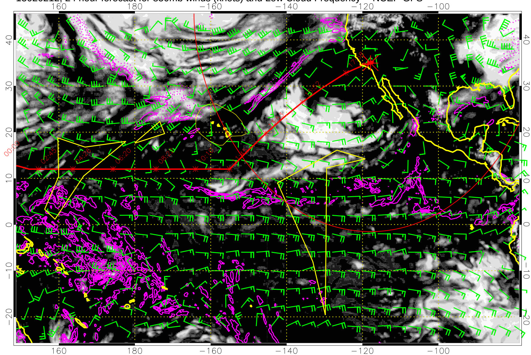
15020212, 24 hour forecast for 850mb winds (knots) and Low Cloud Frequency -- NCEP GFS
