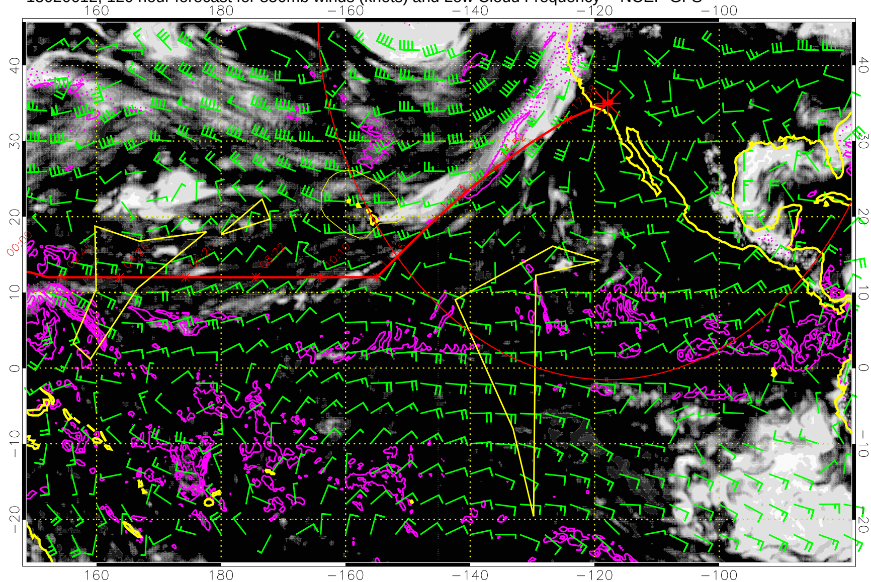
15020612, 120 hour forecast for 850mb winds (knots) and Low Cloud Frequency -- NCEP GFS
