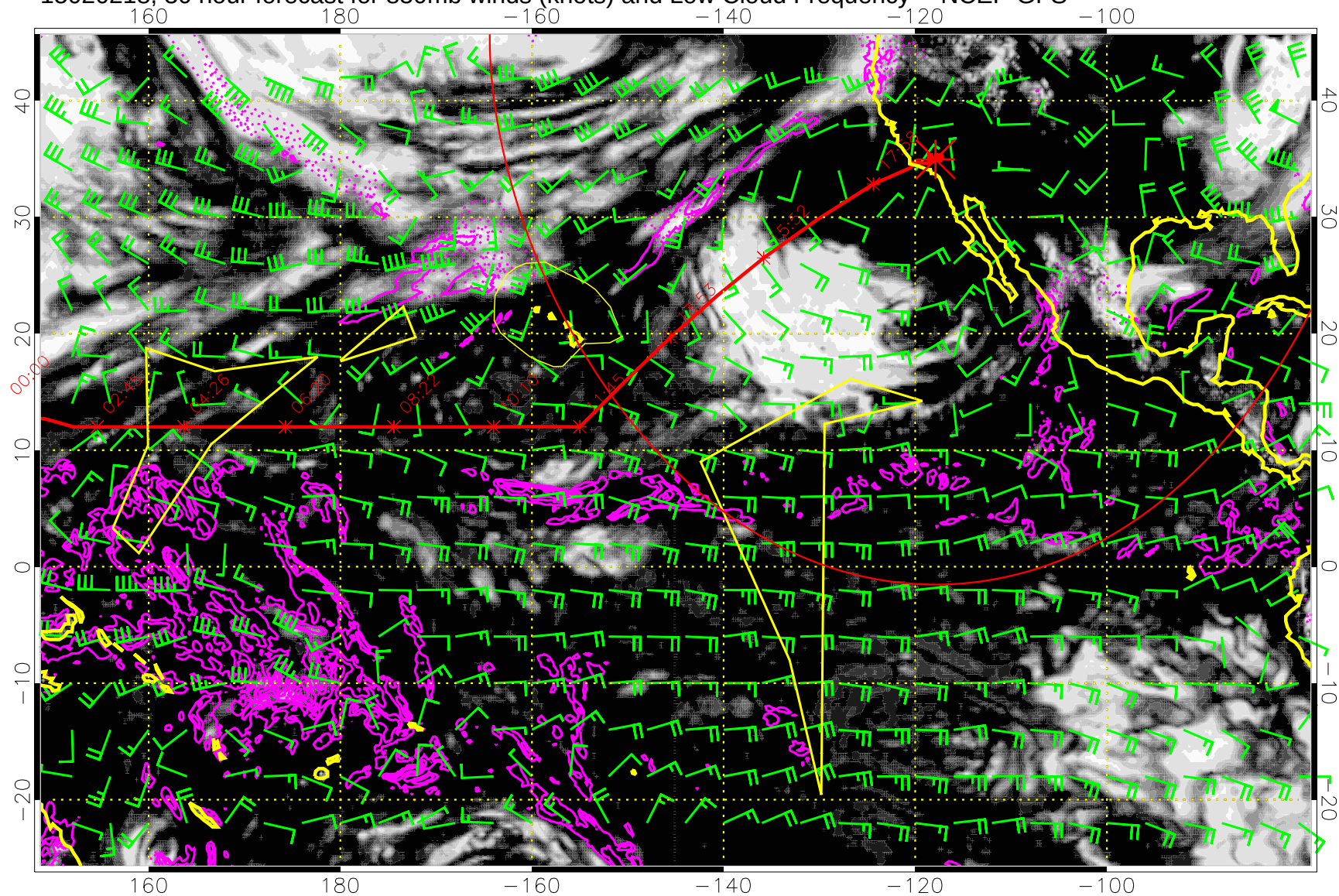
15020218, 30 hour forecast for 850mb winds (knots) and Low Cloud Frequency -- NCEP GFS
