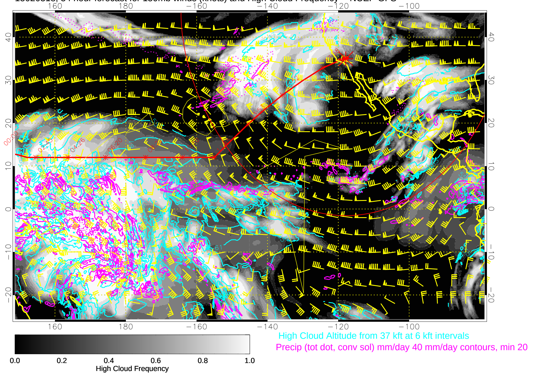
15020318, 54 hour forecast for 150mb winds (knots) and High Cloud Frequency -- NCEP GFS
