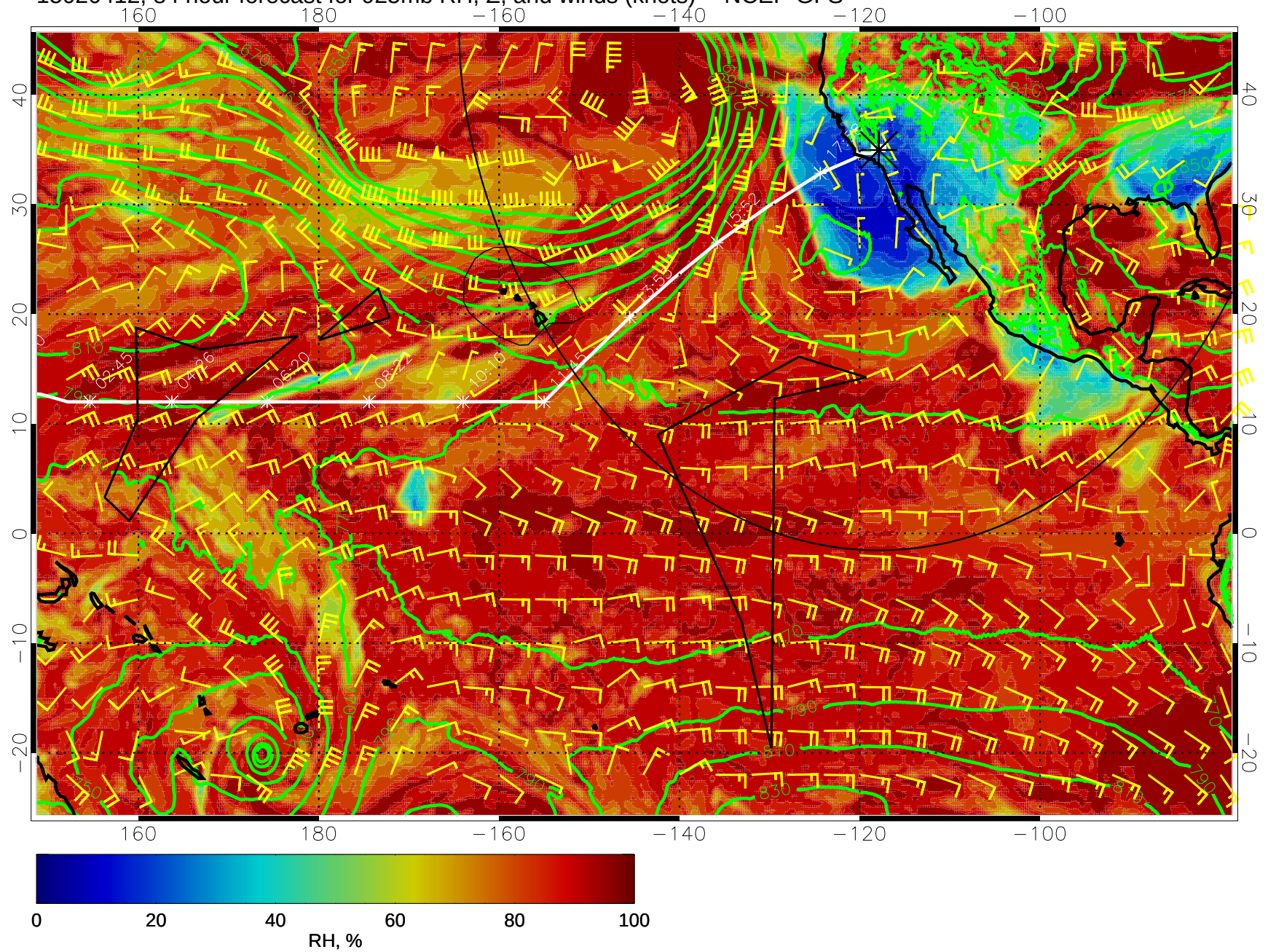
15020412, 84 hour forecast for 925mb RH, Z, and winds (knots) -- NCEP GFS
