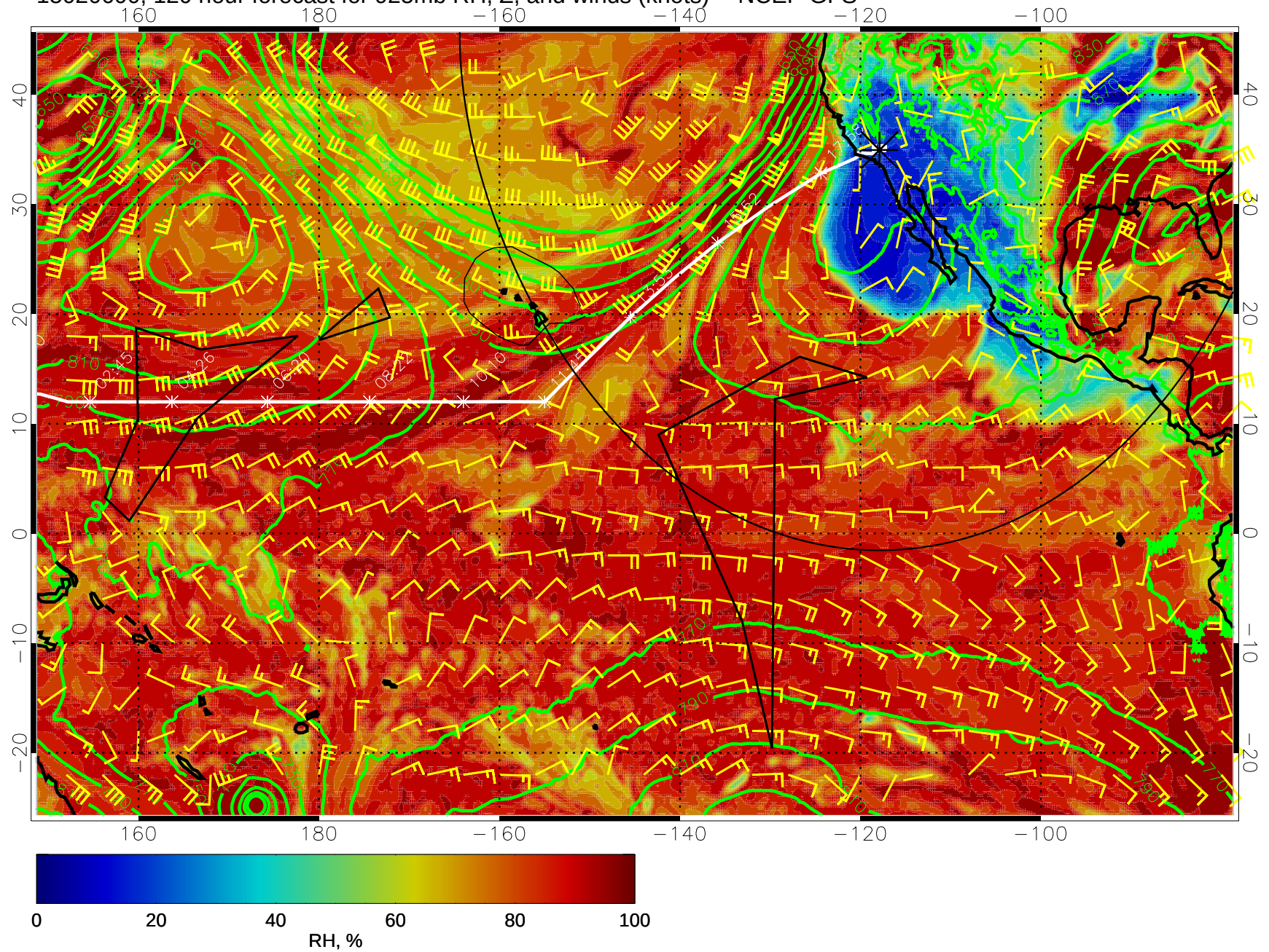
15020600, 120 hour forecast for 925mb RH, Z, and winds (knots) -- NCEP GFS
