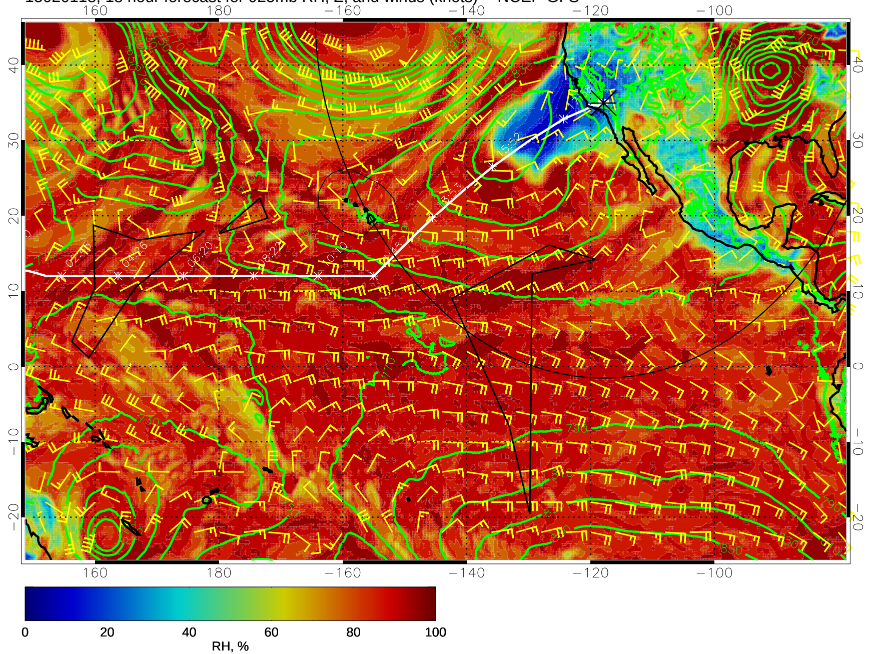
15020118, 18 hour forecast for 925mb RH, Z, and winds (knots) -- NCEP GFS
