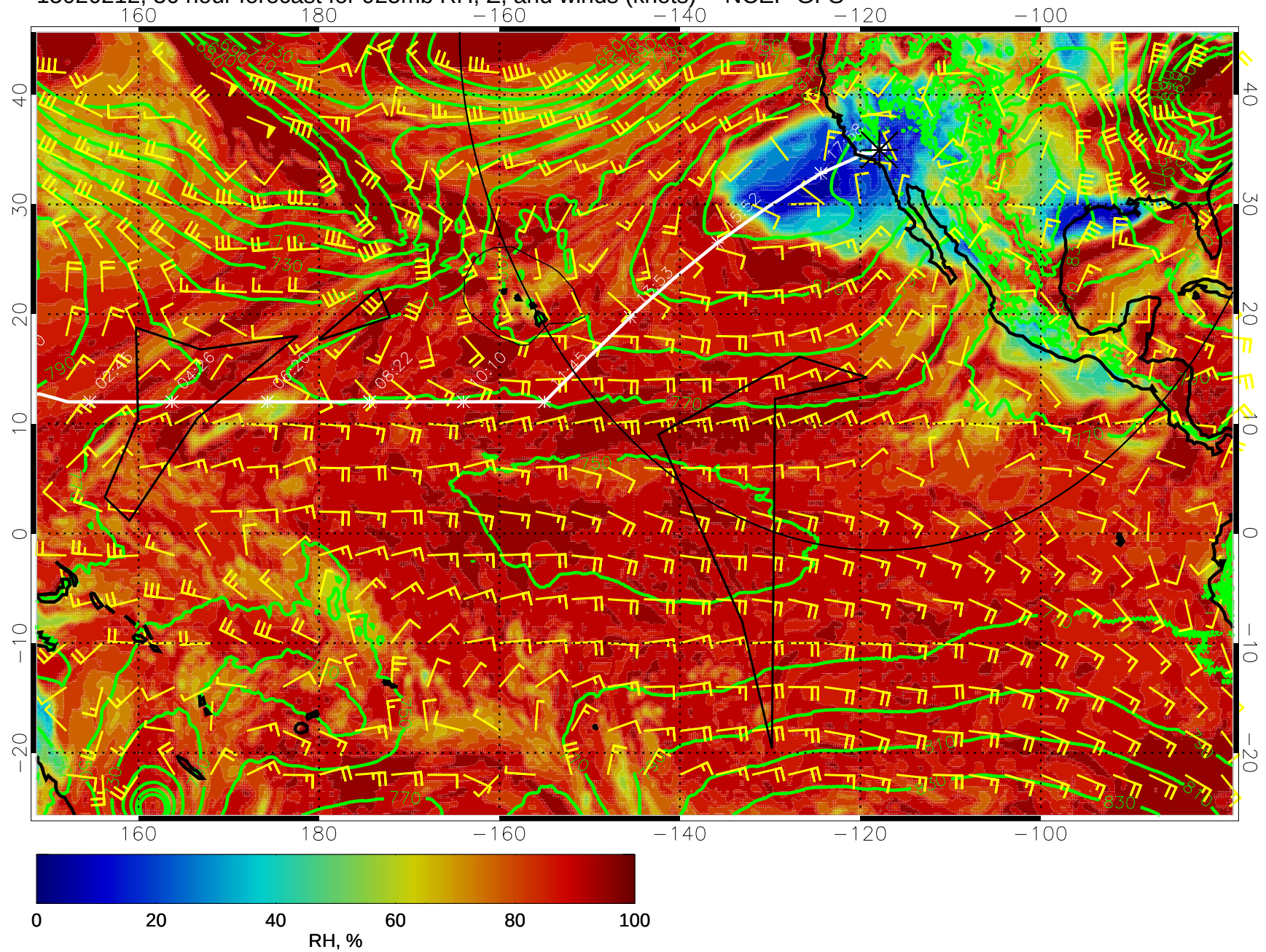
15020212, 36 hour forecast for 925mb RH, Z, and winds (knots) -- NCEP GFS
