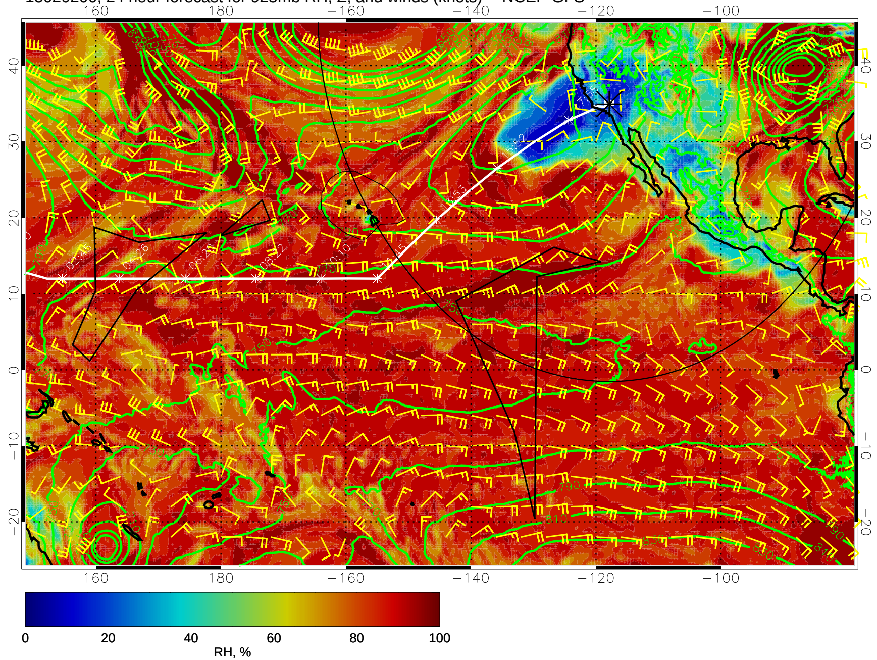
15020200, 24 hour forecast for 925mb RH, Z, and winds (knots) -- NCEP GFS
