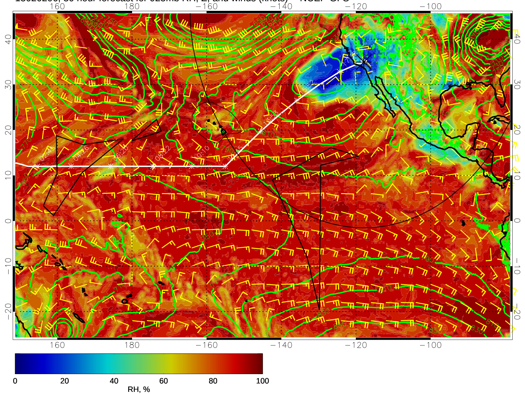
15020206, 30 hour forecast for 925mb RH, Z, and winds (knots) -- NCEP GFS
