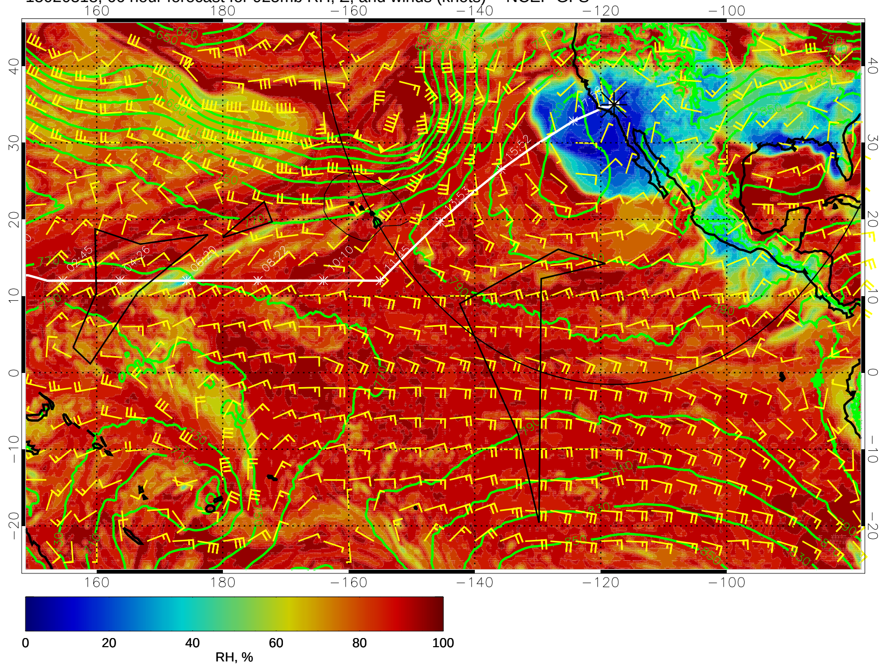
15020318, 66 hour forecast for 925mb RH, Z, and winds (knots) -- NCEP GFS
