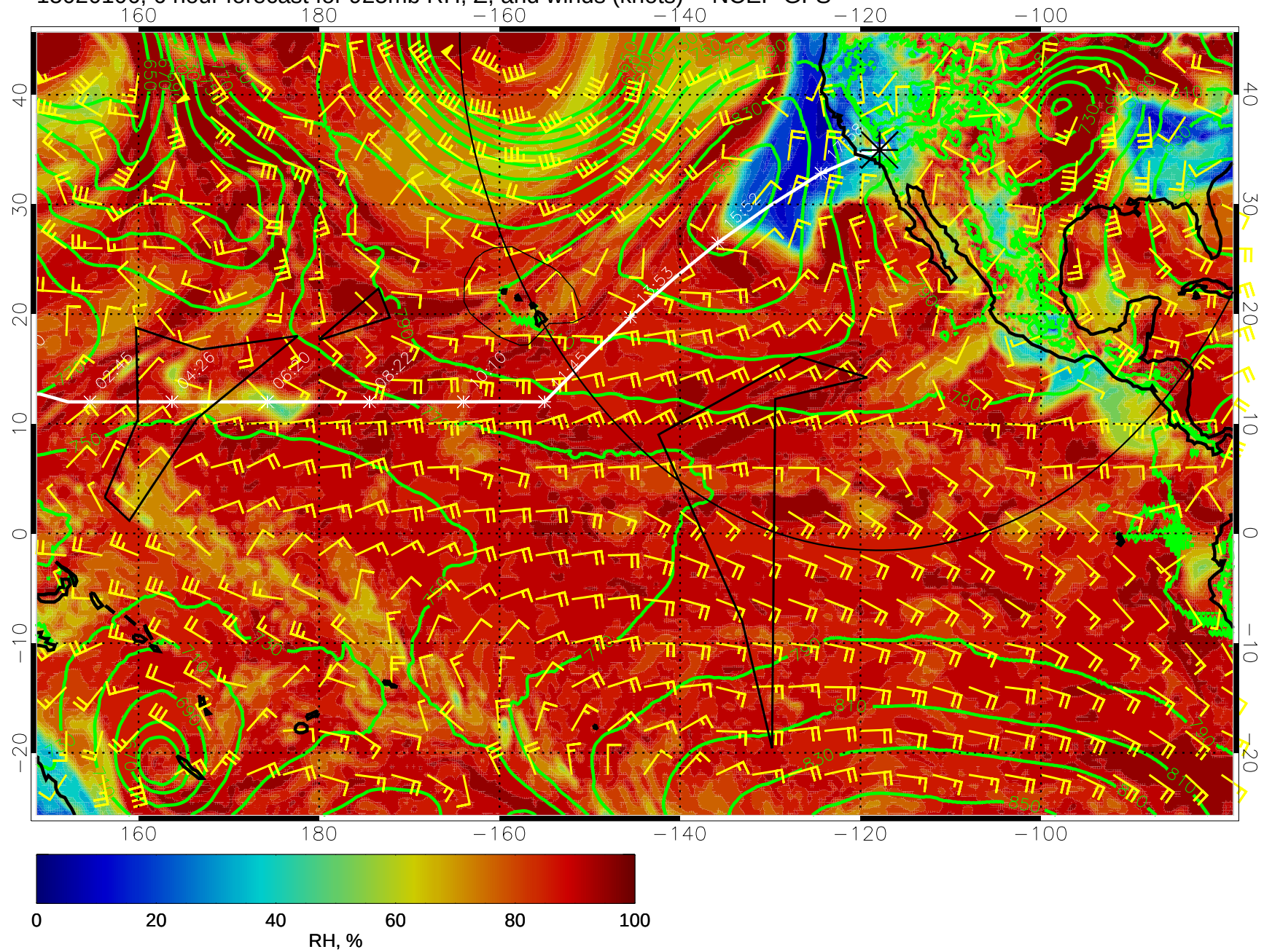
15020106, 6 hour forecast for 925mb RH, Z, and winds (knots) -- NCEP GFS
