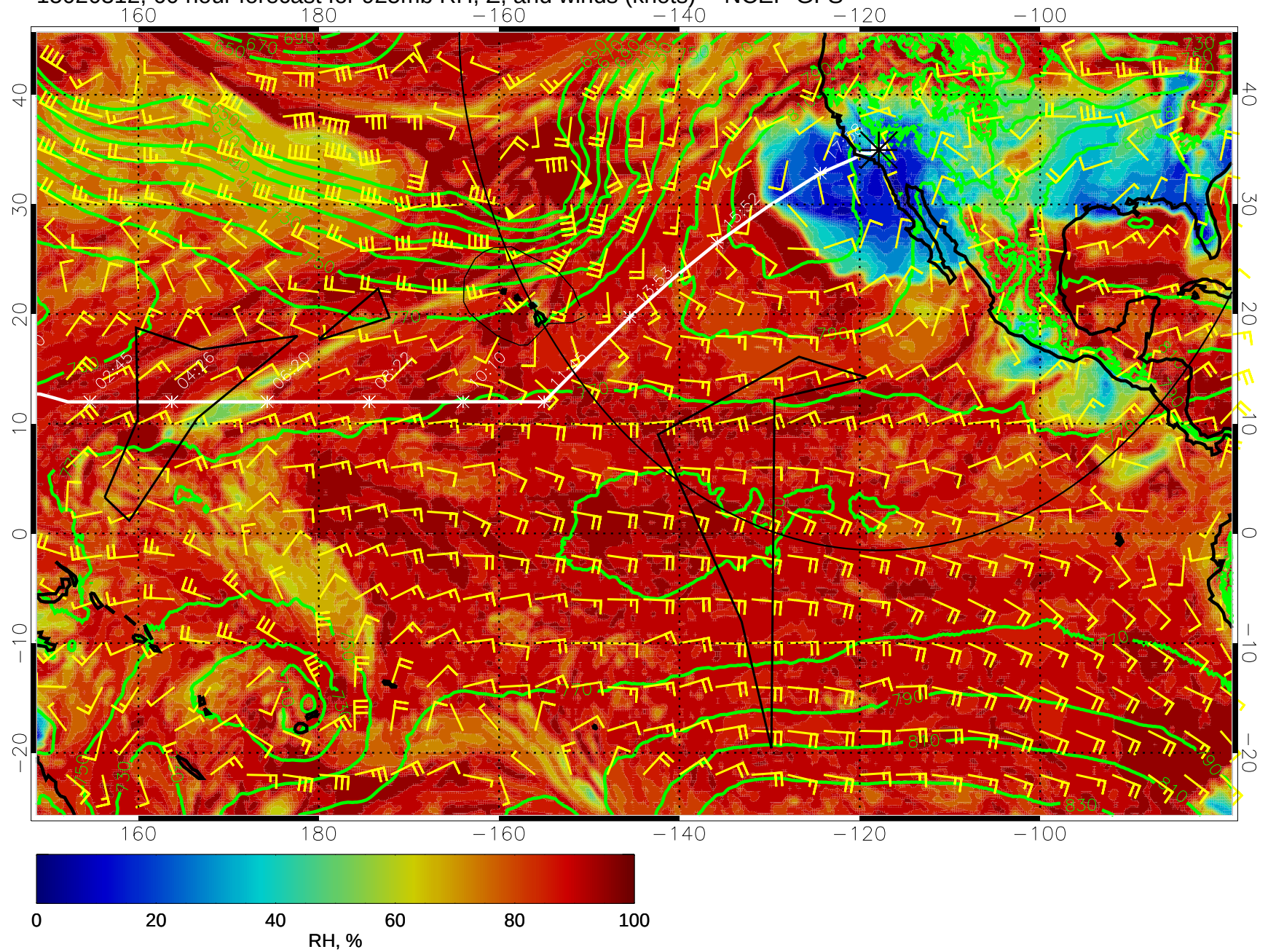
15020312, 60 hour forecast for 925mb RH, Z, and winds (knots) -- NCEP GFS
