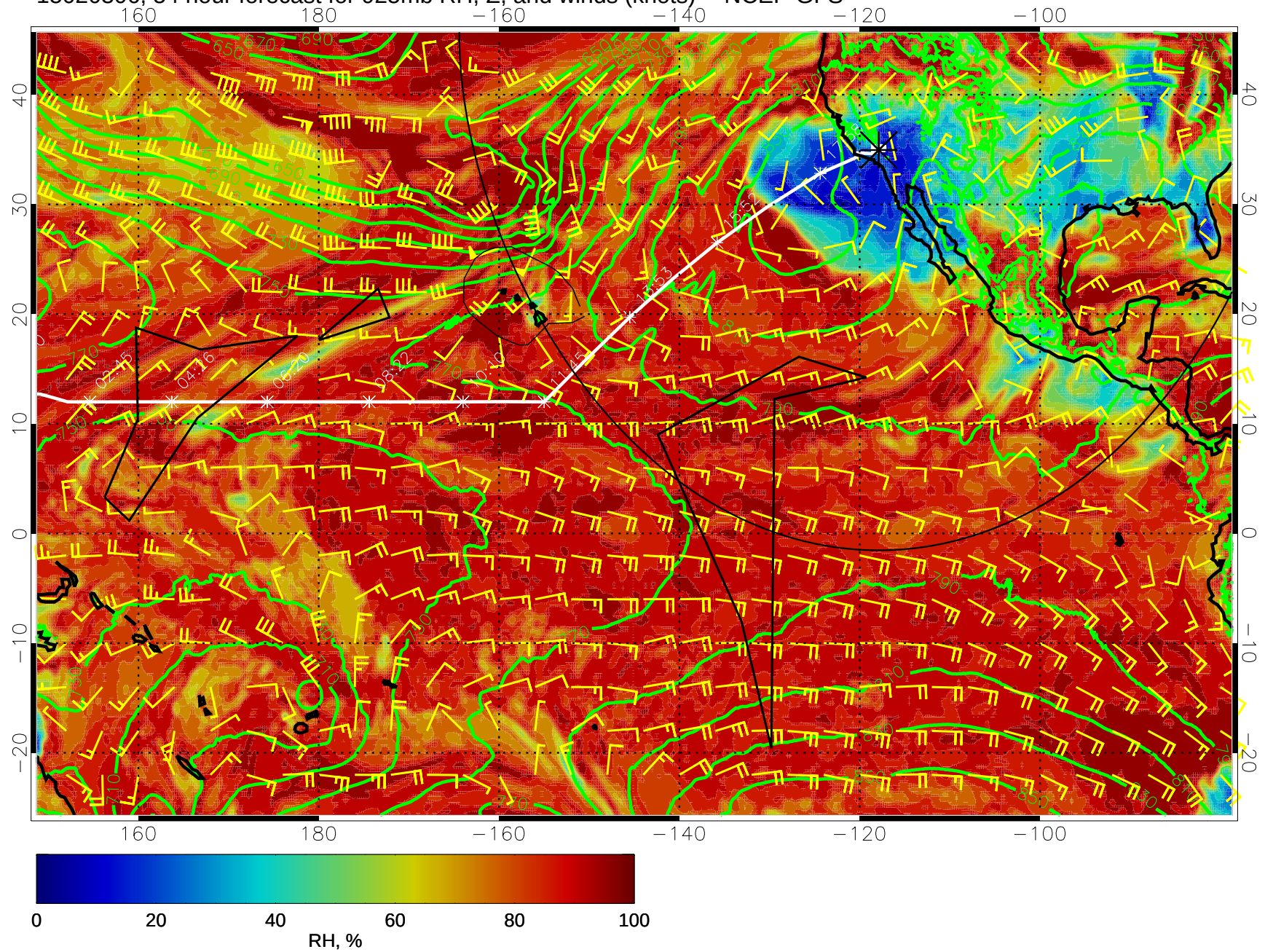
15020306, 54 hour forecast for 925mb RH, Z, and winds (knots) -- NCEP GFS
