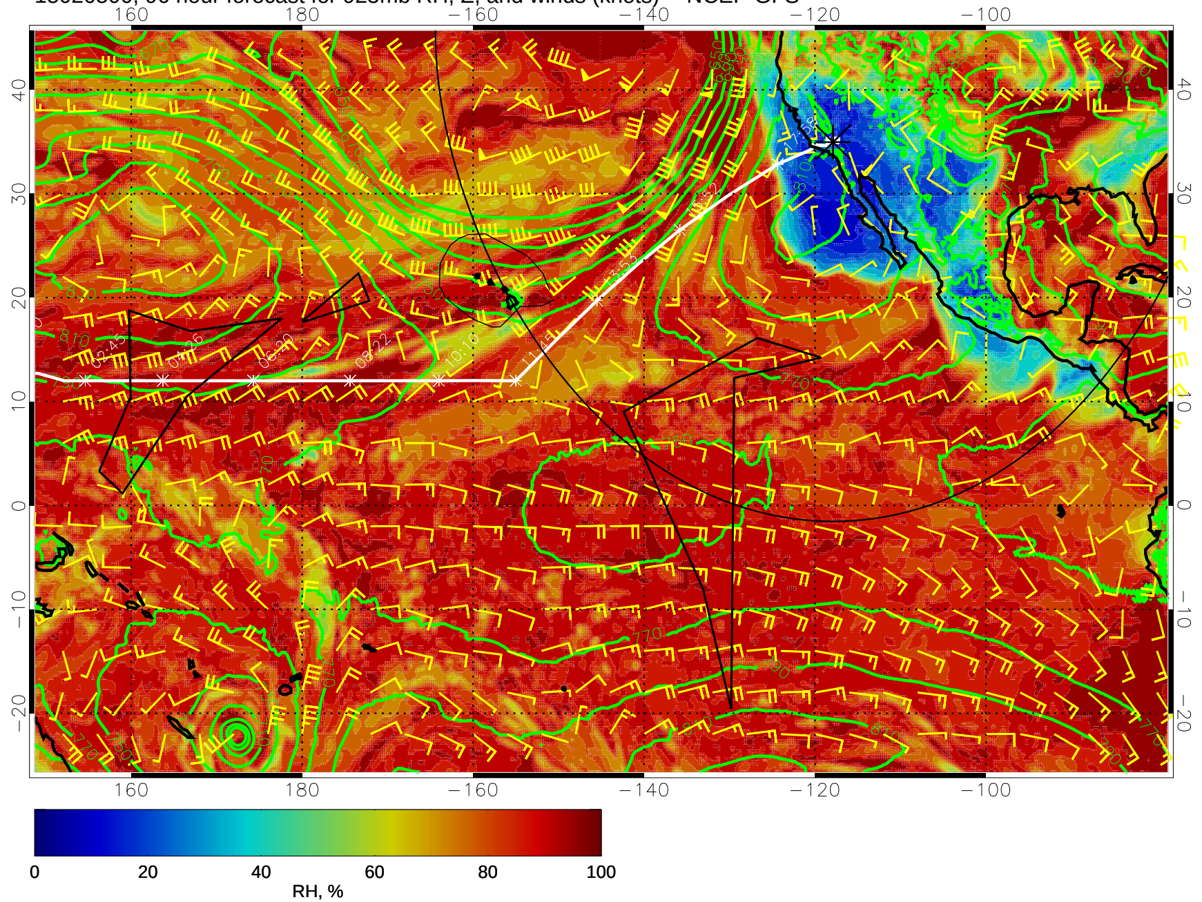
15020500, 96 hour forecast for 925mb RH, Z, and winds (knots) -- NCEP GFS
