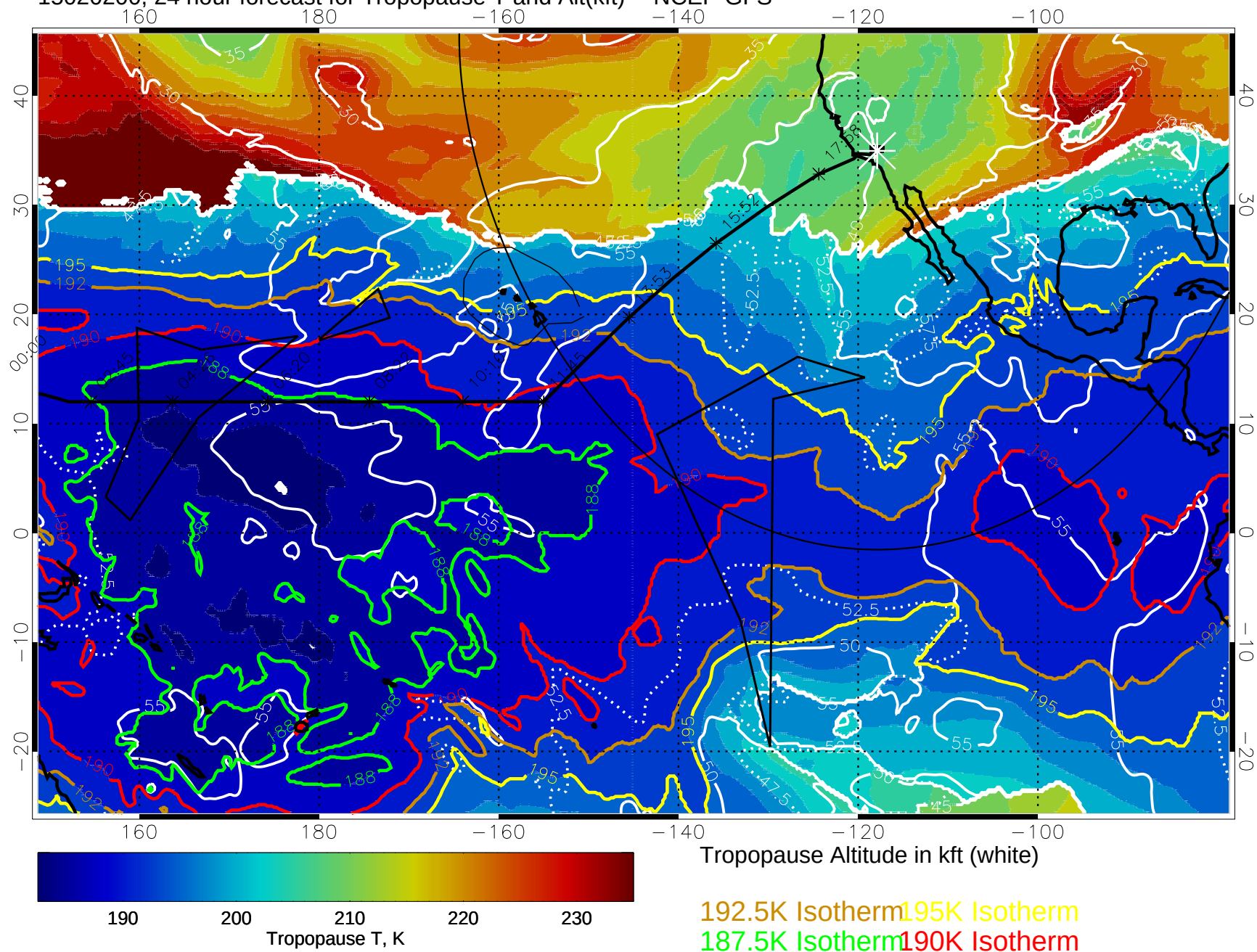
15020200, 24 hour forecast for Tropopause T and Alt(kft) -- NCEP GFS
