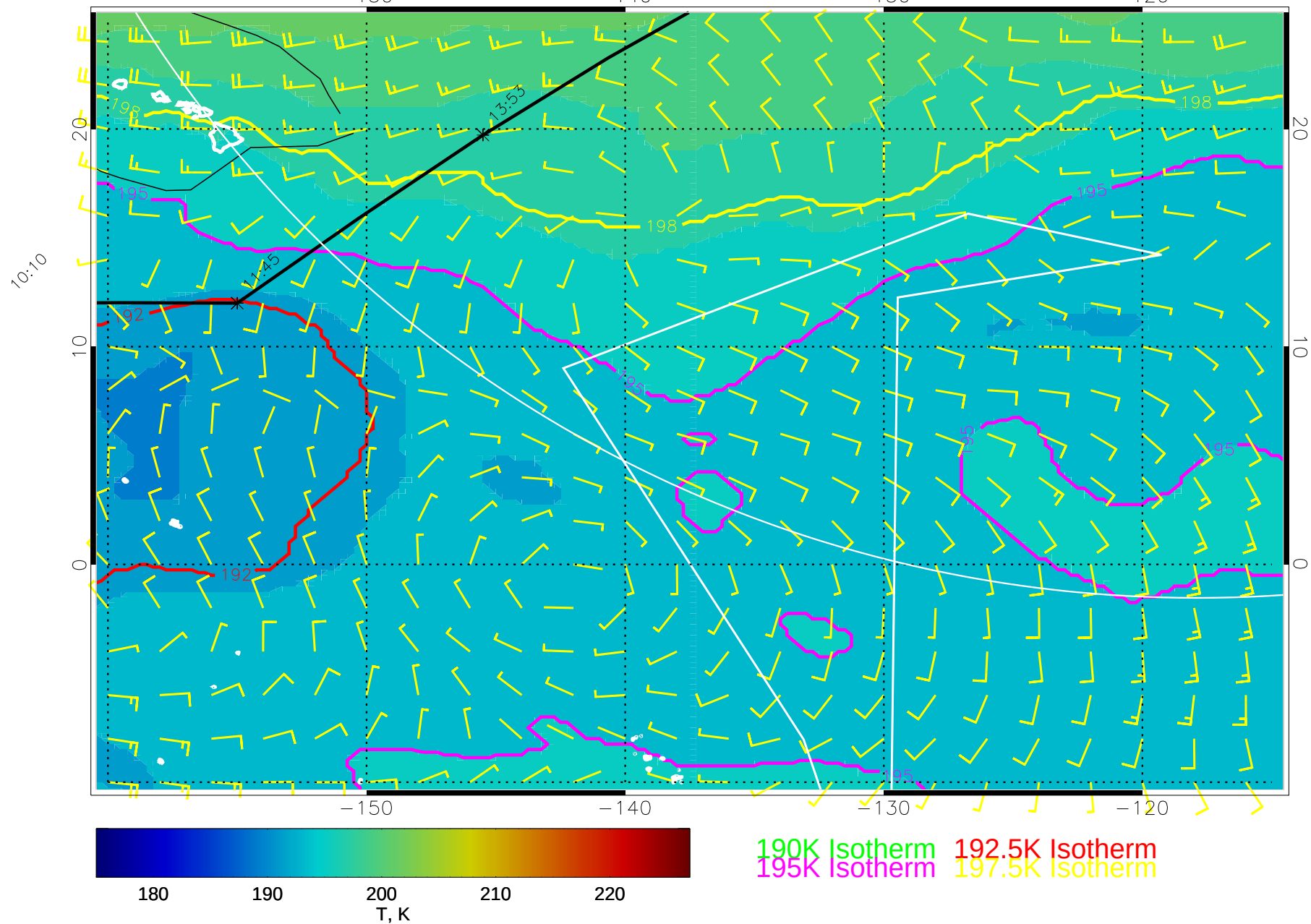
15020106, 6 hour forecast for 70mb T and winds (knots) -- NCEP GFS
