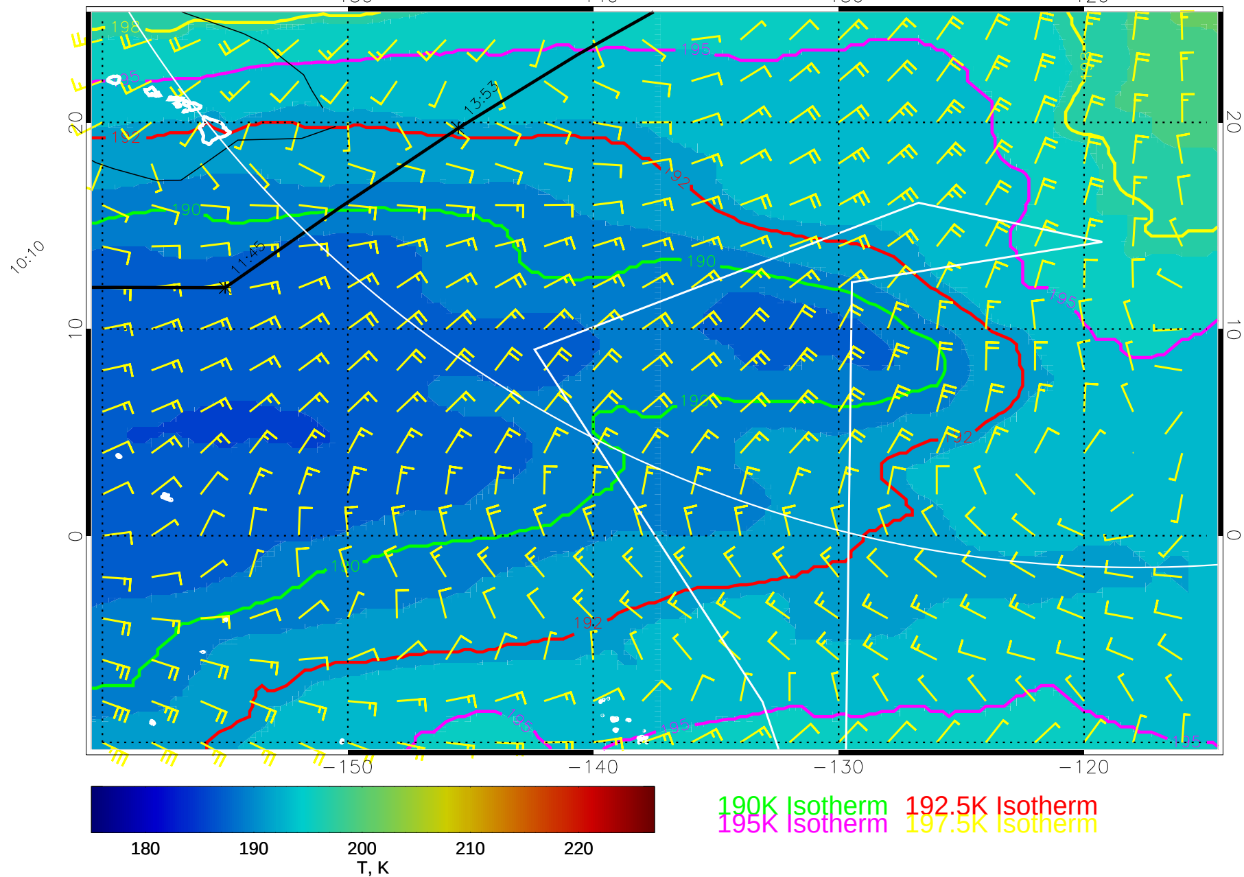
15020600, 120 hour forecast for 70mb T and winds (knots) -- NCEP GFS
