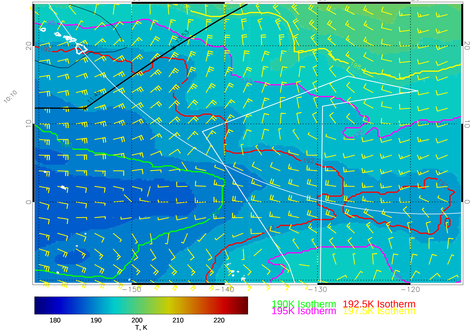
15020400, 72 hour forecast for 70mb T and winds (knots) -- NCEP GFS
