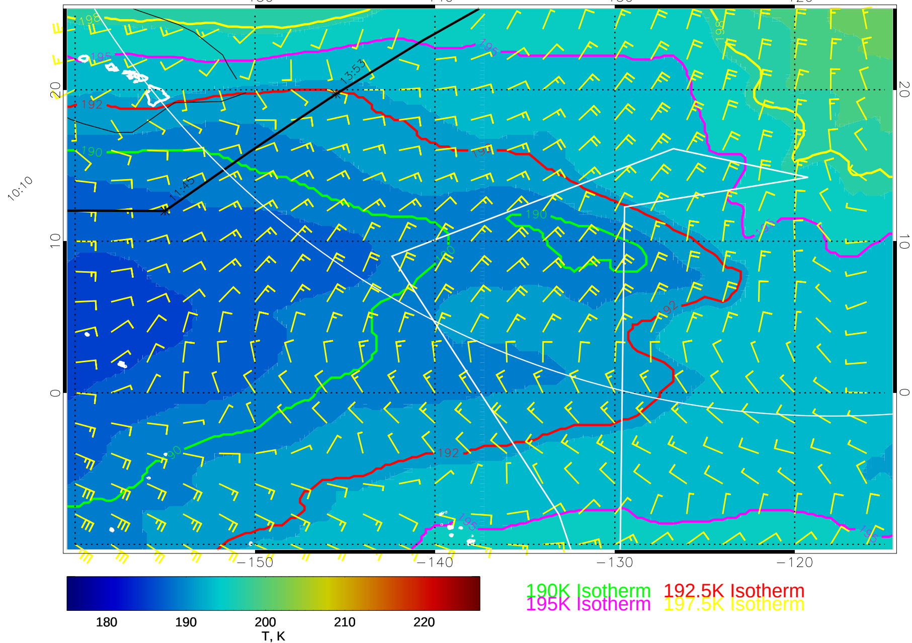
15020518, 114 hour forecast for 70mb T and winds (knots) -- NCEP GFS
