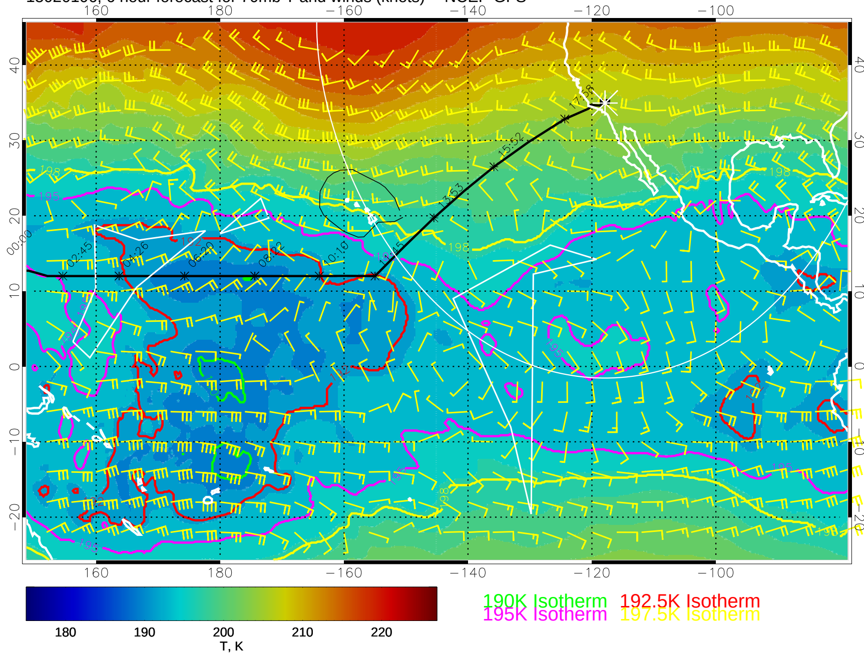
15020106, 6 hour forecast for 70mb T and winds (knots) -- NCEP GFS
