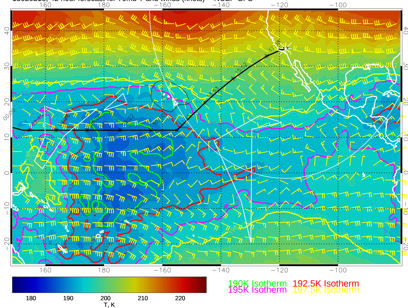
15020218, 42 hour forecast for 70mb T and winds (knots) -- NCEP GFS
