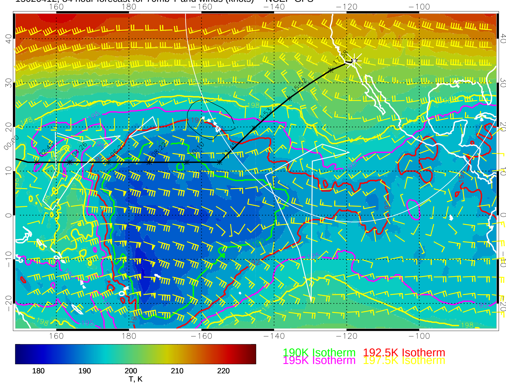
15020412, 84 hour forecast for 70mb T and winds (knots) -- NCEP GFS
