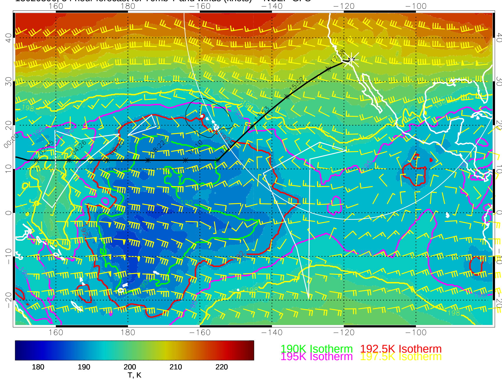
15020306, 54 hour forecast for 70mb T and winds (knots) -- NCEP GFS
