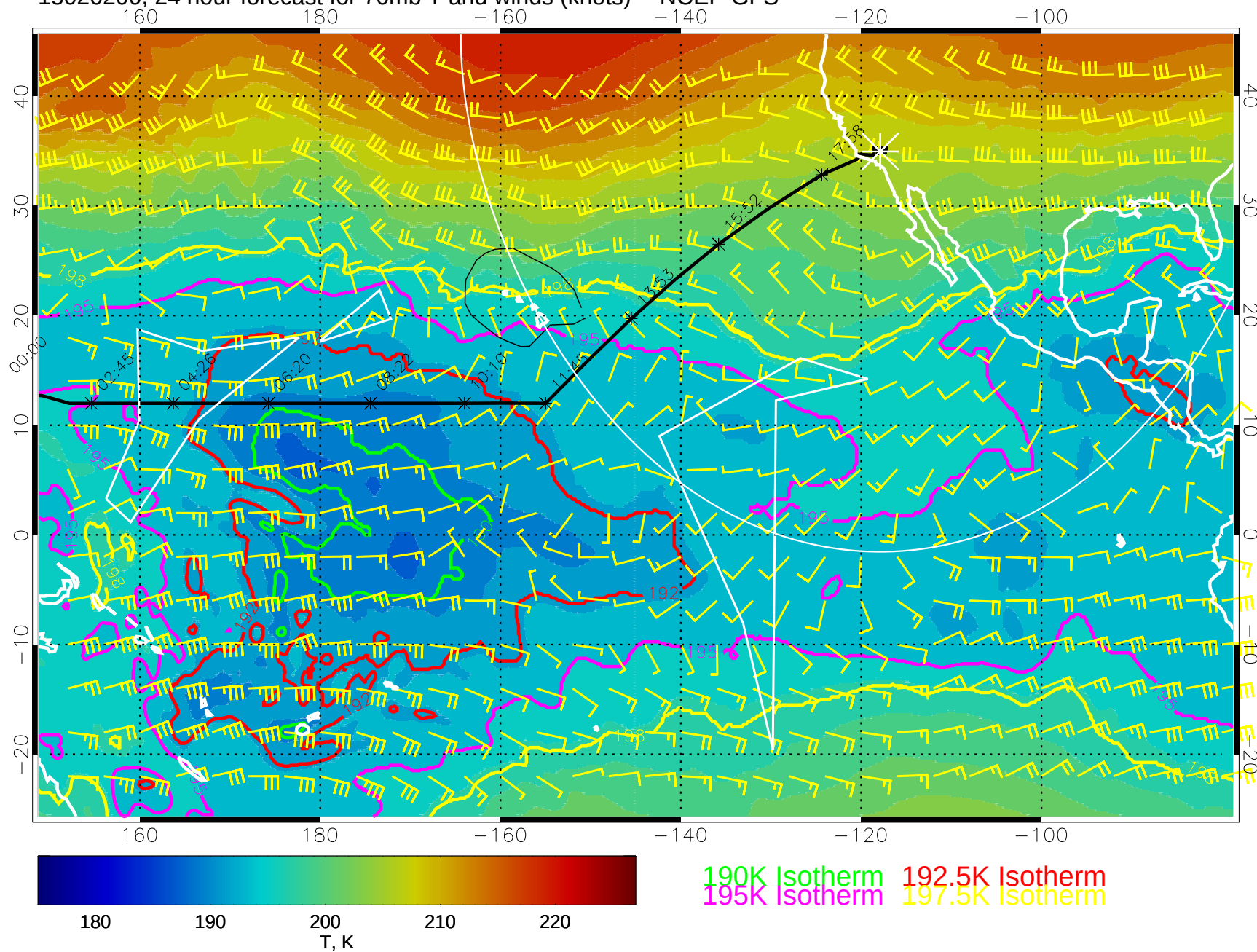
15020200, 24 hour forecast for 70mb T and winds (knots) -- NCEP GFS
