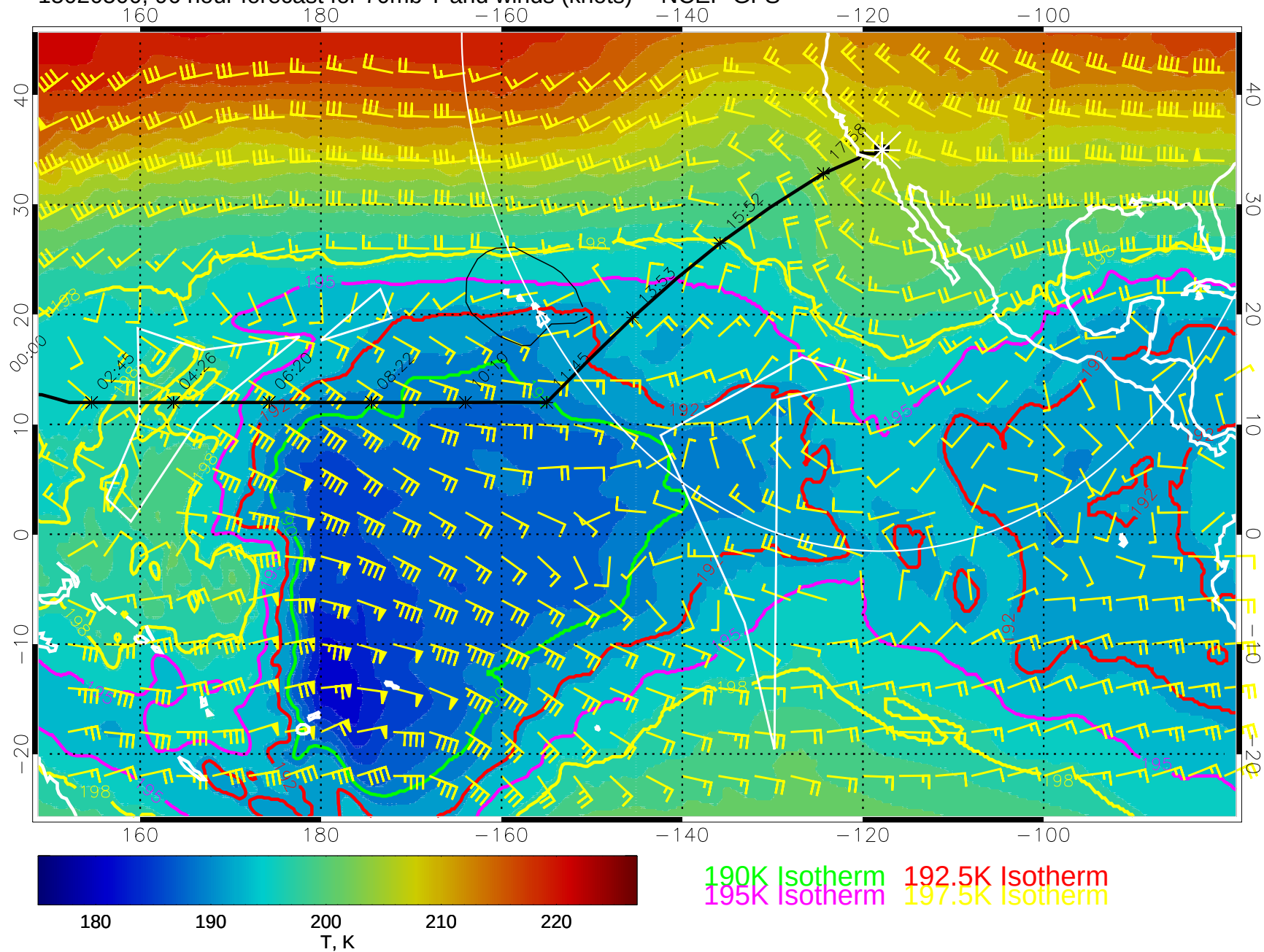
15020500, 96 hour forecast for 70mb T and winds (knots) -- NCEP GFS
