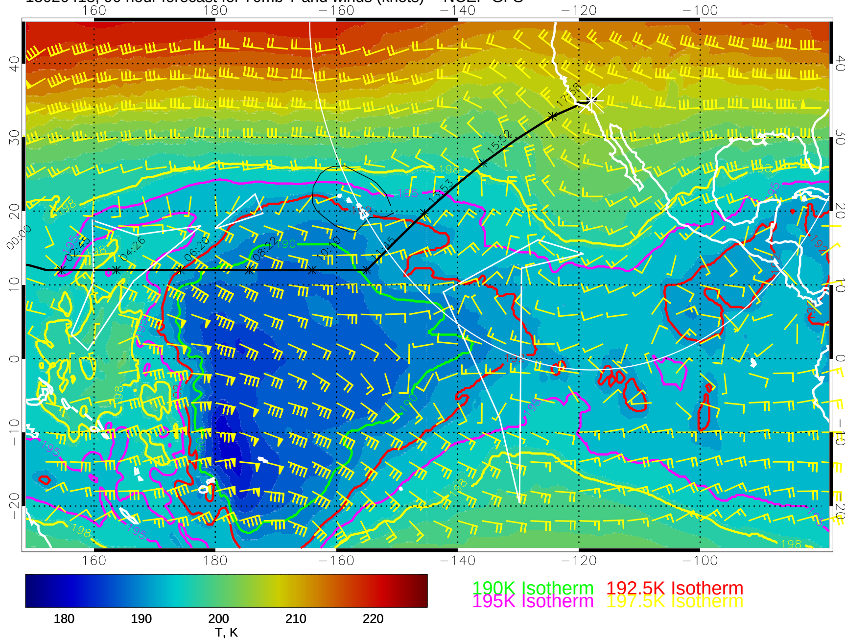
15020418, 90 hour forecast for 70mb T and winds (knots) -- NCEP GFS
