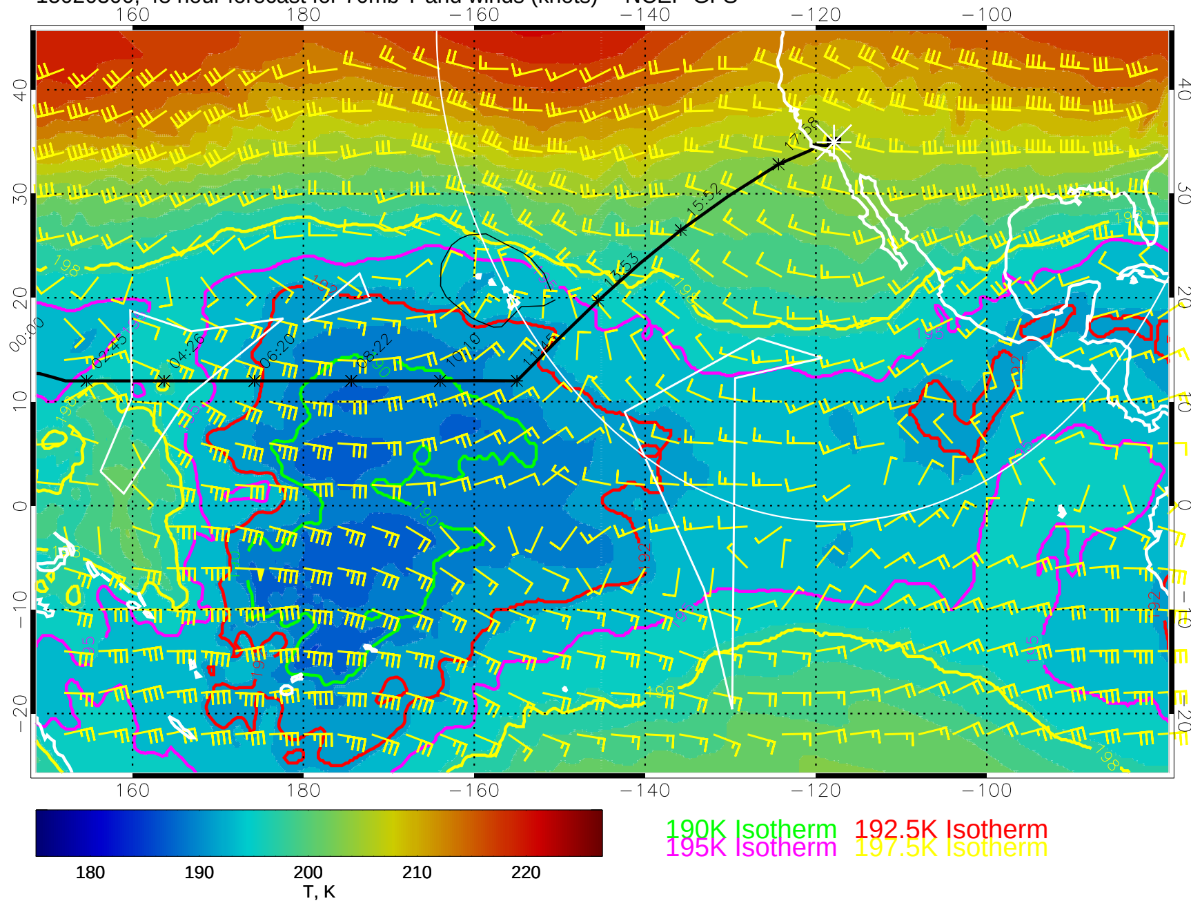
15020300, 48 hour forecast for 70mb T and winds (knots) -- NCEP GFS
