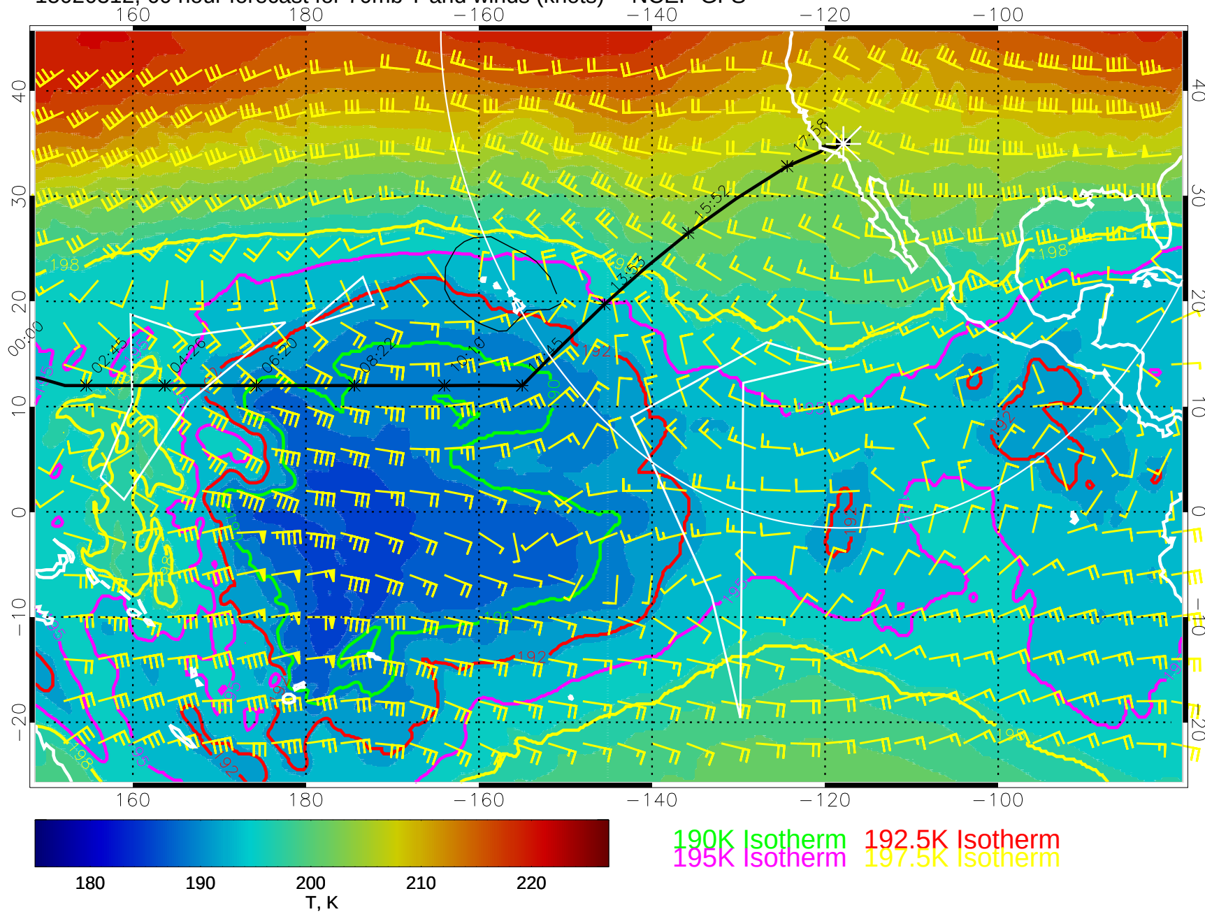
15020312, 60 hour forecast for 70mb T and winds (knots) -- NCEP GFS
