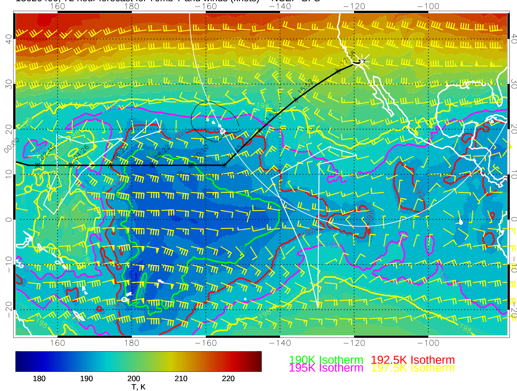
15020400, 72 hour forecast for 70mb T and winds (knots) -- NCEP GFS
