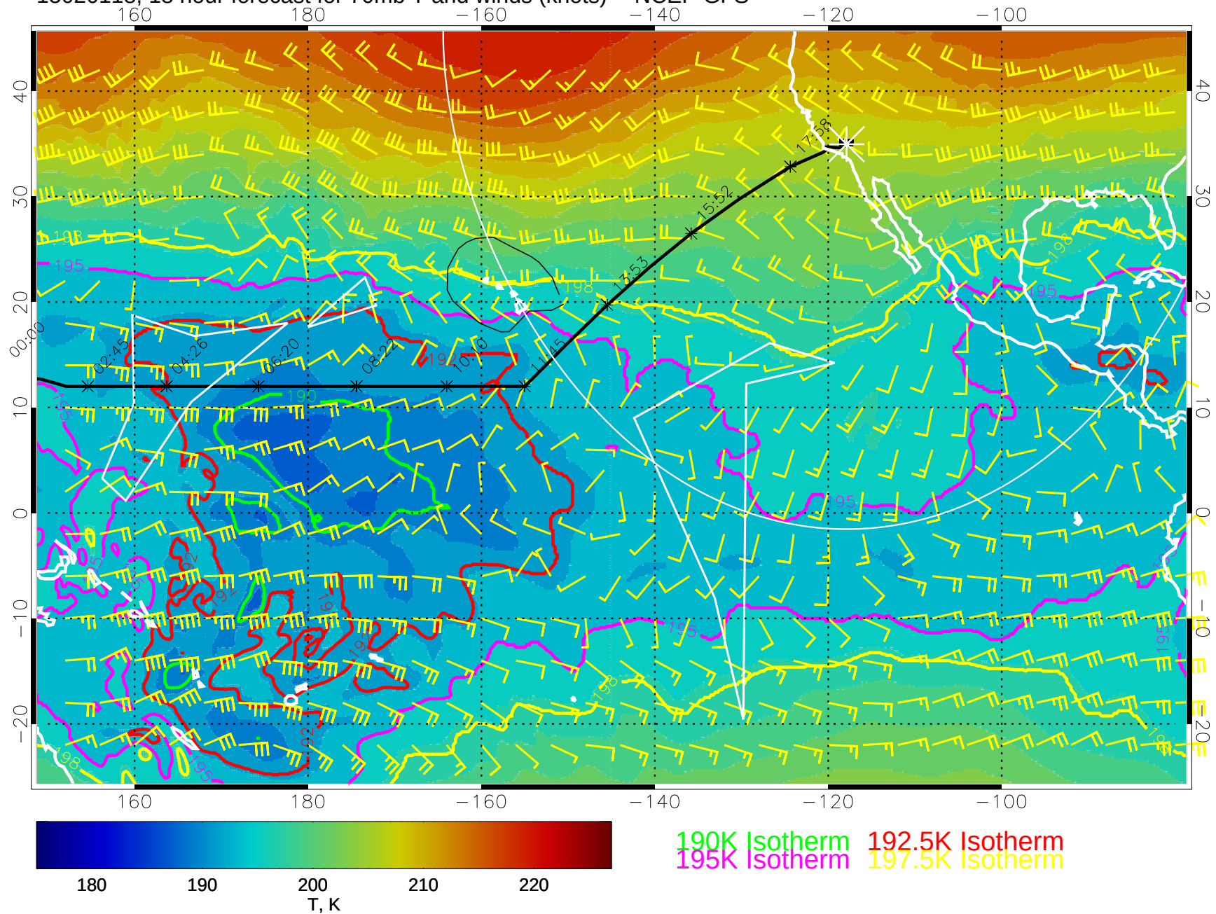
15020118, 18 hour forecast for 70mb T and winds (knots) -- NCEP GFS
