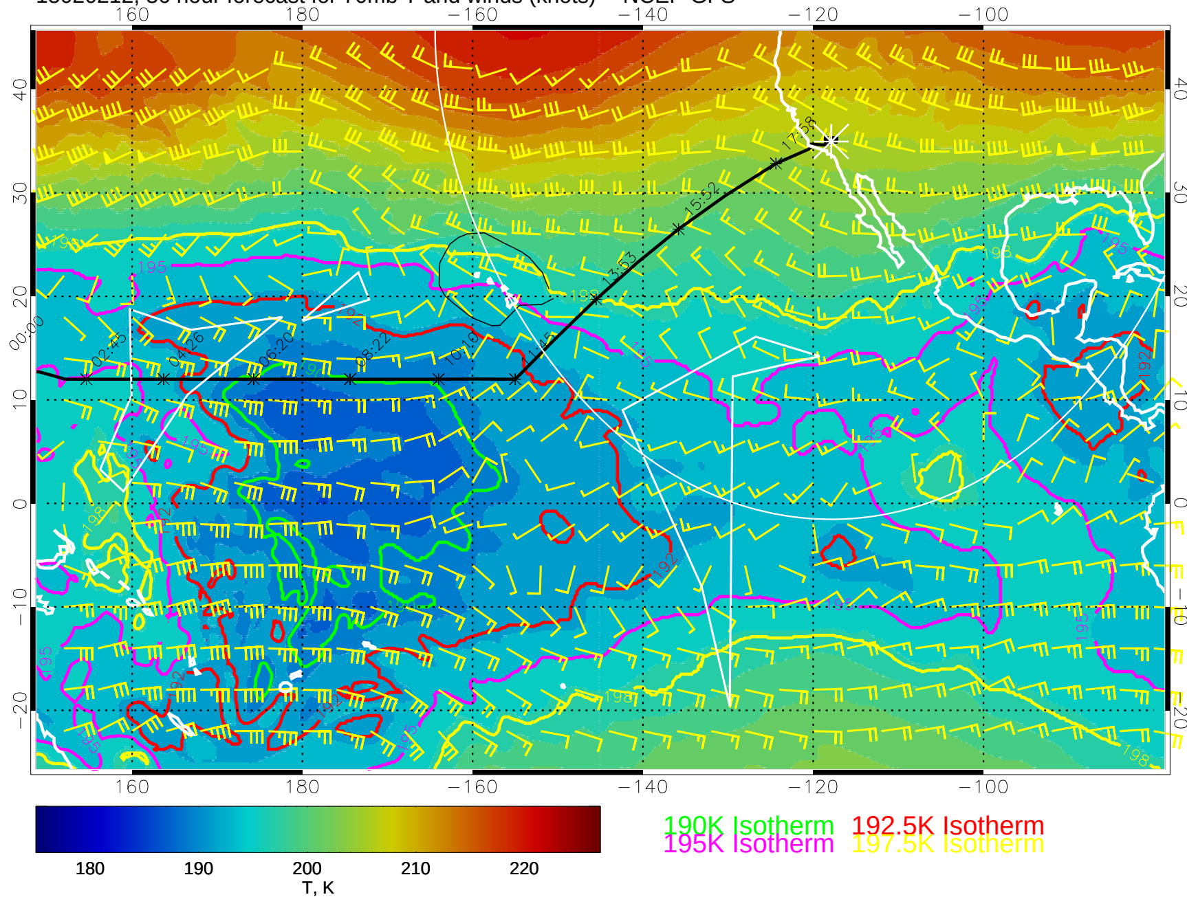
15020212, 36 hour forecast for 70mb T and winds (knots) -- NCEP GFS
