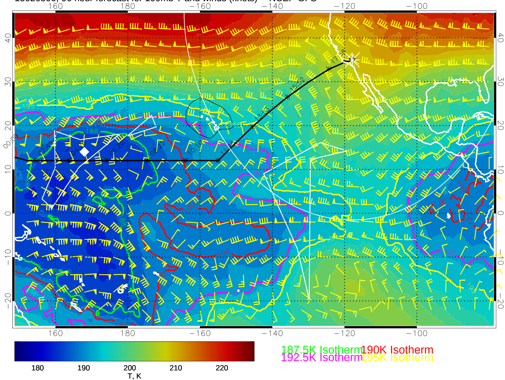
15020500, 96 hour forecast for 100mb T and winds (knots) -- NCEP GFS
