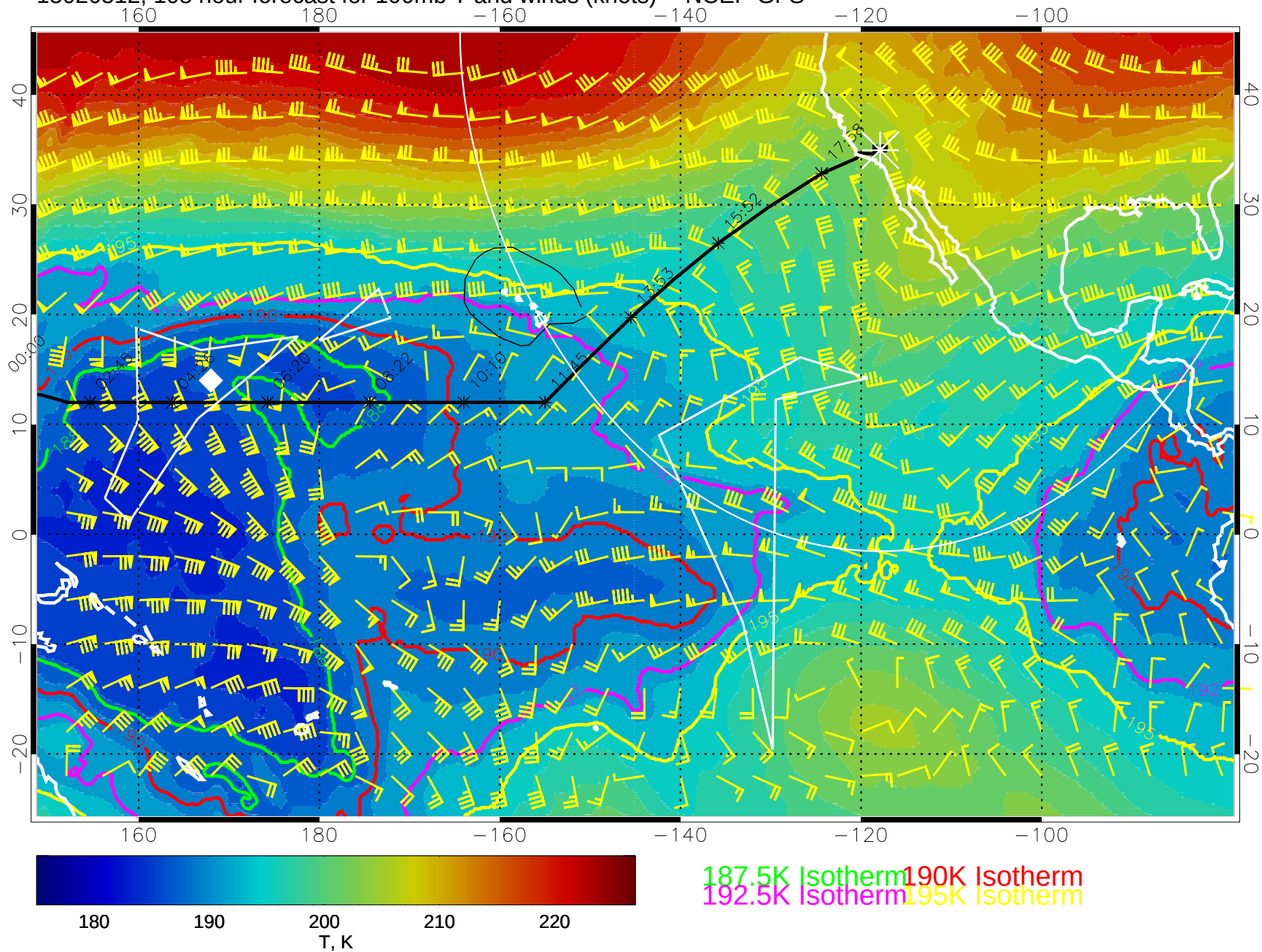
15020512, 108 hour forecast for 100mb T and winds (knots) -- NCEP GFS
