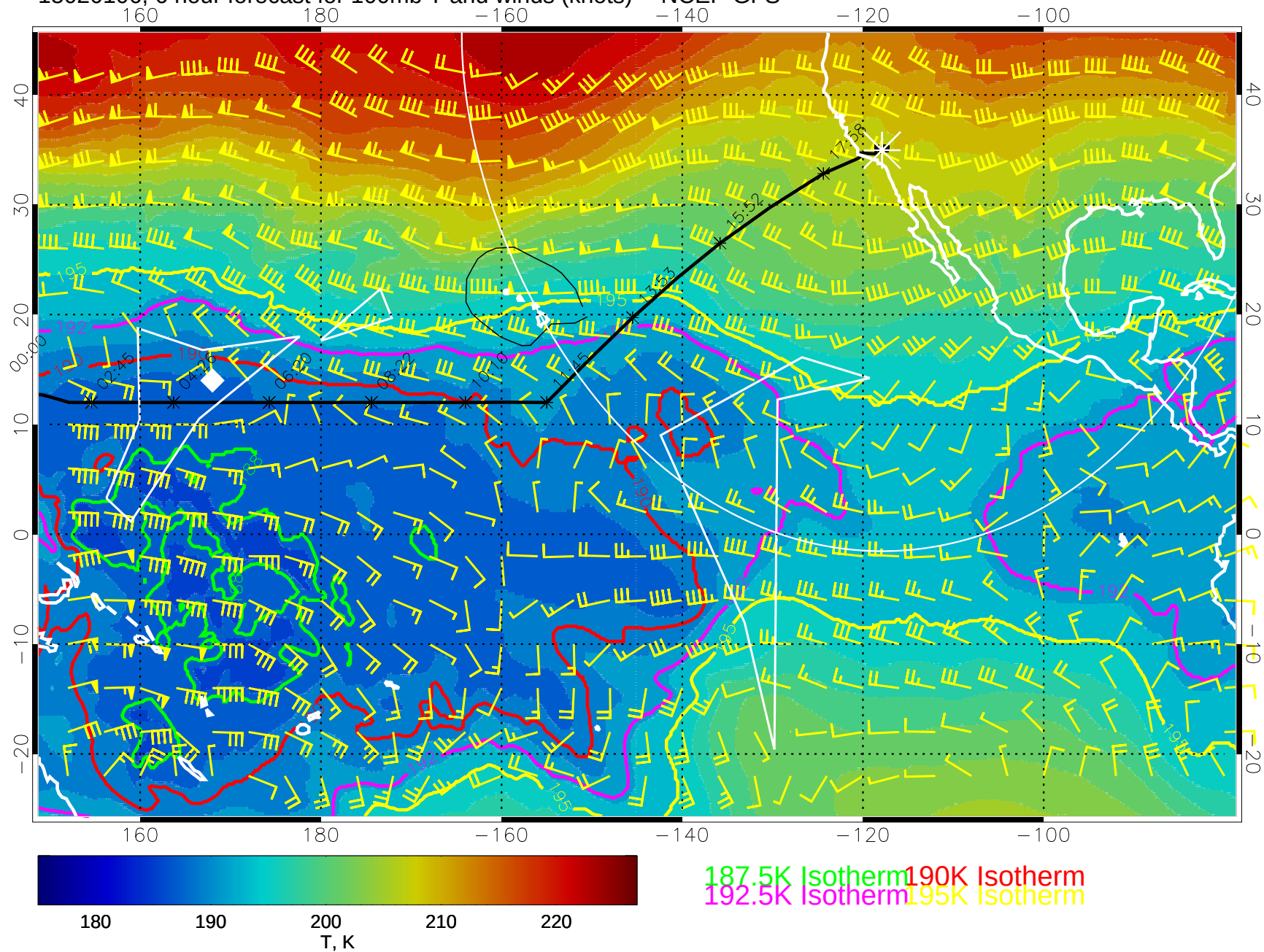
15020106, 6 hour forecast for 100mb T and winds (knots) -- NCEP GFS
