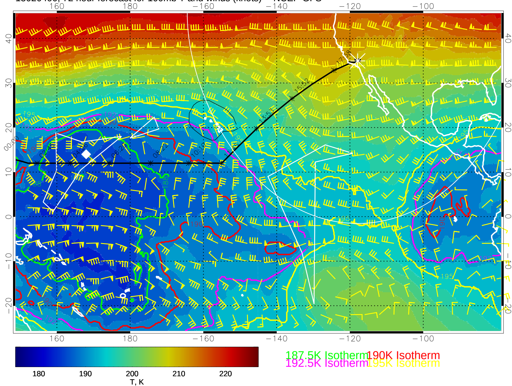
15020400, 72 hour forecast for 100mb T and winds (knots) -- NCEP GFS
