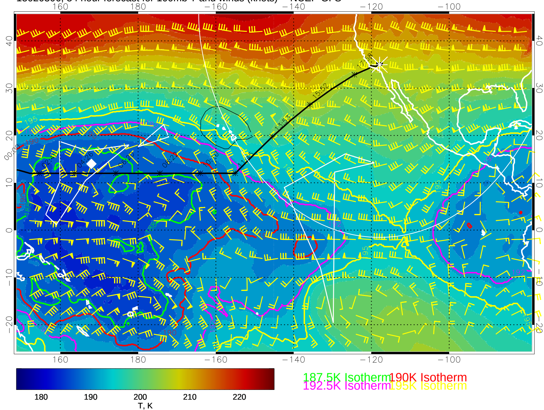
15020306, 54 hour forecast for 100mb T and winds (knots) -- NCEP GFS
