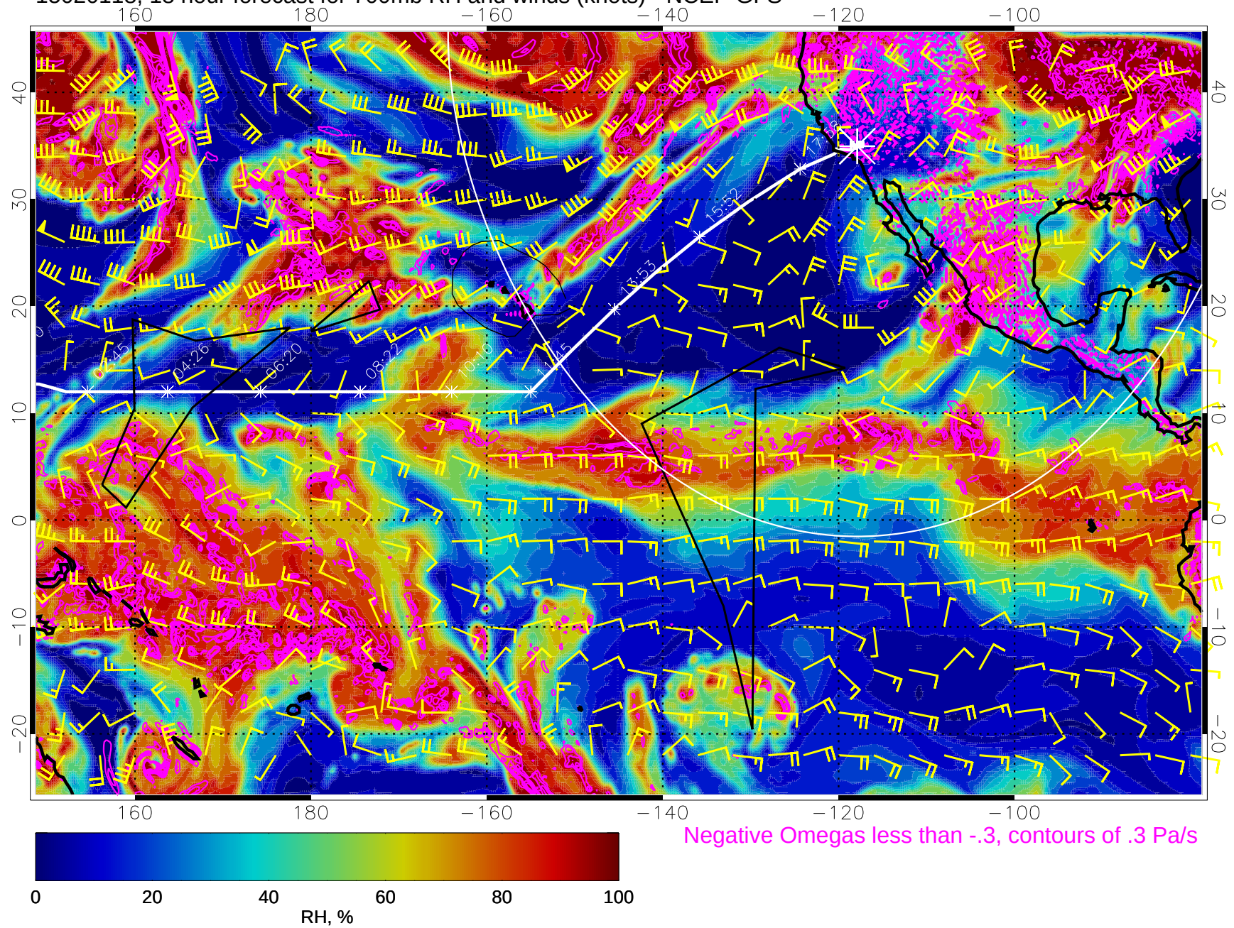
15020118, 18 hour forecast for 700mb RH and winds (knots) - NCEP GFS
