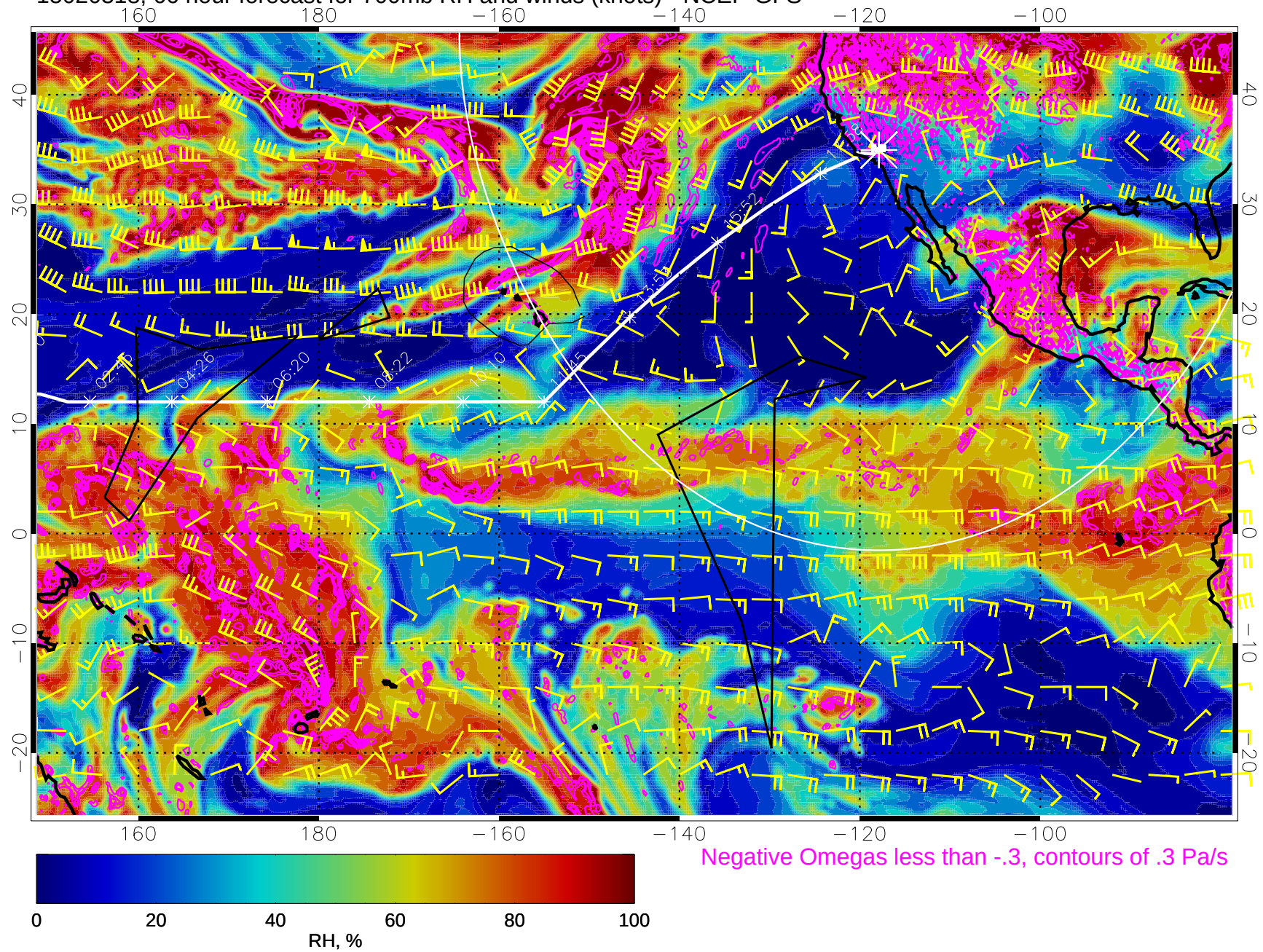
15020318, 66 hour forecast for 700mb RH and winds (knots) - NCEP GFS
