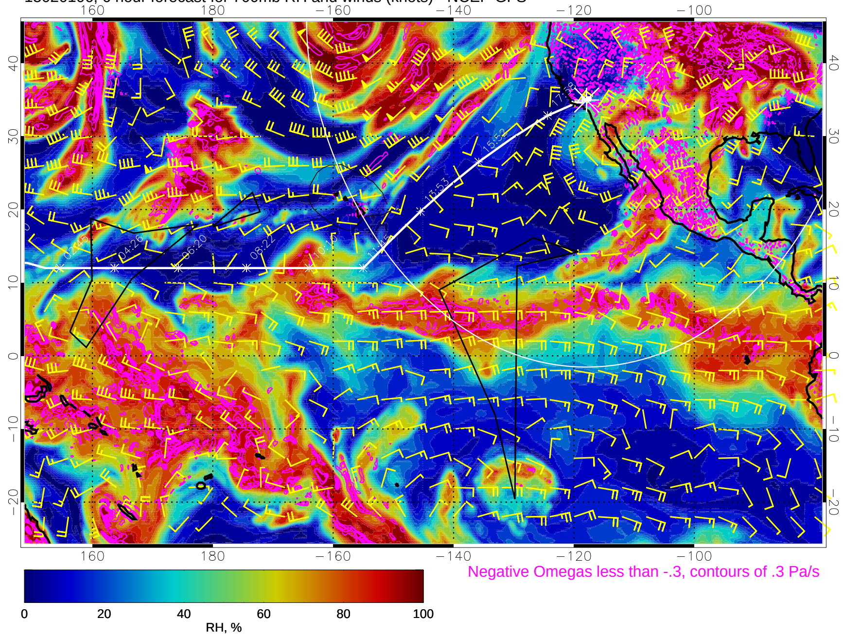
15020106, 6 hour forecast for 700mb RH and winds (knots) - NCEP GFS
