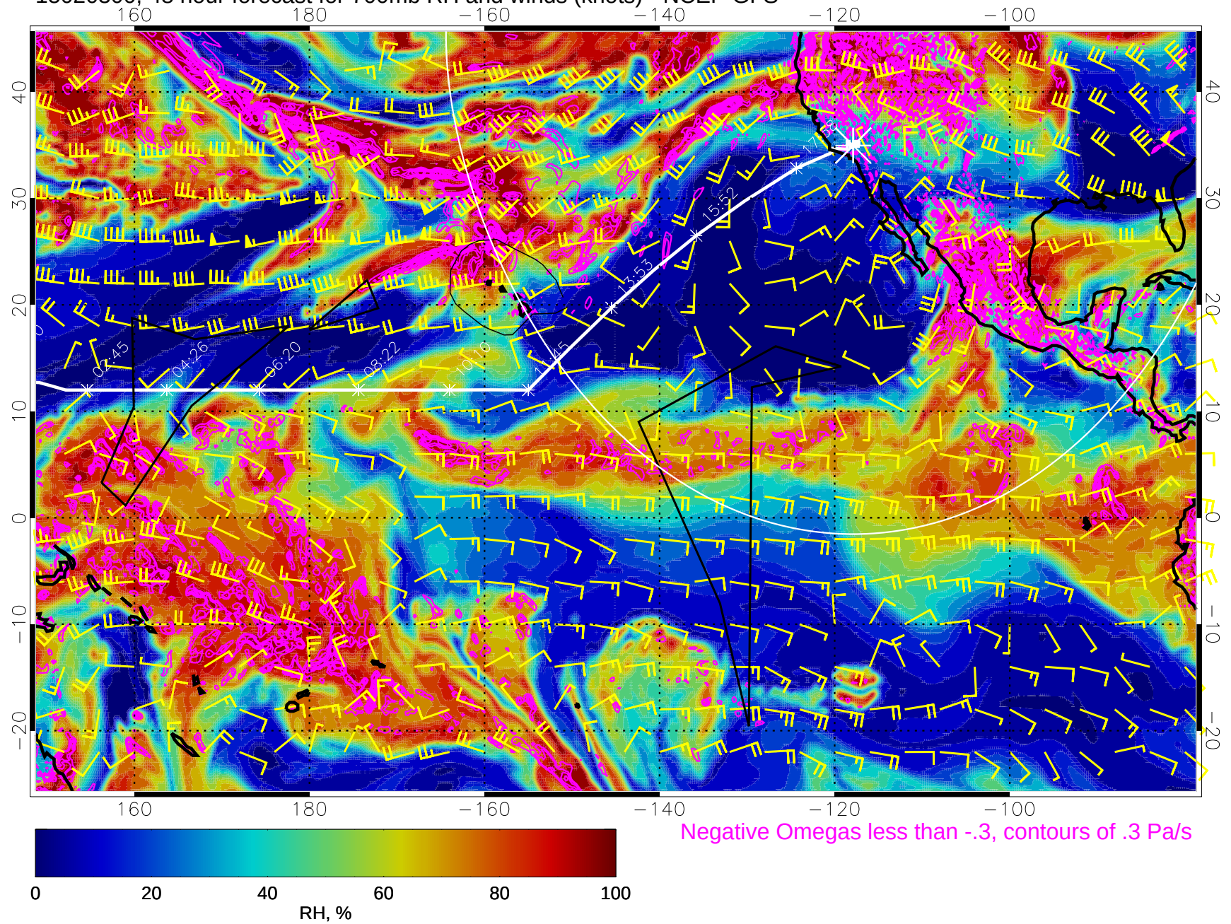
15020300, 48 hour forecast for 700mb RH and winds (knots) - NCEP GFS
