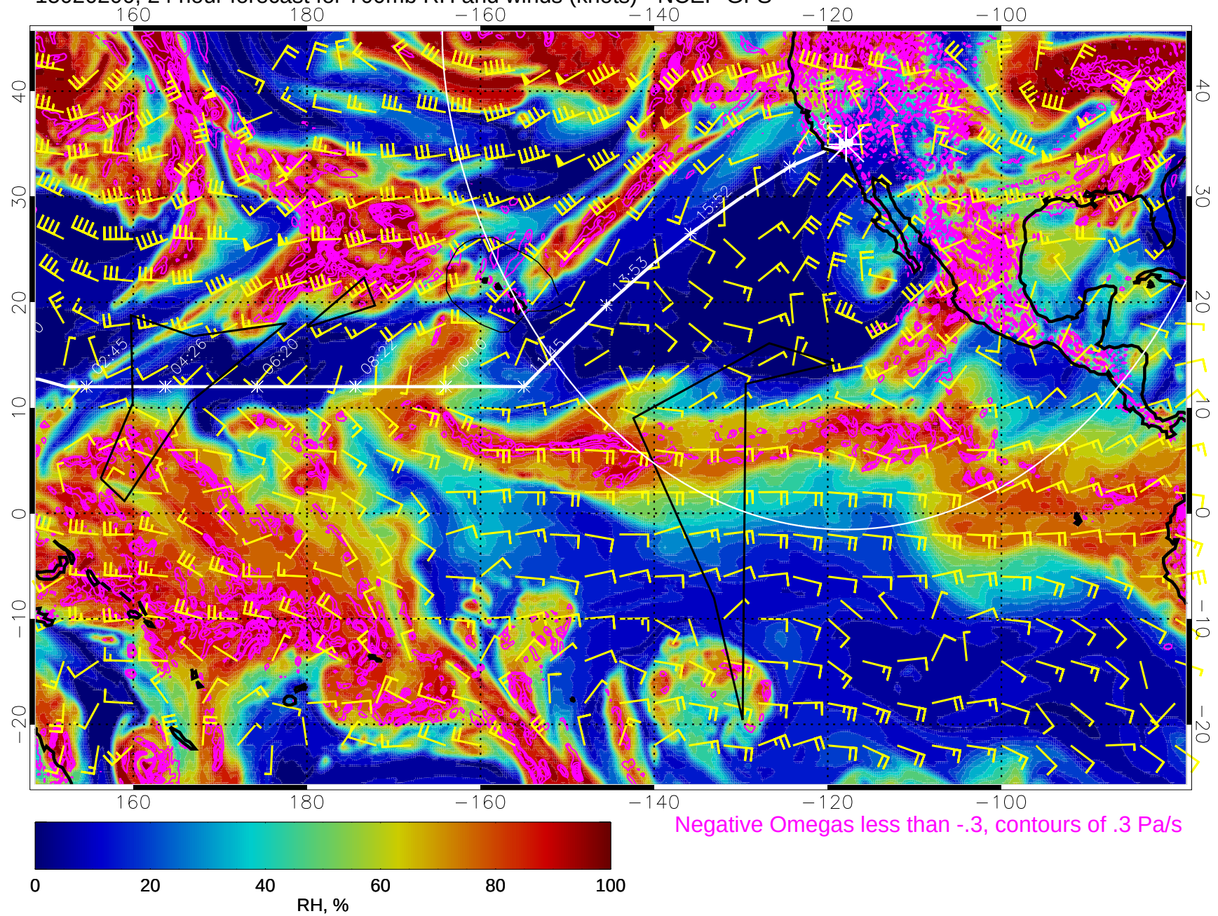
15020200, 24 hour forecast for 700mb RH and winds (knots) - NCEP GFS
