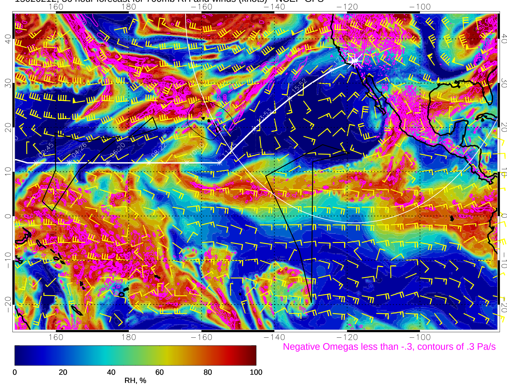
15020212, 36 hour forecast for 700mb RH and winds (knots) - NCEP GFS
