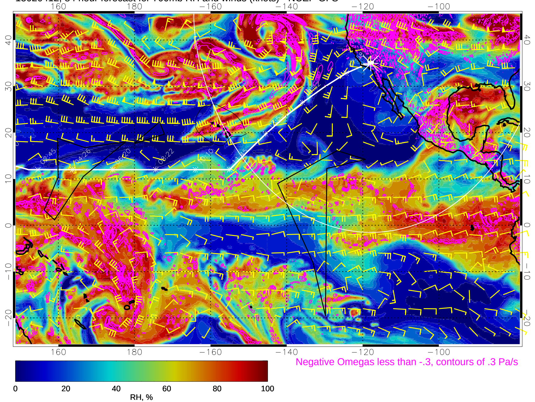
15020412, 84 hour forecast for 700mb RH and winds (knots) - NCEP GFS
