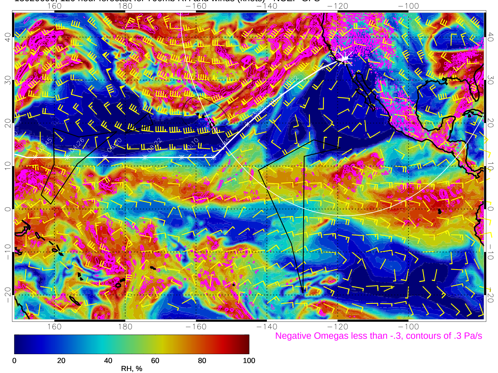
15020600, 120 hour forecast for 700mb RH and winds (knots) - NCEP GFS
