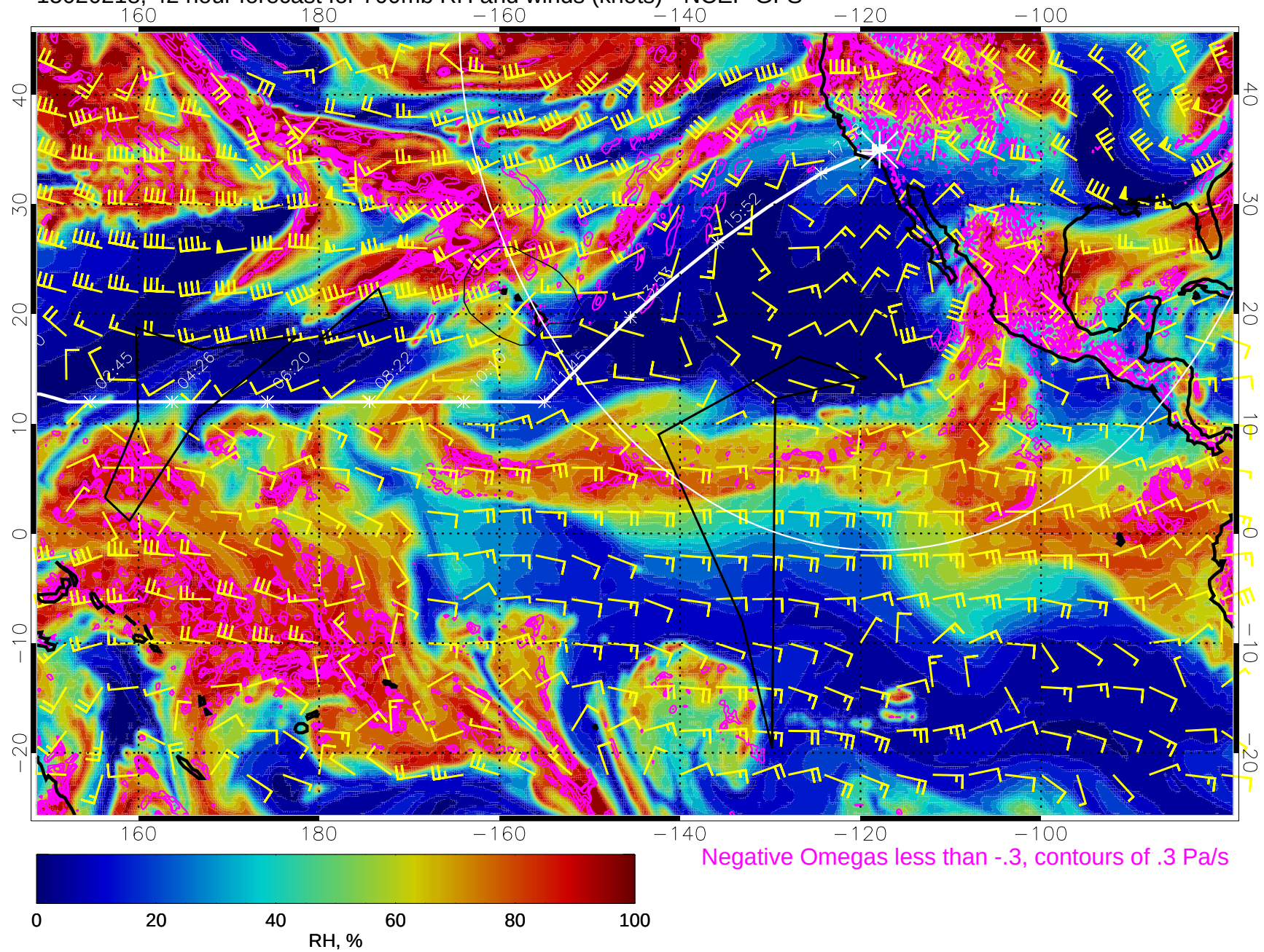
15020218, 42 hour forecast for 700mb RH and winds (knots) - NCEP GFS
