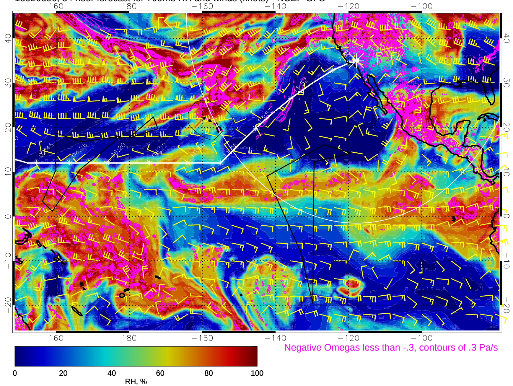
15020306, 54 hour forecast for 700mb RH and winds (knots) - NCEP GFS
