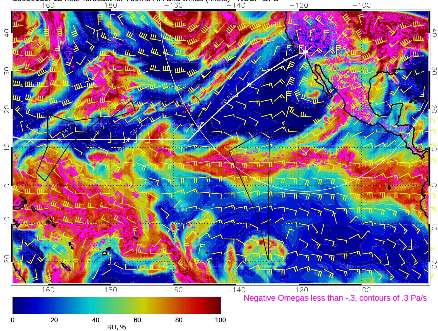
15020112, 12 hour forecast for 700mb RH and winds (knots) - NCEP GFS
