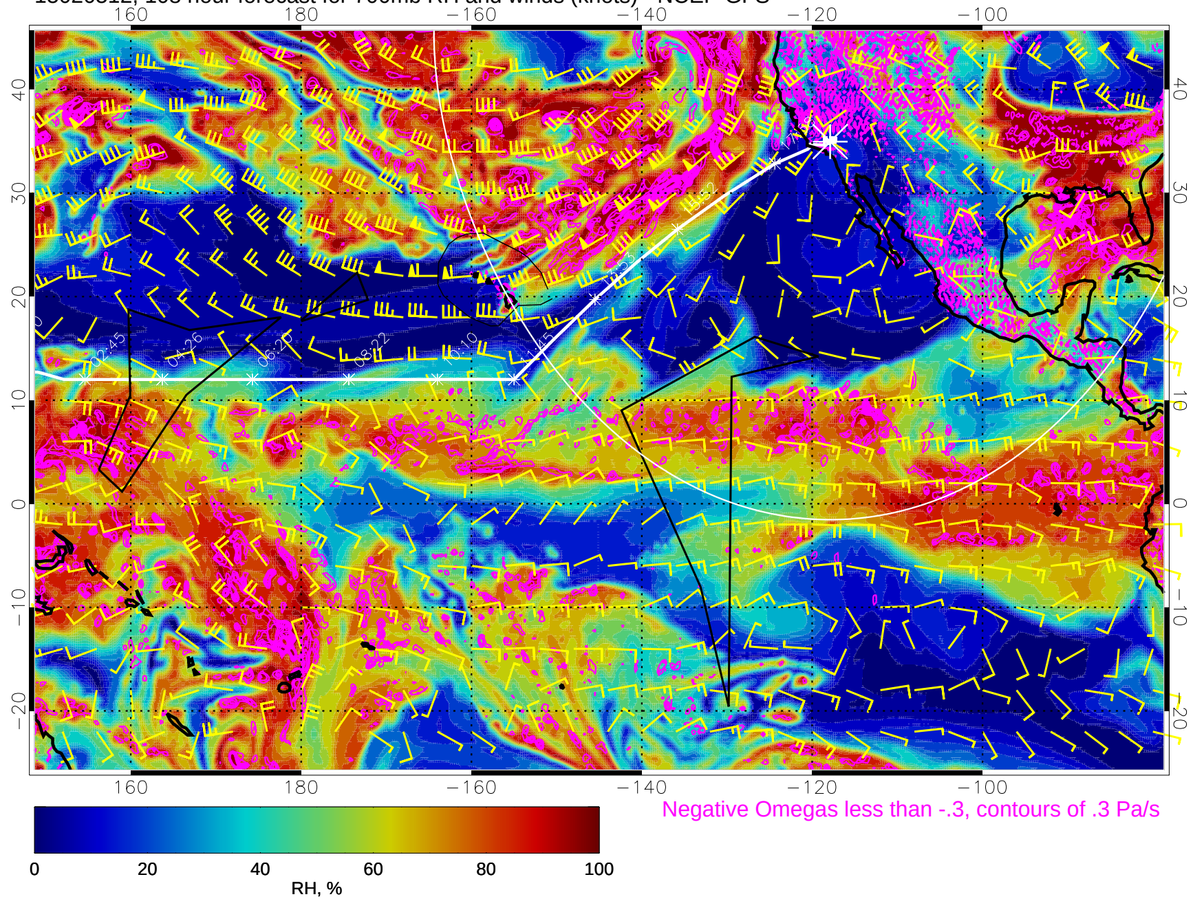
15020512, 108 hour forecast for 700mb RH and winds (knots) - NCEP GFS
