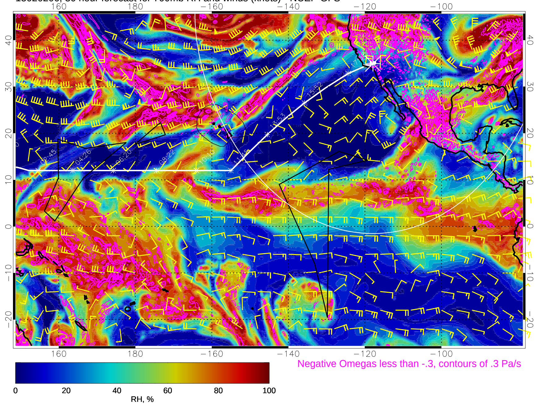
15020206, 30 hour forecast for 700mb RH and winds (knots) - NCEP GFS
