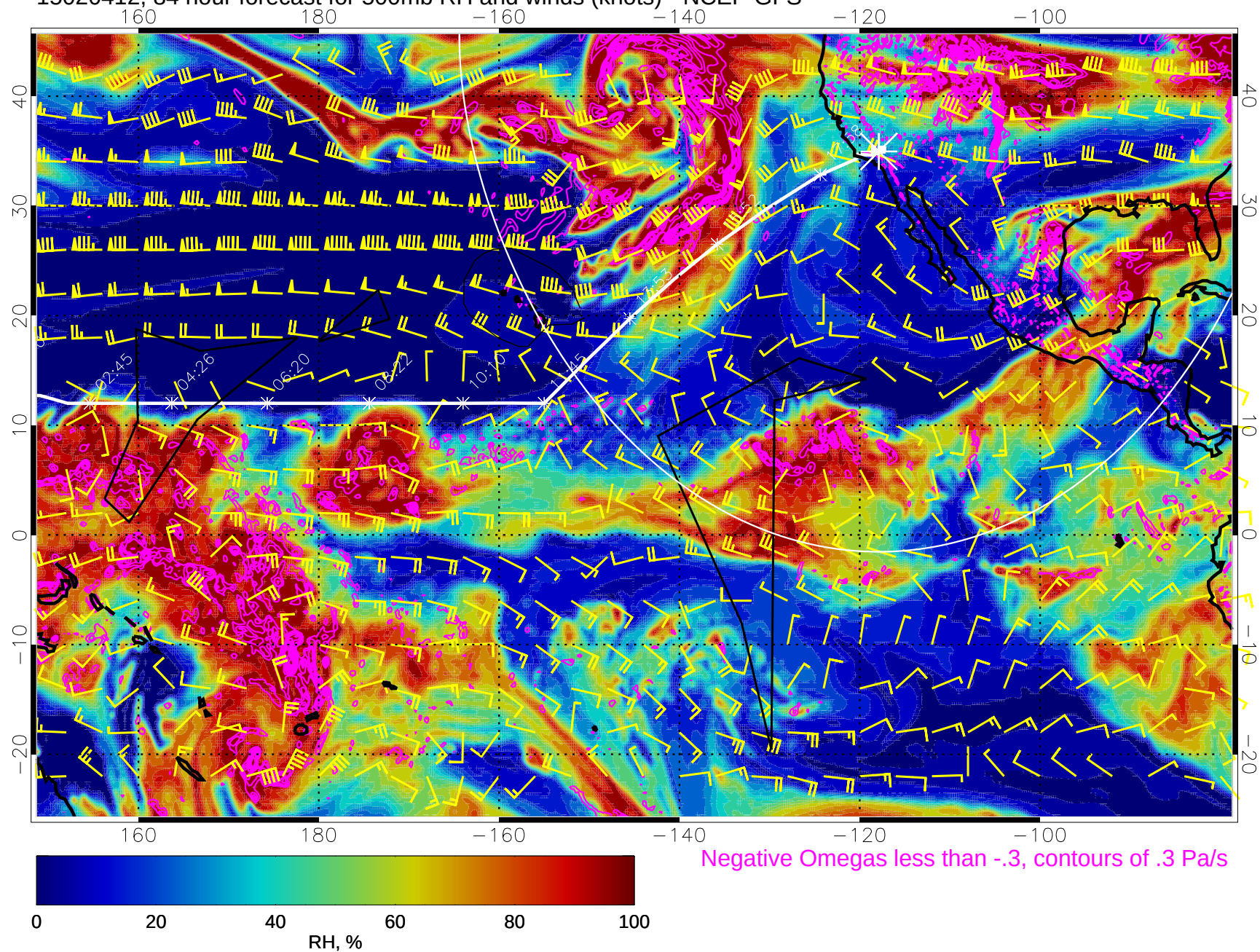
15020412, 84 hour forecast for 500mb RH and winds (knots) - NCEP GFS
