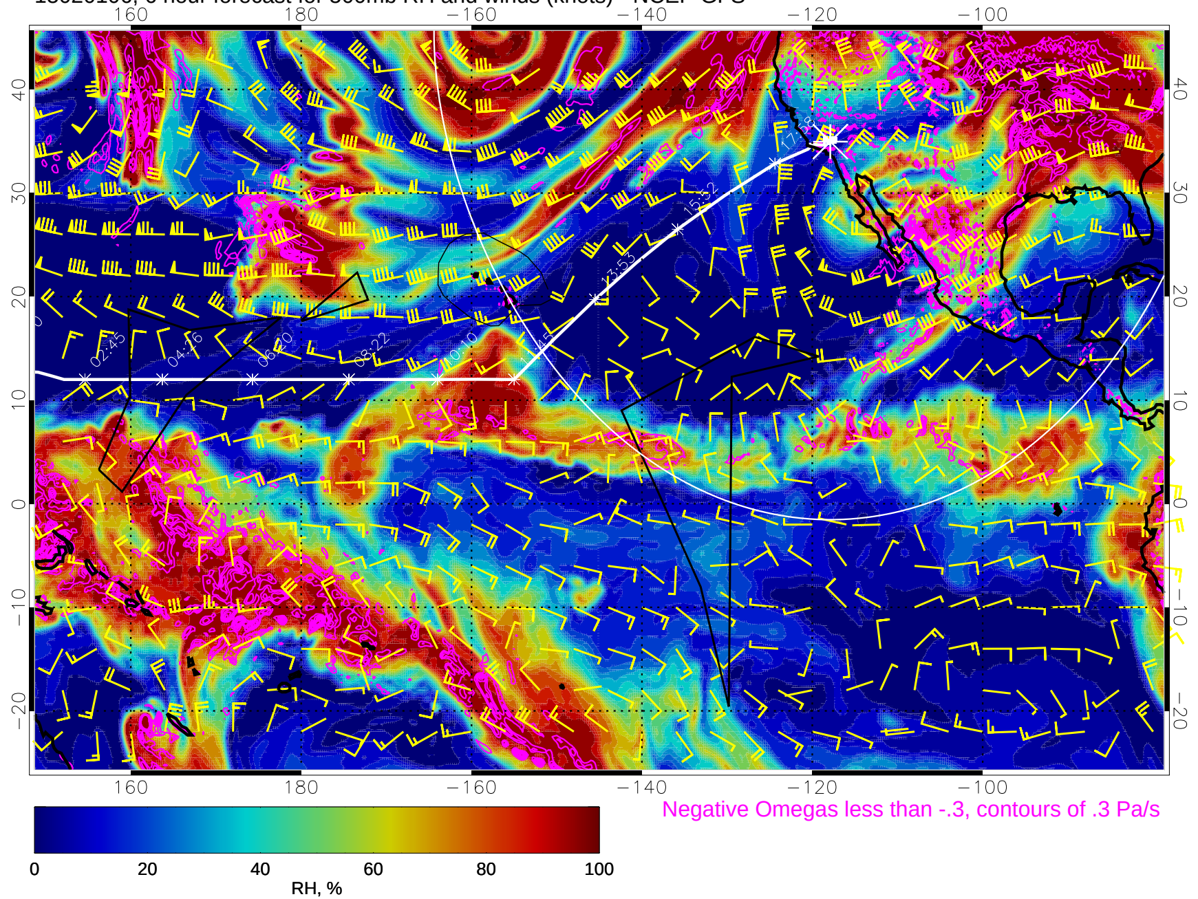
15020106, 6 hour forecast for 500mb RH and winds (knots) - NCEP GFS
