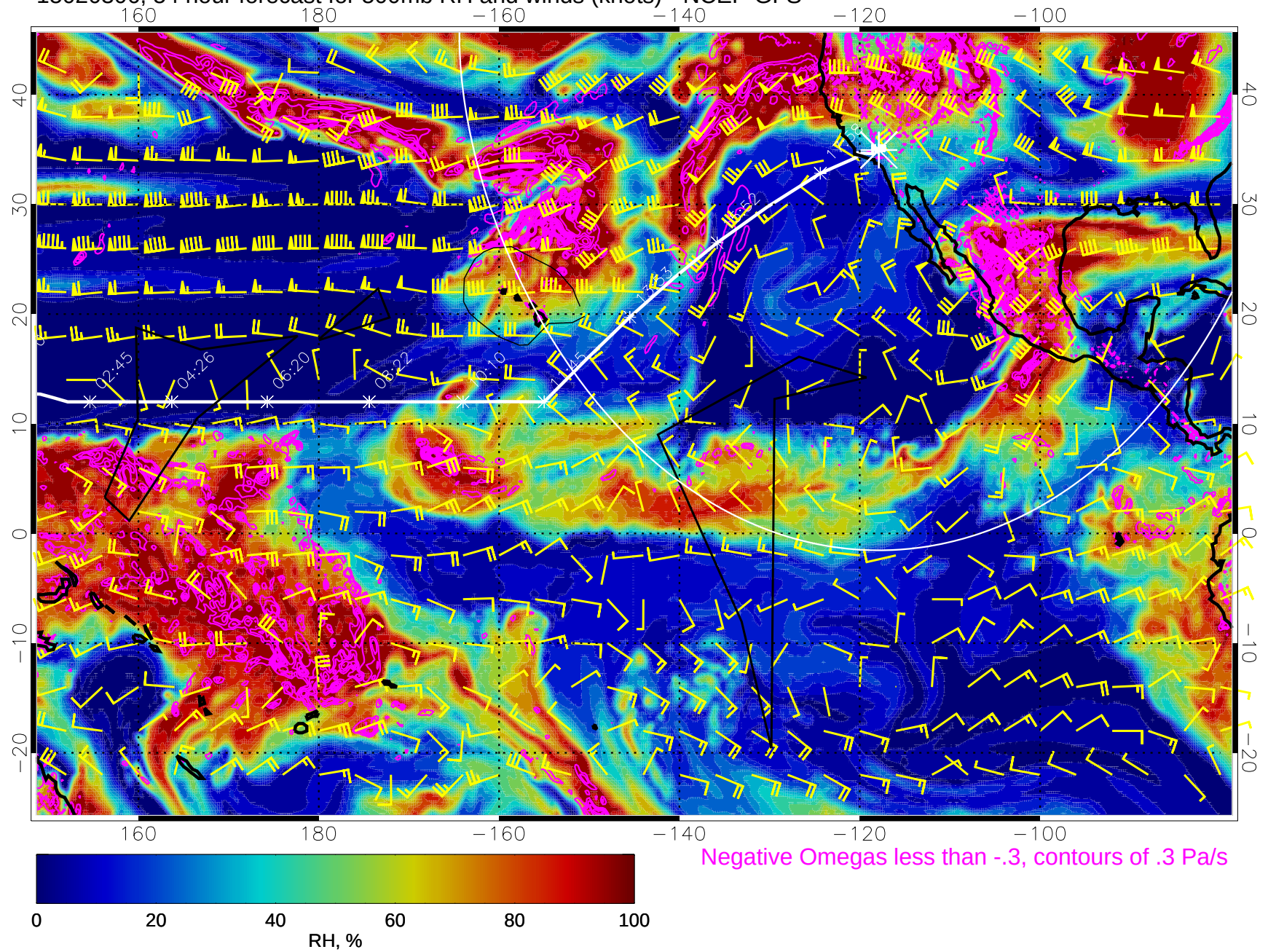
15020306, 54 hour forecast for 500mb RH and winds (knots) - NCEP GFS
