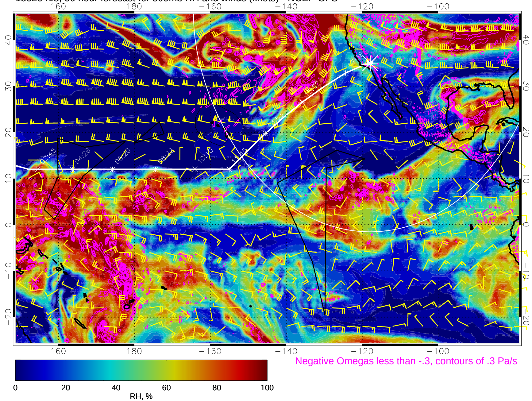
15020418, 90 hour forecast for 500mb RH and winds (knots) - NCEP GFS
