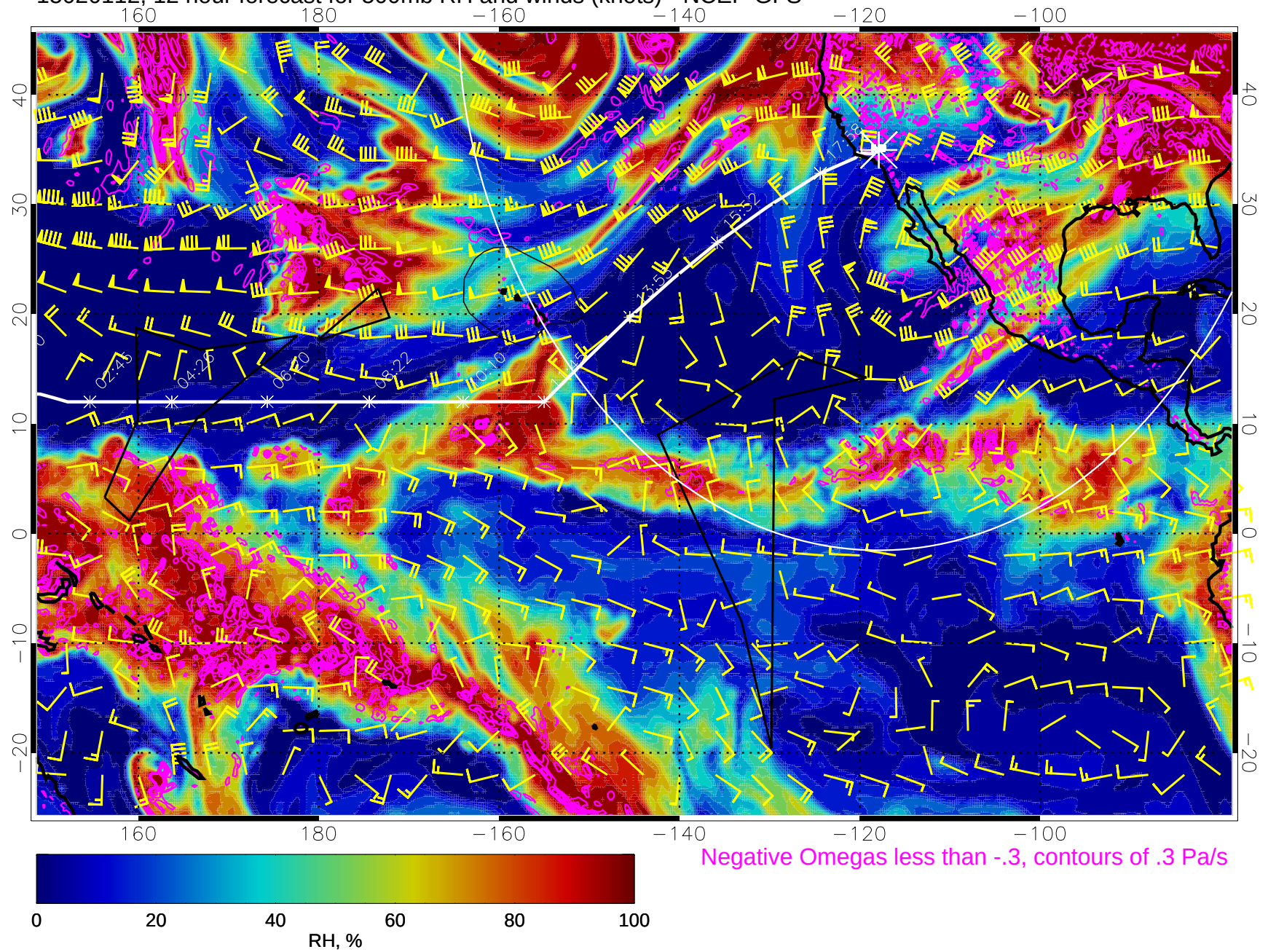
15020112, 12 hour forecast for 500mb RH and winds (knots) - NCEP GFS
