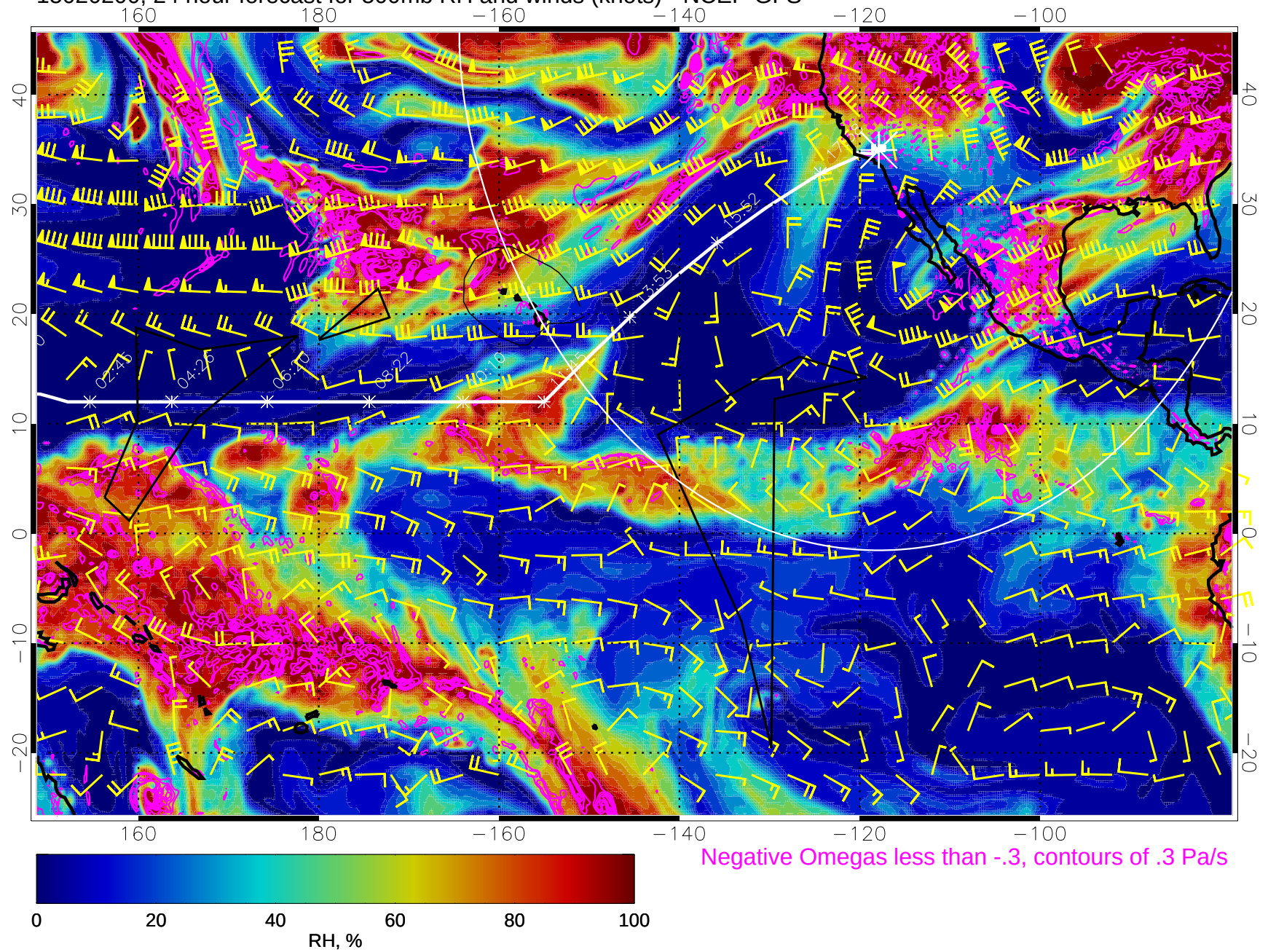
15020200, 24 hour forecast for 500mb RH and winds (knots) - NCEP GFS
