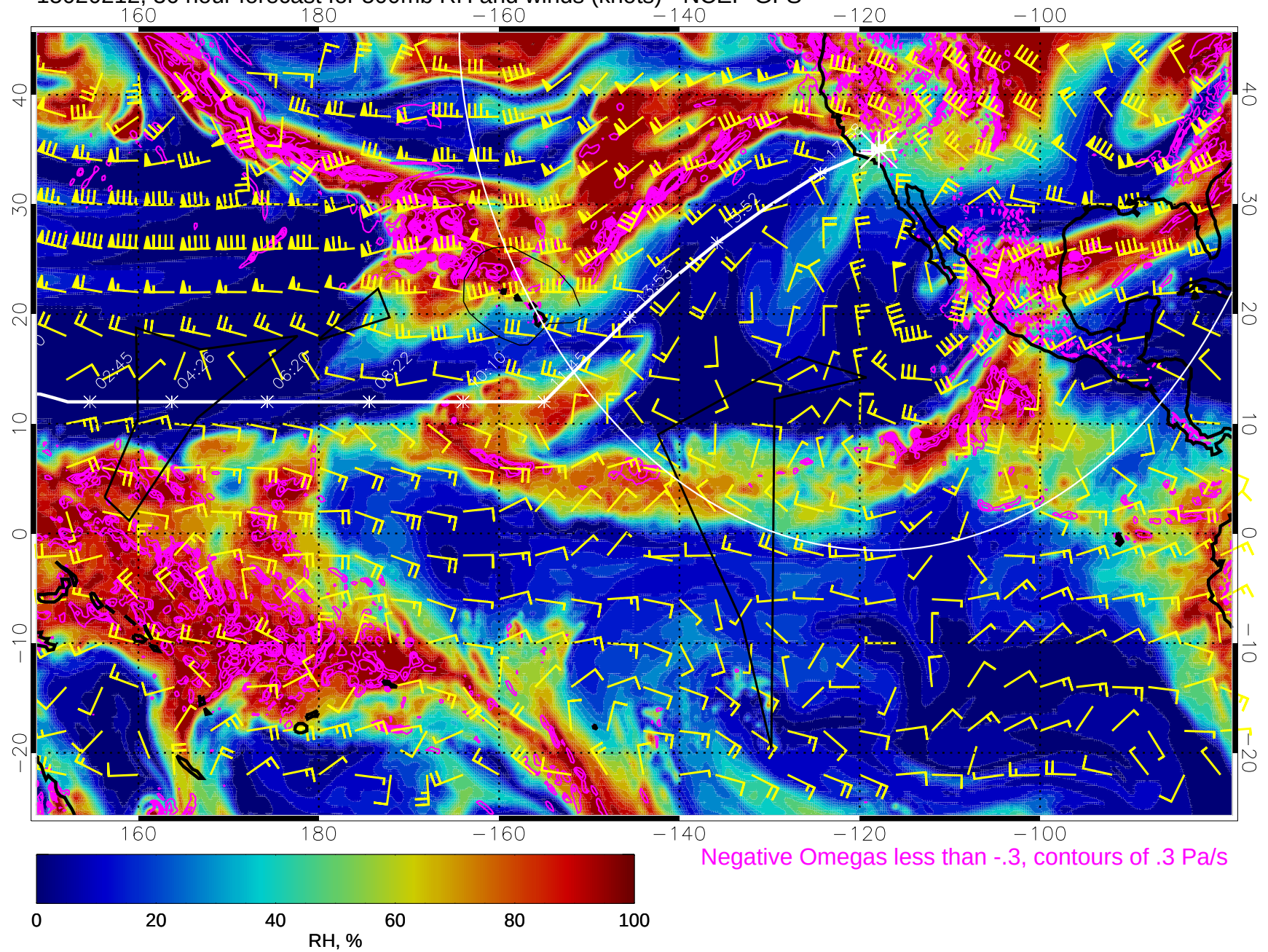
15020212, 36 hour forecast for 500mb RH and winds (knots) - NCEP GFS
