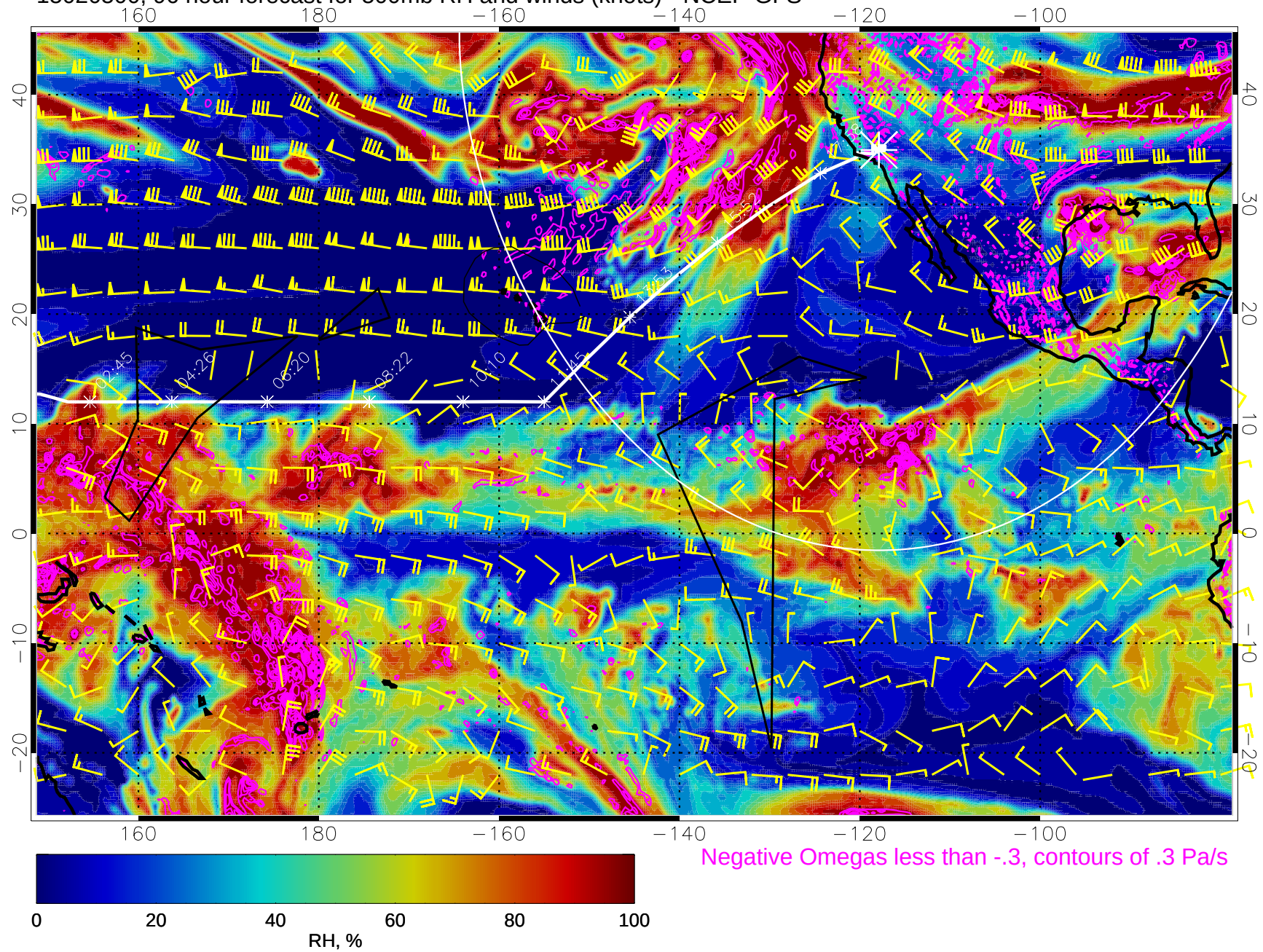
15020500, 96 hour forecast for 500mb RH and winds (knots) - NCEP GFS
