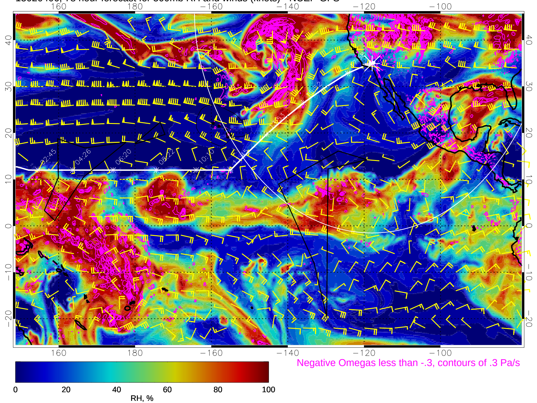
15020406, 78 hour forecast for 500mb RH and winds (knots) - NCEP GFS
