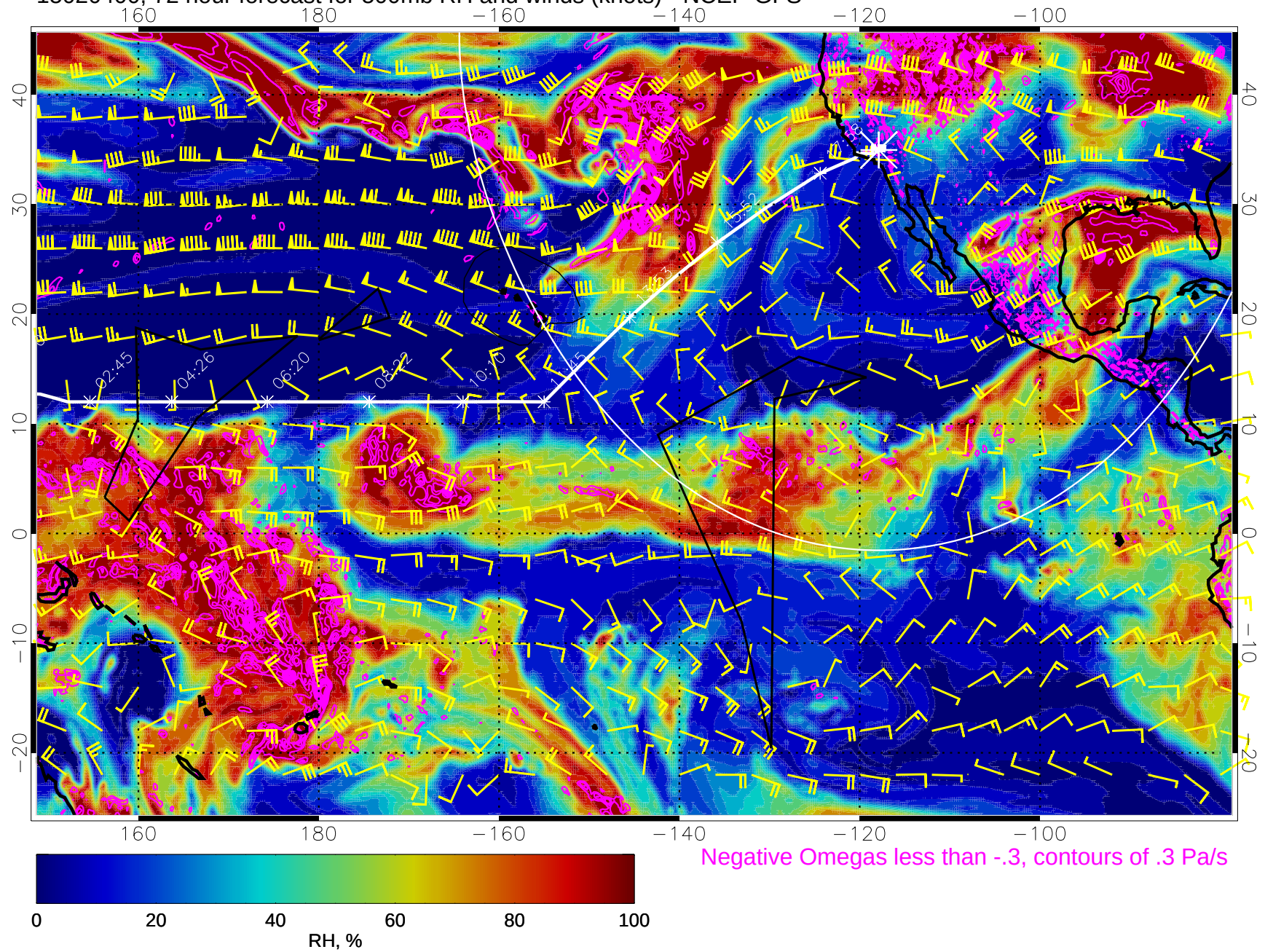
15020400, 72 hour forecast for 500mb RH and winds (knots) - NCEP GFS
