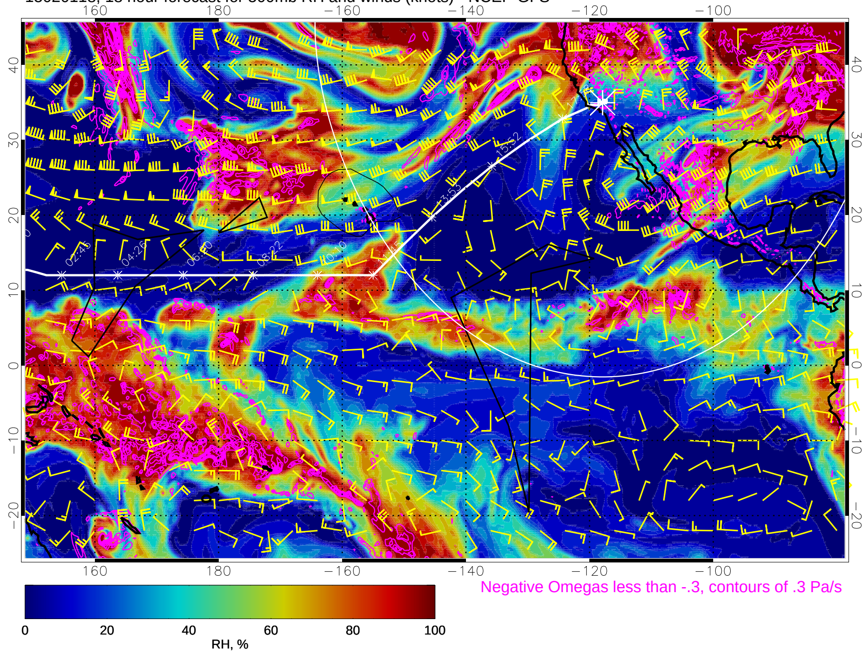
15020118, 18 hour forecast for 500mb RH and winds (knots) - NCEP GFS
