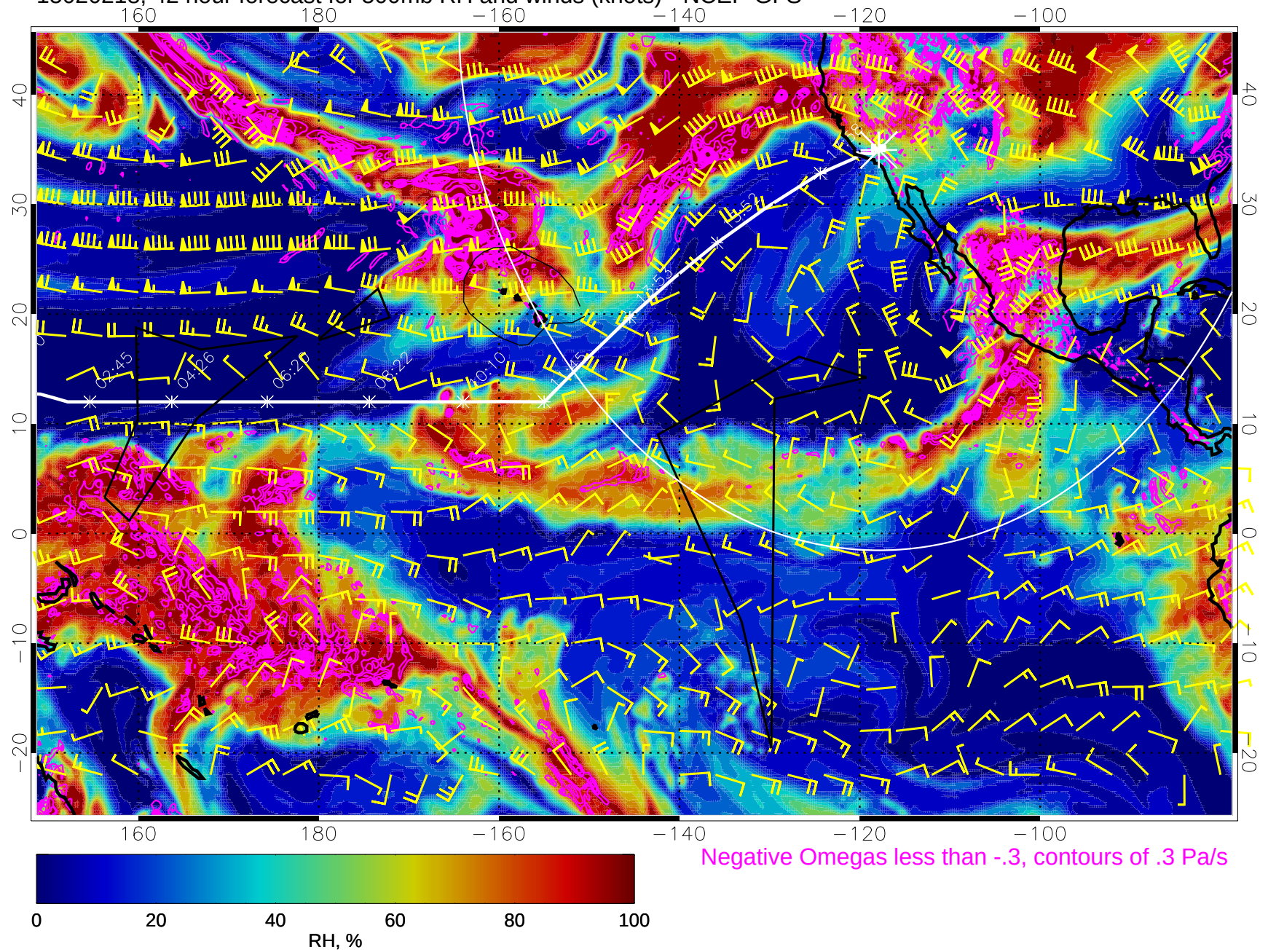
15020218, 42 hour forecast for 500mb RH and winds (knots) - NCEP GFS
