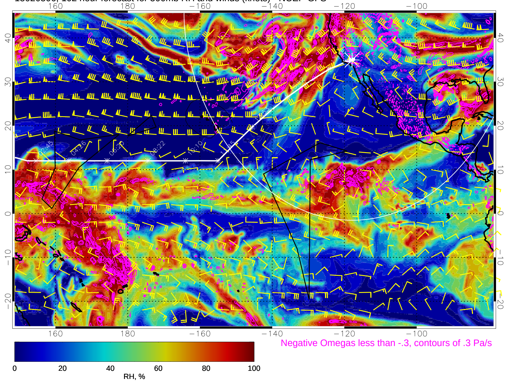
15020506, 102 hour forecast for 500mb RH and winds (knots) - NCEP GFS
