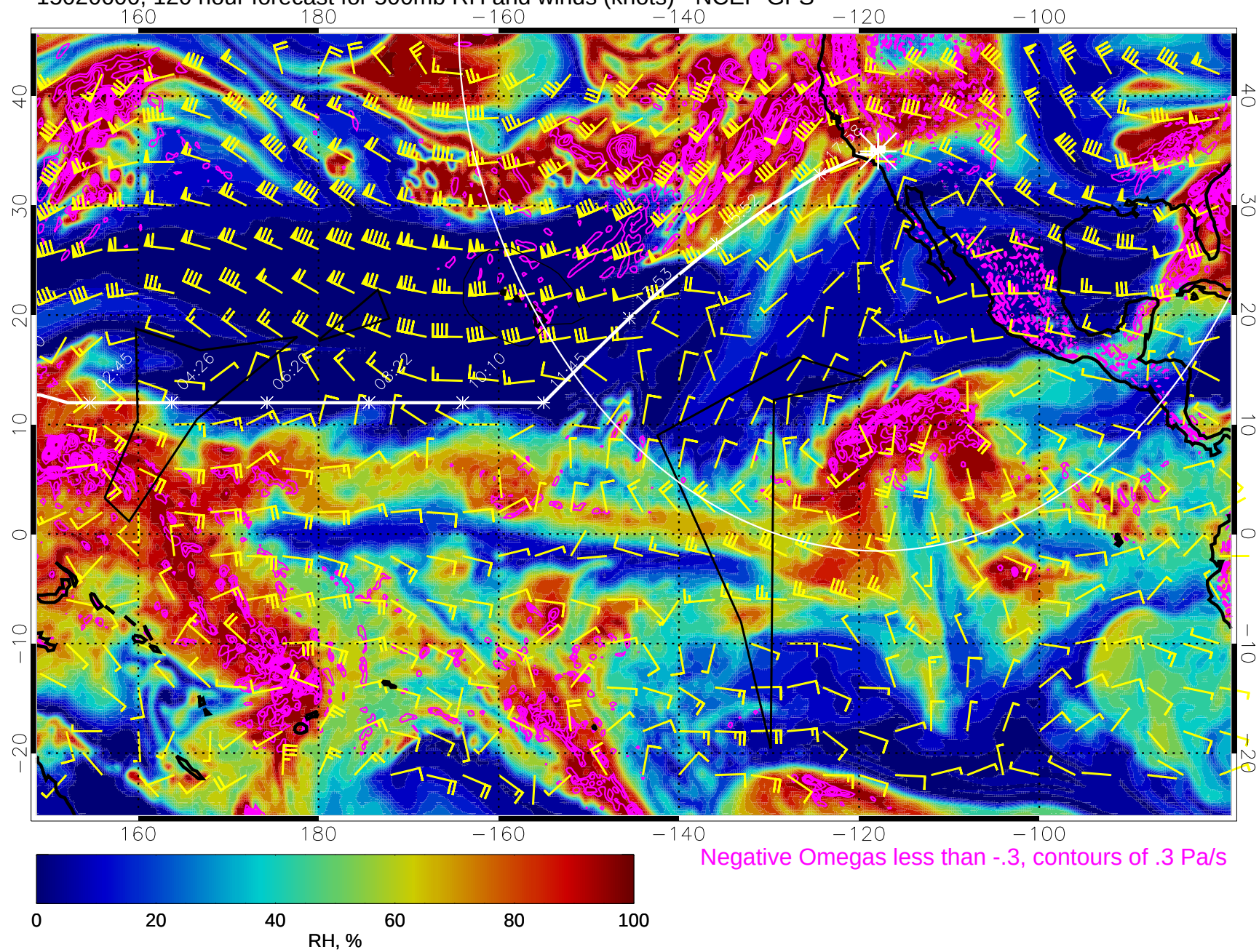
15020600, 120 hour forecast for 500mb RH and winds (knots) - NCEP GFS
