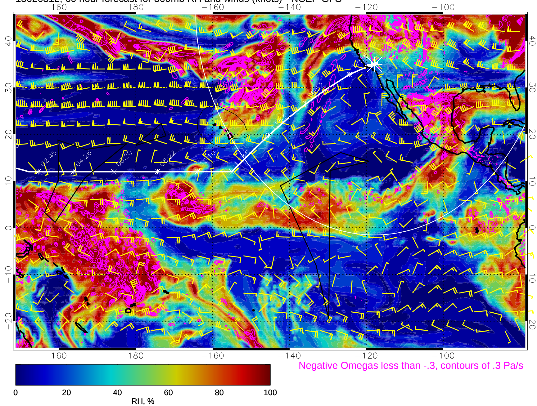
15020312, 60 hour forecast for 500mb RH and winds (knots) - NCEP GFS
