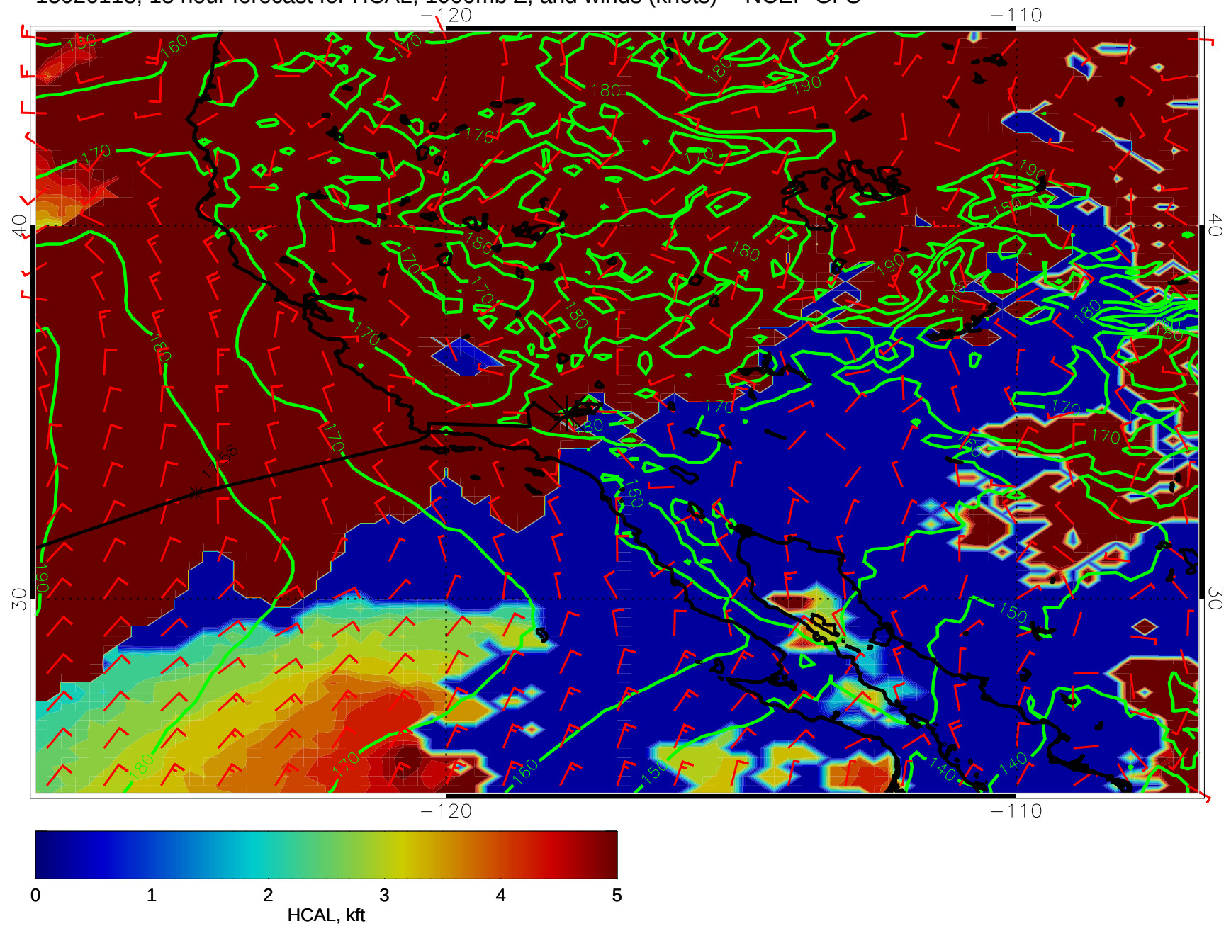
15020118, 18 hour forecast for HCAL, 1000mb Z, and winds (knots) -- NCEP GFS
