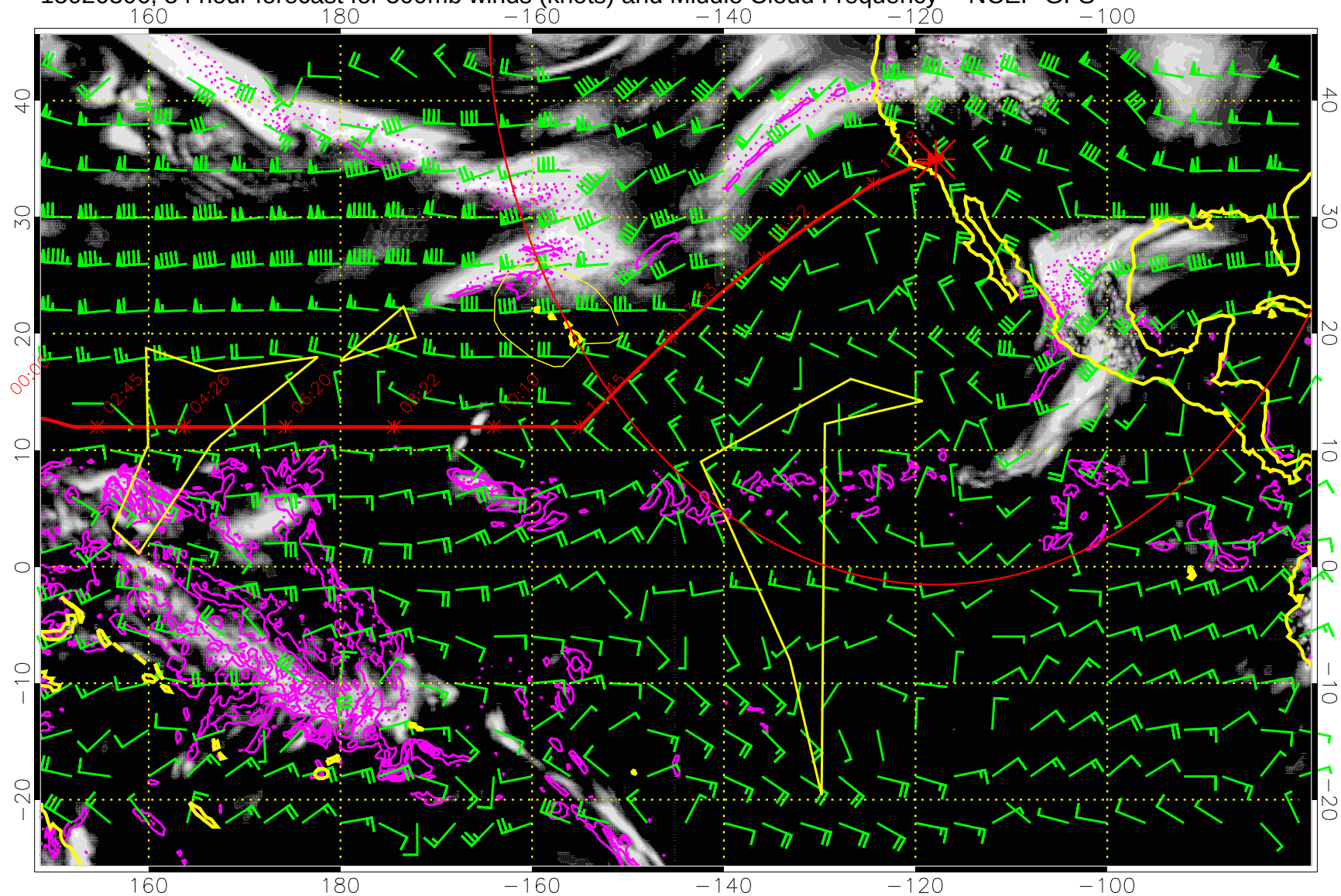
15020306, 54 hour forecast for 500mb winds (knots) and Middle Cloud Frequency -- NCEP GFS
