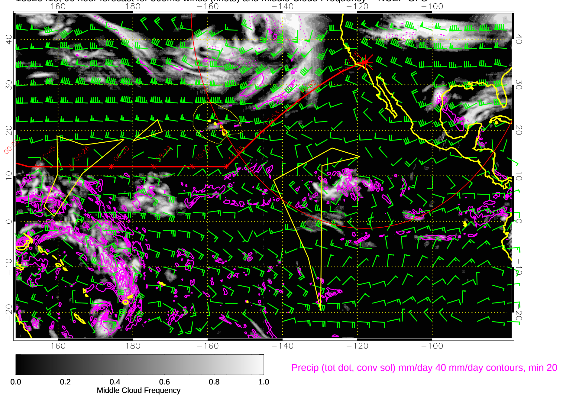
15020418, 90 hour forecast for 500mb winds (knots) and Middle Cloud Frequency -- NCEP GFS
