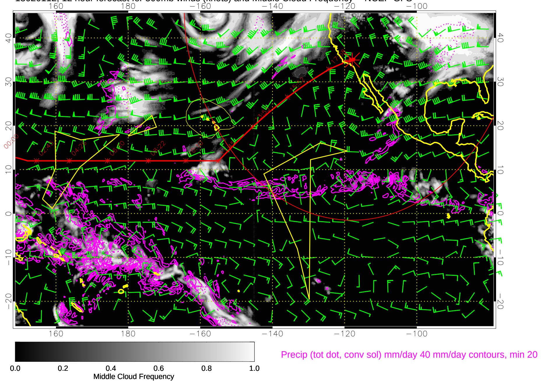
15020112, 12 hour forecast for 500mb winds (knots) and Middle Cloud Frequency -- NCEP GFS
