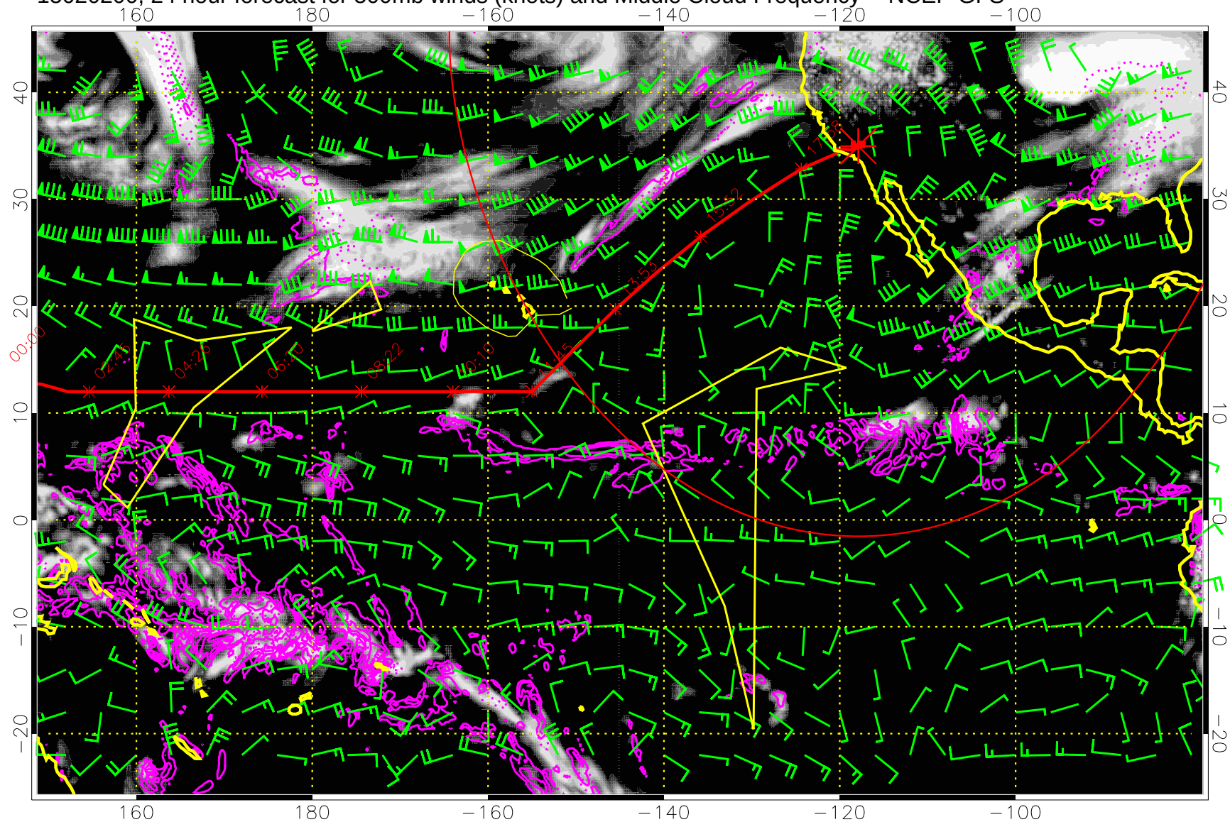
15020200, 24 hour forecast for 500mb winds (knots) and Middle Cloud Frequency -- NCEP GFS
