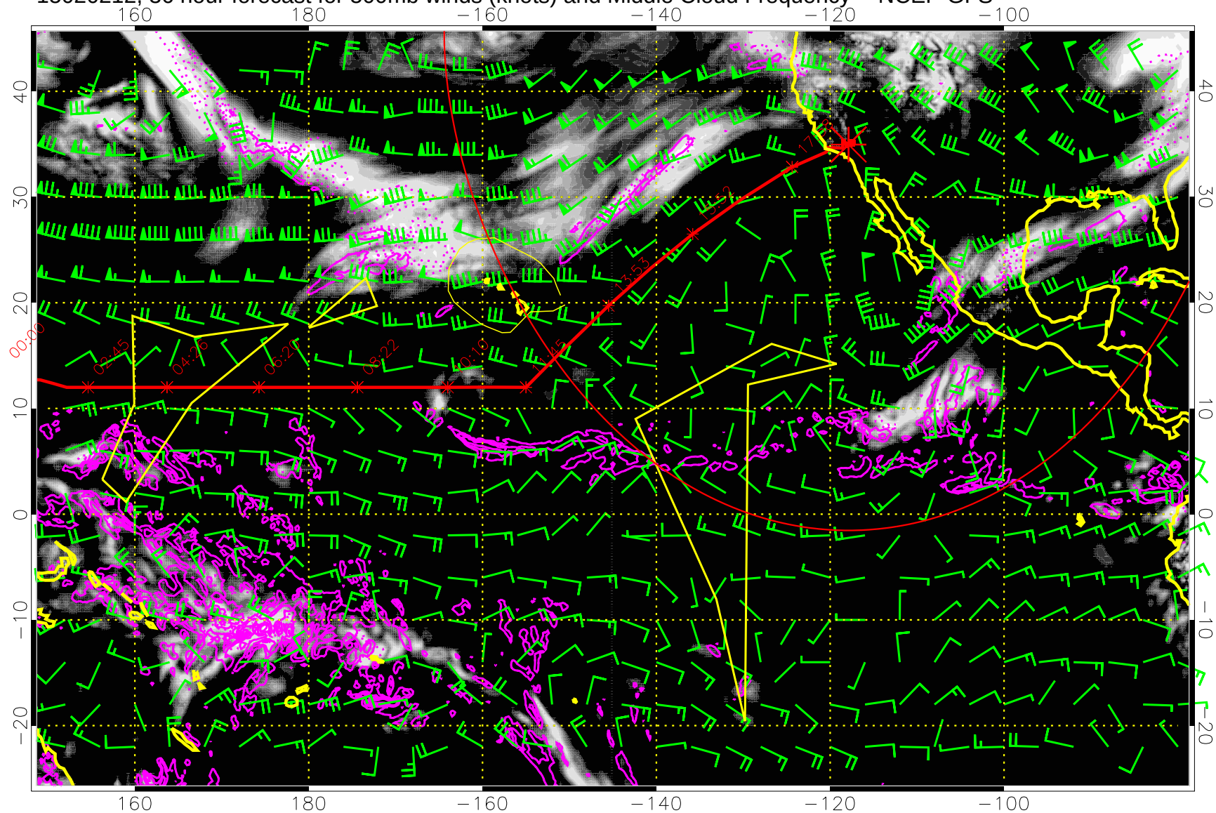
15020212, 36 hour forecast for 500mb winds (knots) and Middle Cloud Frequency -- NCEP GFS
