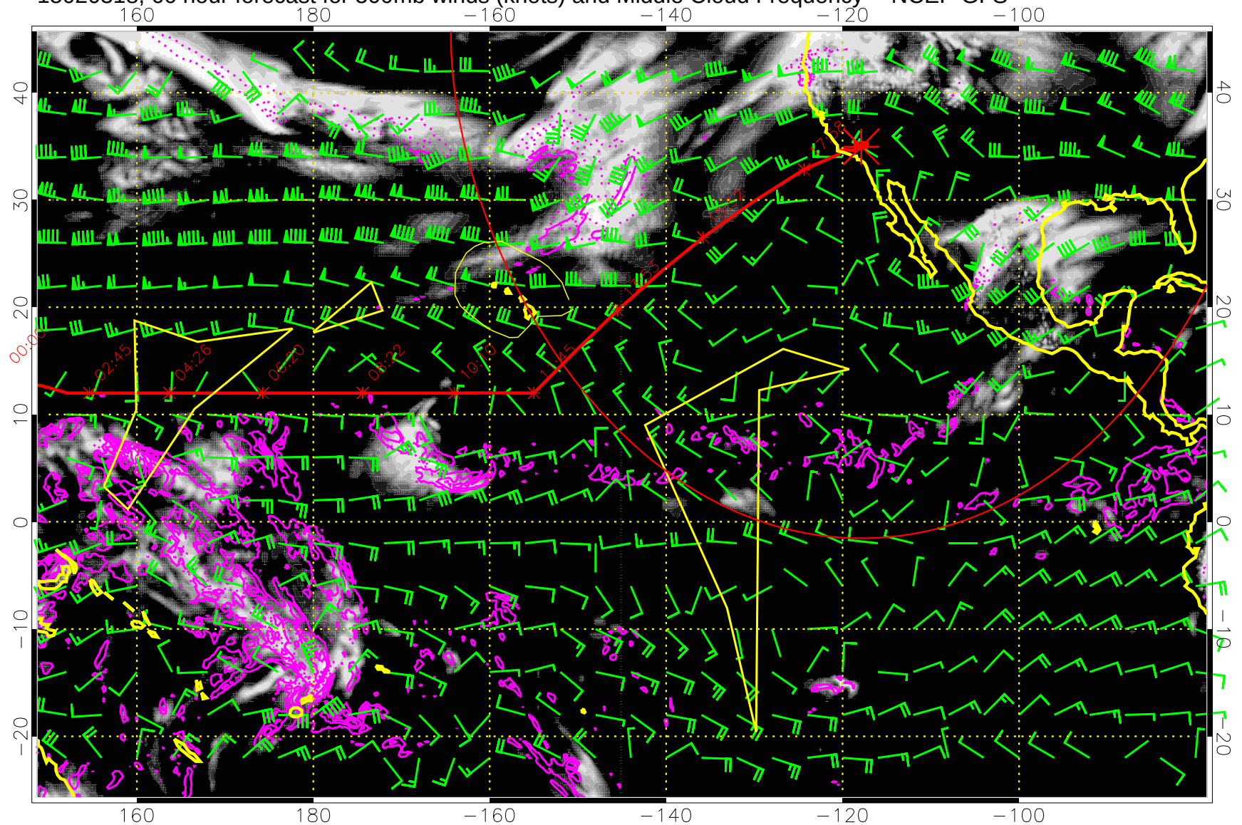
15020318, 66 hour forecast for 500mb winds (knots) and Middle Cloud Frequency -- NCEP GFS
