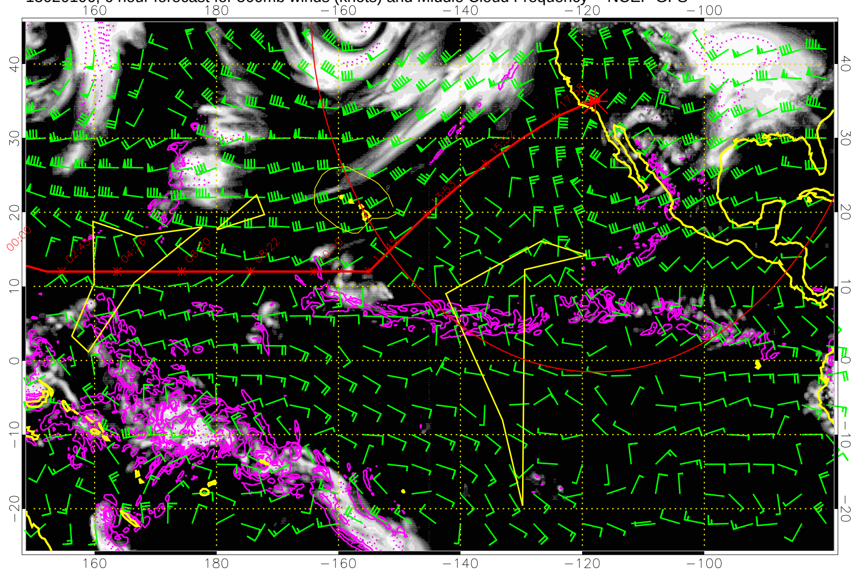
15020106, 6 hour forecast for 500mb winds (knots) and Middle Cloud Frequency -- NCEP GFS
