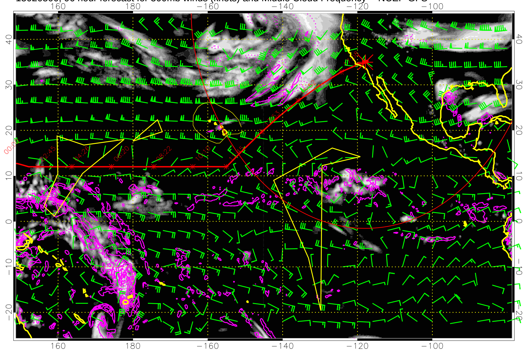
15020500, 96 hour forecast for 500mb winds (knots) and Middle Cloud Frequency -- NCEP GFS
