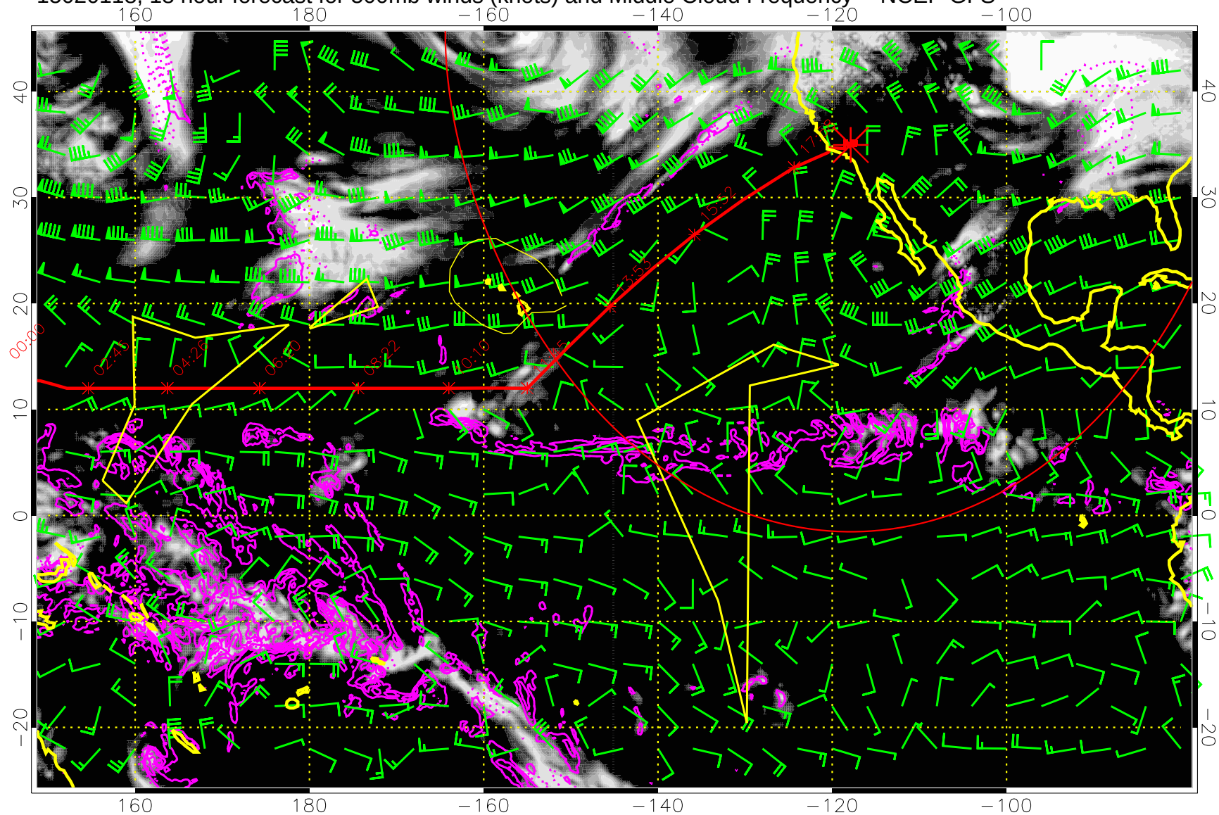
15020118, 18 hour forecast for 500mb winds (knots) and Middle Cloud Frequency -- NCEP GFS
