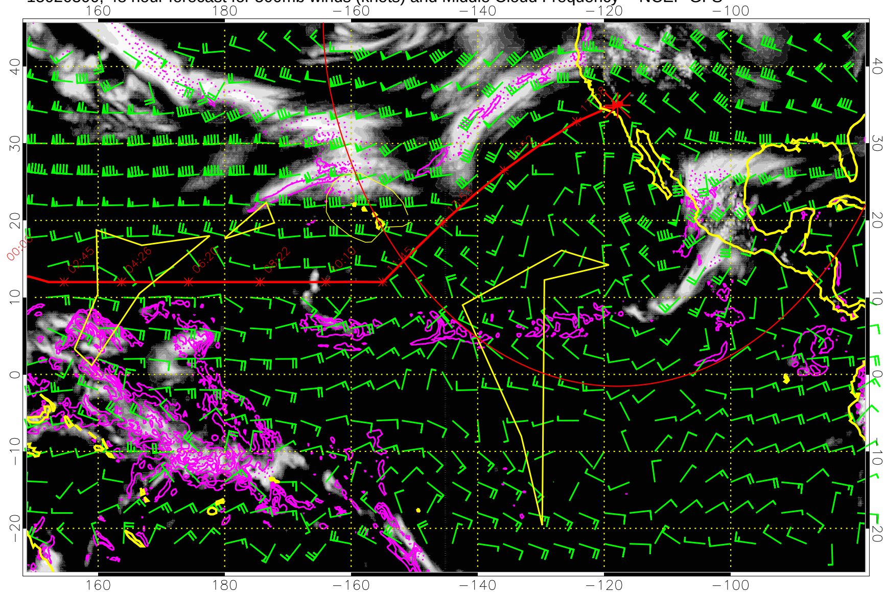
15020300, 48 hour forecast for 500mb winds (knots) and Middle Cloud Frequency -- NCEP GFS
