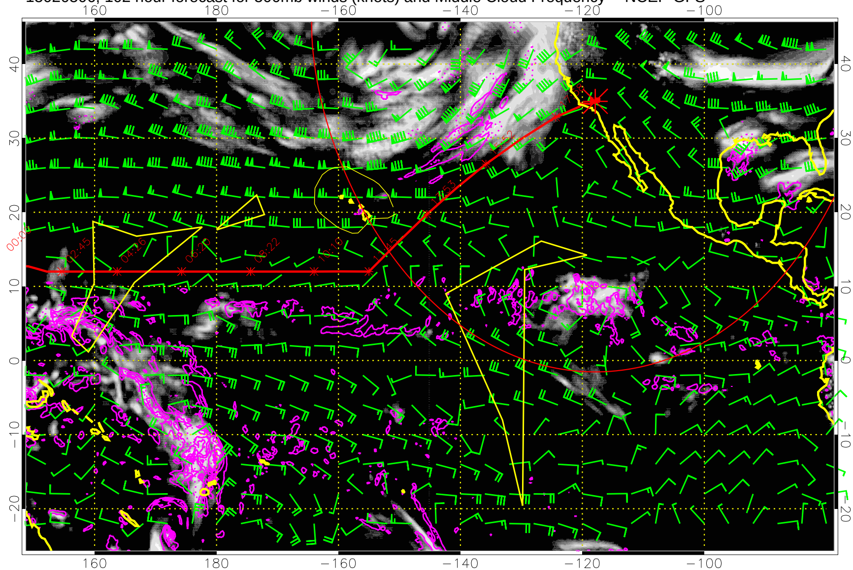
15020506, 102 hour forecast for 500mb winds (knots) and Middle Cloud Frequency -- NCEP GFS
