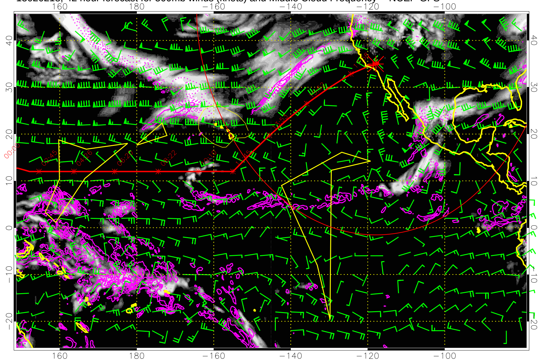
15020218, 42 hour forecast for 500mb winds (knots) and Middle Cloud Frequency -- NCEP GFS
