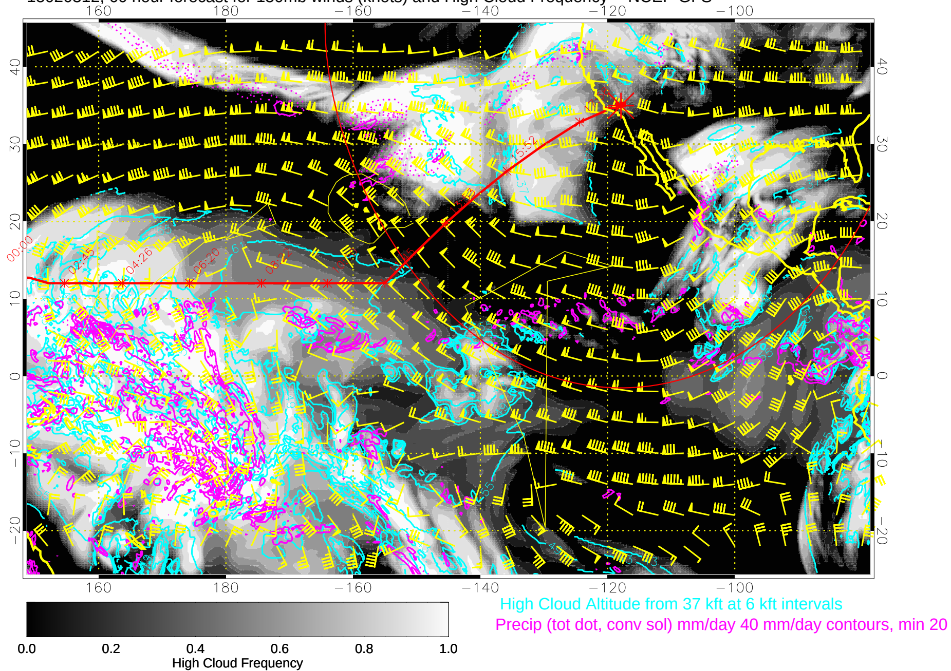
15020312, 60 hour forecast for 150mb winds (knots) and High Cloud Frequency -- NCEP GFS
