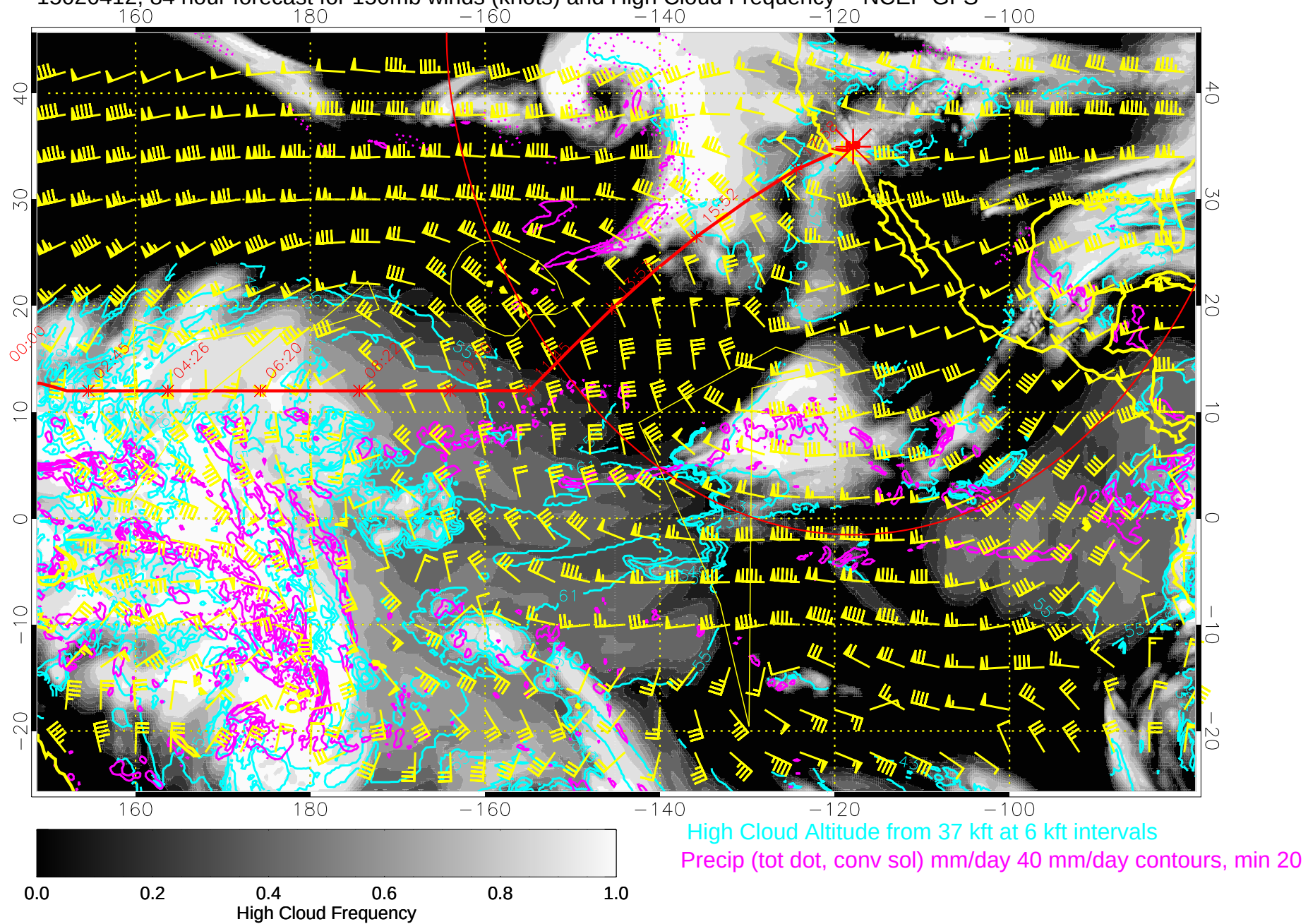
15020412, 84 hour forecast for 150mb winds (knots) and High Cloud Frequency -- NCEP GFS
