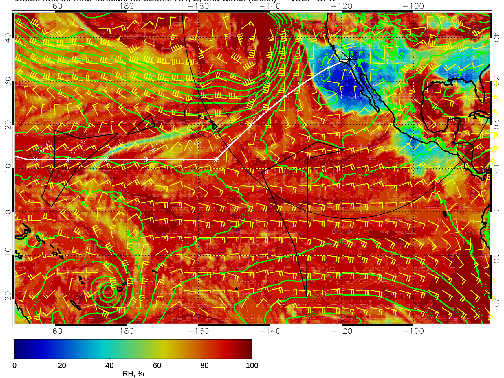
15020406, 90 hour forecast for 925mb RH, Z, and winds (knots) -- NCEP GFS
