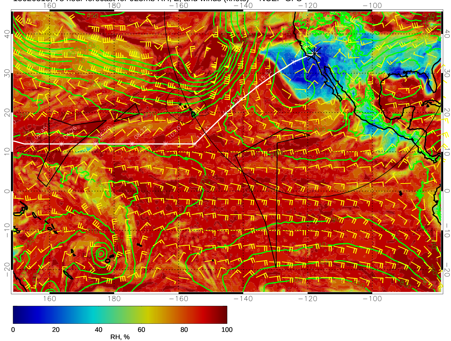
15020318, 78 hour forecast for 925mb RH, Z, and winds (knots) -- NCEP GFS
