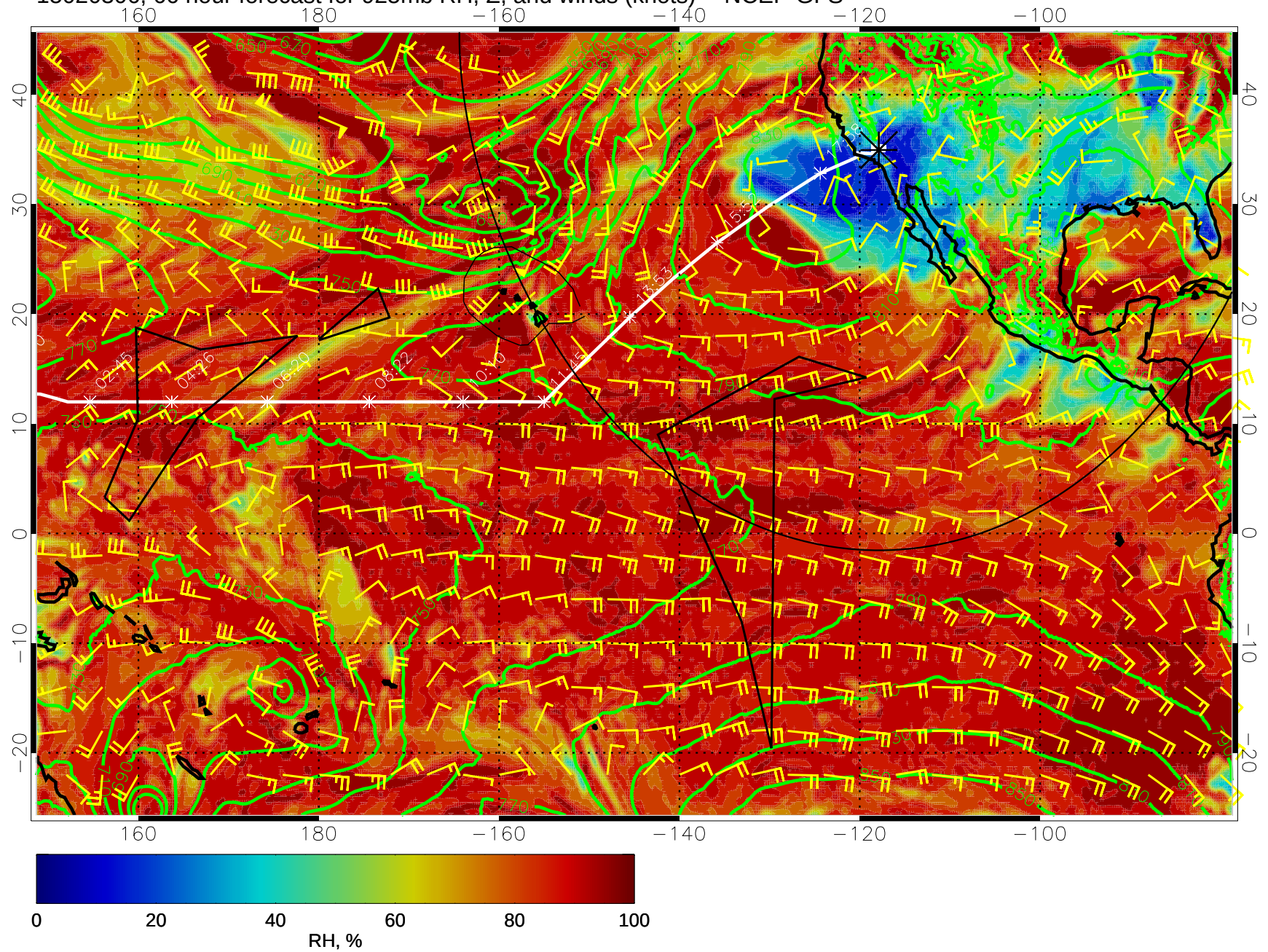
15020306, 66 hour forecast for 925mb RH, Z, and winds (knots) -- NCEP GFS
