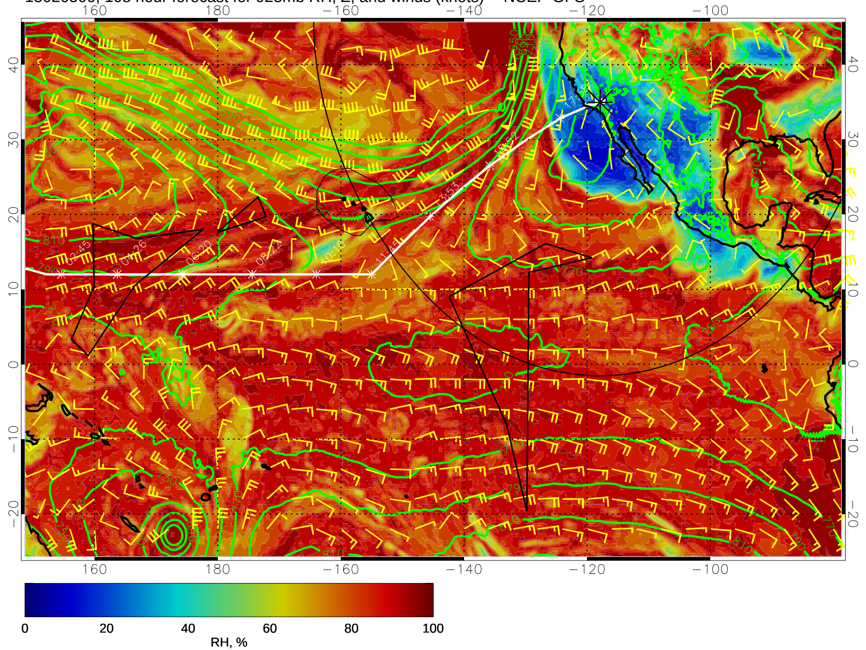
15020500, 108 hour forecast for 925mb RH, Z, and winds (knots) -- NCEP GFS
