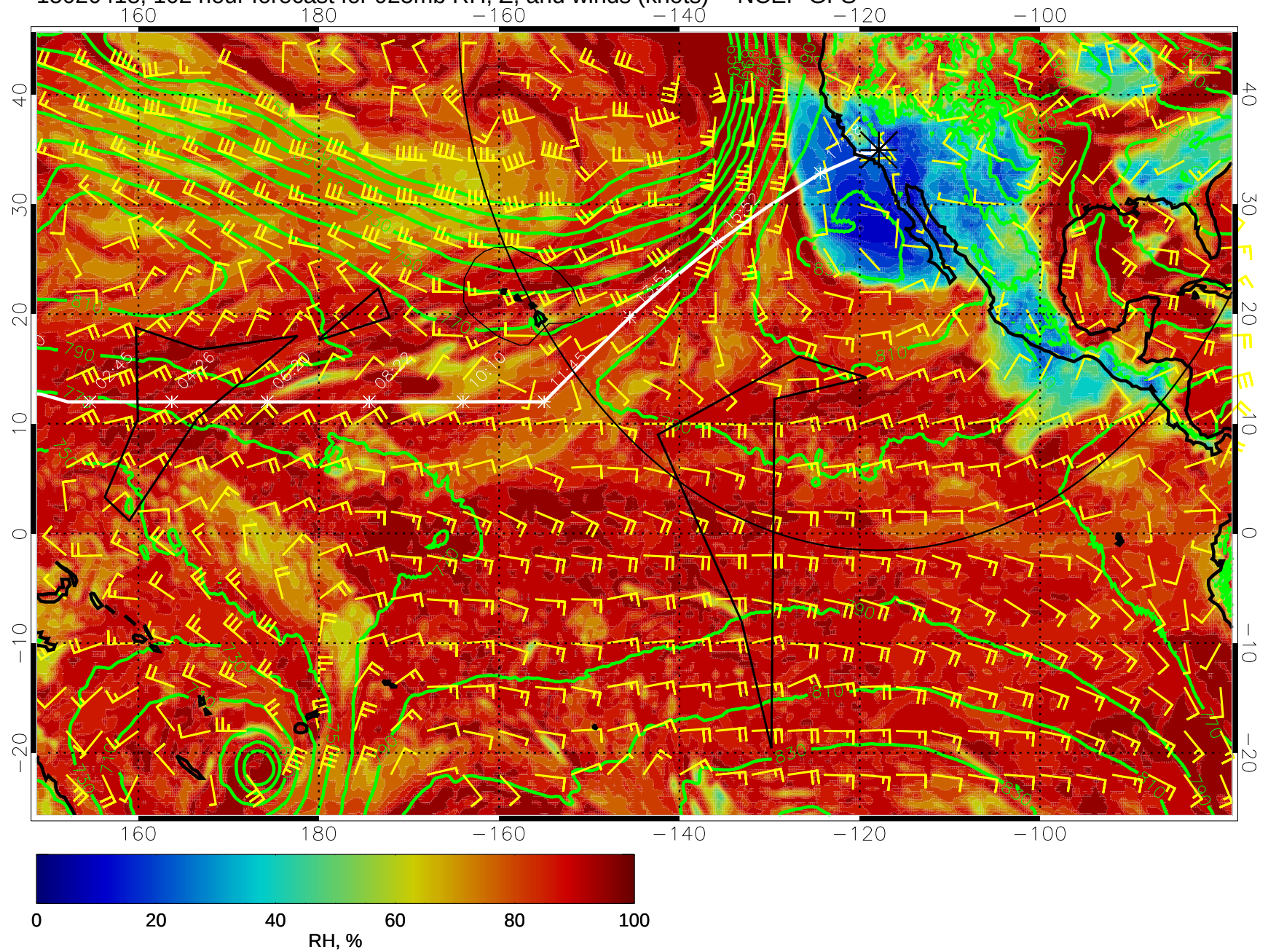
15020418, 102 hour forecast for 925mb RH, Z, and winds (knots) -- NCEP GFS
