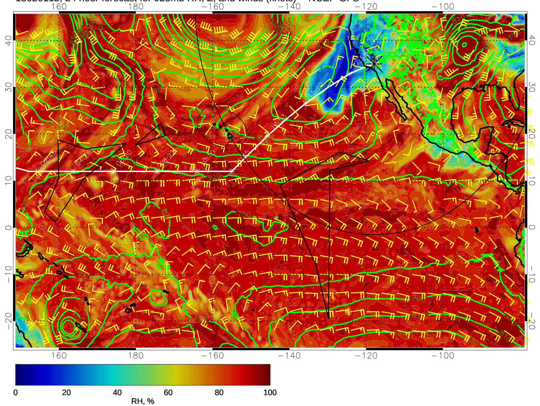
15020112, 24 hour forecast for 925mb RH, Z, and winds (knots) -- NCEP GFS
