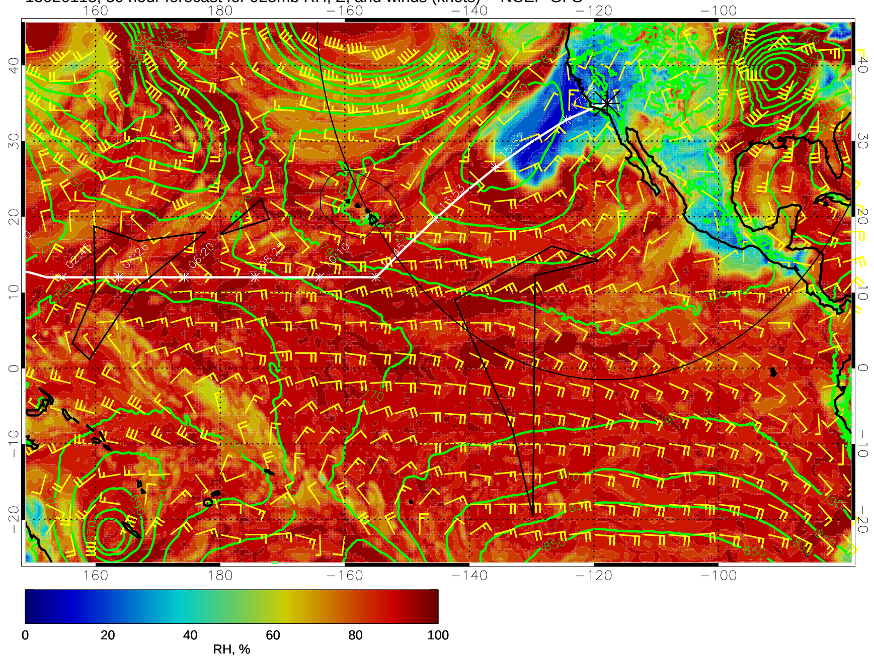
15020118, 30 hour forecast for 925mb RH, Z, and winds (knots) -- NCEP GFS
