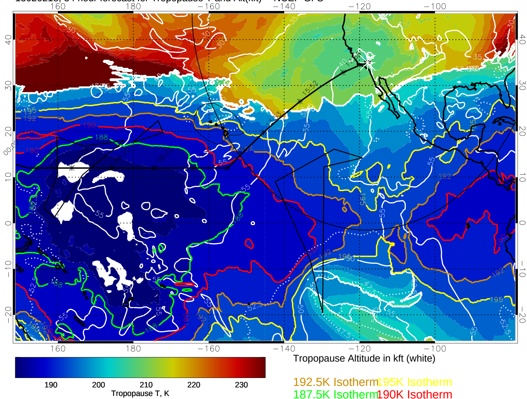
15020218, 54 hour forecast for Tropopause T and Alt(kft) -- NCEP GFS
